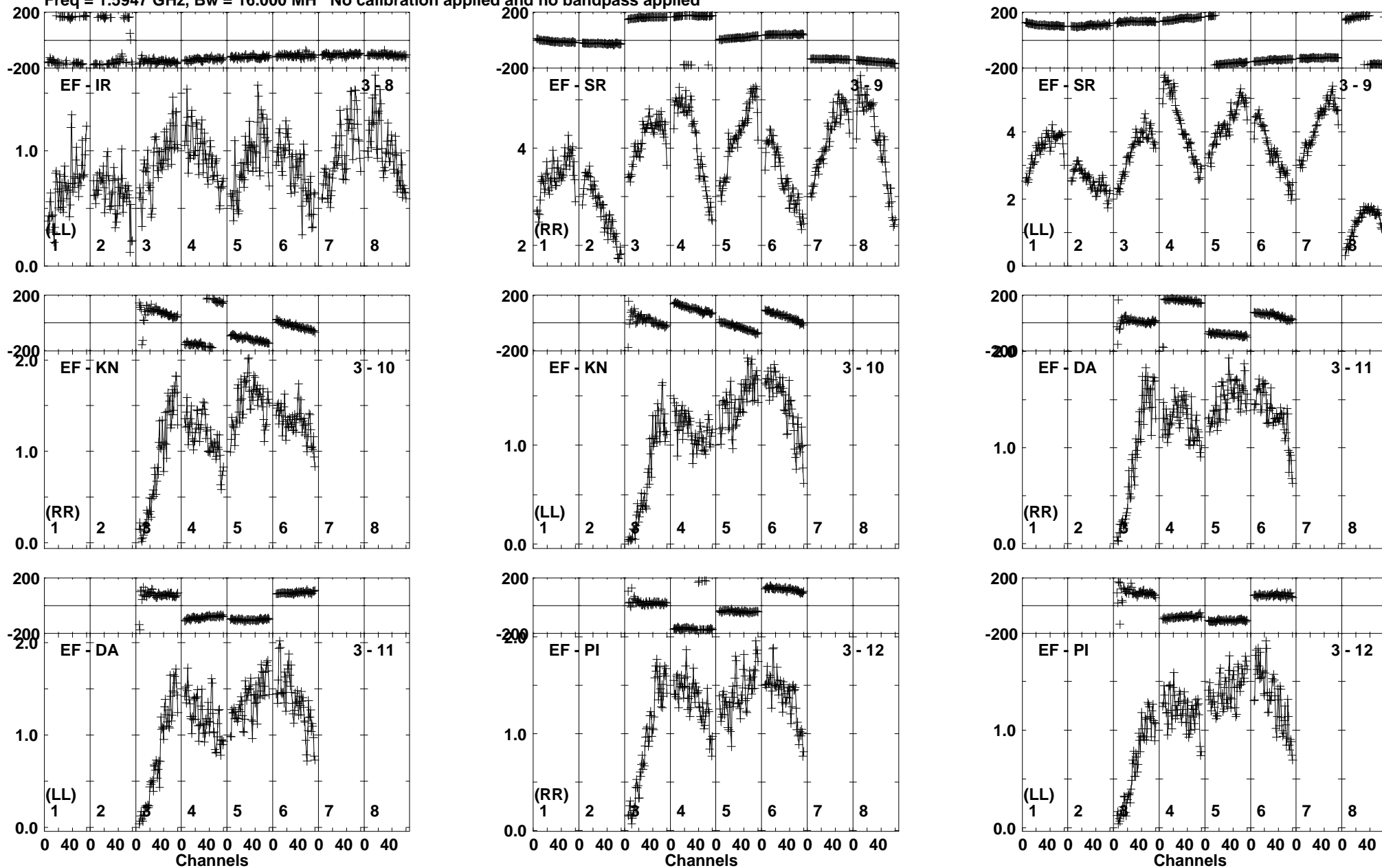
Lower frame: Milli Ampl Jy Top frame: Phas deg Vector averaged cross-power spectrum Baseline: EF (03) - IR (08) Timerange: 01/00:04:41 to 01/00:05:39
