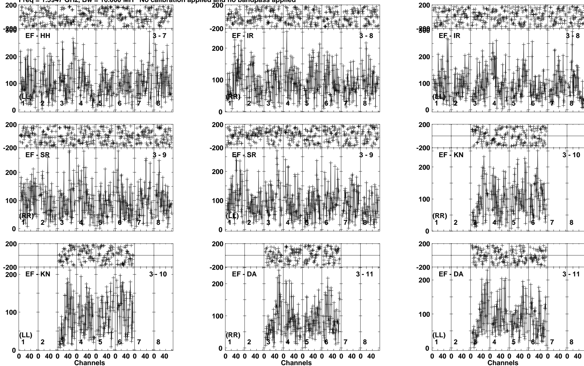
Lower frame: Micro Ampl Jy Top frame: Phas deg Vector averaged cross-power spectrum Baseline: EF (03) - HH (07) Timerange: 00/23:39:41 to 00/23:44:40
