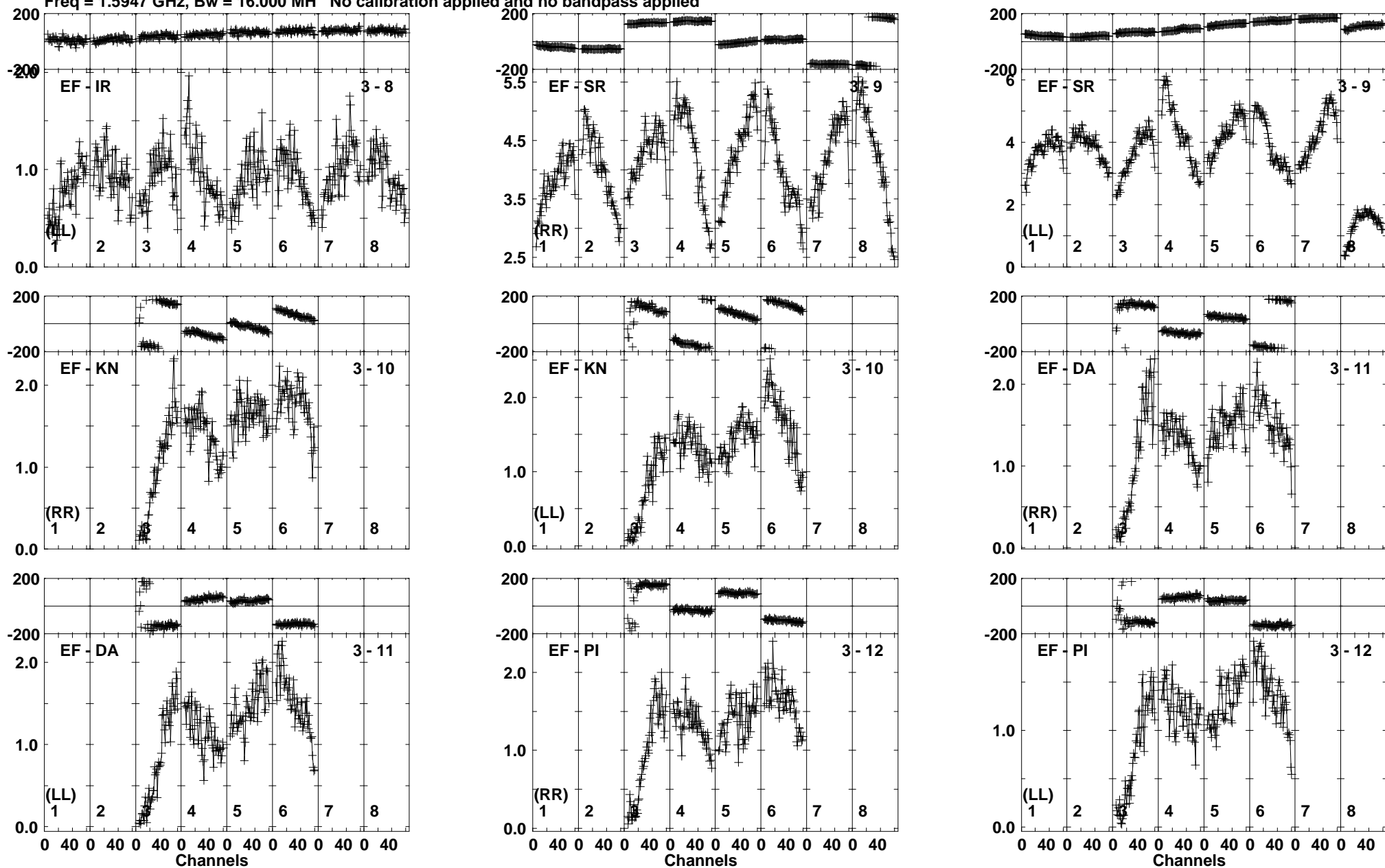
Lower frame: Milli Ampl Jy Top frame: Phas deg Vector averaged cross-power spectrum Baseline: EF (03) - IR (08) Timerange: 01/00:58:31 to 01/00:59:59
