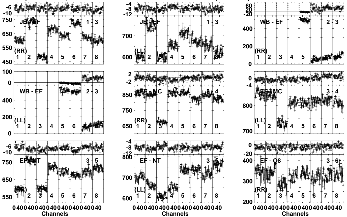
Lower frame: Milli Ampl Jy Top frame: Phas deg Vector averaged cross-power spectrum Several baselines displayed Timerange: 00/09:26:51 to 00/09:27:49
