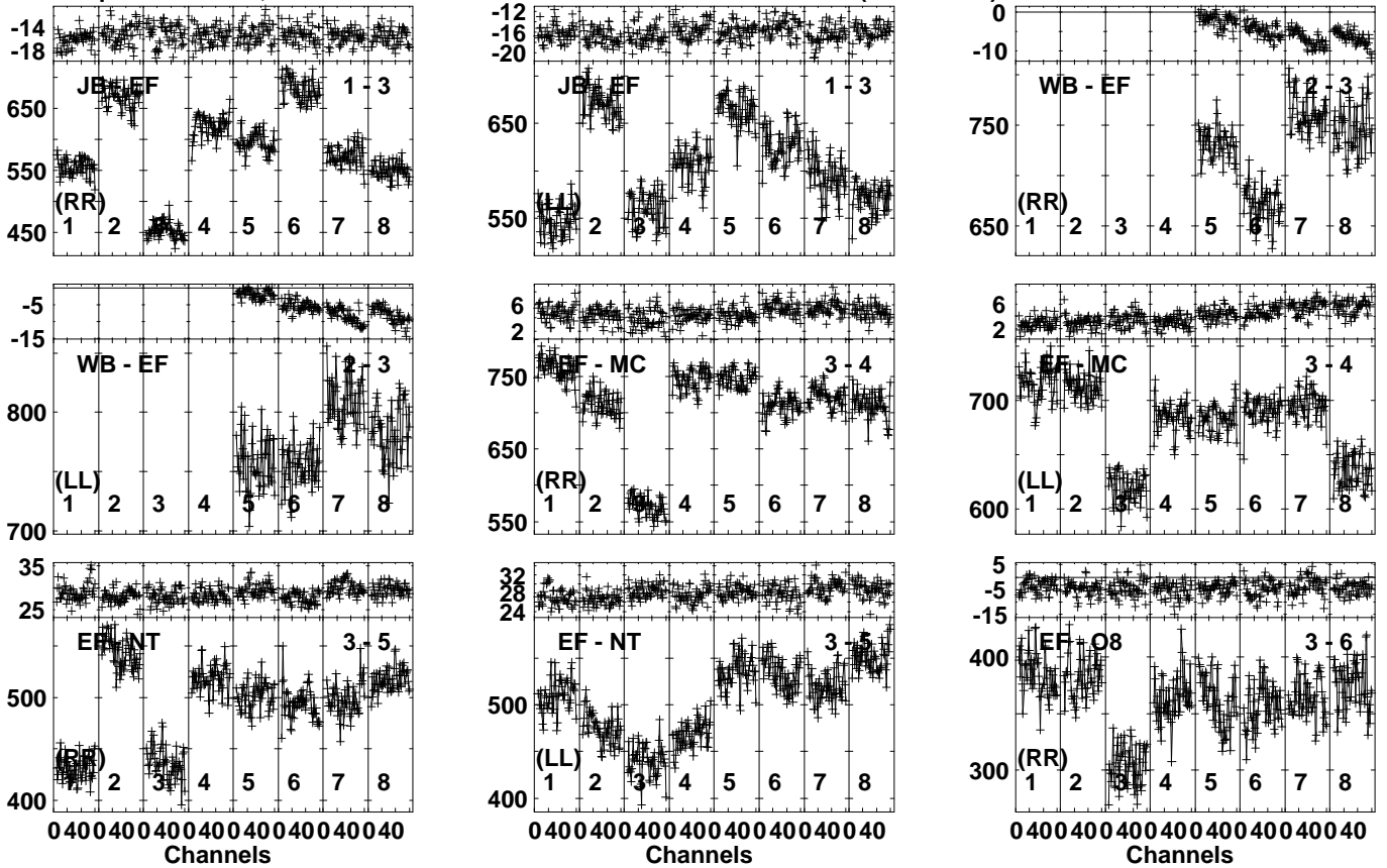
Lower frame: Milli Ampl Jy Top frame: Phas deg Vector averaged cross-power spectrum Several baselines displayed Timerange: 00/10:34:21 to 00/10:35:19
