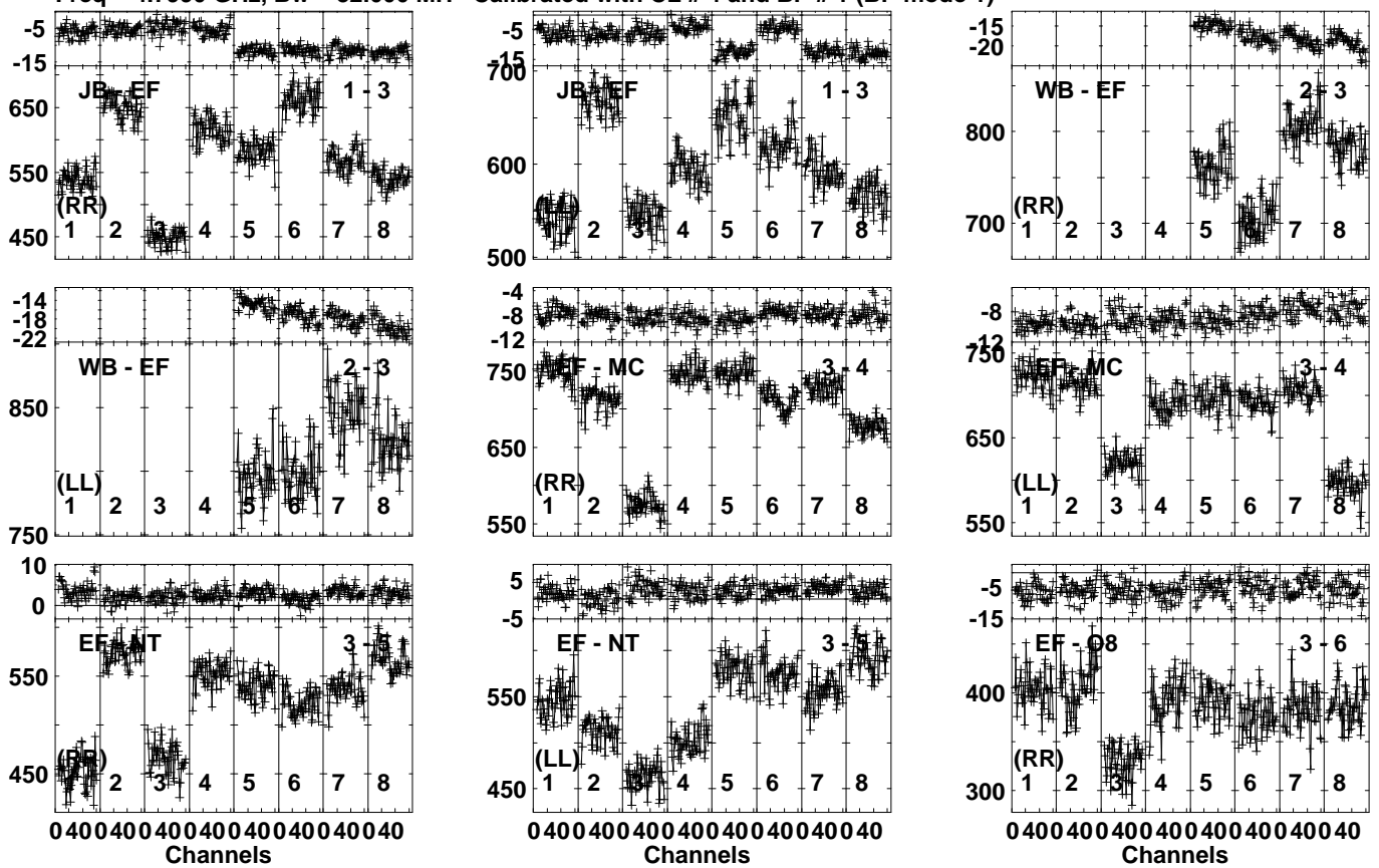
Lower frame: Milli Ampl Jy Top frame: Phas deg Vector averaged cross-power spectrum Several baselines displayed Timerange: 00/10:56:51 to 00/10:57:49
