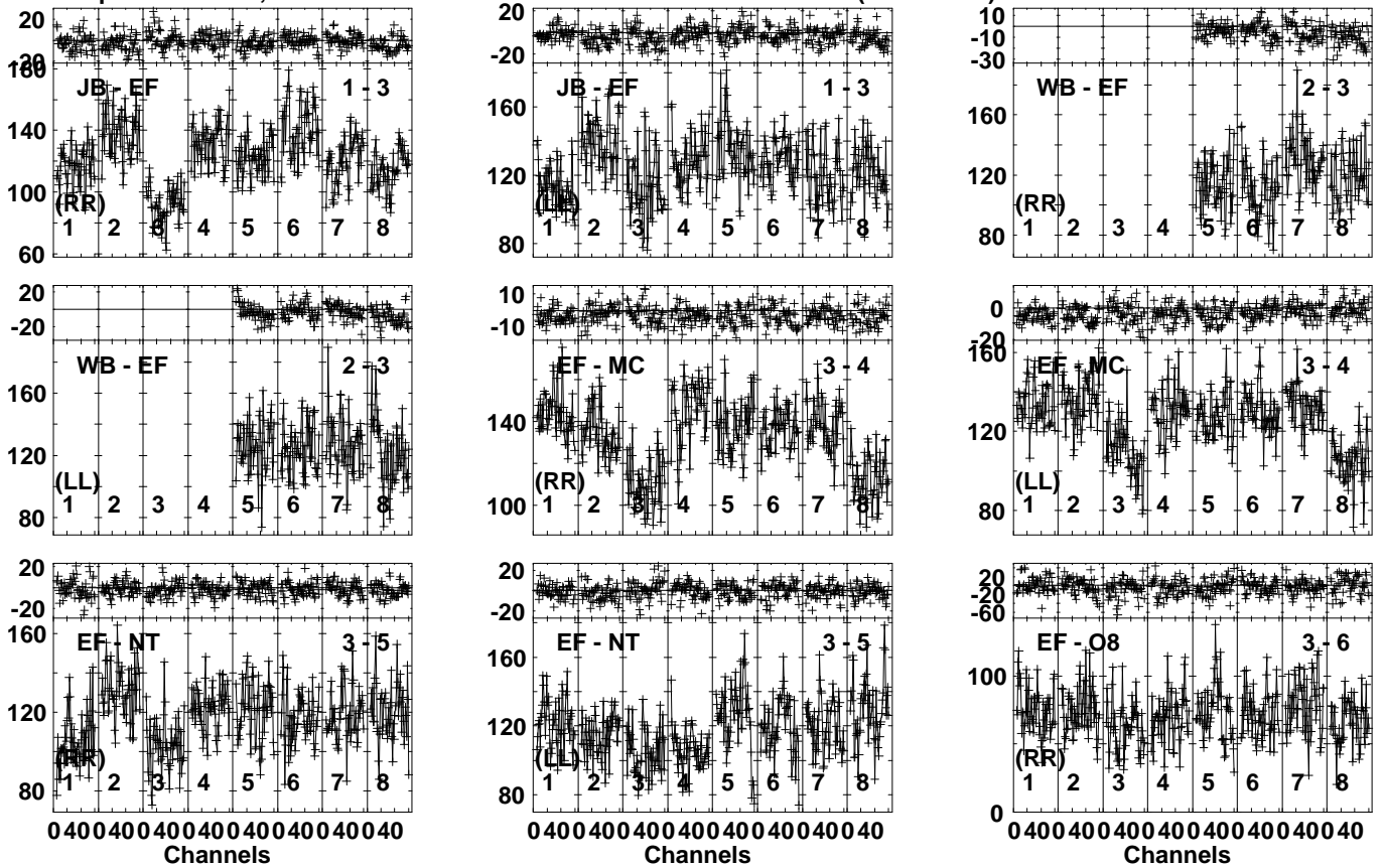
Lower frame: Milli Ampl Jy Top frame: Phas deg Vector averaged cross-power spectrum Several baselines displayed Timerange: 00/11:50:51 to 00/11:51:49
