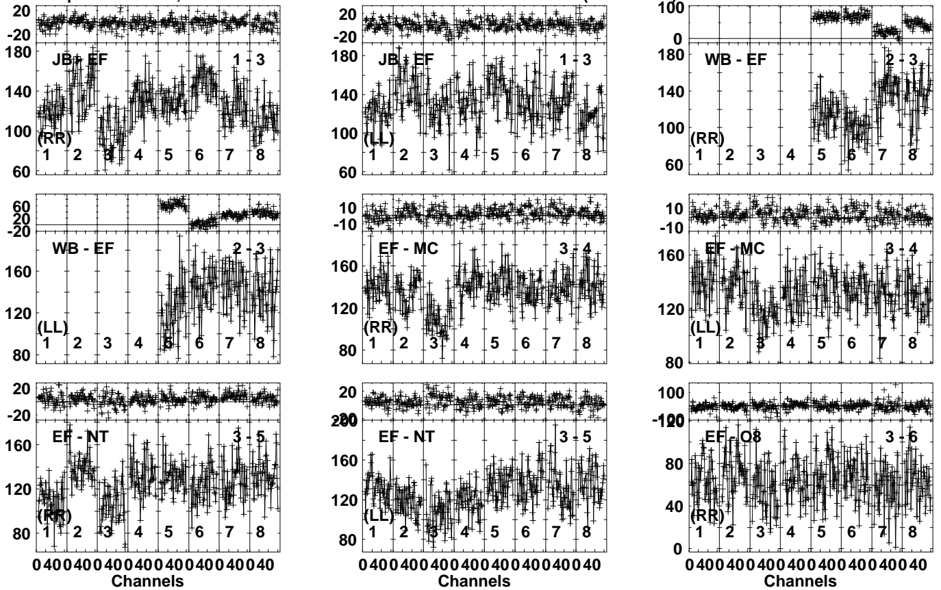
Lower frame: Milli Ampl Jy Top frame: Phas deg Vector averaged cross-power spectrum Several baselines displayed Timerange: 00/10:43:21 to 00/10:44:19
