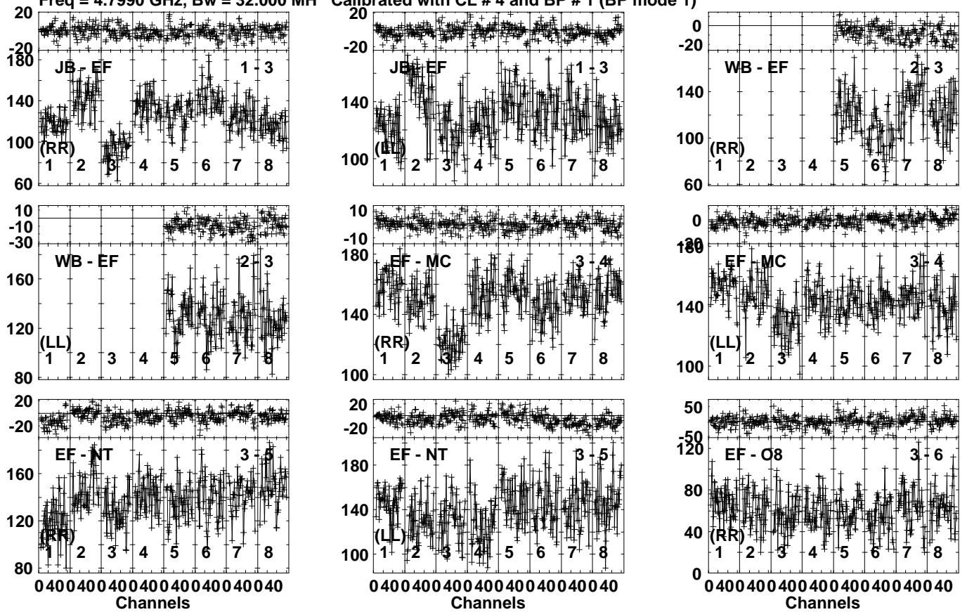
Lower frame: Milli Ampl Jy Top frame: Phas deg Vector averaged cross-power spectrum Several baselines displayed Timerange: 00/09:20:51 to 00/09:21:49
