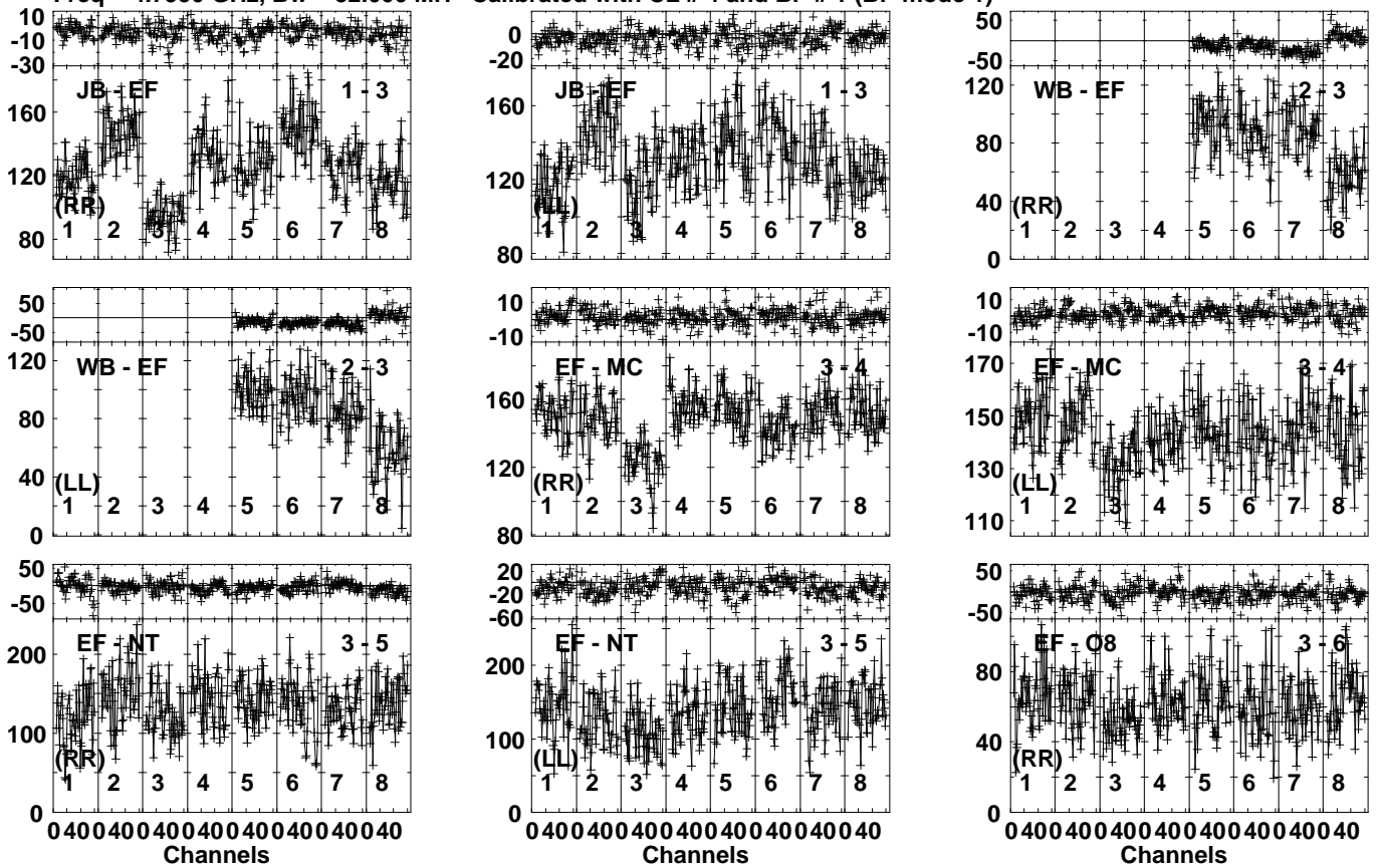
Lower frame: Milli Ampl Jy Top frame: Phas deg Vector averaged cross-power spectrum Several baselines displayed Timerange: 00/09:28:21 to 00/09:29:19
