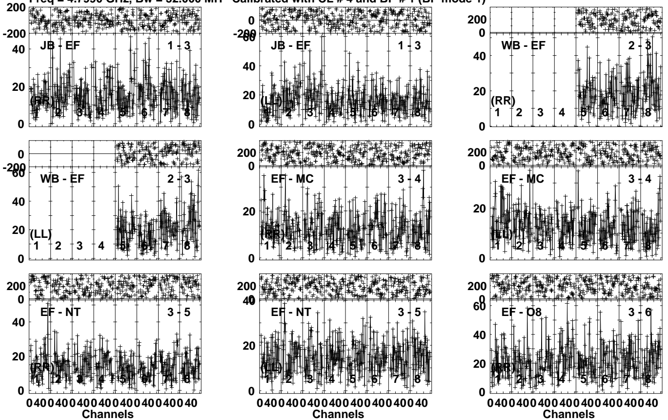
Lower frame: Milli Ampl Jy Top frame: Phas deg Vector averaged cross-power spectrum Several baselines displayed Timerange: 00/10:44:51 to 00/10:45:49
