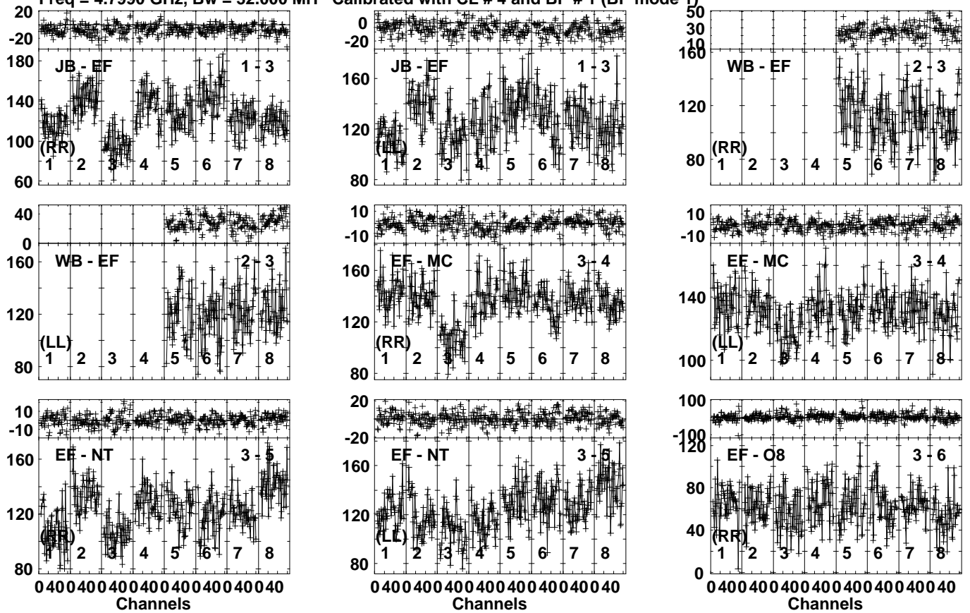
Lower frame: Milli Ampl Jy Top frame: Phas deg Vector averaged cross-power spectrum Several baselines displayed Timerange: 00/11:13:21 to 00/11:14:19
