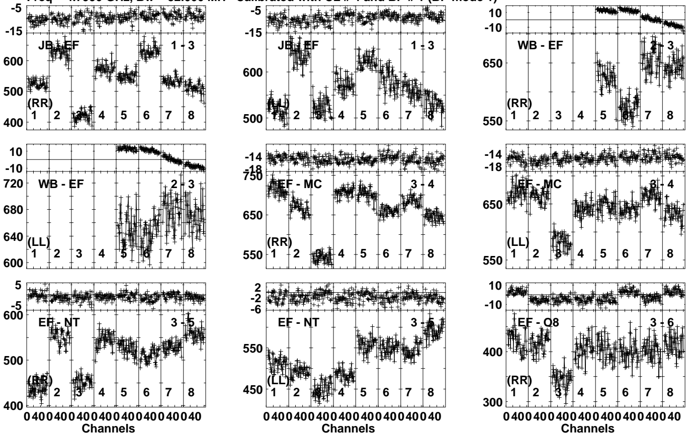
Lower frame: Milli Ampl Jy Top frame: Phas deg Vector averaged cross-power spectrum Several baselines displayed Timerange: 00/11:41:51 to 00/11:42:49
