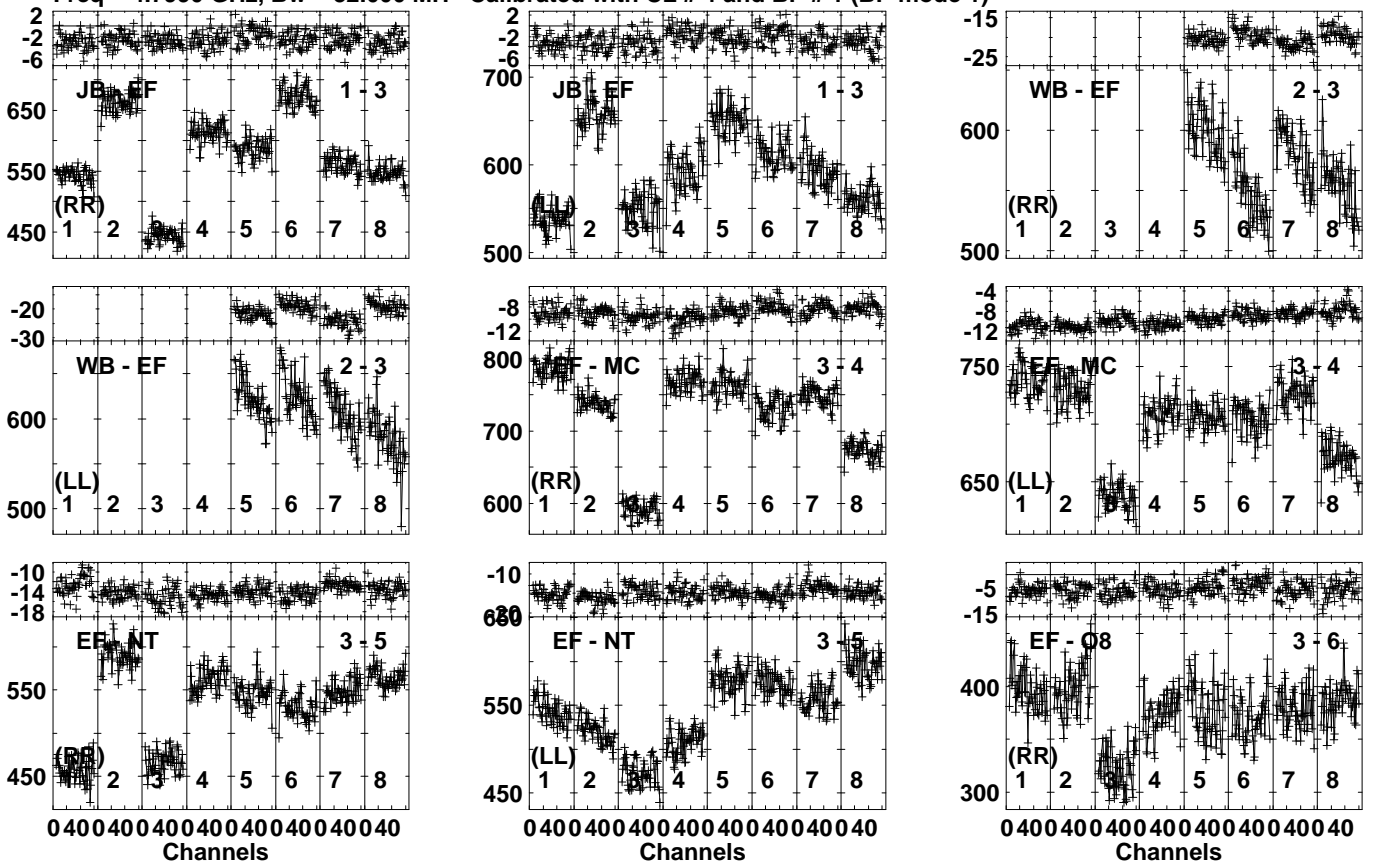
Lower frame: Milli Ampl Jy Top frame: Phas deg Vector averaged cross-power spectrum Several baselines displayed Timerange: 00/10:49:21 to 00/10:50:19
