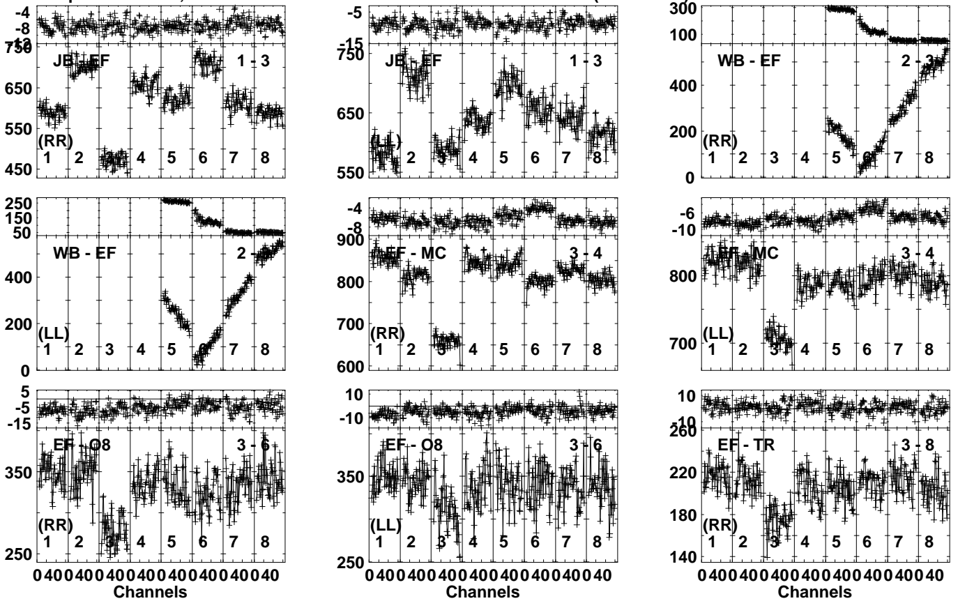
Lower frame: Milli Ampl Jy Top frame: Phas deg Vector averaged cross-power spectrum Several baselines displayed Timerange: 00/09:49:21 to 00/09:50:19
