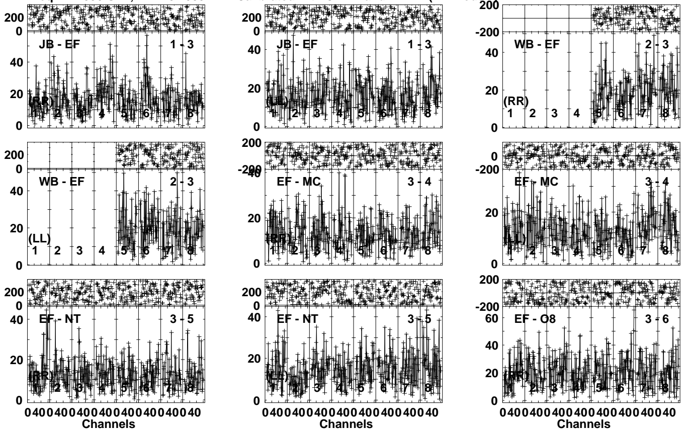
Lower frame: Milli Ampl Jy Top frame: Phas deg Vector averaged cross-power spectrum Several baselines displayed Timerange: 00/10:52:21 to 00/10:53:19
