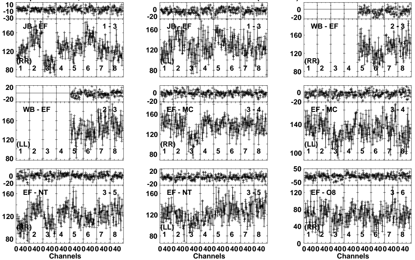
Lower frame: Milli Ampl Jy Top frame: Phas deg Vector averaged cross-power spectrum Several baselines displayed Timerange: 00/10:58:21 to 00/10:59:19
