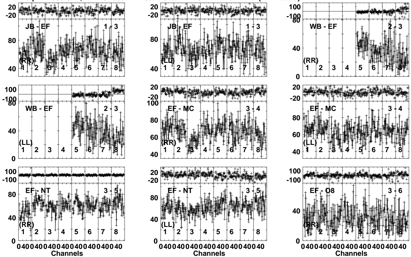
Lower frame: Milli Ampl Jy Top frame: Phas deg Vector averaged cross-power spectrum Several baselines displayed Timerange: 00/11:25:21 to 00/11:26:19
