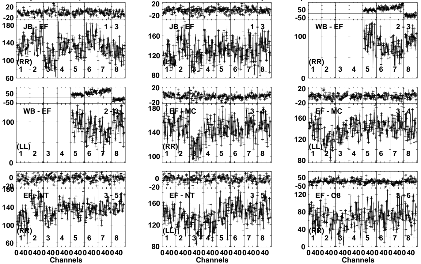
Lower frame: Milli Ampl Jy Top frame: Phas deg Vector averaged cross-power spectrum Several baselines displayed Timerange: 00/09:35:51 to 00/09:36:49
