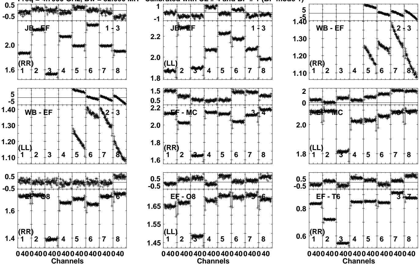
Lower frame: Ampl Jy Top frame: Phas deg Vector averaged cross-power spectrum Several baselines displayed Timerange: 00/09:09:55 to 00/09:13:49
