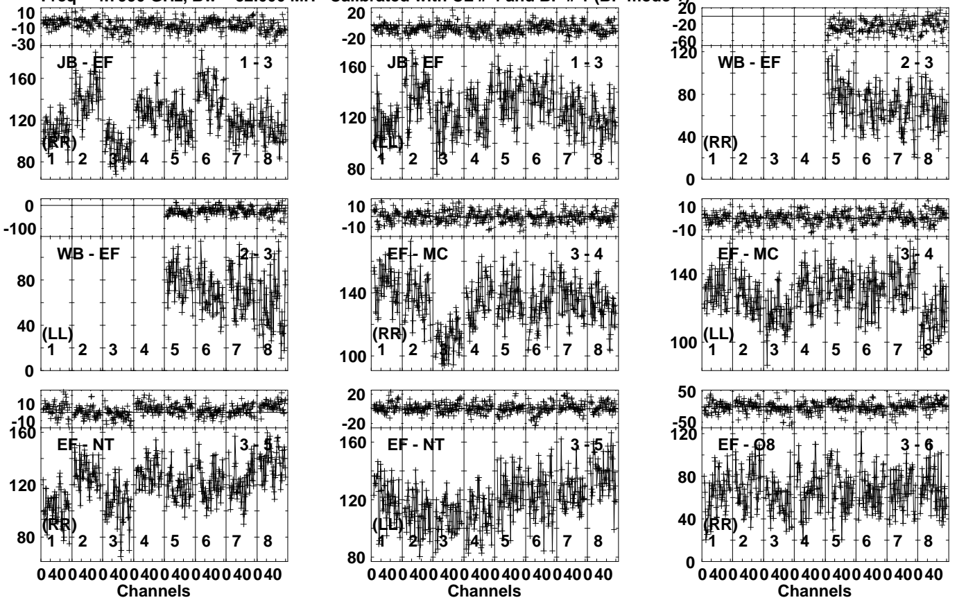
Lower frame: Milli Ampl Jy Top frame: Phas deg Vector averaged cross-power spectrum Several baselines displayed Timerange: 00/11:20:51 to 00/11:21:49
