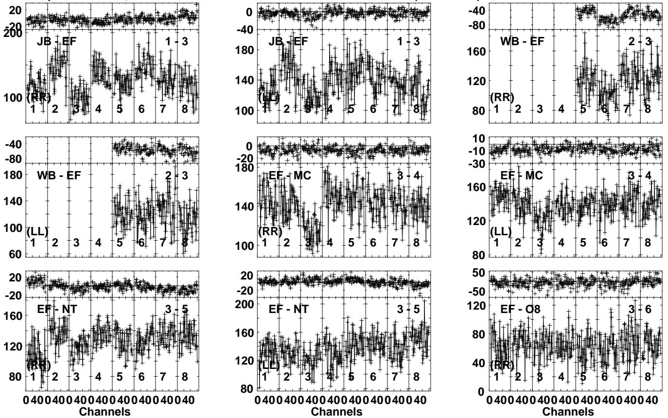
Lower frame: Milli Ampl Jy Top frame: Phas deg Vector averaged cross-power spectrum Several baselines displayed Timerange: 00/10:13:21 to 00/10:14:19
