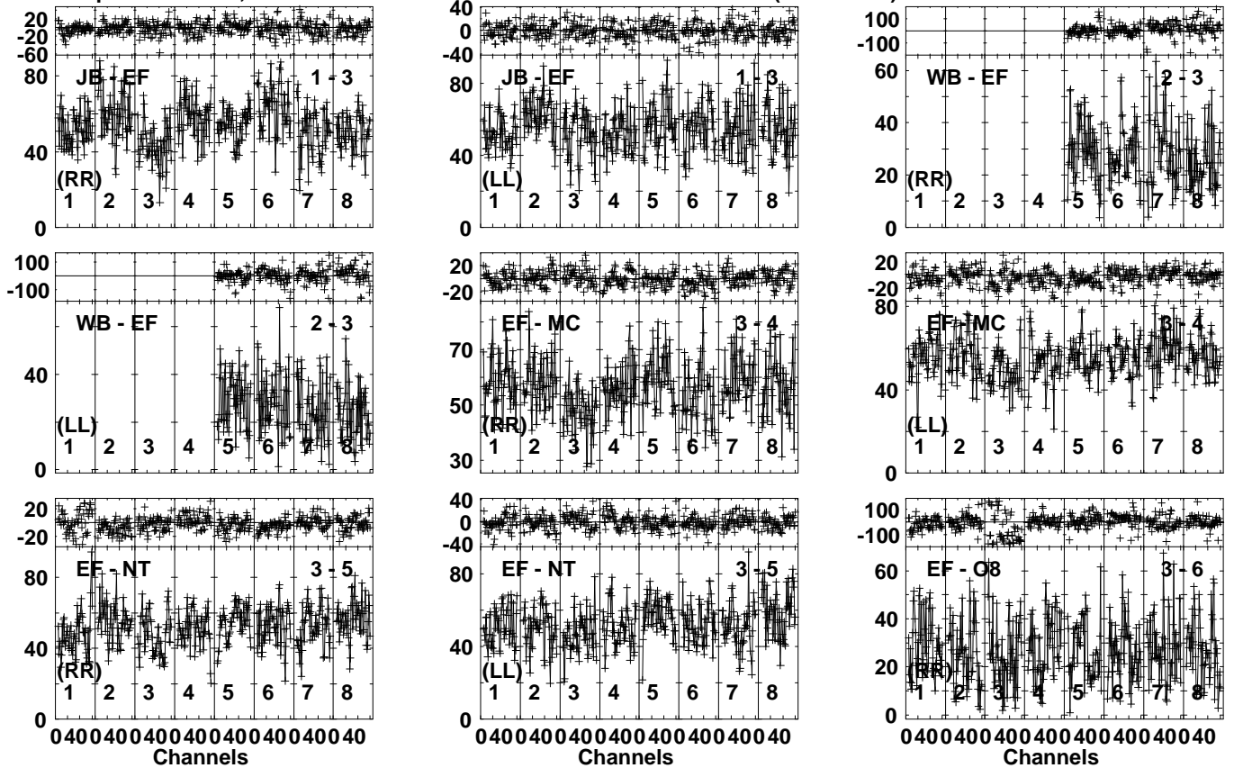
Lower frame: Milli Ampl Jy Top frame: Phas deg Vector averaged cross-power spectrum Several baselines displayed Timerange: 00/10:38:51 to 00/10:39:49
