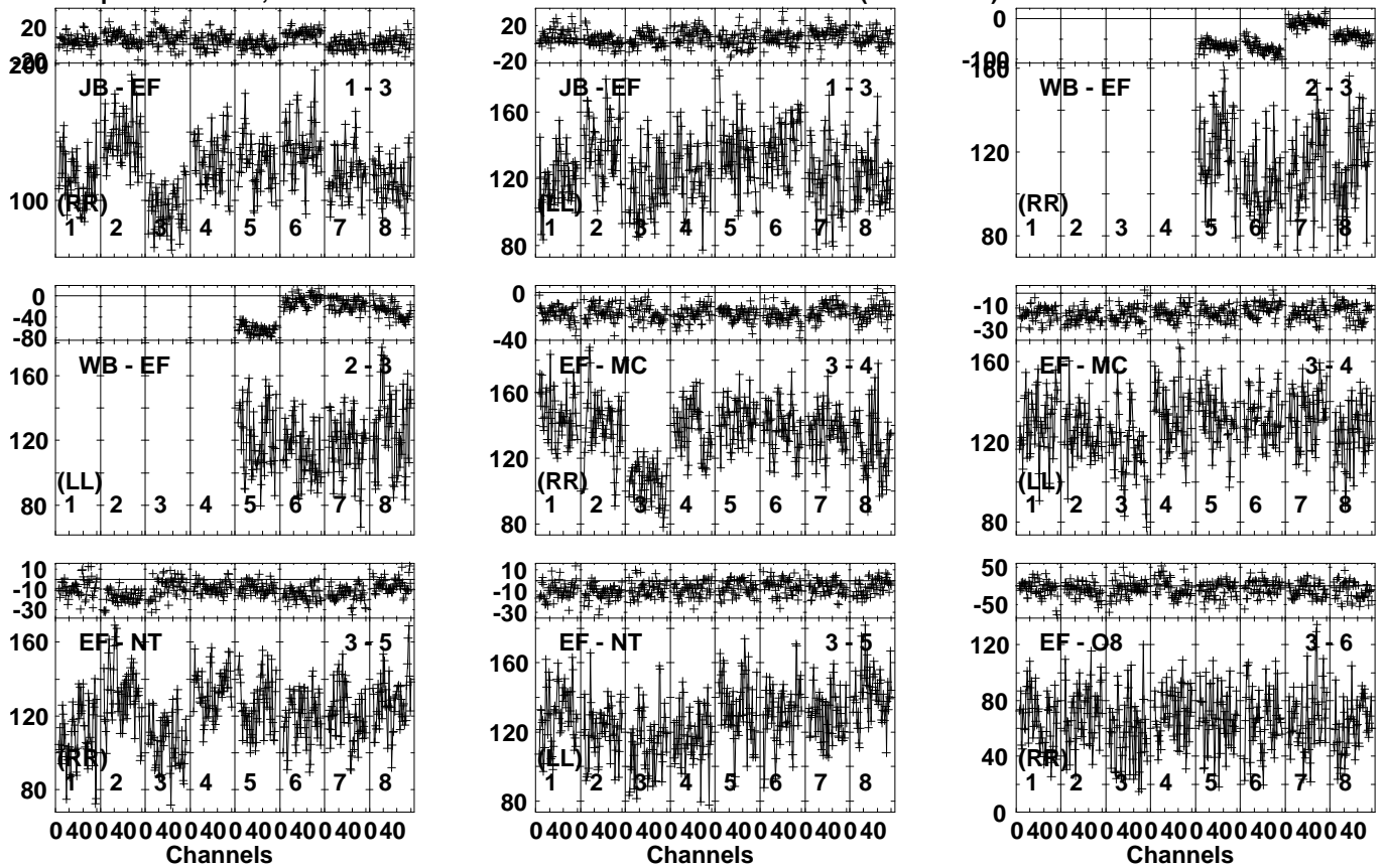
Lower frame: Milli Ampl Jy Top frame: Phas deg Vector averaged cross-power spectrum Several baselines displayed Timerange: 00/10:50:51 to 00/10:51:49
