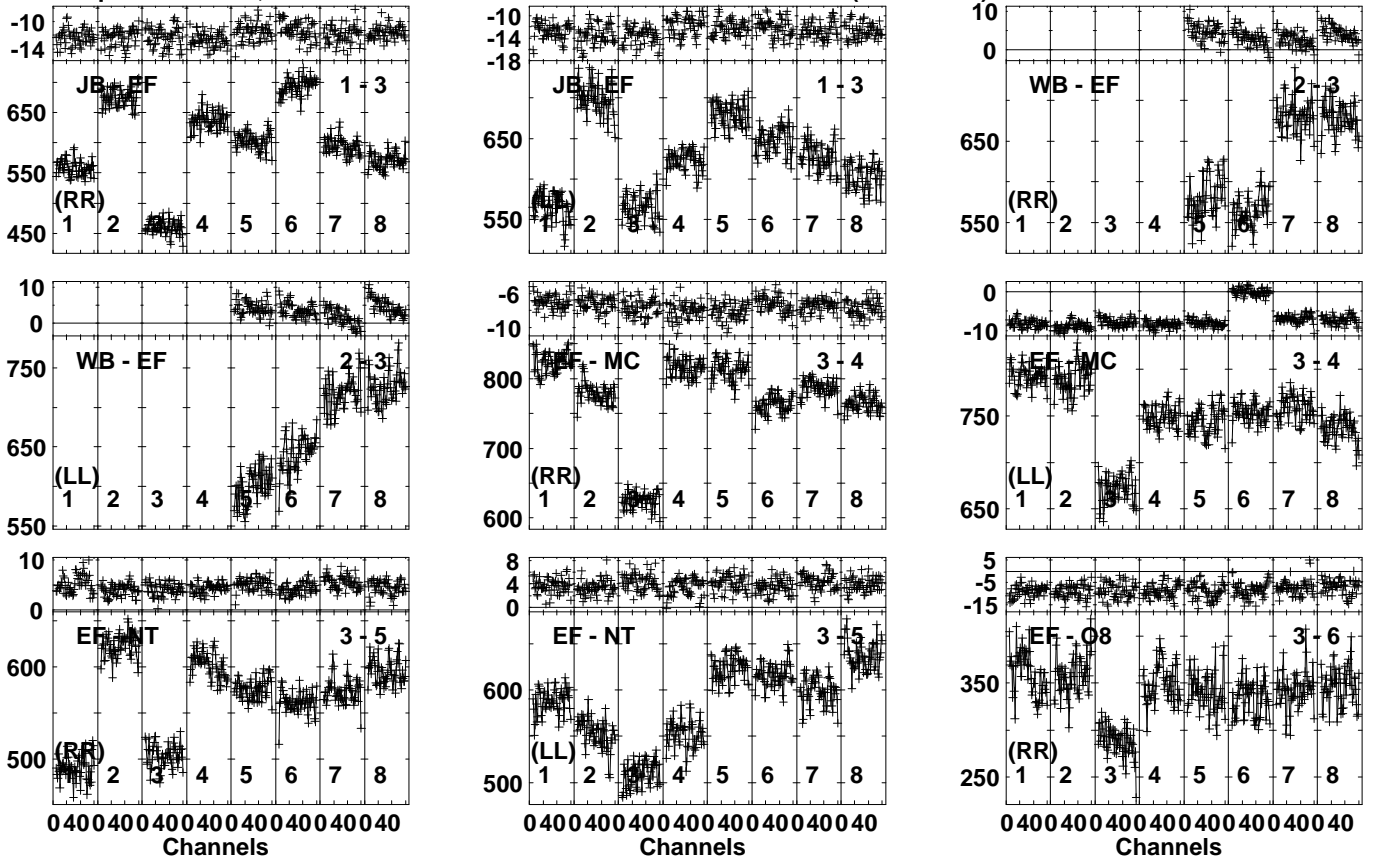
Lower frame: Milli Ampl Jy Top frame: Phas deg Vector averaged cross-power spectrum Several baselines displayed Timerange: 00/10:11:51 to 00/10:12:49
