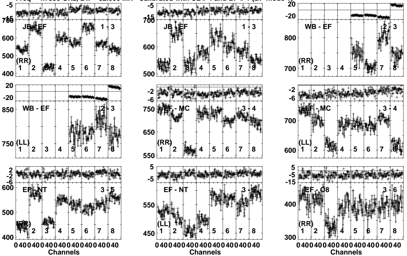
Lower frame: Milli Ampl Jy Top frame: Phas deg Vector averaged cross-power spectrum Several baselines displayed Timerange: 00/11:04:21 to 00/11:05:19
