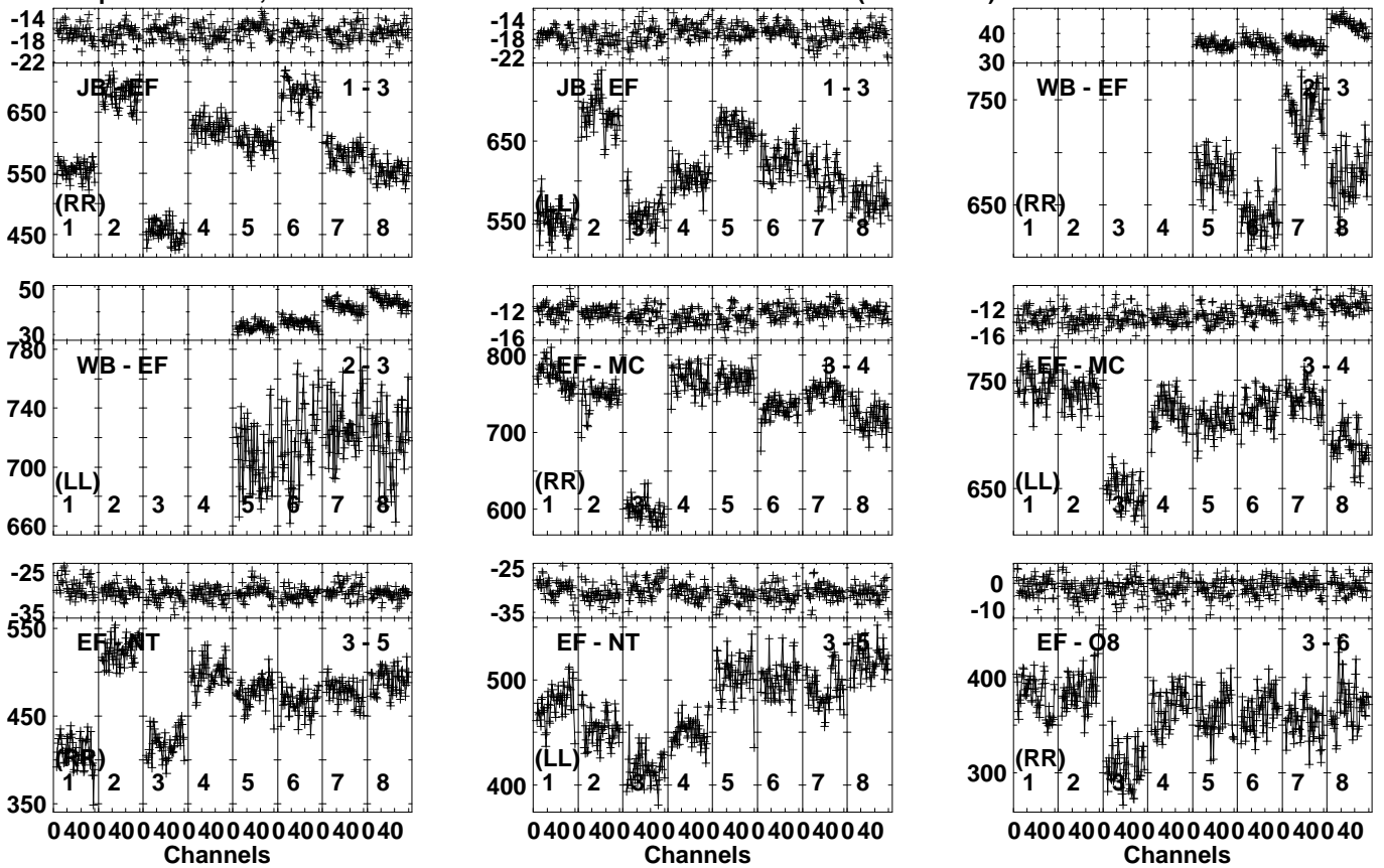
Lower frame: Milli Ampl Jy Top frame: Phas deg Vector averaged cross-power spectrum Several baselines displayed Timerange: 00/10:41:51 to 00/10:42:49
