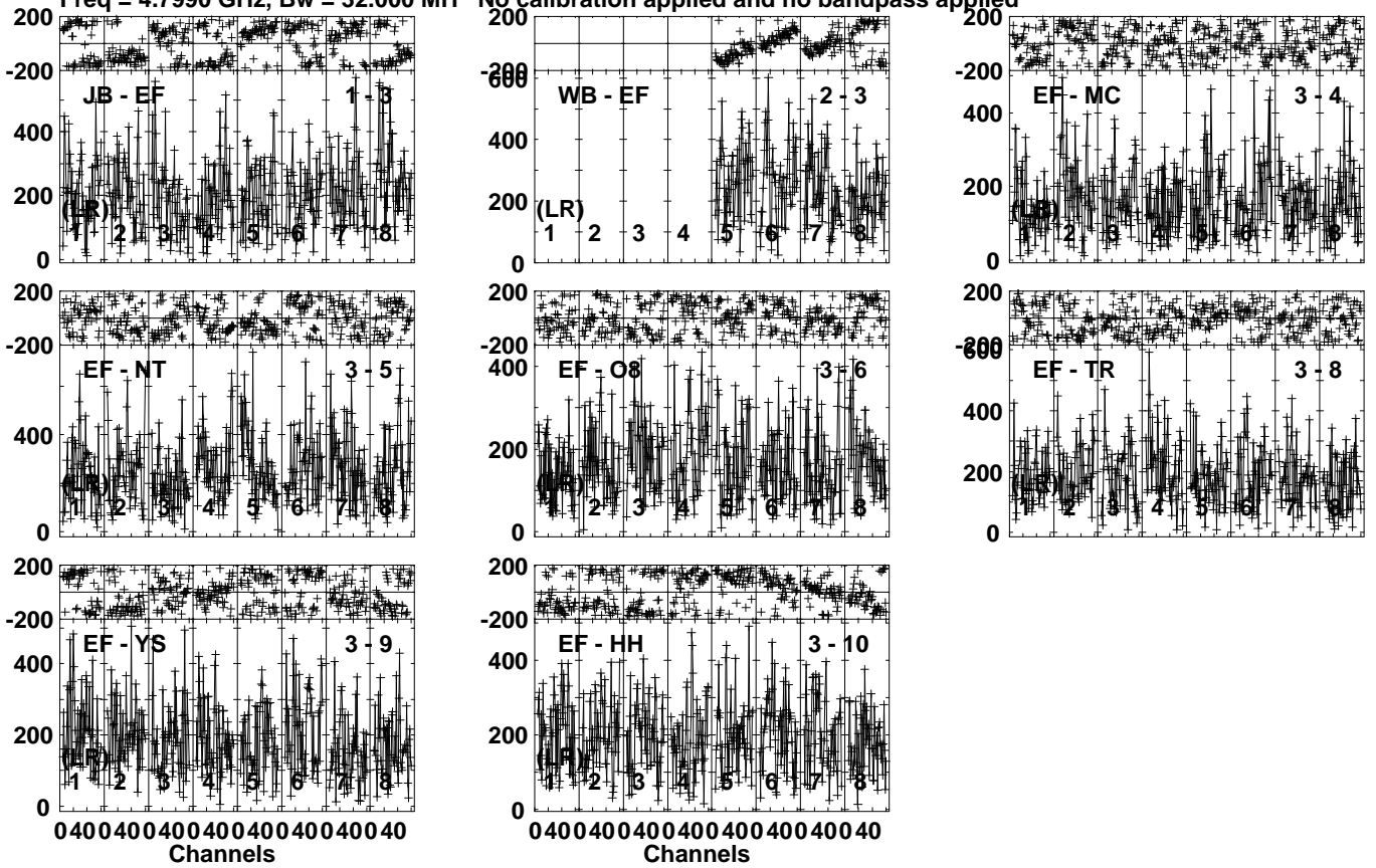
Lower frame: Micro Ampl Jy Top frame: Phas deg Vector averaged cross-power spectrum Several baselines displayed Timerange: 00/09:20:51 to 00/09:21:49
