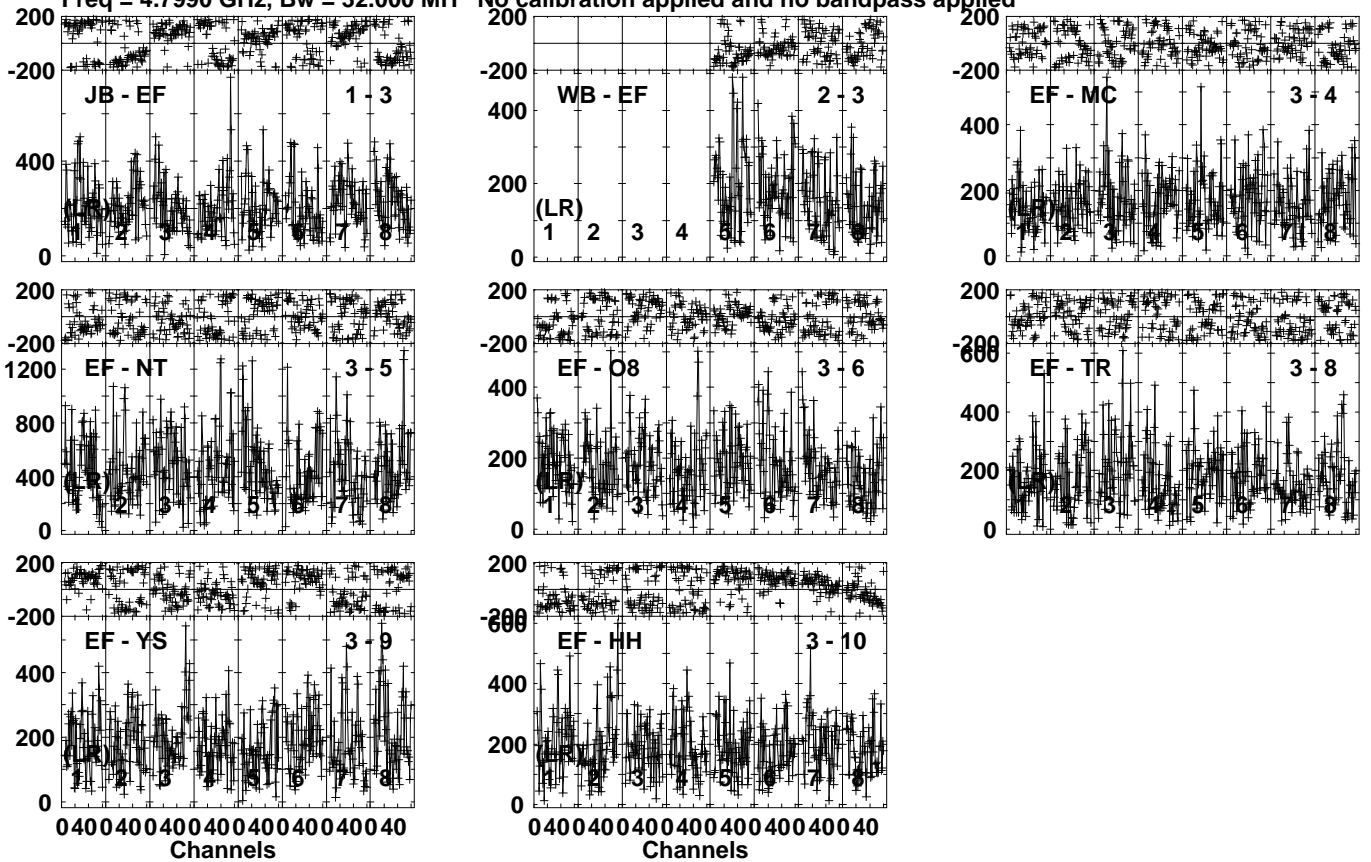
Lower frame: Micro Ampl Jy Top frame: Phas deg Vector averaged cross-power spectrum Several baselines displayed Timerange: 00/09:28:21 to 00/09:29:19
