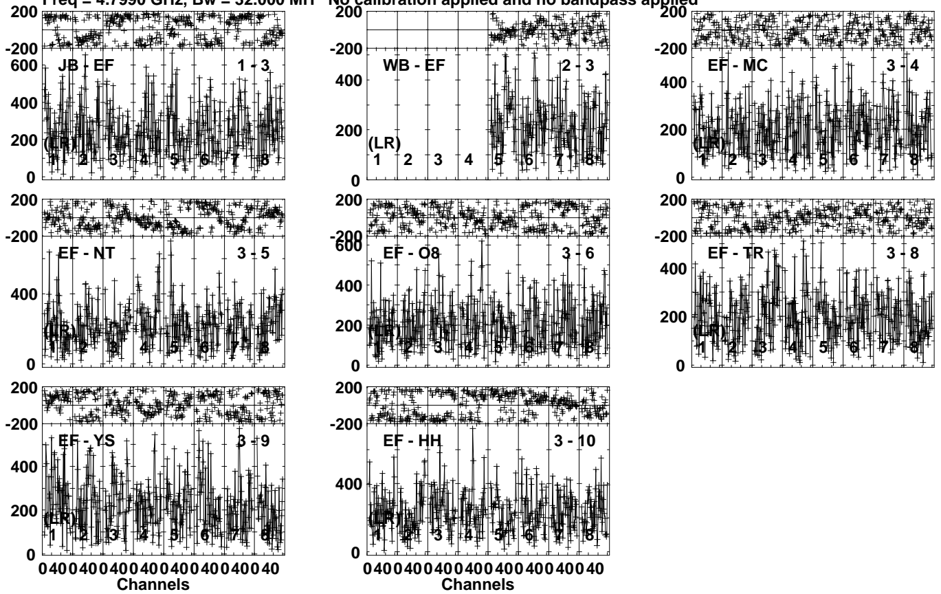
Lower frame: Micro Ampl Jy Top frame: Phas deg Vector averaged cross-power spectrum Several baselines displayed Timerange: 00/09:35:51 to 00/09:36:49
