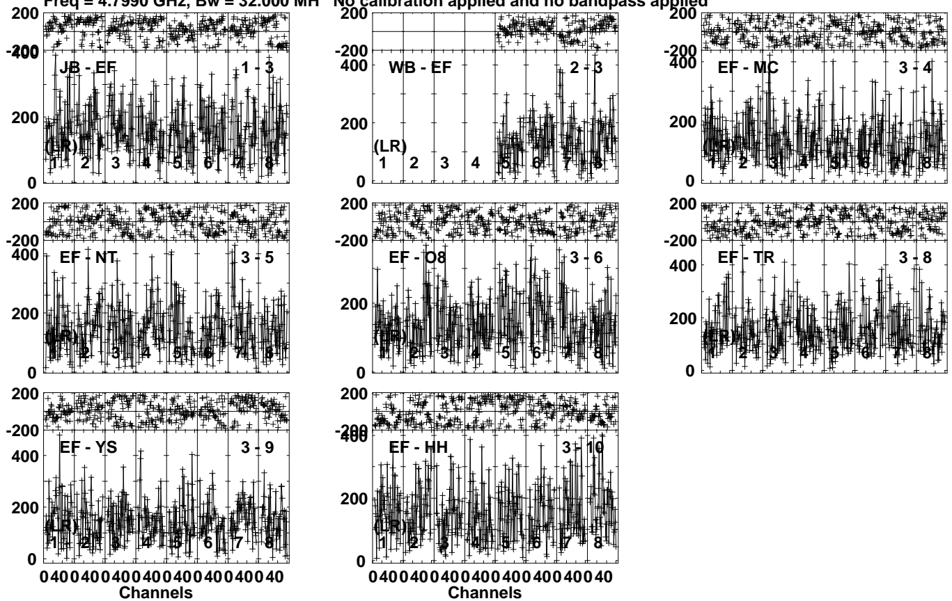
Lower frame: Micro Ampl Jy Top frame: Phas deg Vector averaged cross-power spectrum Several baselines displayed Timerange: 00/10:40:21 to 00/10:41:19
