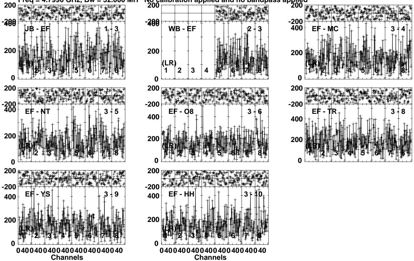
Lower frame: Micro Ampl Jy Top frame: Phas deg Vector averaged cross-power spectrum Several baselines displayed Timerange: 00/10:14:51 to 00/10:15:49
