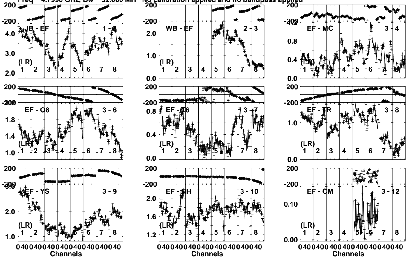
Lower frame: Milli Ampl Jy Top frame: Phas deg Vector averaged cross-power spectrum Several baselines displayed Timerange: 00/09:09:55 to 00/09:13:49
