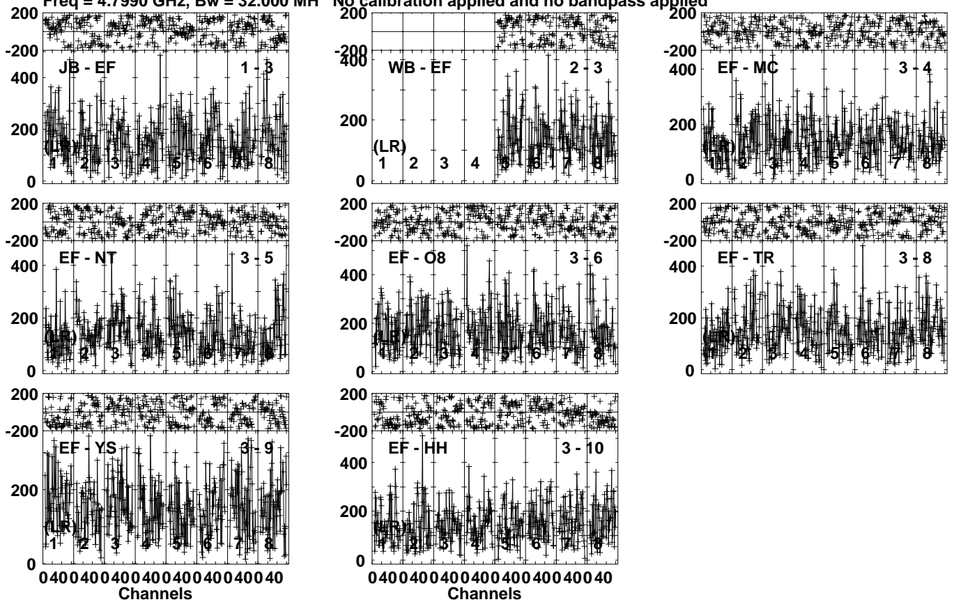
Lower frame: Micro Ampl Jy Top frame: Phas deg Vector averaged cross-power spectrum Several baselines displayed Timerange: 00/11:16:21 to 00/11:17:19
