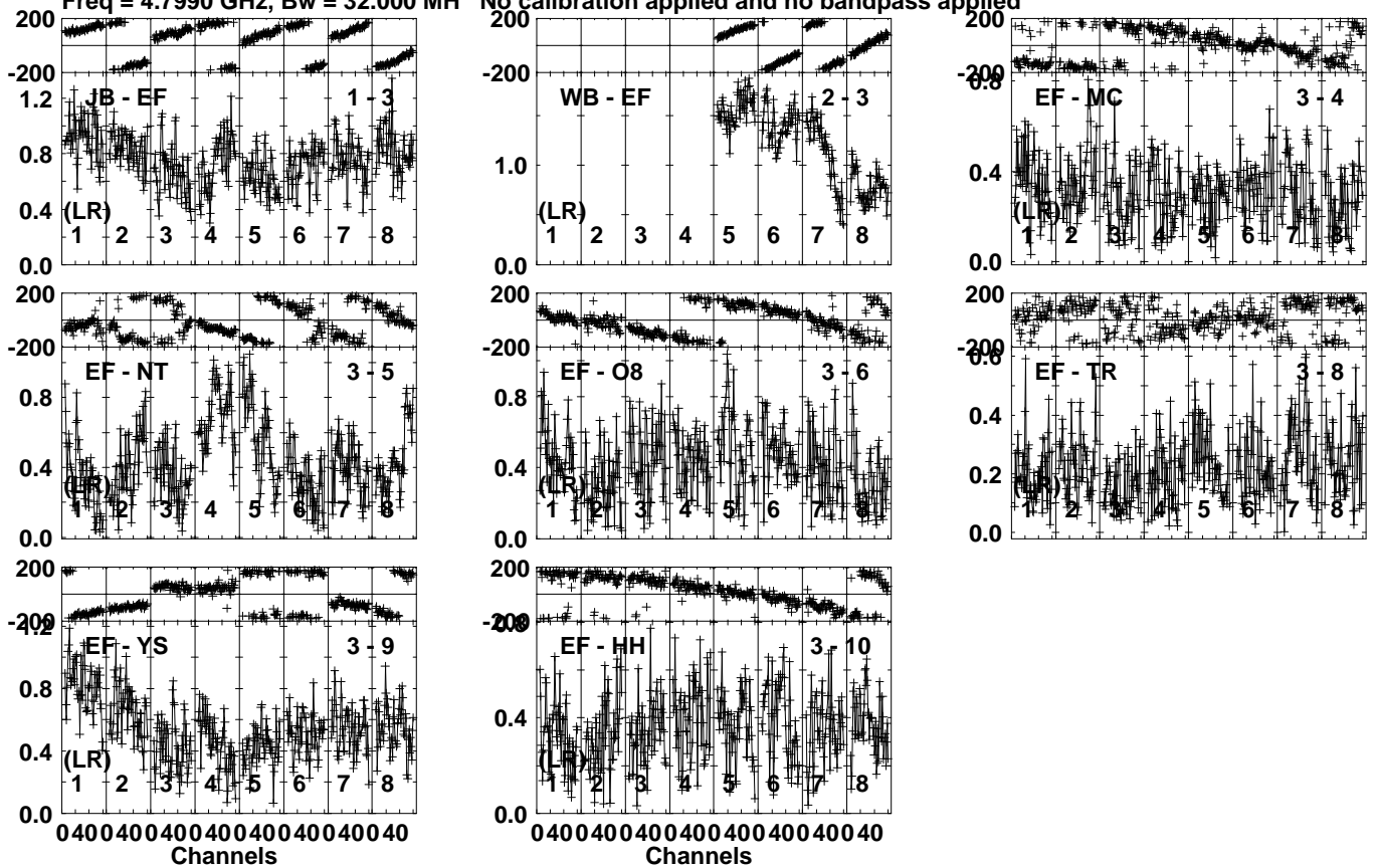
Lower frame: Milli Ampl Jy Top frame: Phas deg Vector averaged cross-power spectrum Several baselines displayed Timerange: 00/11:26:51 to 00/11:27:49
