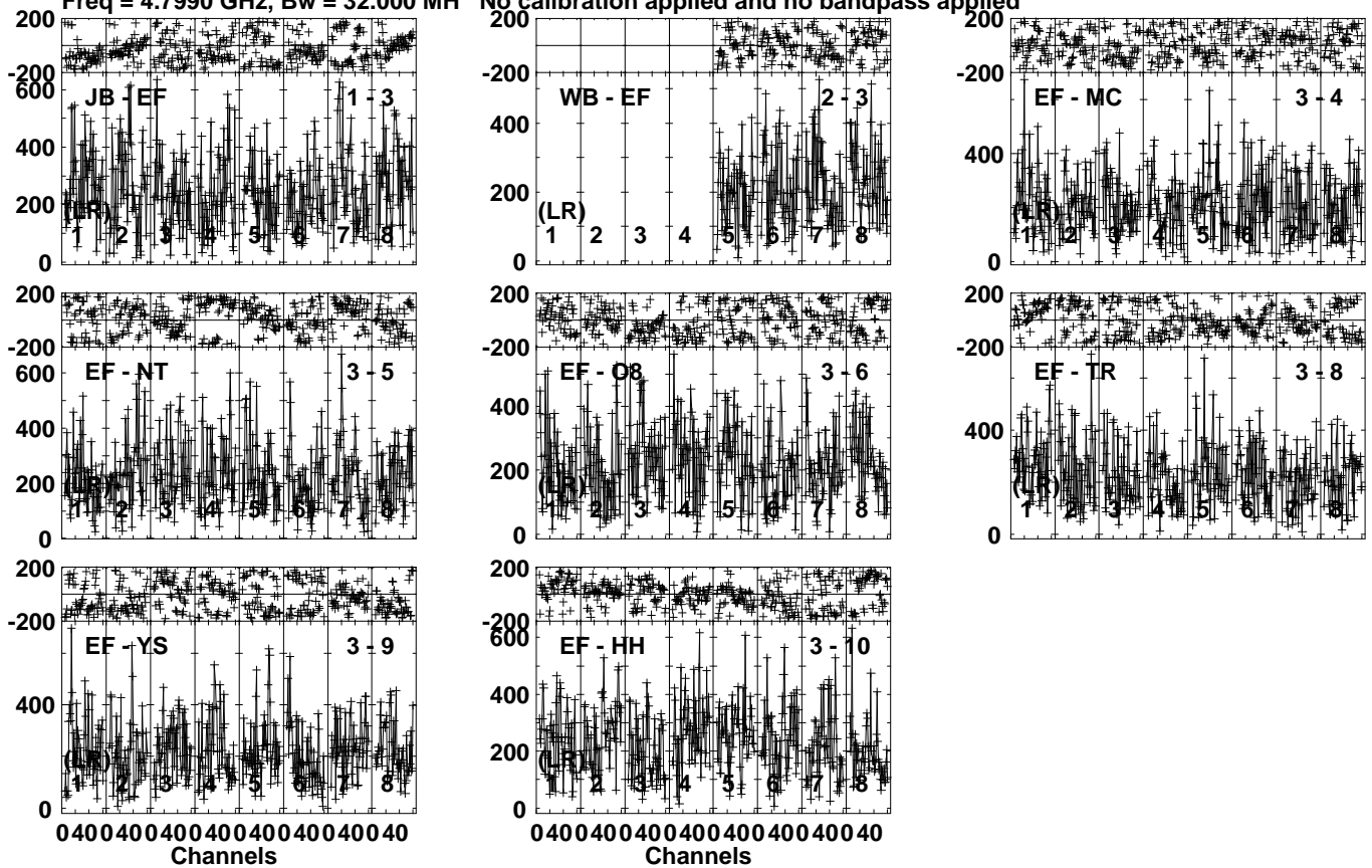
Lower frame: Micro Ampl Jy Top frame: Phas deg Vector averaged cross-power spectrum Several baselines displayed Timerange: 00/10:20:51 to 00/10:21:49
