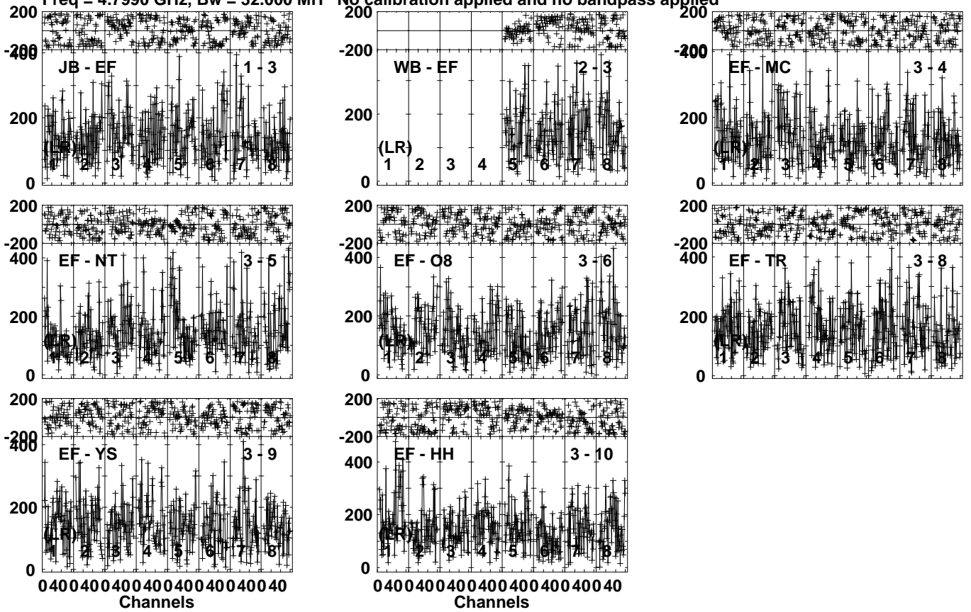
Lower frame: Micro Ampl Jy Top frame: Phas deg Vector averaged cross-power spectrum Several baselines displayed Timerange: 00/10:08:51 to 00/10:09:49
