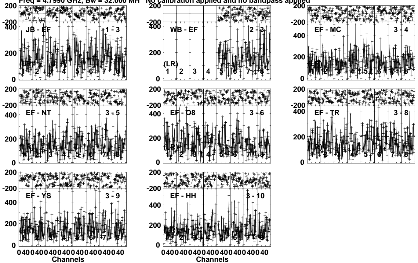
Lower frame: Micro Ampl Jy Top frame: Phas deg Vector averaged cross-power spectrum Several baselines displayed Timerange: 00/10:31:21 to 00/10:32:19
