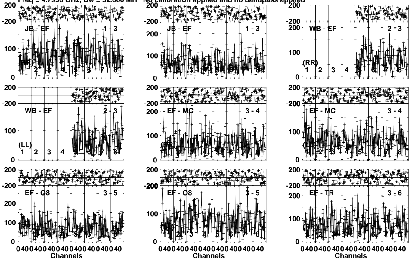
Lower frame: Micro Ampl Jy Top frame: Phas deg Vector averaged cross-power spectrum Several baselines displayed Timerange: 00/06:57:21 to 00/07:01:49
