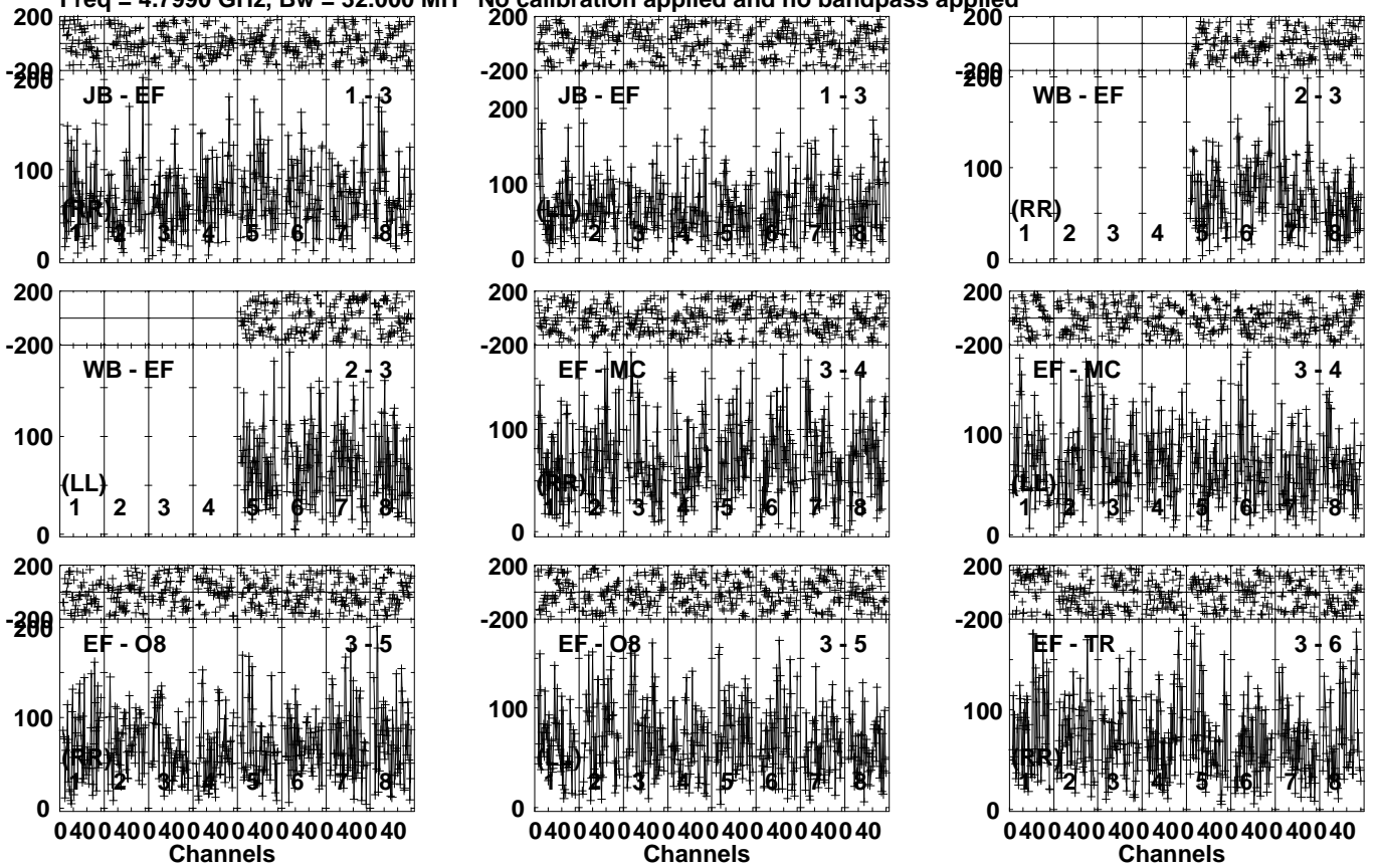
Lower frame: Micro Ampl Jy Top frame: Phas deg Vector averaged cross-power spectrum Several baselines displayed Timerange: 00/06:45:11 to 00/06:49:39
