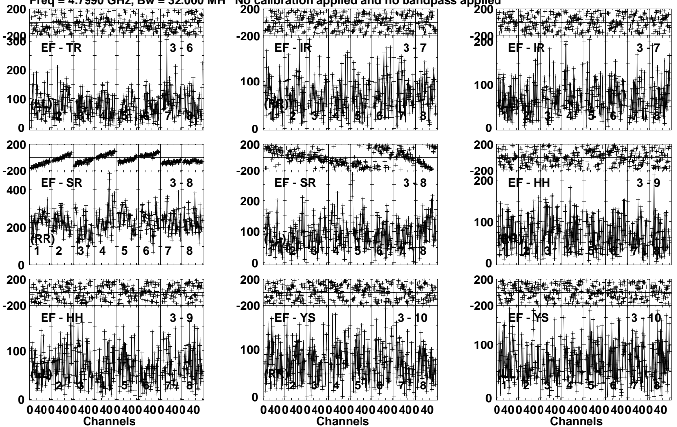
Lower frame: Micro Ampl Jy Top frame: Phas deg Vector averaged cross-power spectrum Several baselines displayed Timerange: 00/06:21:01 to 00/06:25:29
