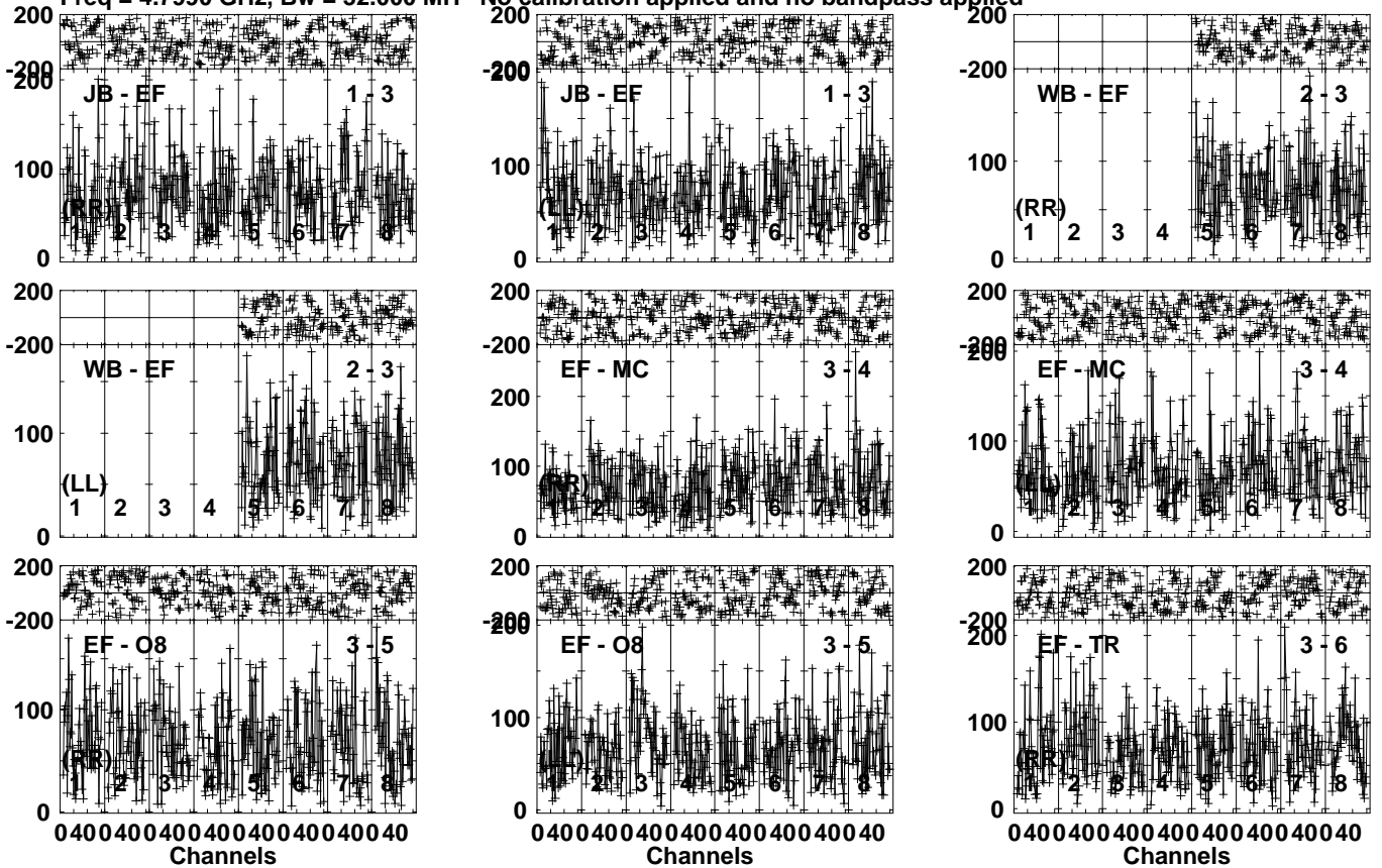
Lower frame: Micro Ampl Jy Top frame: Phas deg Vector averaged cross-power spectrum Several baselines displayed Timerange: 00/07:33:41 to 00/07:38:09
