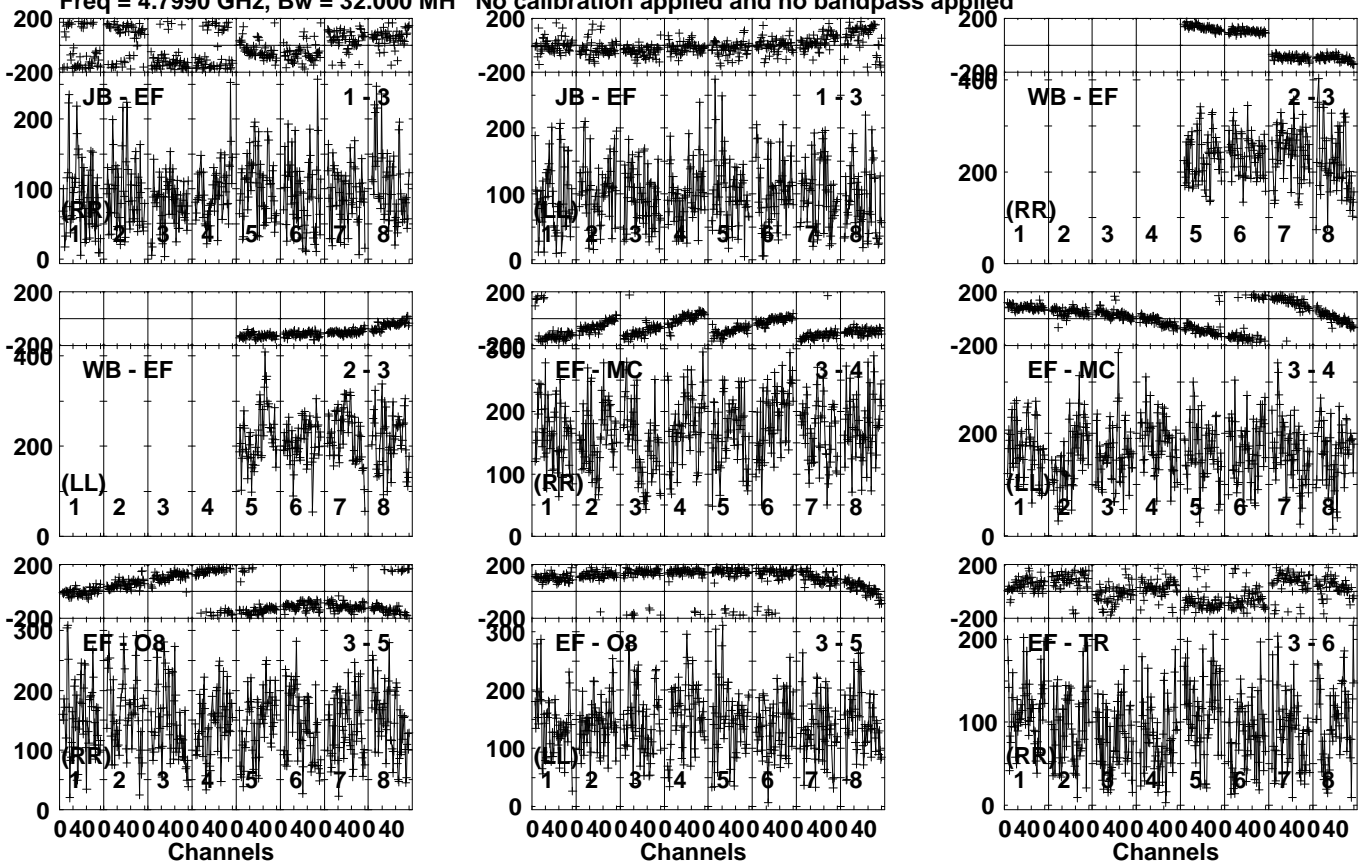
Lower frame: Micro Ampl Jy Top frame: Phas deg Vector averaged cross-power spectrum Several baselines displayed Timerange: 00/07:52:01 to 00/07:56:29
