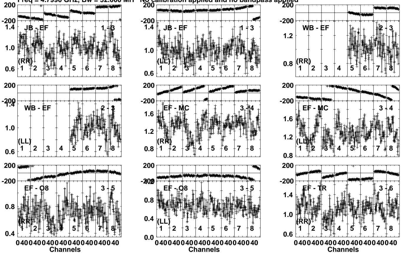
Lower frame: Milli Ampl Jy Top frame: Phas deg Vector averaged cross-power spectrum Several baselines displayed Timerange: 00/07:01:51 to 00/07:03:19
