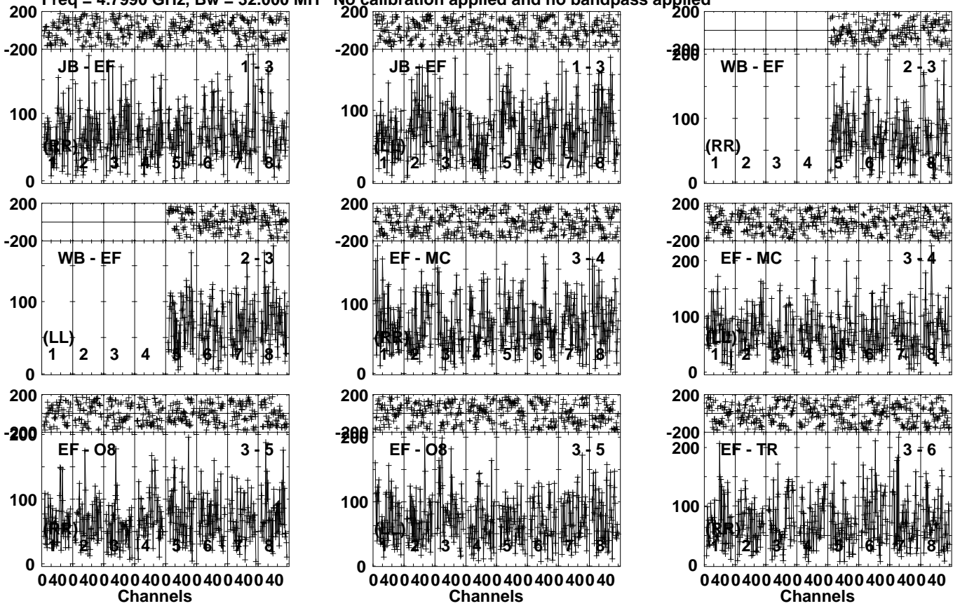
Lower frame: Micro Ampl Jy Top frame: Phas deg Vector averaged cross-power spectrum Several baselines displayed Timerange: 00/06:14:51 to 00/06:19:19
