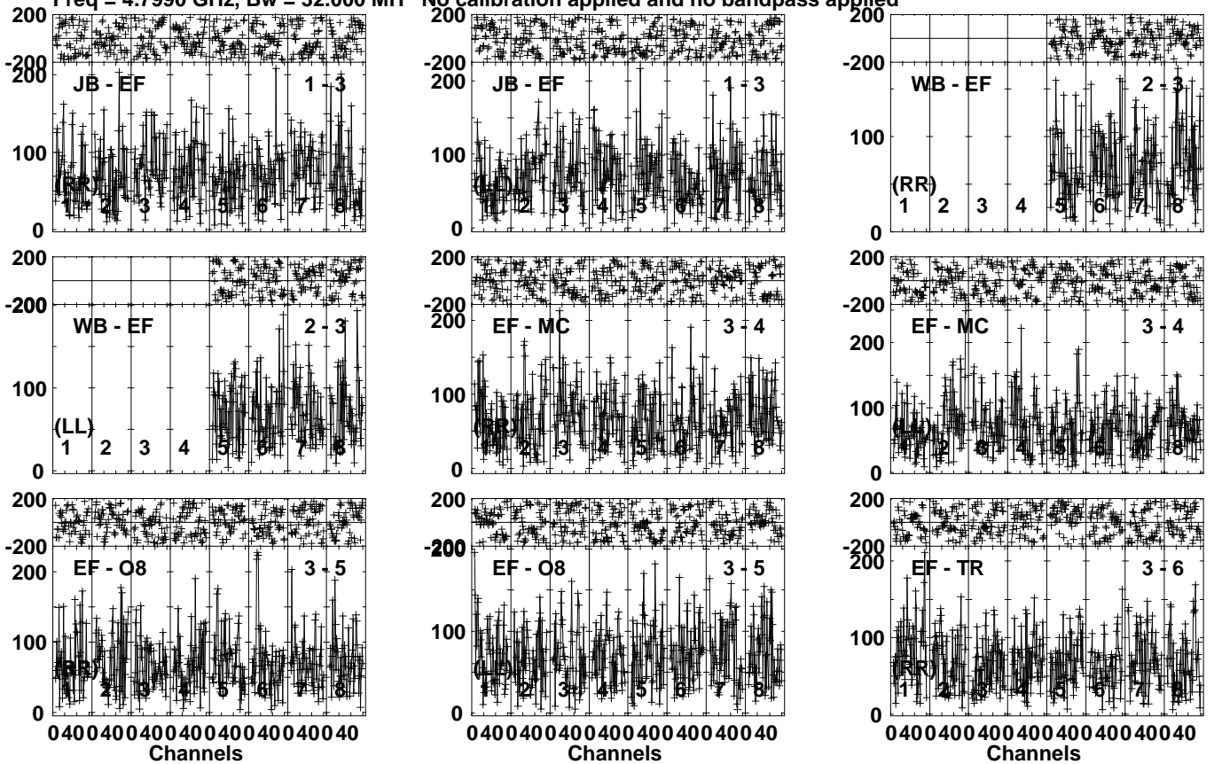
Lower frame: Micro Ampl Jy Top frame: Phas deg Vector averaged cross-power spectrum Several baselines displayed Timerange: 00/08:04:01 to 00/08:08:29
