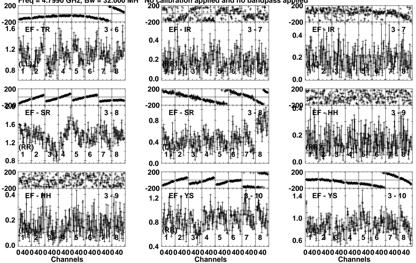
Lower frame: Milli Ampl Jy Top frame: Phas deg Vector averaged cross-power spectrum Several baselines displayed Timerange: 00/07:14:01 to 00/07:15:29
