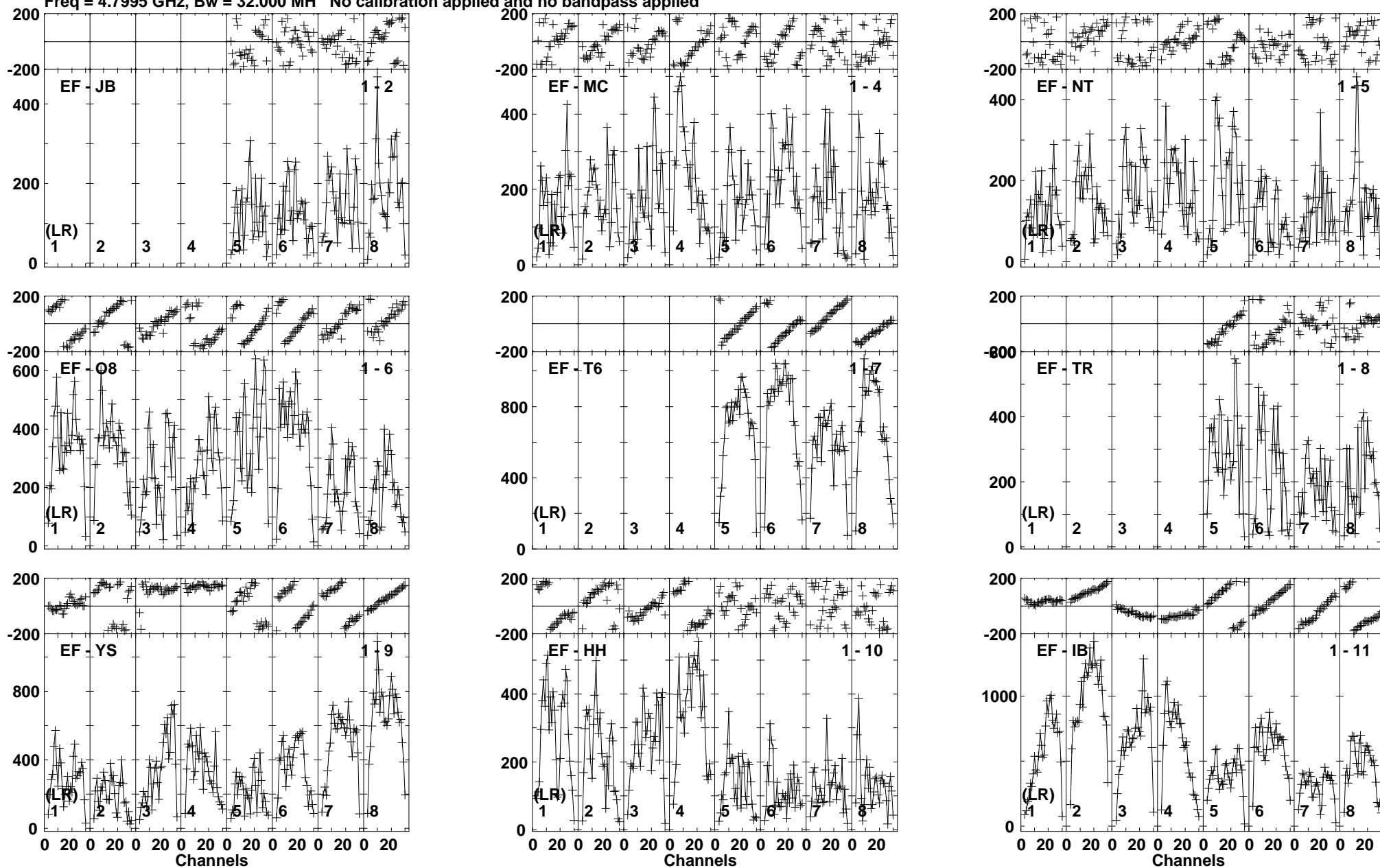
Lower frame: Micro Ampl Jy Top frame: Phas deg Vector averaged cross-power spectrum Baseline: EF (01) - JB (02) Timerange: 00/20:46:22 to 00/20:47:48
