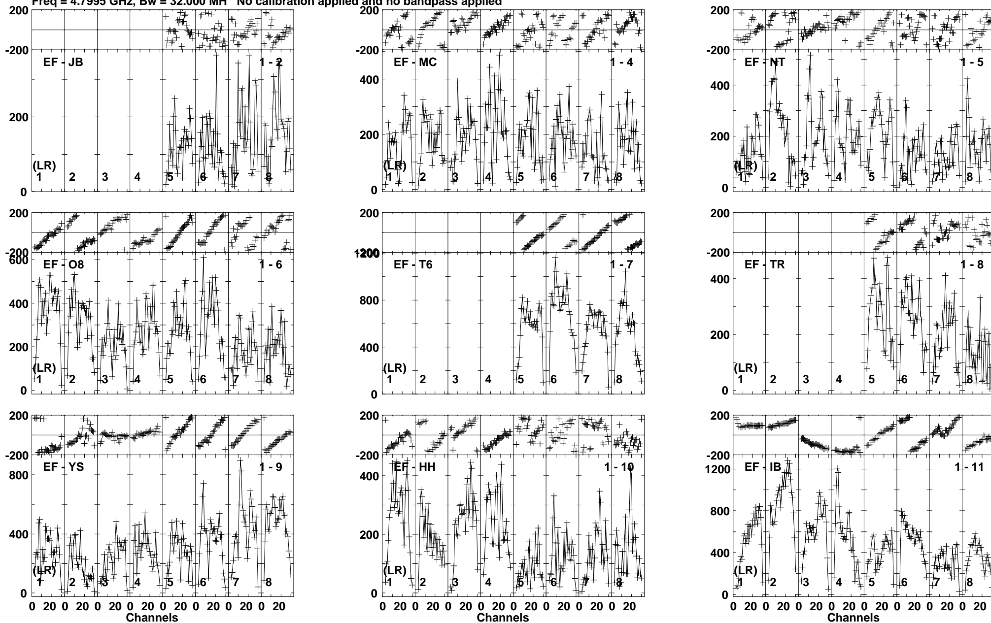
Lower frame: Micro Ampl Jy Top frame: Phas deg Vector averaged cross-power spectrum Baseline: EF (01) - JB (02) Timerange: 00/19:21:02 to 00/19:21:58
