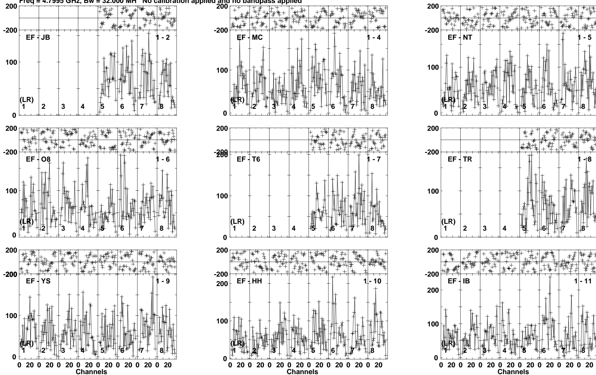
Lower frame: Micro Ampl Jy Top frame: Phas deg Vector averaged cross-power spectrum Baseline: EF (01) - JB (02) Timerange: 00/19:57:22 to 00/20:00:48
