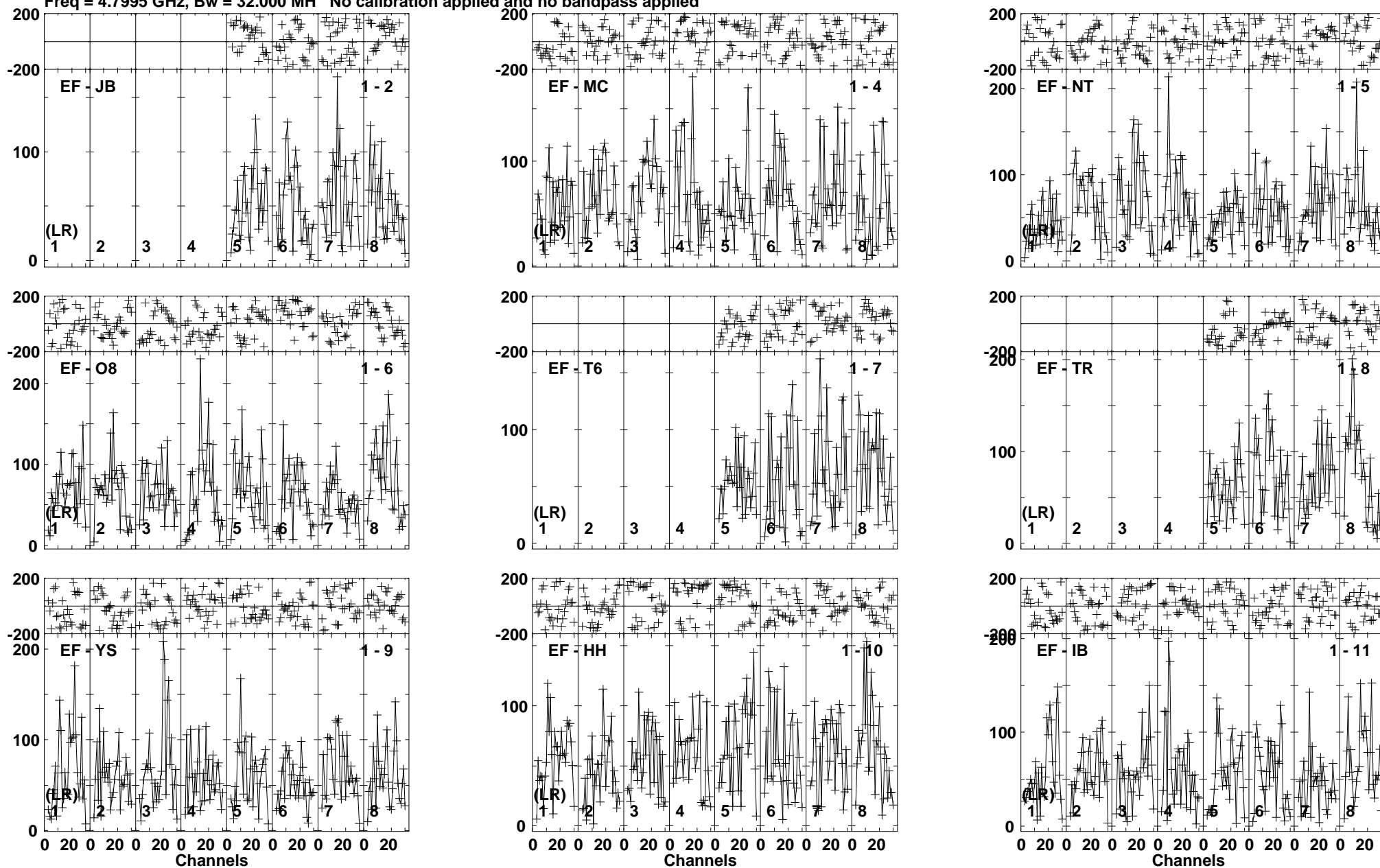
Lower frame: Micro Ampl Jy Top frame: Phas deg Vector averaged cross-power spectrum Baseline: EF (01) - JB (02) Timerange: 00/19:16:52 to 00/19:20:18
