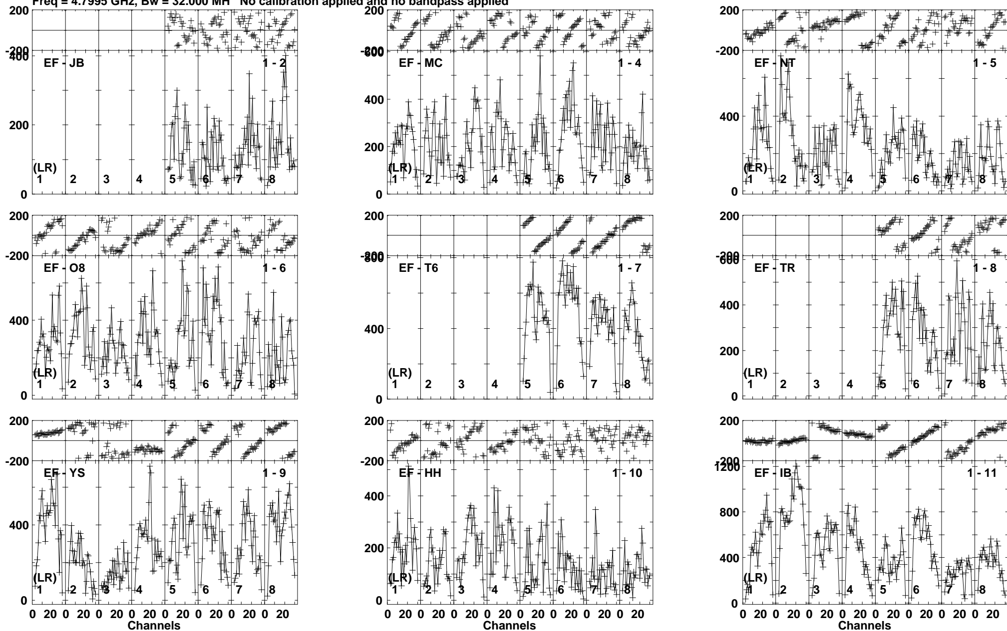
Lower frame: Micro Ampl Jy Top frame: Phas deg Vector averaged cross-power spectrum Baseline: EF (01) - JB (02) Timerange: 00/19:00:12 to 00/19:01:38
