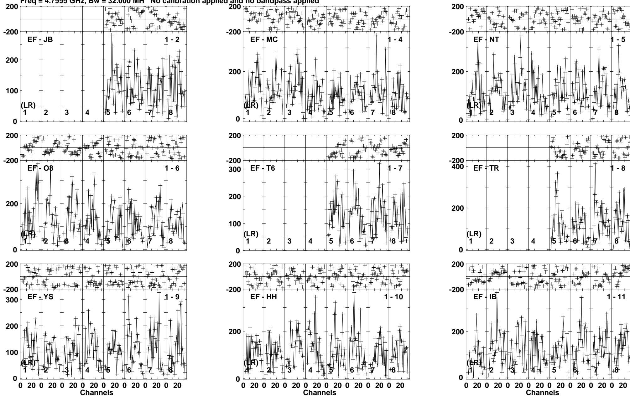
Lower frame: Micro Ampl Jy Top frame: Phas deg Vector averaged cross-power spectrum Baseline: EF (01) - JB (02) Timerange: 00/20:36:52 to 00/20:37:48
