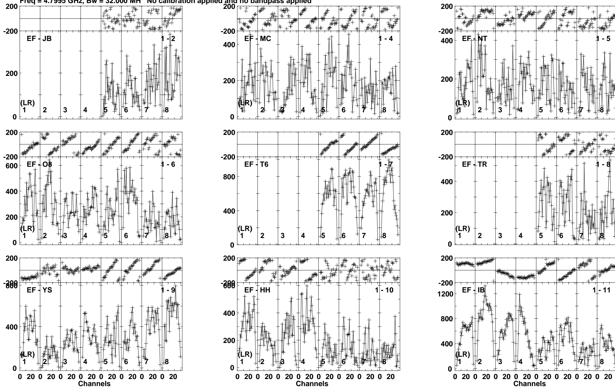
Lower frame: Micro Ampl Jy Top frame: Phas deg Vector averaged cross-power spectrum Baseline: EF (01) - JB (02) Timerange: 00:19:40:42 to 00:19:42:08
