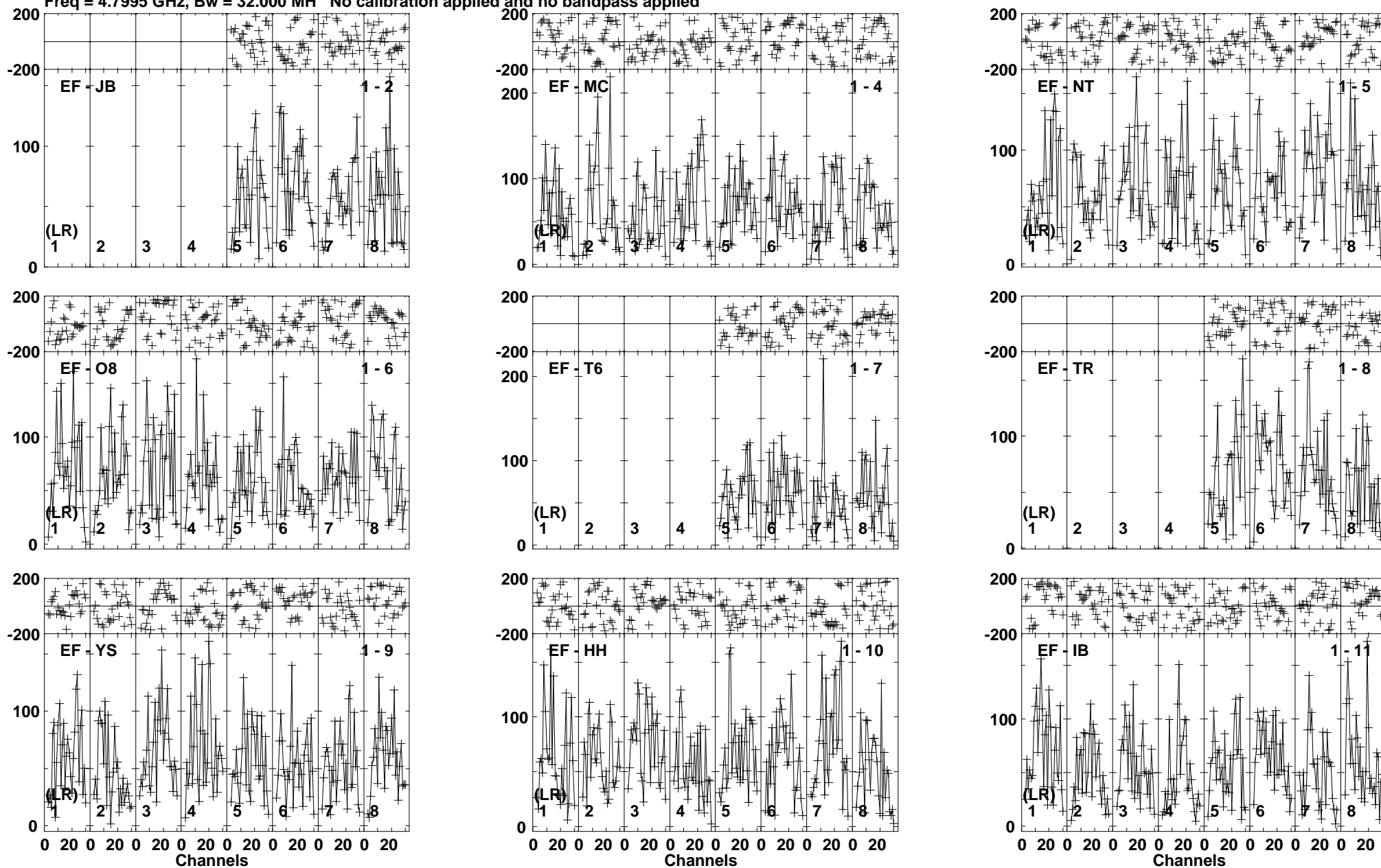
Lower frame: Micro Ampl Jy Top frame: Phas deg Vector averaged cross-power spectrum Baseline: EF (01) - JB (02) Timerange: 00/19:22:02 to 00/19:25:28
