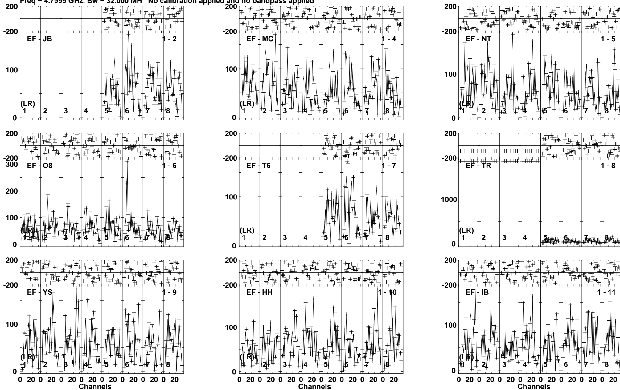
Lower frame: Micro Ampl Jy Top frame: Phas deg Vector averaged cross-power spectrum Baseline: EF (01) - JB (02) Timerange: 00/19:27:02 to 00/19:30:28
