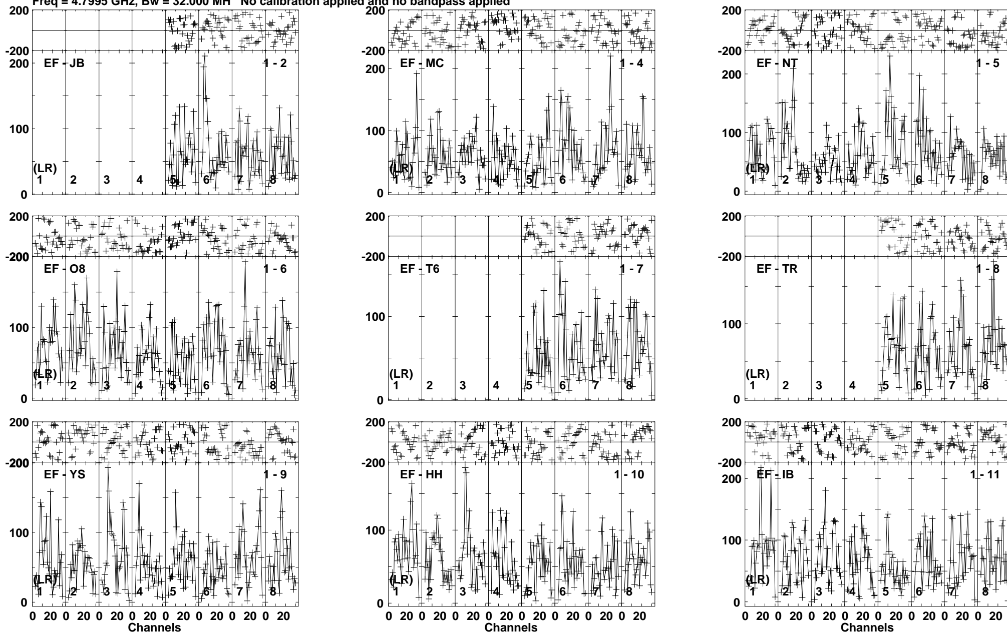
Lower frame: Micro Ampl Jy Top frame: Phas deg Vector averaged cross-power spectrum Baseline: EF (01) - JB (02) Timerange: 00/20:22:42 to 00/20:26:08
