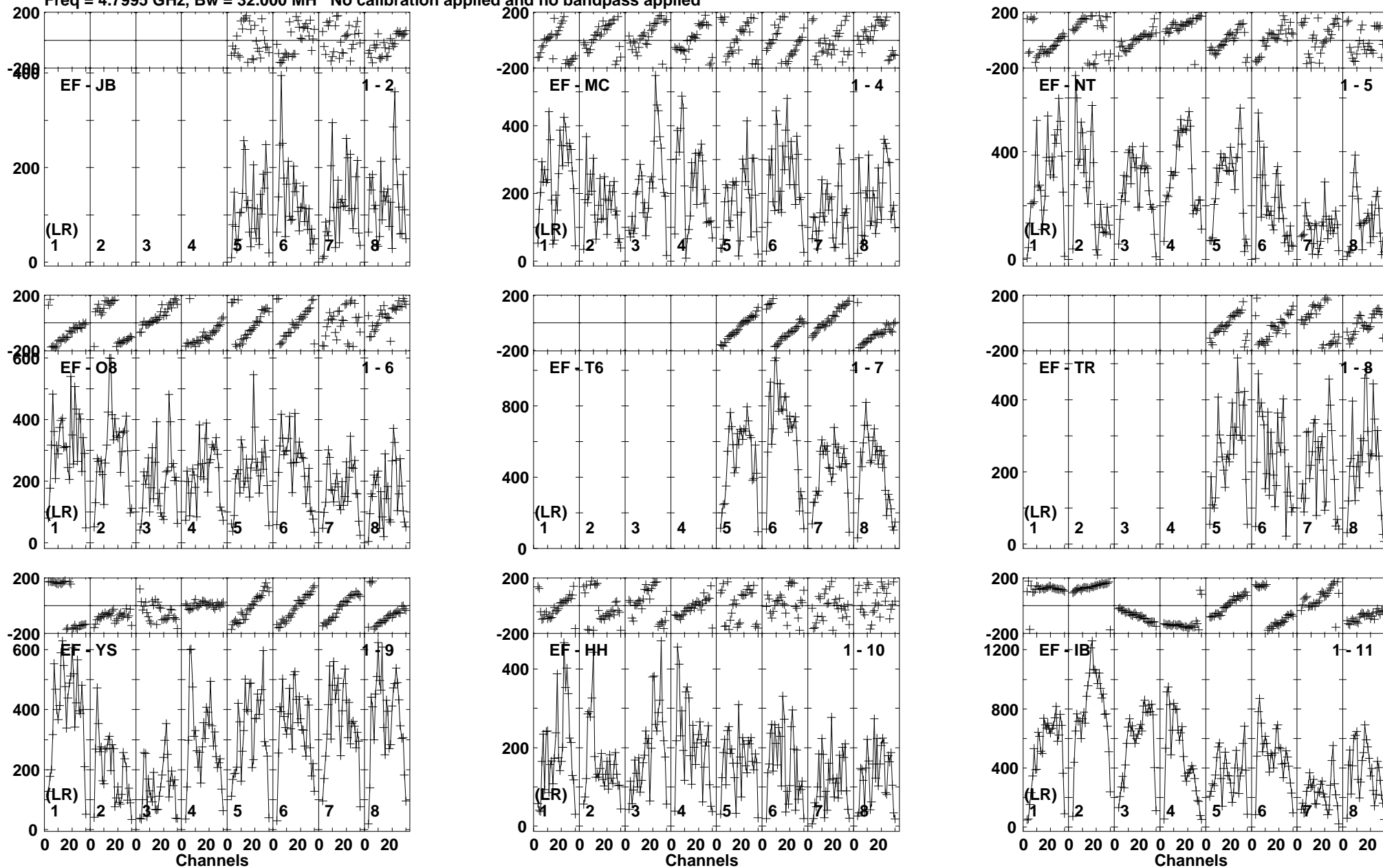
Lower frame: Micro Ampl Jy Top frame: Phas deg Vector averaged cross-power spectrum Baseline: EF (01) - JB (02) Timerange: 00/19:10:22 to 00/19:11:48
