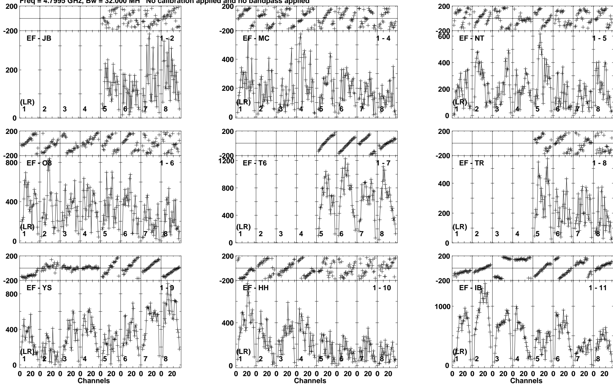
Lower frame: Micro Ampl Jy Top frame: Phas deg Vector averaged cross-power spectrum Baseline: EF (01) - JB (02) Timerange: 00/20:26:12 to 00/20:27:38
