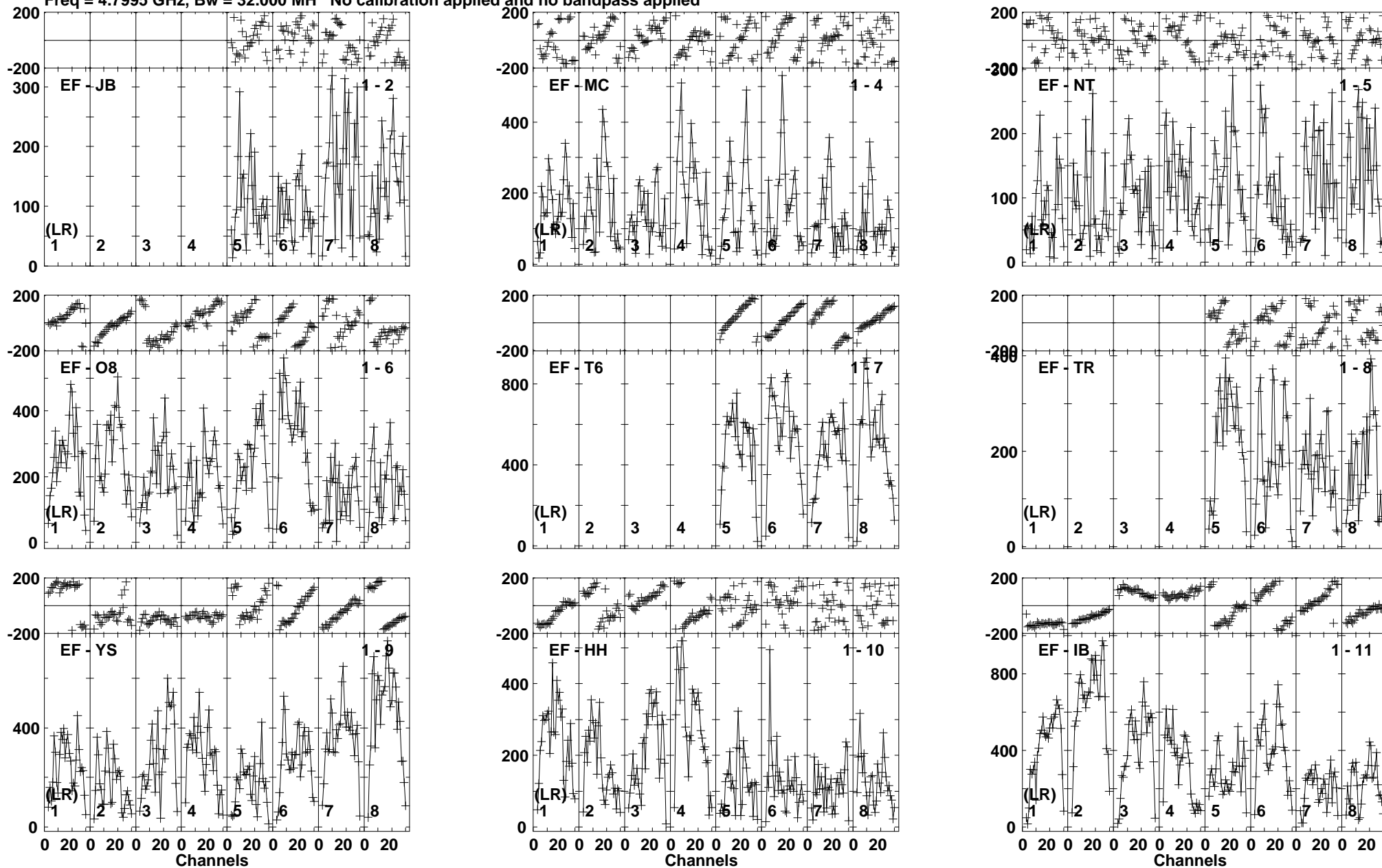
Lower frame: Micro Ampl Jy Top frame: Phas deg Vector averaged cross-power spectrum Baseline: EF (01) - JB (02) Timerange: 00/20:21:42 to 00/20:22:38
