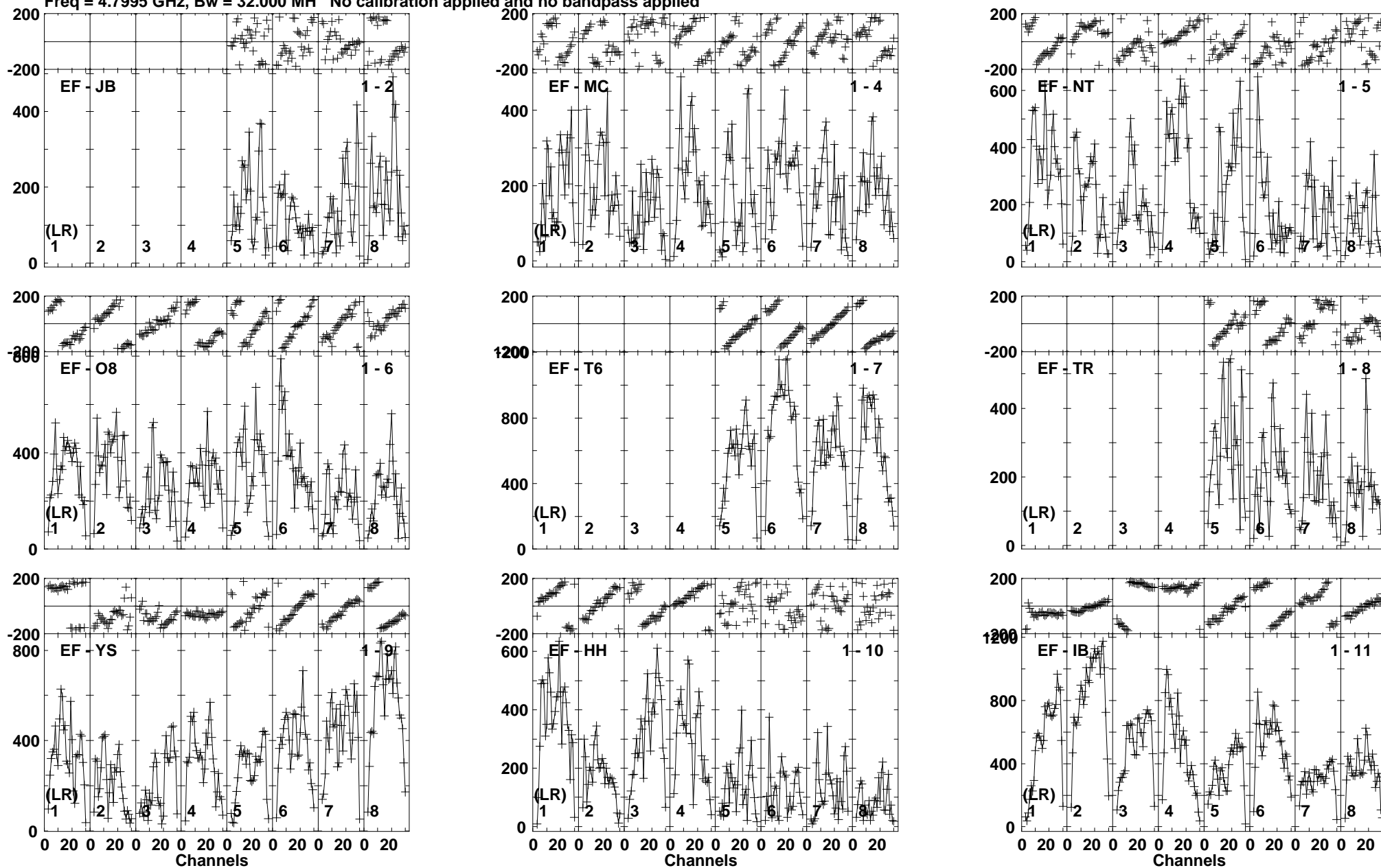
Lower frame: Micro Ampl Jy Top frame: Phas deg Vector averaged cross-power spectrum Baseline: EF (01) - JB (02) Timerange: 00/20:16:02 to 00/20:17:28
