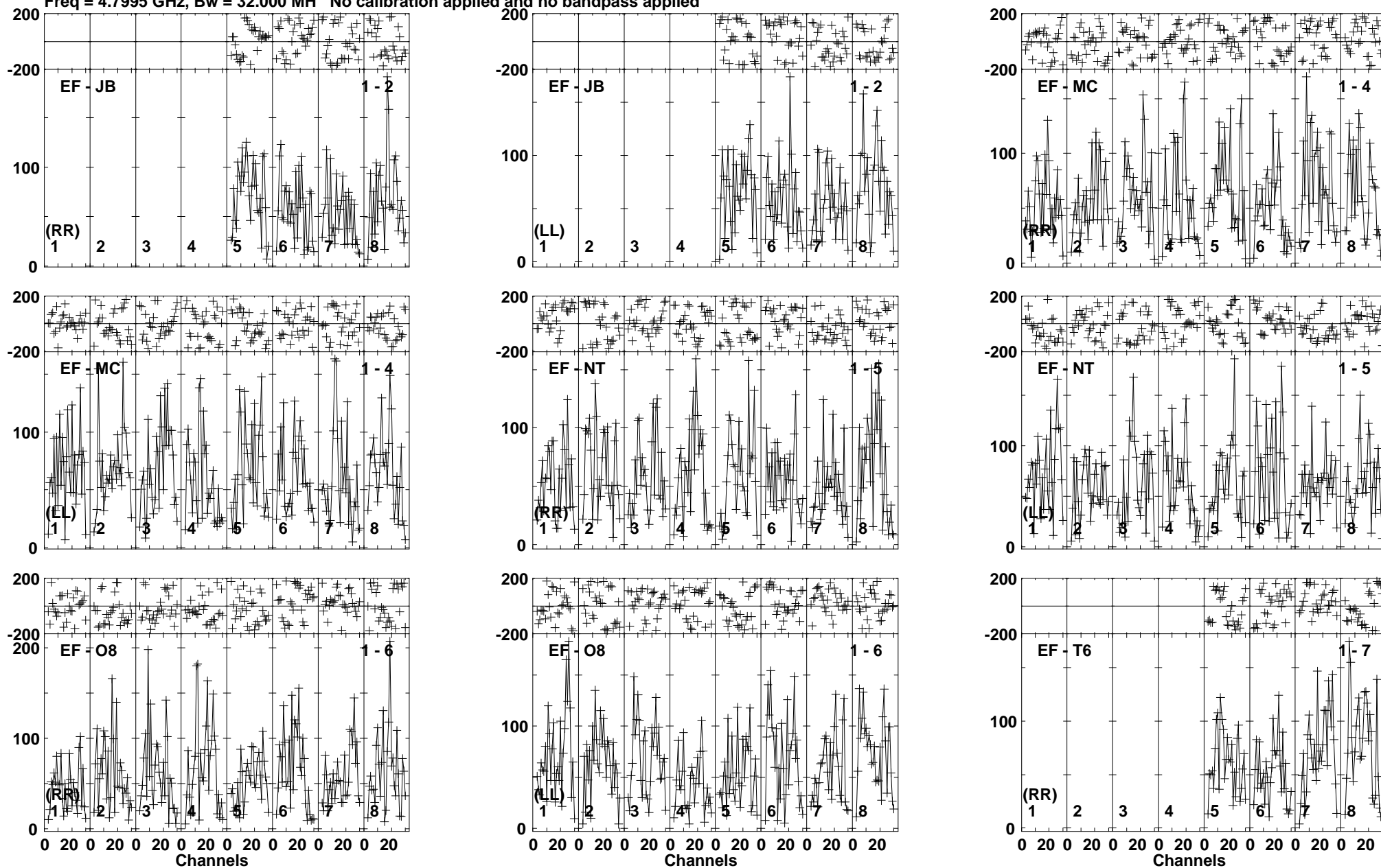
Lower frame: Micro Ampl Jy Top frame: Phas deg Vector averaged cross-power spectrum Baseline: EF (01) - JB (02) Timerange: 00/20:07:32 to 00/20:10:58
