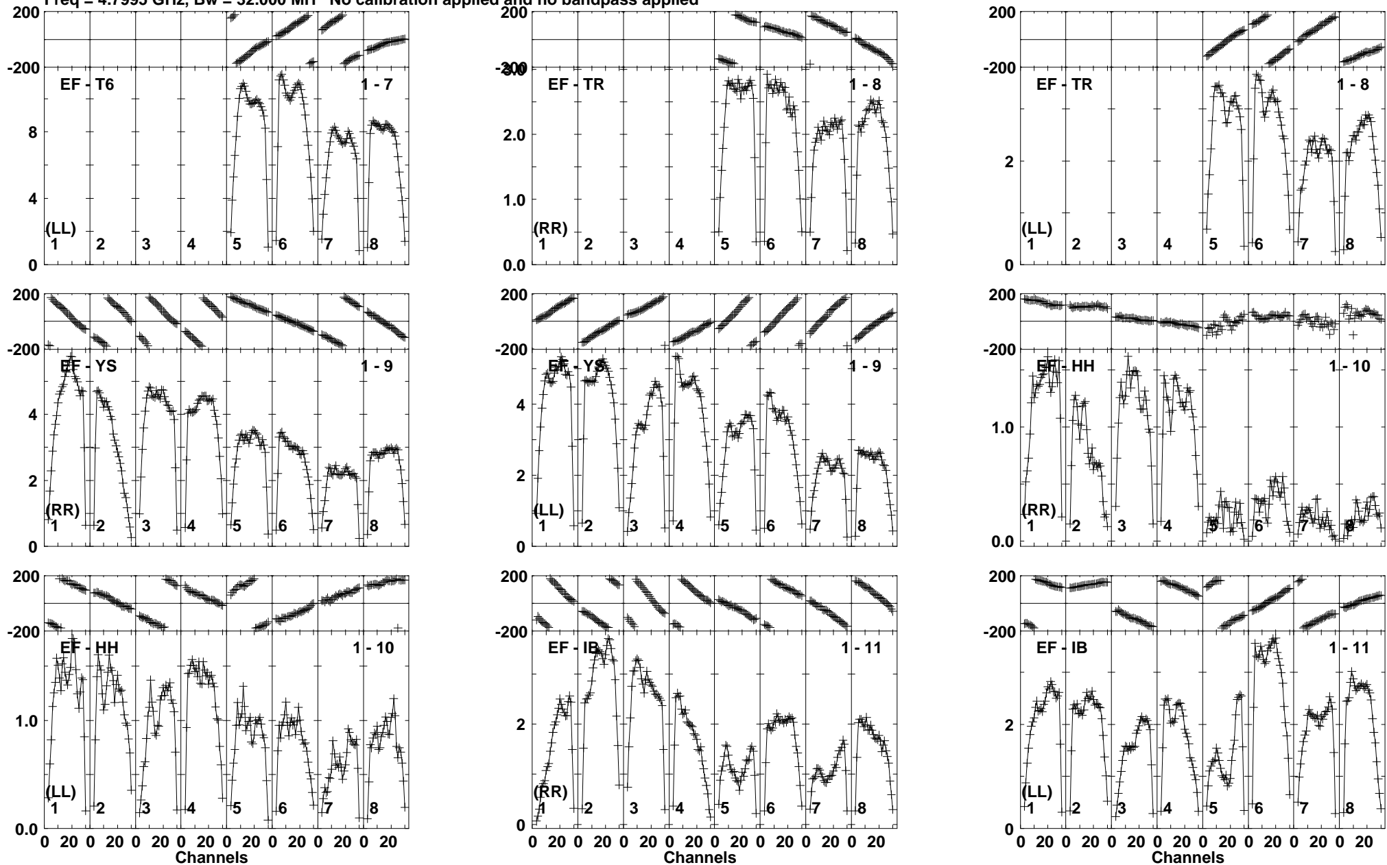
Lower frame: Milli Ampl Jy Top frame: Phas deg Vector averaged cross-power spectrum Baseline: EF (01) - T6 (07) Timerange: 00/19:36:12 to 00/19:37:08
