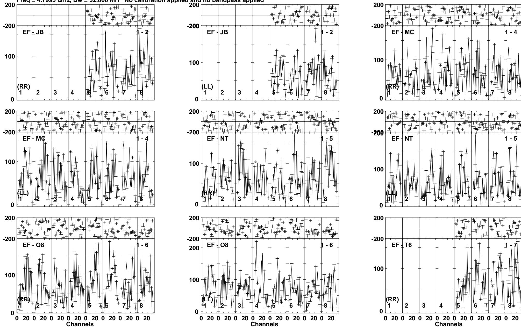
Lower frame: Micro Ampl Jy Top frame: Phas deg Vector averaged cross-power spectrum Baseline: EF (01) - JB (02) Timerange: 00:19:06:52 to 00:19:10:18
