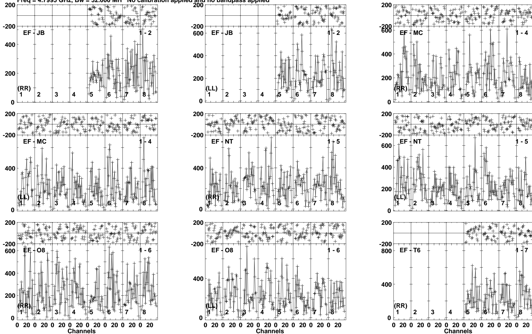
Lower frame: Micro Ampl Jy Top frame: Phas deg Vector averaged cross-power spectrum Baseline: EF (01) - JB (02) Timerange: 00:18:35:32 to 00:18:36:28
