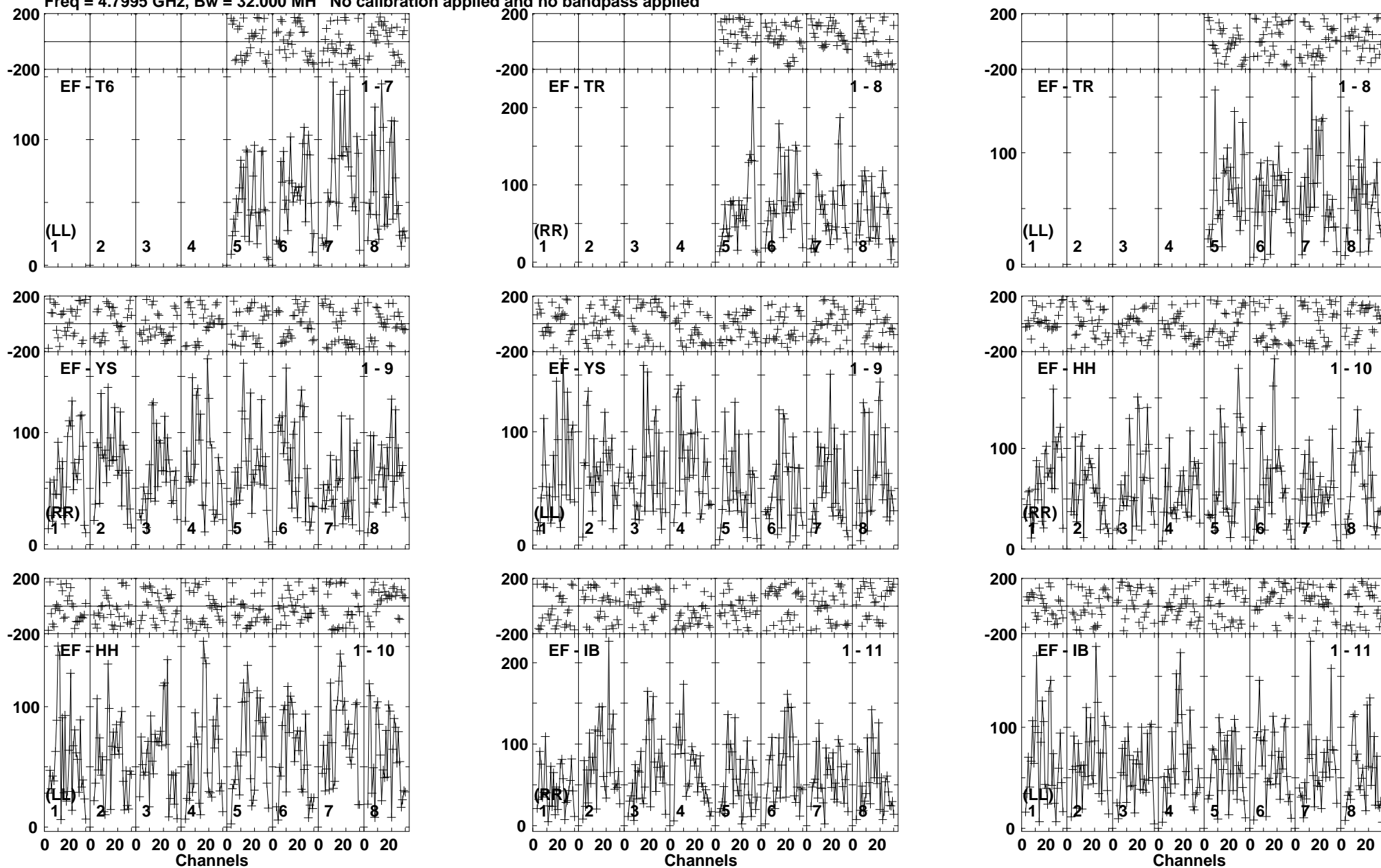
Lower frame: Micro Ampl Jy Top frame: Phas deg Vector averaged cross-power spectrum Baseline: EF (01) - T6 (07) Timerange: 00/19:37:12 to 00/19:40:38
