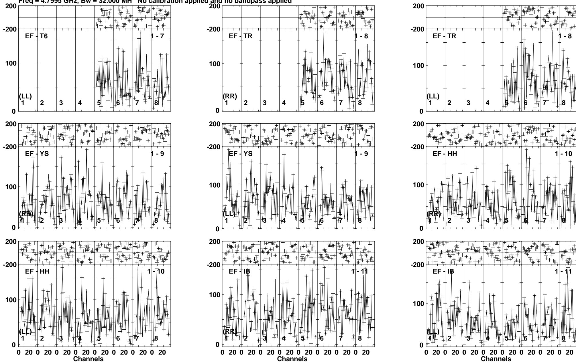
Lower frame: Micro Ampl Jy Top frame: Phas deg Vector averaged cross-power spectrum Baseline: EF (01) - T6 (07) Timerange: 00/20:27:42 to 00/20:31:08
