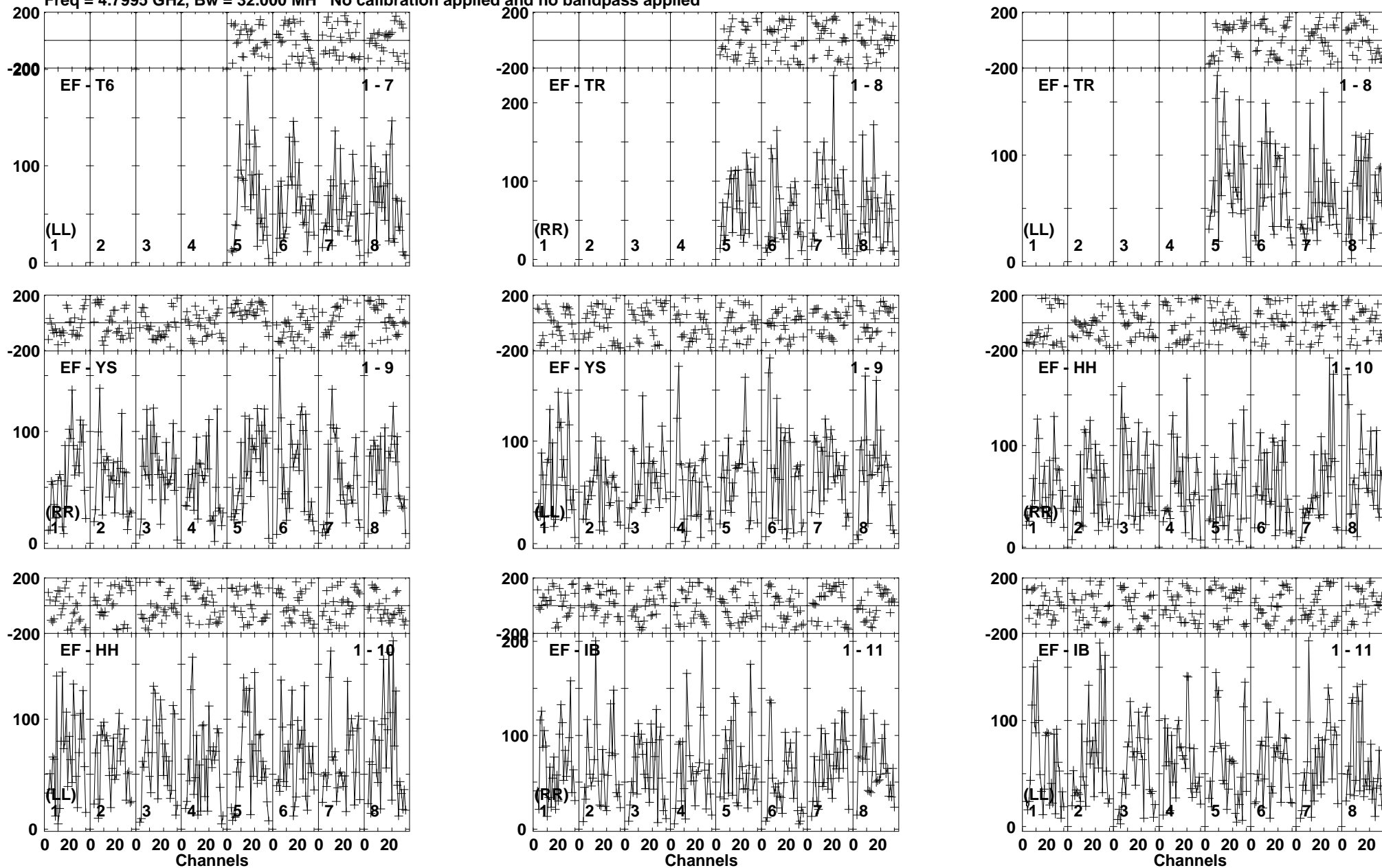
Lower frame: Micro Ampl Jy Top frame: Phas deg Vector averaged cross-power spectrum Baseline: EF (01) - T6 (07) Timerange: 00/19:42:12 to 00/19:45:38
