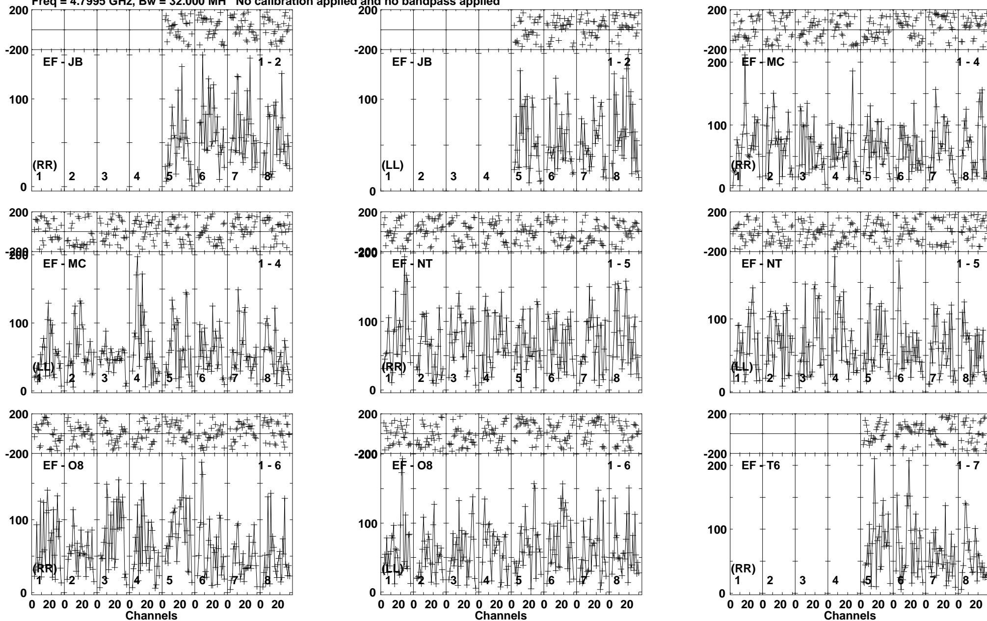
Lower frame: Micro Ampl Jy Top frame: Phas deg Vector averaged cross-power spectrum Baseline: EF (01) - JB (02) Timerange: 00:18:46:32 to 00:18:49:58
