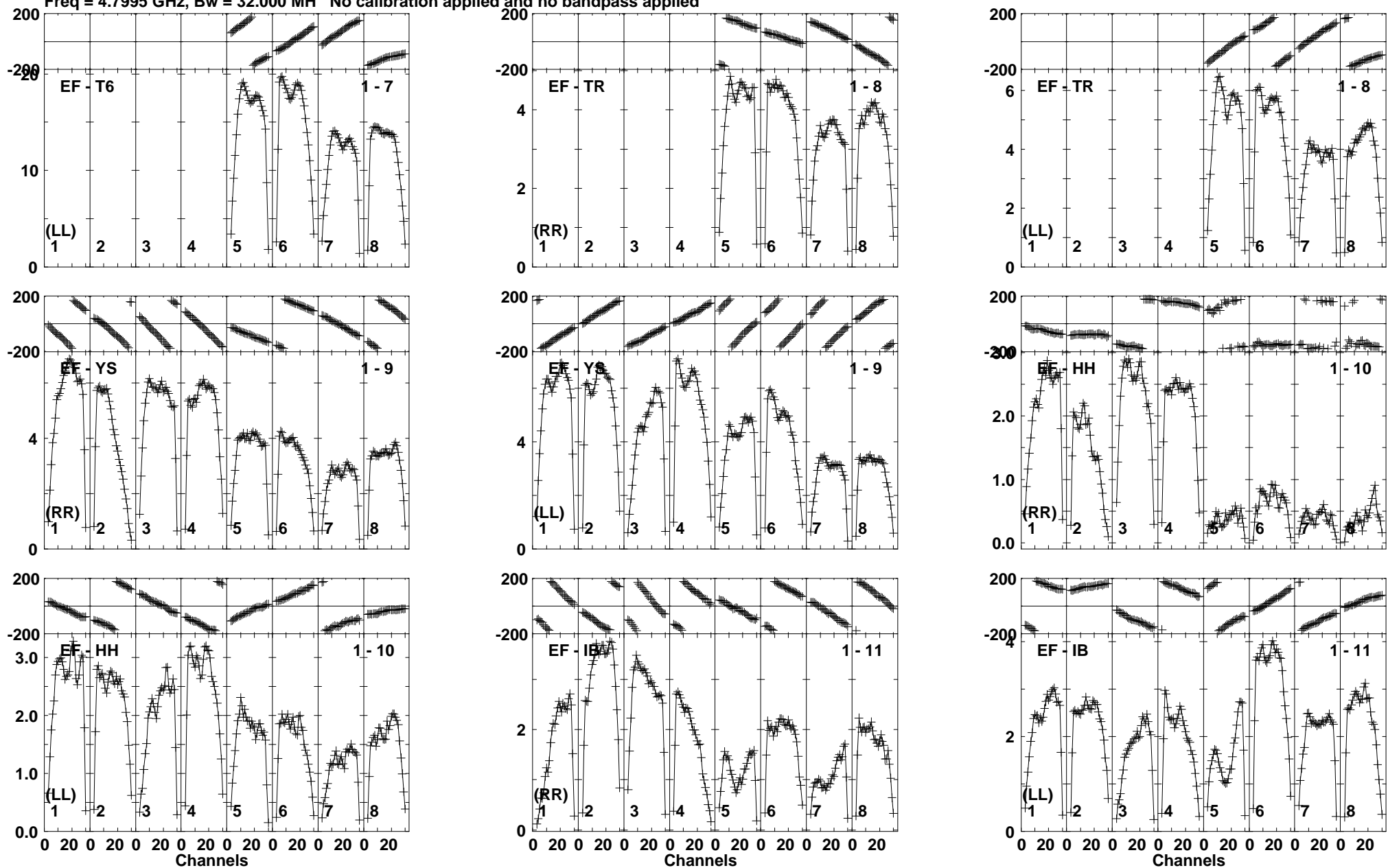
Lower frame: Milli Ampl Jy Top frame: Phas deg Vector averaged cross-power spectrum Baseline: EF (01) - T6 (07) Timerange: 00:19:40:42 to 00:19:42:08
