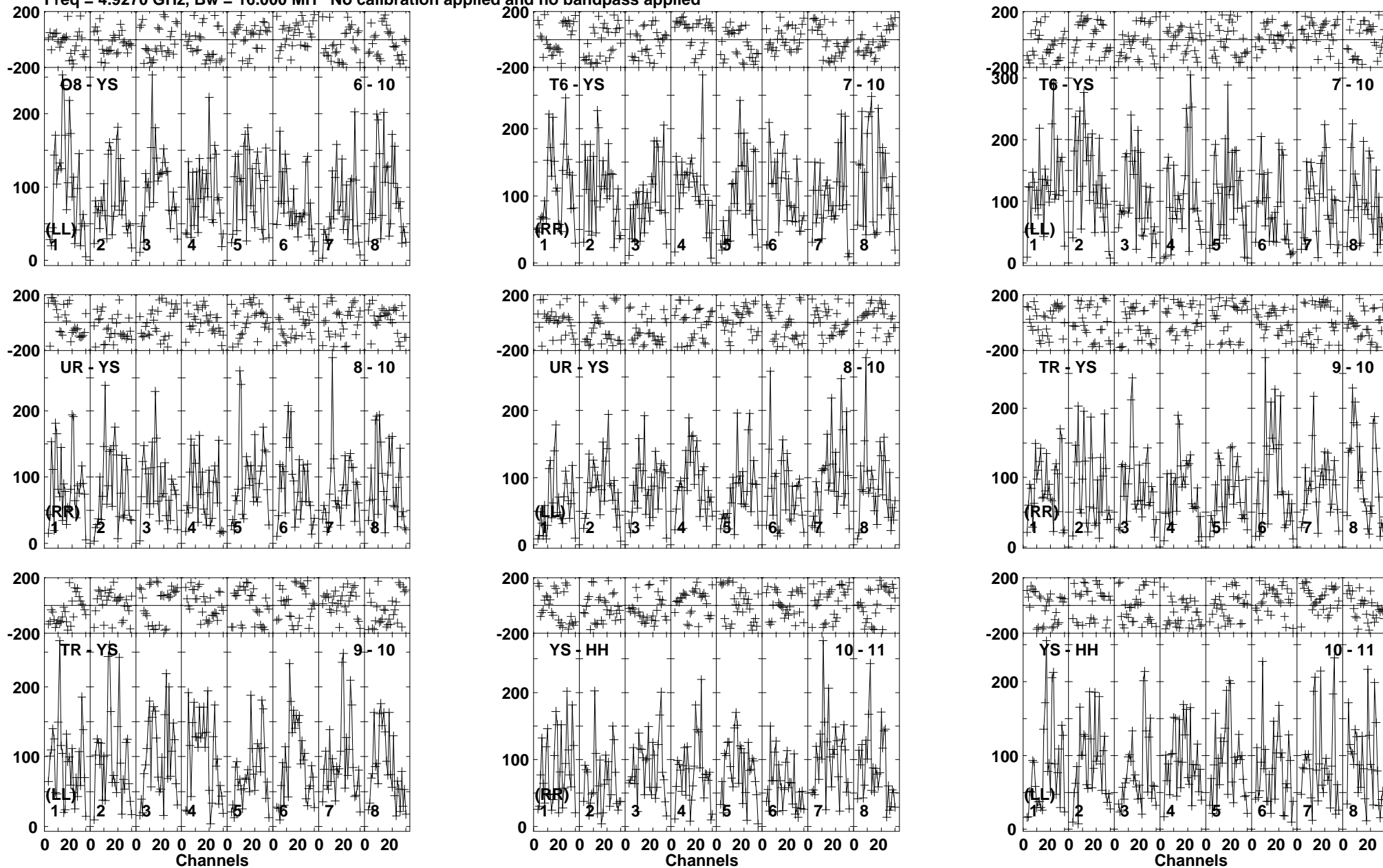
Lower frame: Micro Ampl Jy Top frame: Phas deg Vector averaged cross-power spectrum Baseline: O8 (06) - YS (10) Timerange: 00/06:38:51 to 00/06:42:19
