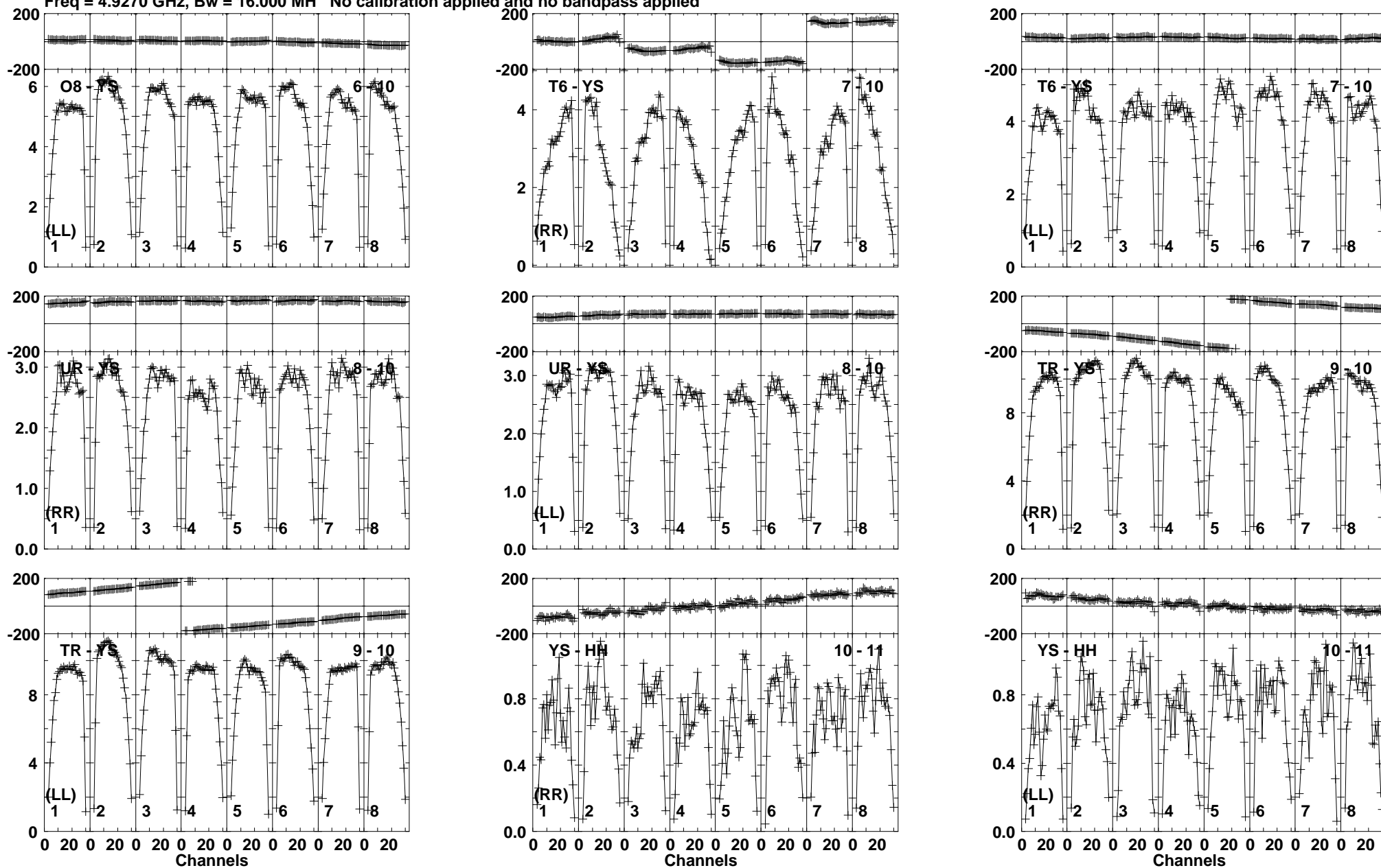
Lower frame: Milli Ampl Jy Top frame: Phas deg Vector averaged cross-power spectrum Baseline: O8 (06) - YS (10) Timerange: 00/07:29:51 to 00/07:31:19
