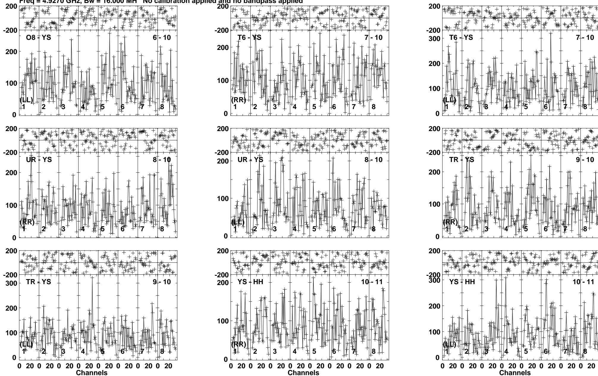
Lower frame: Micro Ampl Jy Top frame: Phas deg Vector averaged cross-power spectrum Baseline: O8 (06) - YS (10) Timerange: 00/04:17:21 to 00/04:20:49
