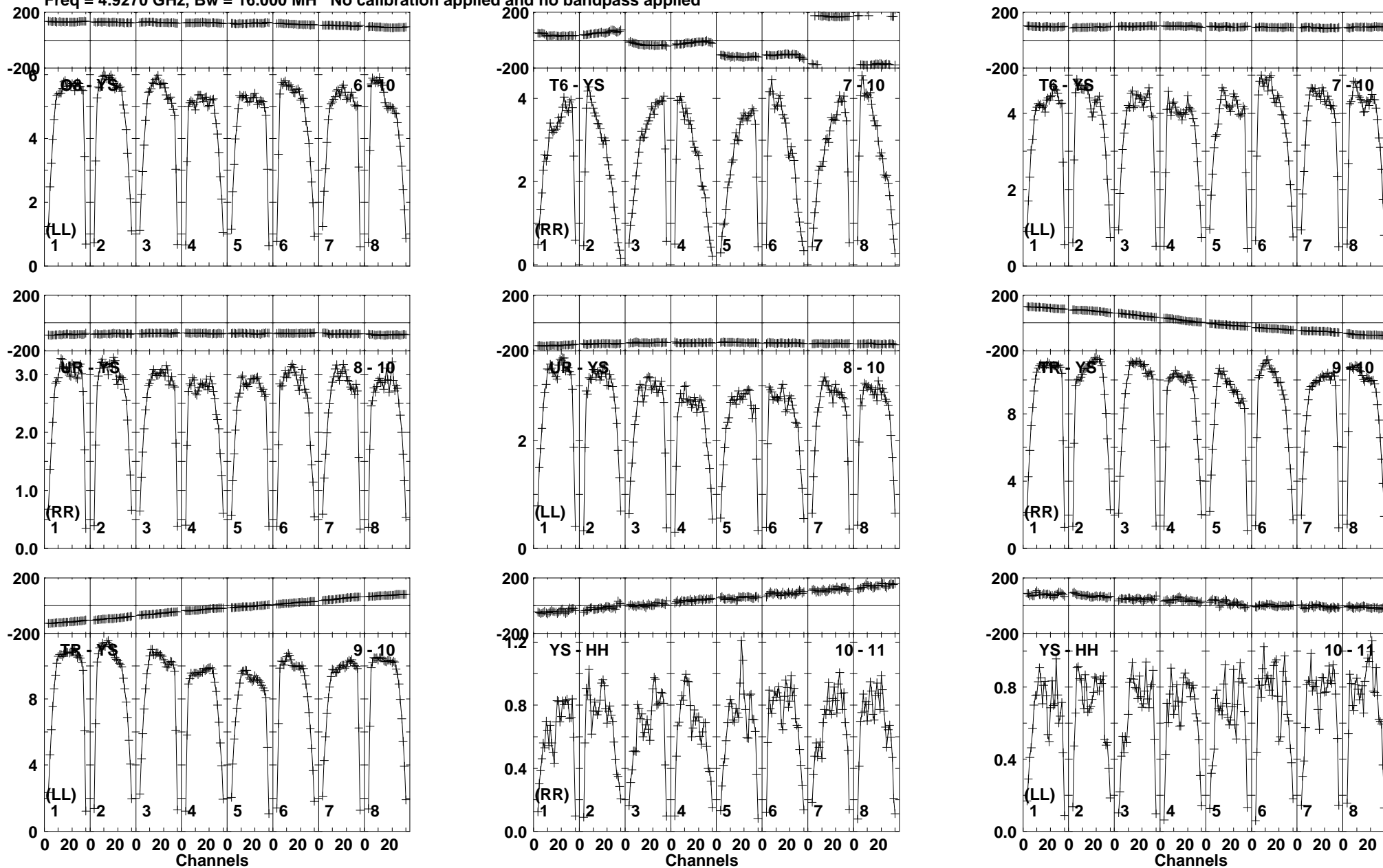
Lower frame: Milli Ampl Jy Top frame: Phas deg Vector averaged cross-power spectrum Baseline: O8 (06) - YS (10) Timerange: 00/06:22:01 to 00/06:23:19
