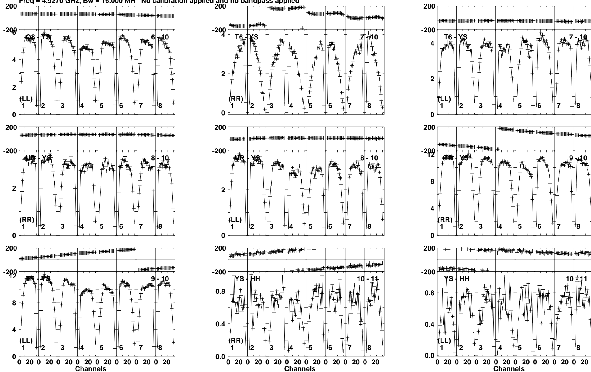
Lower frame: Milli Ampl Jy Top frame: Phas deg Vector averaged cross-power spectrum Baseline: O8 (06) - YS (10) Timerange: 00/05:23:51 to 00/05:25:19
