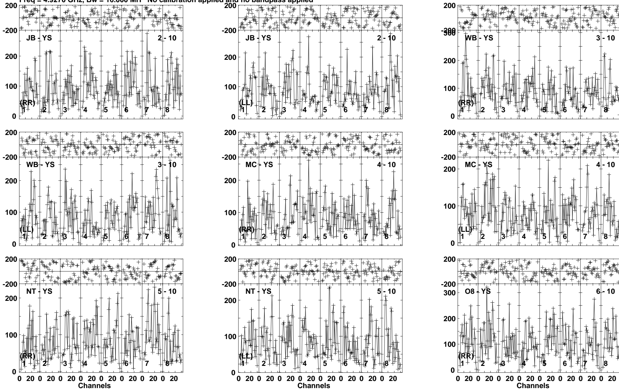
Lower frame: Micro Ampl Jy Top frame: Phas deg Vector averaged cross-power spectrum Baseline: JB (02) - YS (10) Timerange: 00/06:02:21 to 00/06:05:49
