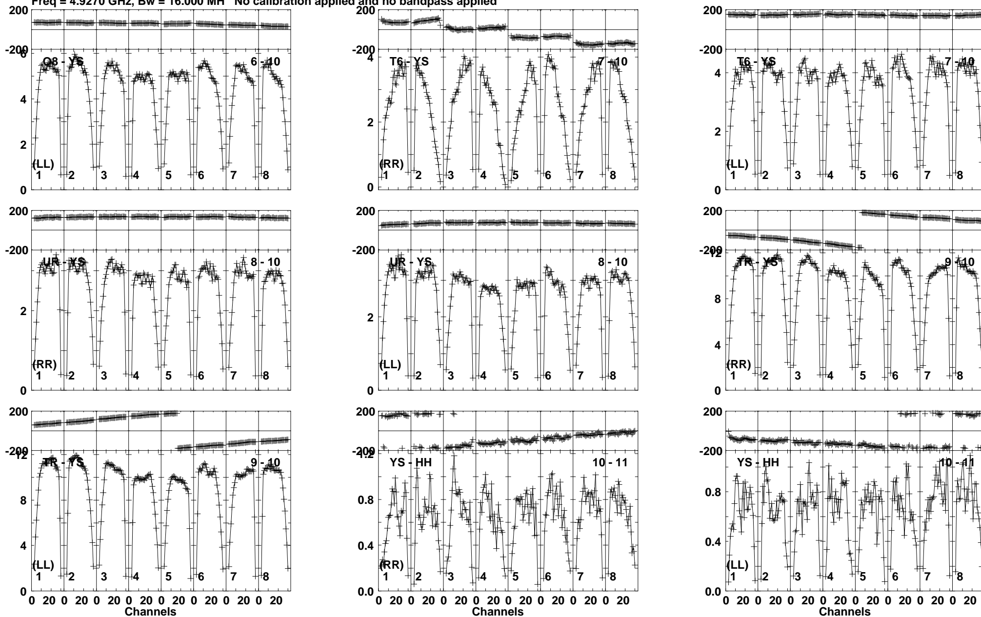
Lower frame: Milli Ampl Jy Top frame: Phas deg Vector averaged cross-power spectrum Baseline: O8 (06) - YS (10) Timerange: 00/05:44:51 to 00/05:46:19
