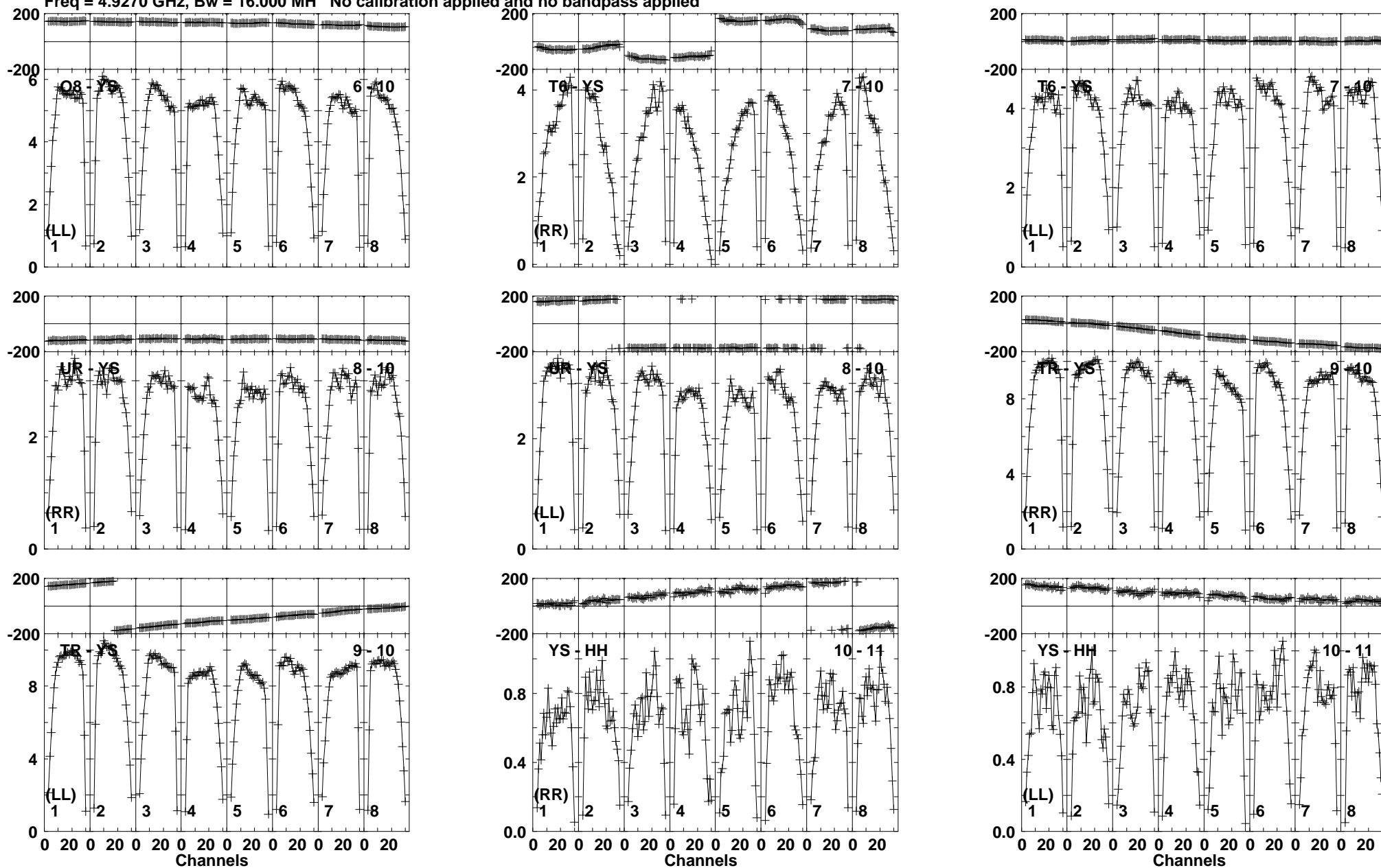
Lower frame: Milli Ampl Jy Top frame: Phas deg Vector averaged cross-power spectrum Baseline: O8 (06) - YS (10) Timerange: 00/06:11:31 to 00/06:12:49
