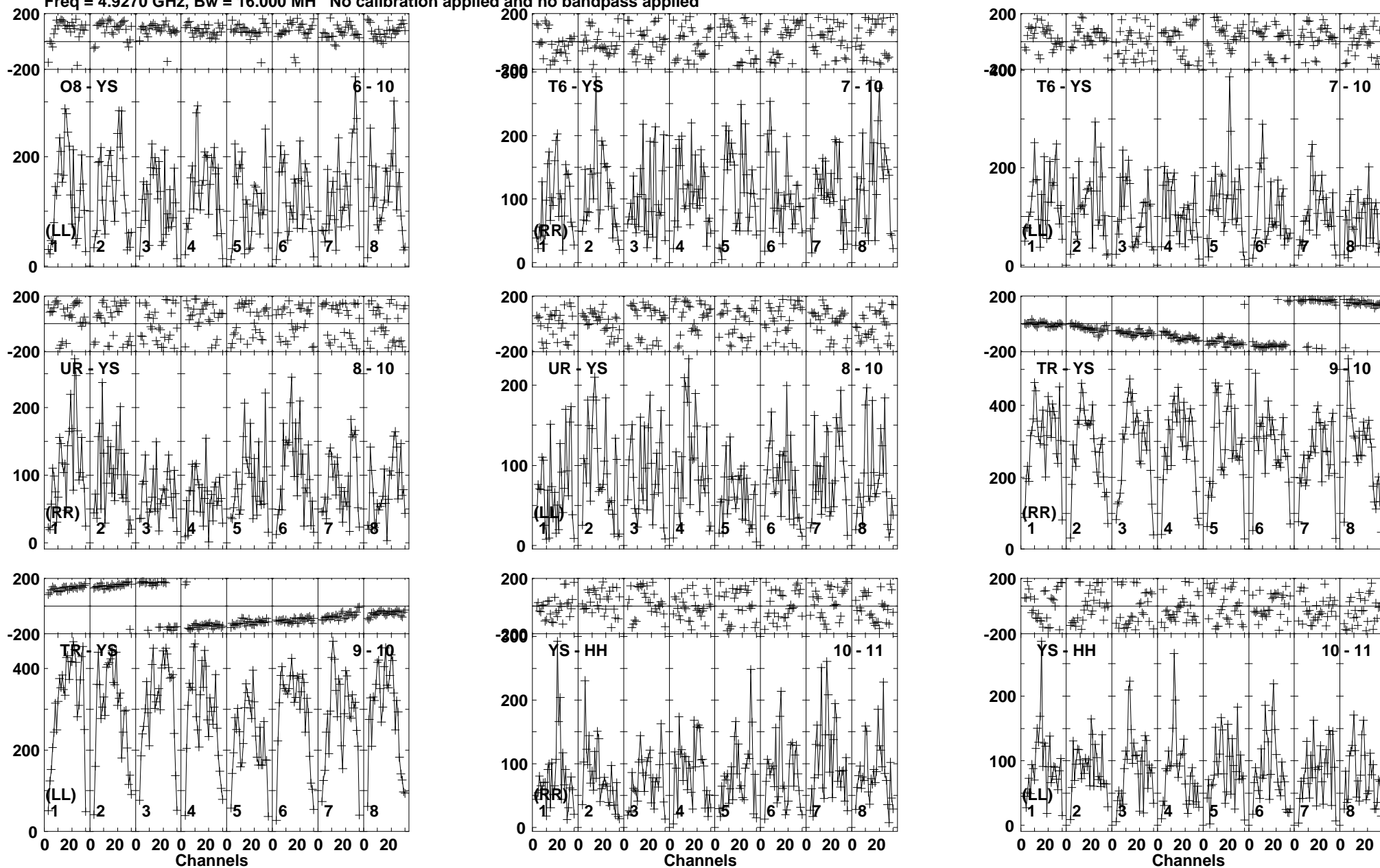
Lower frame: Micro Ampl Jy Top frame: Phas deg Vector averaged cross-power spectrum Baseline: O8 (06) - YS (10) Timerange: 00/05:46:21 to 00/05:49:49
