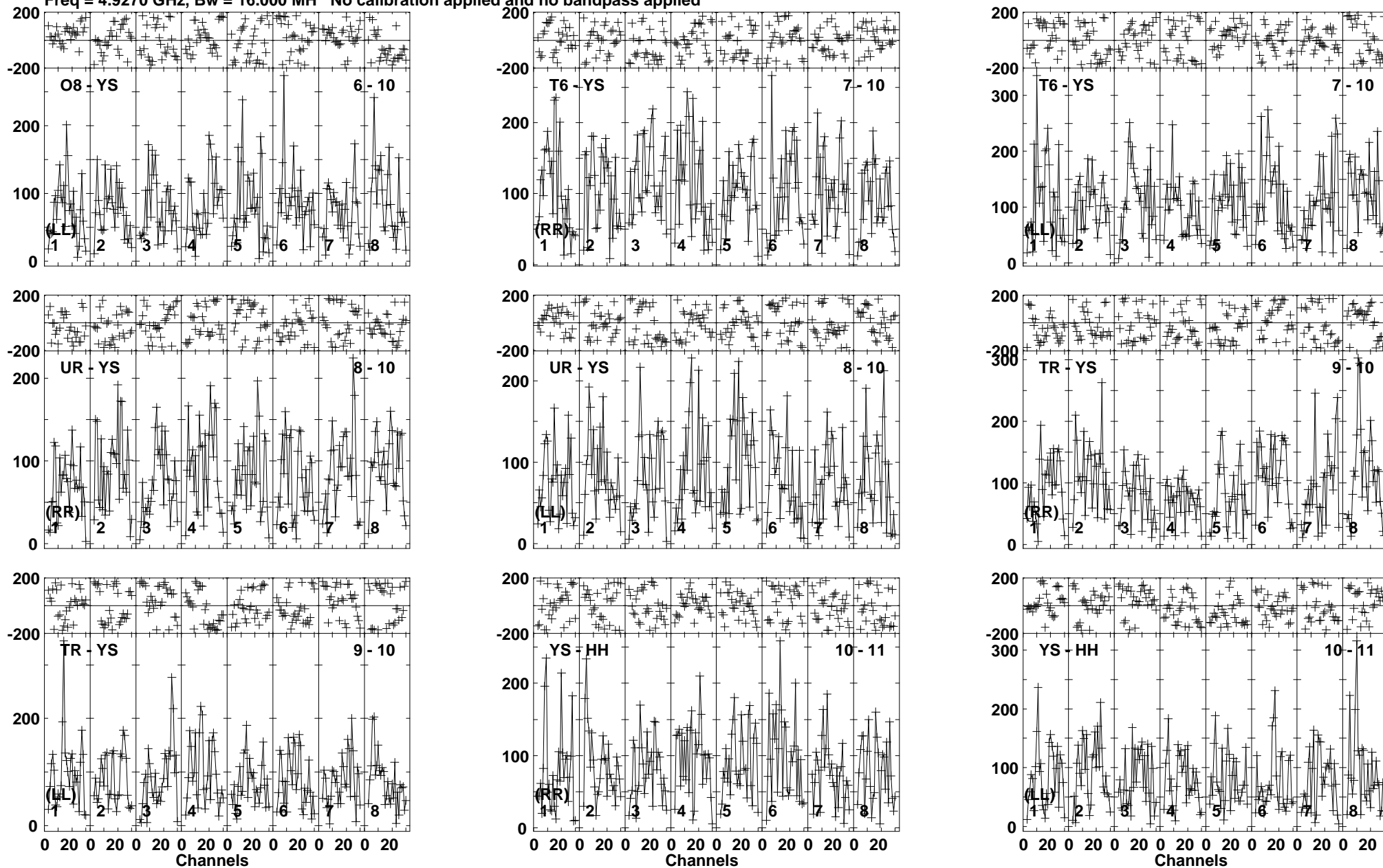
Lower frame: Micro Ampl Jy Top frame: Phas deg Vector averaged cross-power spectrum Baseline: O8 (06) - YS (10) Timerange: 00/07:26:21 to 00/07:29:49
