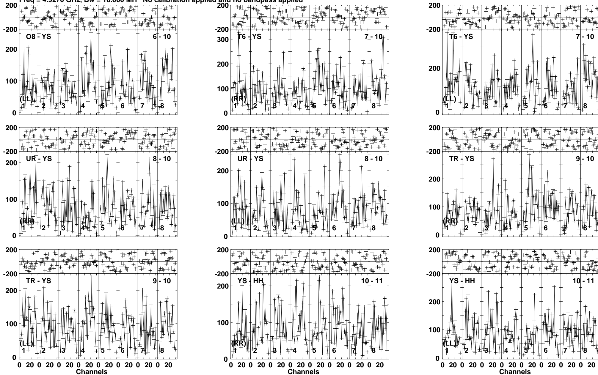
Lower frame: Micro Ampl Jy Top frame: Phas deg Vector averaged cross-power spectrum Baseline: O8 (06) - YS (10) Timerange: 00/05:30:51 to 00/05:34:19
