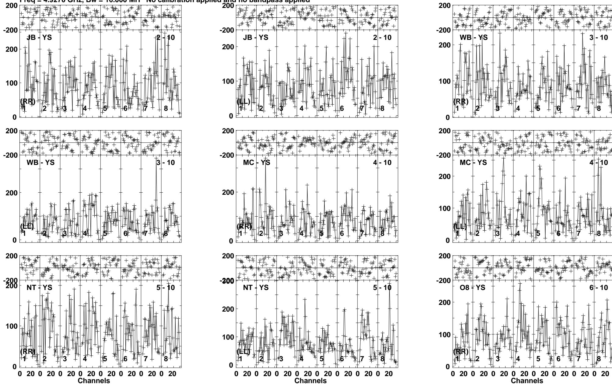
Lower frame: Micro Ampl Jy Top frame: Phas deg Vector averaged cross-power spectrum Baseline: JB (02) - YS (10) Timerange: 00/06:44:21 to 00/06:47:49
