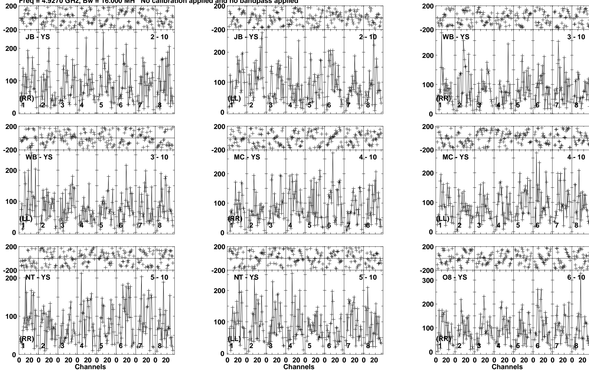
Lower frame: Micro Ampl Jy Top frame: Phas deg Vector averaged cross-power spectrum Baseline: JB (02) - YS (10) Timerange: 00/04:32:51 to 00/04:36:19
