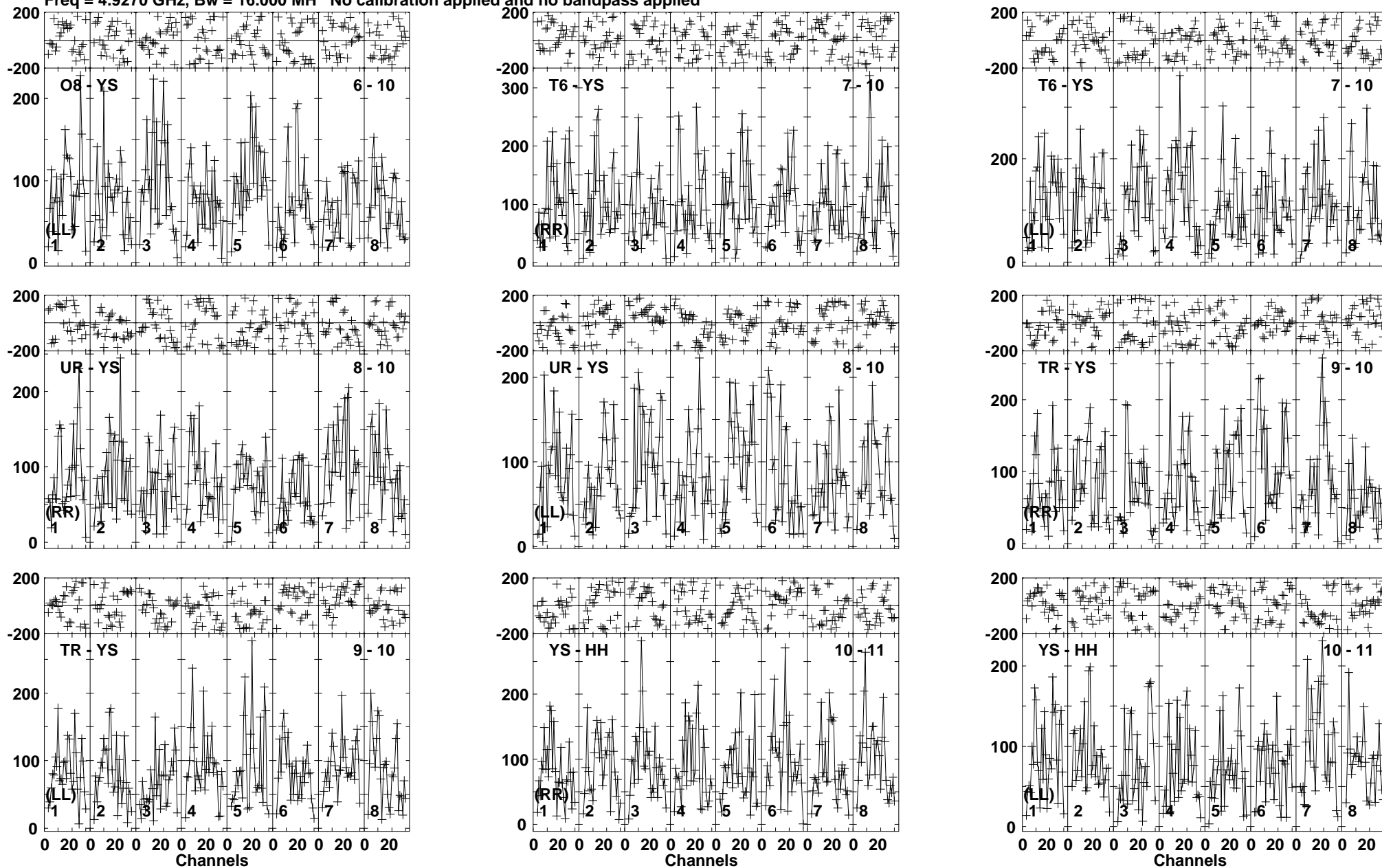
Lower frame: Micro Ampl Jy Top frame: Phas deg Vector averaged cross-power spectrum Baseline: O8 (06) - YS (10) Timerange: 00/05:14:51 to 00/05:18:19
