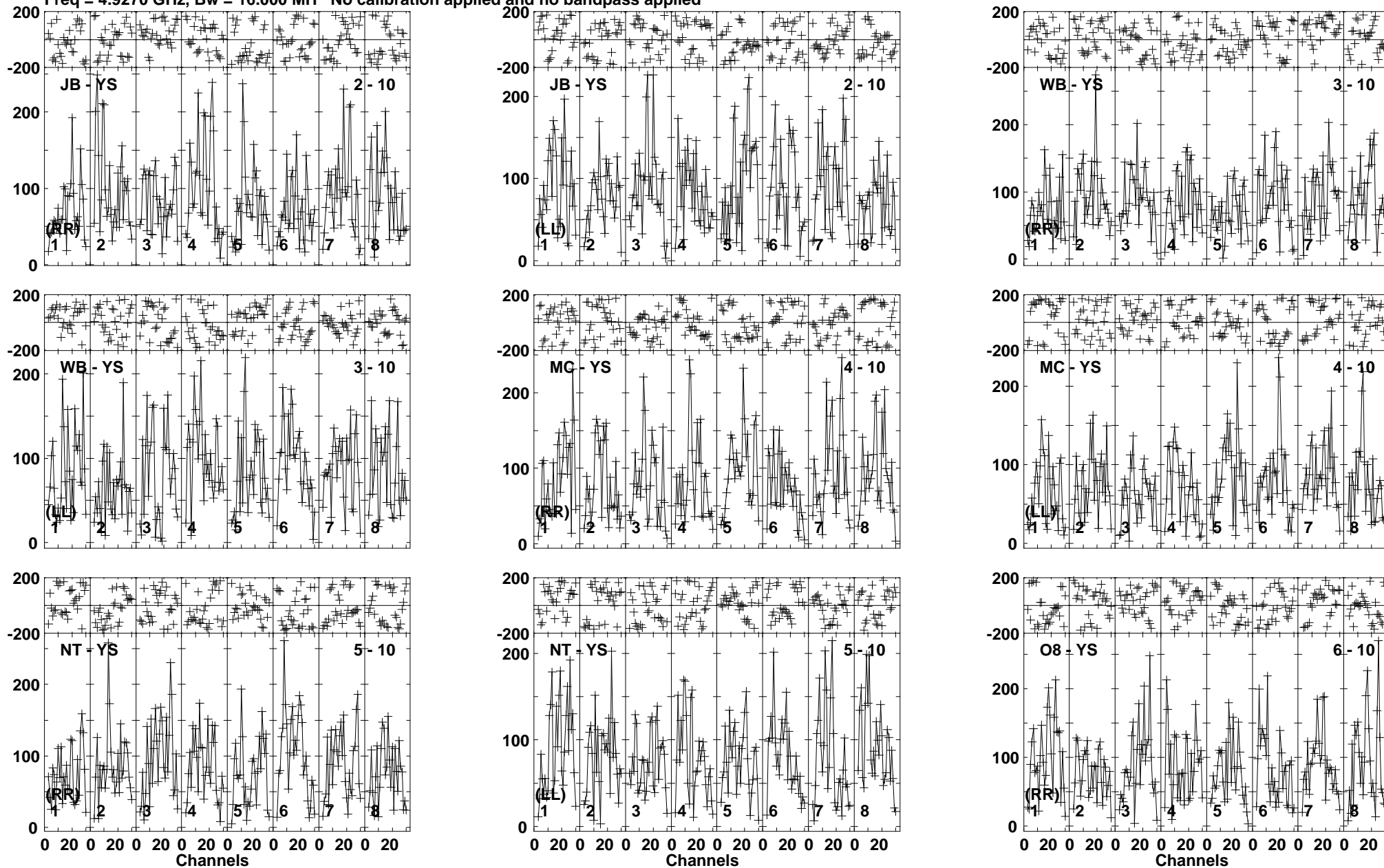
Lower frame: Micro Ampl Jy Top frame: Phas deg Vector averaged cross-power spectrum Baseline: JB (02) - YS (10) Timerange: 00/04:11:51 to 00/04:15:19
