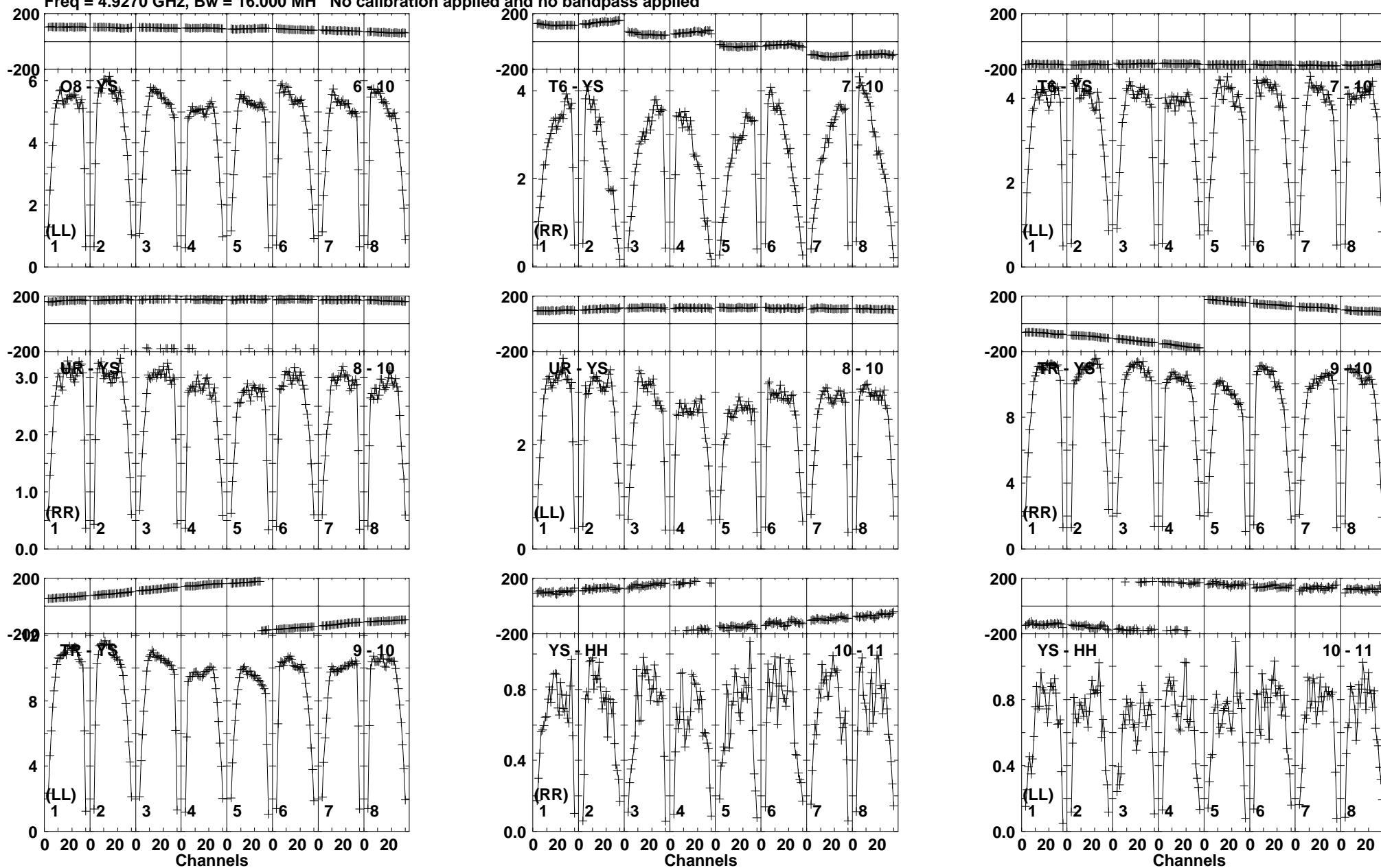
Lower frame: Milli Ampl Jy Top frame: Phas deg Vector averaged cross-power spectrum Baseline: O8 (06) - YS (10) Timerange: 00/05:50:31 to 00/05:51:49
