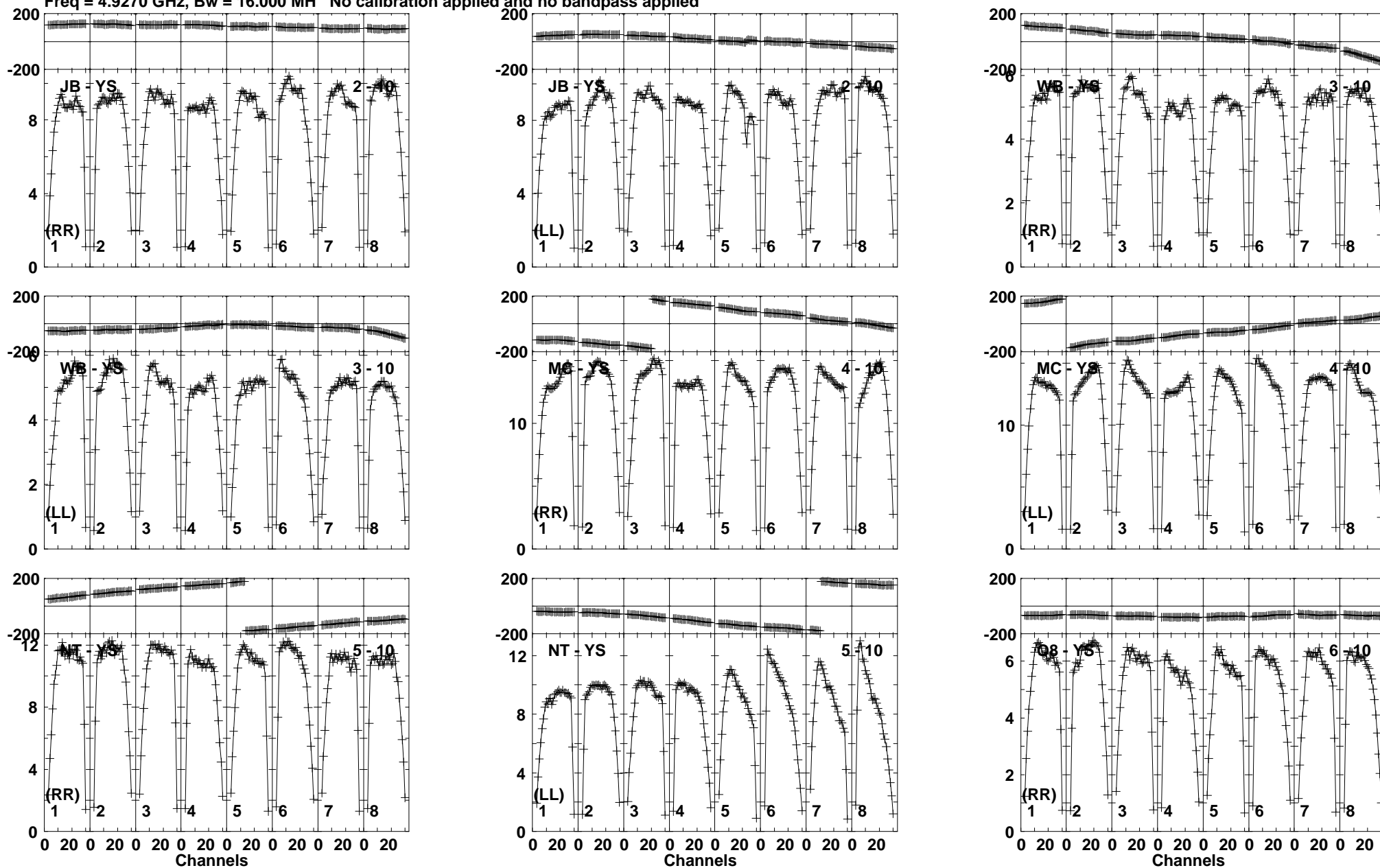
Lower frame: Milli Ampl Jy Top frame: Phas deg Vector averaged cross-power spectrum Baseline: JB (02) - YS (10) Timerange: 00/07:19:21 to 00/07:20:49
