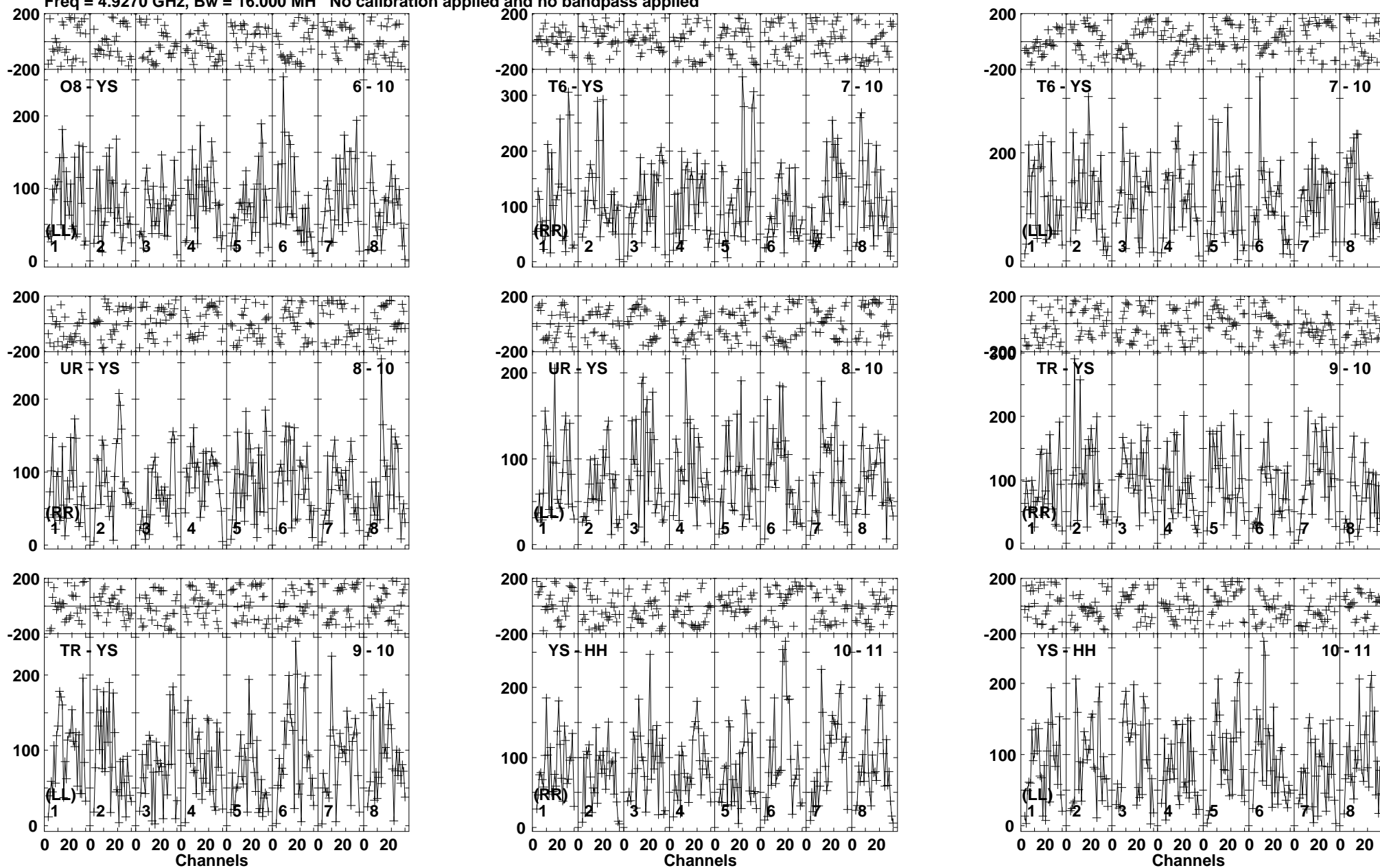
Lower frame: Micro Ampl Jy Top frame: Phas deg Vector averaged cross-power spectrum Baseline: O8 (06) - YS (10) Timerange: 00/05:41:21 to 00/05:44:49
