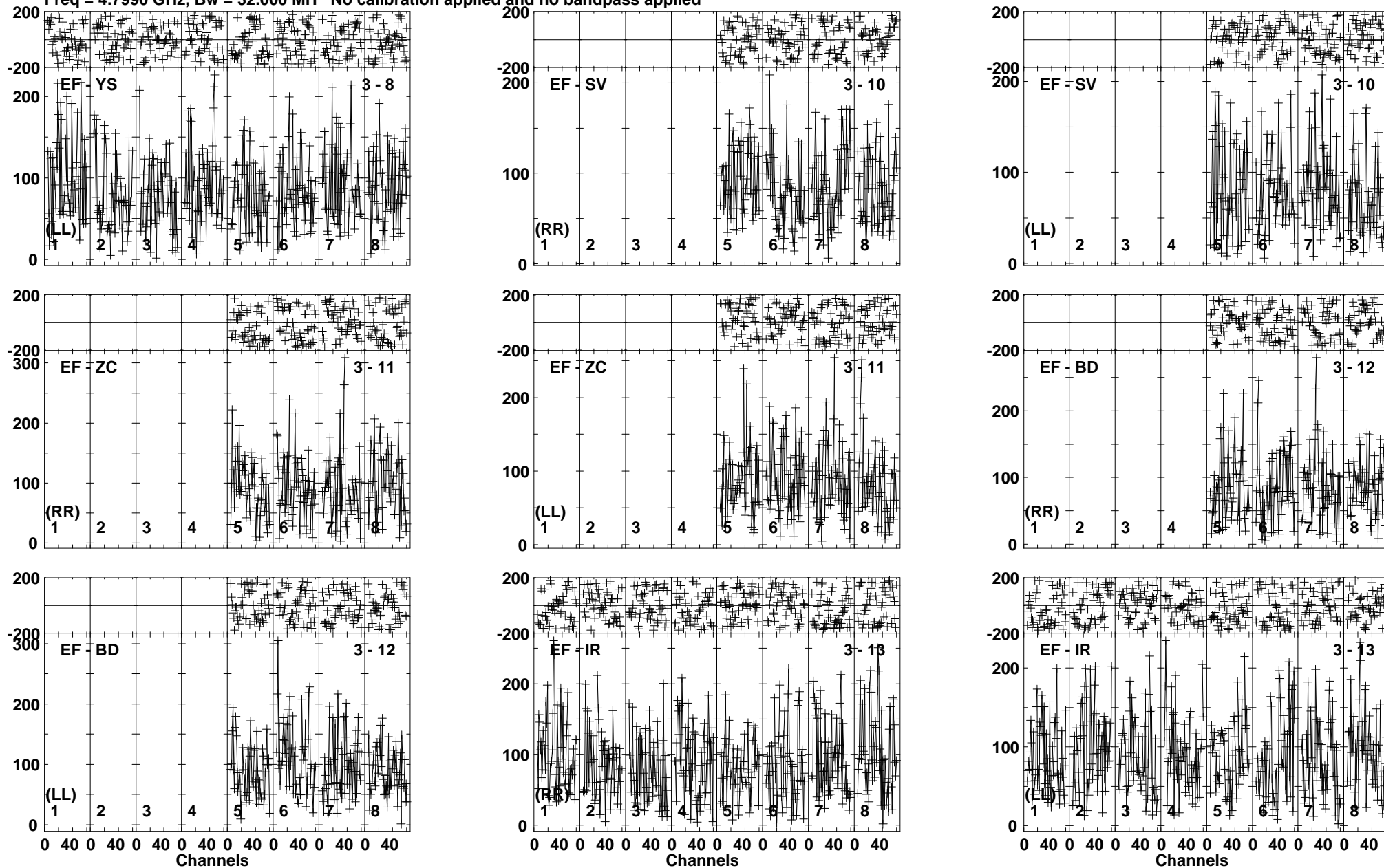
Lower frame: Micro Ampl Jy Top frame: Phas deg Vector averaged cross-power spectrum Baseline: EF (03) - YS (08) Timerange: 00/14:36:30 to 00/14:39:30
