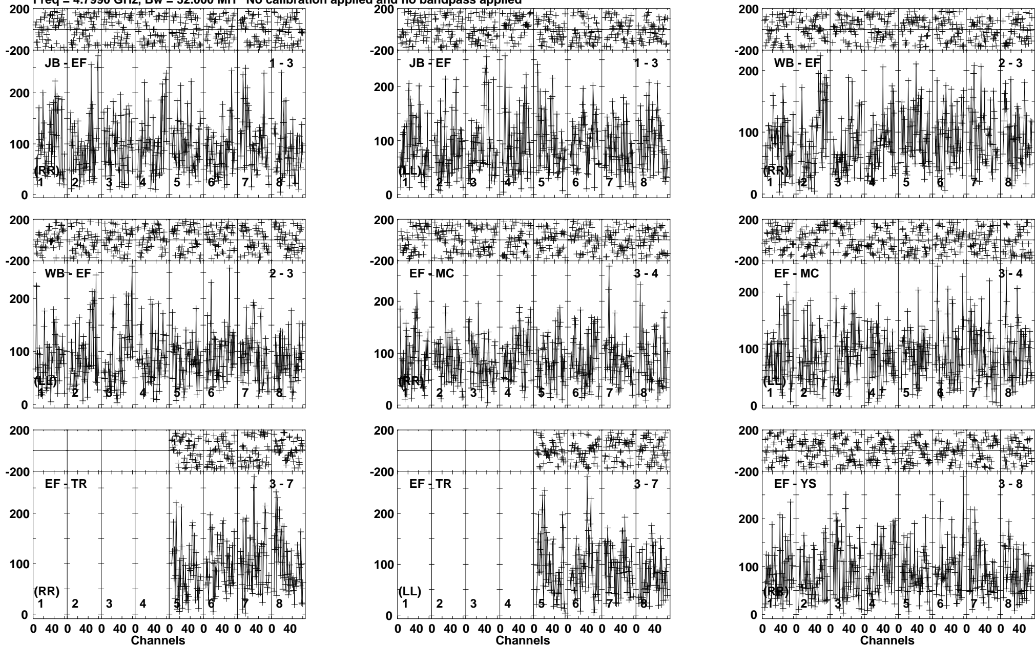
Lower frame: Micro Ampl Jy Top frame: Phas deg Vector averaged cross-power spectrum Baseline: JB (01) - EF (03) Timerange: 00/14:12:20 to 00/14:15:20
