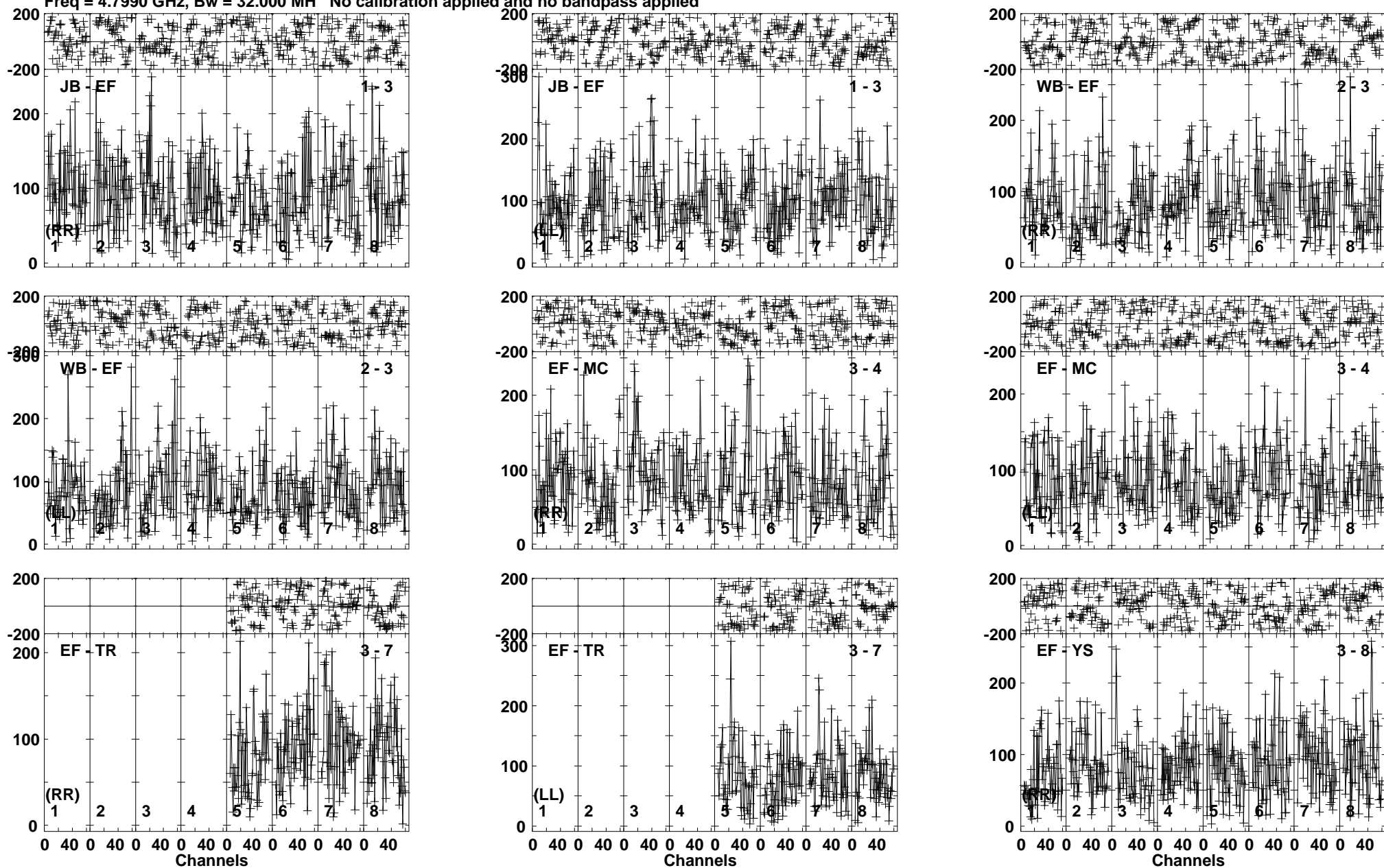
Lower frame: Micro Ampl Jy Top frame: Phas deg Vector averaged cross-power spectrum Baseline: JB (01) - EF (03) Timerange: 00/14:07:50 to 00/14:10:50
