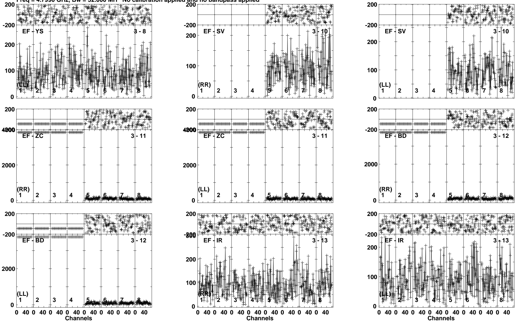
Lower frame: Micro Ampl Jy Top frame: Phas deg Vector averaged cross-power spectrum Baseline: EF (03) - YS (08) Timerange: 00/14:55:20 to 00/14:58:20
