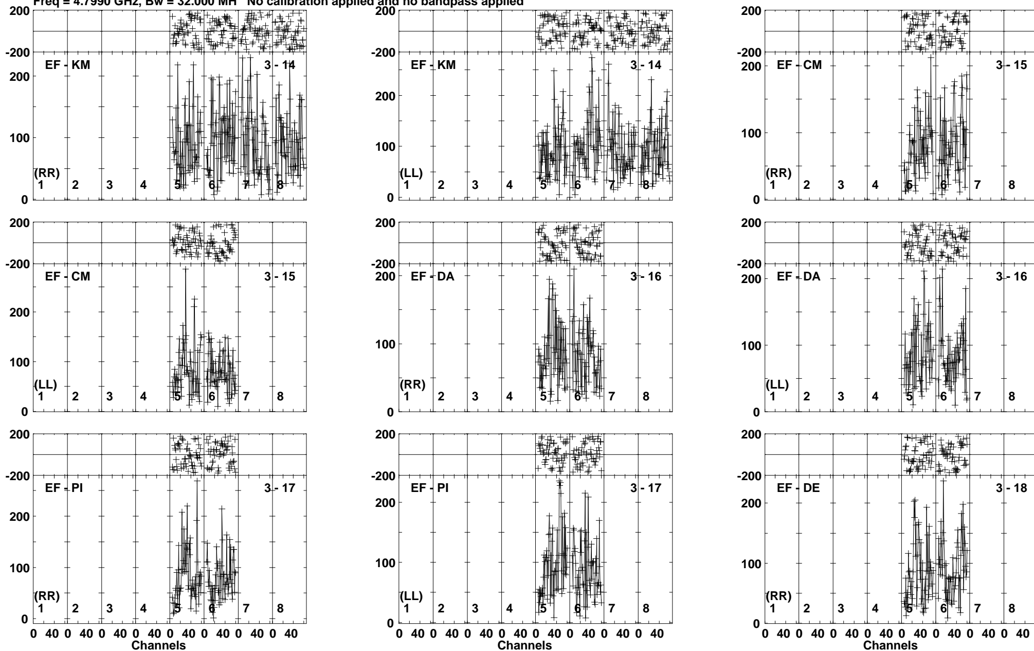
Lower frame: Micro Ampl Jy Top frame: Phas deg Vector averaged cross-power spectrum Baseline: EF (03) - KM (14) Timerange: 00/14:22:10 to 00/14:25:10
