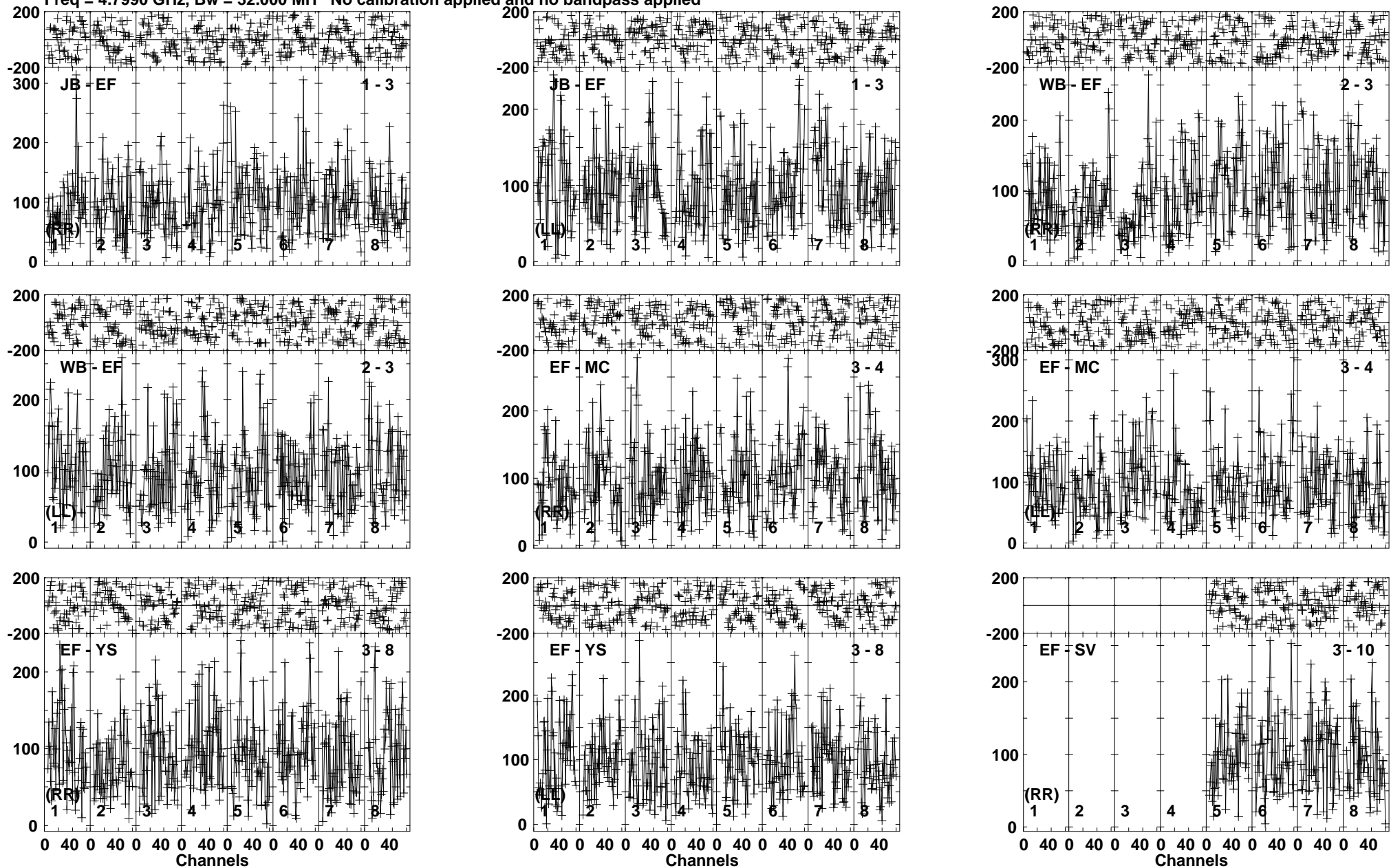
Lower frame: Micro Ampl Jy Top frame: Phas deg Vector averaged cross-power spectrum Baseline: JB (01) - EF (03) Timerange: 00/13:49:00 to 00/13:51:59
