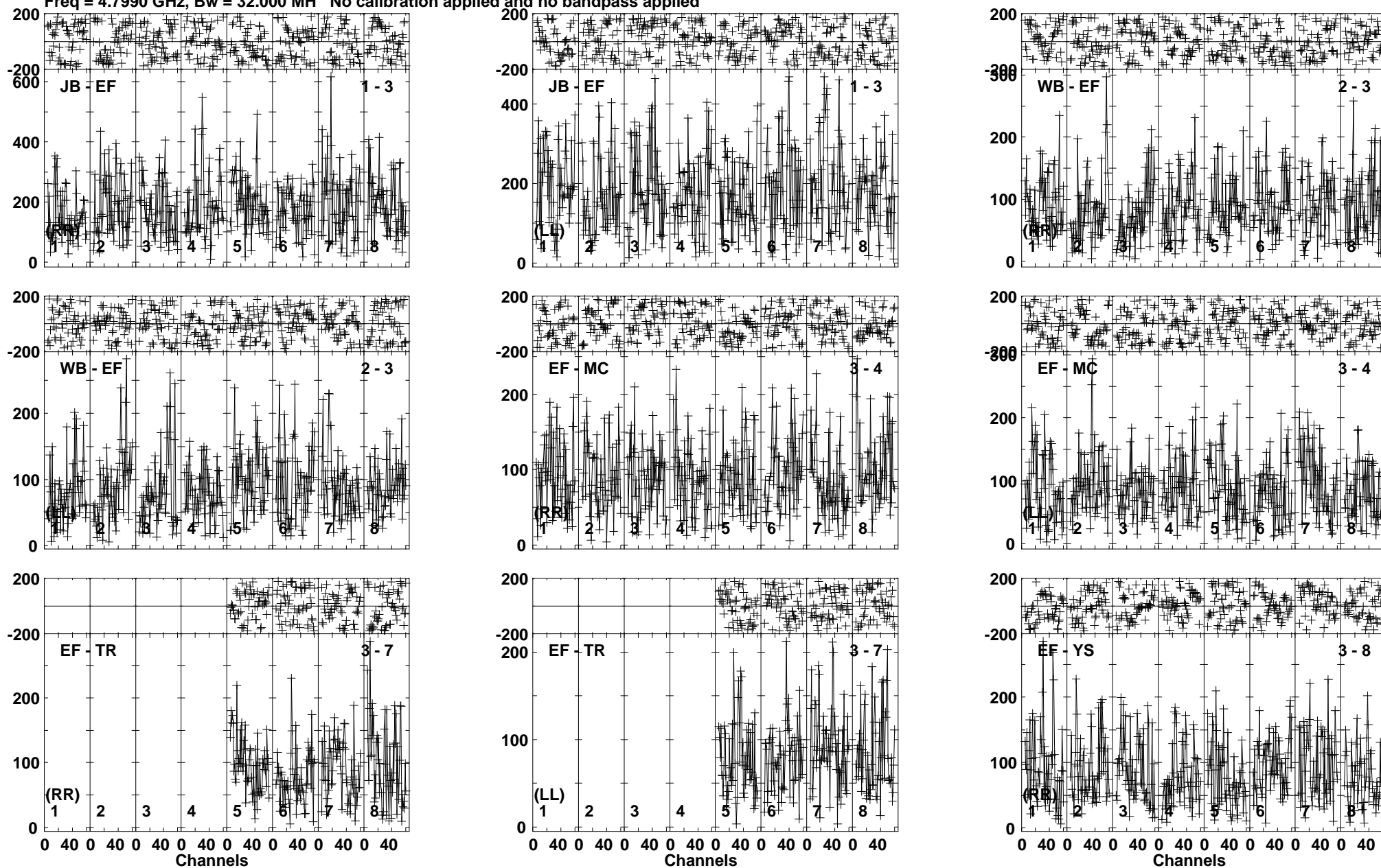
Lower frame: Micro Ampl Jy Top frame: Phas deg Vector averaged cross-power spectrum Baseline: JB (01) - EF (03) Timerange: 00/14:36:30 to 00/14:39:30
