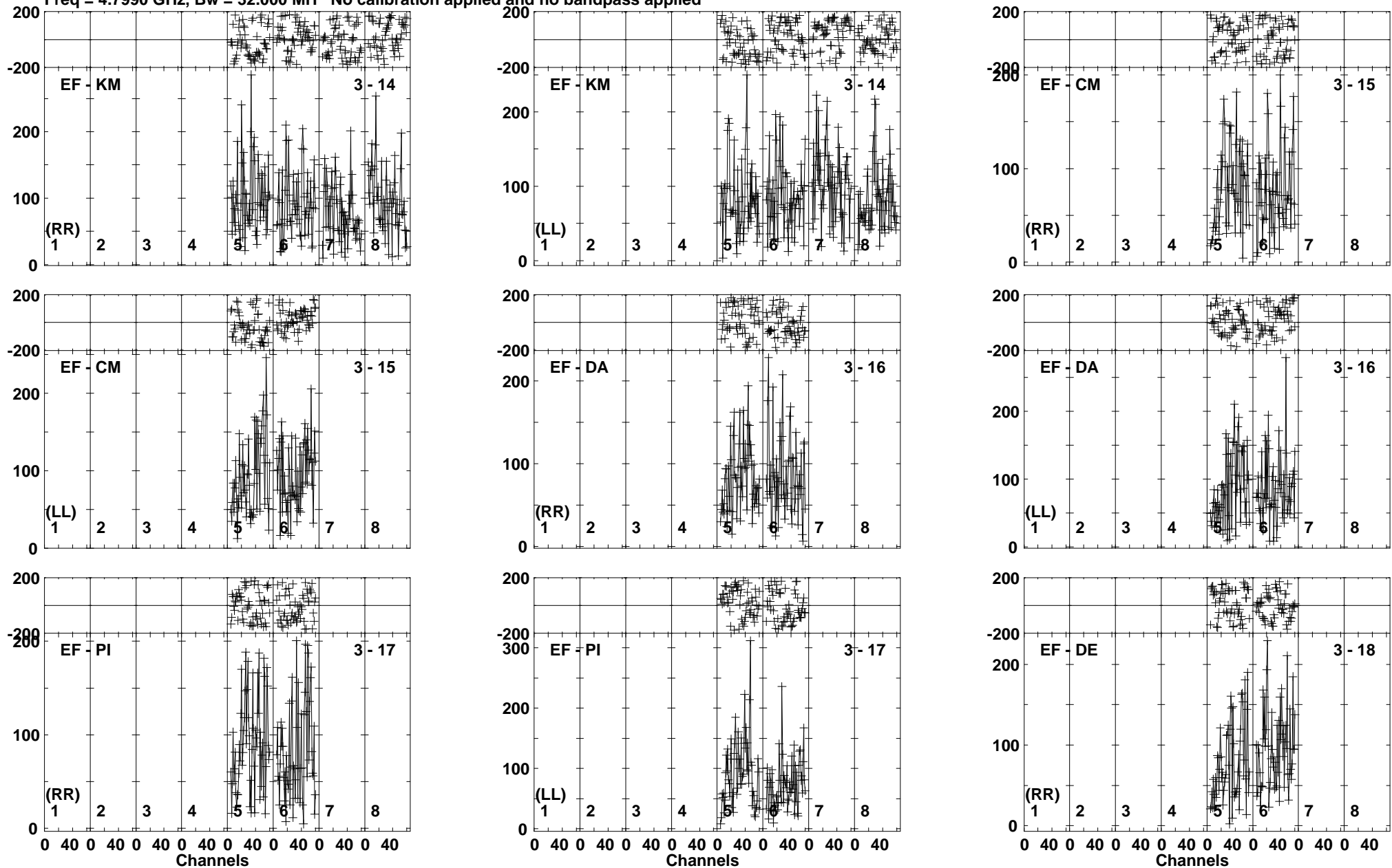
Lower frame: Micro Ampl Jy Top frame: Phas deg Vector averaged cross-power spectrum Baseline: EF (03) - KM (14) Timerange: 00/14:26:41 to 00/14:29:40
