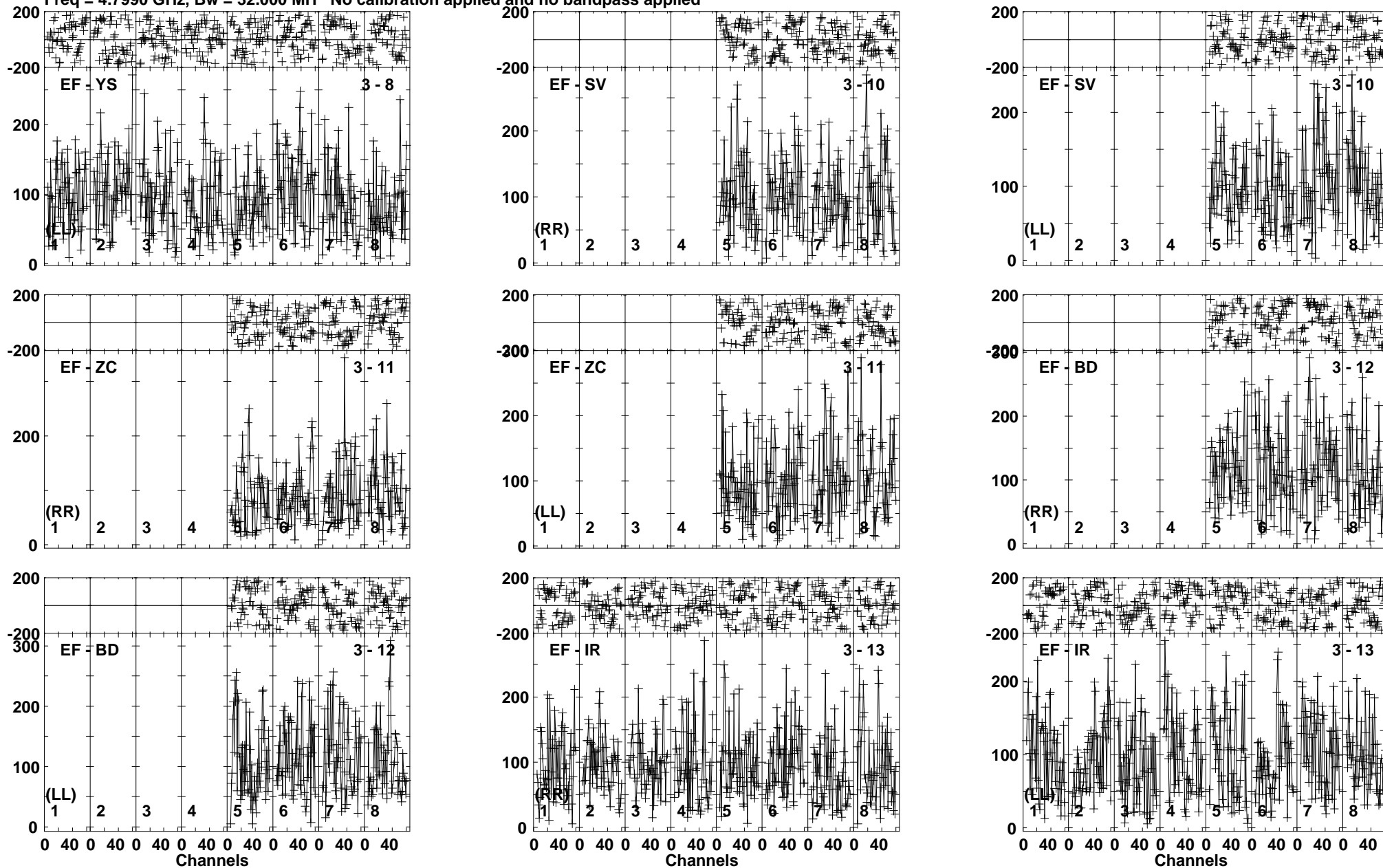
Lower frame: Micro Ampl Jy Top frame: Phas deg Vector averaged cross-power spectrum Baseline: EF (03) - YS (08) Timerange: 00/13:39:10 to 00/13:42:10
