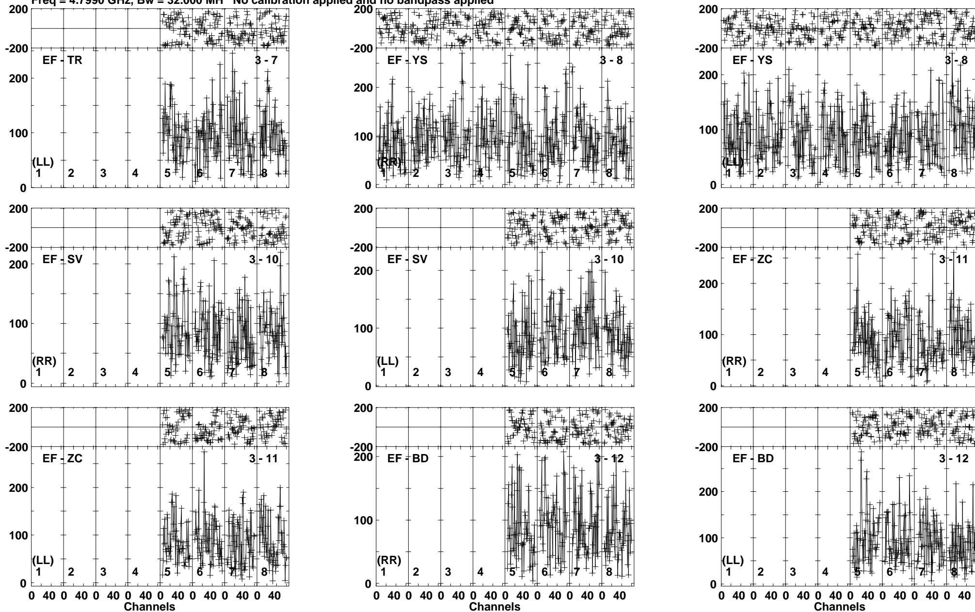
Lower frame: Micro Ampl Jy Top frame: Phas deg Vector averaged cross-power spectrum Baseline: EF (03) - TR (07) Timerange: 00/15:33:51 to 00/15:36:49
