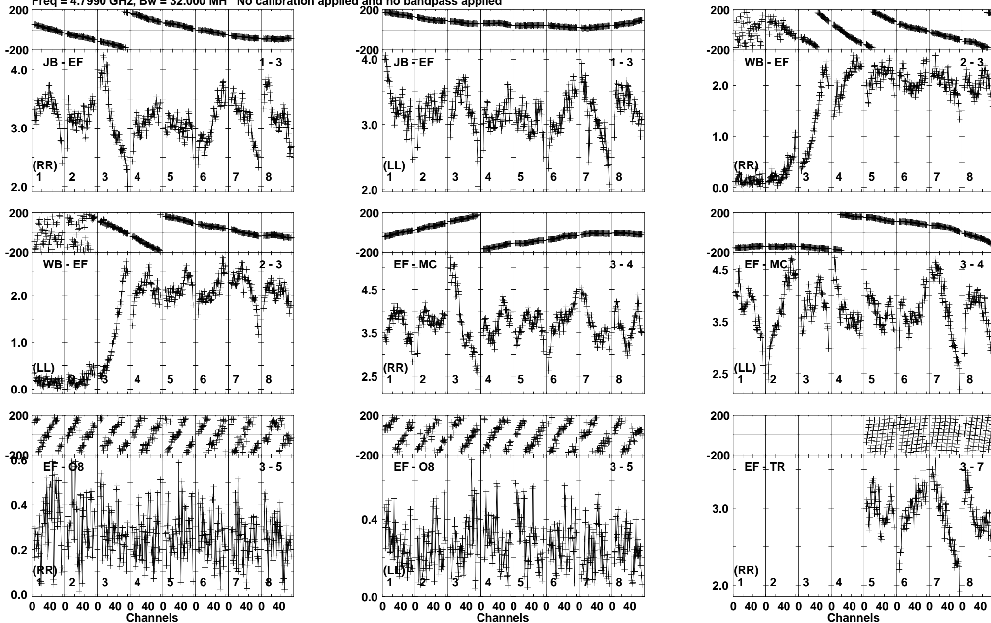
Lower frame: Milli Ampl Jy Top frame: Phas deg Vector averaged cross-power spectrum Baseline: JB (01) - EF (03) Timerange: 00/15:32:21 to 00/15:33:50
