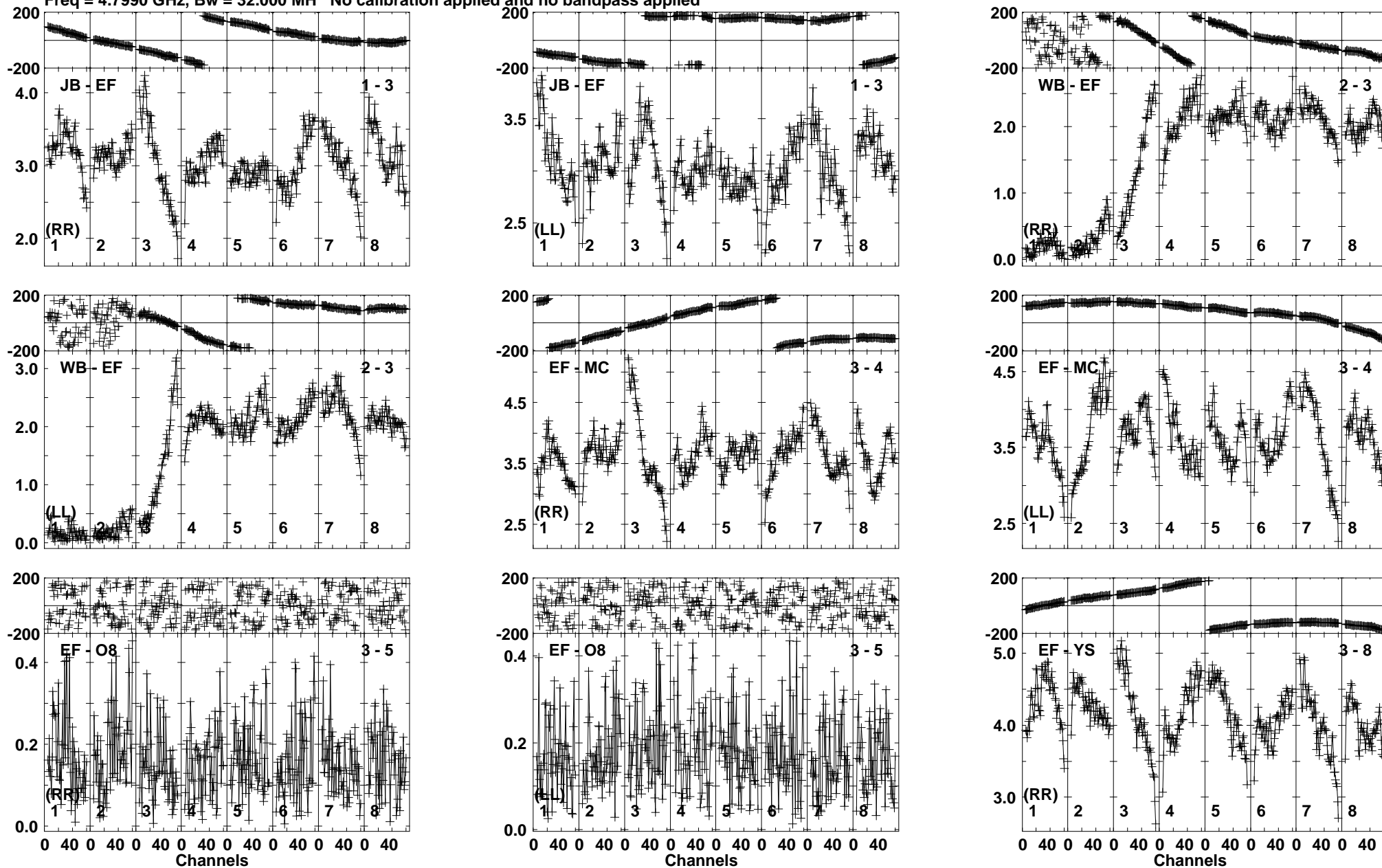
Lower frame: Milli Ampl Jy Top frame: Phas deg Vector averaged cross-power spectrum Baseline: JB (01) - EF (03) Timerange: 00/13:13:30 to 00/13:14:59
