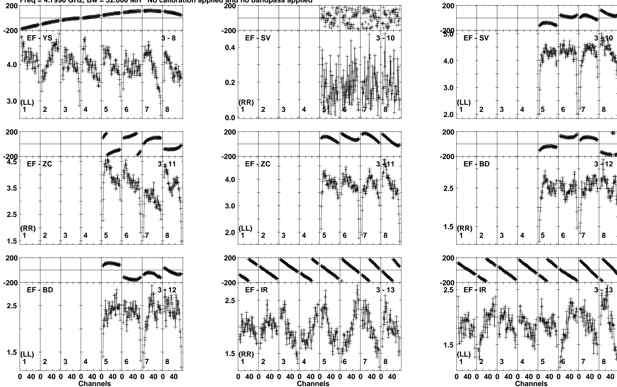
Lower frame: Milli Ampl Jy Top frame: Phas deg Vector averaged cross-power spectrum Baseline: EF (03) - YS (08) Timerange: 00/14:25:10 to 00/14:26:39
