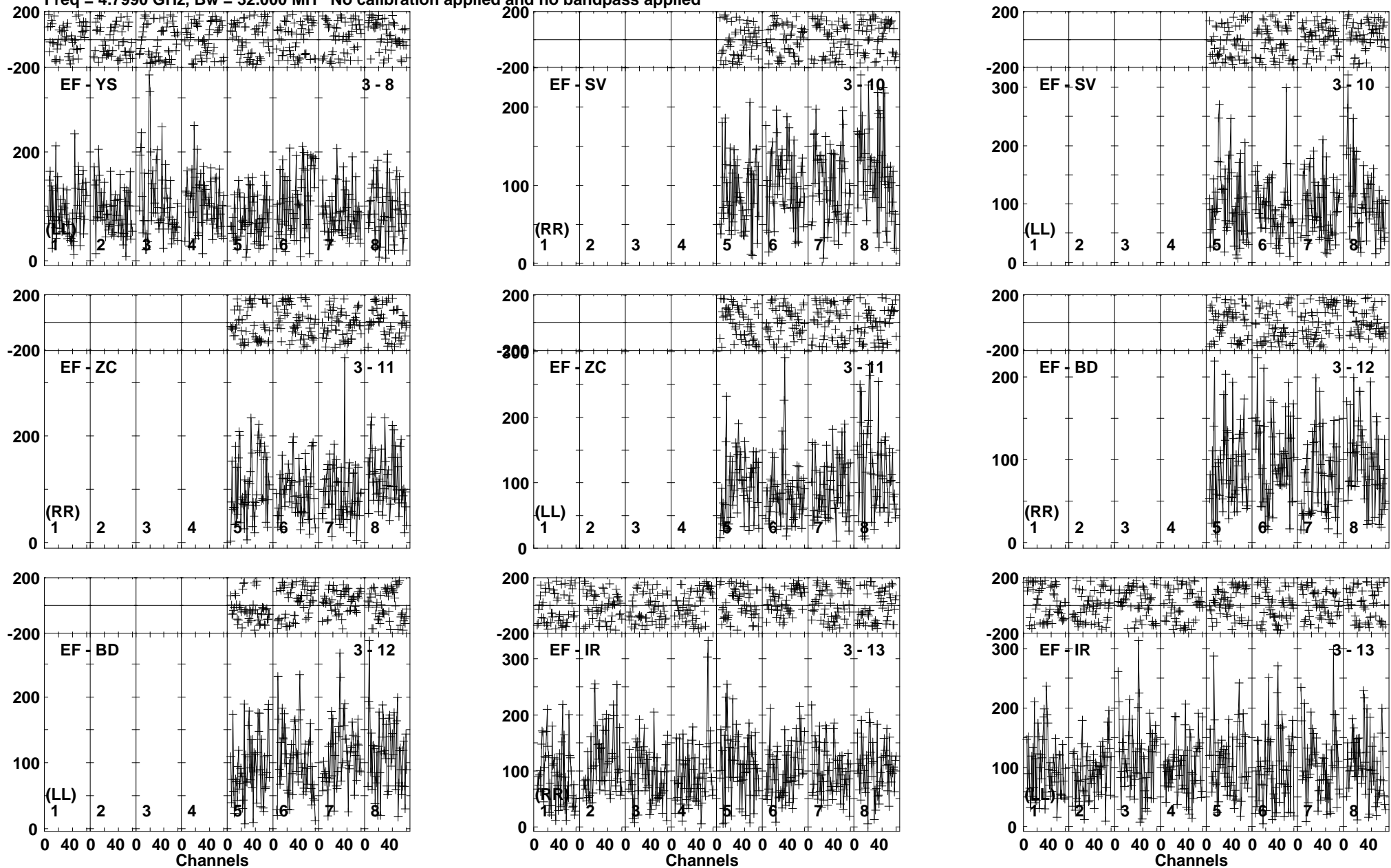
Lower frame: Micro Ampl Jy Top frame: Phas deg Vector averaged cross-power spectrum Baseline: EF (03) - YS (08) Timerange: 00/13:29:21 to 00/13:32:19
