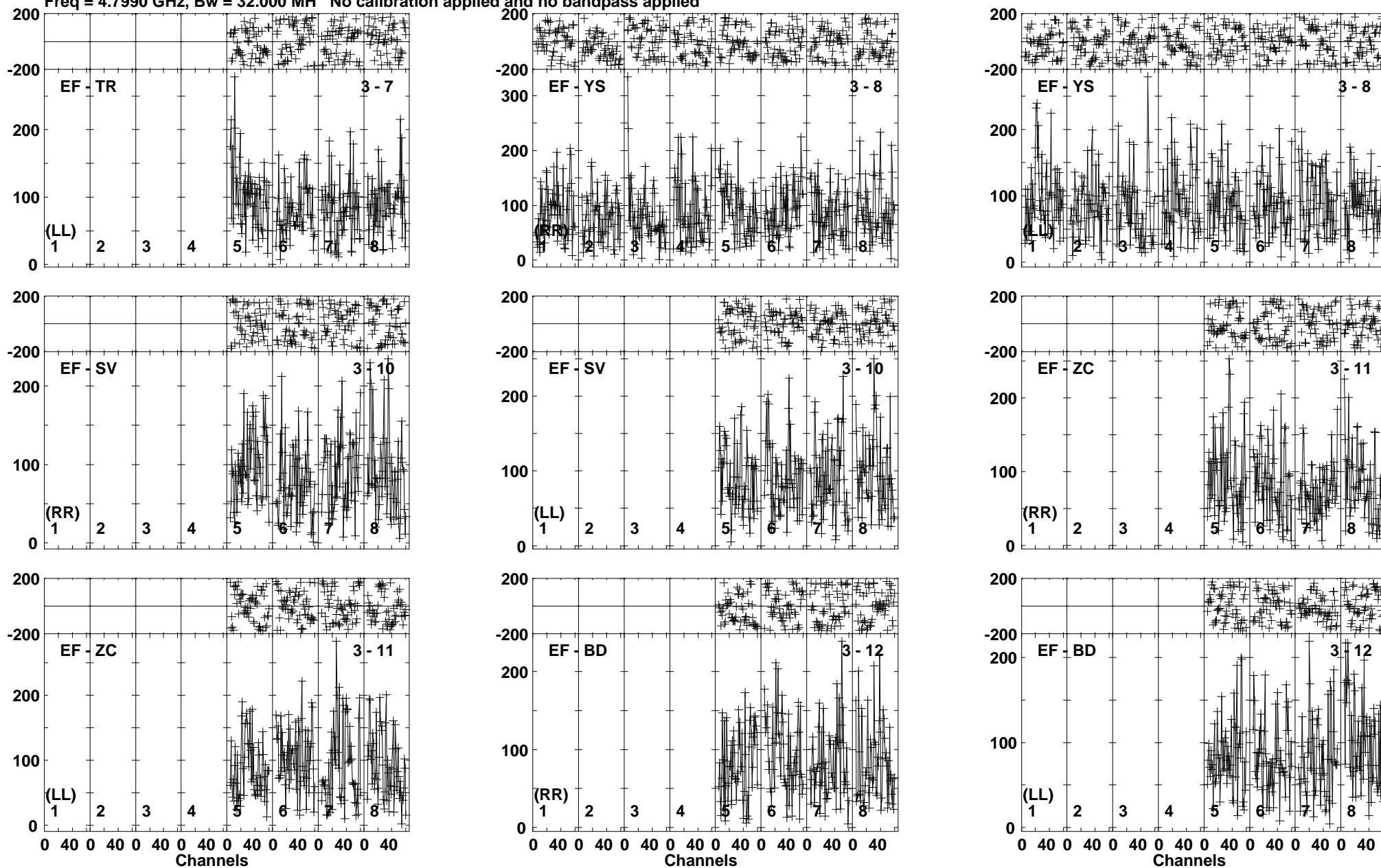
Lower frame: Micro Ampl Jy Top frame: Phas deg Vector averaged cross-power spectrum Baseline: EF (03) - TR (07) Timerange: 00/15:29:20 to 00/15:32:20
