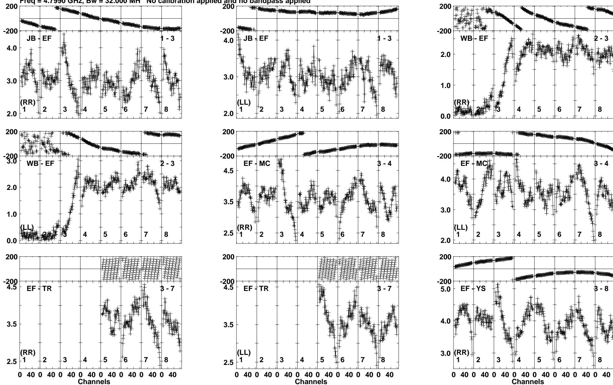
Lower frame: Milli Ampl Jy Top frame: Phas deg Vector averaged cross-power spectrum Baseline: JB (01) - EF (03) Timerange: 00/14:20:41 to 00/14:22:10
