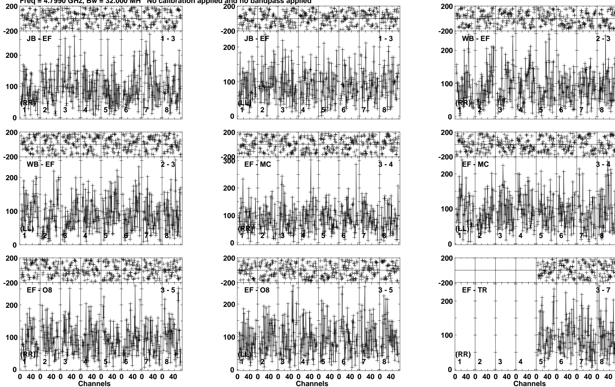
Lower frame: Micro Ampl Jy Top frame: Phas deg Vector averaged cross-power spectrum Baseline: JB (01) - EF (03) Timerange: 00/15:29:20 to 00/15:32:20
