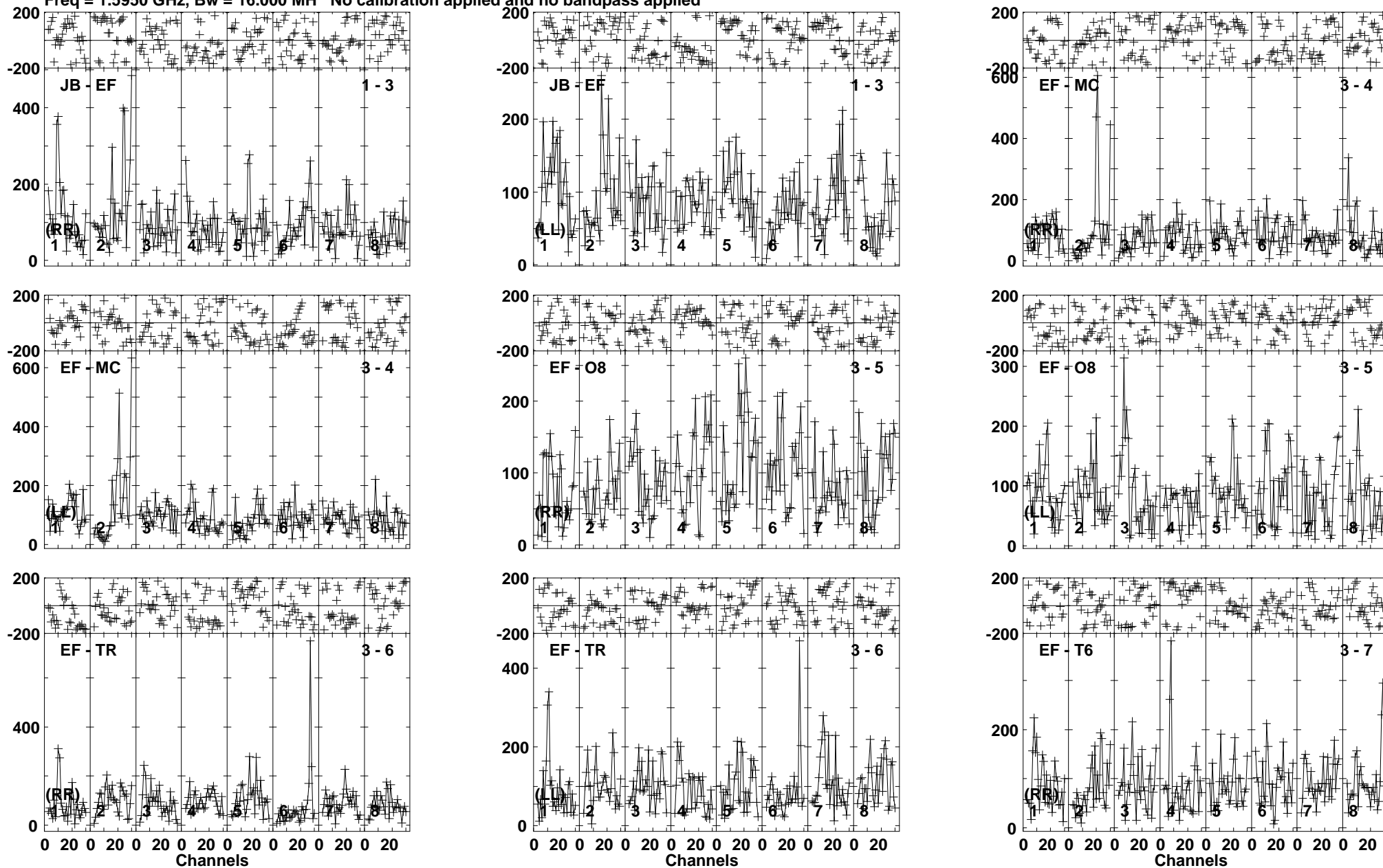
Lower frame: Micro Ampl Jy Top frame: Phas deg Vector averaged cross-power spectrum Baseline: JB (01) - EF (03) Timerange: 00:18:09:41 to 00:18:12:39
