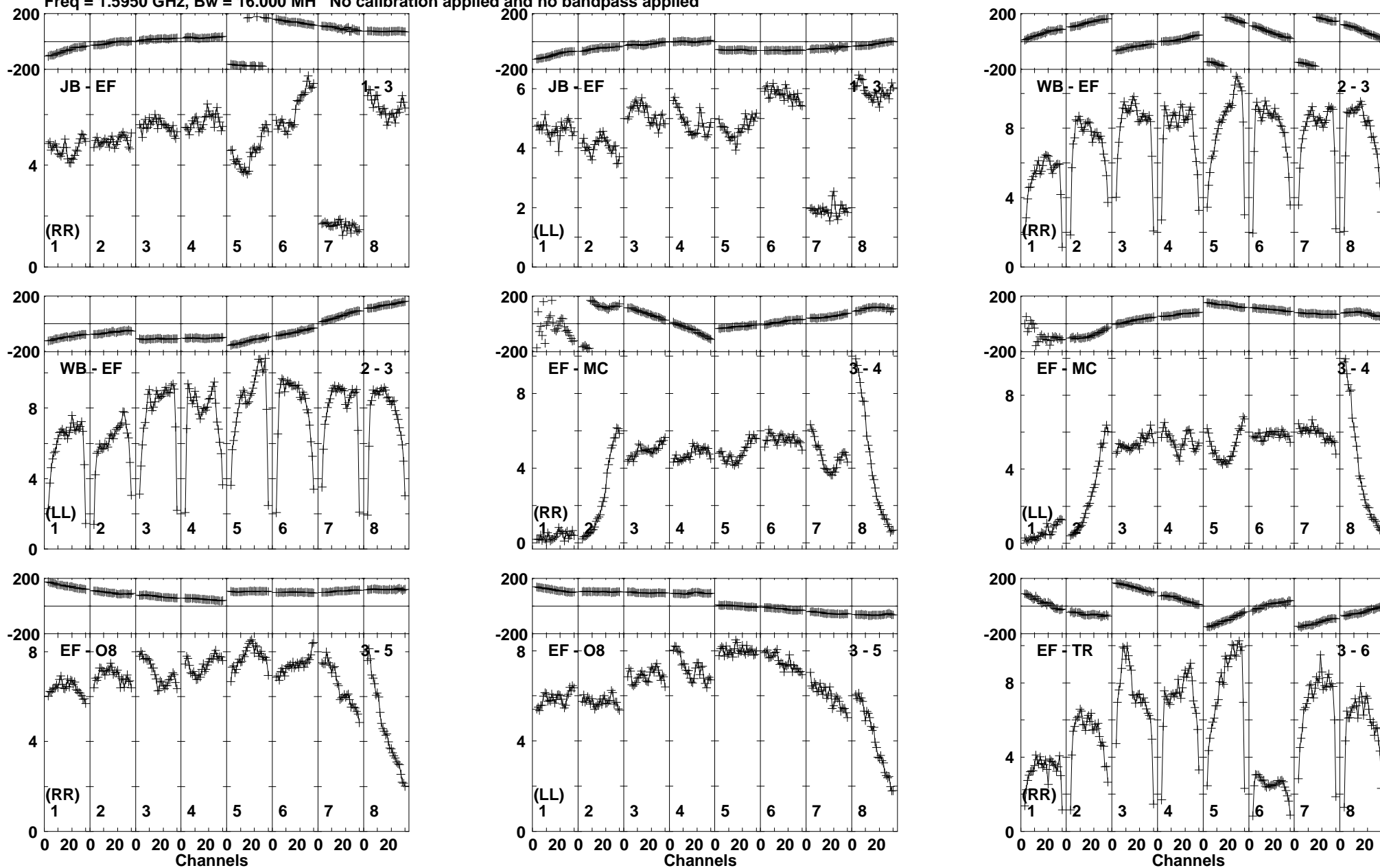
Lower frame: Milli Ampl Jy Top frame: Phas deg Vector averaged cross-power spectrum Baseline: JB (01) - EF (03) Timerange: 00:19:12:31 to 00:19:13:29
