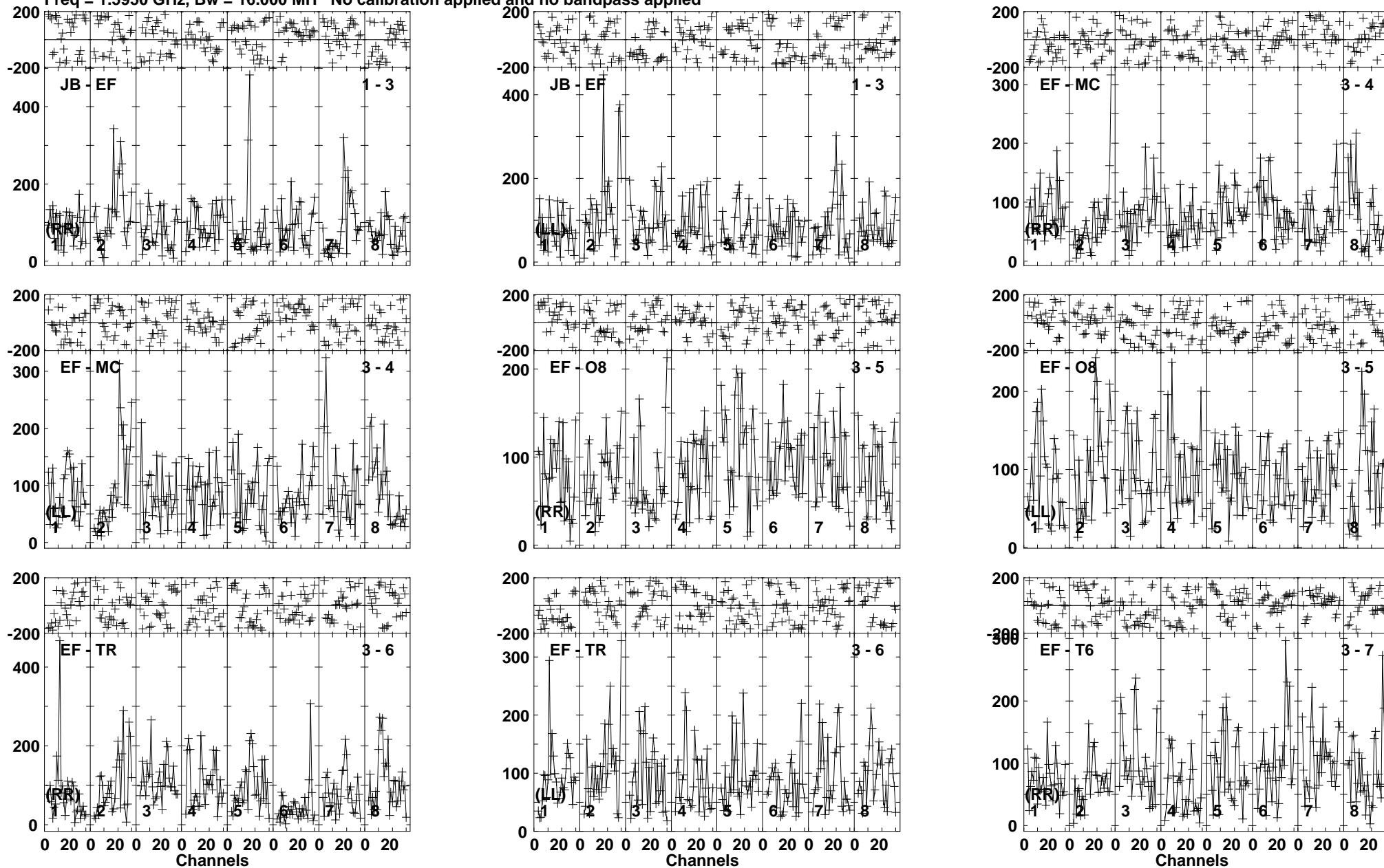
Lower frame: Micro Ampl Jy Top frame: Phas deg Vector averaged cross-power spectrum Baseline: JB (01) - EF (03) Timerange: 00:18:30:11 to 00:18:33:09
