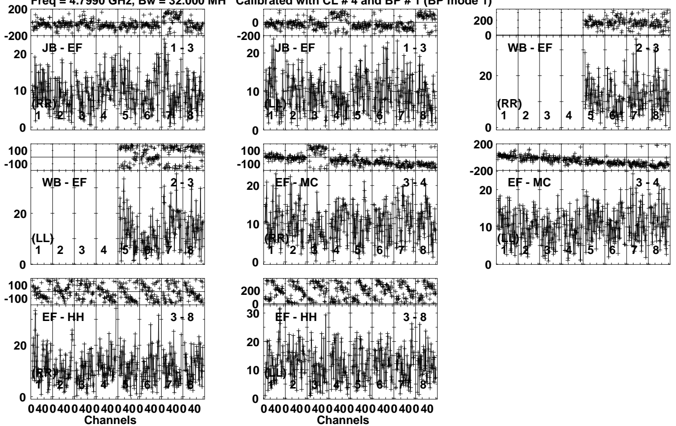
Lower frame: Milli Ampl Jy Top frame: Phas deg Vector averaged cross-power spectrum Several baselines displayed Timerange: 01/00:32:01 to 01/00:34:59
