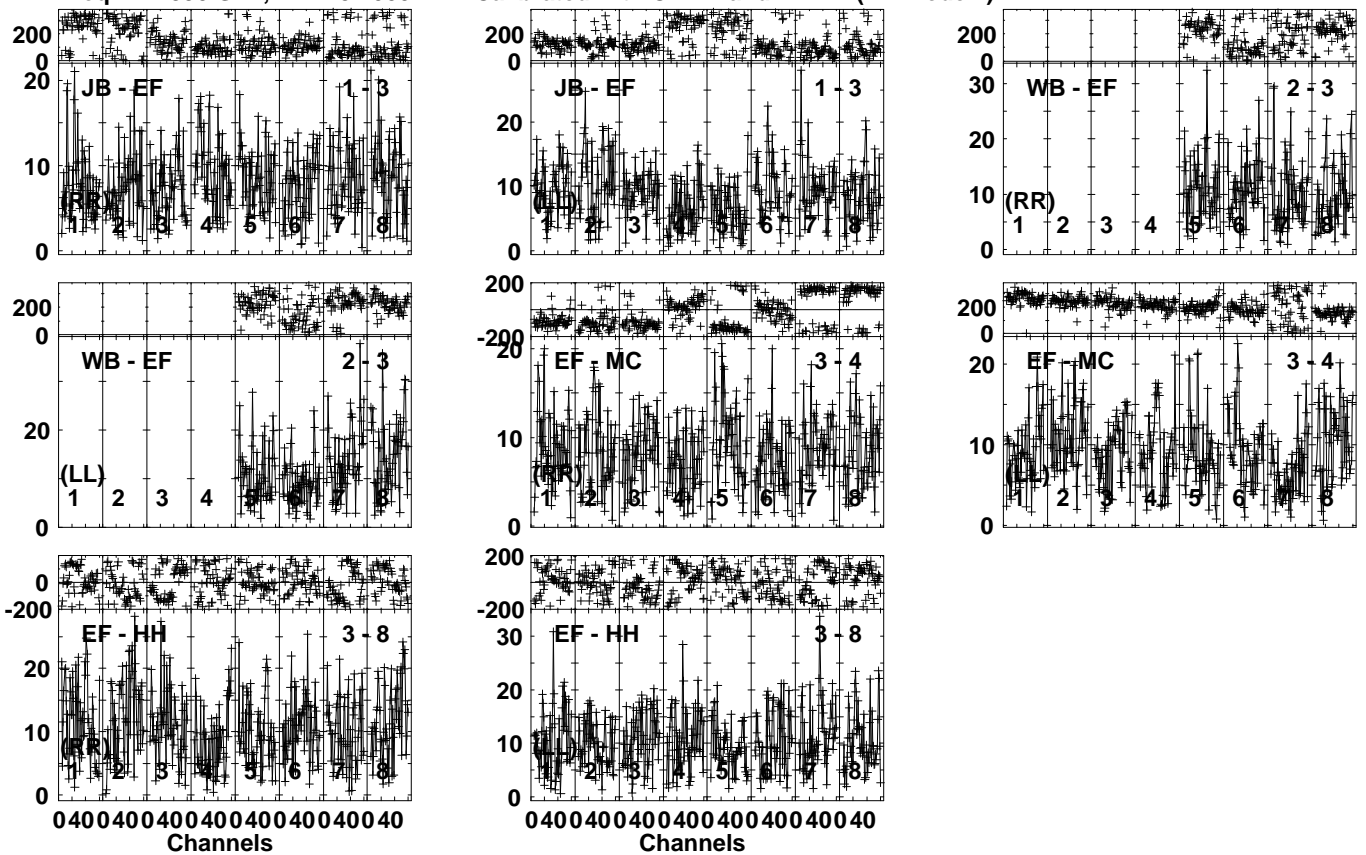
Lower frame: Milli Ampl Jy Top frame: Phas deg Vector averaged cross-power spectrum Several baselines displayed Timerange: 01/00:27:01 to 01/00:29:59
