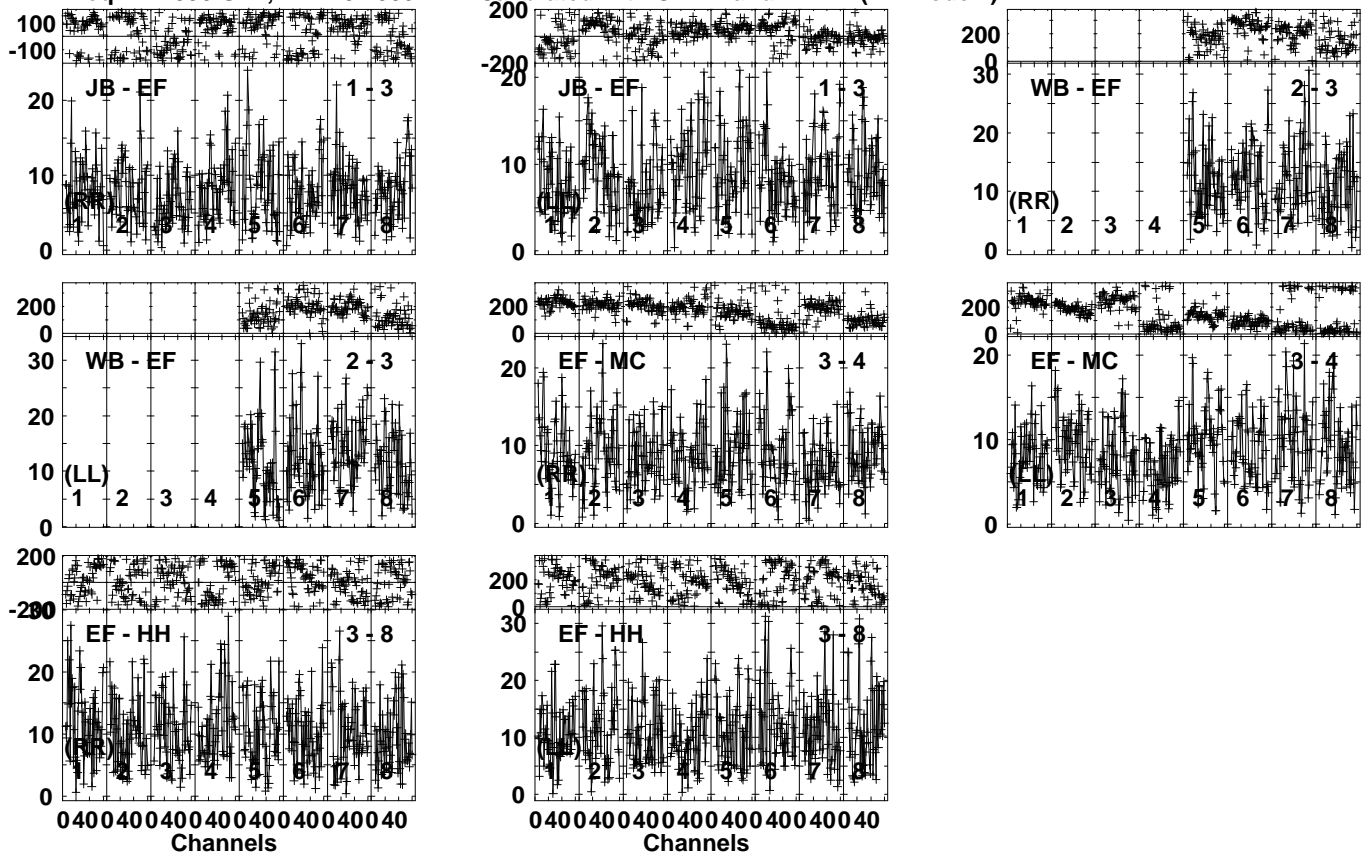
Lower frame: Milli Ampl Jy Top frame: Phas deg Vector averaged cross-power spectrum Several baselines displayed Timerange: 01/00:42:01 to 01/00:44:59
