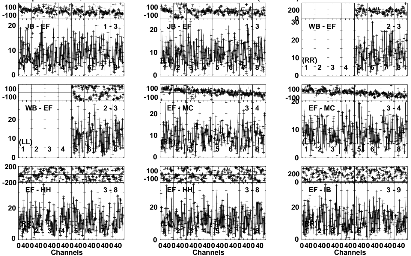
Lower frame: Milli Ampl Jy Top frame: Phas deg Vector averaged cross-power spectrum Several baselines displayed Timerange: 01/01:27:01 to 01/01:29:59
