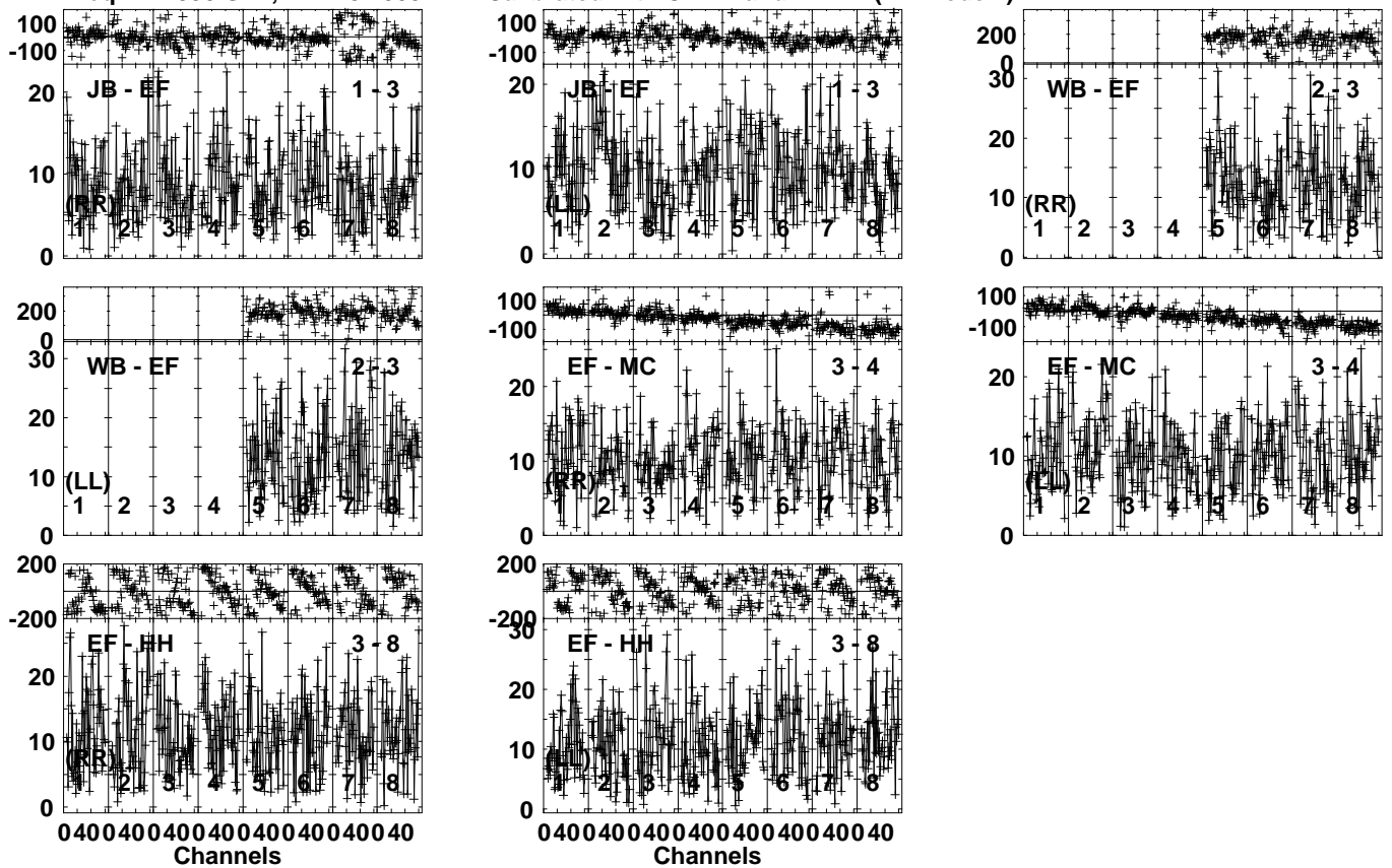
Lower frame: Milli Ampl Jy Top frame: Phas deg Vector averaged cross-power spectrum Several baselines displayed Timerange: 01/00:47:01 to 01/00:49:59
