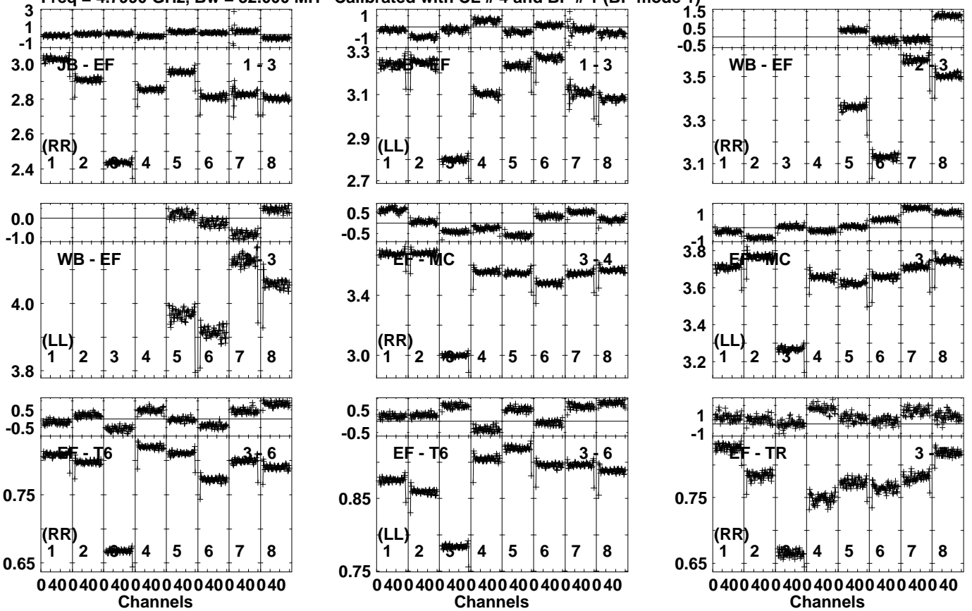
Lower frame: Ampl Jy Top frame: Phas deg Vector averaged cross-power spectrum Several baselines displayed Timerange: 00/23:58:09 to 01/00:04:49
