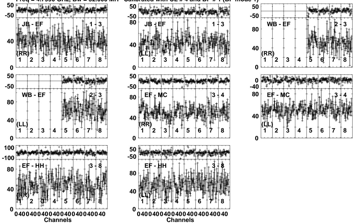
Lower frame: Milli Ampl Jy Top frame: Phas deg Vector averaged cross-power spectrum Several baselines displayed Timerange: 01/01:15:41 to 01/01:16:19
