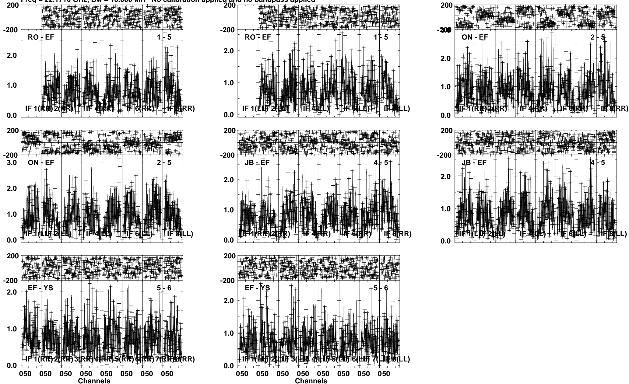
Lower frame: Milli Ampl Jy Top frame: Phas deg Vector averaged cross-power spectrum Several baselines displayed Timerange: 01/00:00:00 to 01/00:00:45
