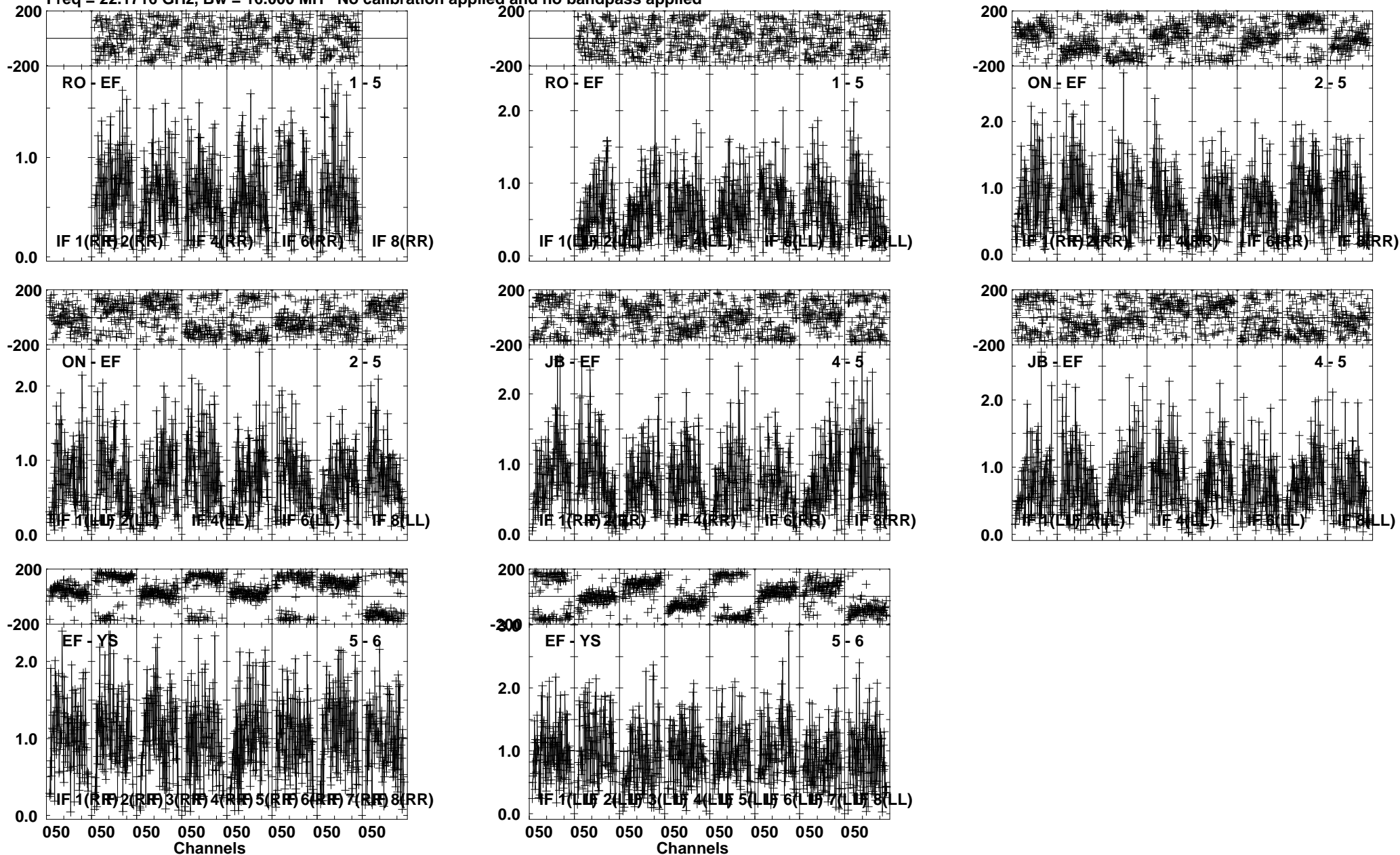
Lower frame: Milli Ampl Jy Top frame: Phas deg Vector averaged cross-power spectrum Several baselines displayed Timerange: 00/15:51:01 to 00/15:52:00
