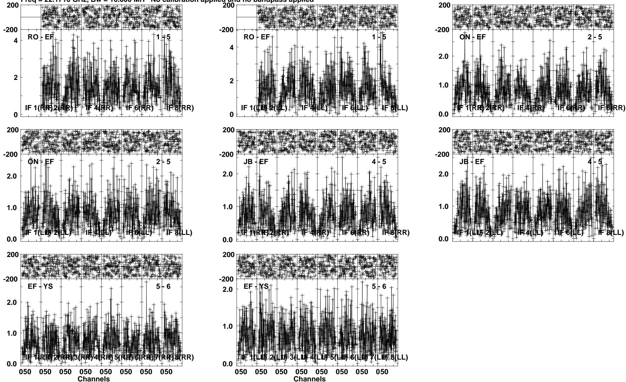
Lower frame: Milli Ampl Jy Top frame: Phas deg Vector averaged cross-power spectrum Several baselines displayed Timerange: 00/23:47:16 to 00/23:48:00
