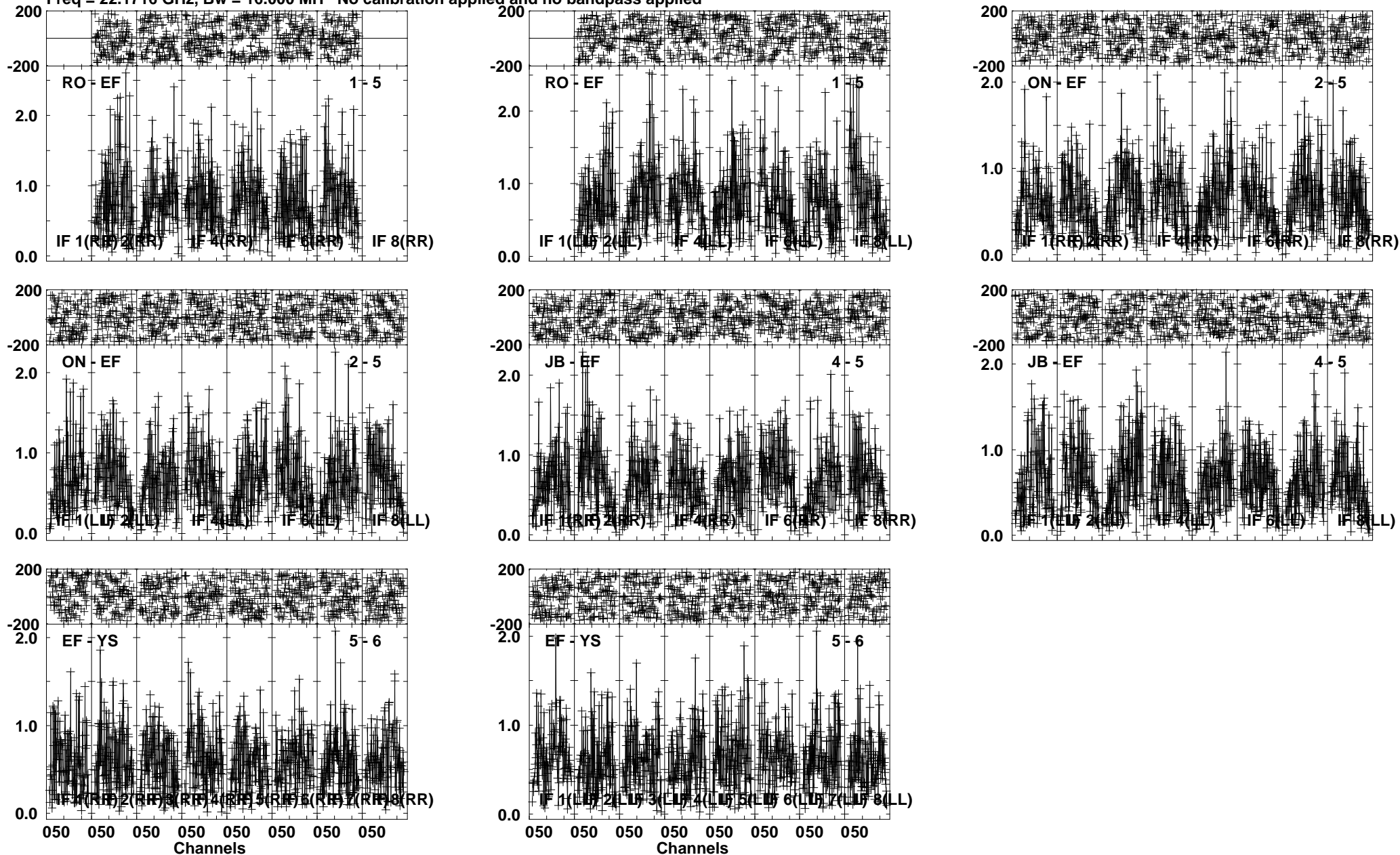
Lower frame: Milli Ampl Jy Top frame: Phas deg Vector averaged cross-power spectrum Several baselines displayed Timerange: 00/17:57:01 to 00/17:58:00
