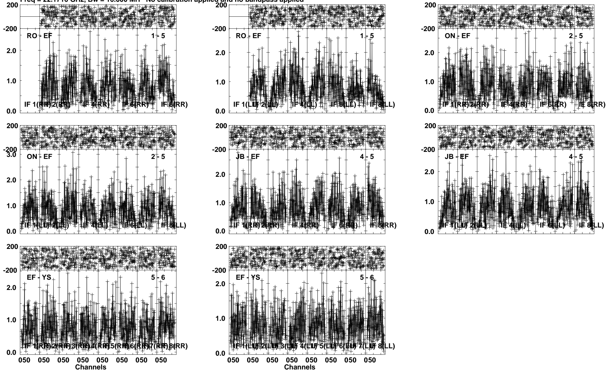
Lower frame: Milli Ampl Jy Top frame: Phas deg Vector averaged cross-power spectrum Several baselines displayed Timerange: 01/00:07:16 to 01/00:08:00
