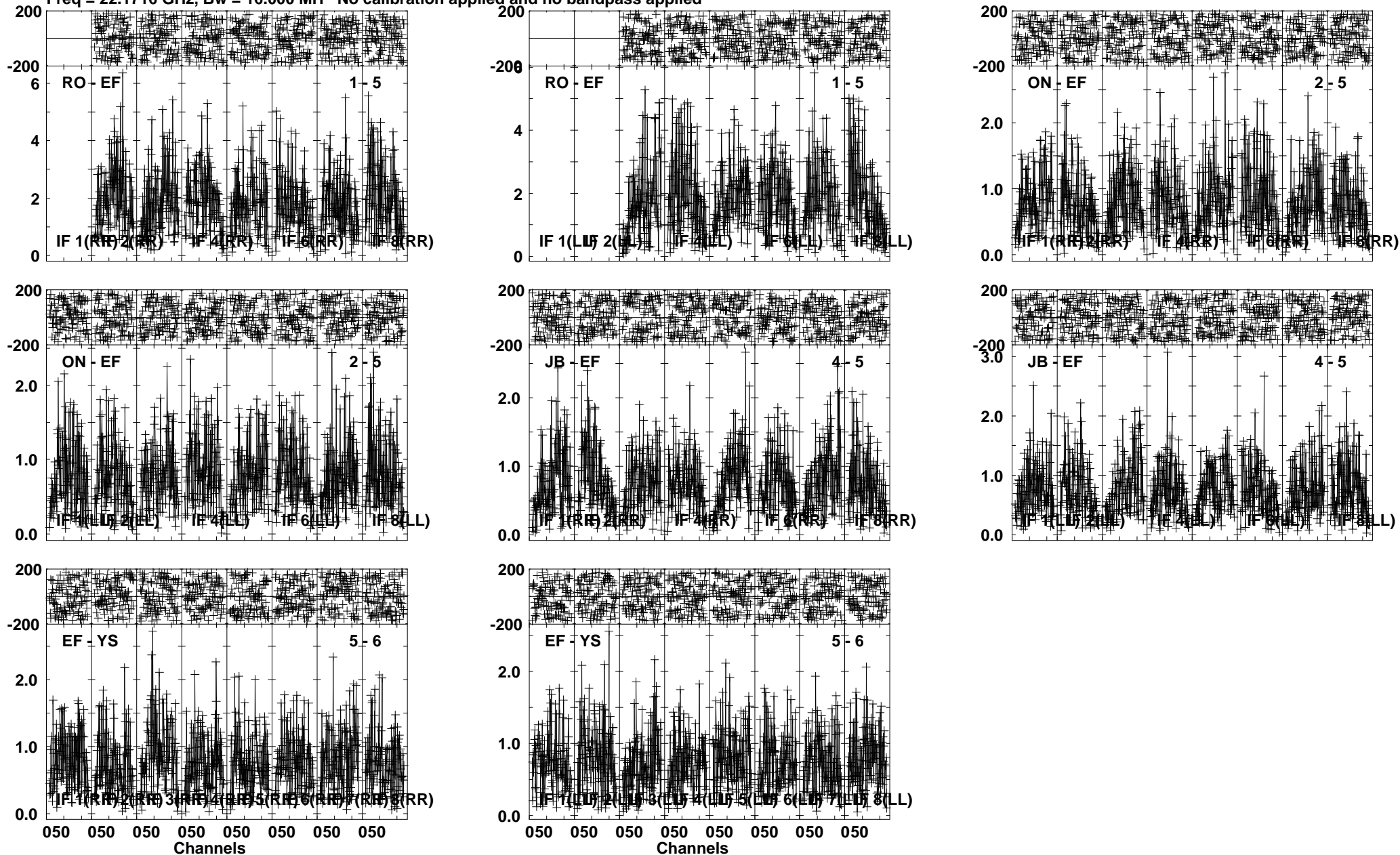
Lower frame: Milli Ampl Jy Top frame: Phas deg Vector averaged cross-power spectrum Several baselines displayed Timerange: 00/23:26:46 to 00/23:27:30
