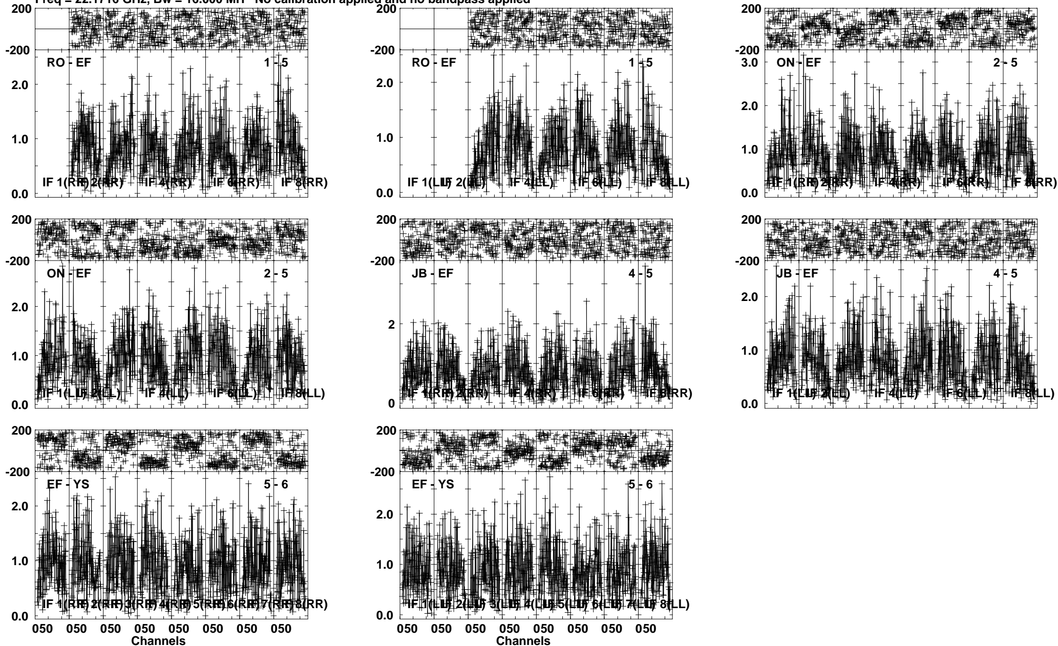
Lower frame: Milli Ampl Jy Top frame: Phas deg Vector averaged cross-power spectrum Several baselines displayed Timerange: 01/01:30:01 to 01/01:30:45
