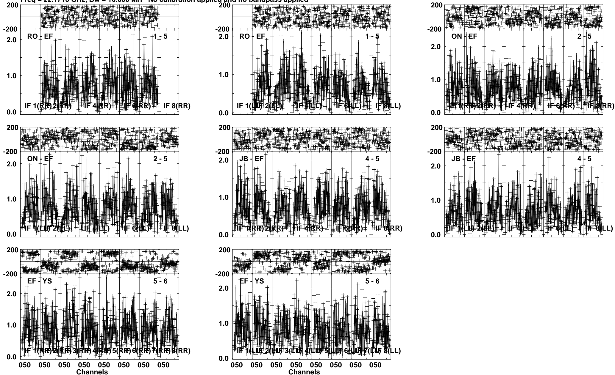
Lower frame: Milli Ampl Jy Top frame: Phas deg Vector averaged cross-power spectrum Several baselines displayed Timerange: 00/18:12:31 to 00/18:13:30
