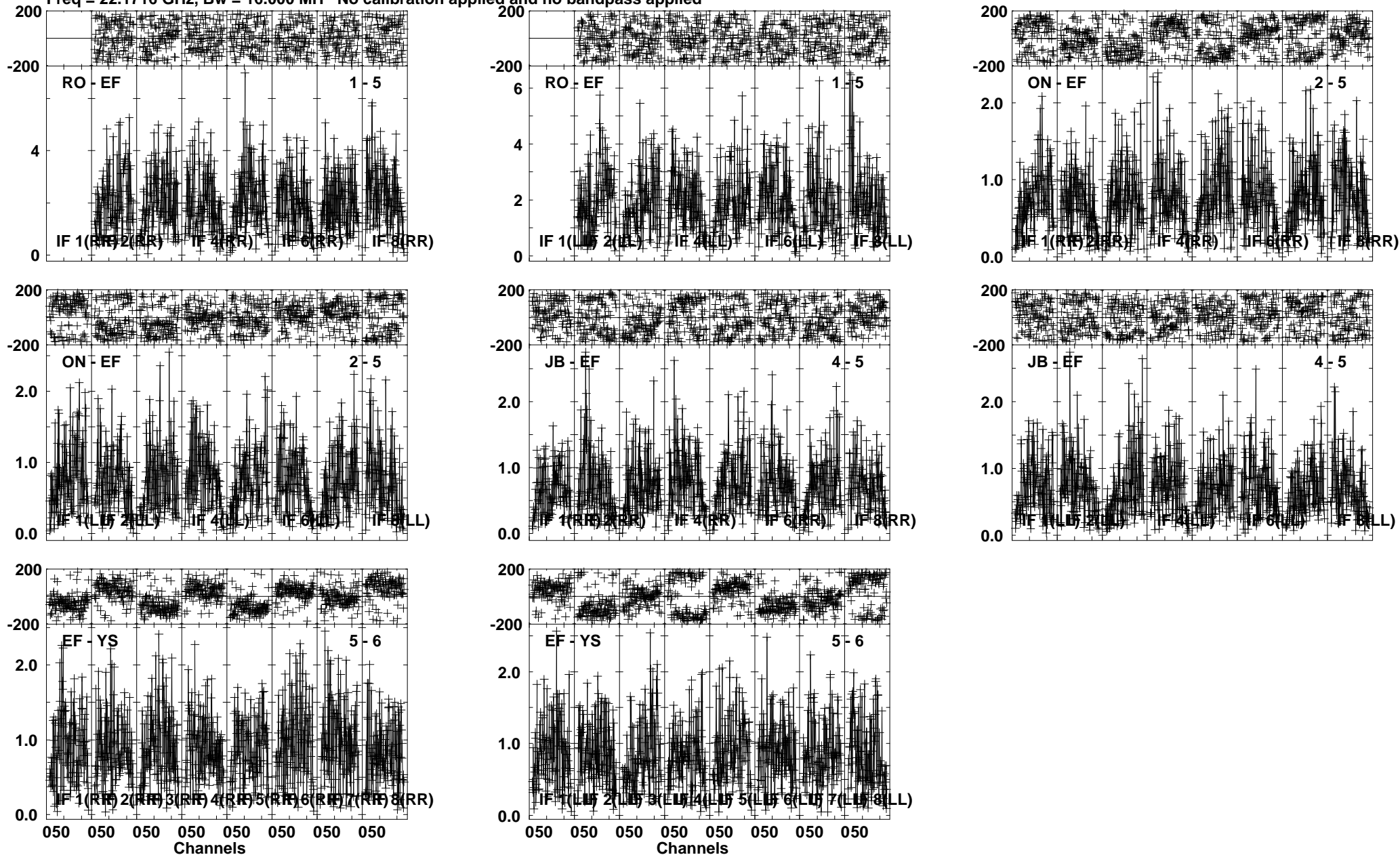
Lower frame: Milli Ampl Jy Top frame: Phas deg Vector averaged cross-power spectrum Several baselines displayed Timerange: 00/18:33:31 to 00/18:34:30
