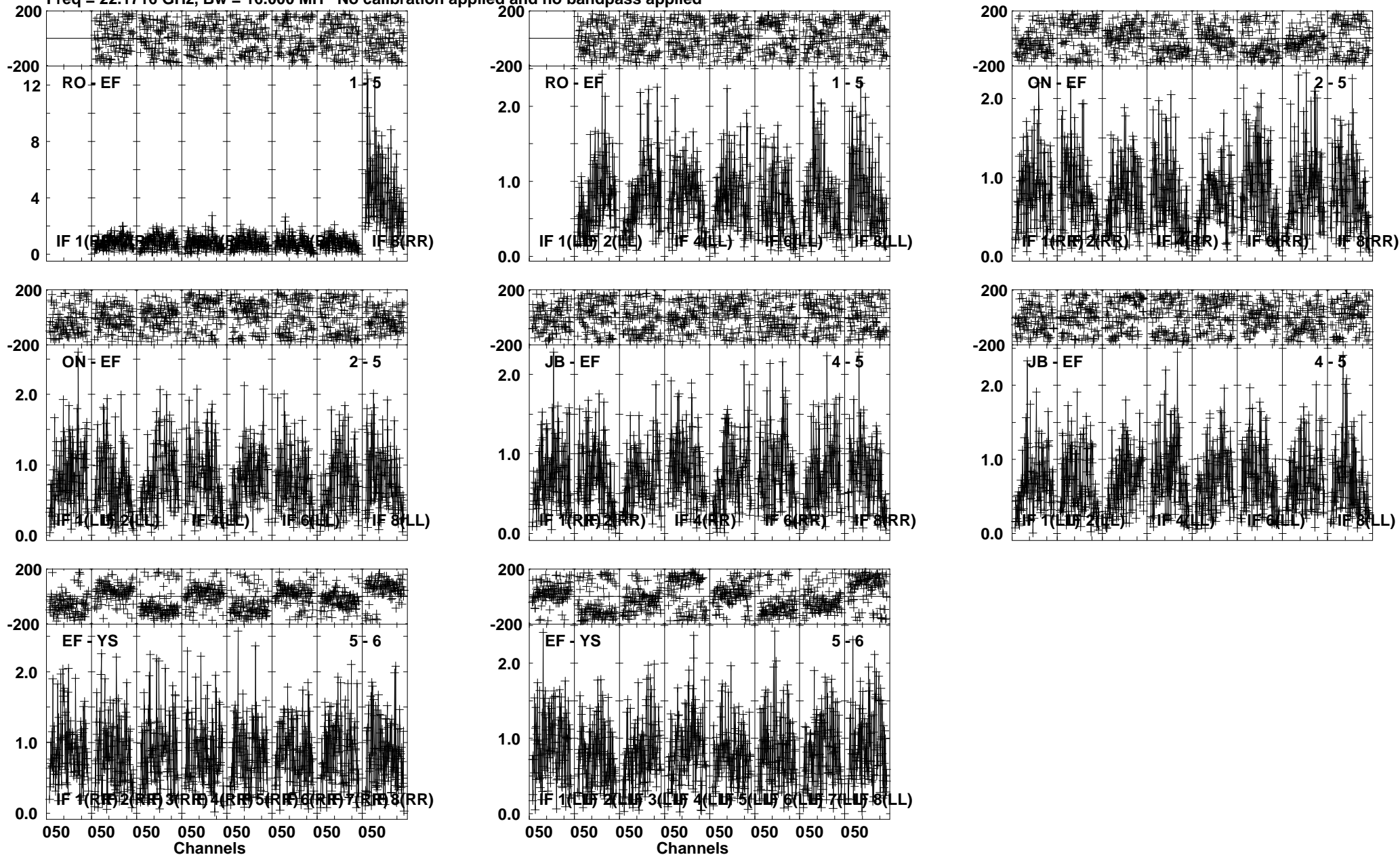
Lower frame: Milli Ampl Jy Top frame: Phas deg Vector averaged cross-power spectrum Several baselines displayed Timerange: 00:18:10:31 to 00:18:11:30
