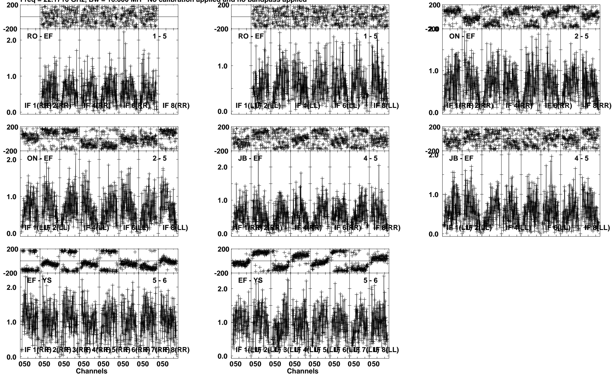
Lower frame: Milli Ampl Jy Top frame: Phas deg Vector averaged cross-power spectrum Several baselines displayed Timerange: 00/16:12:01 to 00/16:13:00
