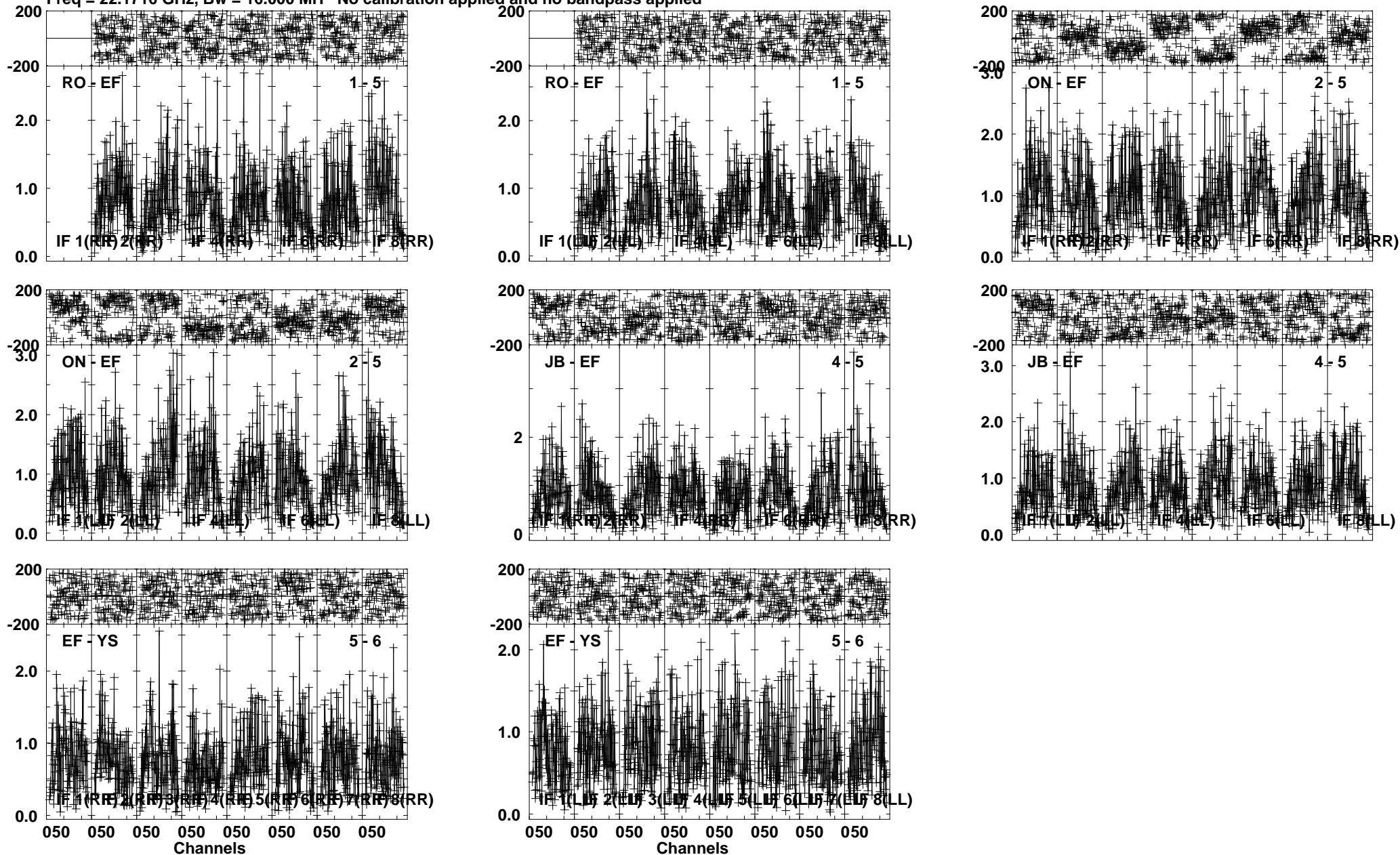
Lower frame: Milli Amp Jy Top frame: Phas deg Vector averaged cross-power spectrum Several baselines displayed Timerange: 01/00:20:31 to 01/00:21:15
