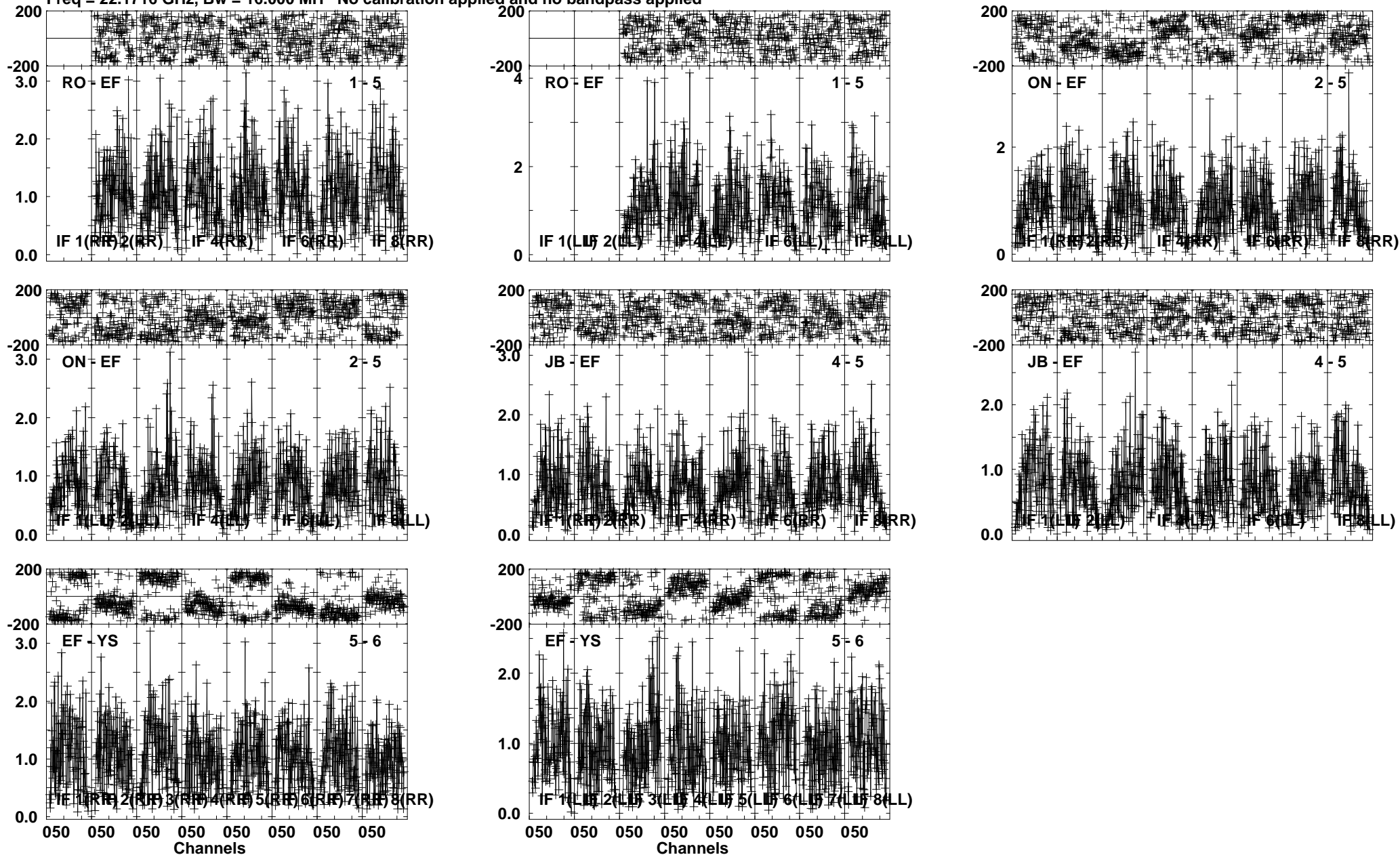
Lower frame: Milli Ampl Jy Top frame: Phas deg Vector averaged cross-power spectrum Several baselines displayed Timerange: 00/18:48:01 to 00/18:49:00
