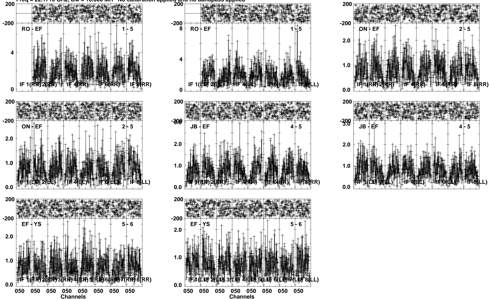
Lower frame: Milli Ampl Jy Top frame: Phas deg Vector averaged cross-power spectrum Several baselines displayed Timerange: 01/00:39:46 to 01/00:40:30
