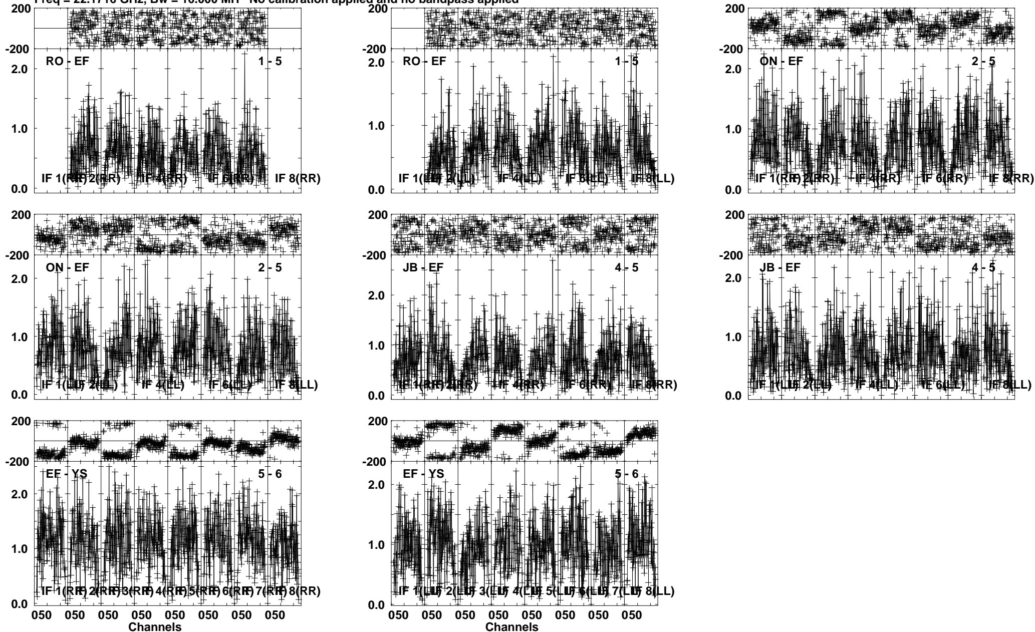
Lower frame: Milli Amp Jy Top frame: Phas deg Vector averaged cross-power spectrum Several baselines displayed Timerange: 00/16:18:01 to 00/16:19:00
