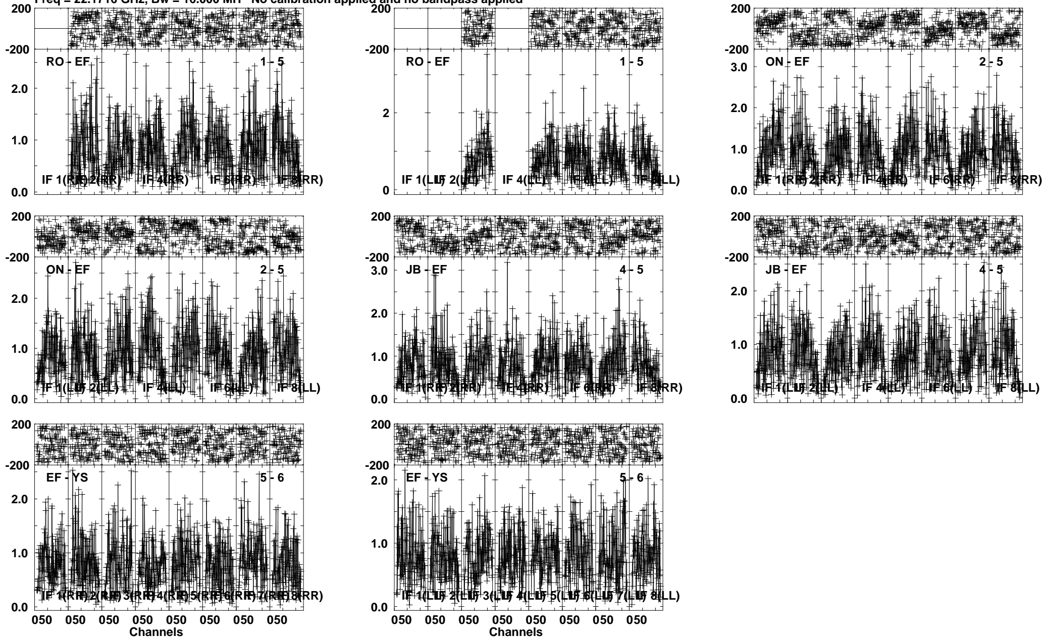
Lower frame: Milli Ampl Jy Top frame: Phas deg Vector averaged cross-power spectrum Several baselines displayed Timerange: 00/23:38:31 to 00/23:39:15
