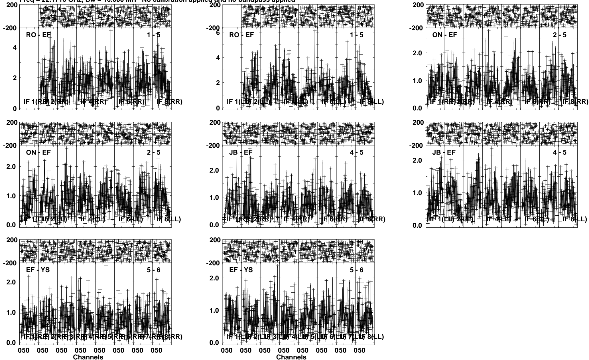
Lower frame: Milli Ampl Jy Top frame: Phas deg Vector averaged cross-power spectrum Several baselines displayed Timerange: 01/00:04:16 to 01/00:05:00
