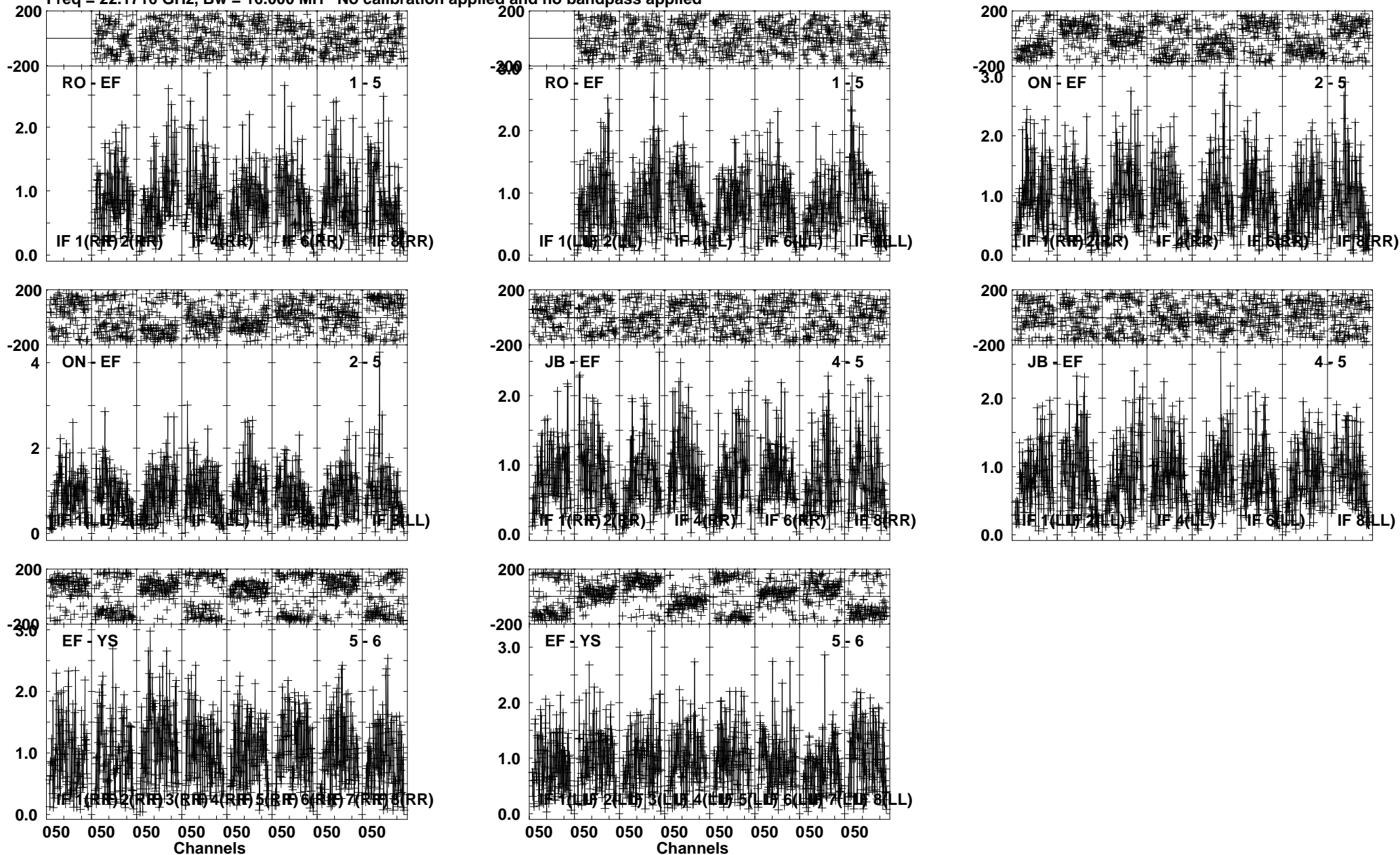
Lower frame: Milli Ampl Jy Top frame: Phas deg Vector averaged cross-power spectrum Several baselines displayed Timerange: 01/01:36:31 to 01/01:37:15
