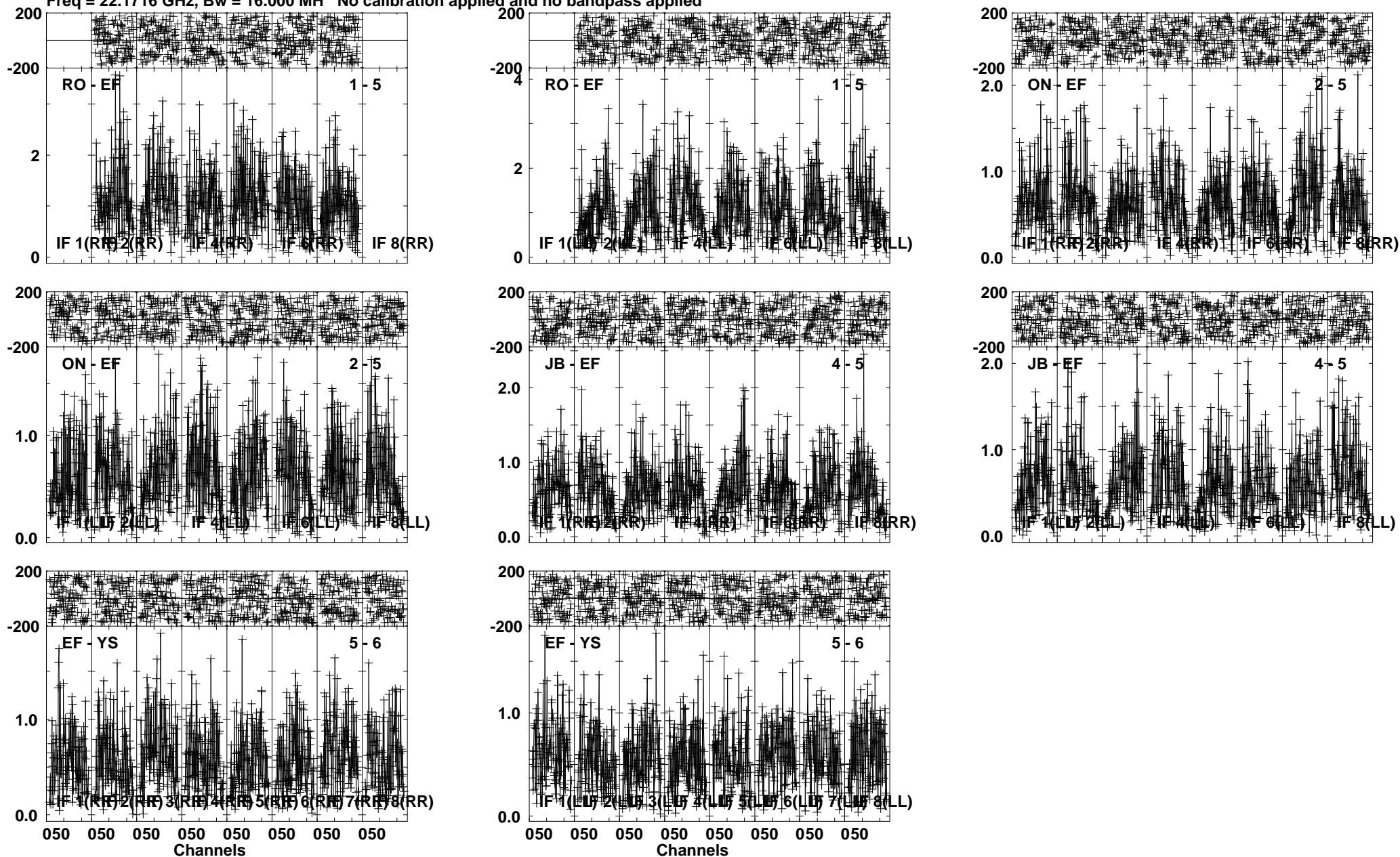
Lower frame: Milli Ampl Jy Top frame: Phas deg Vector averaged cross-power spectrum Several baselines displayed Timerange: 00/15:50:01 to 00/15:51:00
