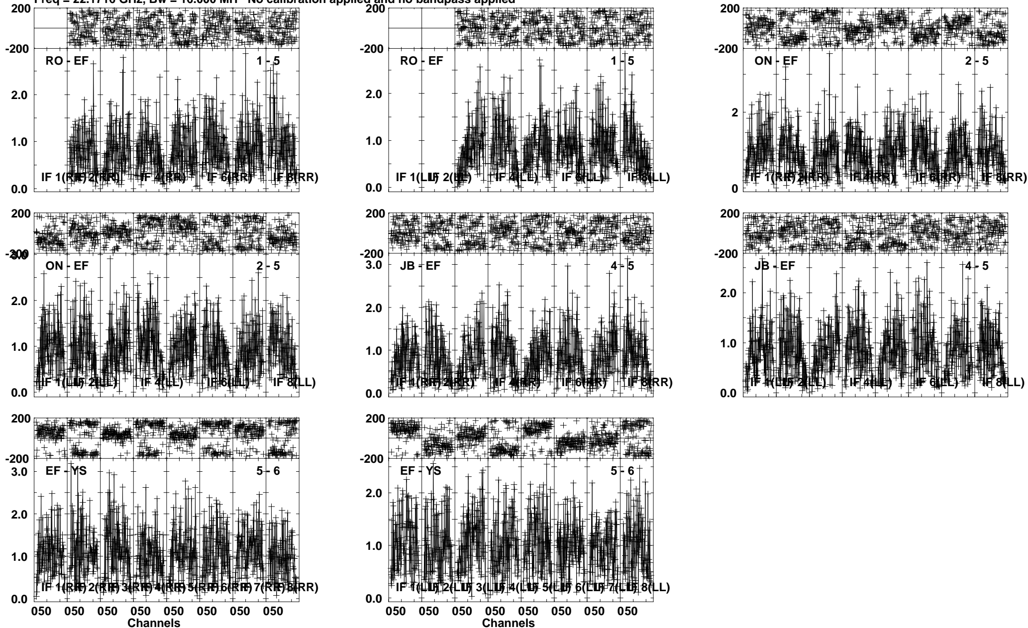
Lower frame: Milli Ampl Jy Top frame: Phas deg Vector averaged cross-power spectrum Several baselines displayed Timerange: 00/23:26:01 to 00/23:26:45
