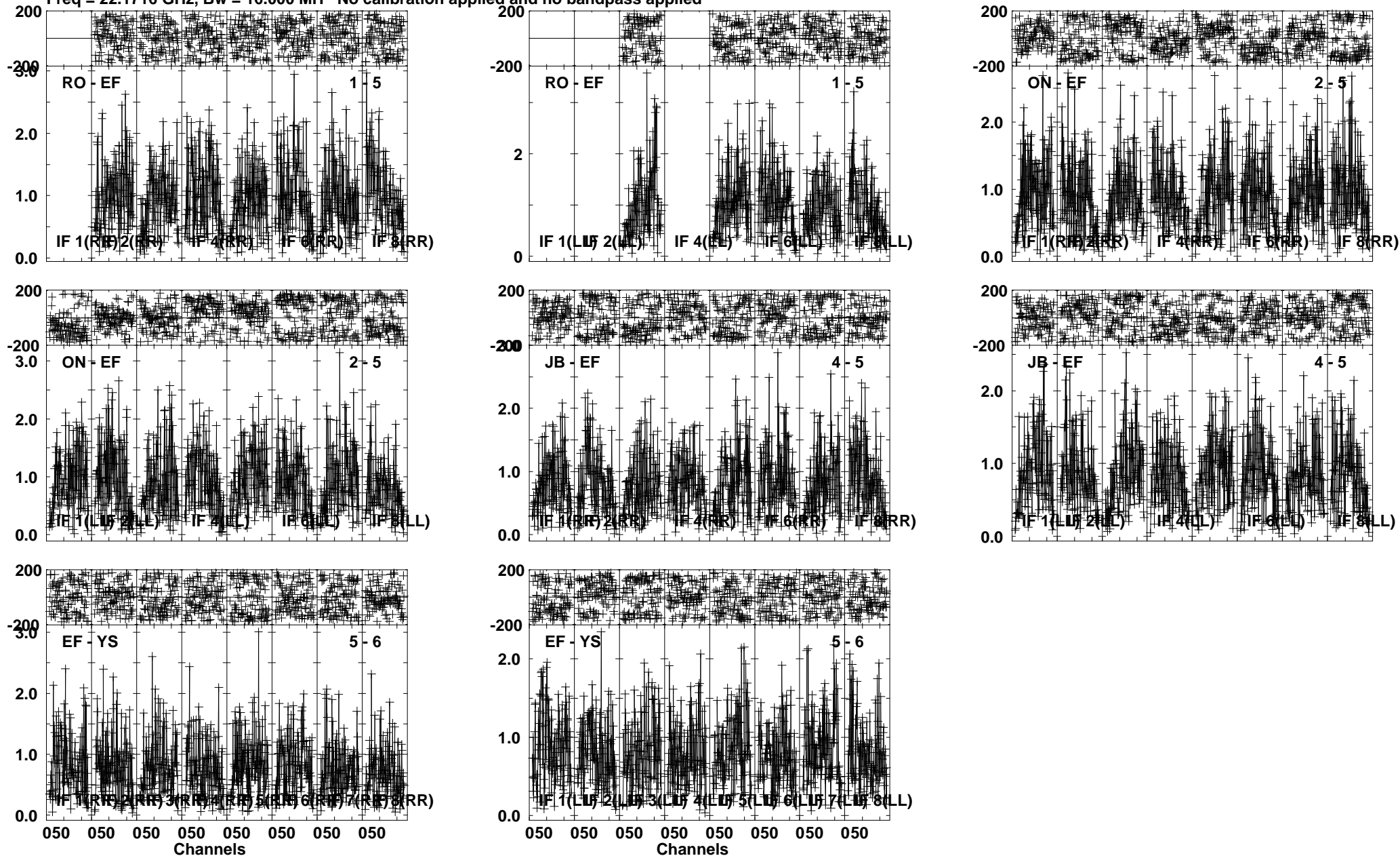
Lower frame: Milli Ampl Jy Top frame: Phas deg Vector averaged cross-power spectrum Several baselines displayed Timerange: 00/23:32:31 to 00/23:33:15
