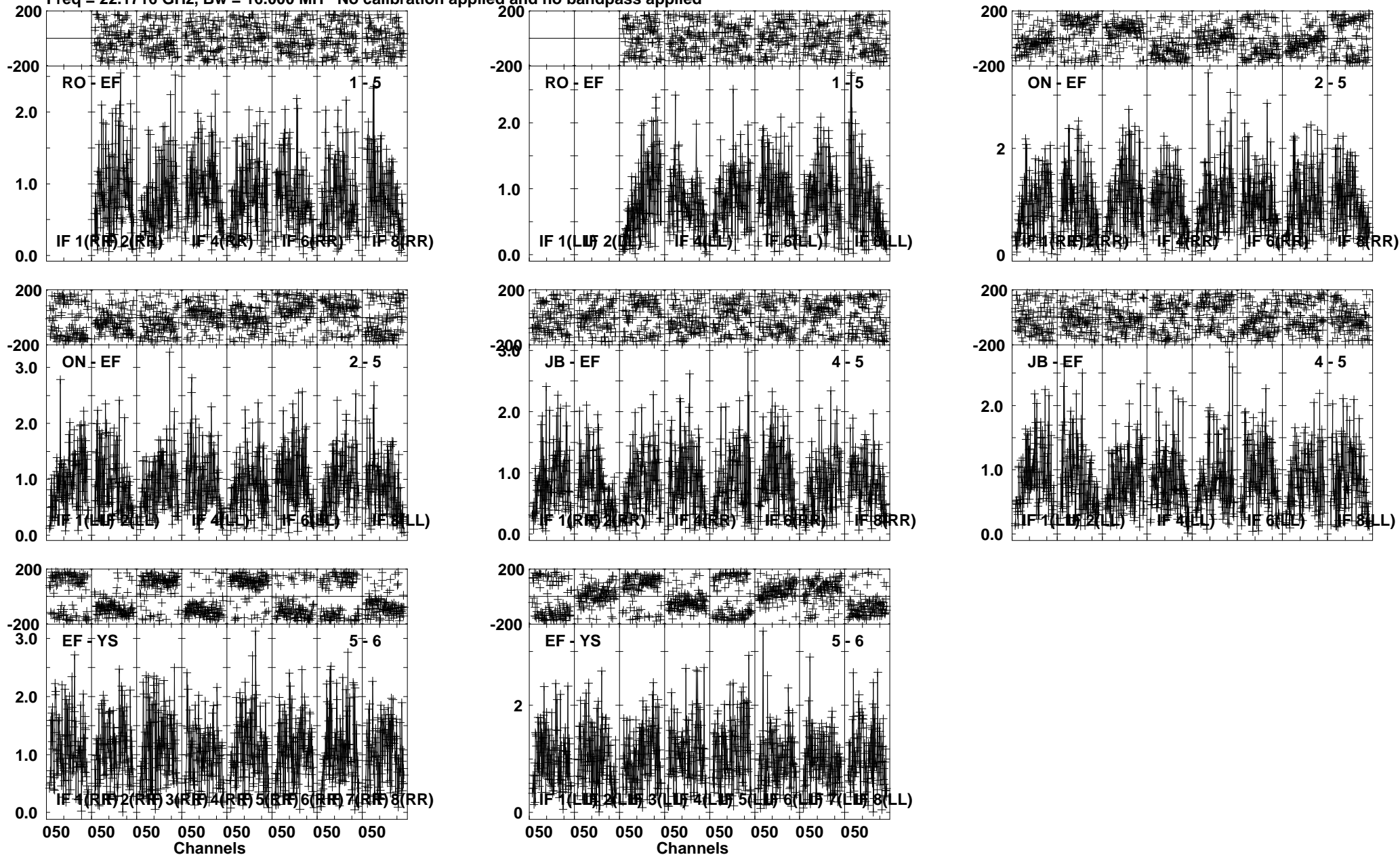
Lower frame: Milli Ampl Jy Top frame: Phas deg Vector averaged cross-power spectrum Several baselines displayed Timerange: 00/23:27:31 to 00/23:28:15
