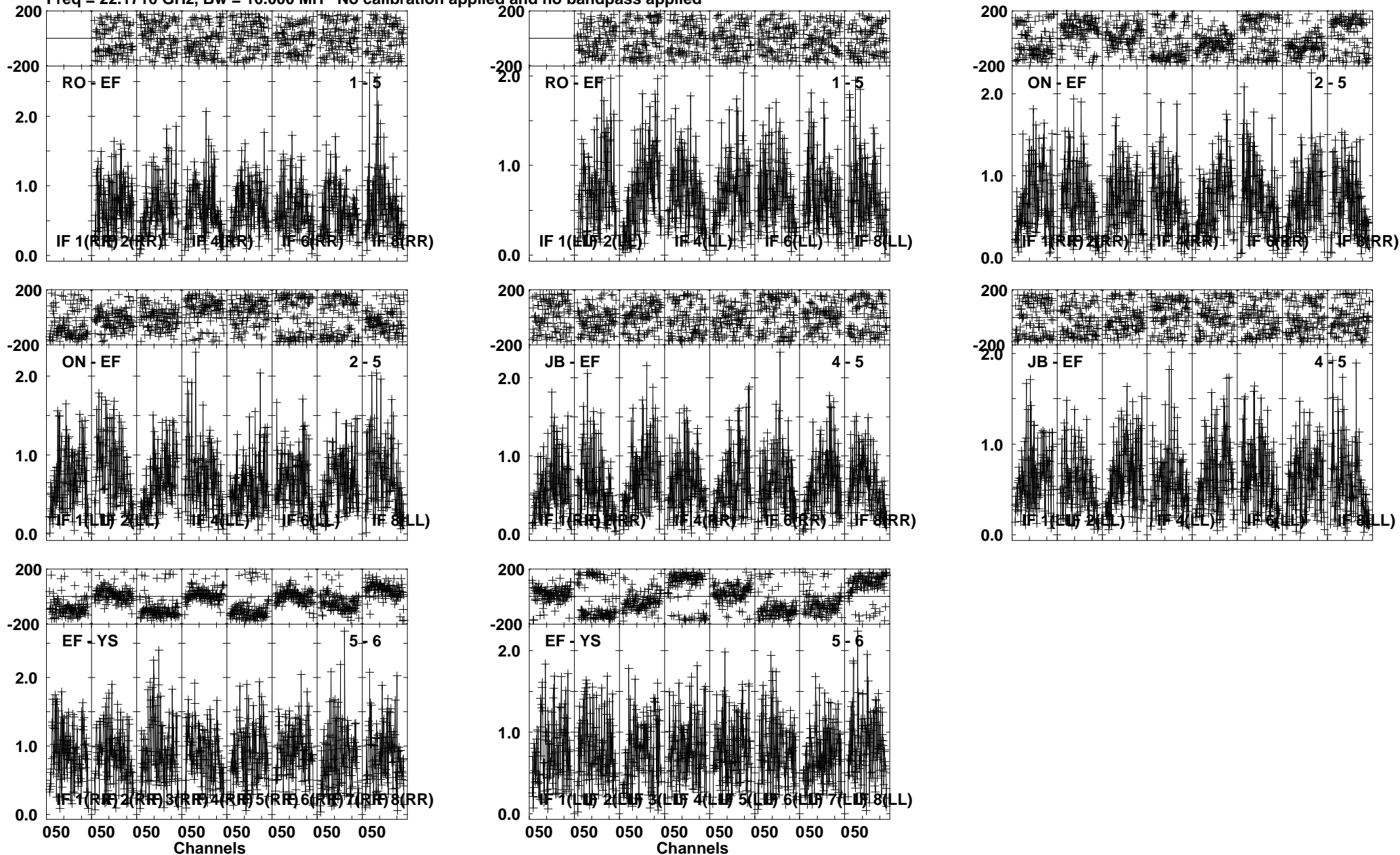
Lower frame: Milli Ampl Jy Top frame: Phas deg Vector averaged cross-power spectrum Several baselines displayed Timerange: 00/18:31:31 to 00/18:32:30
