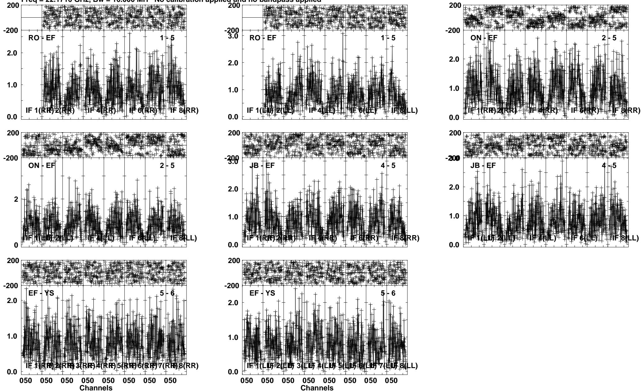
Lower frame: Milli Ampl Jy Top frame: Phas deg Vector averaged cross-power spectrum Several baselines displayed Timerange: 01/00:31:01 to 01/00:31:45
