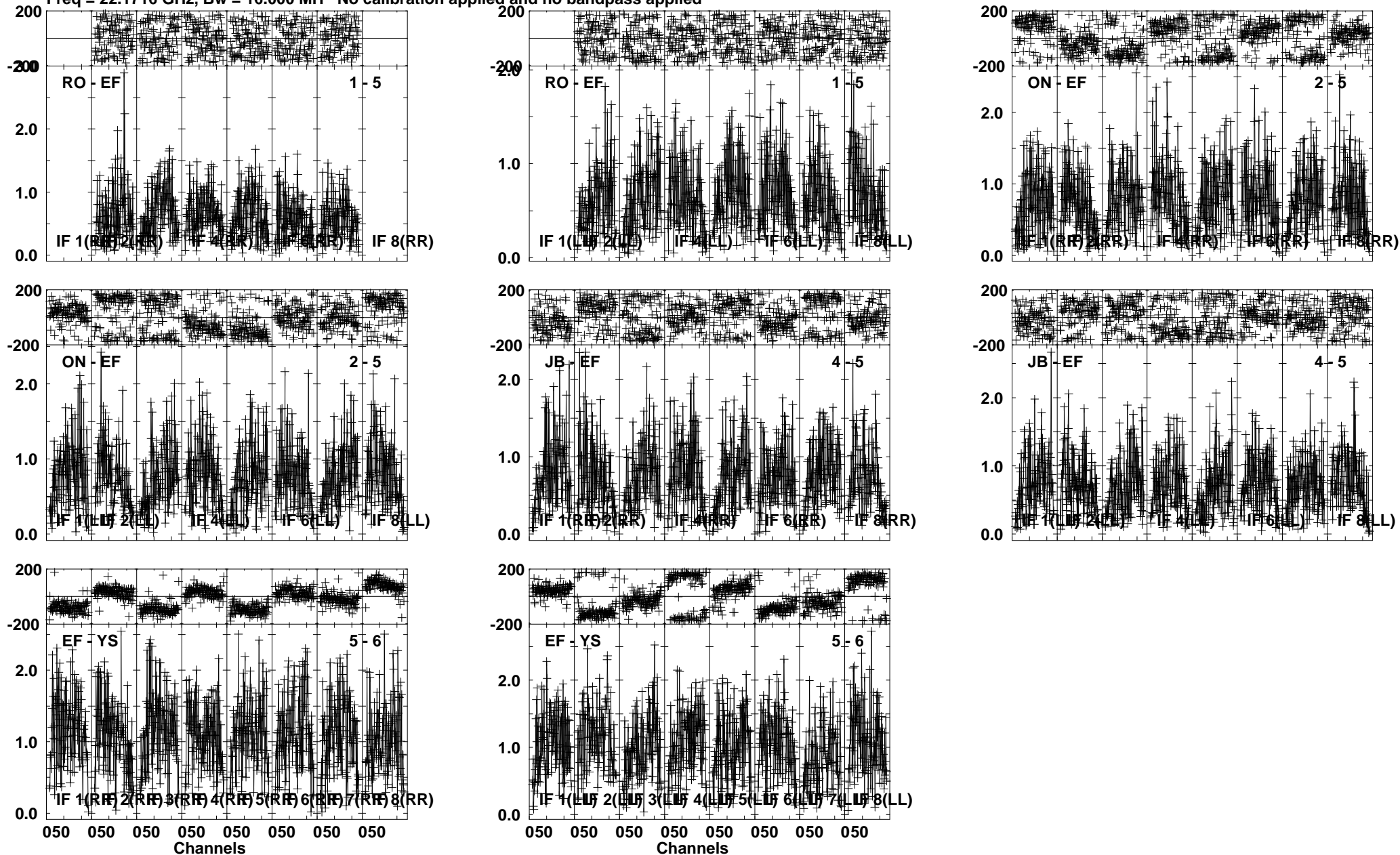
Lower frame: Milli Amp Jy Top frame: Phas deg Vector averaged cross-power spectrum Several baselines displayed Timerange: 00/16:09:31 to 00/16:10:30
