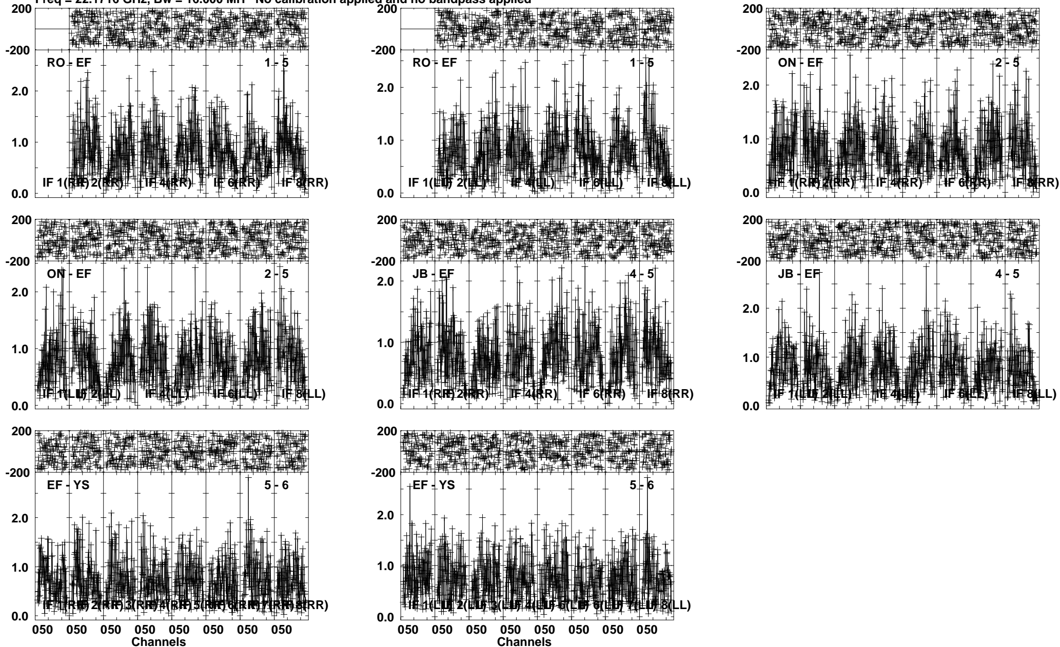
Lower frame: Milli Amp Jy Top frame: Phas deg Vector averaged cross-power spectrum Several baselines displayed Timerange: 01/00:02:46 to 01/00:03:30
