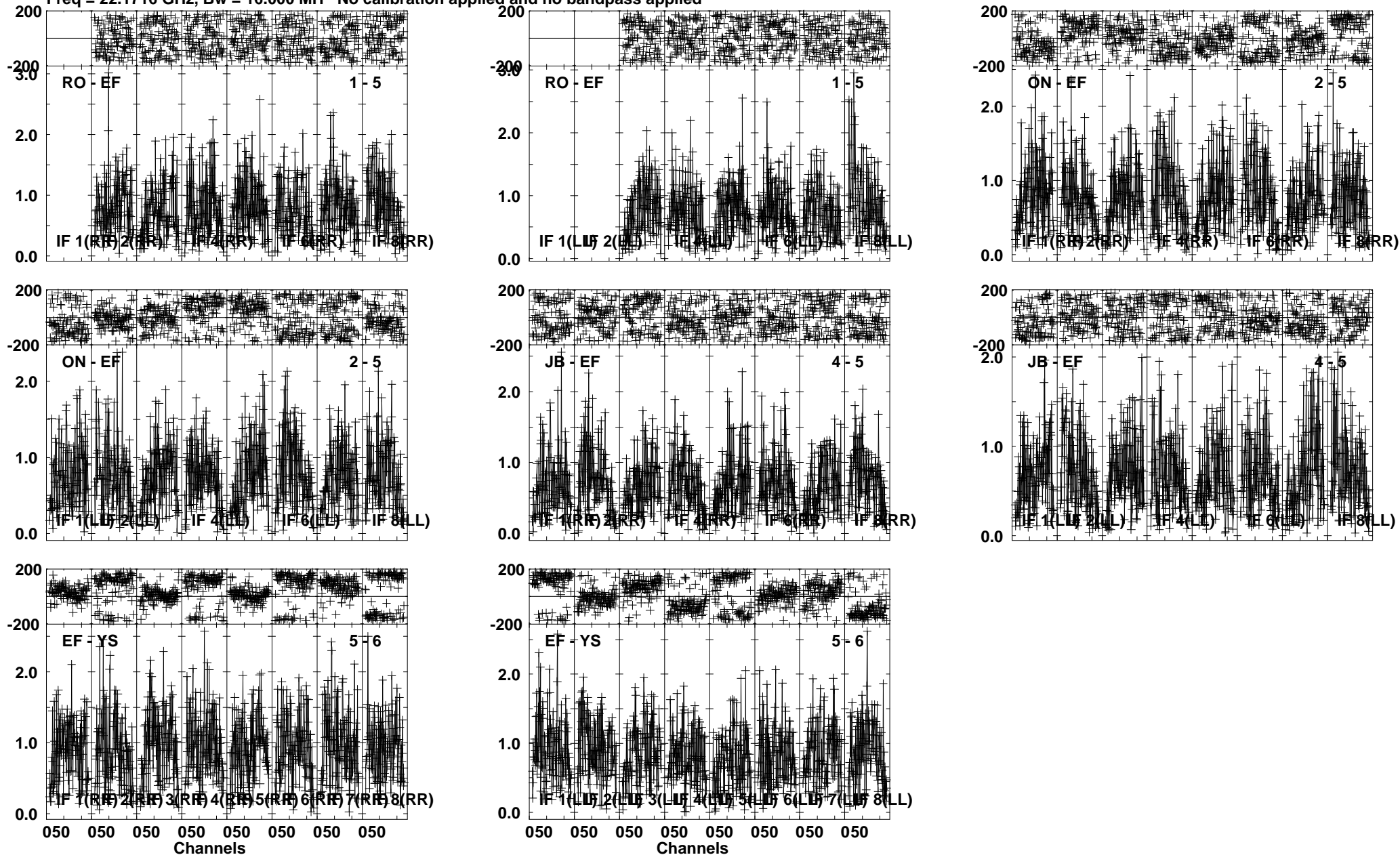
Lower frame: Milli Ampl Jy Top frame: Phas deg Vector averaged cross-power spectrum Several baselines displayed Timerange: 00/18:27:01 to 00/18:28:00
