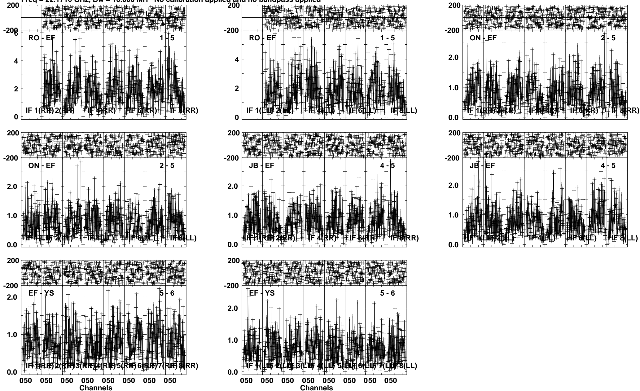
Lower frame: Milli Ampl Jy Top frame: Phas deg Vector averaged cross-power spectrum Several baselines displayed Timerange: 01/00:30:16 to 01/00:31:00
