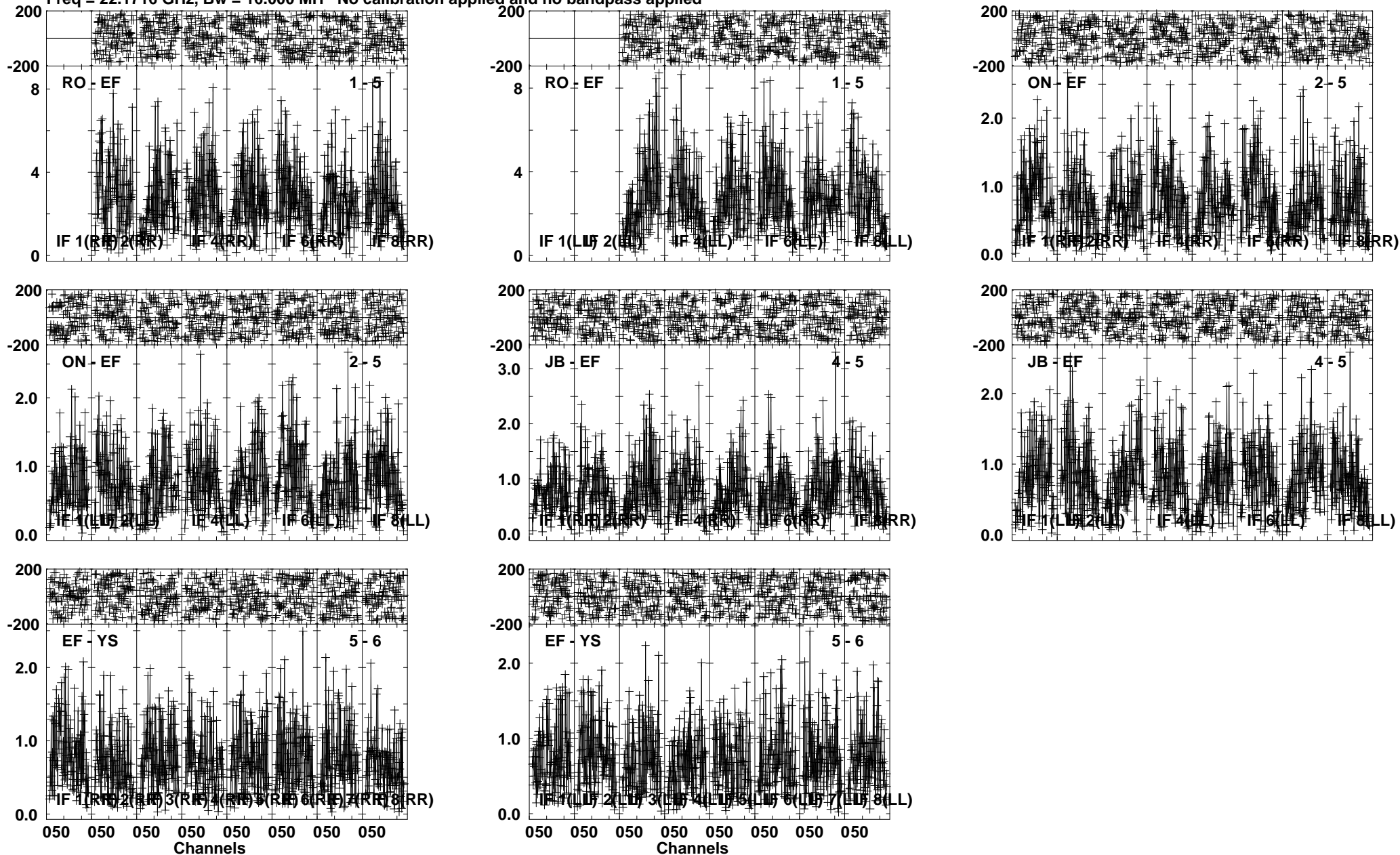
Lower frame: Milli Ampl Jy Top frame: Phas deg Vector averaged cross-power spectrum Several baselines displayed Timerange: 01/01:20:16 to 01/01:21:00
