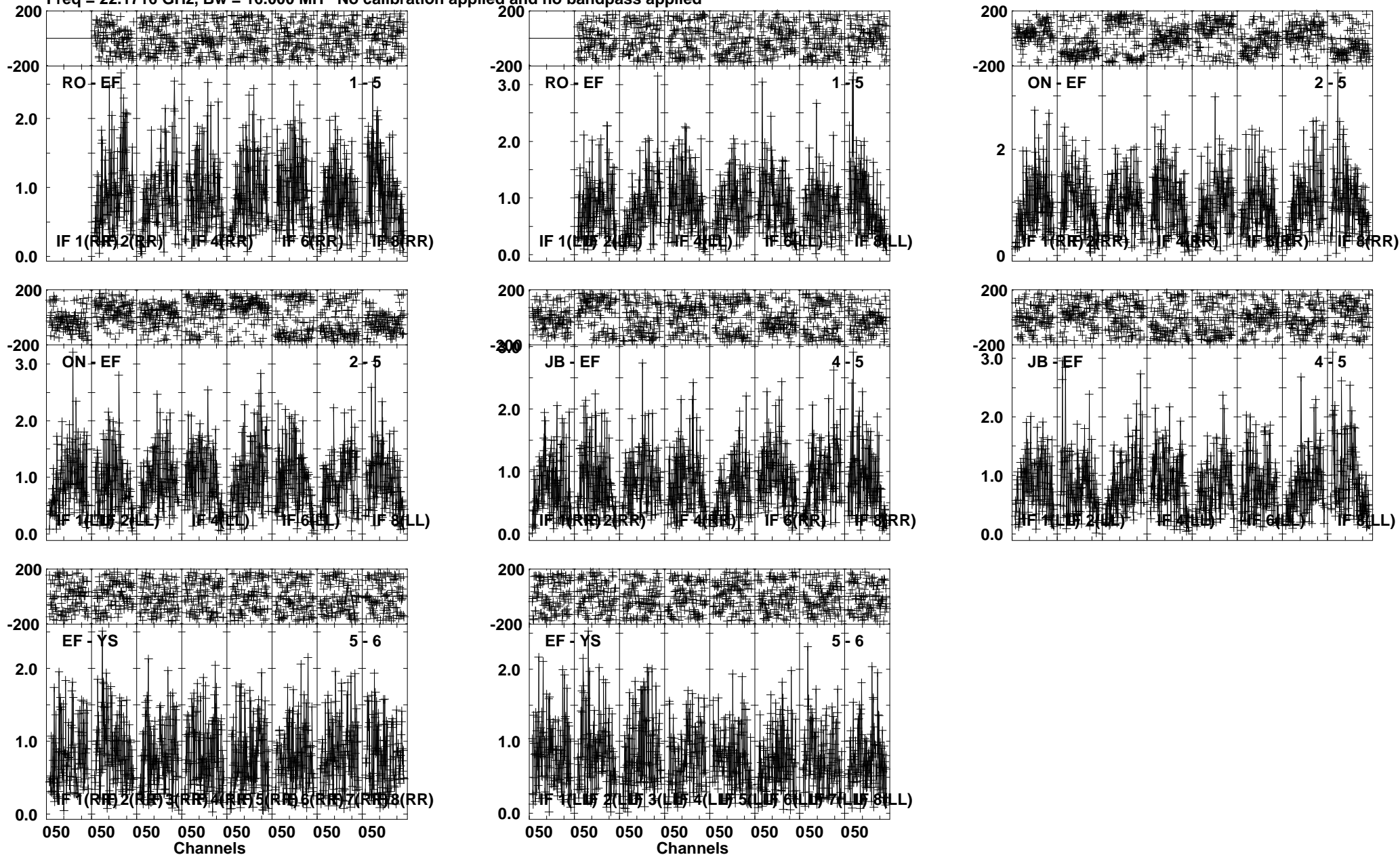
Lower frame: Milli Ampl Jy Top frame: Phas deg Vector averaged cross-power spectrum Several baselines displayed Timerange: 01/00:45:01 to 01/00:45:45
