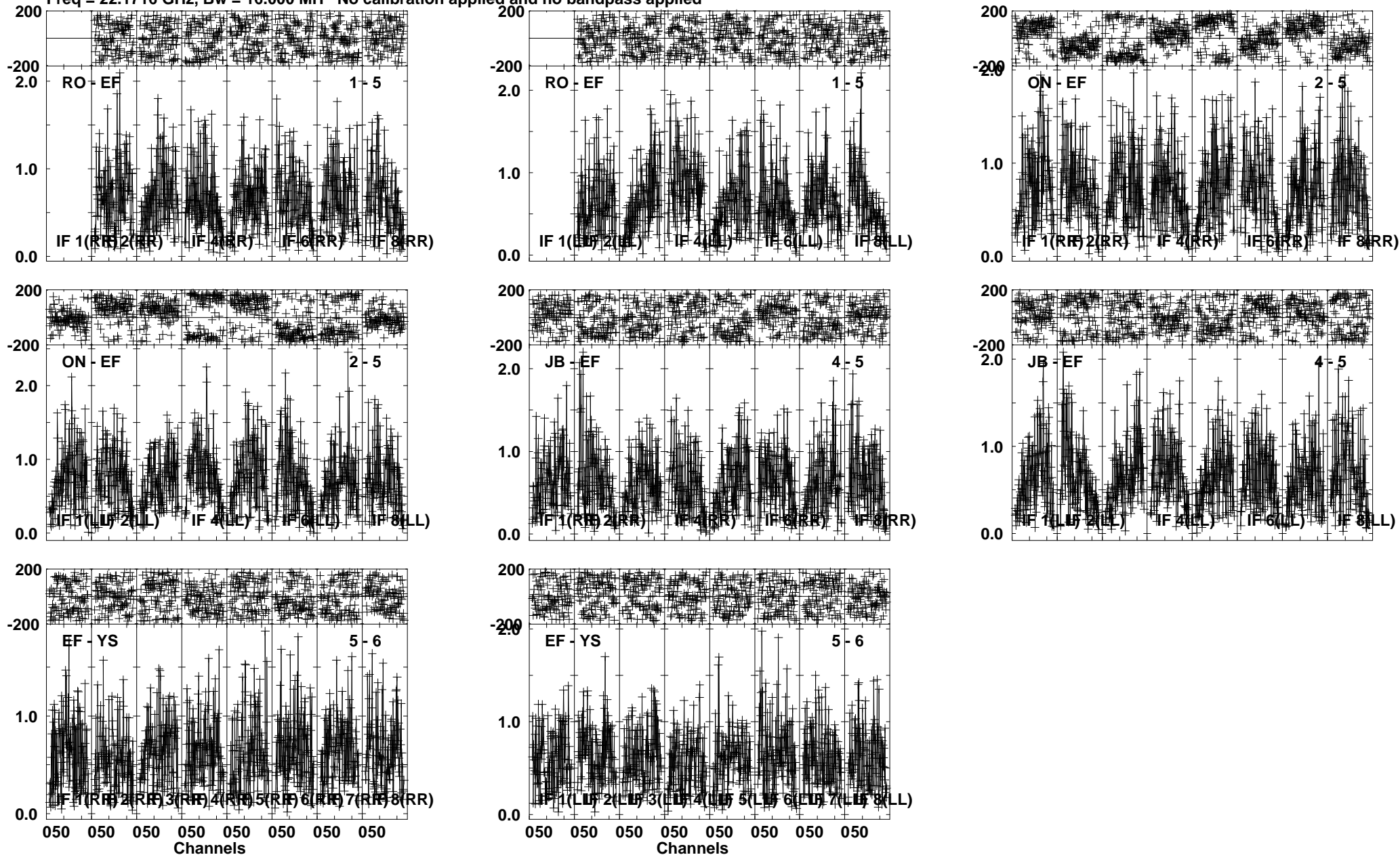
Lower frame: Milli Ampl Jy Top frame: Phas deg Vector averaged cross-power spectrum Several baselines displayed Timerange: 01/00:48:31 to 01/00:49:15
