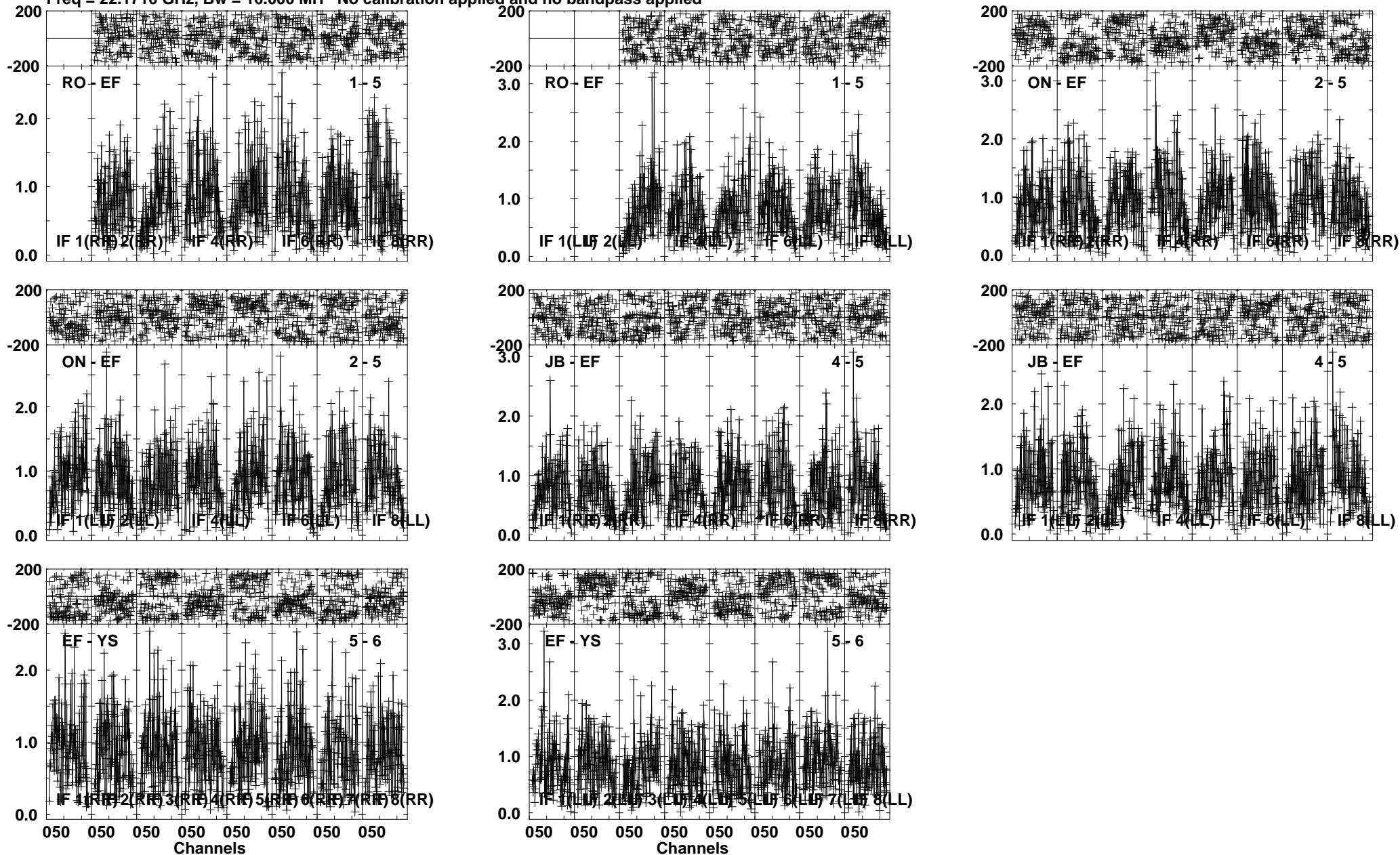
Lower frame: Milli Ampl Jy Top frame: Phas deg Vector averaged cross-power spectrum Several baselines displayed Timerange: 01/01:11:31 to 01/01:12:15
