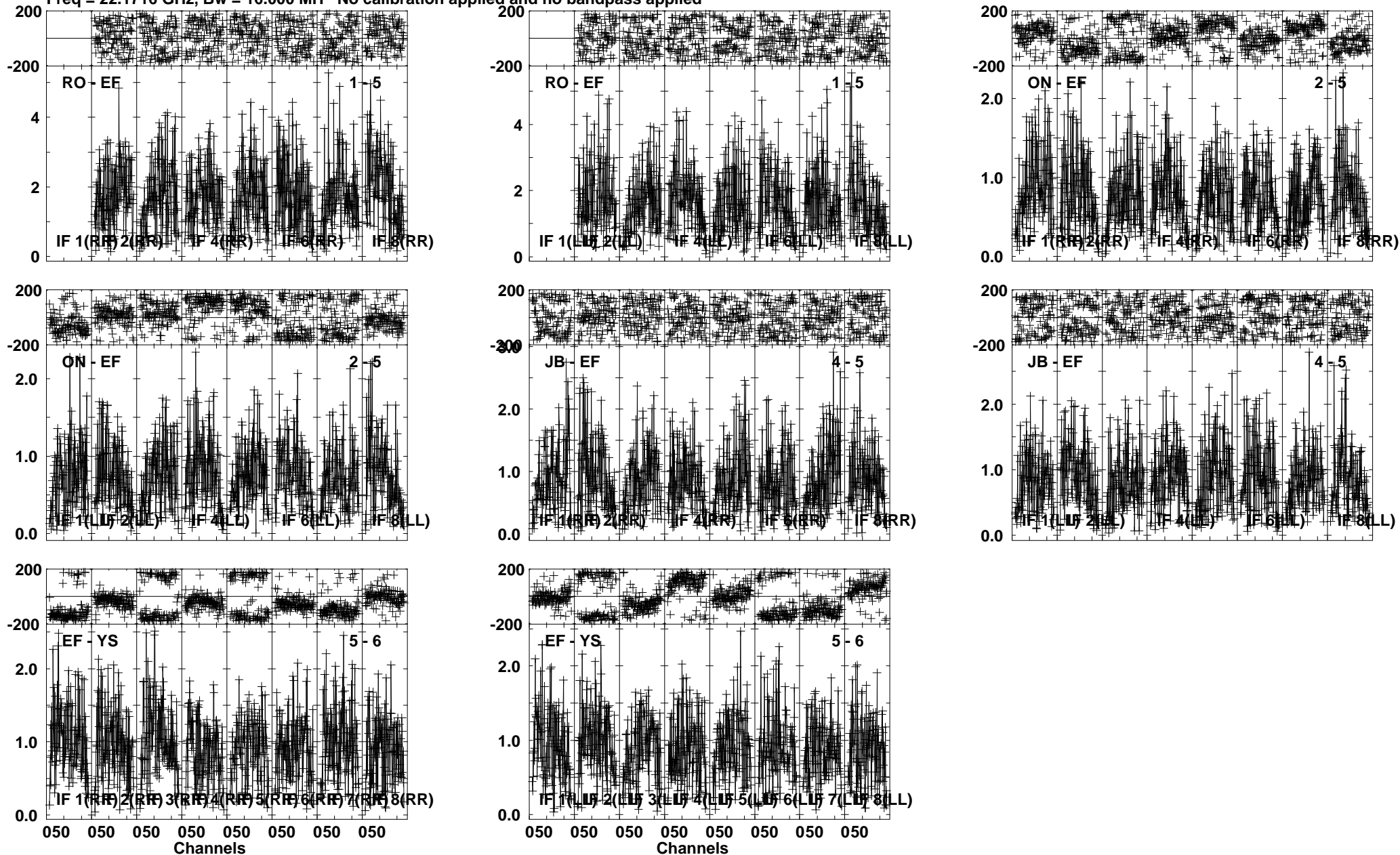
Lower frame: Milli Ampl Jy Top frame: Phas deg Vector averaged cross-power spectrum Several baselines displayed Timerange: 00/20:02:31 to 00/20:03:30
