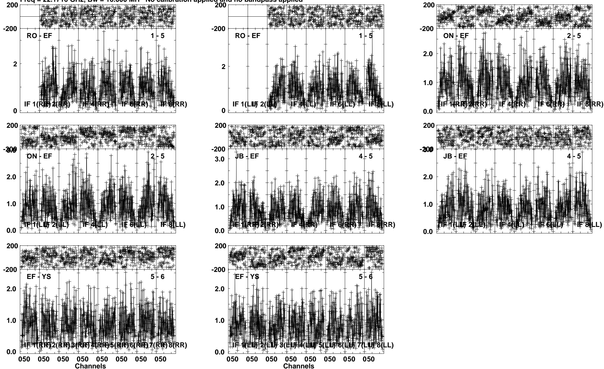
Lower frame: Milli Ampl Jy Top frame: Phas deg Vector averaged cross-power spectrum Several baselines displayed Timerange: 00/23:29:01 to 00/23:29:45
