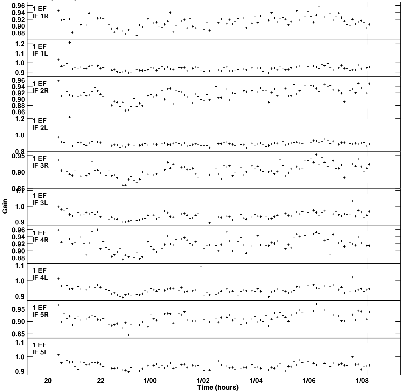
Plot file version 1 created 10-JUN-2016 18:04:34 Gain amp vs UTC time for J1957+3338.MULTI.1 SN 2 Rpol & Lpol IF 1 - 8
