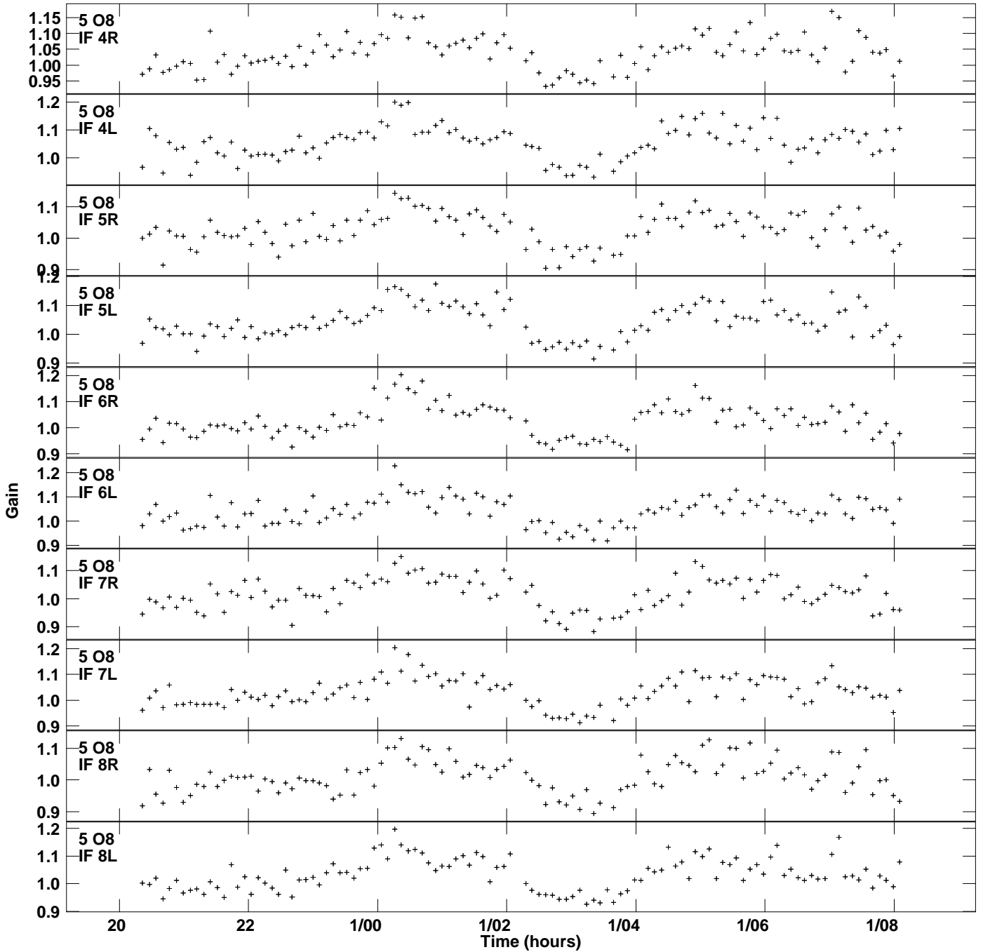
Plot file version 8 created 10-JUN-2016 18:04:34 Gain amp vs UTC time for J1957+3338.MULTI.1 SN 2 Rpol & Lpol IF 1 - 8
