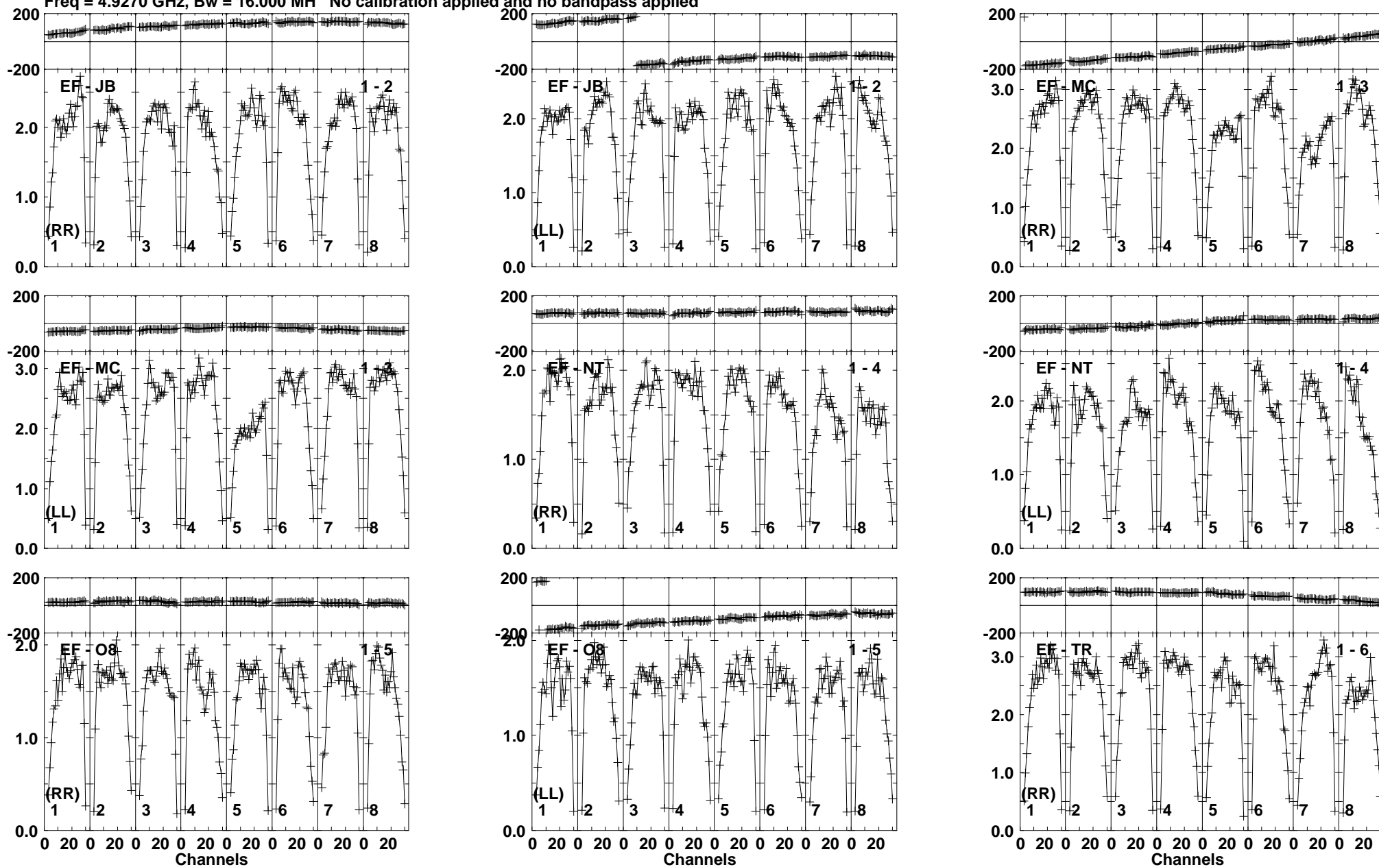
Lower frame: Milli Ampl Jy Top frame: Phas deg Vector averaged cross-power spectrum Baseline: EF (01) - JB (02) Timerange: 01/01:37:11 to 01/01:38:39
