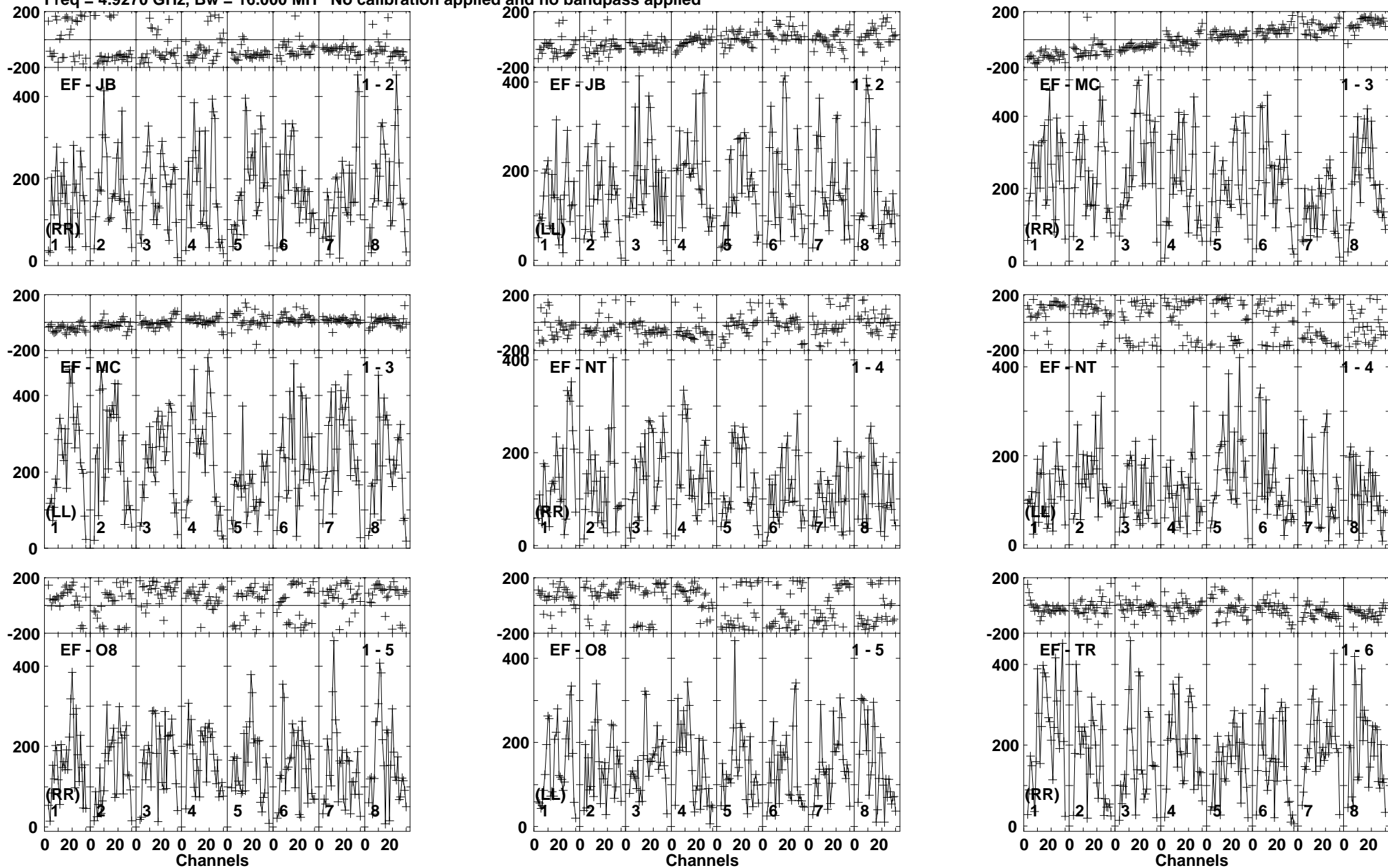
Lower frame: Micro Ampl Jy Top frame: Phas deg Vector averaged cross-power spectrum Baseline: EF (01) - JB (02) Timerange: 01/07:47:20 to 01/07:49:19
