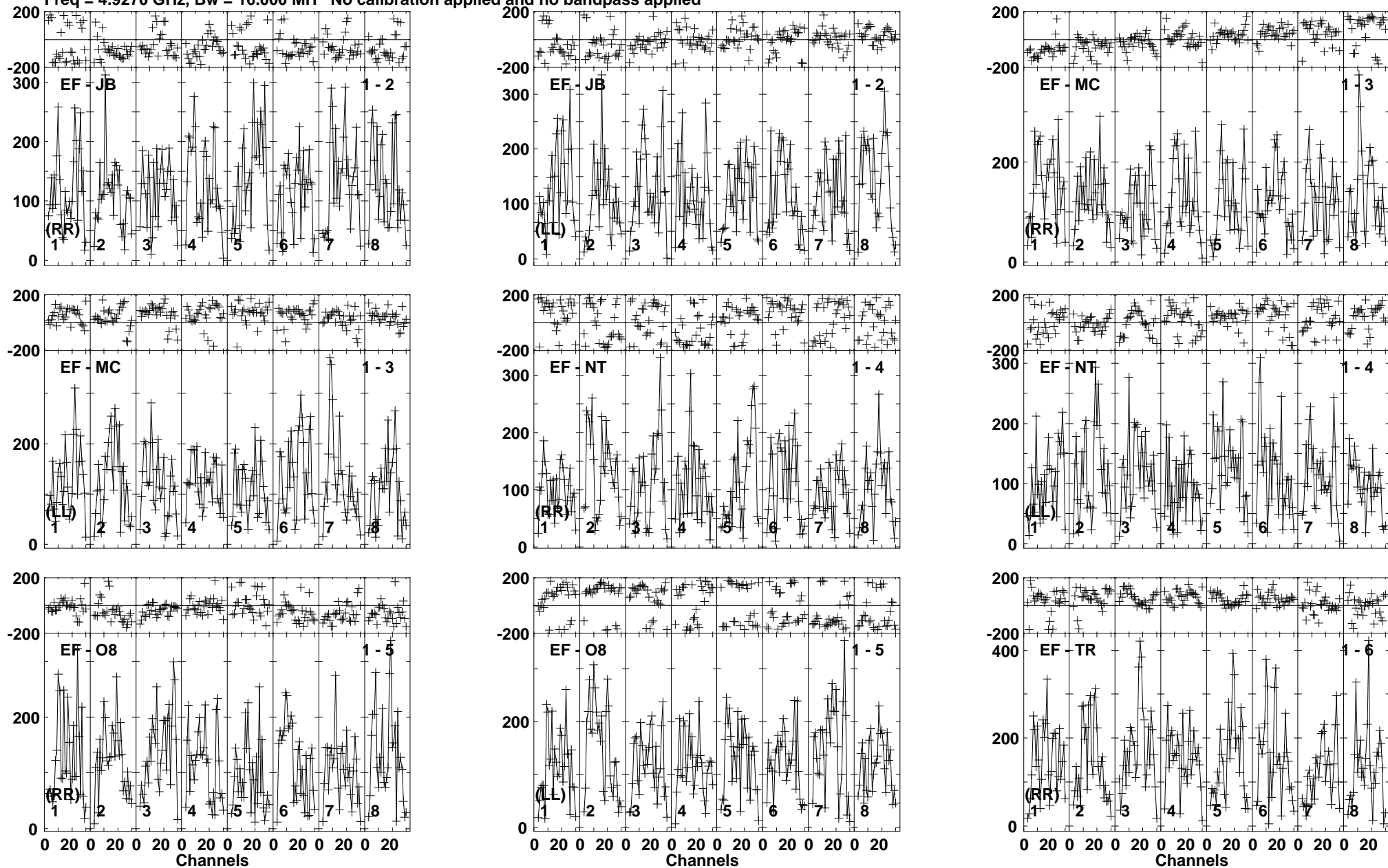
Lower frame: Micro Ampl Jy Top frame: Phas deg Vector averaged cross-power spectrum Baseline: EF (01) - JB (02) Timerange: 01/00:44:00 to 01/00:46:30
