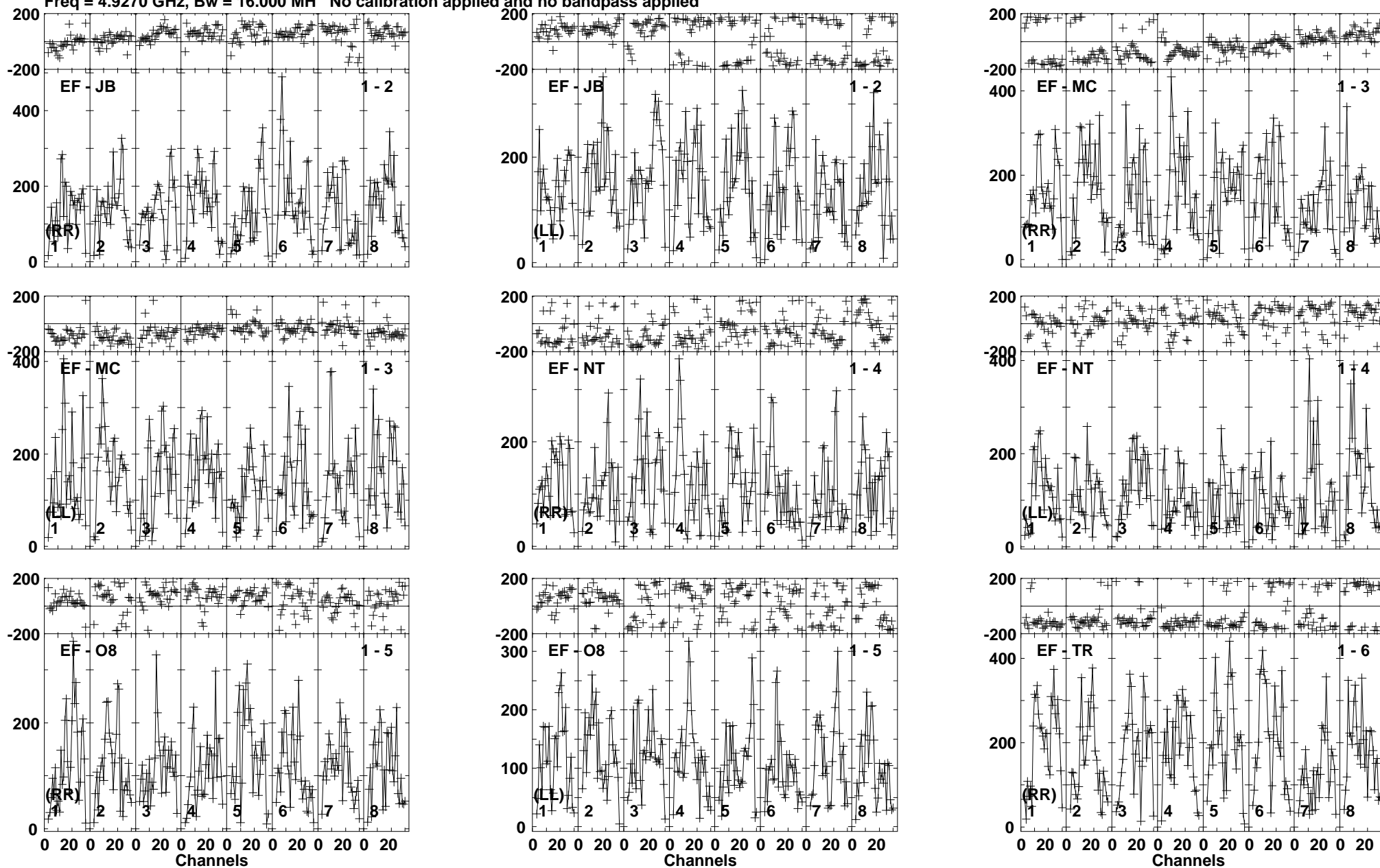
Lower frame: Micro Ampl Jy Top frame: Phas deg Vector averaged cross-power spectrum Baseline: EF (01) - JB (02) Timerange: 01/06:40:01 to 01/06:42:30
