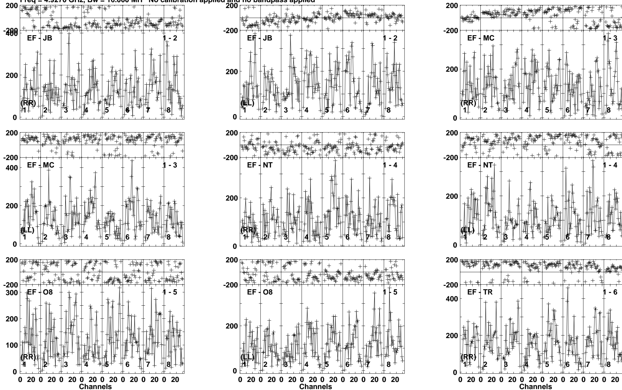
Lower frame: Micro Ampl Jy Top frame: Phas deg Vector averaged cross-power spectrum Baseline: EF (01) - JB (02) Timerange: 01/05:30:01 to 01/05:32:29
