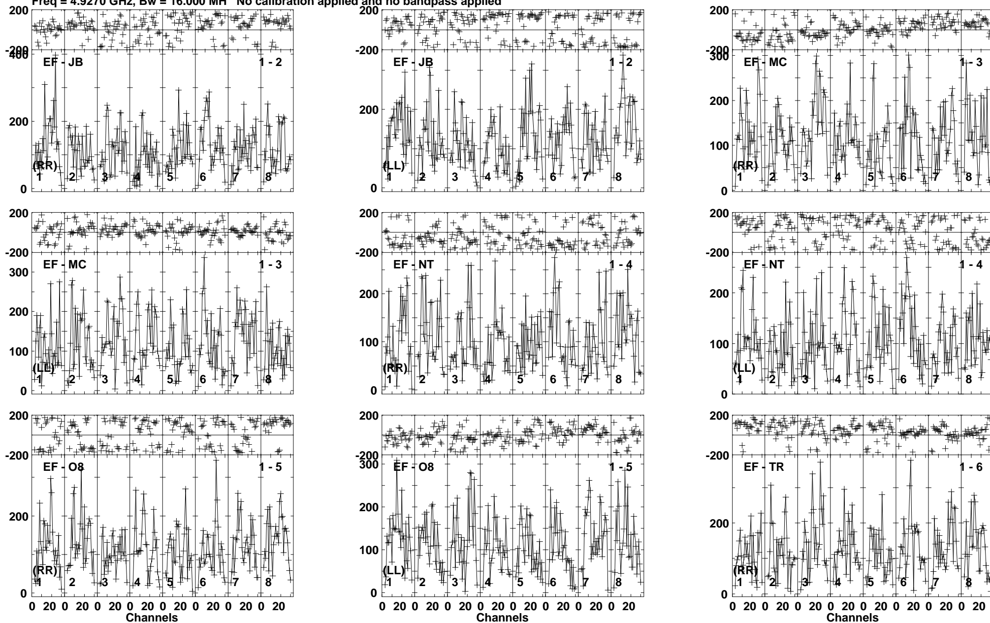
Lower frame: Micro Ampl Jy Top frame: Phas deg Vector averaged cross-power spectrum Baseline: EF (01) - JB (02) Timerange: 00/20:43:20 to 00/20:45:49
