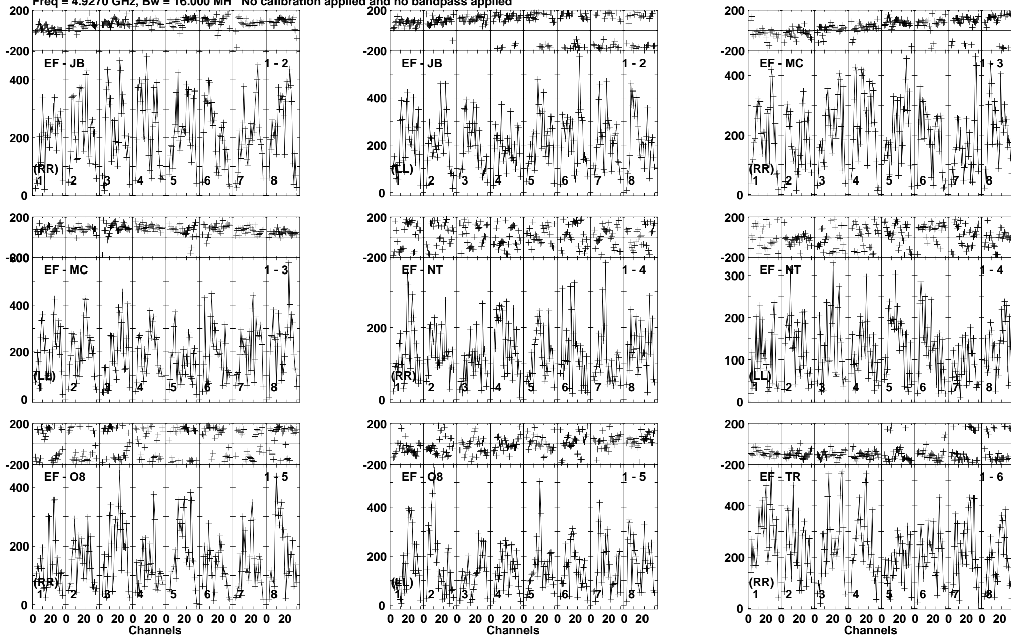
Lower frame: Micro Ampl Jy Top frame: Phas deg Vector averaged cross-power spectrum Baseline: EF (01) - JB (02) Timerange: 00/21:44:40 to 00/21:46:40
