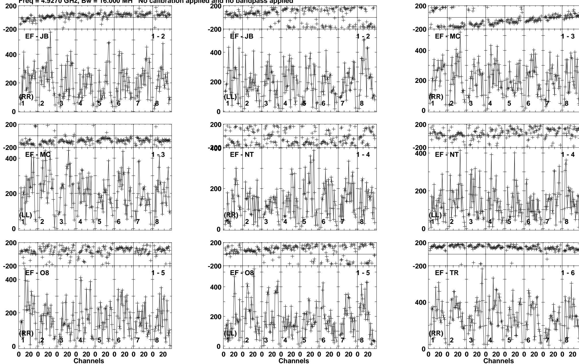
Lower frame: Micro Ampl Jy Top frame: Phas deg Vector averaged cross-power spectrum Baseline: EF (01) - JB (02) Timerange: 01/06:31:20 to 01/06:33:19
