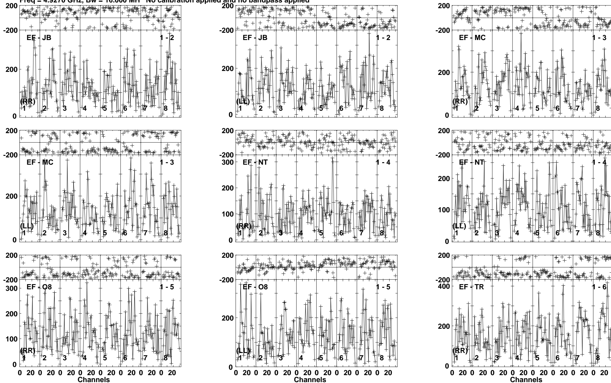
Lower frame: Micro Ampl Jy Top frame: Phas deg Vector averaged cross-power spectrum Baseline: EF (01) - JB (02) Timerange: 00/23:22:01 to 00/23:24:30
