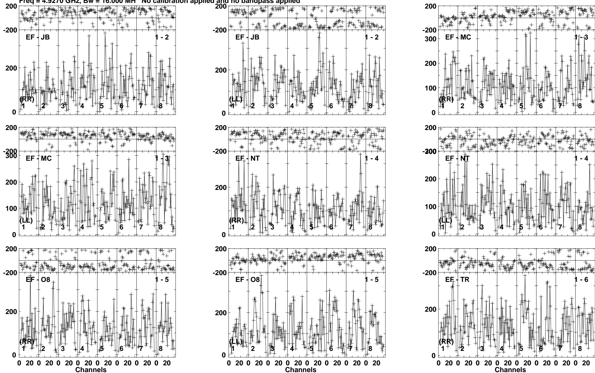
Lower frame: Micro Ampl Jy Top frame: Phas deg Vector averaged cross-power spectrum Baseline: EF (01) - JB (02) Timerange: 00/21:46:41 to 00/21:49:09
