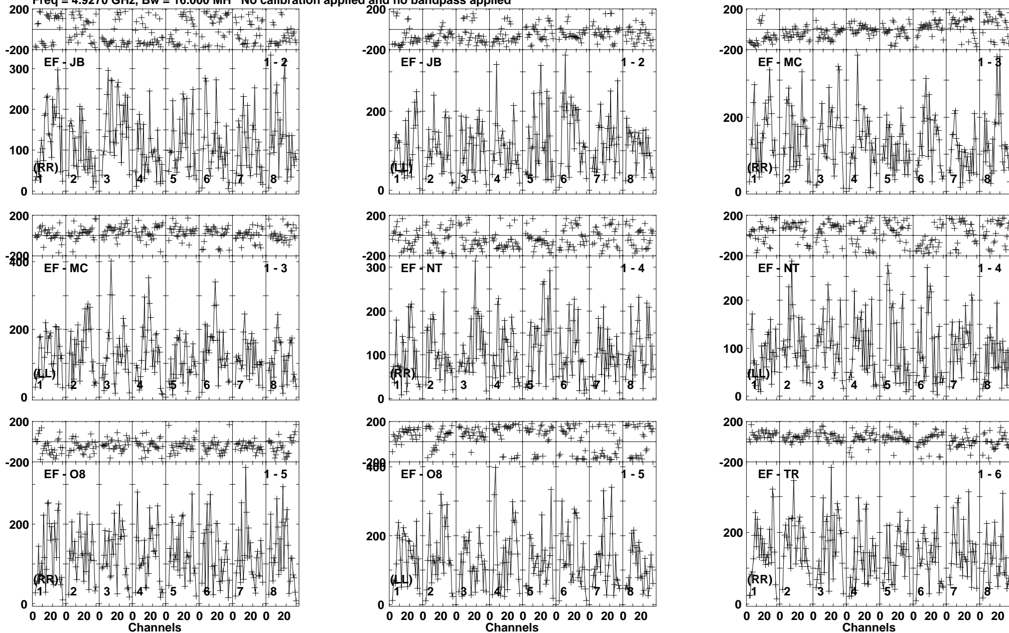
Lower frame: Micro Ampl Jy Top frame: Phas deg Vector averaged cross-power spectrum Baseline: EF (01) - JB (02) Timerange: 00:22:12:00 to 00:22:14:29
