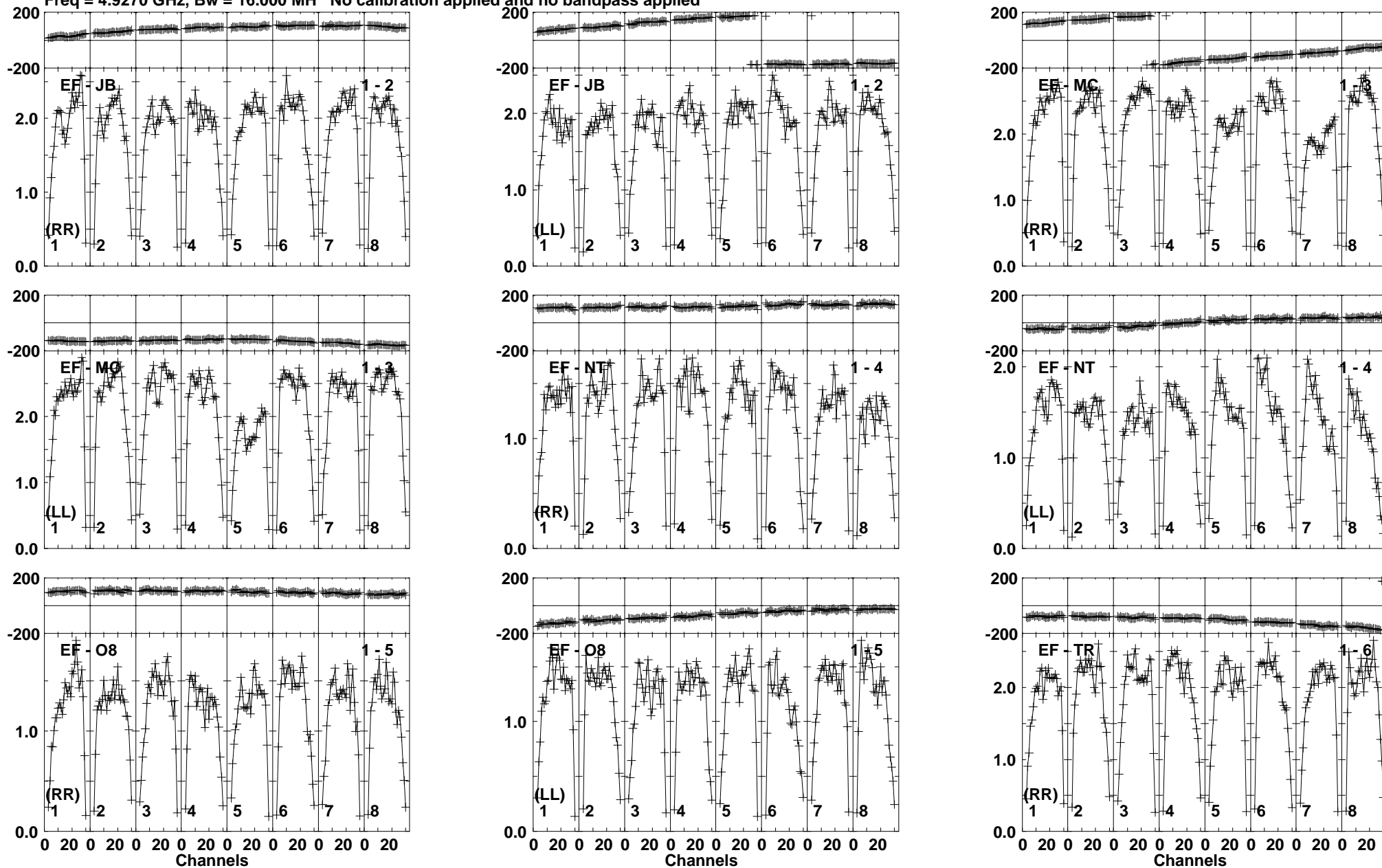
Lower frame: Milli Ampl Jy Top frame: Phas deg Vector averaged cross-power spectrum Baseline: EF (01) - JB (02) Timerange: 00/21:23:51 to 00/21:25:20
