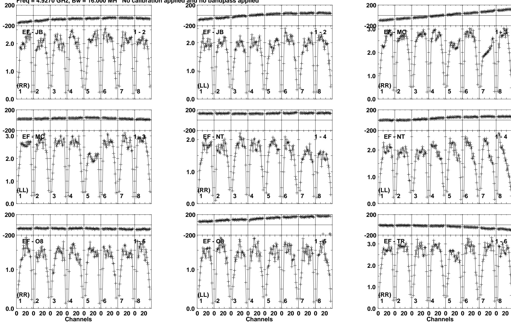
Lower frame: Milli Ampl Jy Top frame: Phas deg Vector averaged cross-power spectrum Baseline: EF (01) - JB (02) Timerange: 01/00:33:51 to 01/00:35:19
