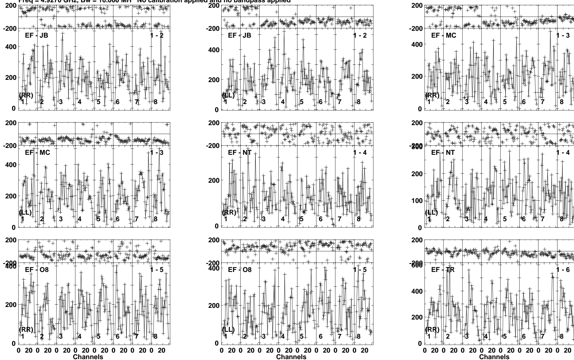
Lower frame: Micro Ampl Jy Top frame: Phas deg Vector averaged cross-power spectrum Baseline: EF (01) - JB (02) Timerange: 00/21:57:20 to 00/21:59:20
