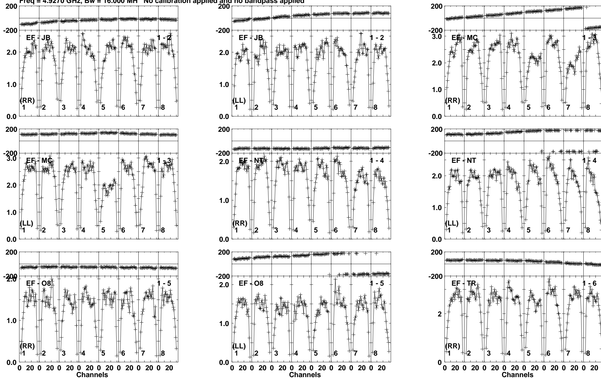
Lower frame: Milli Ampl Jy Top frame: Phas deg Vector averaged cross-power spectrum Baseline: EF (01) - JB (02) Timerange: 01/00:53:11 to 01/00:54:40
