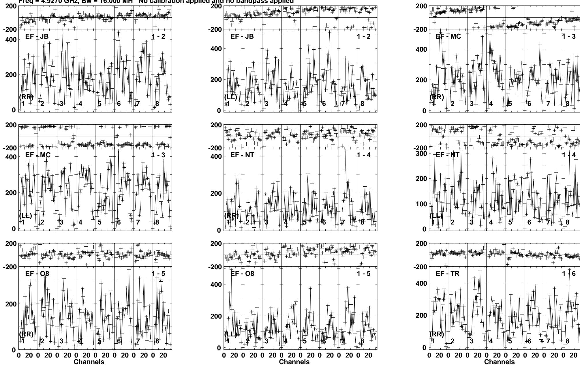
Lower frame: Micro Ampl Jy Top frame: Phas deg Vector averaged cross-power spectrum Baseline: EF (01) - JB (02) Timerange: 01/06:00:00 to 01/06:01:59
