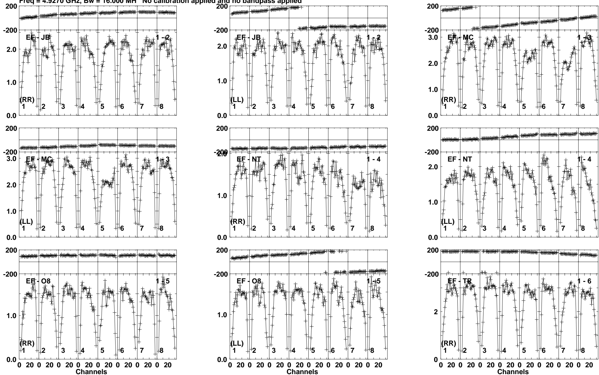
Lower frame: Milli Ampl Jy Top frame: Phas deg Vector averaged cross-power spectrum Baseline: EF (01) - JB (02) Timerange: 01/06:29:50 to 01/06:31:19
