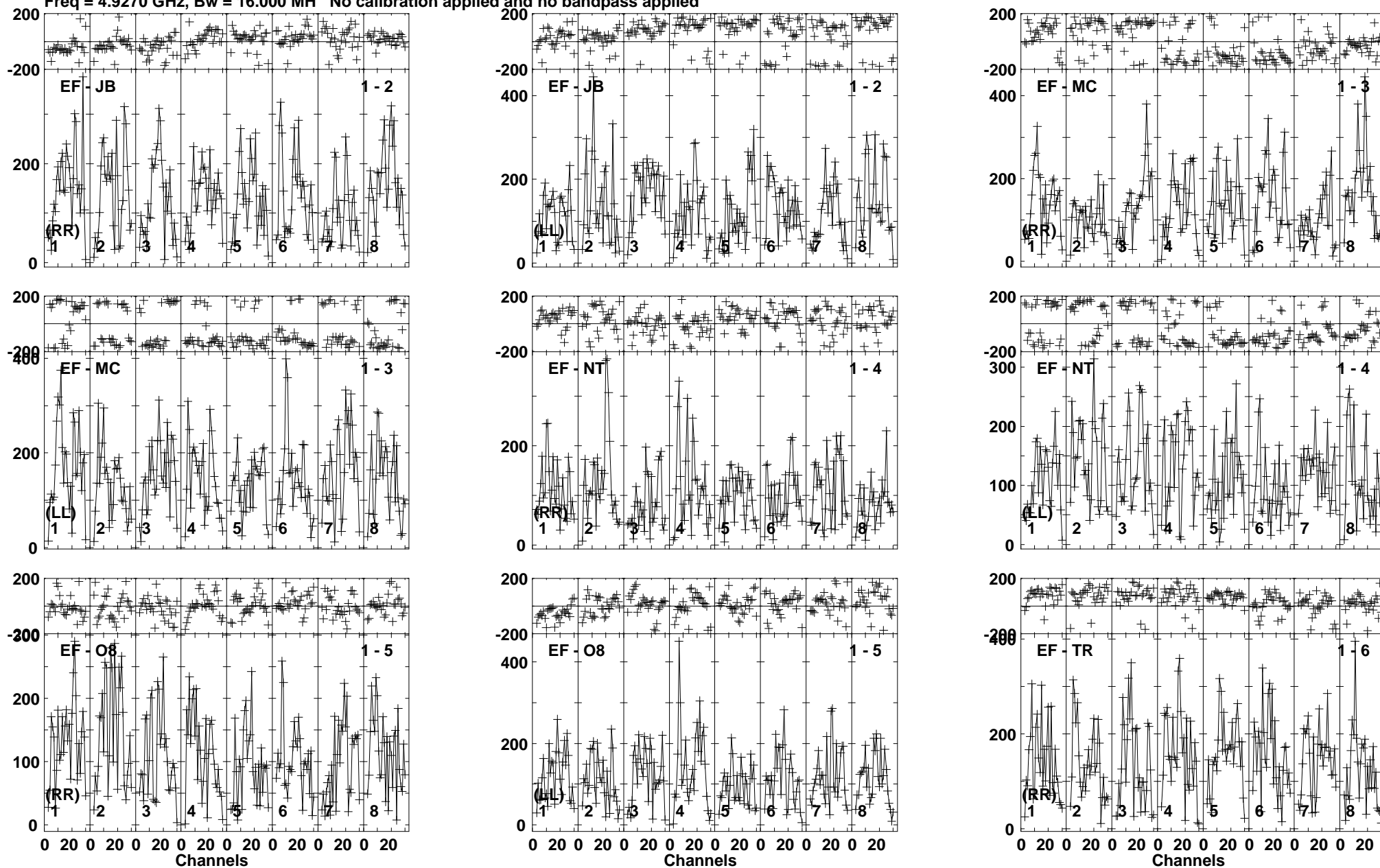
Lower frame: Micro Ampl Jy Top frame: Phas deg Vector averaged cross-power spectrum Baseline: EF (01) - JB (02) Timerange: 01/05:55:20 to 01/05:57:50
