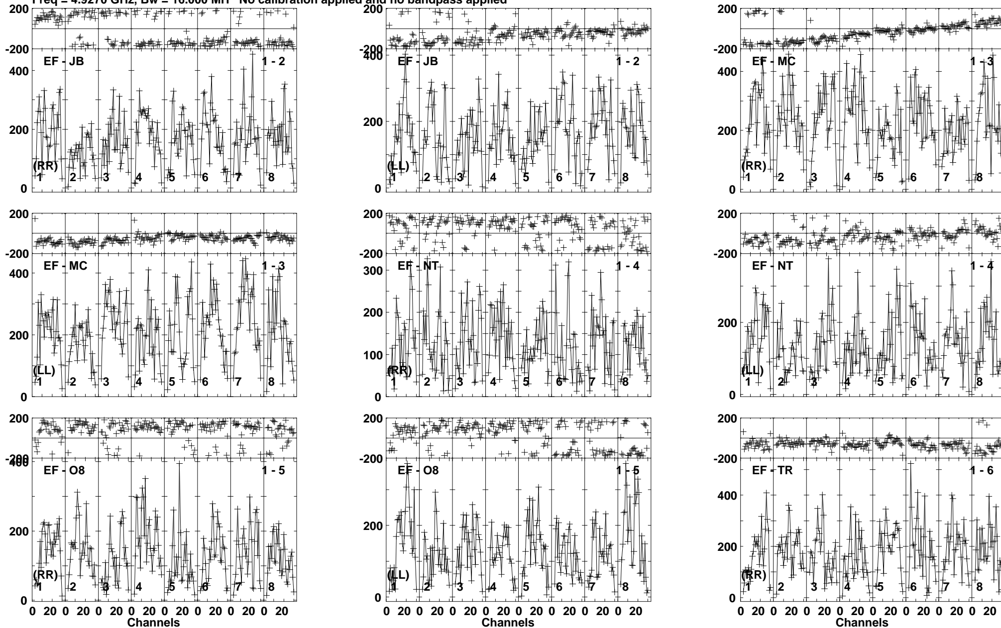
Lower frame: Micro Ampl Jy Top frame: Phas deg Vector averaged cross-power spectrum Baseline: EF (01) - JB (02) Timerange: 01/07:28:40 to 01/07:30:39
