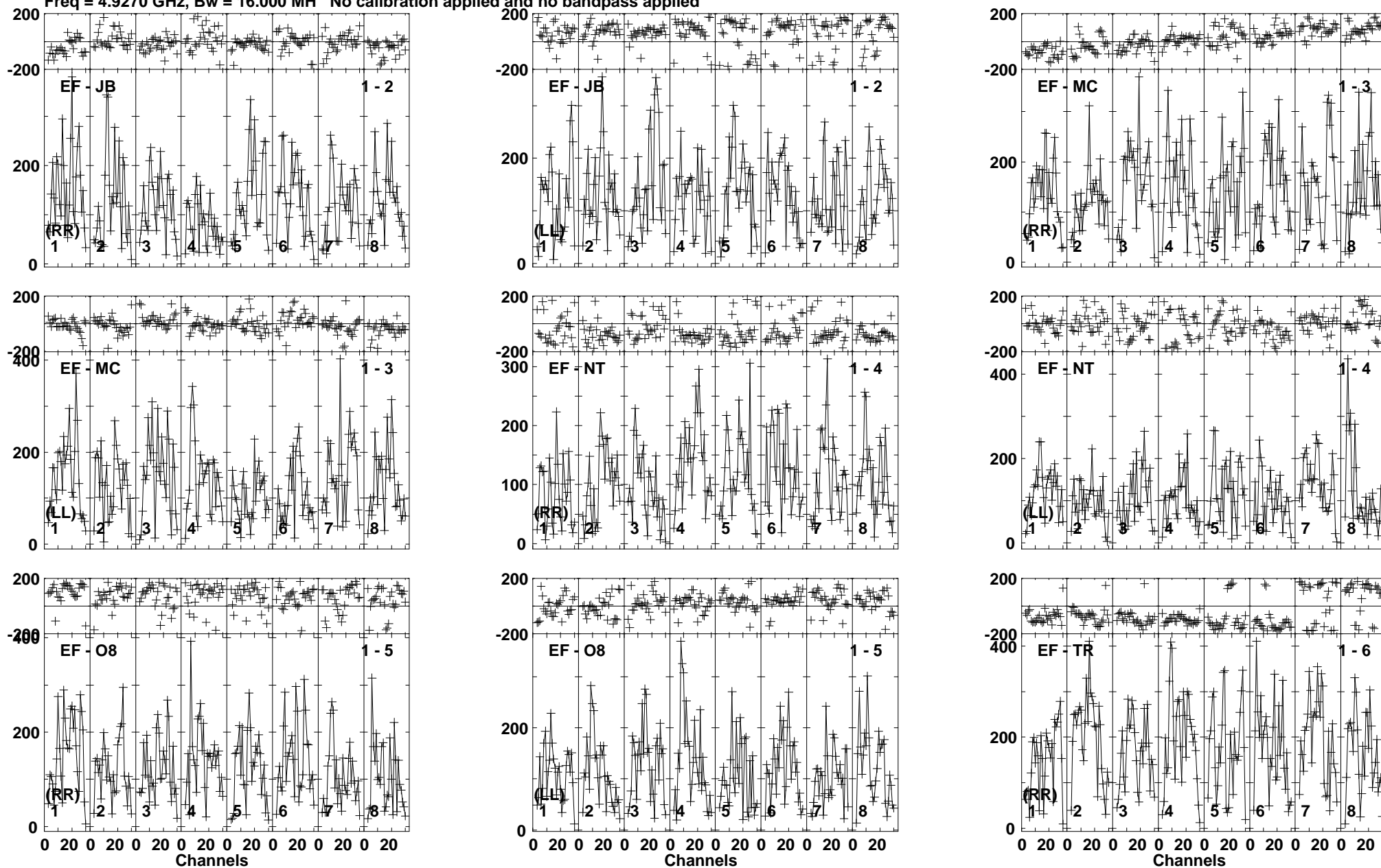
Lower frame: Micro Ampl Jy Top frame: Phas deg Vector averaged cross-power spectrum Baseline: EF (01) - JB (02) Timerange: 01/02:41:20 to 01/02:43:50
