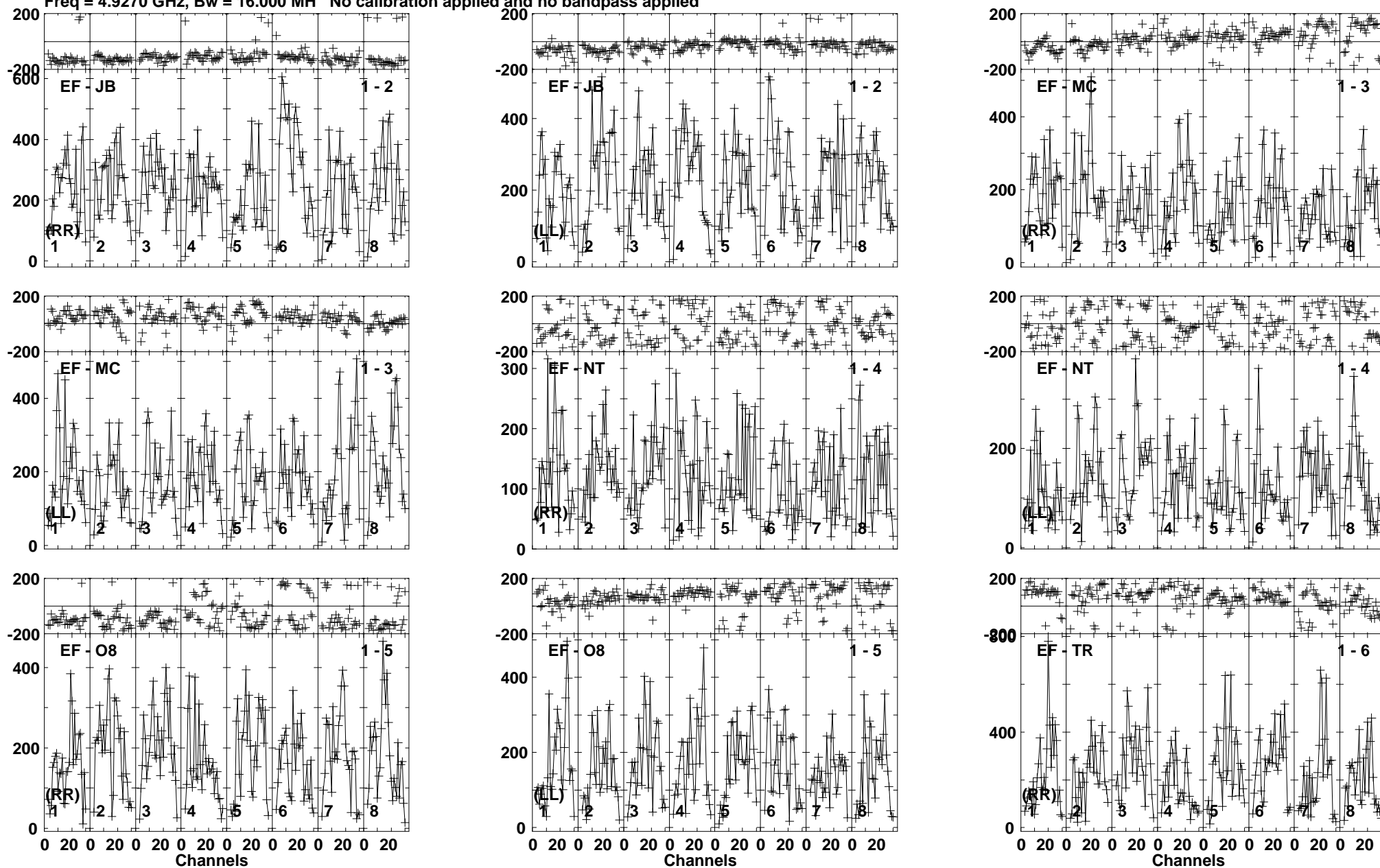
Lower frame: Micro Ampl Jy Top frame: Phas deg Vector averaged cross-power spectrum Baseline: EF (01) - JB (02) Timerange: 01/01:14:30 to 01/01:16:29
