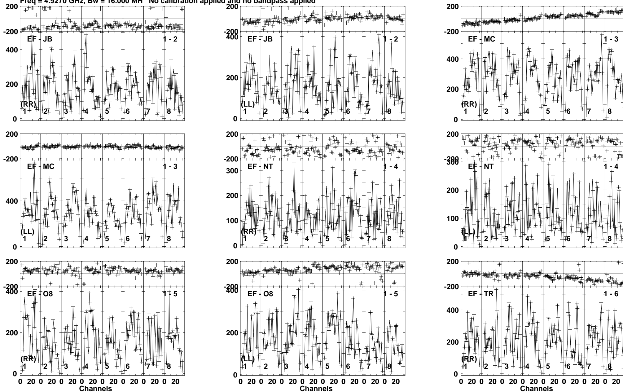
Lower frame: Micro Ampl Jy Top frame: Phas deg Vector averaged cross-power spectrum Baseline: EF (01) - JB (02) Timerange: 01/04:27:20 to 01/04:29:20
