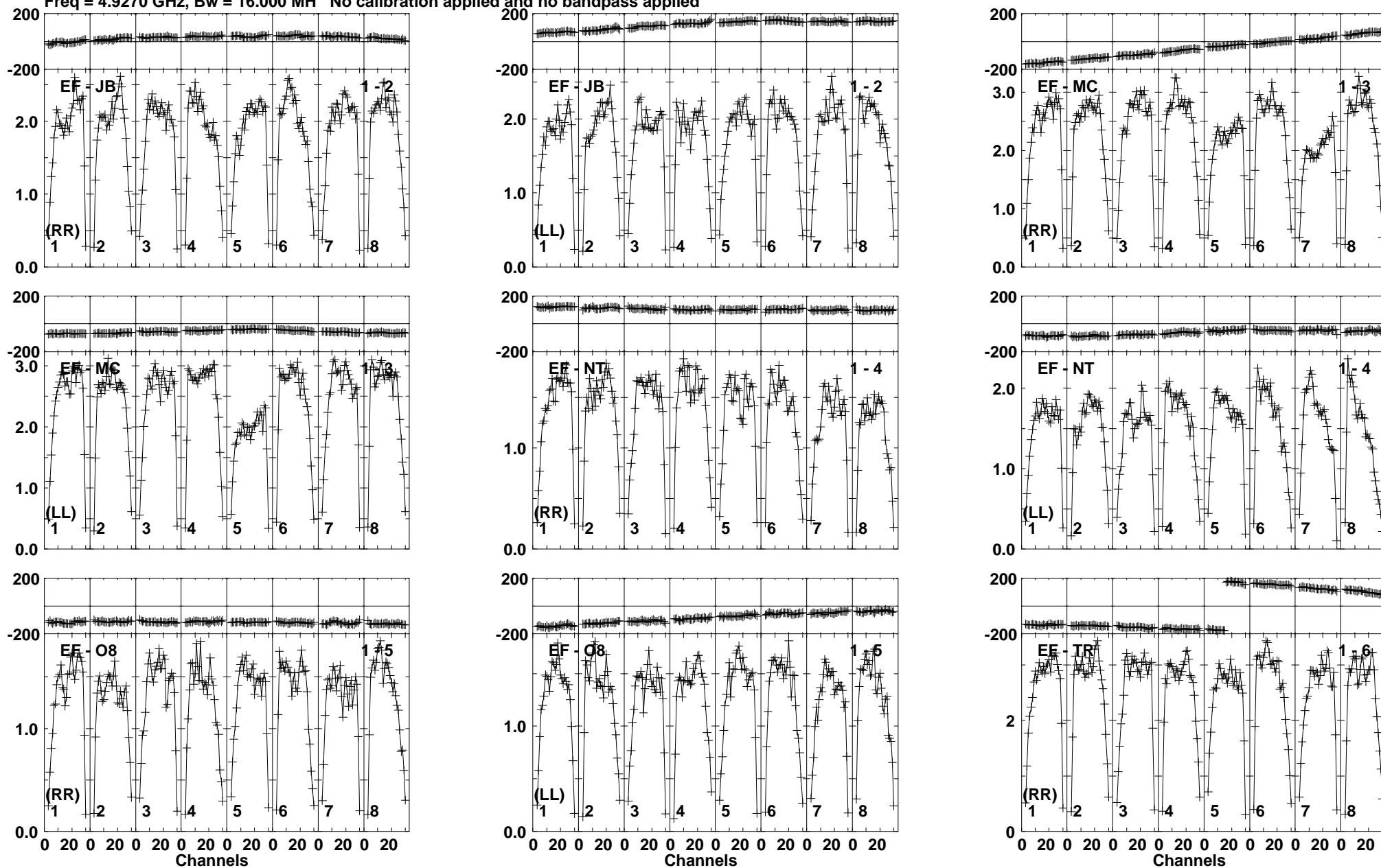
Lower frame: Milli Ampl Jy Top frame: Phas deg Vector averaged cross-power spectrum Baseline: EF (01) - JB (02) Timerange: 01/06:38:31 to 01/06:39:59
