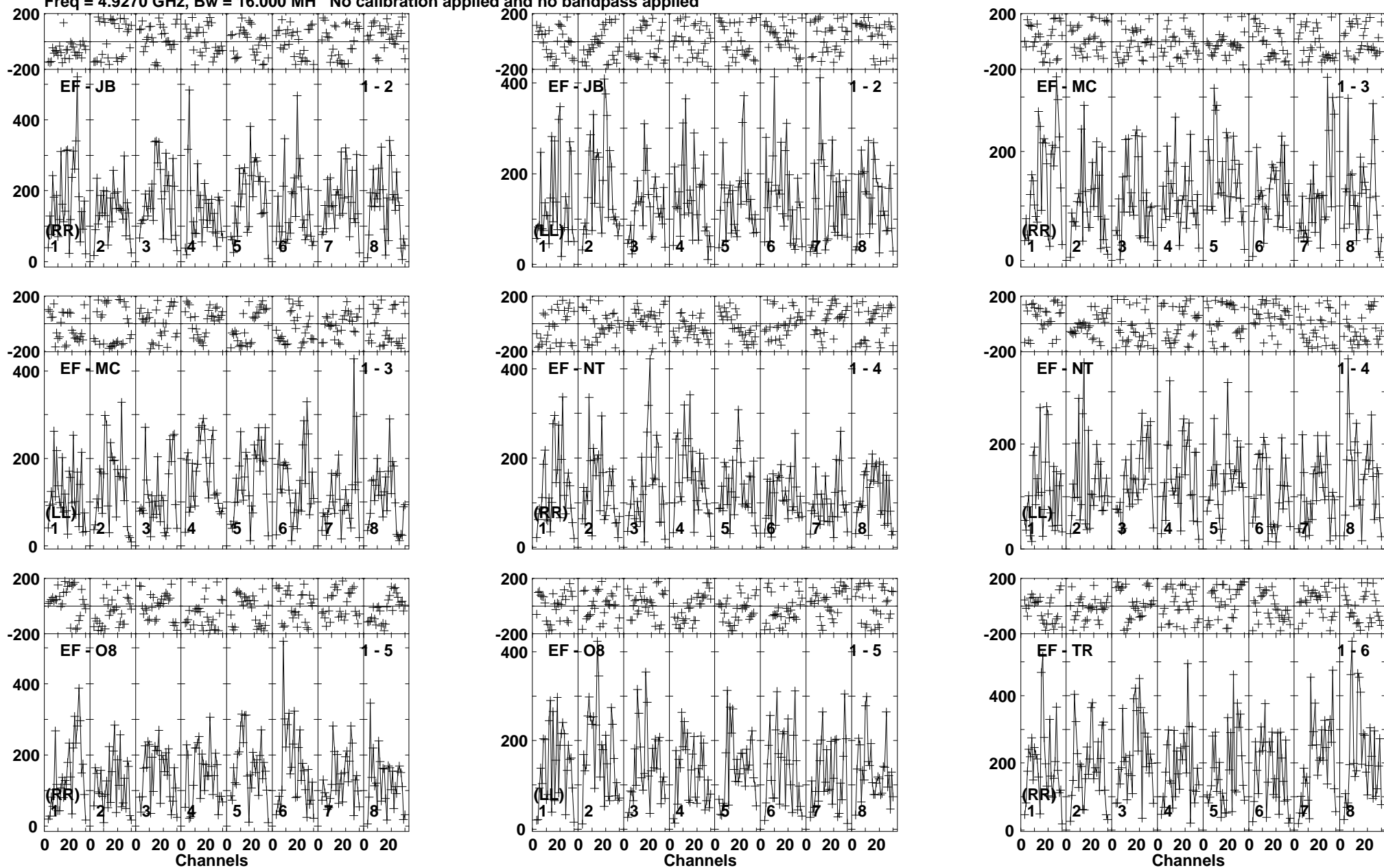
Lower frame: Micro Ampl Jy Top frame: Phas deg Vector averaged cross-power spectrum Baseline: EF (01) - JB (02) Timerange: 01/05:22:31 to 01/05:23:59
