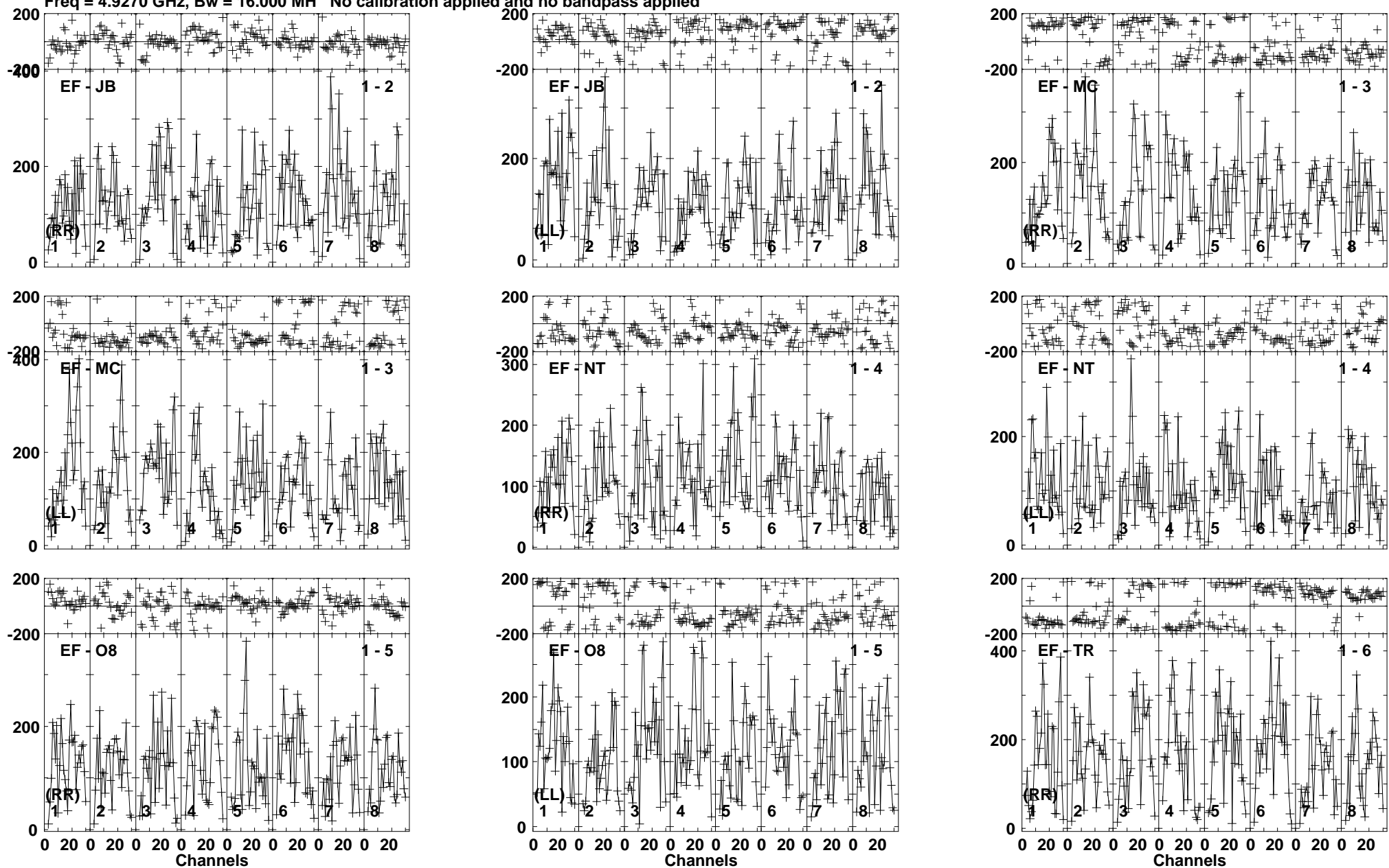
Lower frame: Micro Ampl Jy Top frame: Phas deg Vector averaged cross-power spectrum Baseline: EF (01) - JB (02) Timerange: 01/01:35:50 to 01/01:38:20
