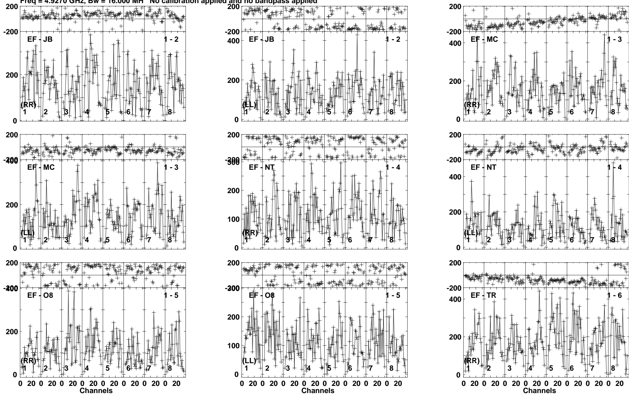
Lower frame: Micro Ampl Jy Top frame: Phas deg Vector averaged cross-power spectrum Baseline: EF (01) - JB (02) Timerange: 01/05:20:01 to 01/05:22:29
