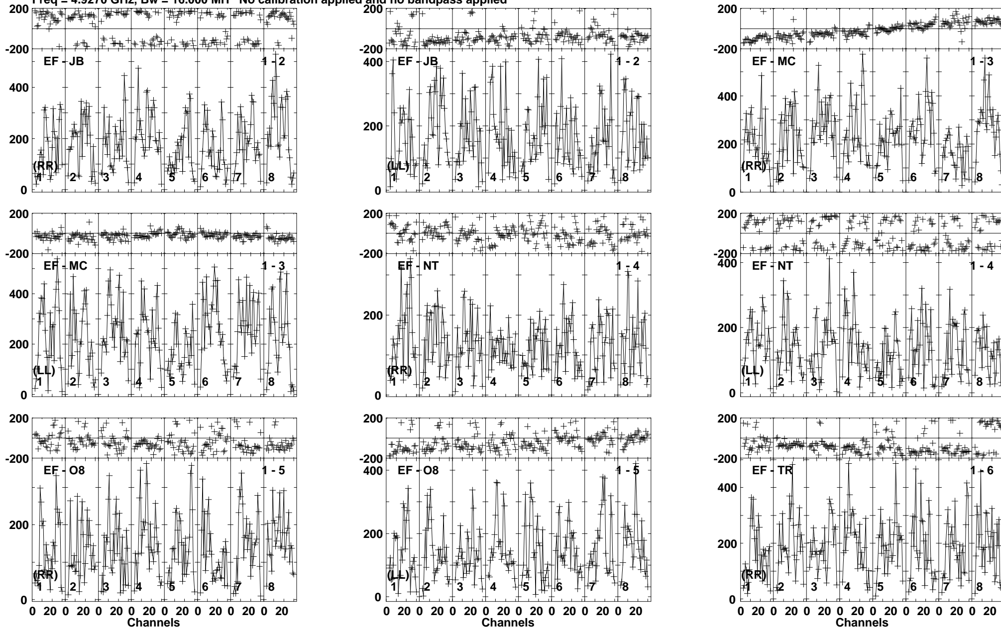
Lower frame: Micro Ampl Jy Top frame: Phas deg Vector averaged cross-power spectrum Baseline: EF (01) - JB (02) Timerange: 01/05:36:40 to 01/05:38:40
