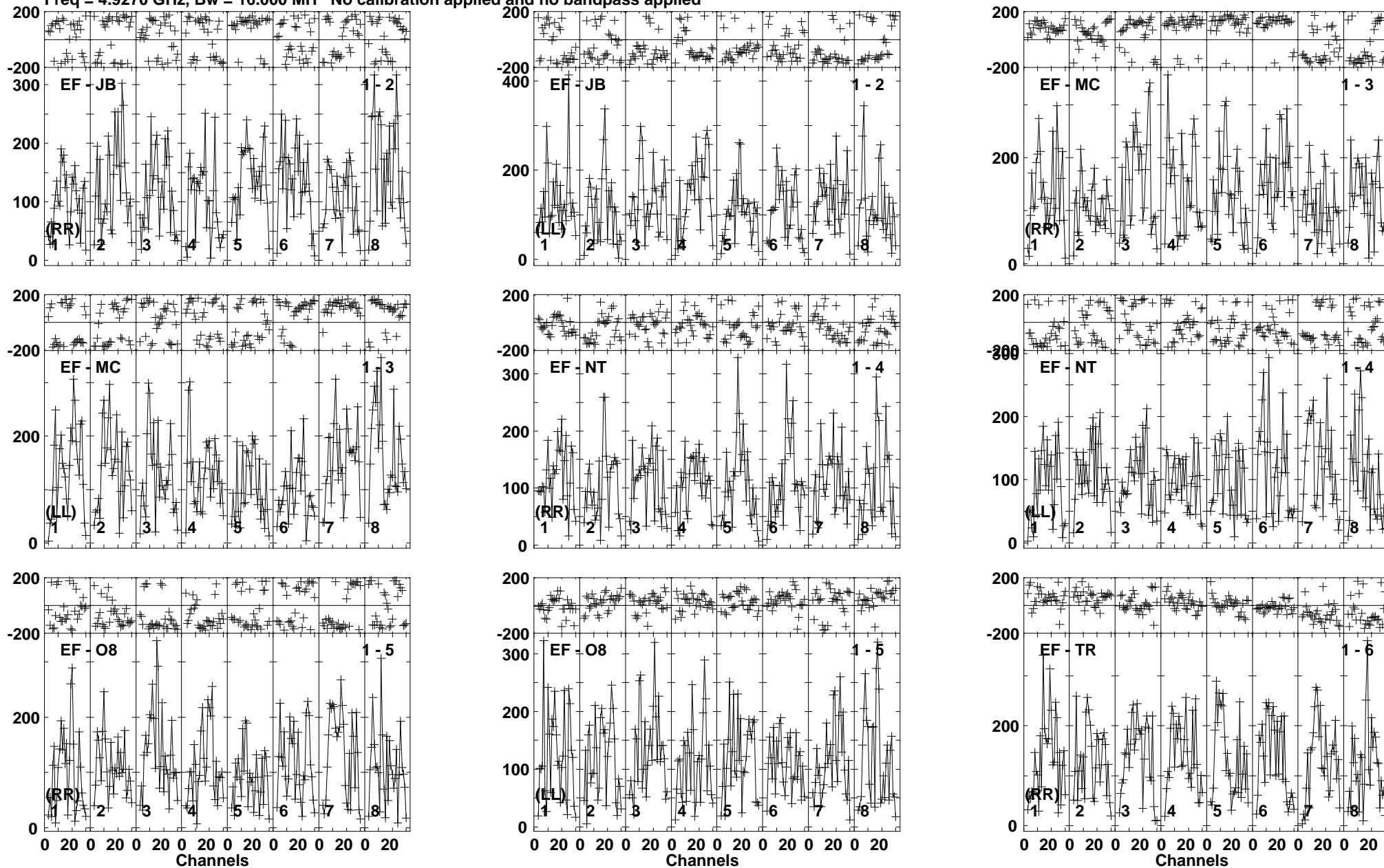
Lower frame: Micro Ampl Jy Top frame: Phas deg Vector averaged cross-power spectrum Baseline: EF (01) - JB (02) Timerange: 00/21:35:11 to 00/21:37:39
