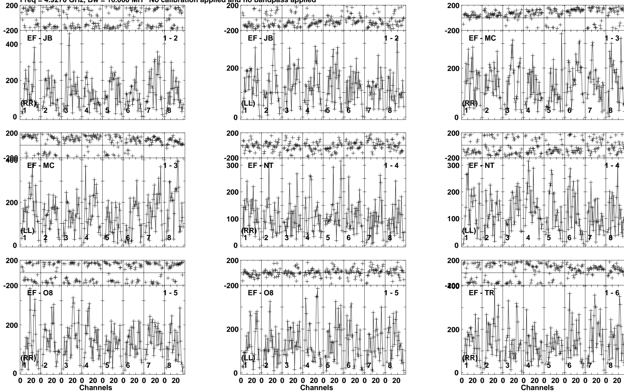
Lower frame: Micro Ampl Jy Top frame: Phas deg Vector averaged cross-power spectrum Baseline: EF (01) - JB (02) Timerange: 00:22:38:31 to 00:22:40:59
