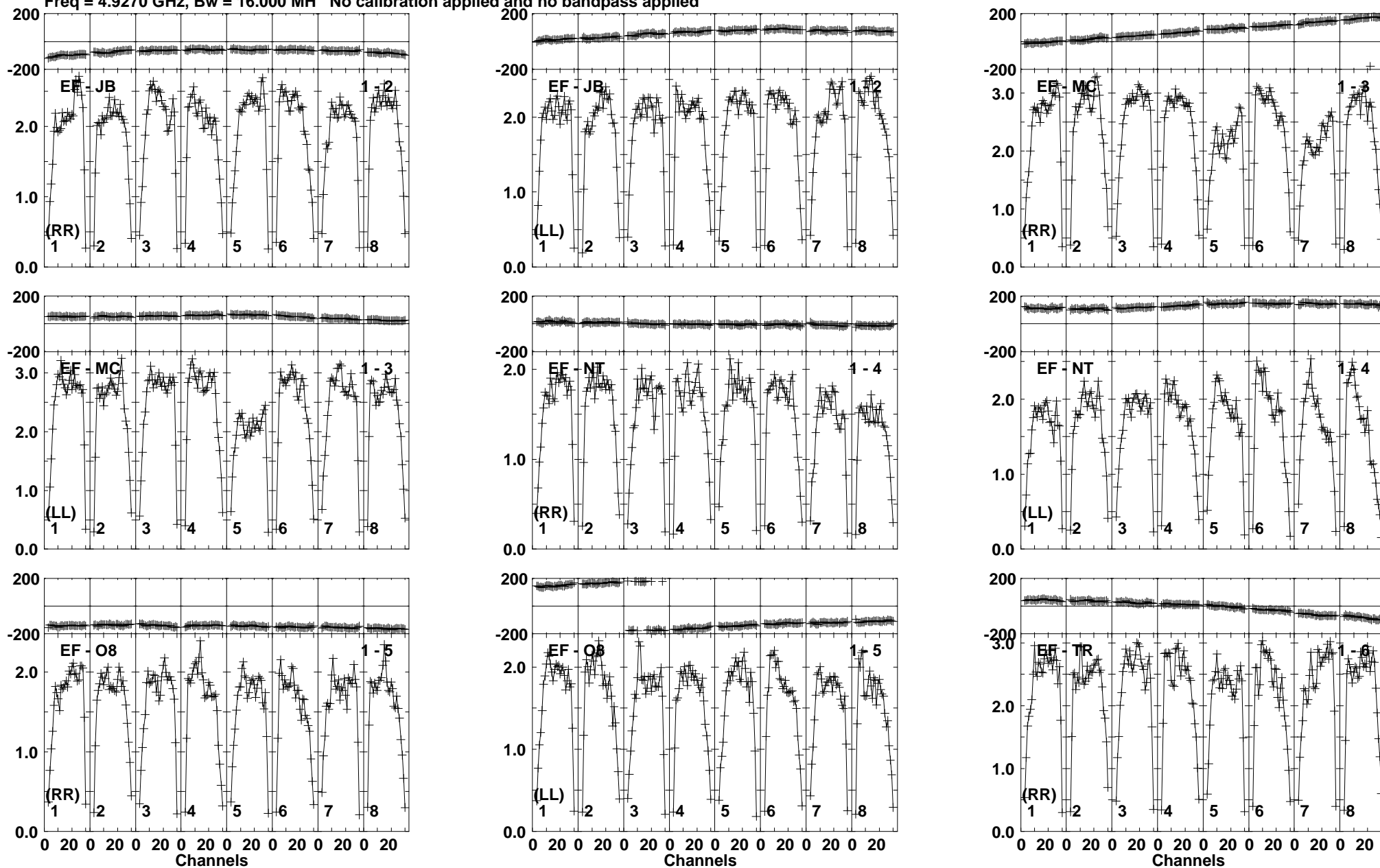
Lower frame: Milli Ampl Jy Top frame: Phas deg Vector averaged cross-power spectrum Baseline: EF (01) - JB (02) Timerange: 01/03:34:31 to 01/03:35:59
