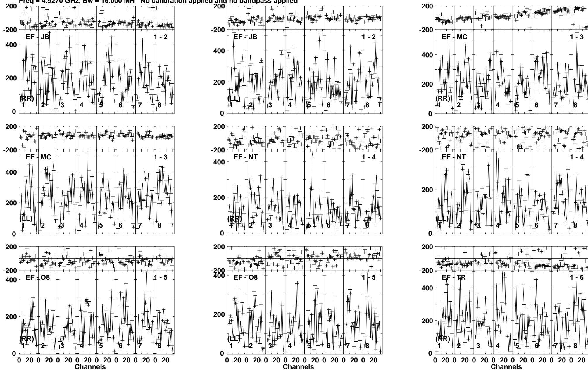
Lower frame: Micro Ampl Jy Top frame: Phas deg Vector averaged cross-power spectrum Baseline: EF (01) - JB (02) Timerange: 01/05:49:21 to 01/05:51:19
