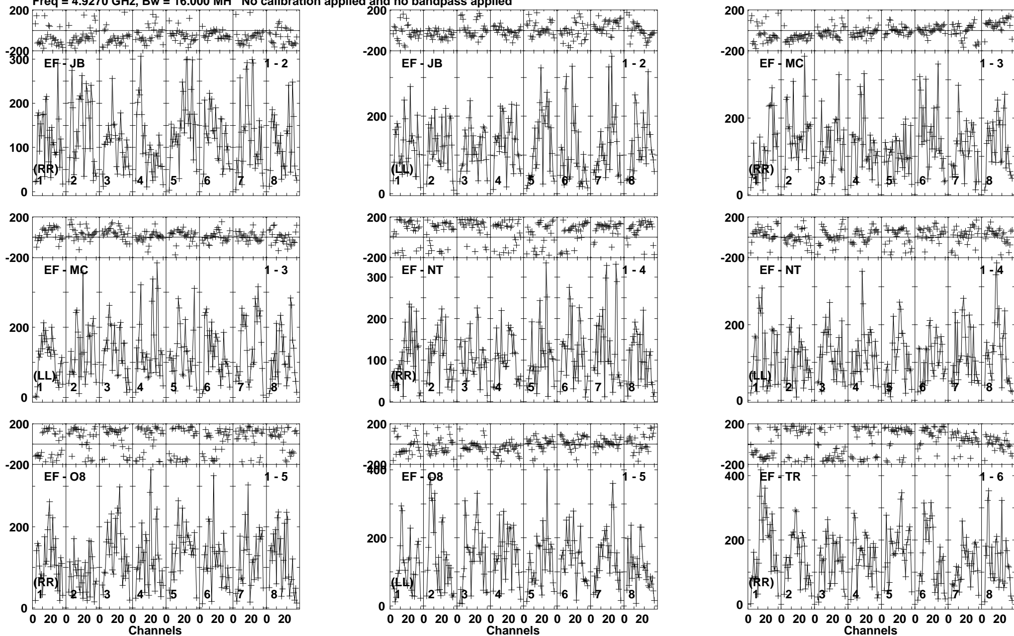
Lower frame: Micro Ampl Jy Top frame: Phas deg Vector averaged cross-power spectrum Baseline: EF (01) - JB (02) Timerange: 00/23:29:11 to 00/23:31:40
