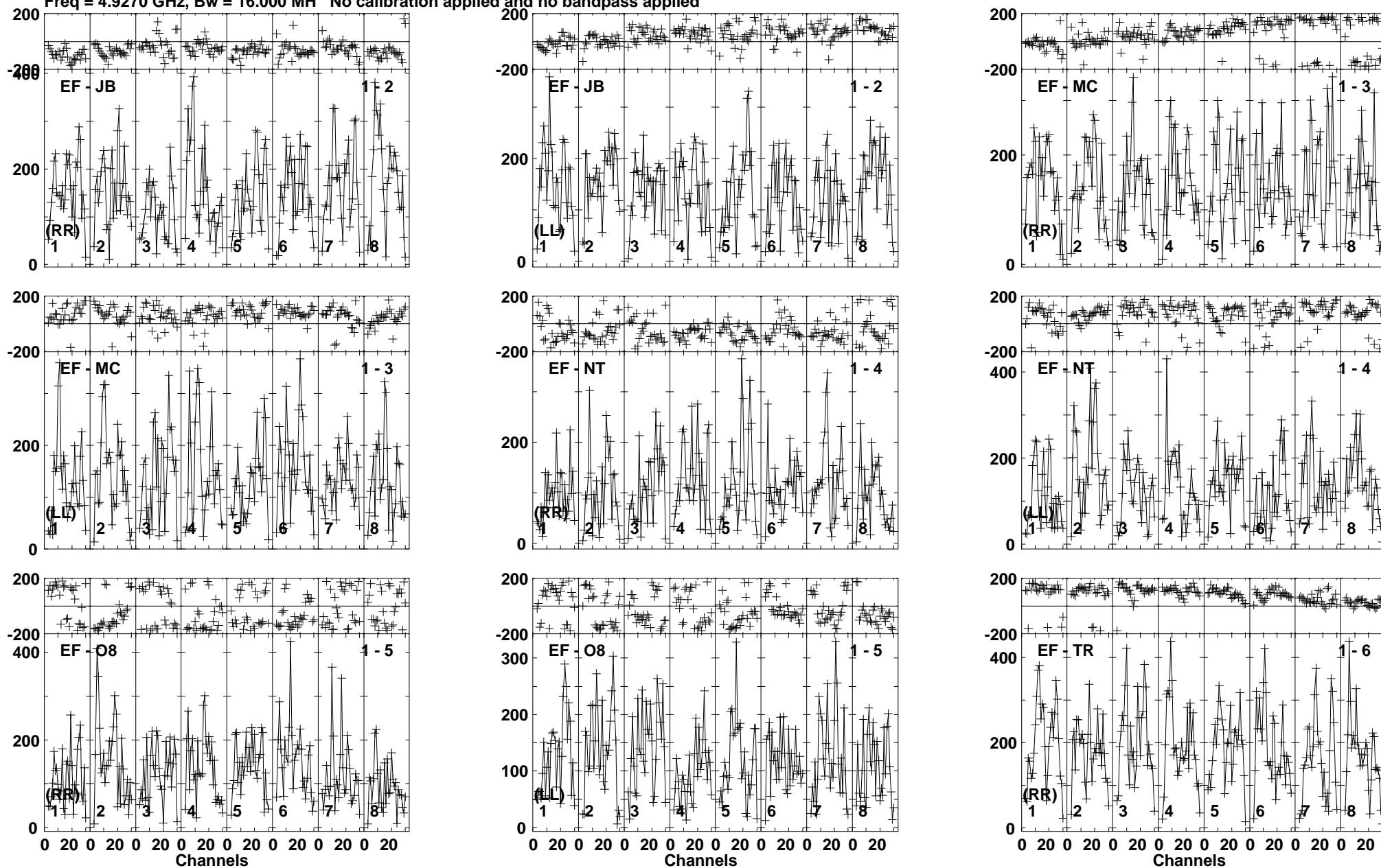
Lower frame: Micro Ampl Jy Top frame: Phas deg Vector averaged cross-power spectrum Baseline: EF (01) - JB (02) Timerange: 01/04:42:01 to 01/04:44:29
