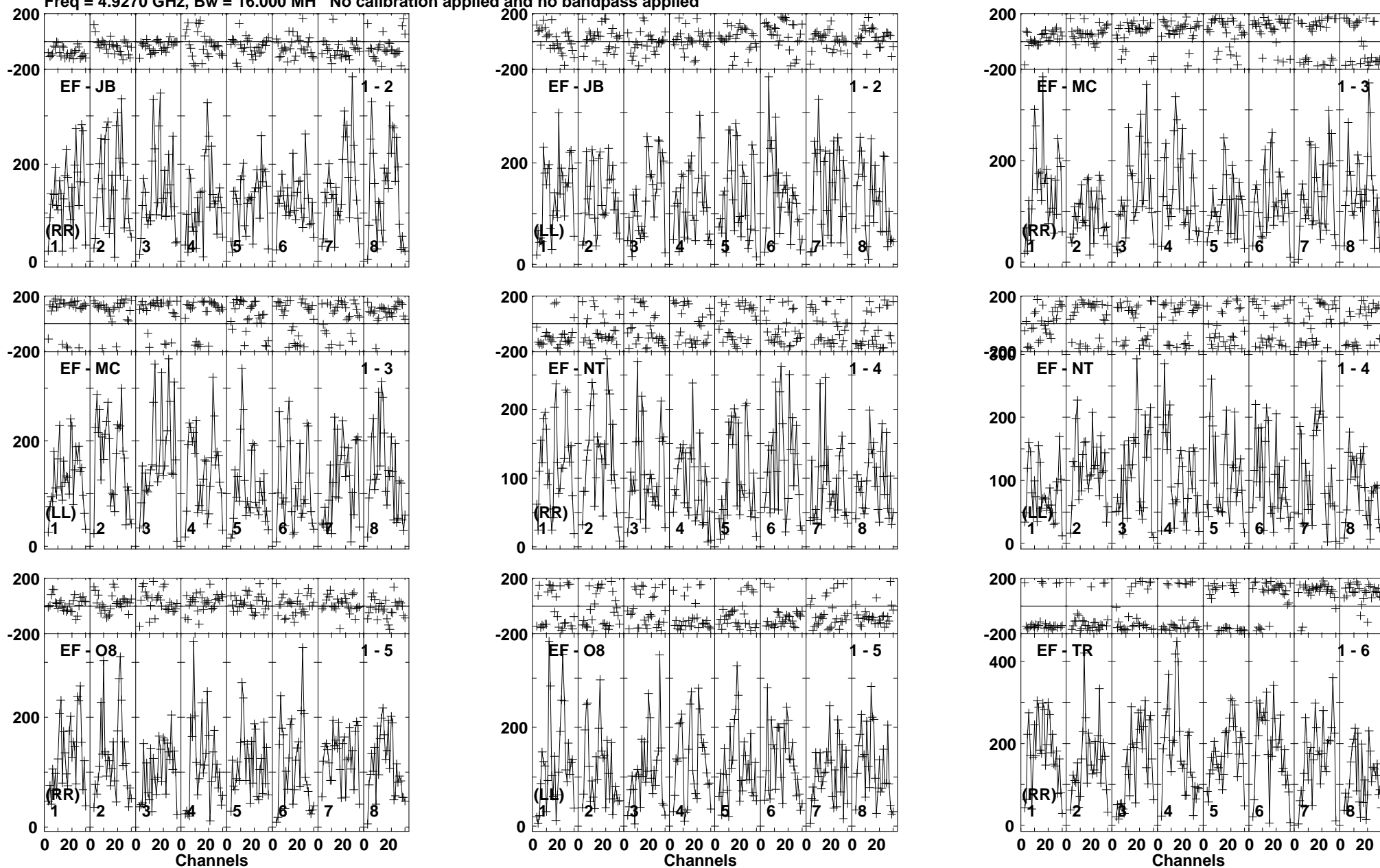
Lower frame: Micro Ampl Jy Top frame: Phas deg Vector averaged cross-power spectrum Baseline: EF (01) - JB (02) Timerange: 01/01:23:11 to 01/01:25:40
