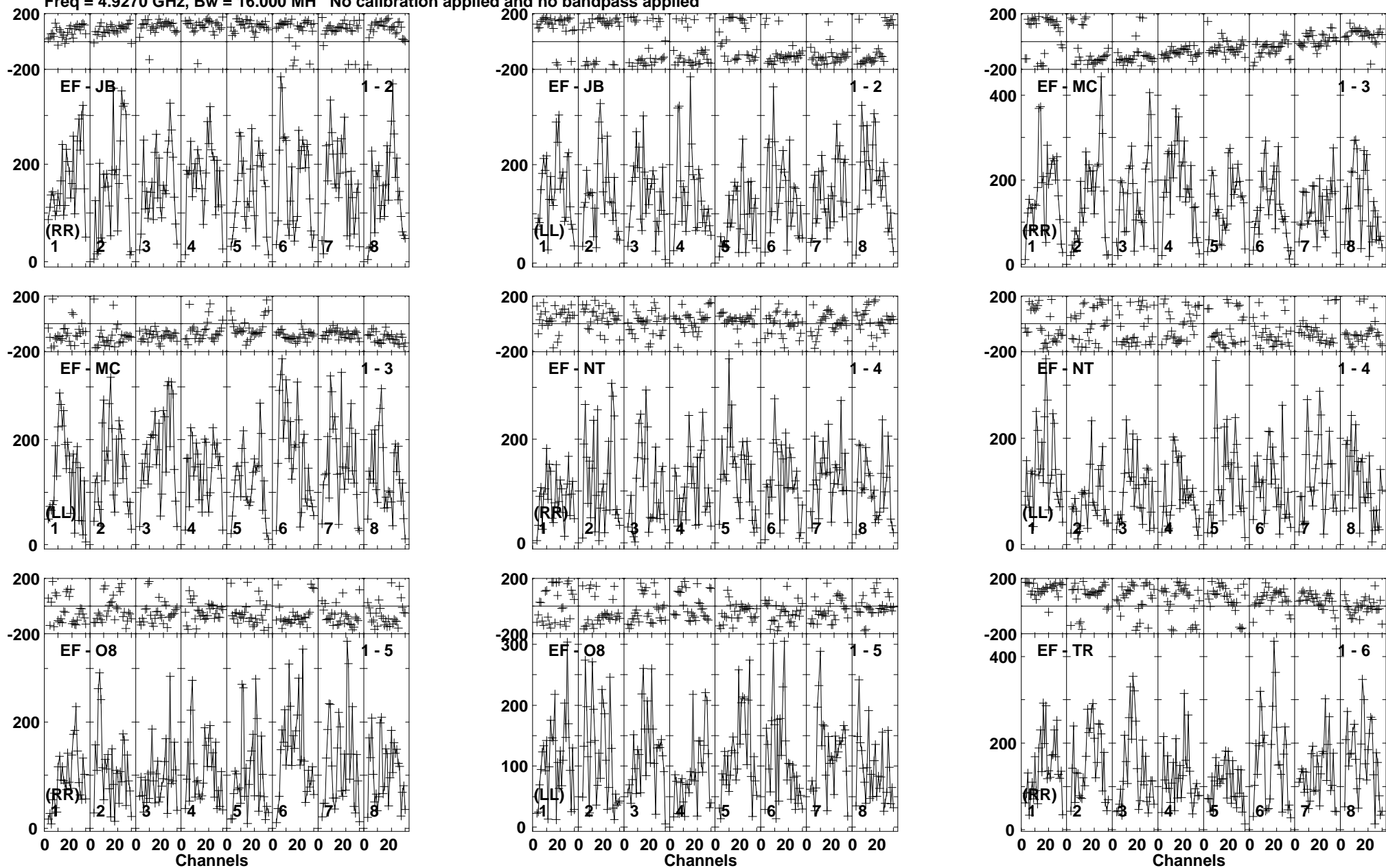
Lower frame: Micro Ampl Jy Top frame: Phas deg Vector averaged cross-power spectrum Baseline: EF (01) - JB (02) Timerange: 01/07:58:00 to 01/08:00:30
