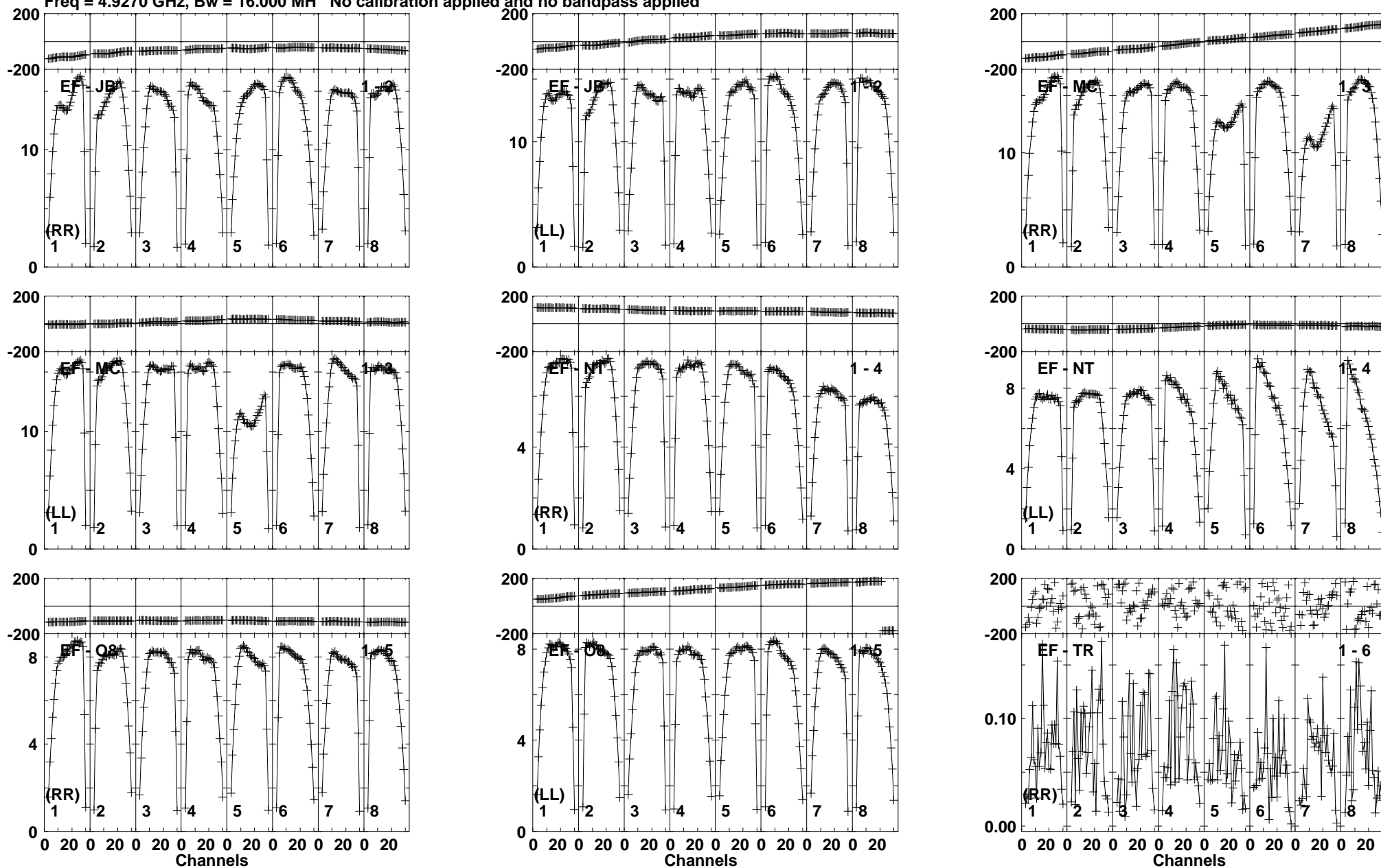
Lower frame: Milli Ampl Jy Top frame: Phas deg Vector averaged cross-power spectrum Baseline: EF (01) - JB (02) Timerange: 01/09:45:00 to 01/09:59:19
