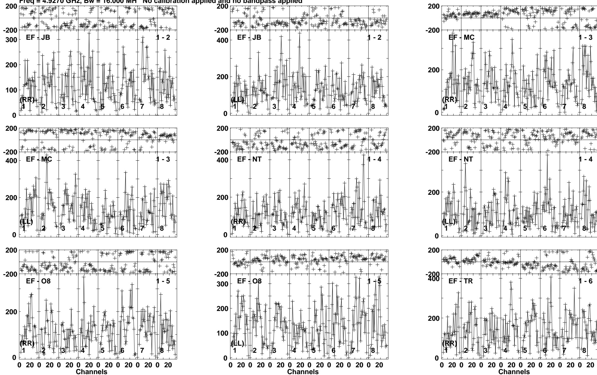
Lower frame: Micro Ampl Jy Top frame: Phas deg Vector averaged cross-power spectrum Baseline: EF (01) - JB (02) Timerange: 00/21:15:51 to 00/21:18:19
