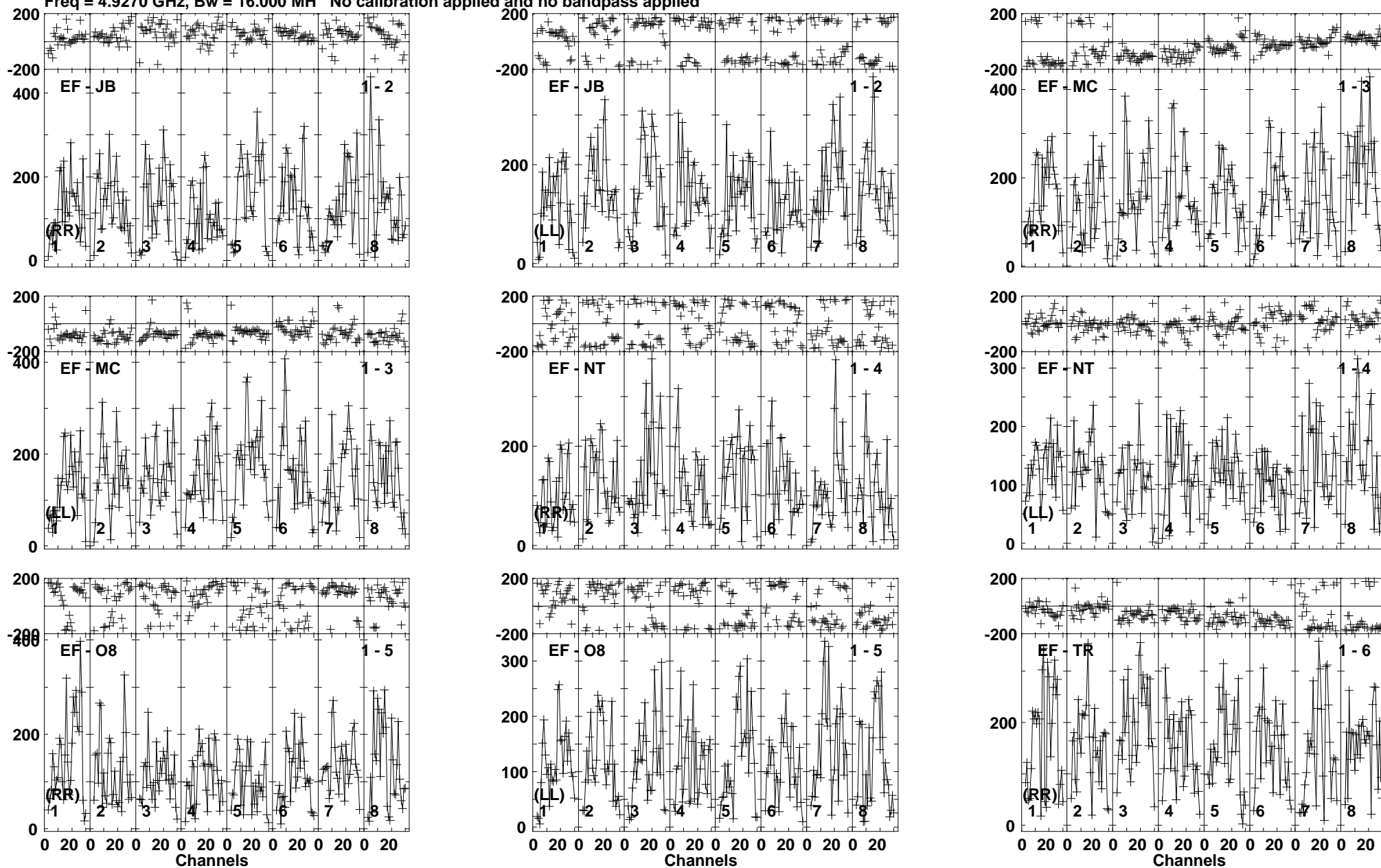
Lower frame: Micro Ampl Jy Top frame: Phas deg Vector averaged cross-power spectrum Baseline: EF (01) - JB (02) Timerange: 01/05:13:21 to 01/05:15:50
