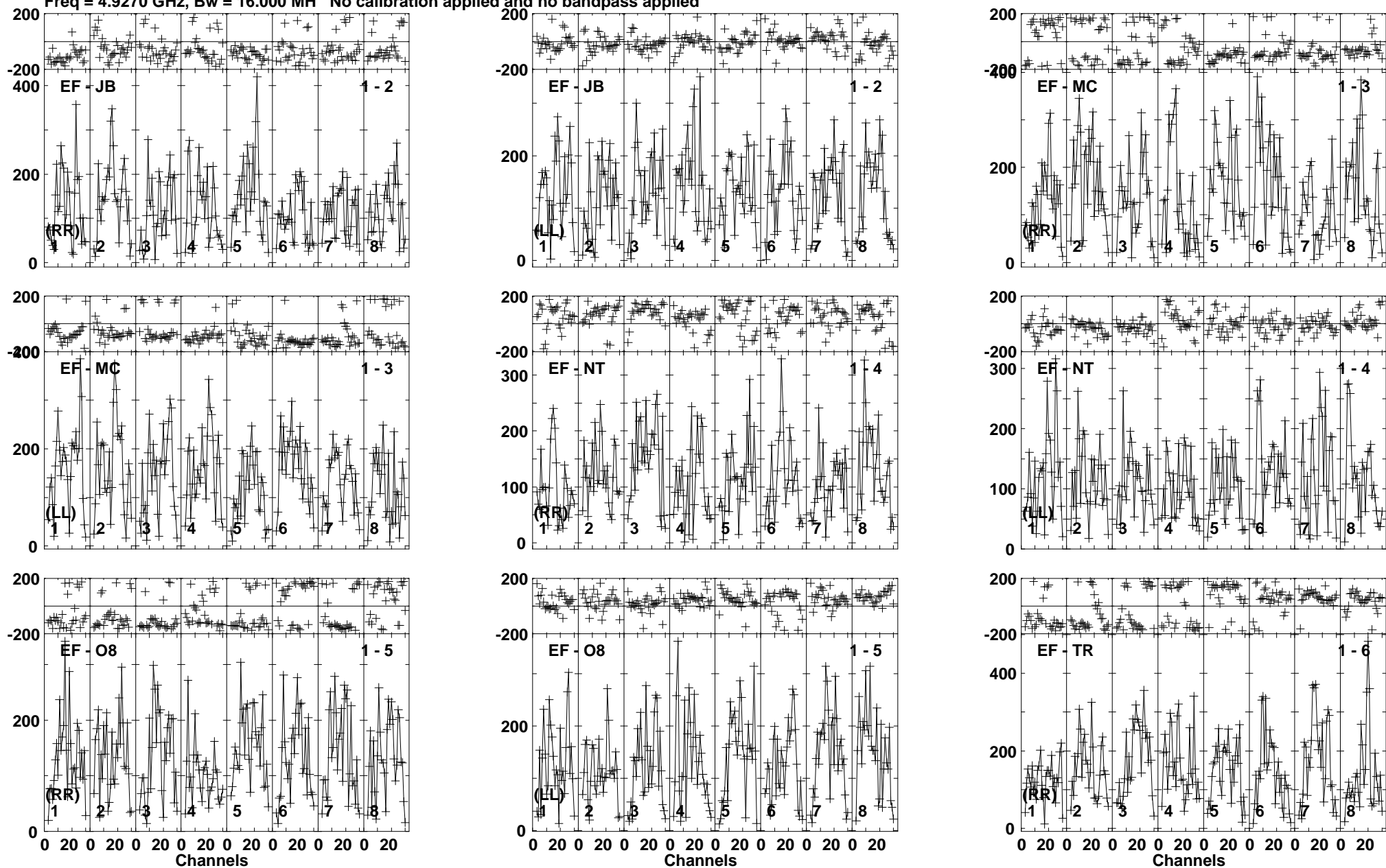
Lower frame: Micro Ampl Jy Top frame: Phas deg Vector averaged cross-power spectrum Baseline: EF (01) - JB (02) Timerange: 00/23:03:51 to 00/23:06:19
