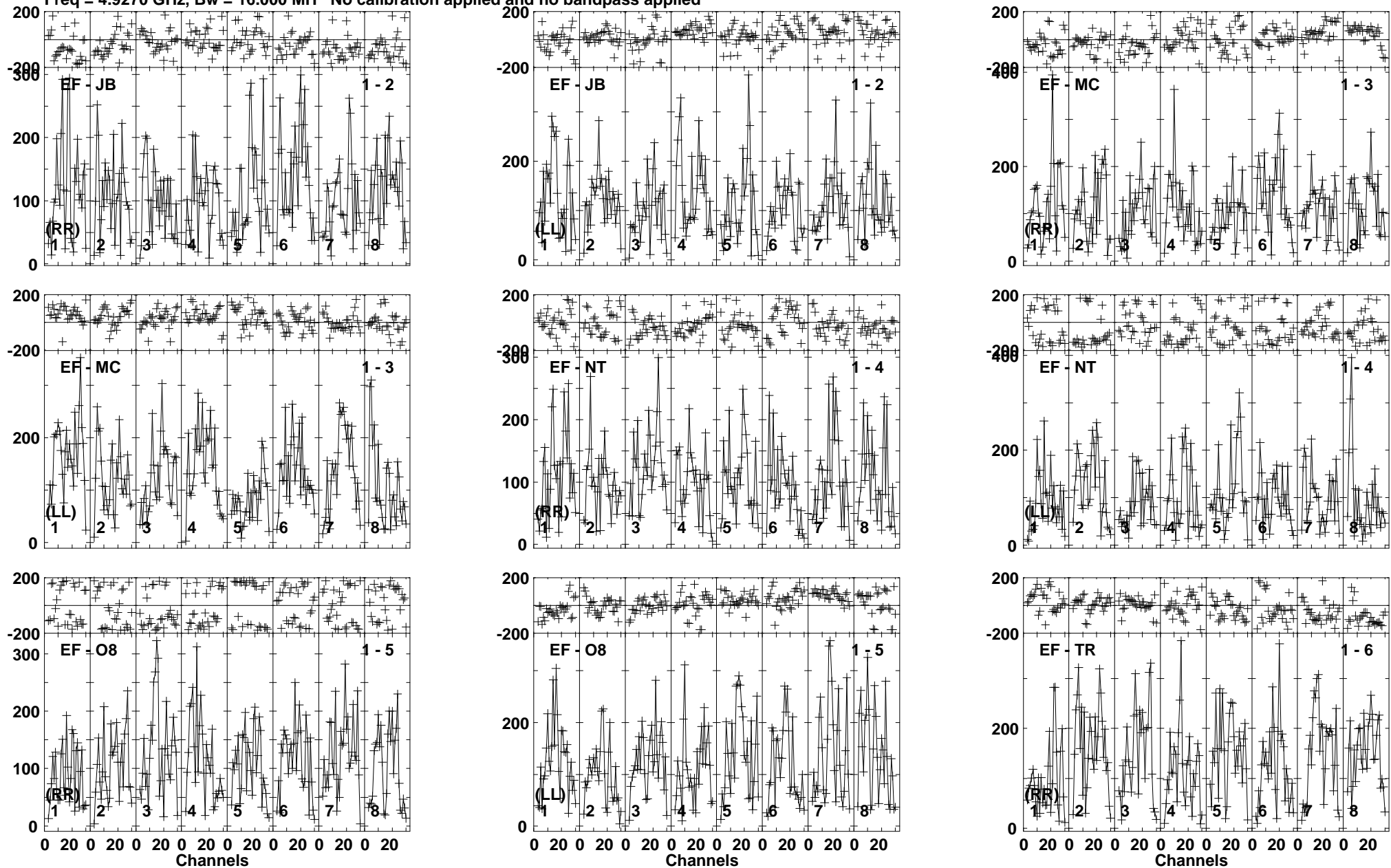
Lower frame: Micro Ampl Jy Top frame: Phas deg Vector averaged cross-power spectrum Baseline: EF (01) - JB (02) Timerange: 01/00:25:51 to 01/00:28:19
