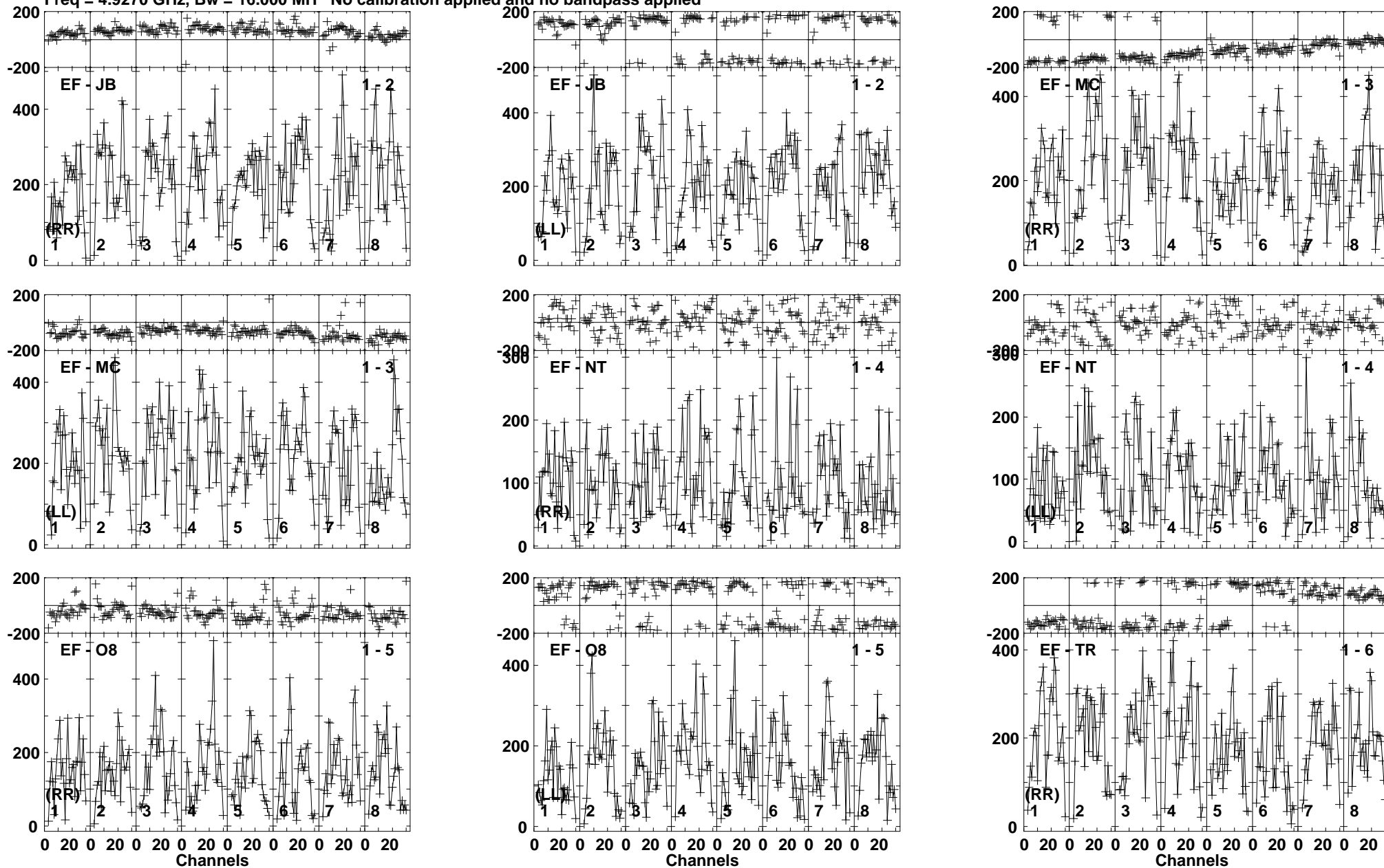
Lower frame: Micro Ampl Jy Top frame: Phas deg Vector averaged cross-power spectrum Baseline: EF (01) - JB (02) Timerange: 01/01:46:30 to 01/01:48:30
