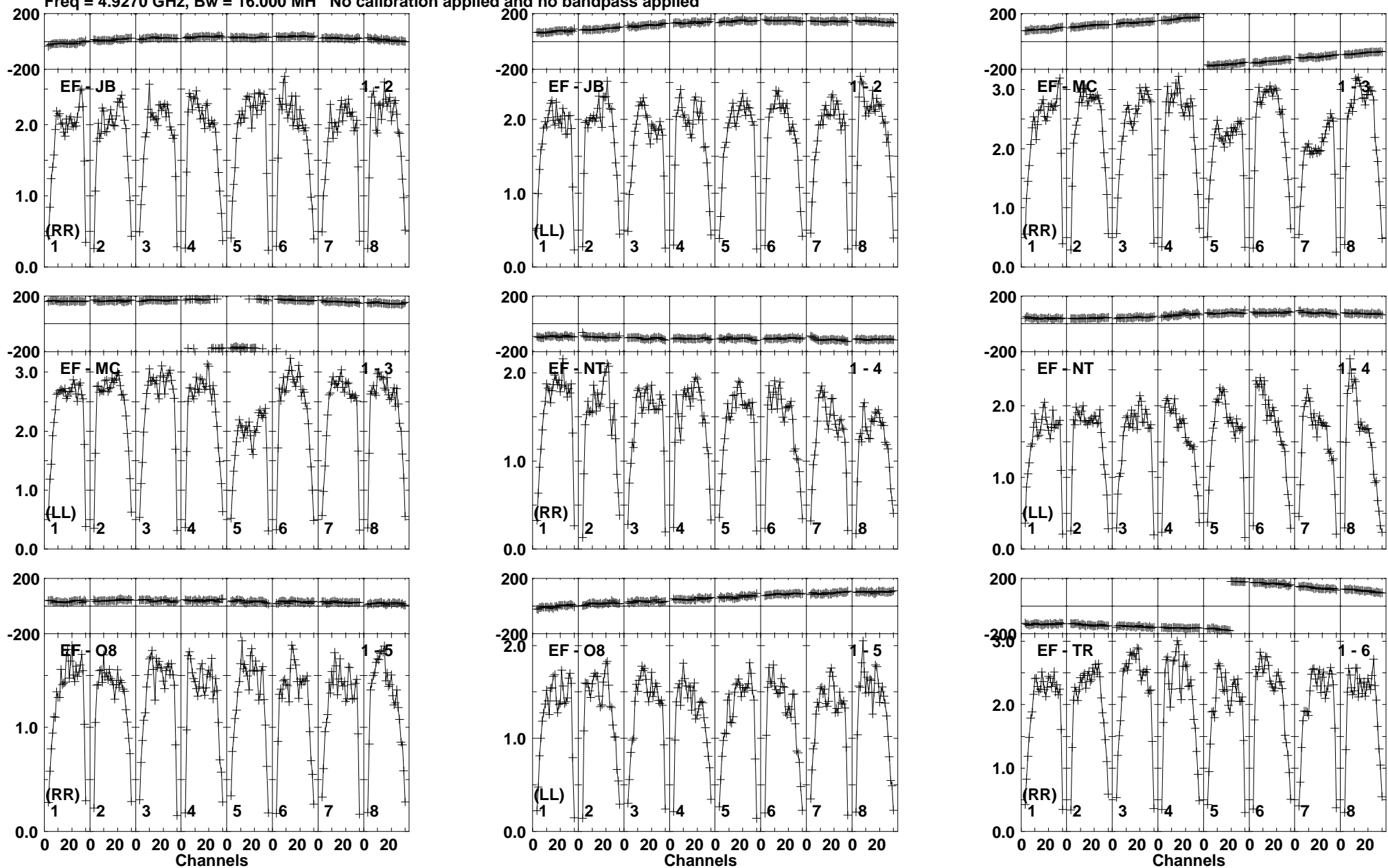
Lower frame: Milli Ampl Jy Top frame: Phas deg Vector averaged cross-power spectrum Baseline: EF (01) - JB (02) Timerange: 01/05:03:10 to 01/05:04:39
