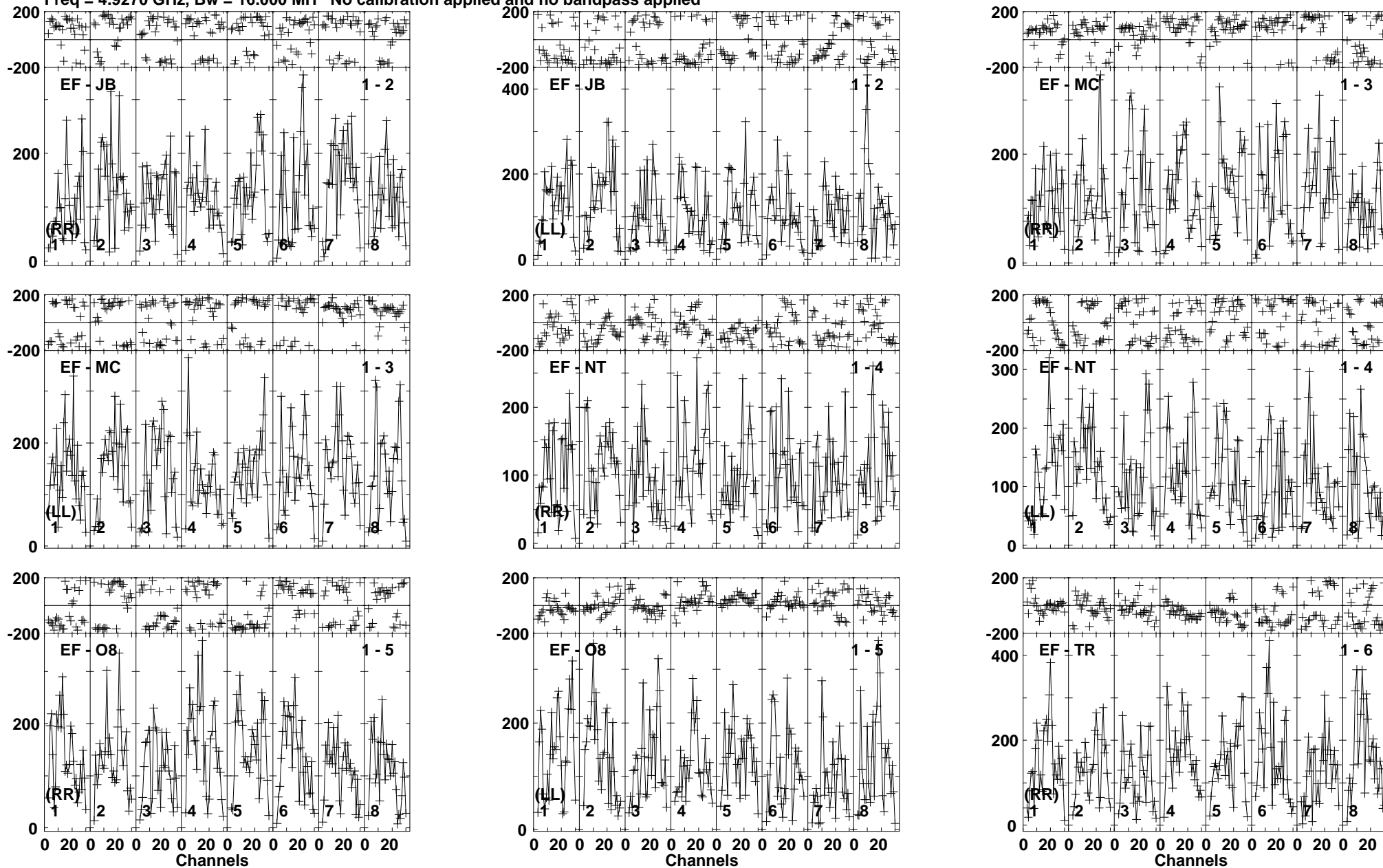
Lower frame: Micro Ampl Jy Top frame: Phas deg Vector averaged cross-power spectrum Baseline: EF (01) - JB (02) Timerange: 00/21:22:31 to 00/21:24:59
