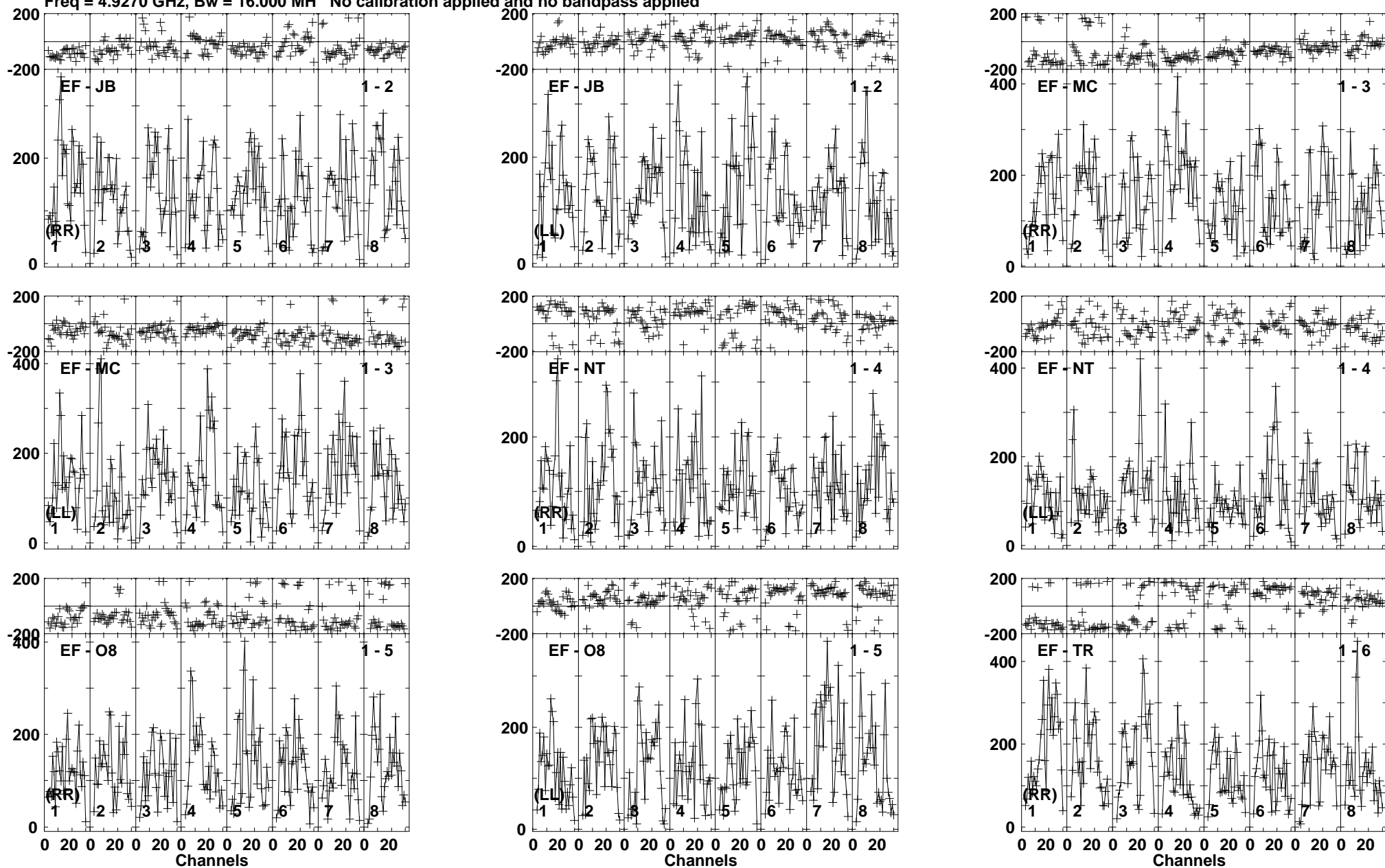
Lower frame: Micro Ampl Jy Top frame: Phas deg Vector averaged cross-power spectrum Baseline: EF (01) - JB (02) Timerange: 00/23:09:51 to 00/23:12:20
