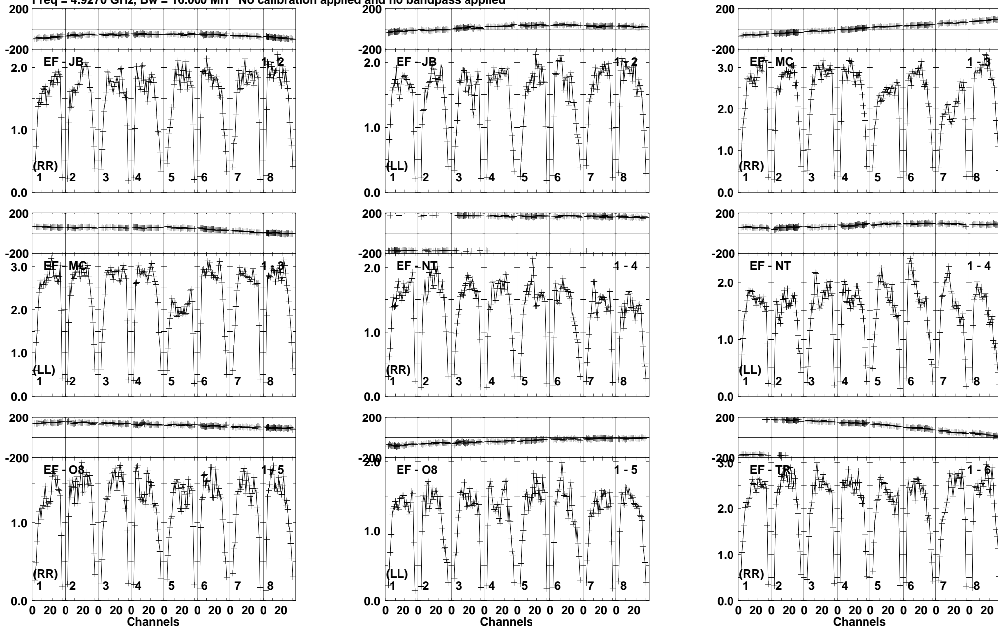
Lower frame: Milli Ampl Jy Top frame: Phas deg Vector averaged cross-power spectrum Baseline: EF (01) - JB (02) Timerange: 00/23:31:40 to 00/23:33:10
