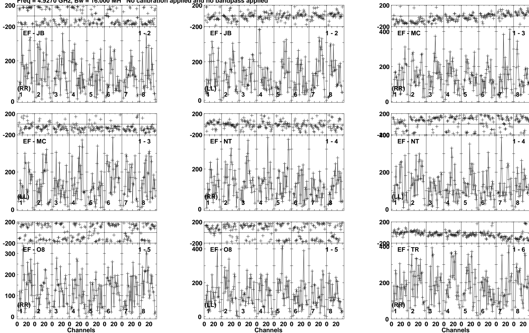
Lower frame: Micro Ampl Jy Top frame: Phas deg Vector averaged cross-power spectrum Baseline: EF (01) - JB (02) Timerange: 01/03:19:20 to 01/03:21:50
