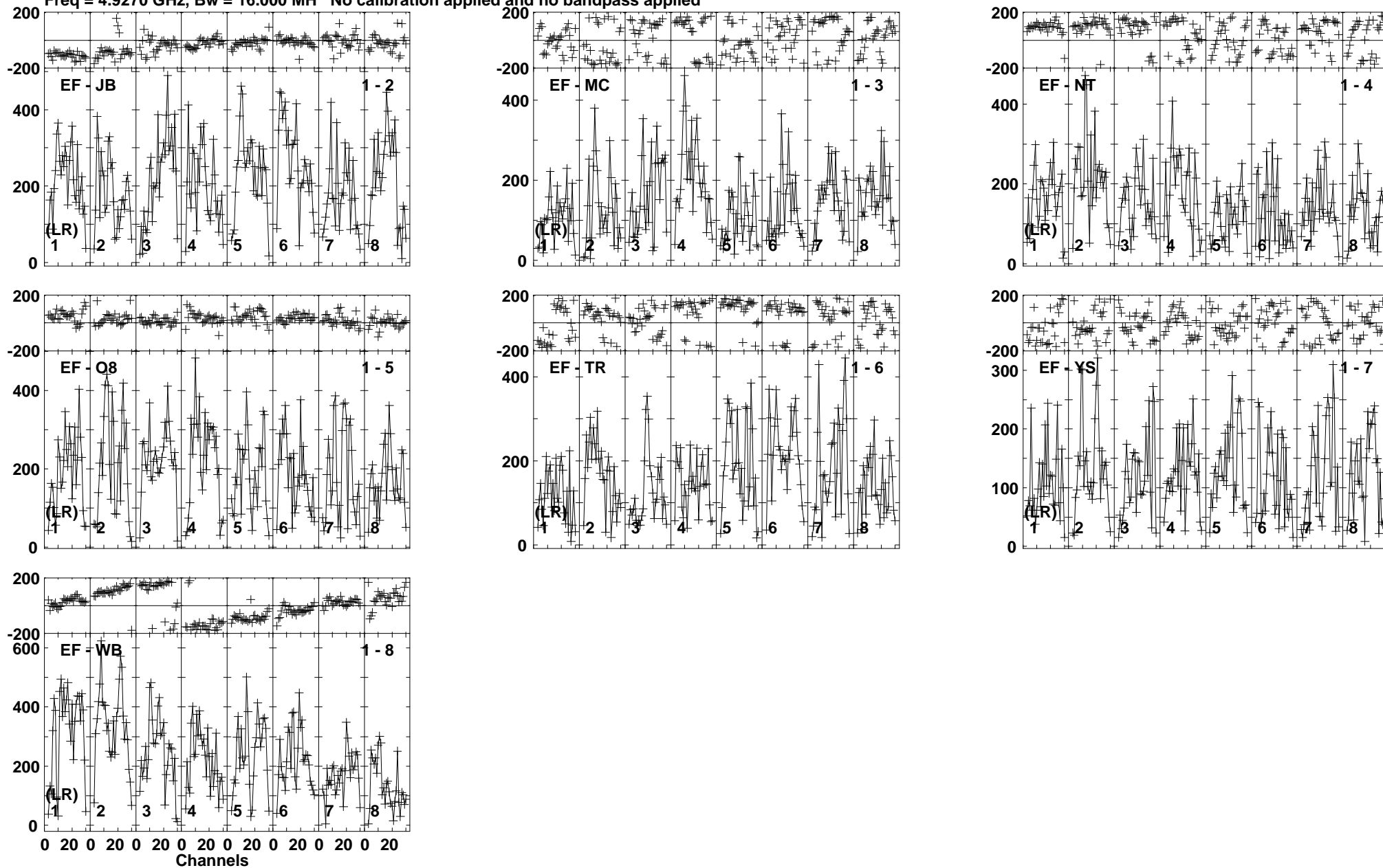
Lower frame: Micro Ampl Jy Top frame: Phas deg Vector averaged cross-power spectrum Baseline: EF (01) - JB (02) Timerange: 01/07:18:30 to 01/07:19:59
