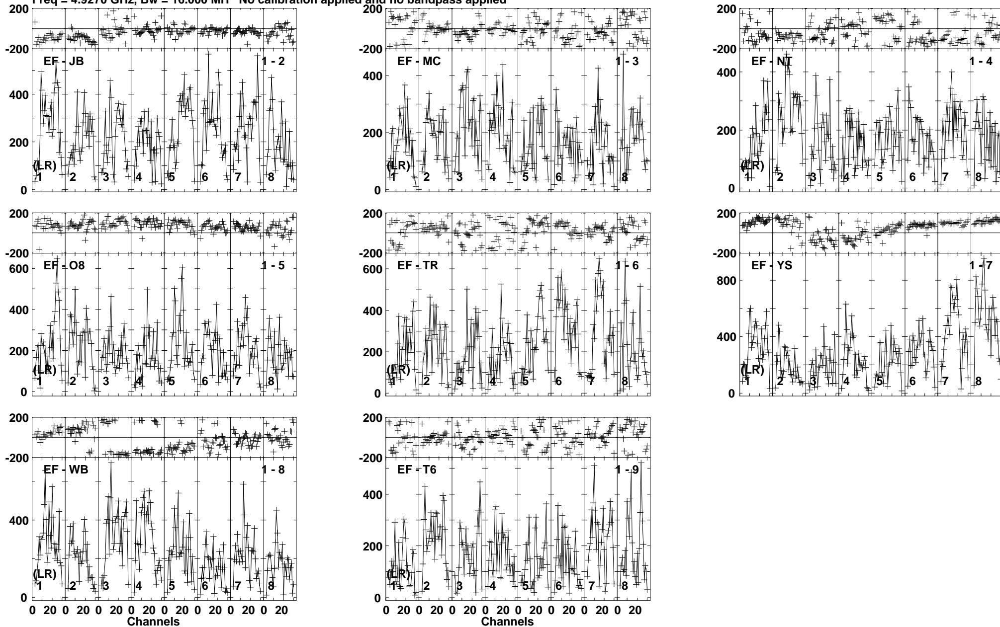
Lower frame: Micro Ampl Jy Top frame: Phas deg Vector averaged cross-power spectrum Baseline: EF (01) - JB (02) Timerange: 00:22:25:00 to 00:22:26:30
