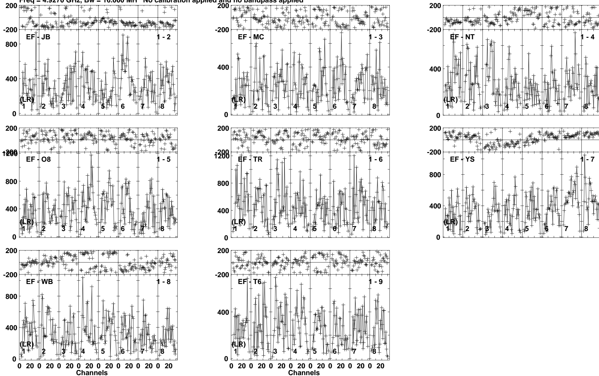
Lower frame: Micro Ampl Jy Top frame: Phas deg Vector averaged cross-power spectrum Baseline: EF (01) - JB (02) Timerange: 00/22:19:01 to 00/22:20:30
