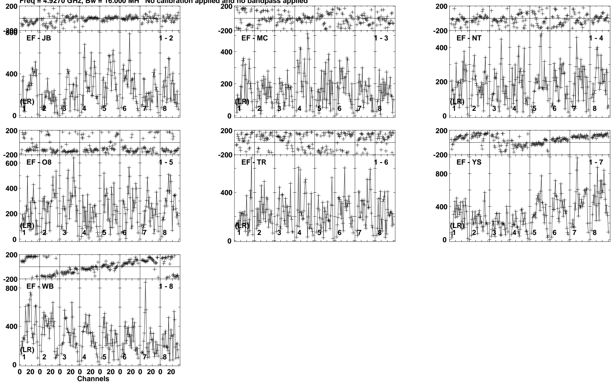
Lower frame: Micro Ampl Jy Top frame: Phas deg Vector averaged cross-power spectrum Baseline: EF (01) - JB (02) Timerange: 01/05:02:41 to 01/05:04:09
