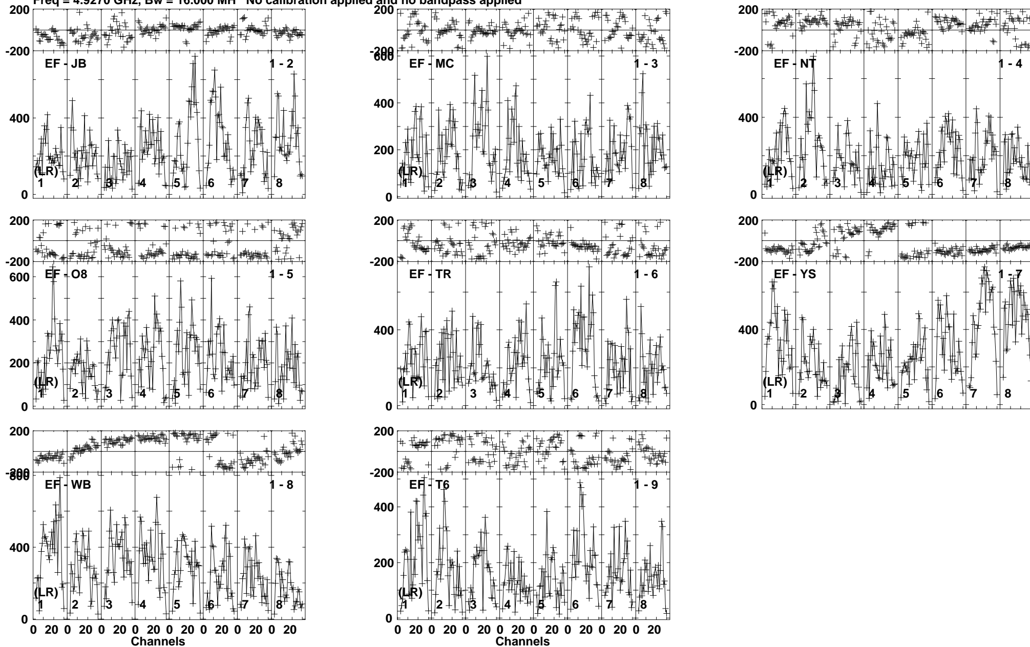
Lower frame: Micro Ampl Jy Top frame: Phas deg Vector averaged cross-power spectrum Baseline: EF (01) - JB (02) Timerange: 00/23:22:21 to 00/23:23:49
