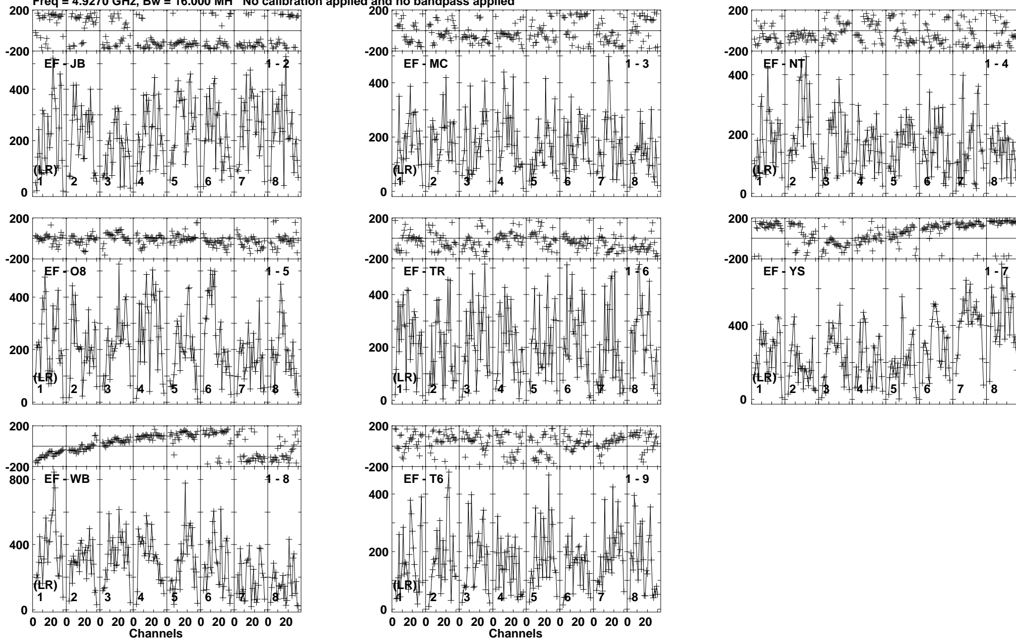
Lower frame: Micro Ampl Jy Top frame: Phas deg Vector averaged cross-power spectrum Baseline: EF (01) - JB (02) Timerange: 00/21:15:40 to 00/21:17:10
