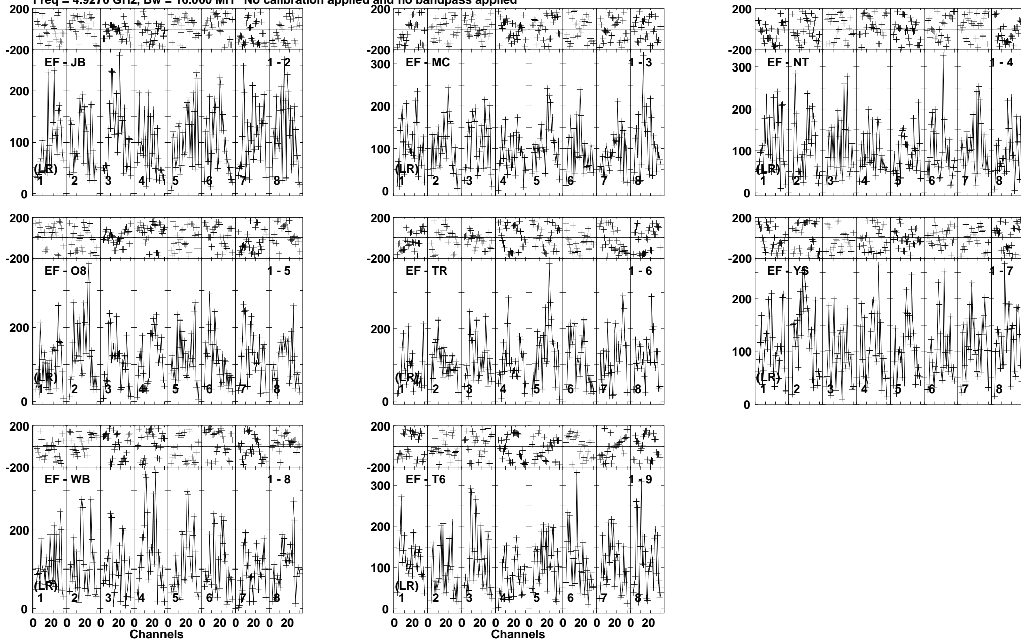
Lower frame: Micro Ampl Jy Top frame: Phas deg Vector averaged cross-power spectrum Baseline: EF (01) - JB (02) Timerange: 00/22:29:10 to 00/22:31:39
