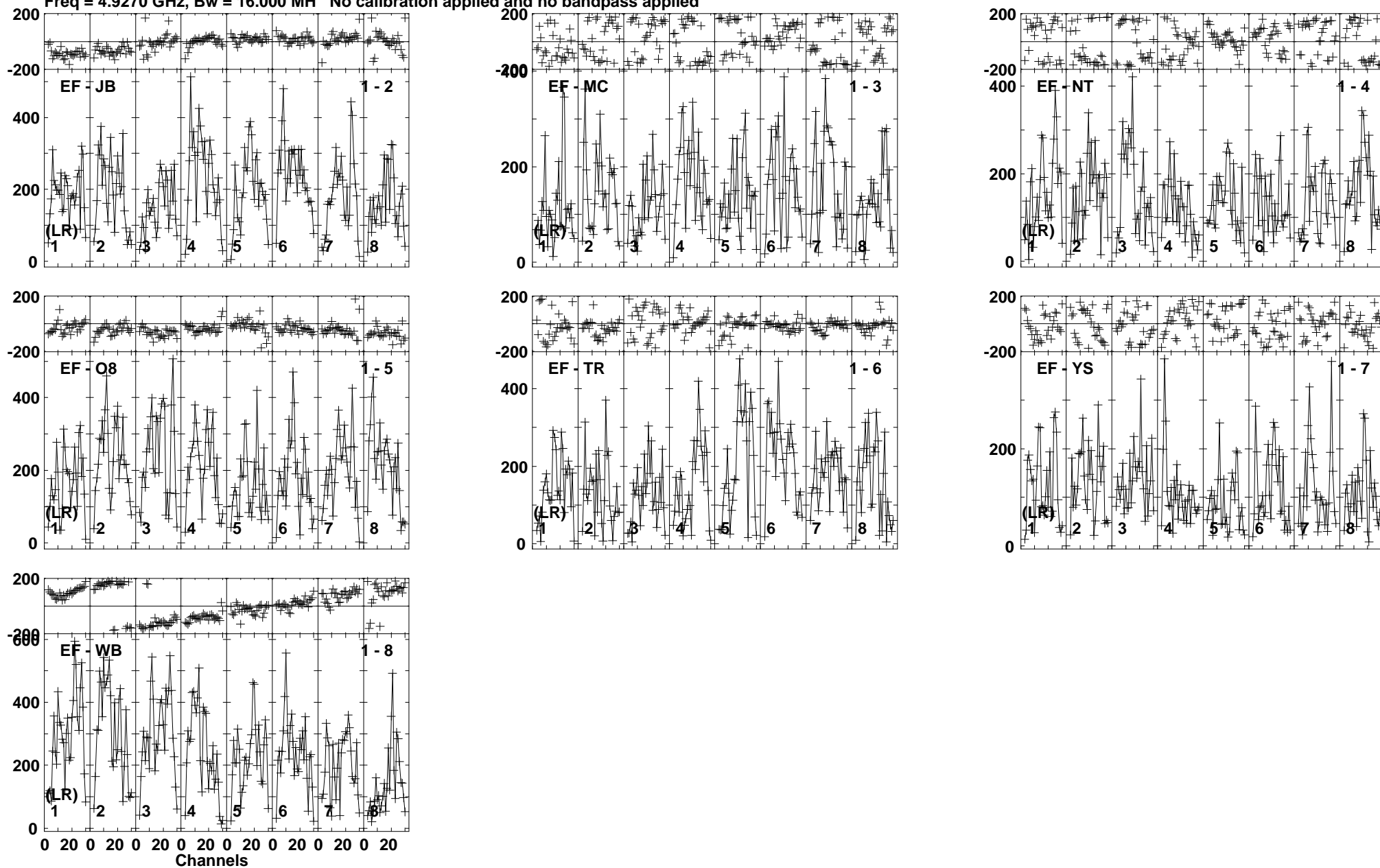
Lower frame: Micro Ampl Jy Top frame: Phas deg Vector averaged cross-power spectrum Baseline: EF (01) - JB (02) Timerange: 01/07:34:20 to 01/07:35:49
