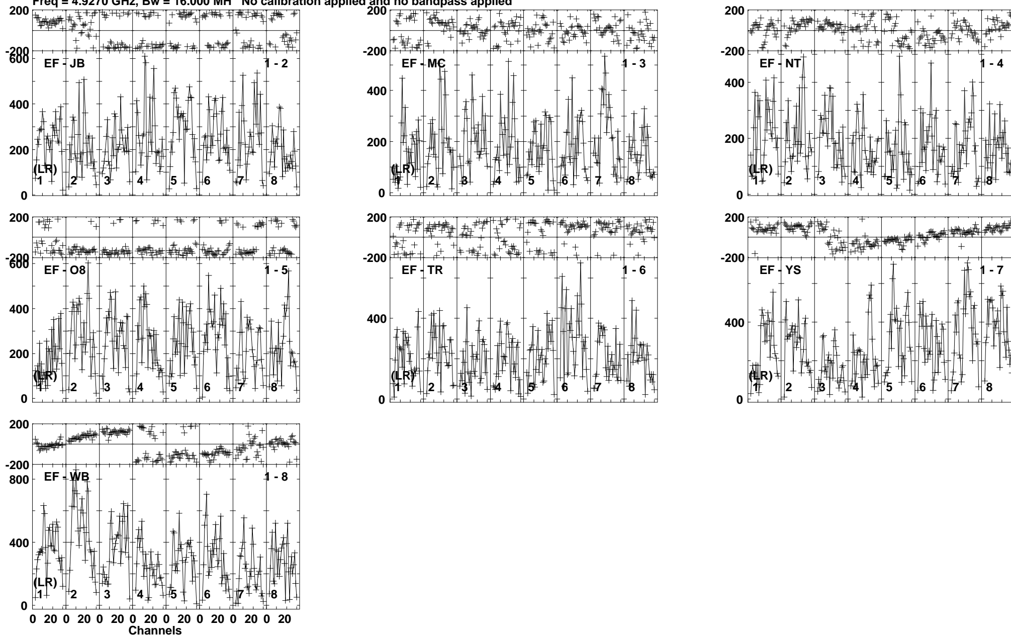
Lower frame: Micro Ampl Jy Top frame: Phas deg Vector averaged cross-power spectrum Baseline: EF (01) - JB (02) Timerange: 01/03:43:30 to 01/03:45:00
