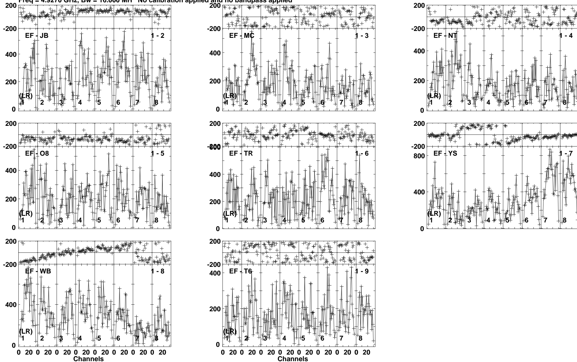
Lower frame: Micro Ampl Jy Top frame: Phas deg Vector averaged cross-power spectrum Baseline: EF (01) - JB (02) Timerange: 00:21:59:40 to 00:22:01:10
