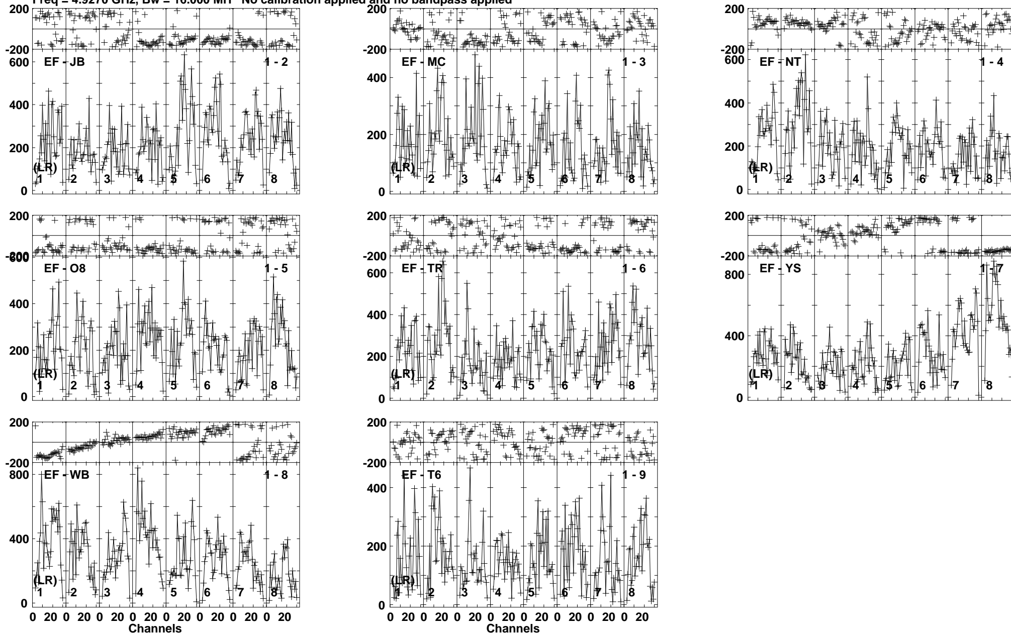
Lower frame: Micro Ampl Jy Top frame: Phas deg Vector averaged cross-power spectrum Baseline: EF (01) - JB (02) Timerange: 00/22:57:00 to 00/22:58:30
