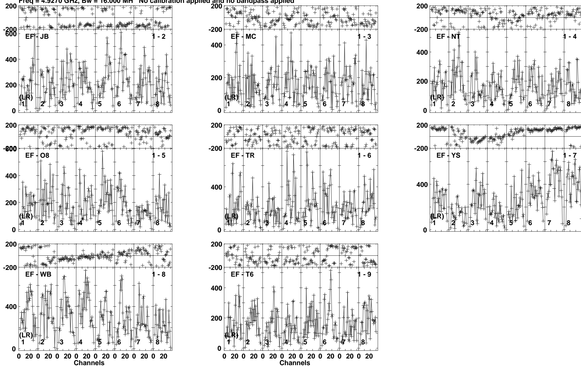
Lower frame: Micro Ampl Jy Top frame: Phas deg Vector averaged cross-power spectrum Baseline: EF (01) - JB (02) Timerange: 00/20:43:41 to 00/20:45:10
