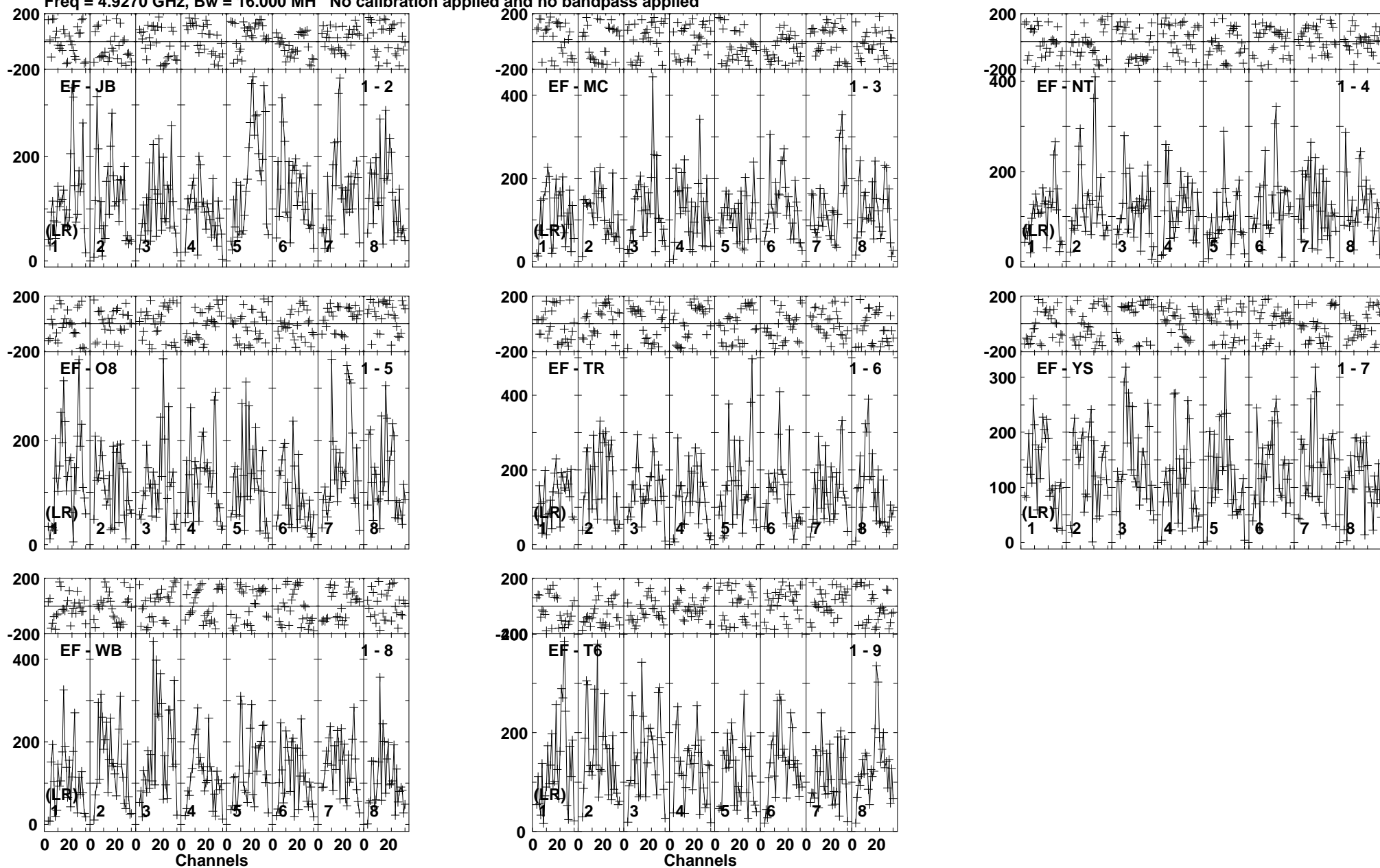
Lower frame: Micro Ampl Jy Top frame: Phas deg Vector averaged cross-power spectrum Baseline: EF (01) - JB (02) Timerange: 01/00:52:30 to 01/00:54:30
