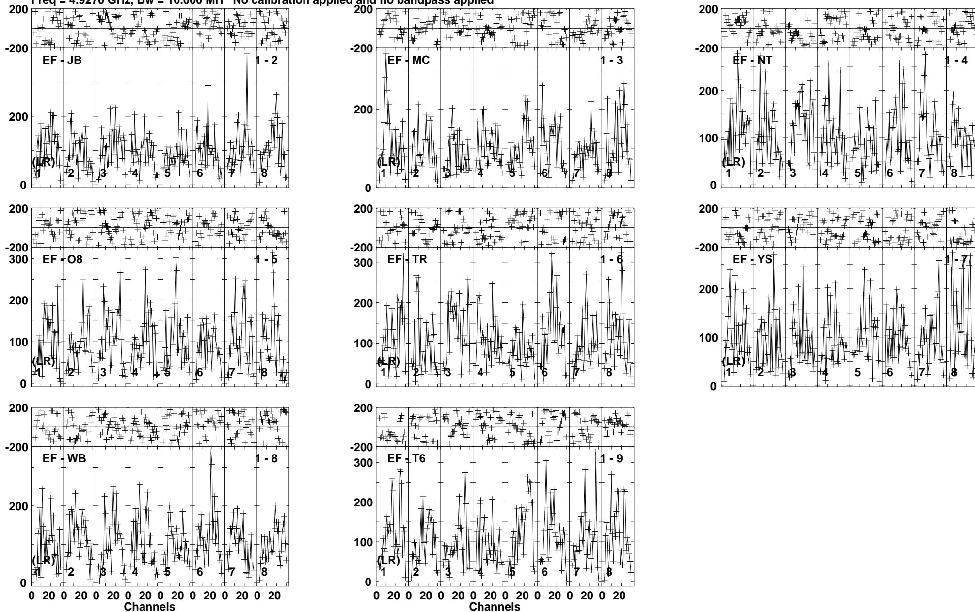
Lower frame: Micro Ampl Jy Top frame: Phas deg Vector averaged cross-power spectrum Baseline: EF (01) - JB (02) Timerange: 00/21:44:31 to 00/21:46:59
