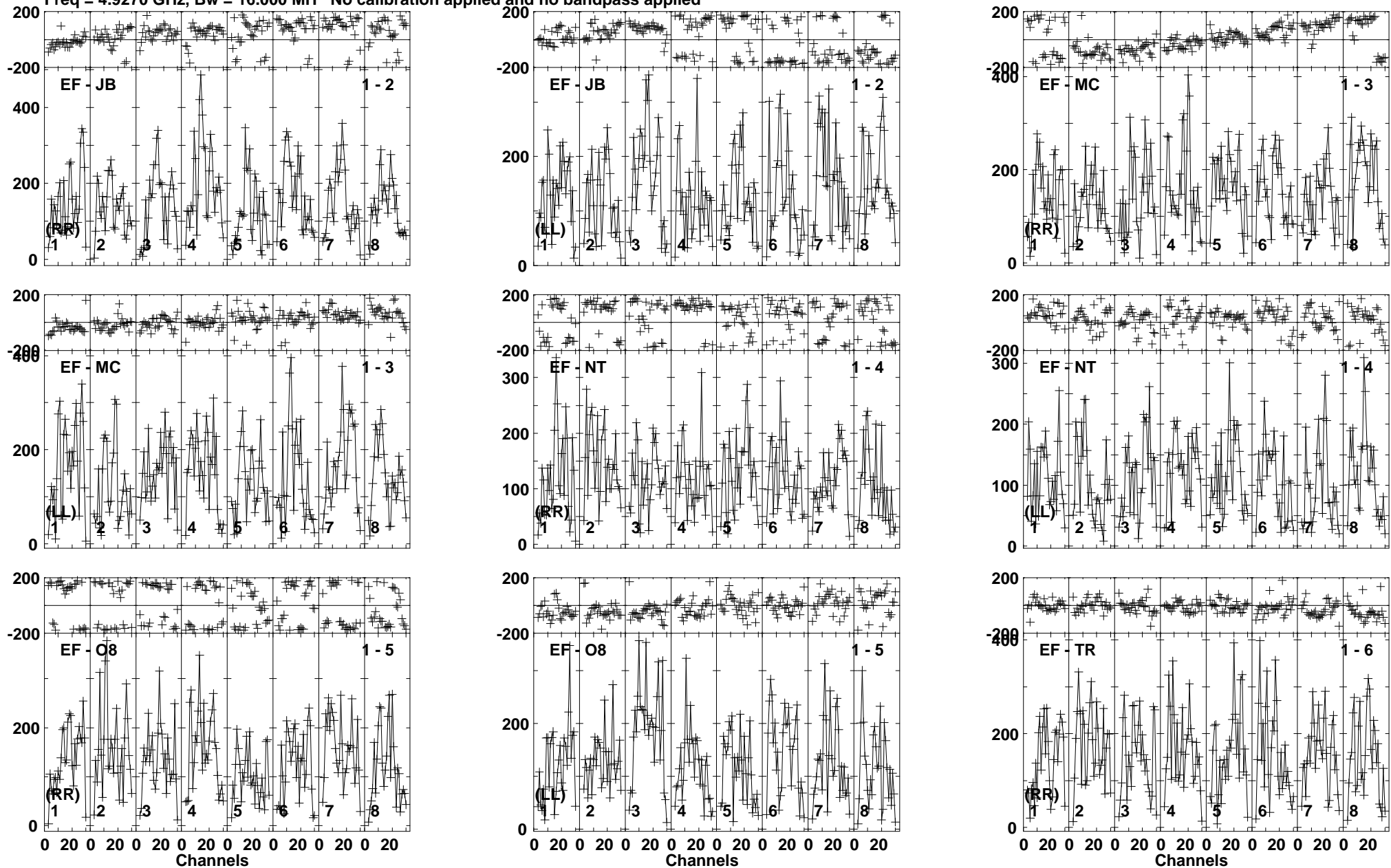
Lower frame: Micro Ampl Jy Top frame: Phas deg Vector averaged cross-power spectrum Baseline: EF (01) - JB (02) Timerange: 01/00:03:50 to 01/00:06:20
