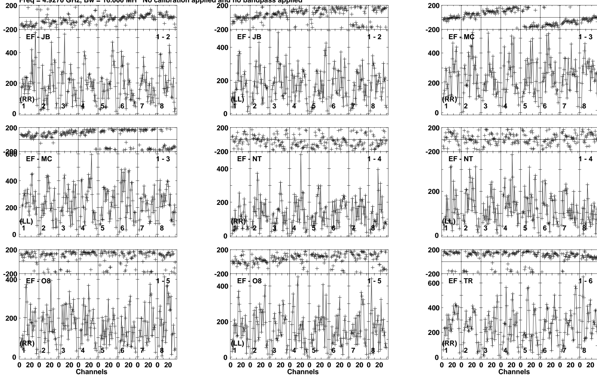
Lower frame: Micro Ampl Jy Top frame: Phas deg Vector averaged cross-power spectrum Baseline: EF (01) - JB (02) Timerange: 01/02:41:40 to 01/02:43:40
