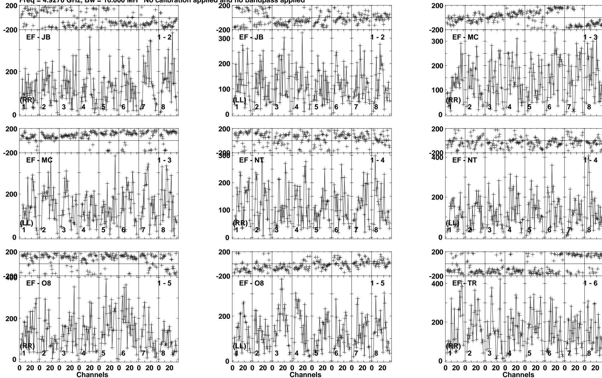
Lower frame: Micro Ampl Jy Top frame: Phas deg Vector averaged cross-power spectrum Baseline: EF (01) - JB (02) Timerange: 00/23:07:10 to 00/23:09:39
