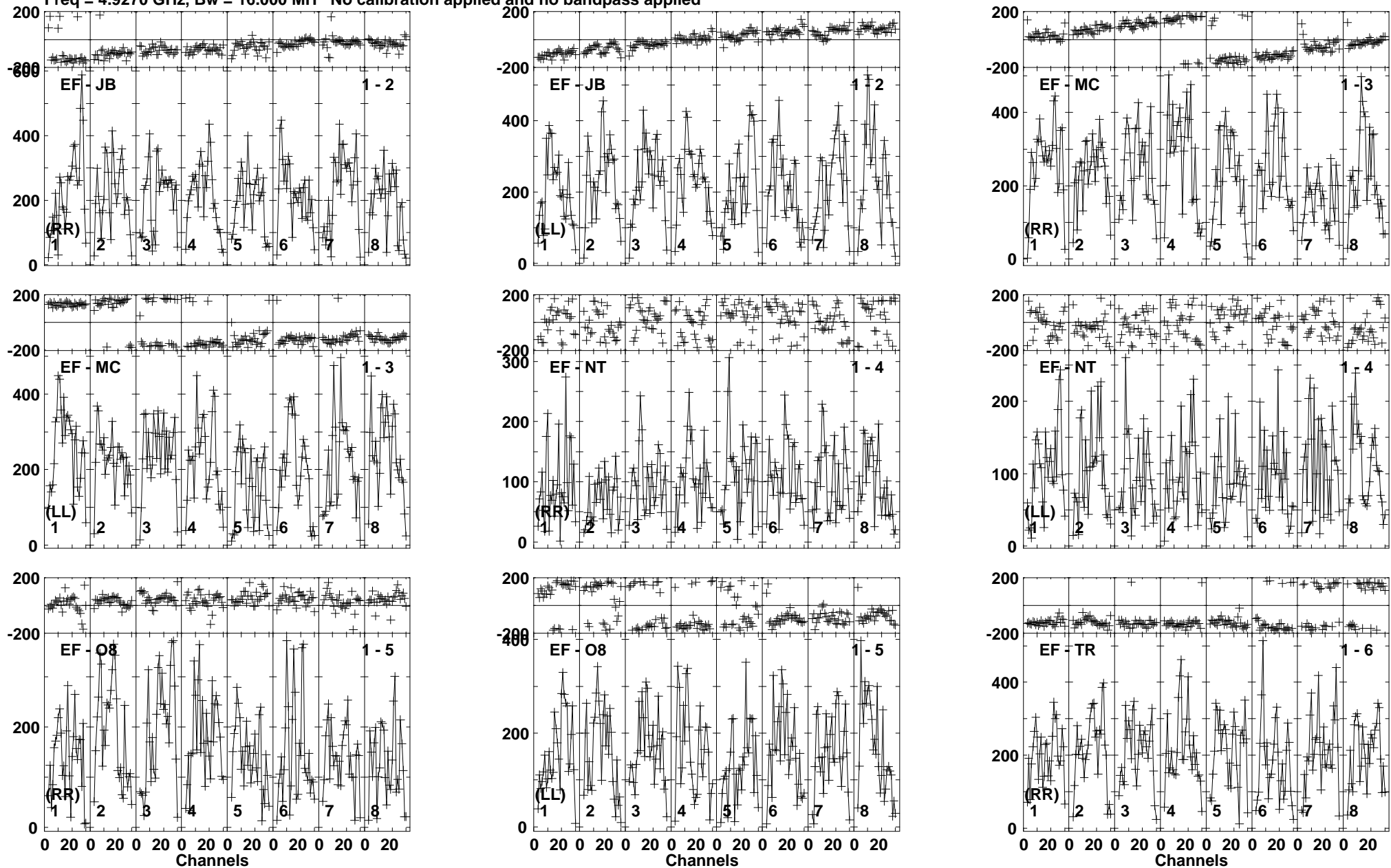
Lower frame: Micro Ampl Jy Top frame: Phas deg Vector averaged cross-power spectrum Baseline: EF (01) - JB (02) Timerange: 00/23:30:31 to 00/23:32:30
