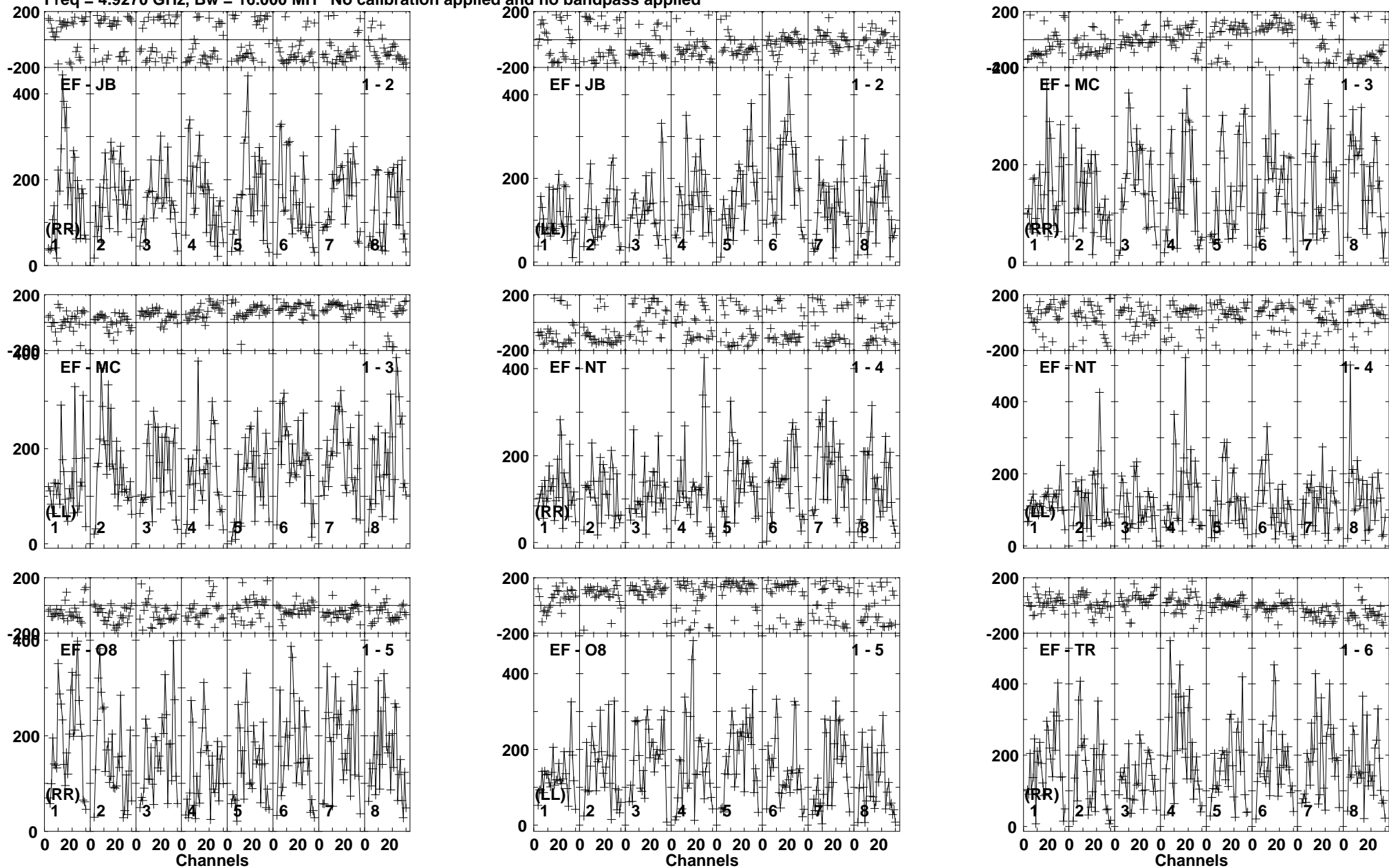
Lower frame: Micro Ampl Jy Top frame: Phas deg Vector averaged cross-power spectrum Baseline: EF (01) - JB (02) Timerange: 00/22:22:31 to 00/22:24:59
