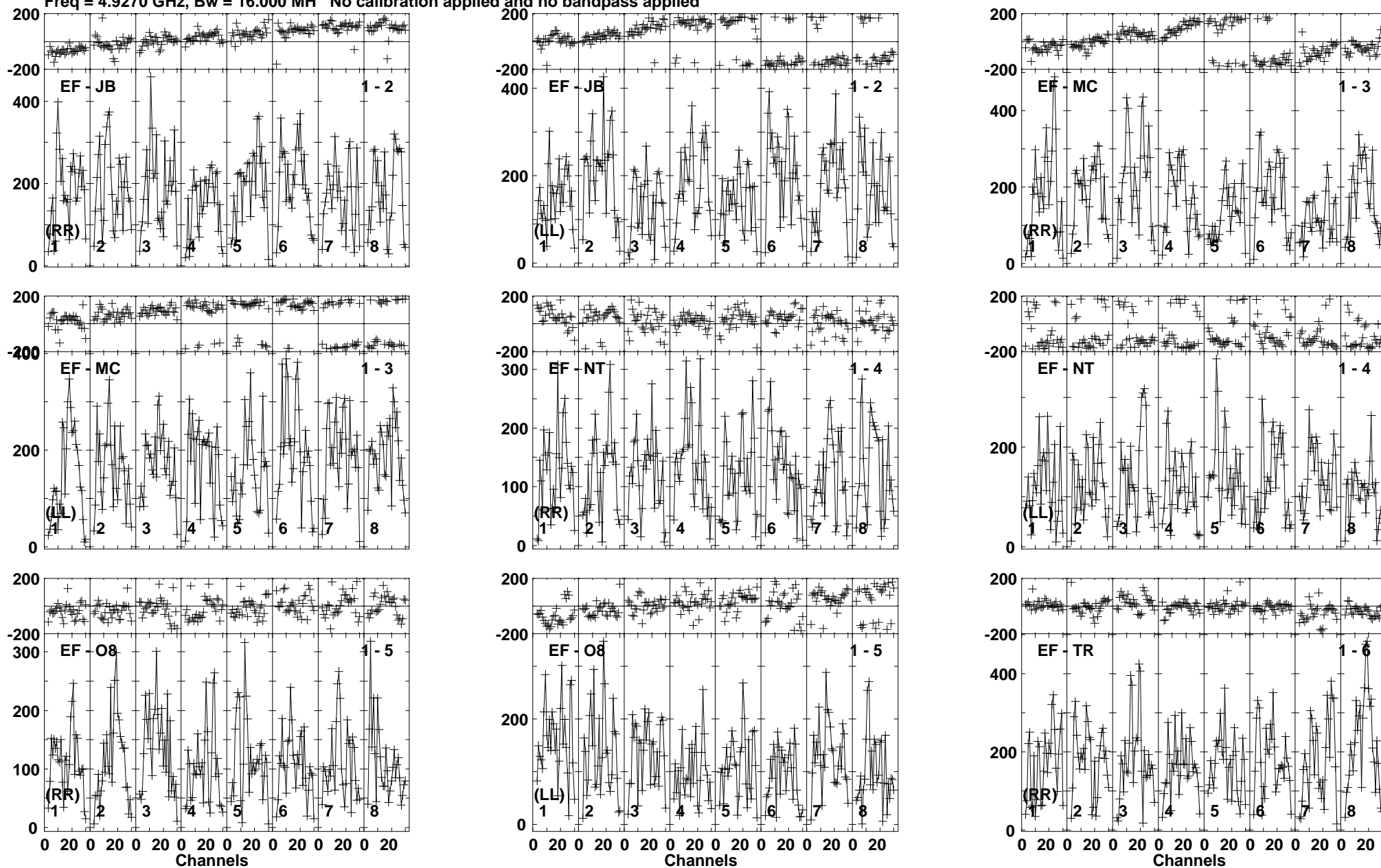
Lower frame: Micro Ampl Jy Top frame: Phas deg Vector averaged cross-power spectrum Baseline: EF (01) - JB (02) Timerange: 01/06:09:30 to 01/06:11:59
