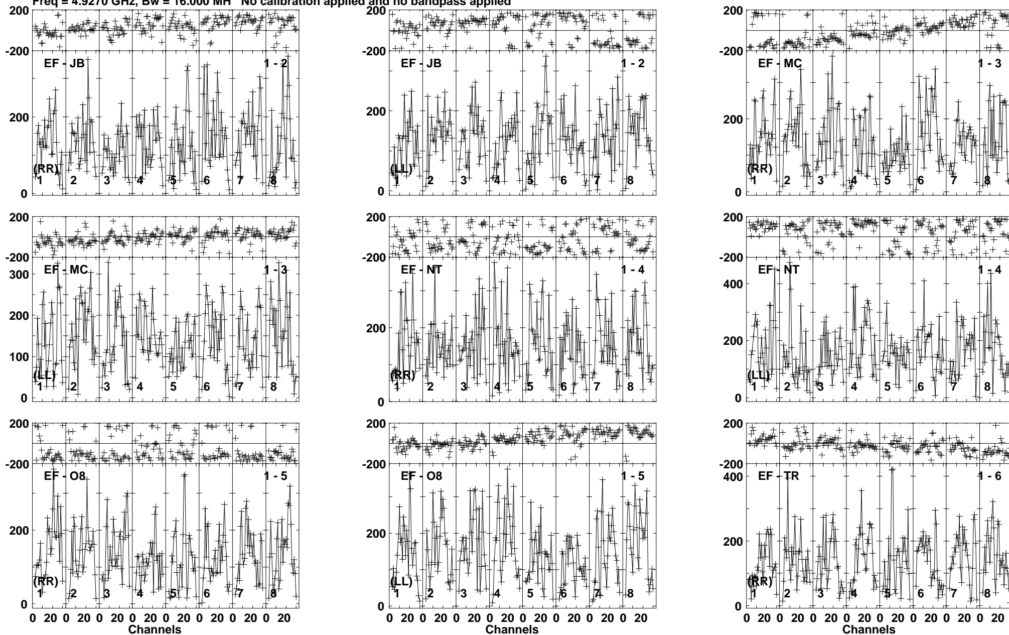
Lower frame: Micro Ampl Jy Top frame: Phas deg Vector averaged cross-power spectrum Baseline: EF (01) - JB (02) Timerange: 00/22:03:51 to 00/22:06:19
