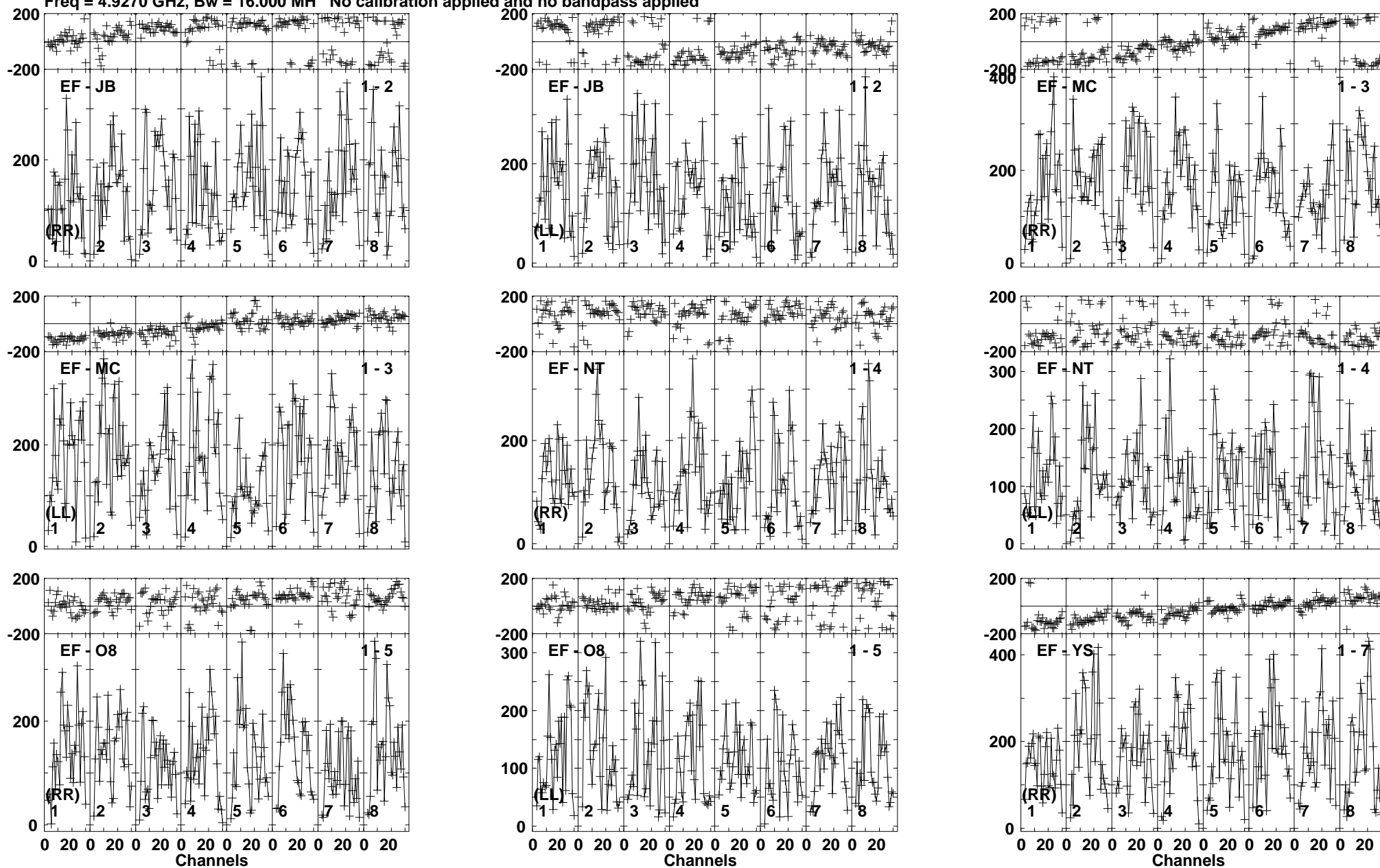
Lower frame: Micro Ampl Jy Top frame: Phas deg Vector averaged cross-power spectrum Baseline: EF (01) - JB (02) Timerange: 01/04:12:40 to 01/04:15:10
