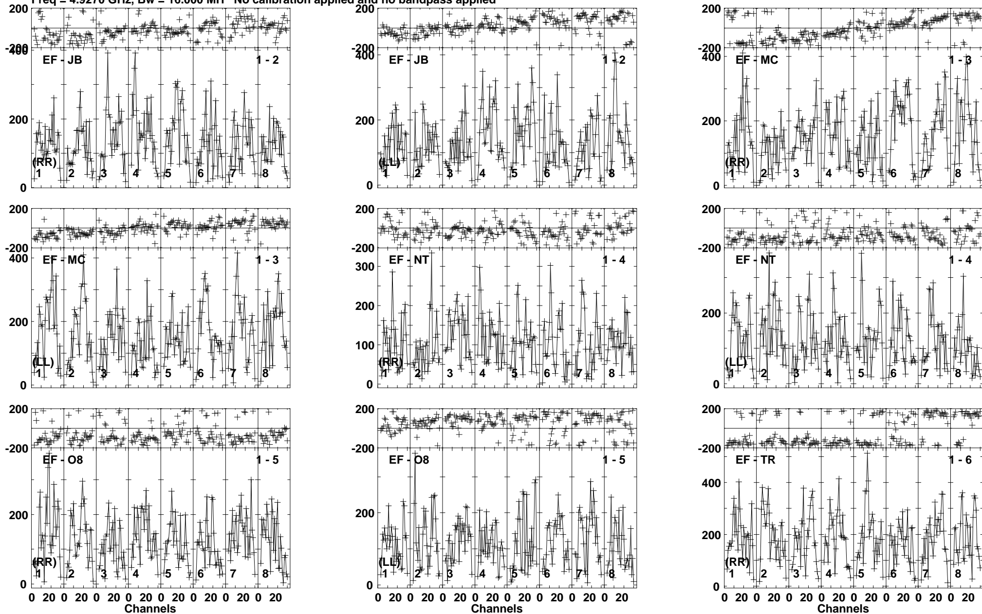
Lower frame: Micro Ampl Jy Top frame: Phas deg Vector averaged cross-power spectrum Baseline: EF (01) - JB (02) Timerange: 01/01:13:51 to 01/01:16:19
