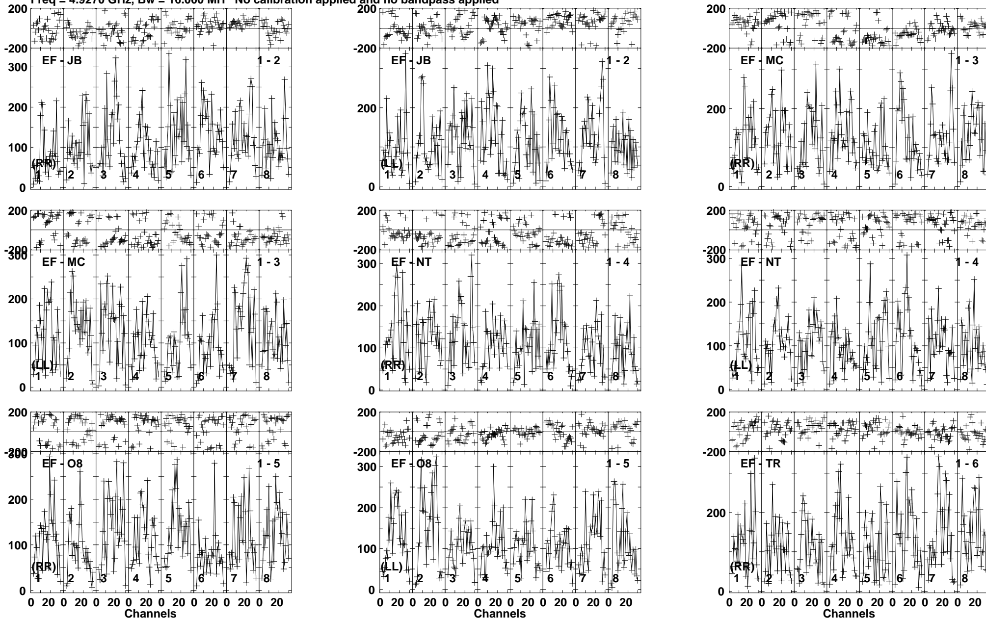
Lower frame: Micro Ampl Jy Top frame: Phas deg Vector averaged cross-power spectrum Baseline: EF (01) - JB (02) Timerange: 00/20:09:51 to 00/20:12:20
