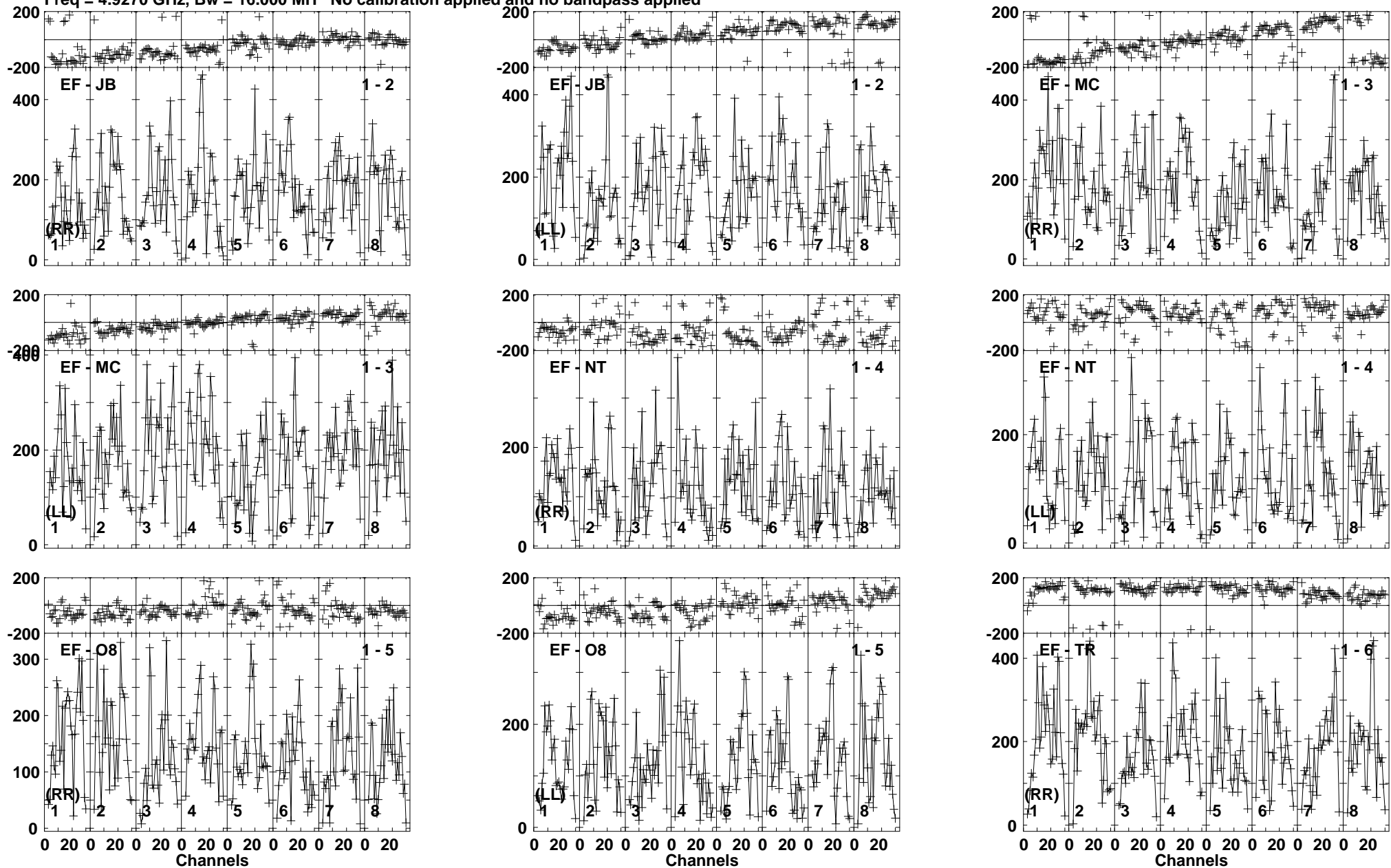
Lower frame: Micro Ampl Jy Top frame: Phas deg Vector averaged cross-power spectrum Baseline: EF (01) - JB (02) Timerange: 01/05:37:50 to 01/05:40:20
