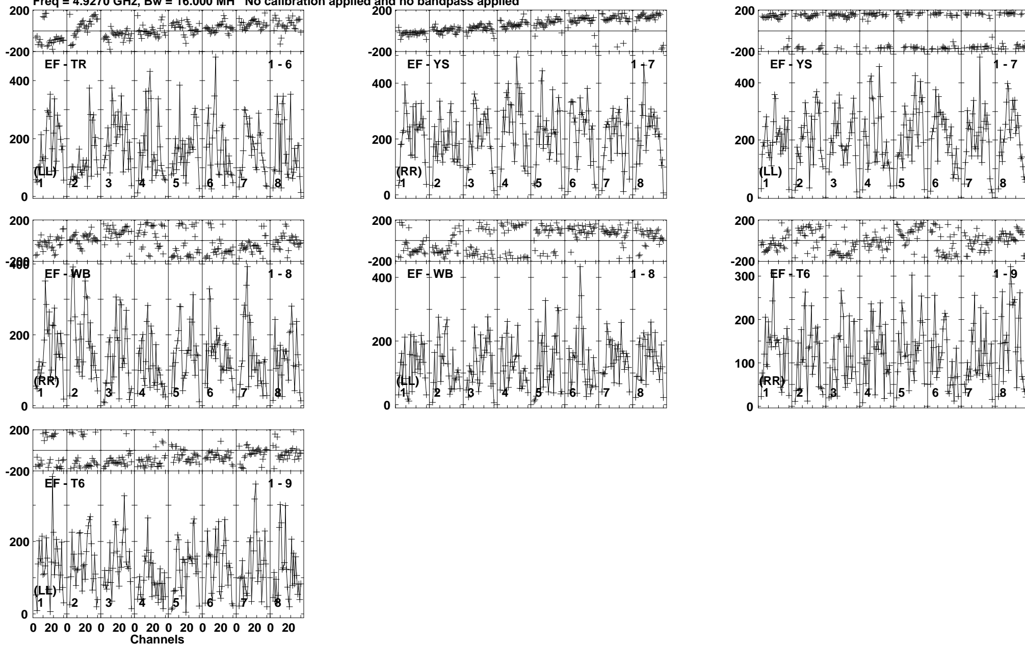
Lower frame: Micro Ampl Jy Top frame: Phas deg Vector averaged cross-power spectrum Baseline: EF (01) - TR (06) Timerange: 01/00:10:30 to 01/00:13:00
