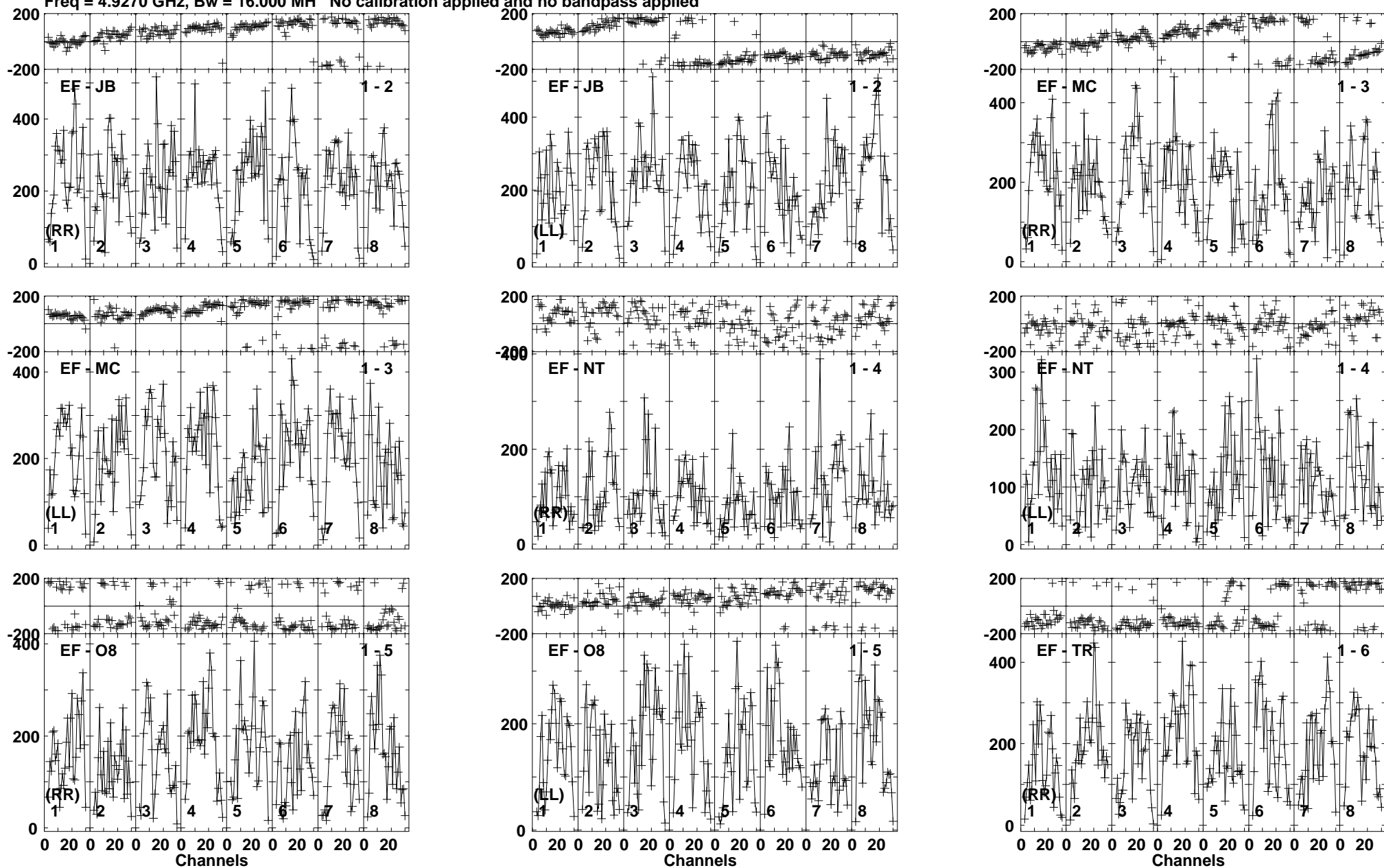
Lower frame: Micro Ampl Jy Top frame: Phas deg Vector averaged cross-power spectrum Baseline: EF (01) - JB (02) Timerange: 01/01:37:10 to 01/01:39:09
