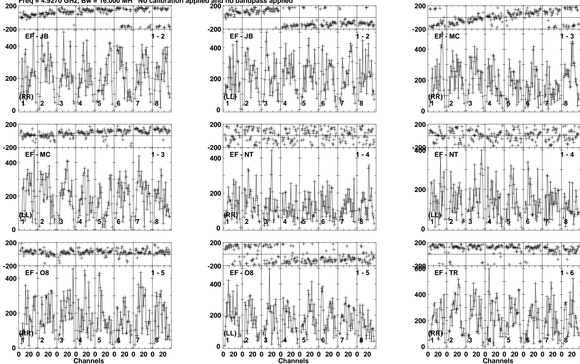
Lower frame: Micro Ampl Jy Top frame: Phas deg Vector averaged cross-power spectrum Baseline: EF (01) - JB (02) Timerange: 00/22:58:31 to 00/23:00:29
