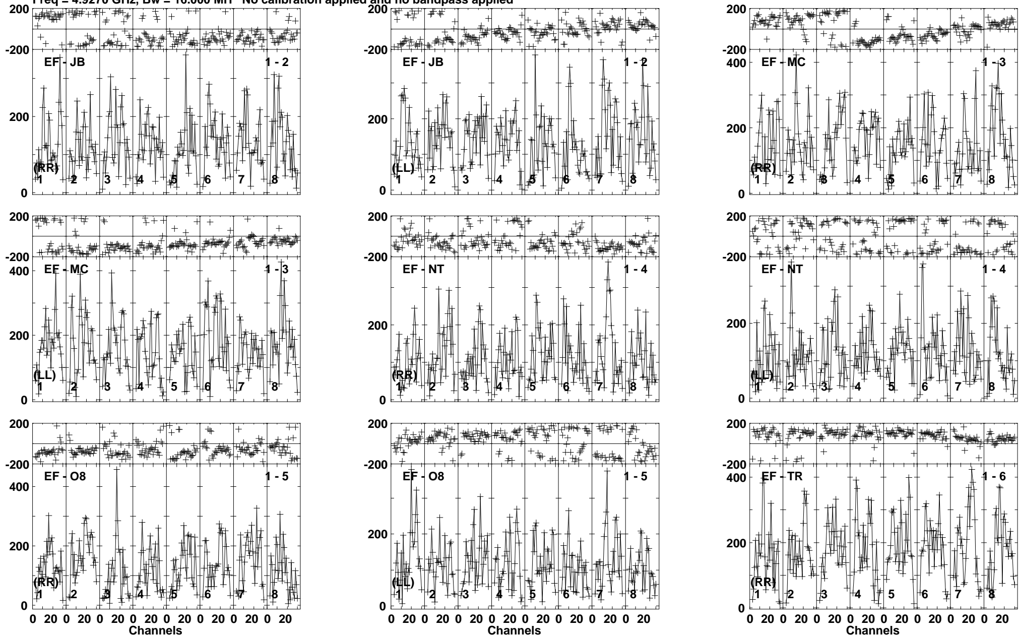
Lower frame: Micro Ampl Jy Top frame: Phas deg Vector averaged cross-power spectrum Baseline: EF (01) - JB (02) Timerange: 01/00:48:31 to 01/00:51:00
