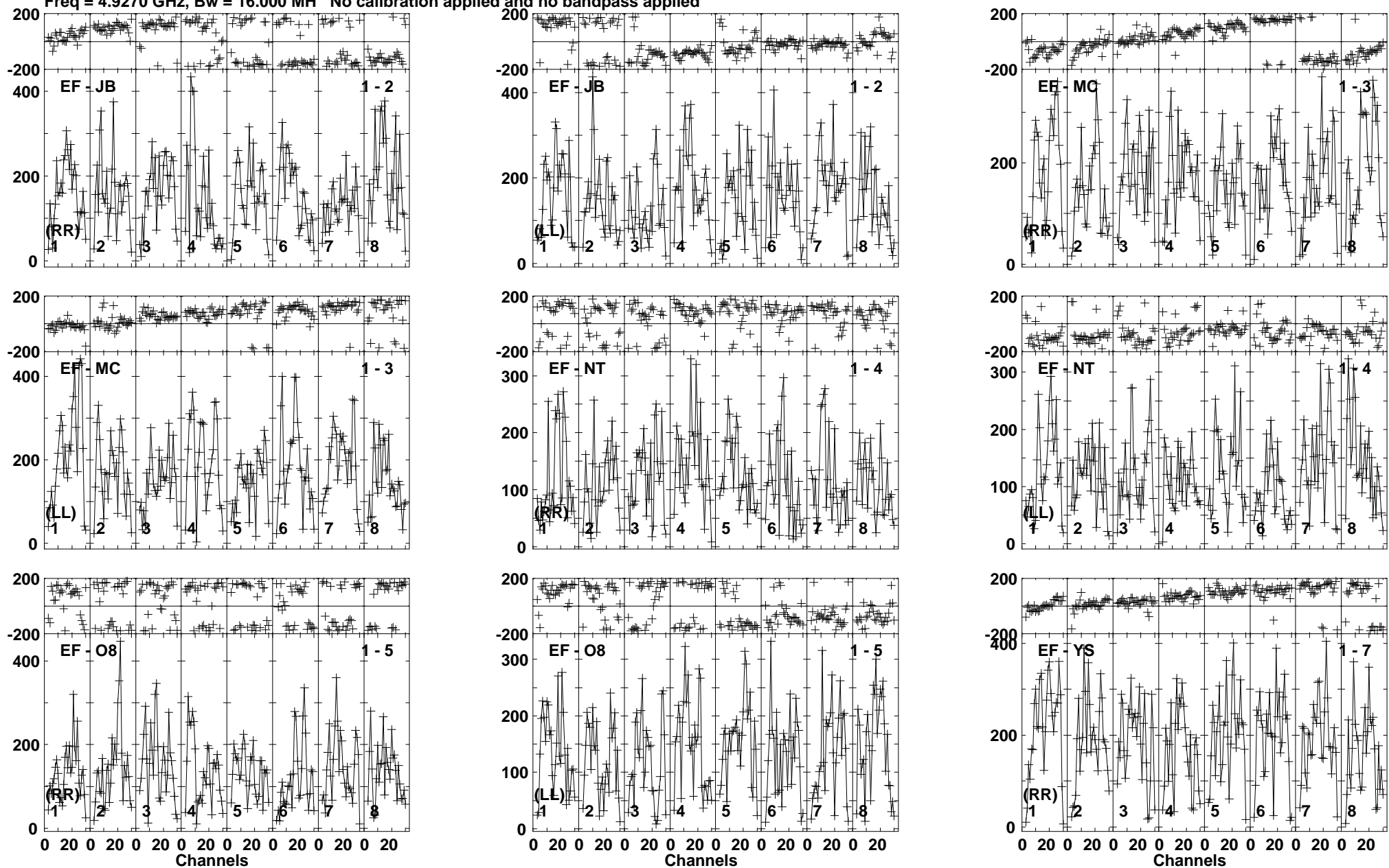
Lower frame: Micro Ampl Jy Top frame: Phas deg Vector averaged cross-power spectrum Baseline: EF (01) - JB (02) Timerange: 01/04:44:20 to 01/04:46:50
