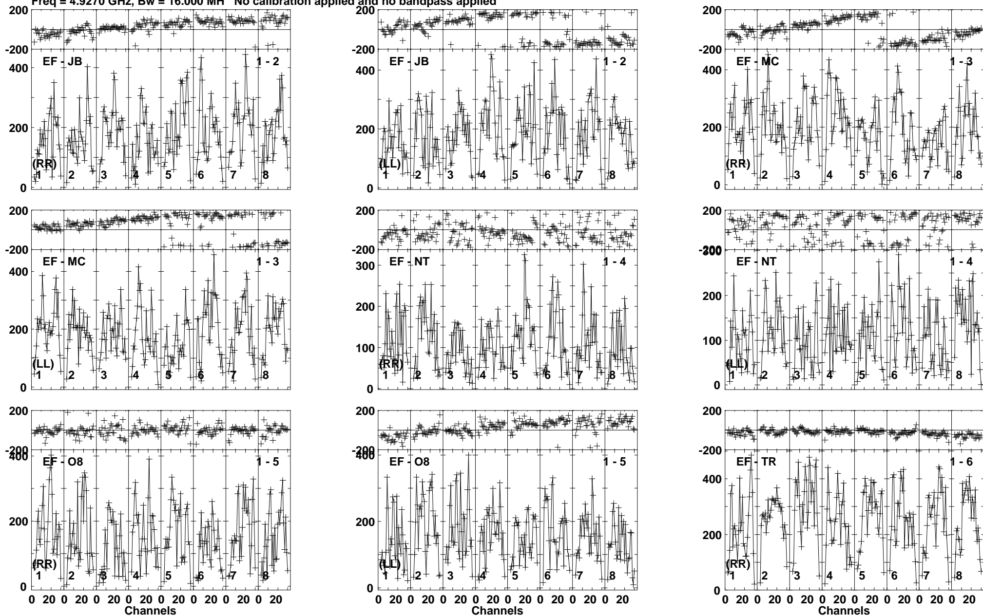
Lower frame: Micro Ampl Jy Top frame: Phas deg Vector averaged cross-power spectrum Baseline: EF (01) - JB (02) Timerange: 01/06:17:20 to 01/06:19:19
