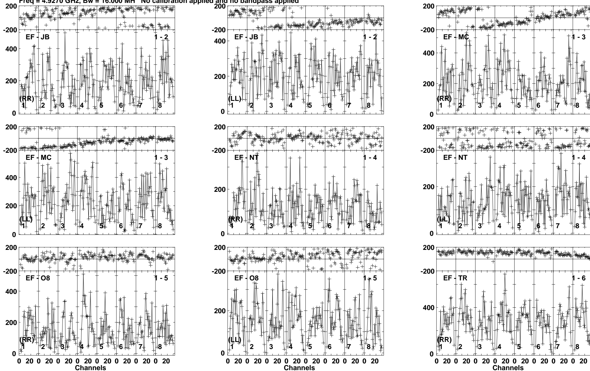
Lower frame: Micro Ampl Jy Top frame: Phas deg Vector averaged cross-power spectrum Baseline: EF (01) - JB (02) Timerange: 01/06:55:01 to 01/06:56:59
