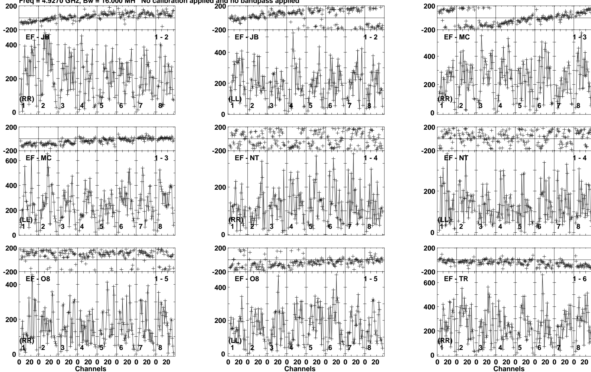
Lower frame: Micro Ampl Jy Top frame: Phas deg Vector averaged cross-power spectrum Baseline: EF (01) - JB (02) Timerange: 00/23:49:11 to 00/23:51:10
