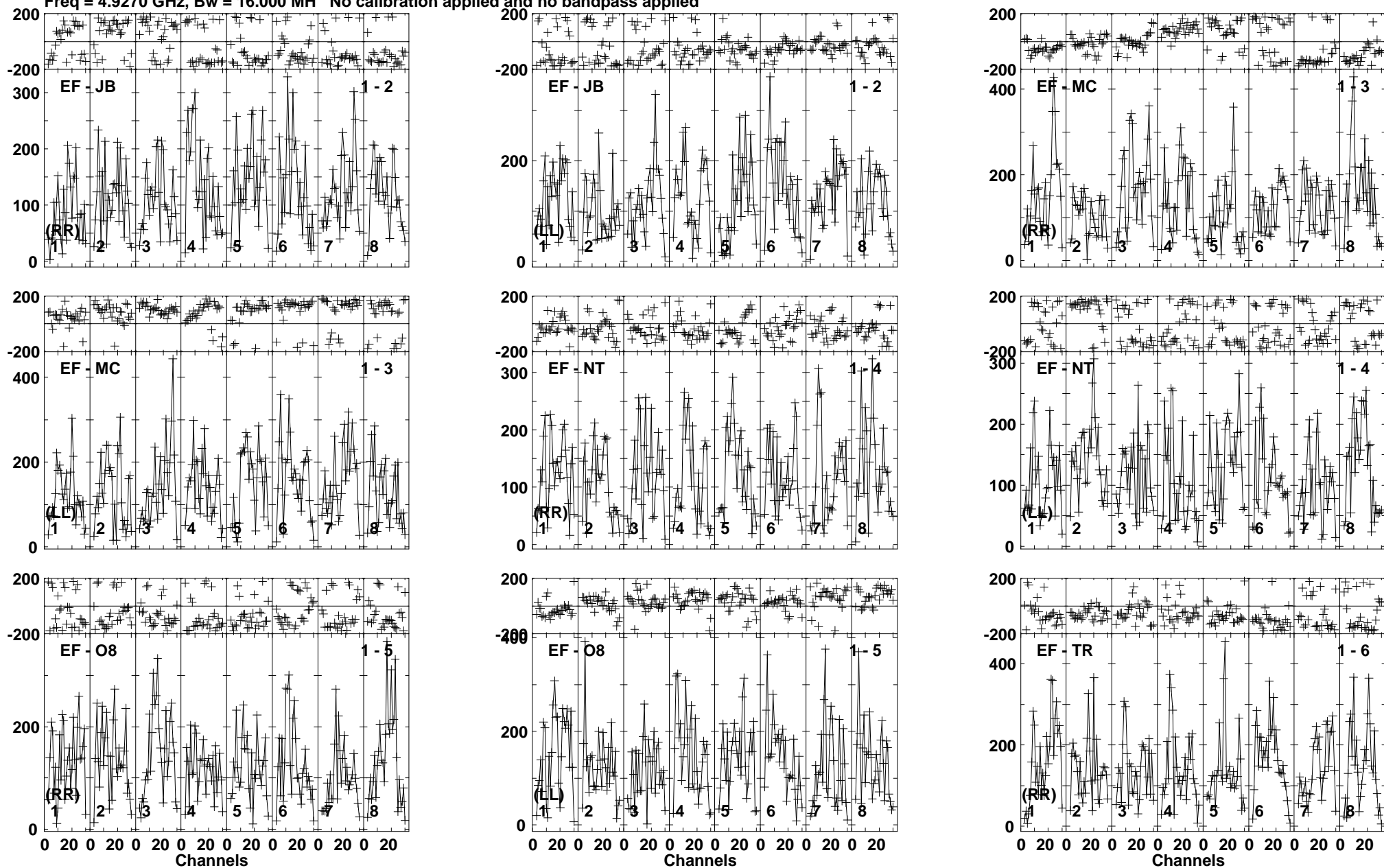
Lower frame: Micro Ampl Jy Top frame: Phas deg Vector averaged cross-power spectrum Baseline: EF (01) - JB (02) Timerange: 00/21:19:11 to 00/21:21:40
