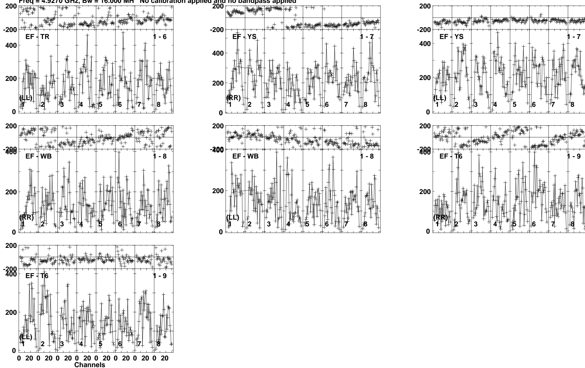
Lower frame: Micro Ampl Jy Top frame: Phas deg Vector averaged cross-power spectrum Baseline: EF (01) - TR (06) Timerange: 00/23:19:51 to 00/23:22:19
