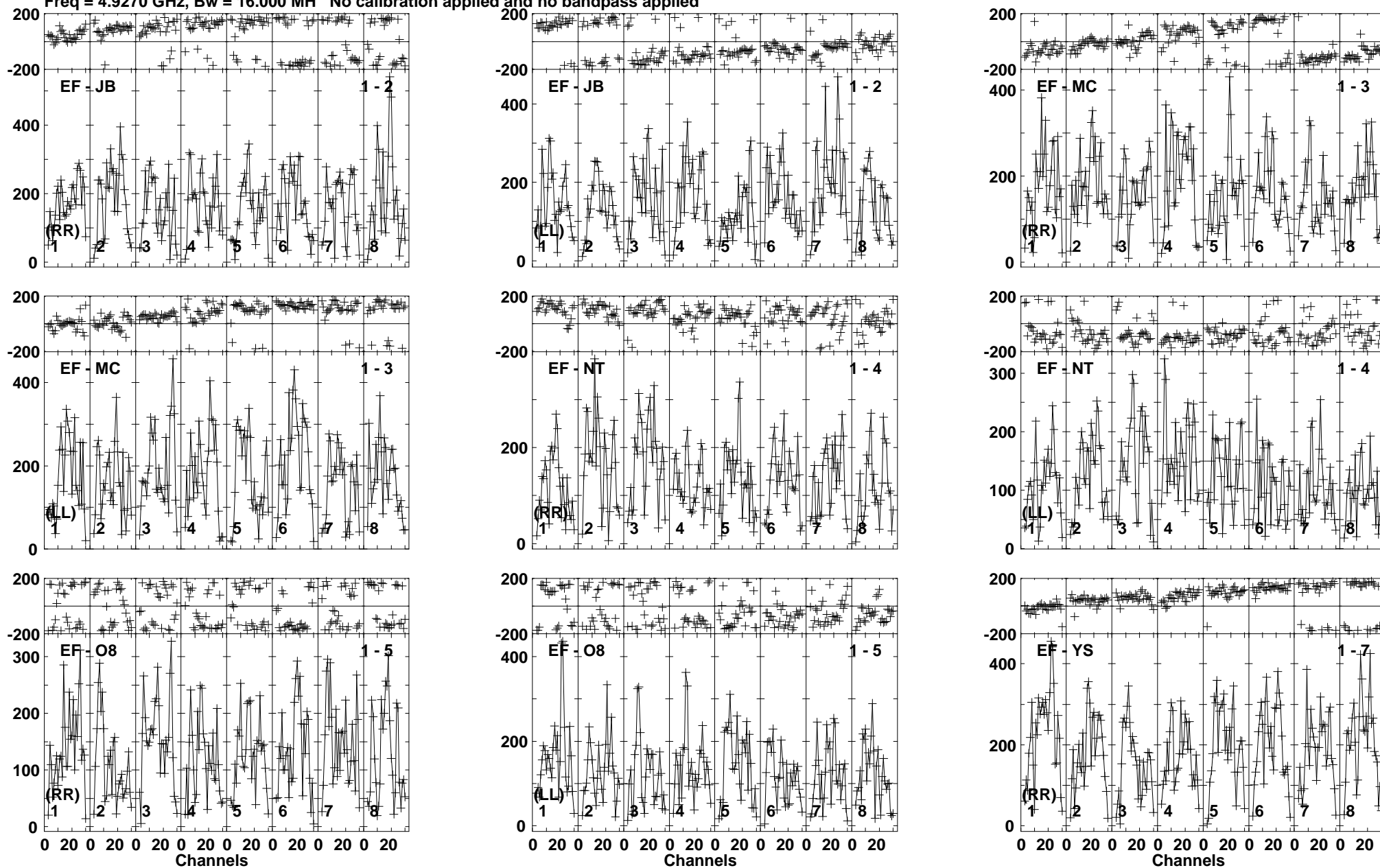
Lower frame: Micro Ampl Jy Top frame: Phas deg Vector averaged cross-power spectrum Baseline: EF (01) - JB (02) Timerange: 01/04:50:21 to 01/04:52:49
