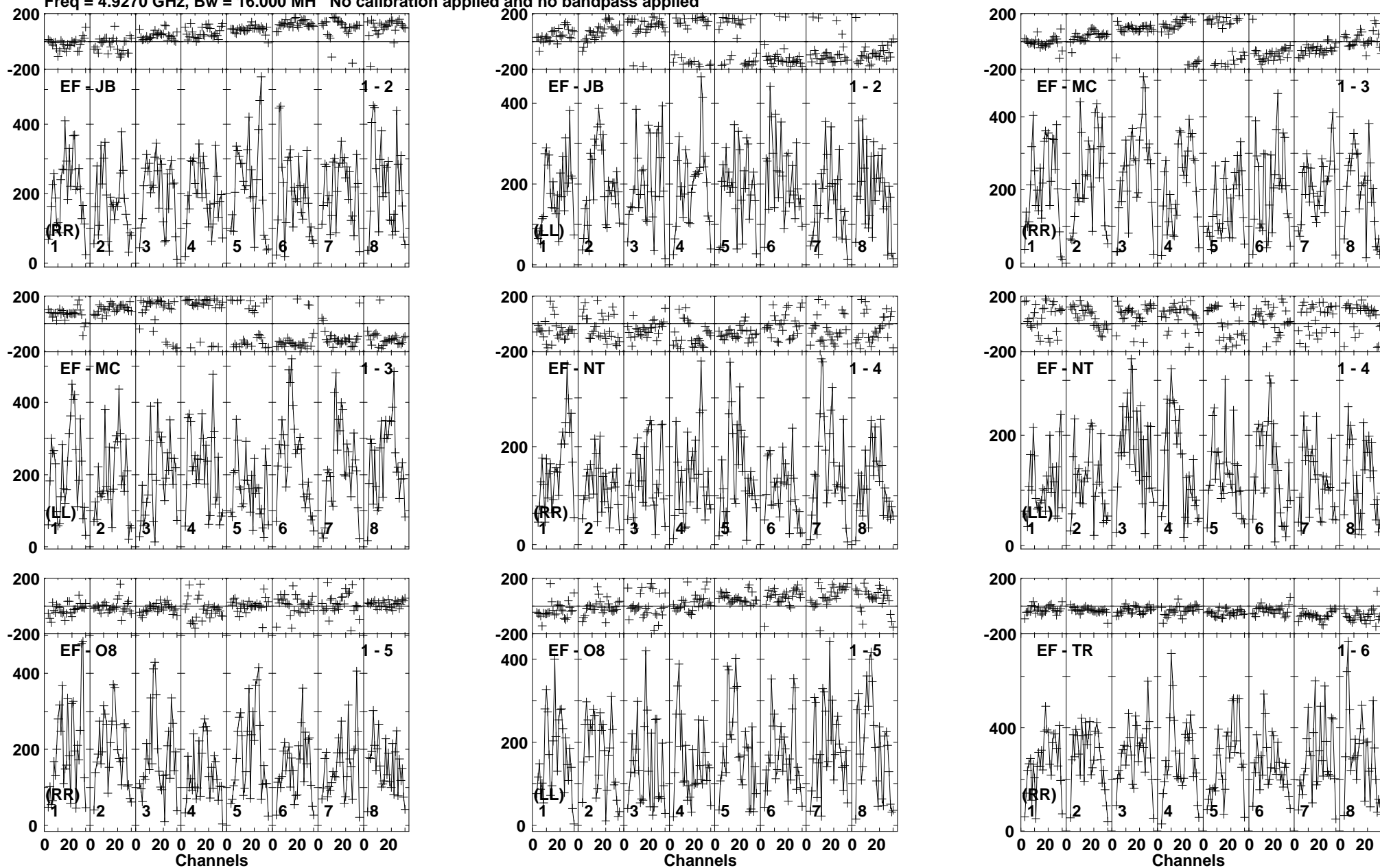
Lower frame: Micro Ampl Jy Top frame: Phas deg Vector averaged cross-power spectrum Baseline: EF (01) - JB (02) Timerange: 01/06:23:20 to 01/06:25:20
