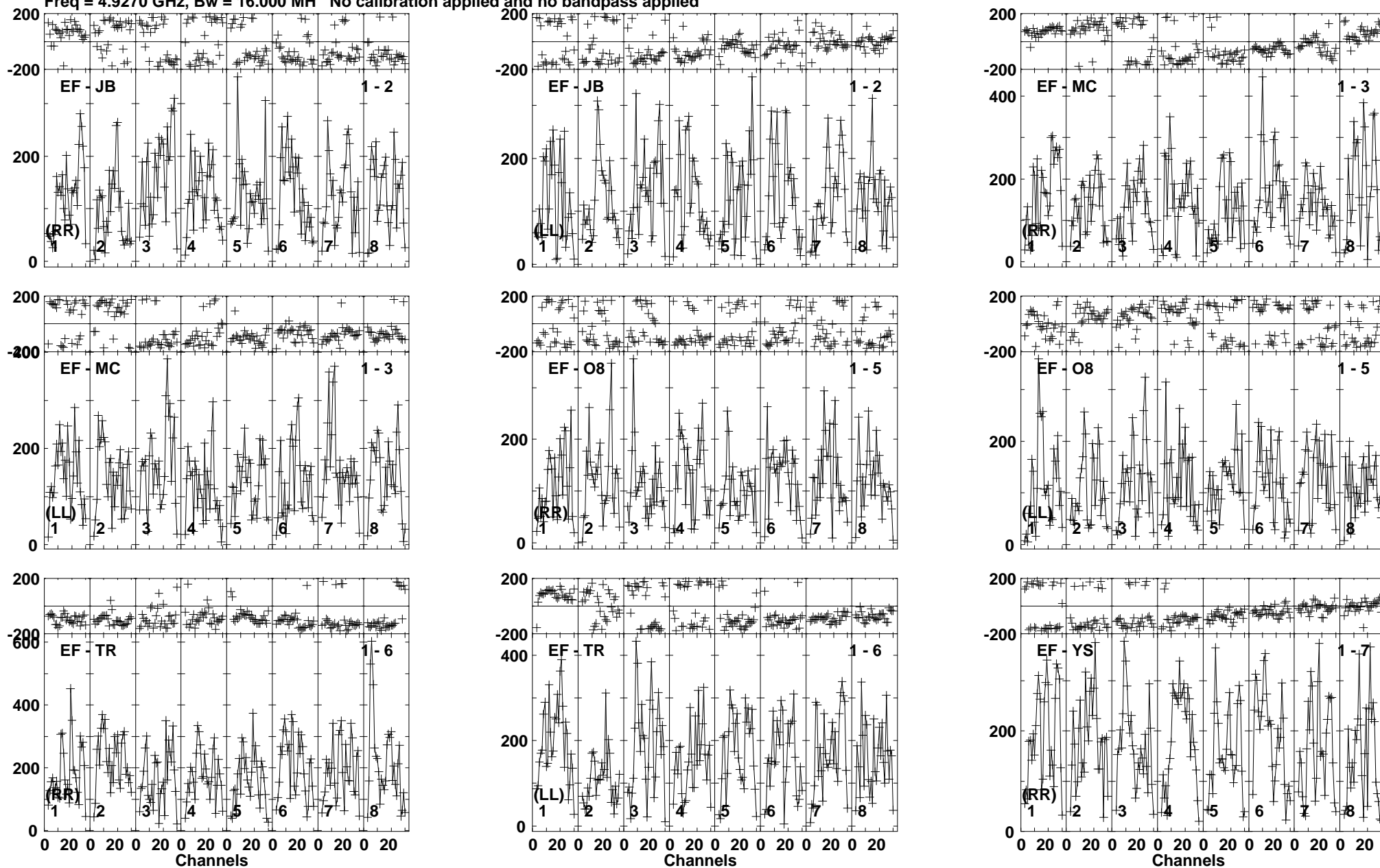
Lower frame: Micro Ampl Jy Top frame: Phas deg Vector averaged cross-power spectrum Baseline: EF (01) - JB (02) Timerange: 01/02:06:01 to 01/02:08:29
