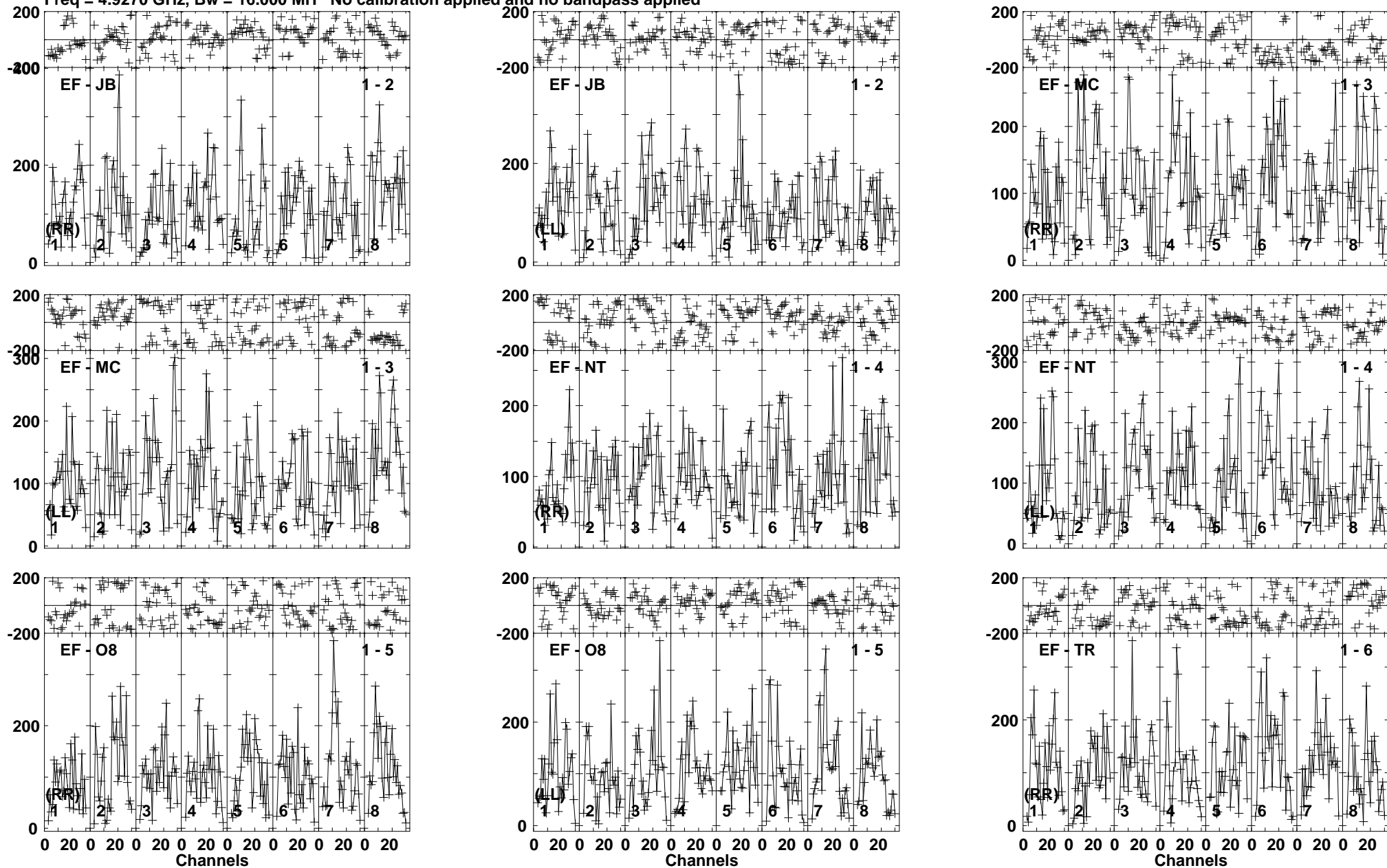
Lower frame: Micro Ampl Jy Top frame: Phas deg Vector averaged cross-power spectrum Baseline: EF (01) - JB (02) Timerange: 00/19:37:51 to 00/19:40:19
