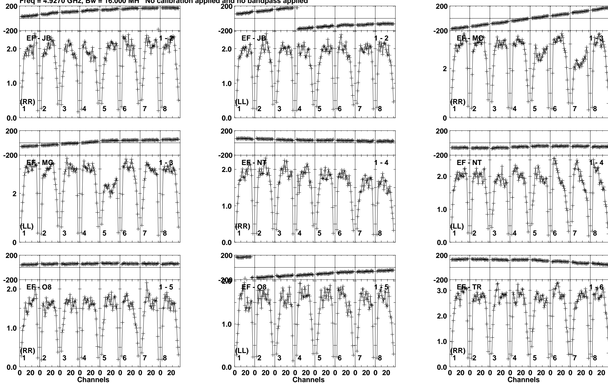
Lower frame: Milli Ampl Jy Top frame: Phas deg Vector averaged cross-power spectrum Baseline: EF (01) - JB (02) Timerange: 00/22:50:20 to 00/22:51:50
