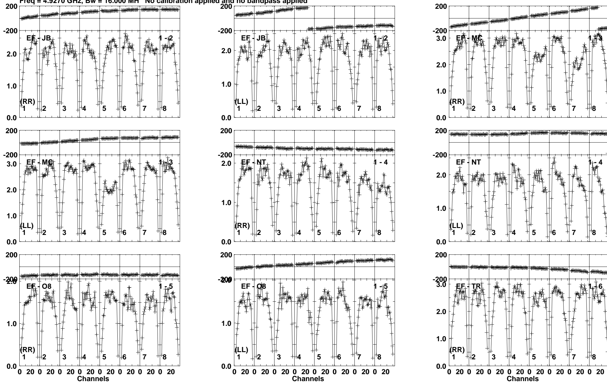
Lower frame: Milli Ampl Jy Top frame: Phas deg Vector averaged cross-power spectrum Baseline: EF (01) - JB (02) Timerange: 00/22:12:21 to 00/22:13:50
