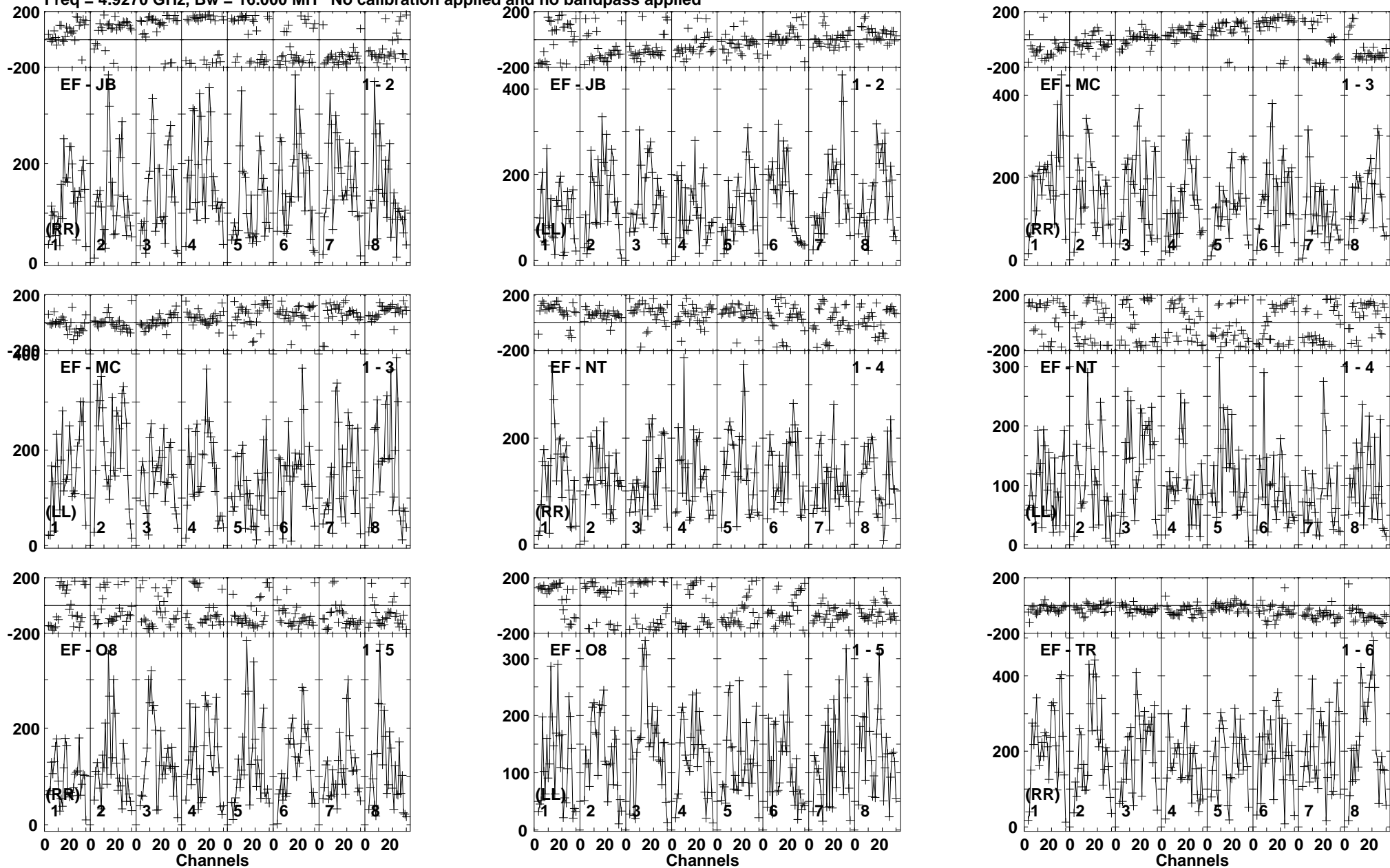
Lower frame: Micro Ampl Jy Top frame: Phas deg Vector averaged cross-power spectrum Baseline: EF (01) - JB (02) Timerange: 01/03:15:21 to 01/03:17:49
