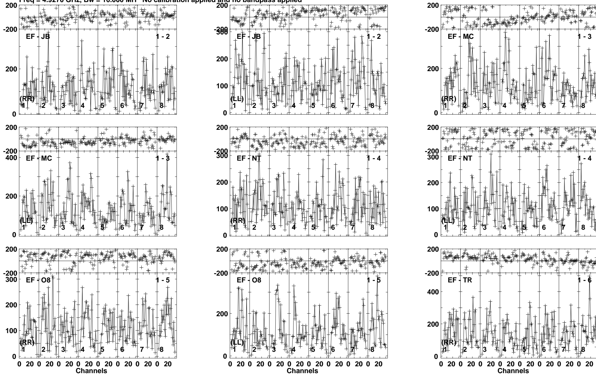
Lower frame: Micro Ampl Jy Top frame: Phas deg Vector averaged cross-power spectrum Baseline: EF (01) - JB (02) Timerange: 00/20:22:30 to 00/20:24:59
