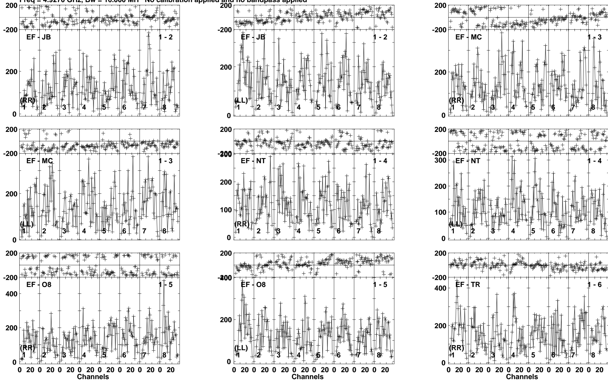
Lower frame: Micro Ampl Jy Top frame: Phas deg Vector averaged cross-power spectrum Baseline: EF (01) - JB (02) Timerange: 00/21:31:50 to 00/21:34:19
