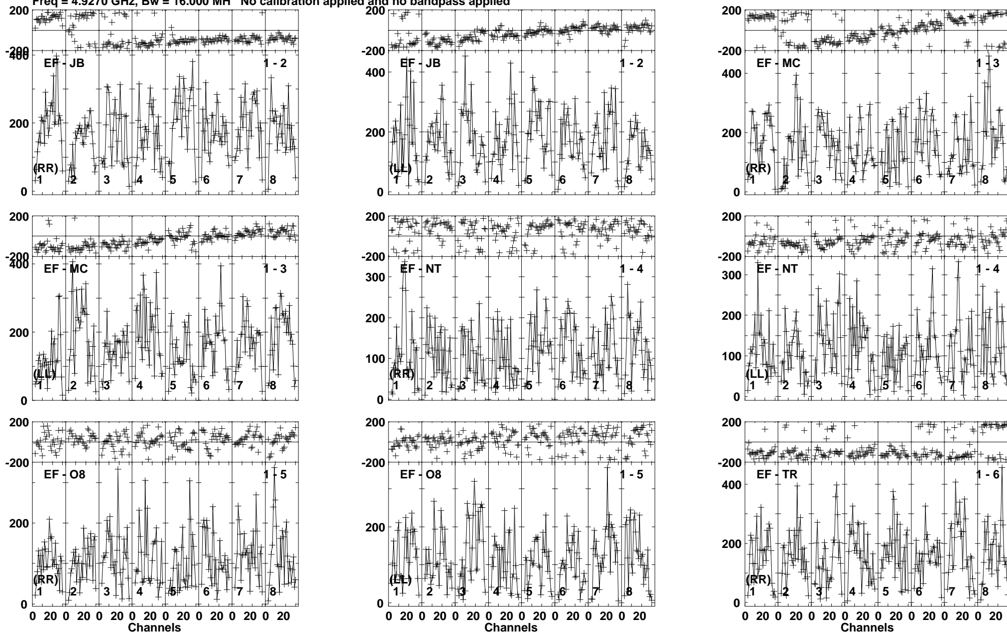
Lower frame: Micro Ampl Jy Top frame: Phas deg Vector averaged cross-power spectrum Baseline: EF (01) - JB (02) Timerange: 01/07:22:41 to 01/07:25:09
