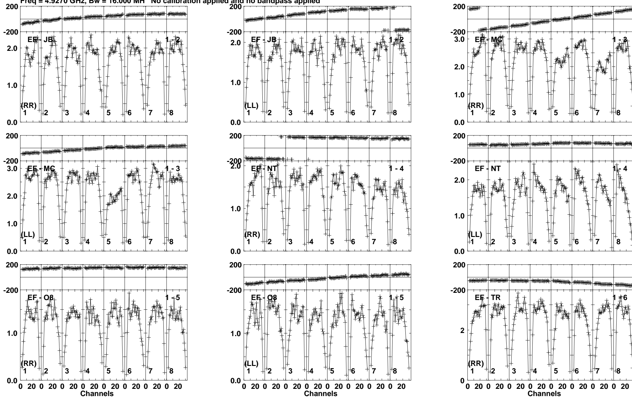
Lower frame: Milli Ampl Jy Top frame: Phas deg Vector averaged cross-power spectrum Baseline: EF (01) - JB (02) Timerange: 01/00:00:20 to 01/00:01:49
