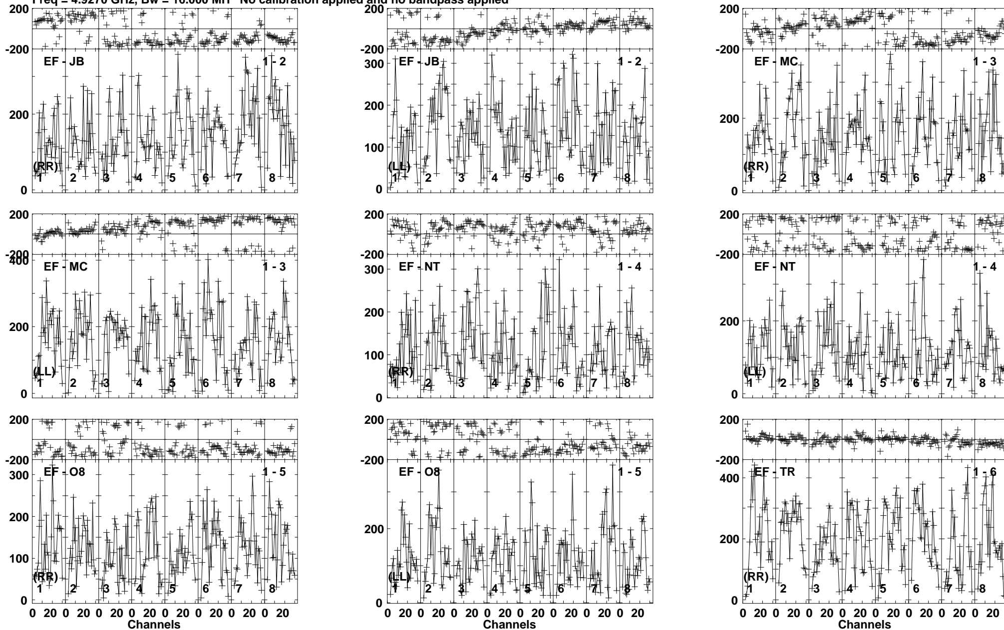
Lower frame: Micro Ampl Jy Top frame: Phas deg Vector averaged cross-power spectrum Baseline: EF (01) - JB (02) Timerange: 01/03/31:11 to 01/03/33:39
