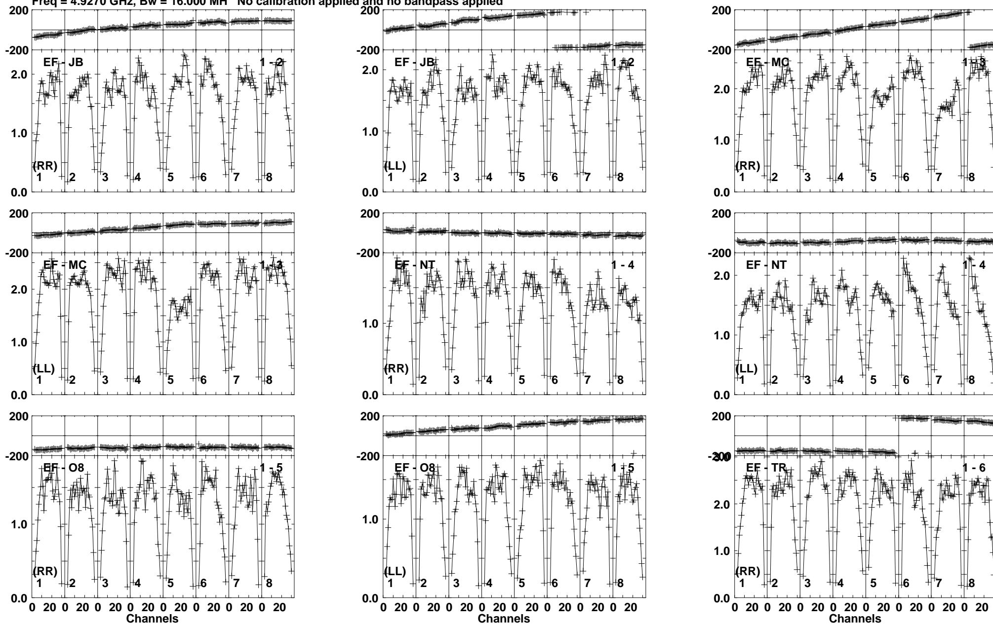
Lower frame: Milli Ampl Jy Top frame: Phas deg Vector averaged cross-power spectrum Baseline: EF (01) - JB (02) Timerange: 01/01:22:21 to 01/01:23:49
