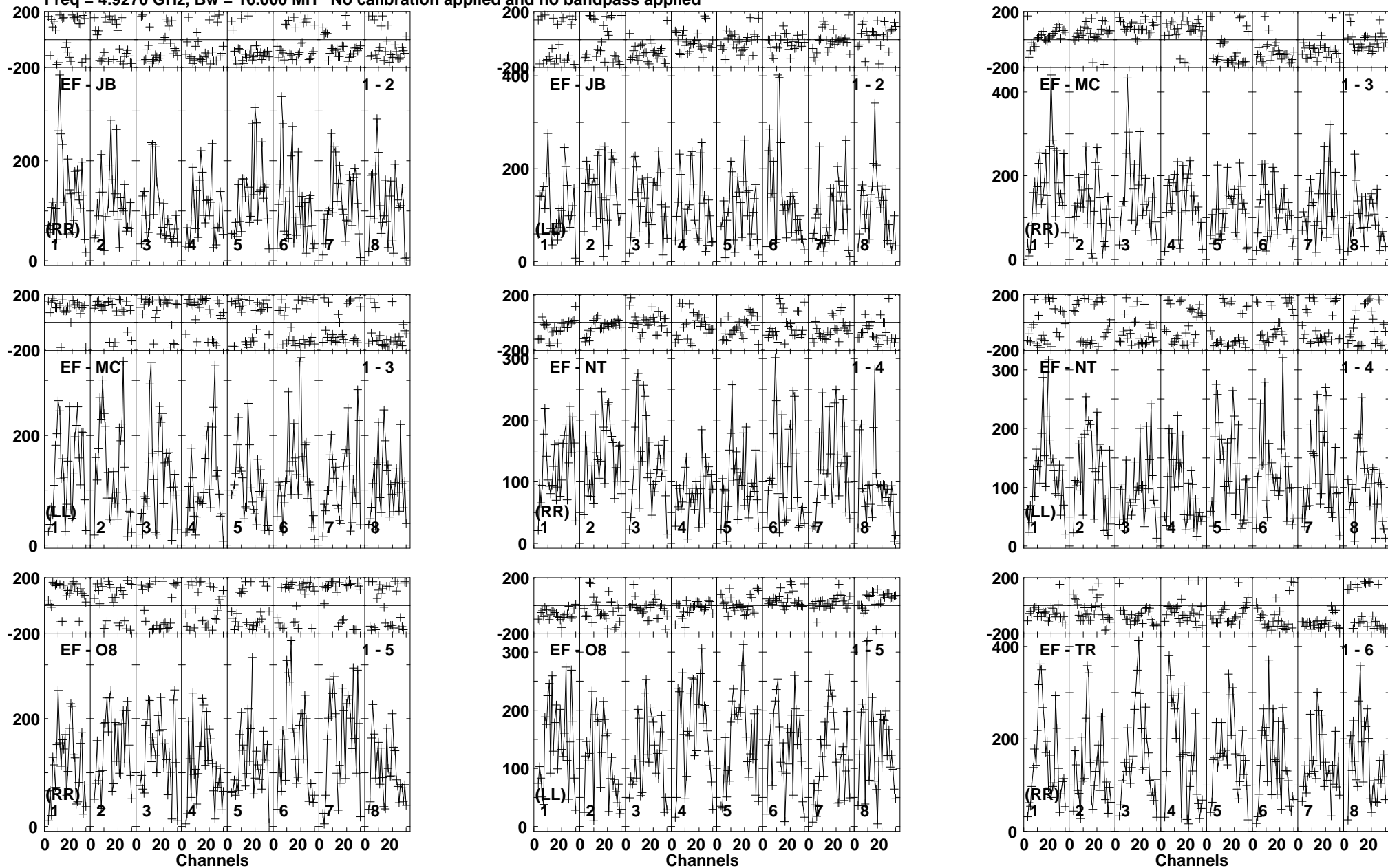
Lower frame: Micro Ampl Jy Top frame: Phas deg Vector averaged cross-power spectrum Baseline: EF (01) - JB (02) Timerange: 00/21:25:51 to 00/21:28:20
