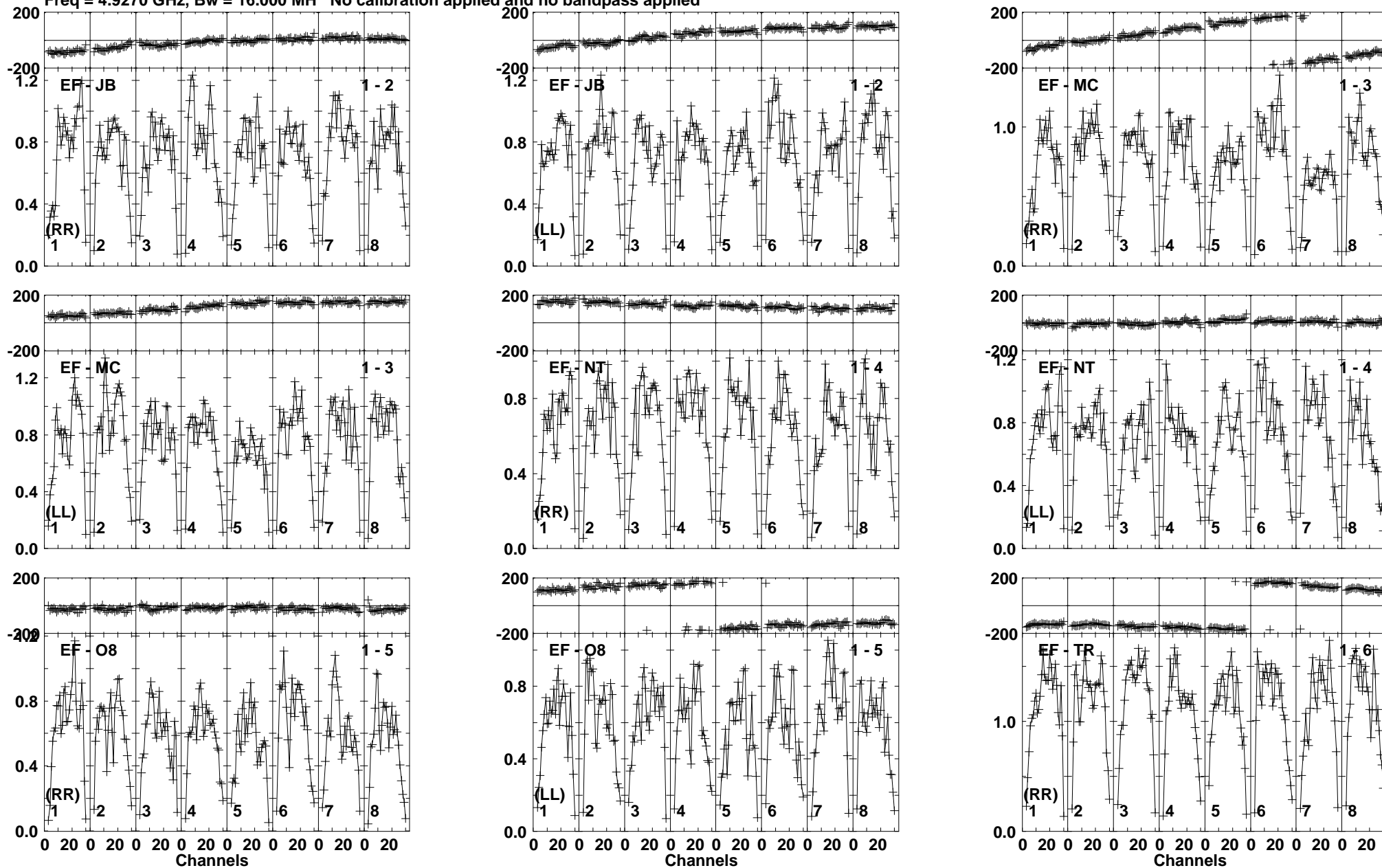
Lower frame: Milli Ampl Jy Top frame: Phas deg Vector averaged cross-power spectrum Baseline: EF (01) - JB (02) Timerange: 00:19:53:01 to 00:19:54:30
