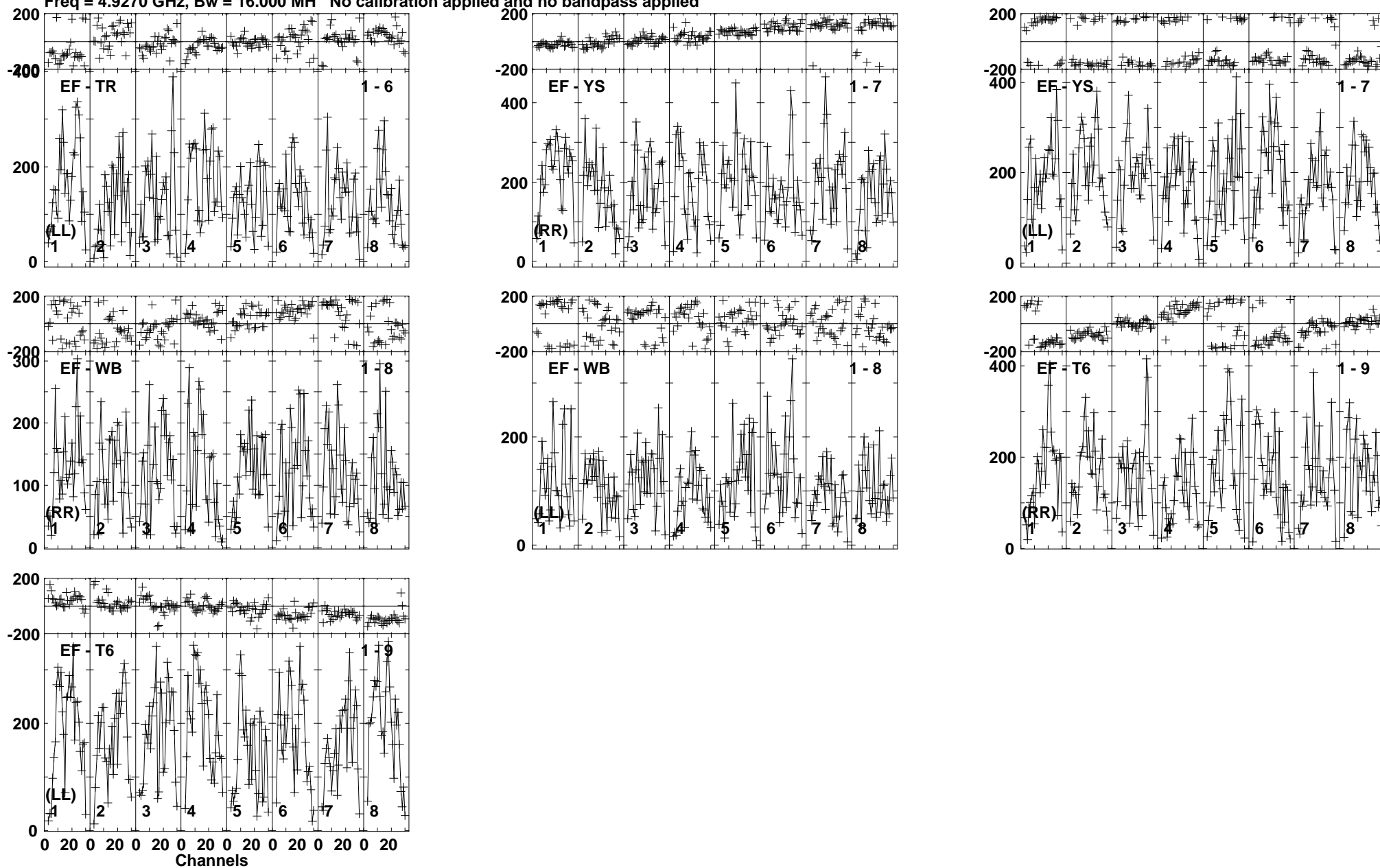
Lower frame: Micro Ampl Jy Top frame: Phas deg Vector averaged cross-power spectrum Baseline: EF (01) - TR (06) Timerange: 00/21:31:50 to 00/21:34:19
