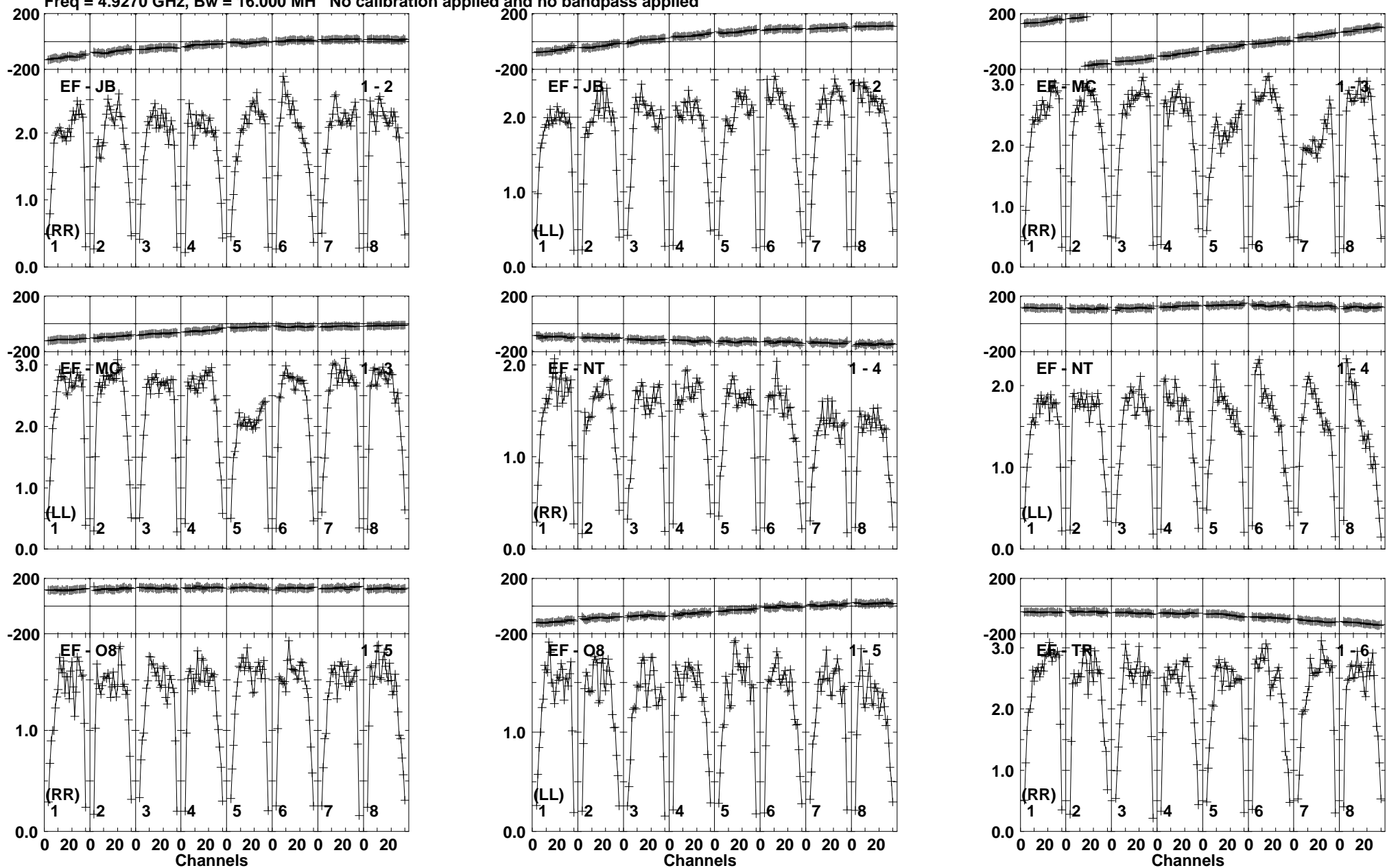
Lower frame: Milli Ampl Jy Top frame: Phas deg Vector averaged cross-power spectrum Baseline: EF (01) - JB (02) Timerange: 00/21:59:40 to 00/22:01:10
