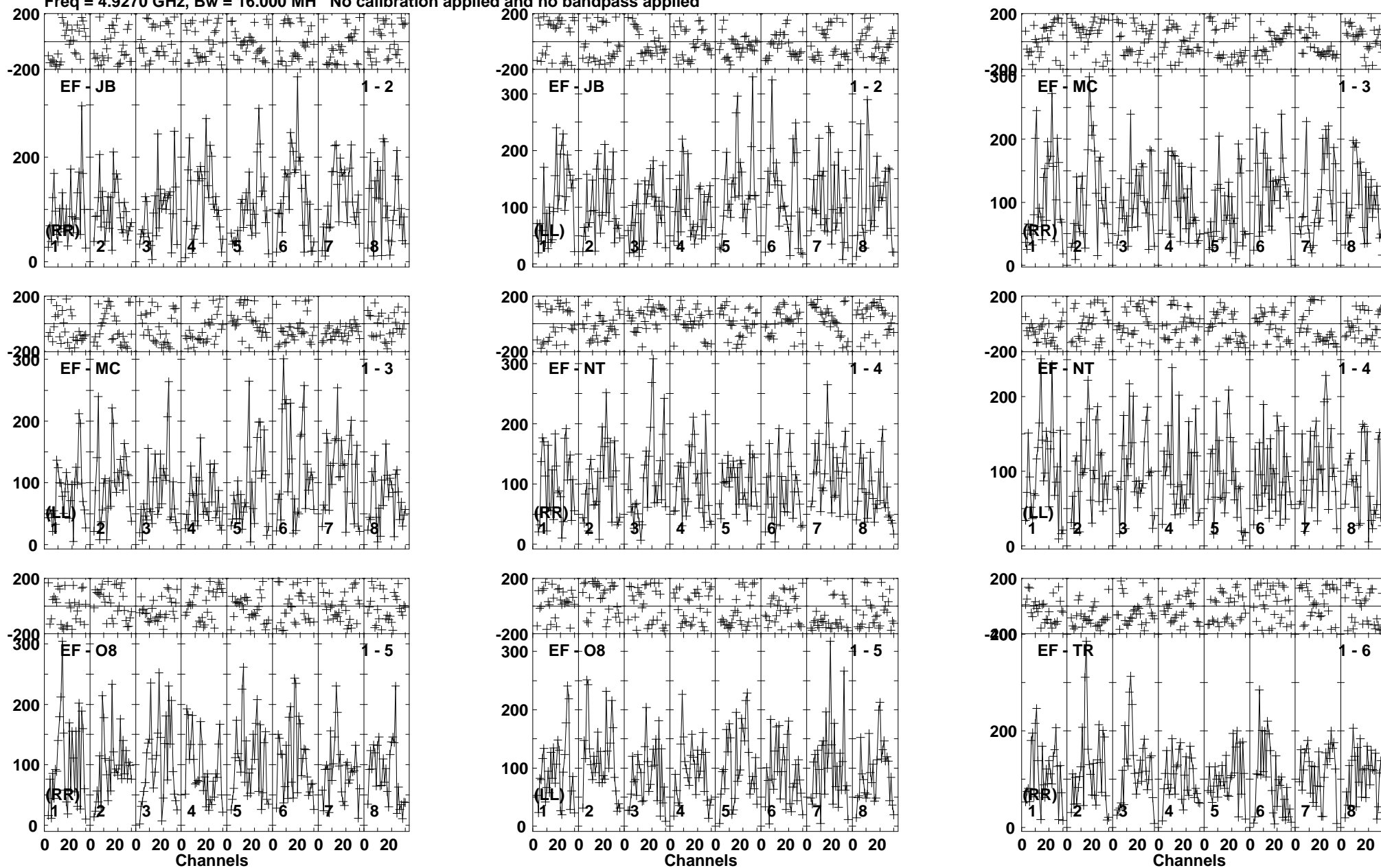
Lower frame: Micro Ampl Jy Top frame: Phas deg Vector averaged cross-power spectrum Baseline: EF (01) - JB (02) Timerange: 00/19:25:11 to 00/19:27:39
