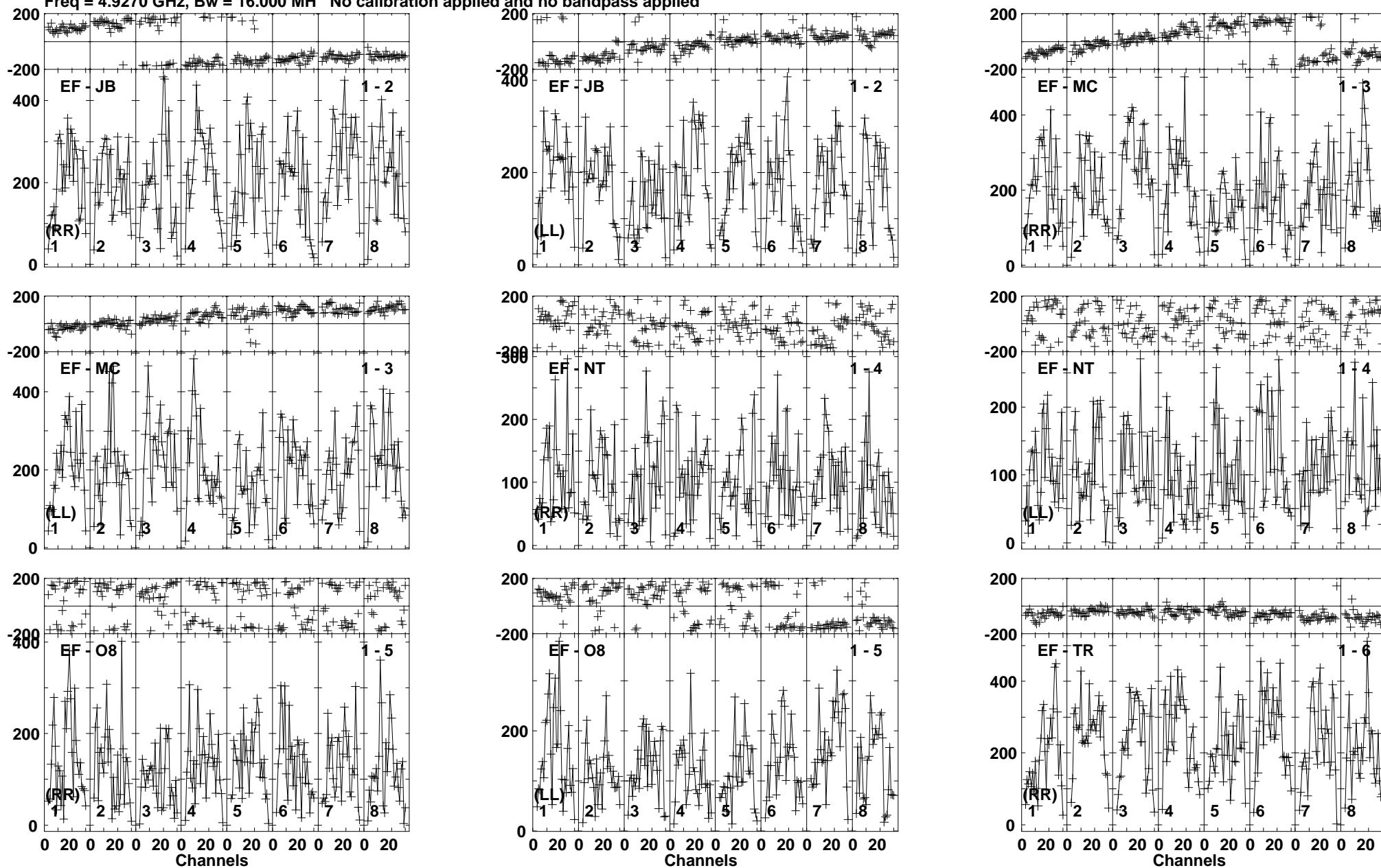
Lower frame: Micro Ampl Jy Top frame: Phas deg Vector averaged cross-power spectrum Baseline: EF (01) - JB (02) Timerange: 01/03:23:10 to 01/03:25:10
