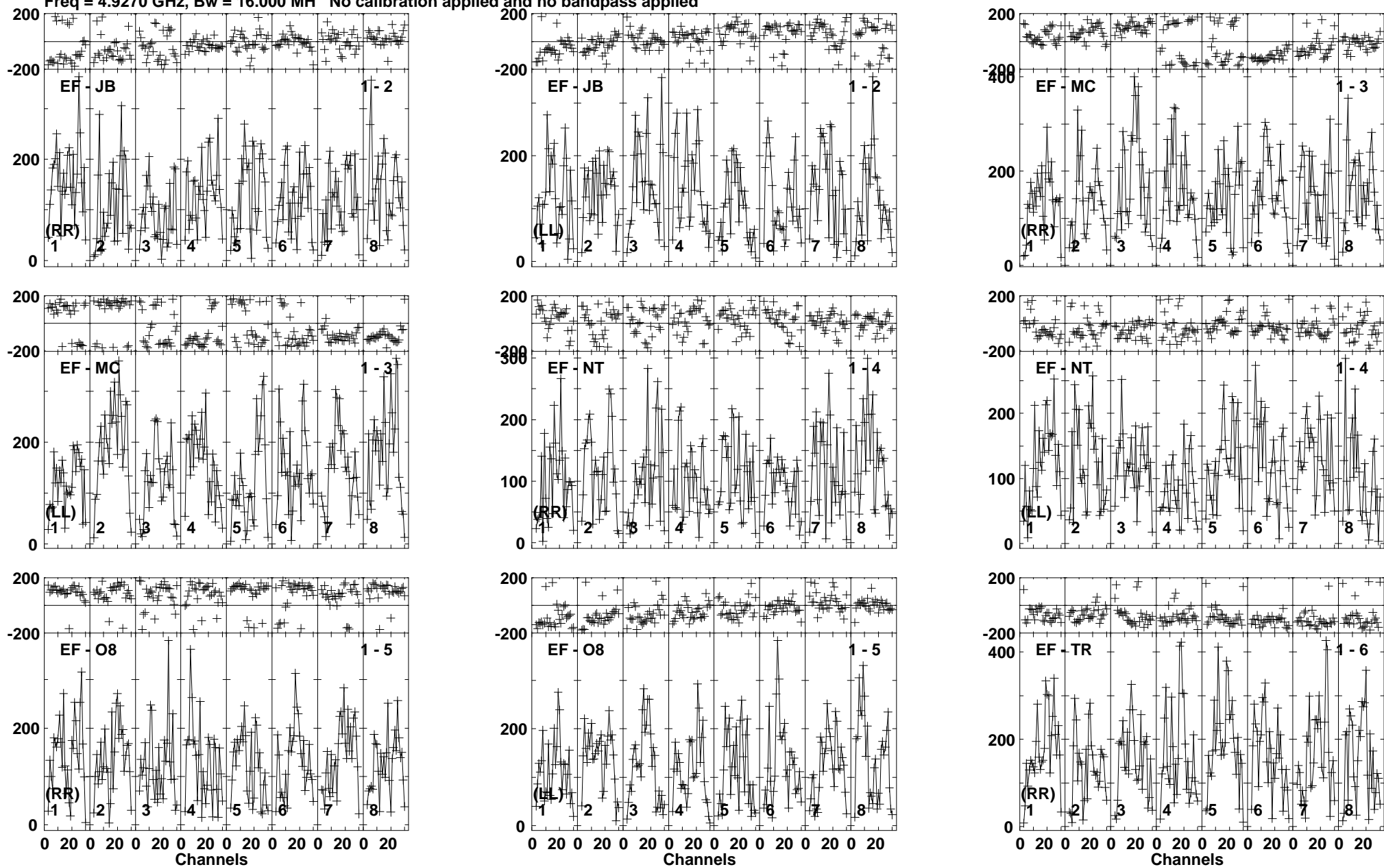
Lower frame: Micro Ampl Jy Top frame: Phas deg Vector averaged cross-power spectrum Baseline: EF (01) - JB (02) Timerange: 00/23:32:31 to 00/23:35:00
