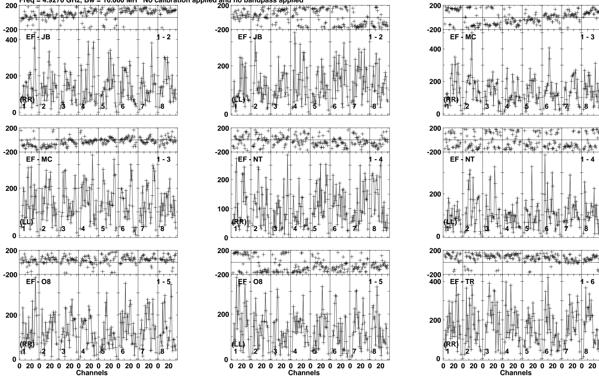
Lower frame: Micro Ampl Jy Top frame: Phas deg Vector averaged cross-power spectrum Baseline: EF (01) - JB (02) Timerange: 00:22:47:50 to 00:22:50:19
