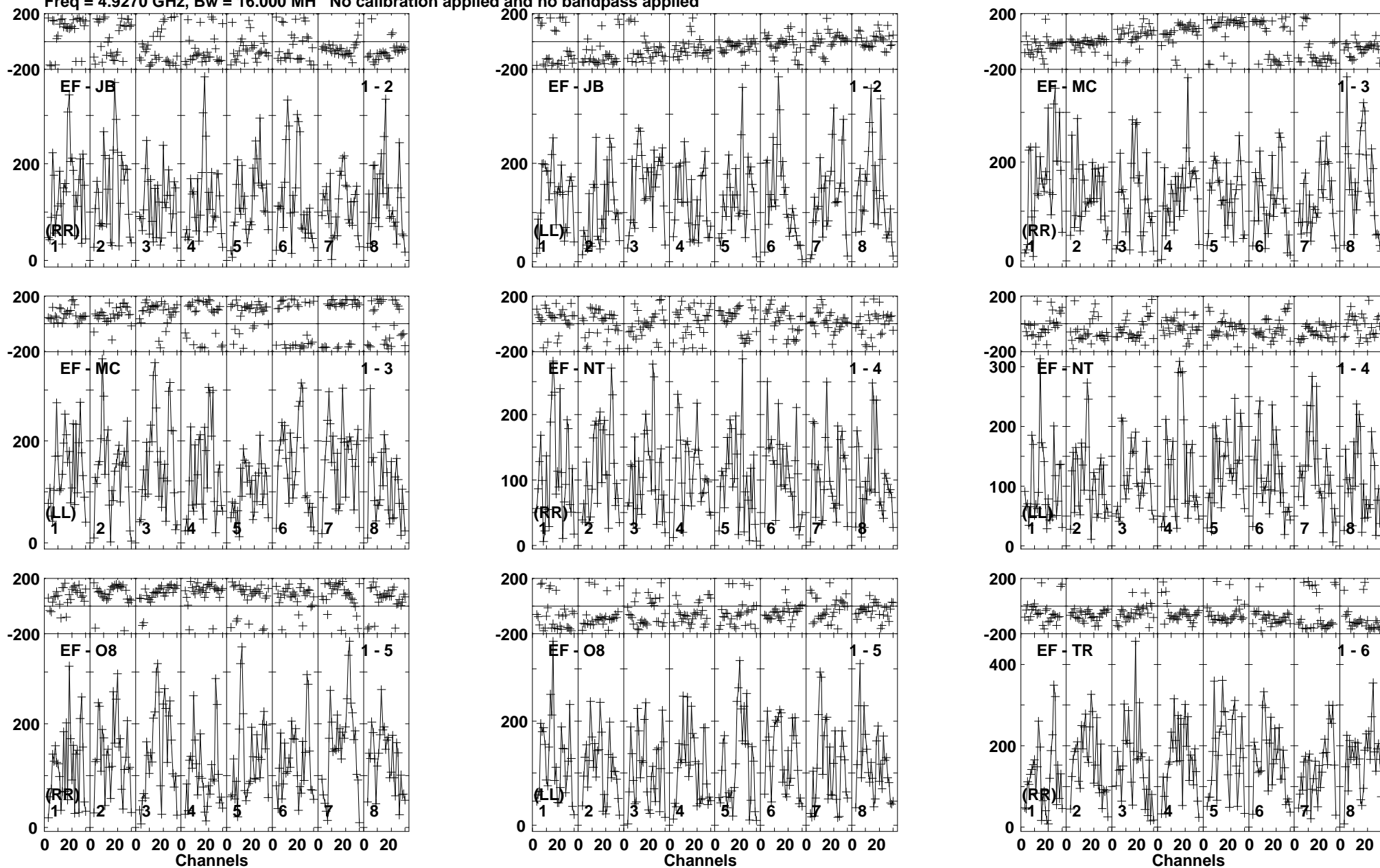
Lower frame: Micro Ampl Jy Top frame: Phas deg Vector averaged cross-power spectrum Baseline: EF (01) - JB (02) Timerange: 00/23:19:51 to 00/23:22:19
