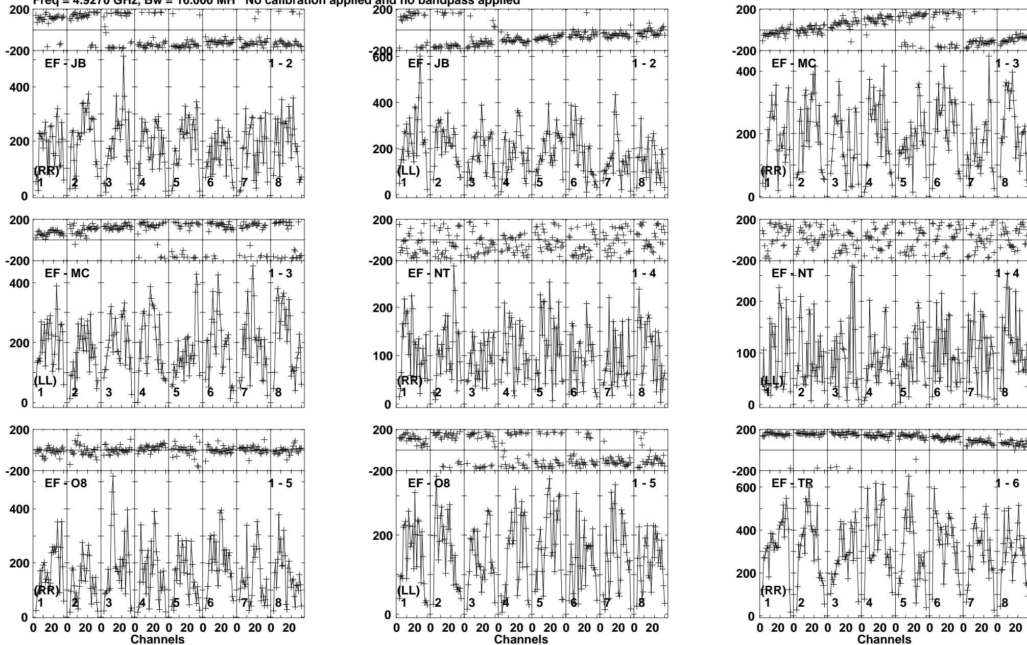
Lower frame: Micro Ampl Jy Top frame: Phas deg Vector averaged cross-power spectrum Baseline: EF (01) - JB (02) Timerange: 00/20:45:50 to 00/20:47:49
