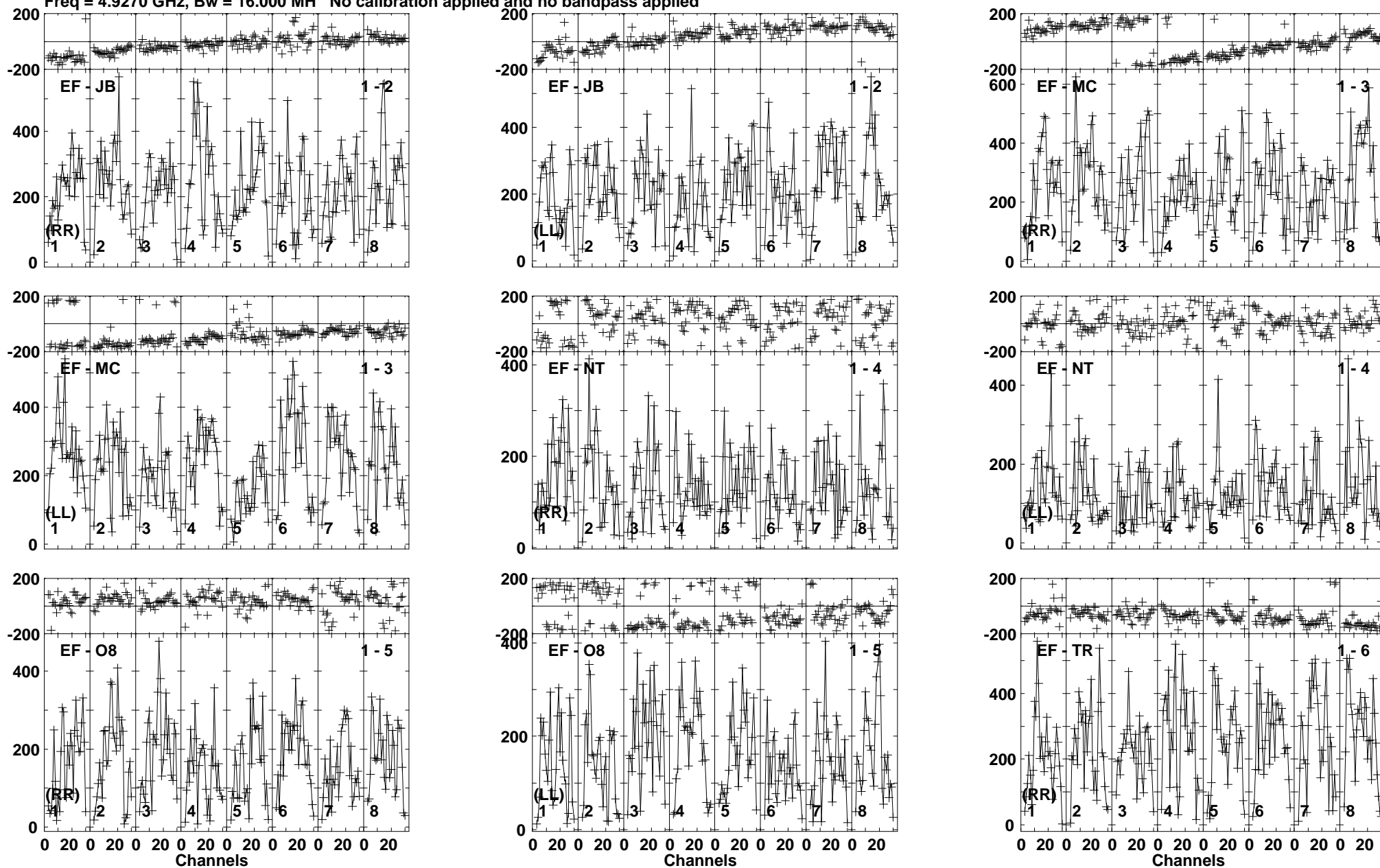
Lower frame: Micro Ampl Jy Top frame: Phas deg Vector averaged cross-power spectrum Baseline: EF (01) - JB (02) Timerange: 00/23:36:30 to 00/23:38:30
