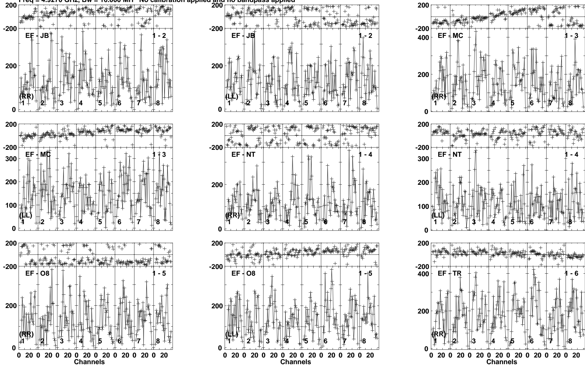
Lower frame: Micro Ampl Jy Top frame: Phas deg Vector averaged cross-power spectrum Baseline: EF (01) - JB (02) Timerange: 01/00:10:30 to 01/00:13:00
