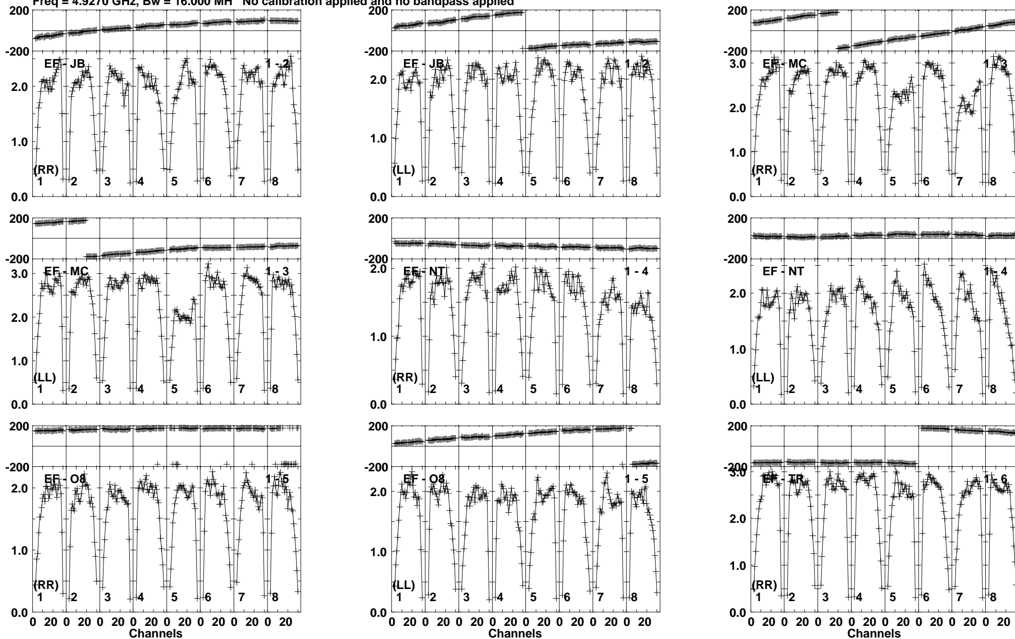
Lower frame: Milli Ampl Jy Top frame: Phas deg Vector averaged cross-power spectrum Baseline: EF (01) - JB (02) Timerange: 01/02:49:21 to 01/02:50:50
