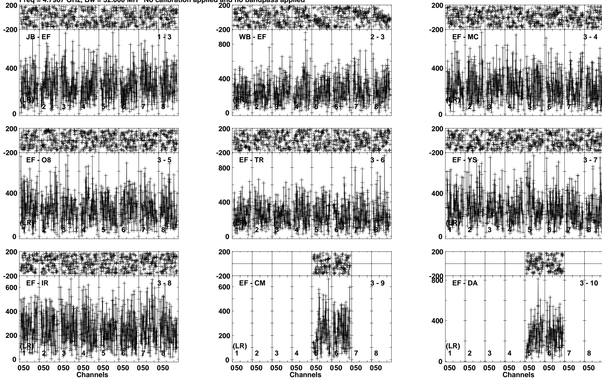
Lower frame: Micro Ampl Jy Top frame: Phas deg Vector averaged cross-power spectrum Baseline: JB (01) - EF (03) Timerange: 01/03:17:50 to 01/03:20:20
