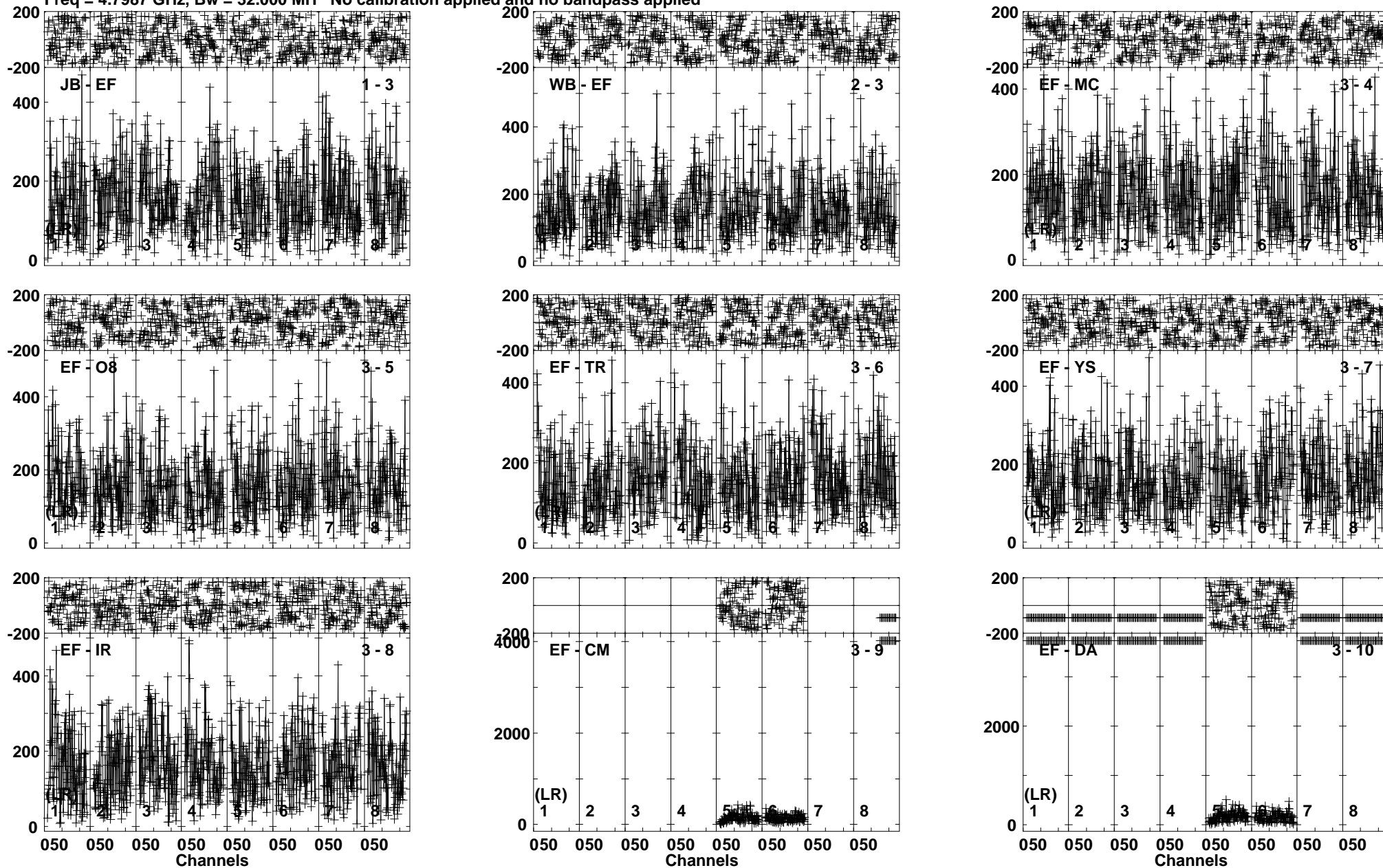
Lower frame: Micro Ampl Jy Top frame: Phas deg Vector averaged cross-power spectrum Baseline: JB (01) - EF (03) Timerange: 01/08:43:30 to 01/08:46:00
