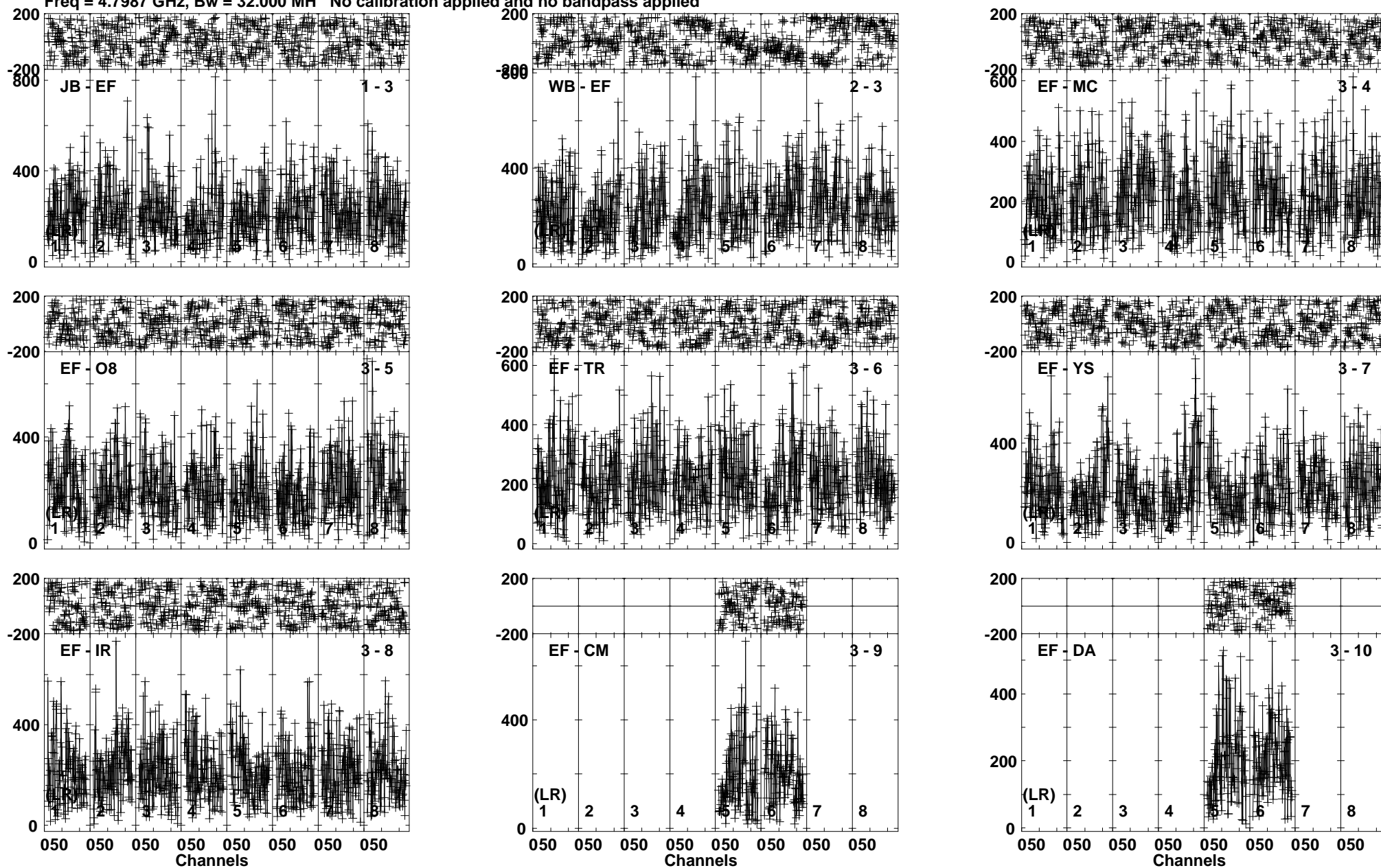
Lower frame: Micro Ampl Jy Top frame: Phas deg Vector averaged cross-power spectrum Baseline: JB (01) - EF (03) Timerange: 01/02:13:21 to 01/02:15:50
