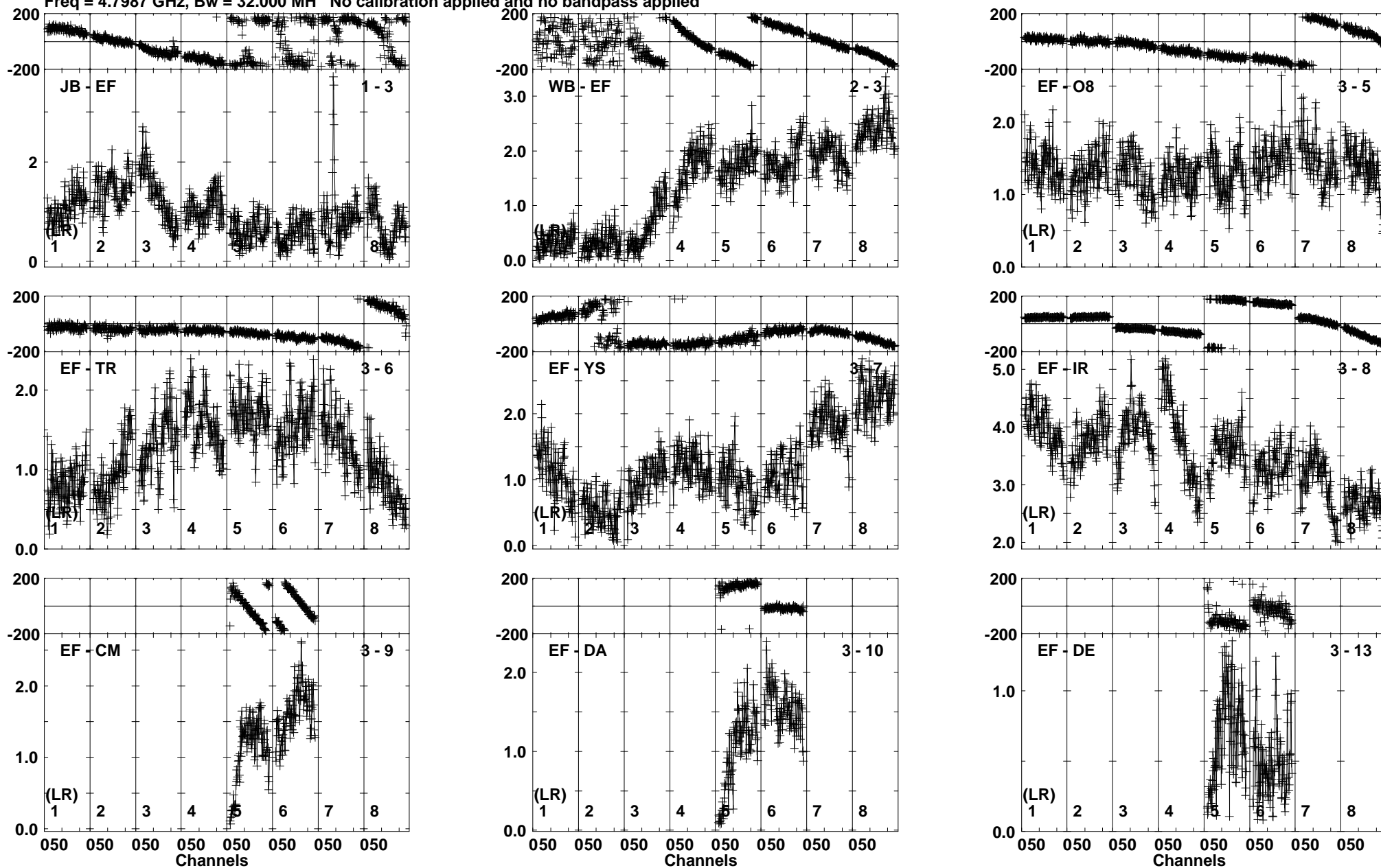
Lower frame: Milli Ampl Jy Top frame: Phas deg Vector averaged cross-power spectrum Baseline: JB (01) - EF (03) Timerange: 01/06:09:10 to 01/06:10:39
