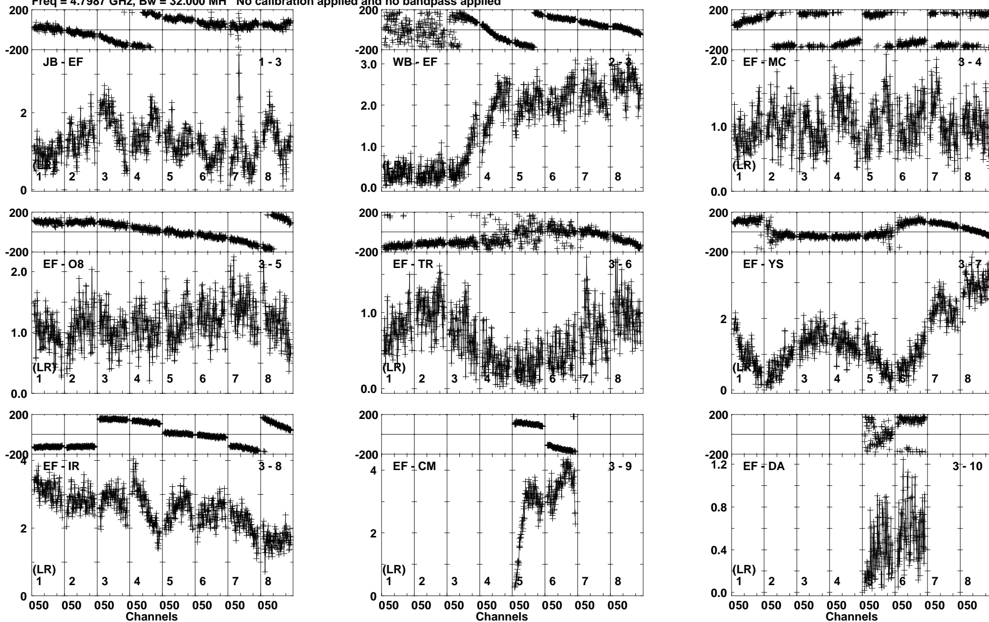
Lower frame: Milli Ampl Jy Top frame: Phas deg Vector averaged cross-power spectrum Baseline: JB (01) - EF (03) Timerange: 01/02:05:41 to 01/02:07:09
