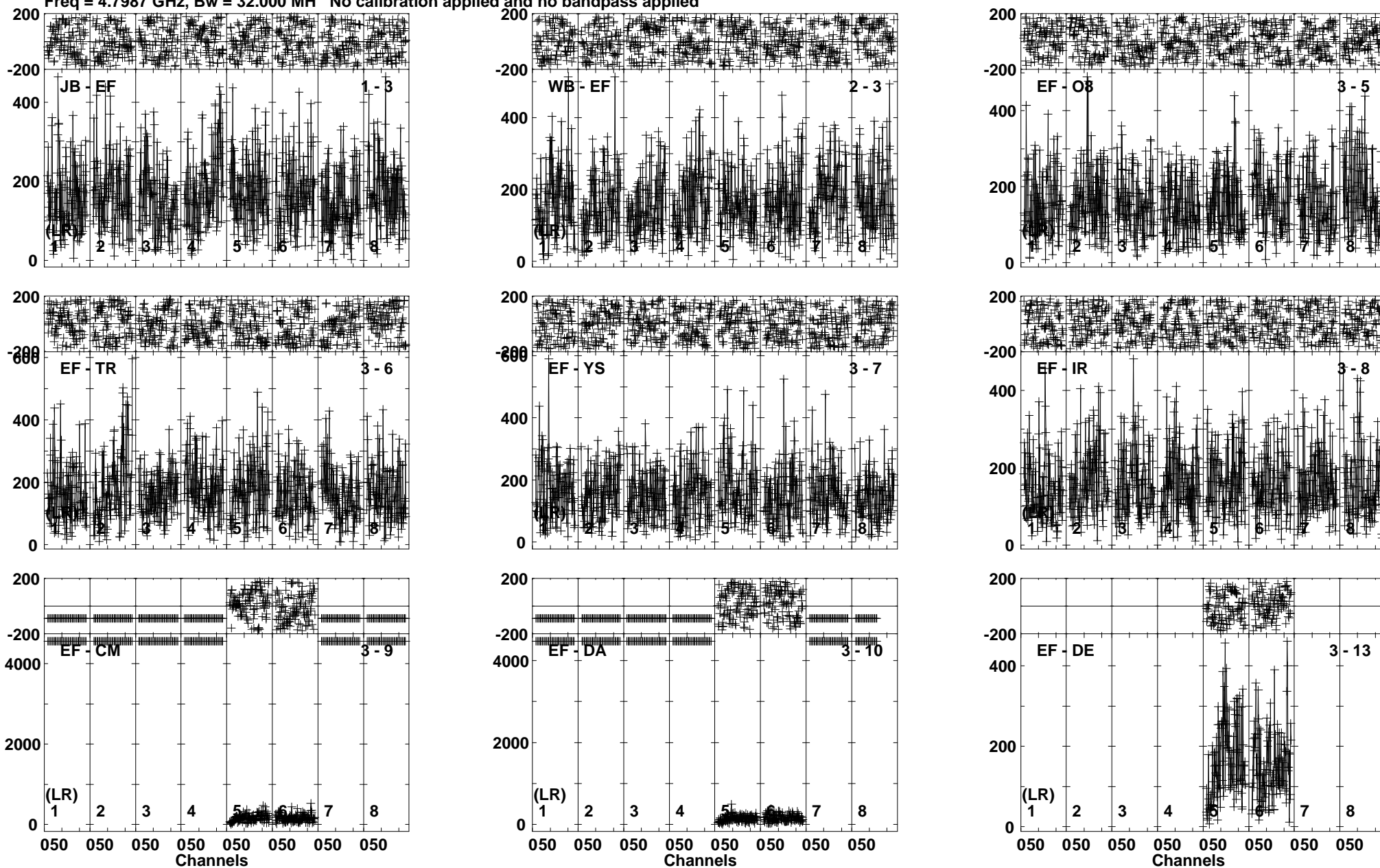
Lower frame: Micro Ampl Jy Top frame: Phas deg Vector averaged cross-power spectrum Baseline: JB (01) - EF (03) Timerange: 01/06:10:40 to 01/06:13:10
