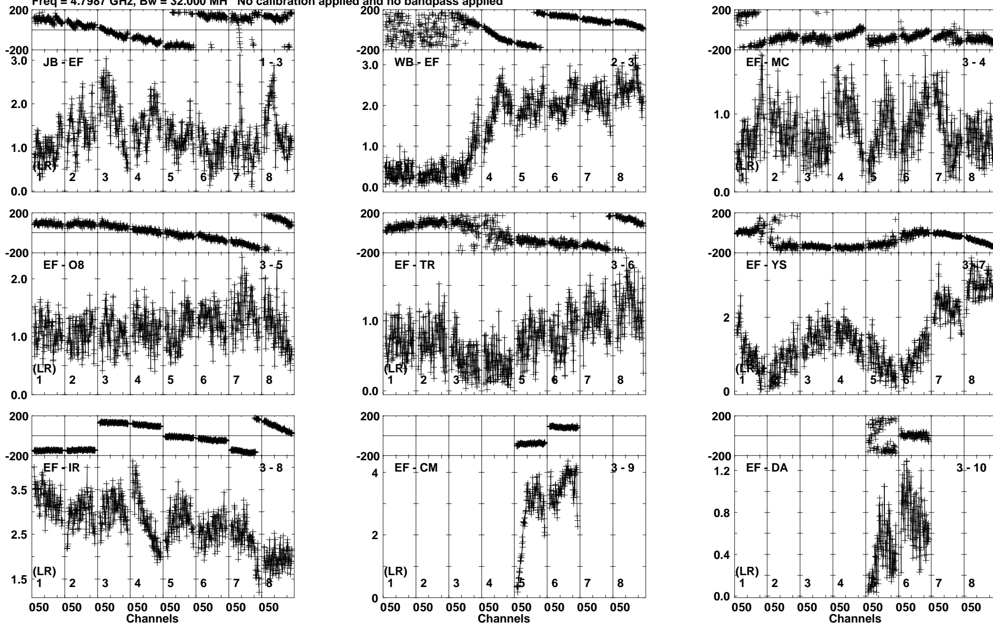
Lower frame: Milli Ampl Jy Top frame: Phas deg Vector averaged cross-power spectrum Baseline: JB (01) - EF (03) Timerange: 01/00:42:11 to 01/00:43:39
