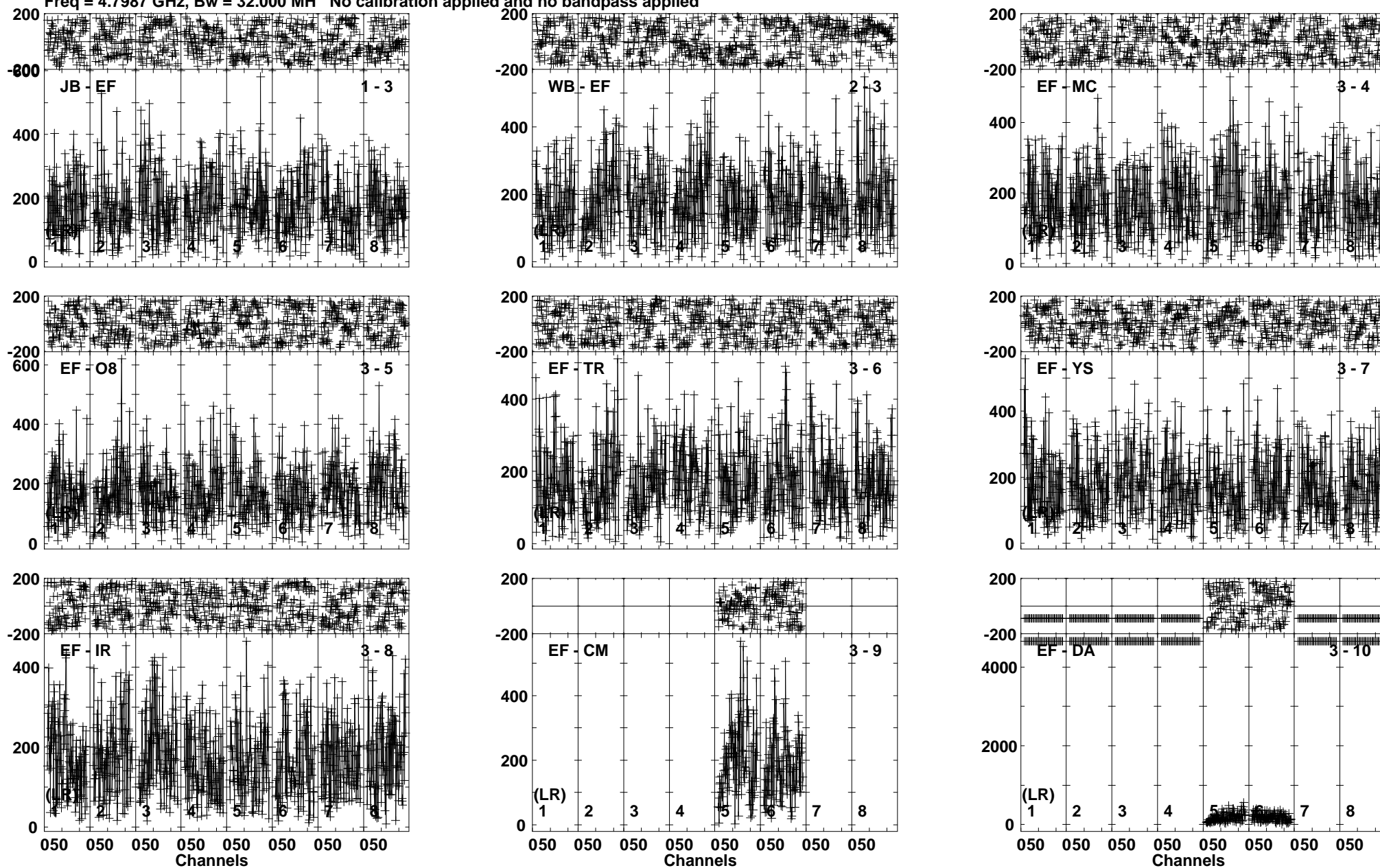
Lower frame: Micro Ampl Jy Top frame: Phas deg Vector averaged cross-power spectrum Baseline: JB (01) - EF (03) Timerange: 01/00:07:50 to 01/00:10:19
