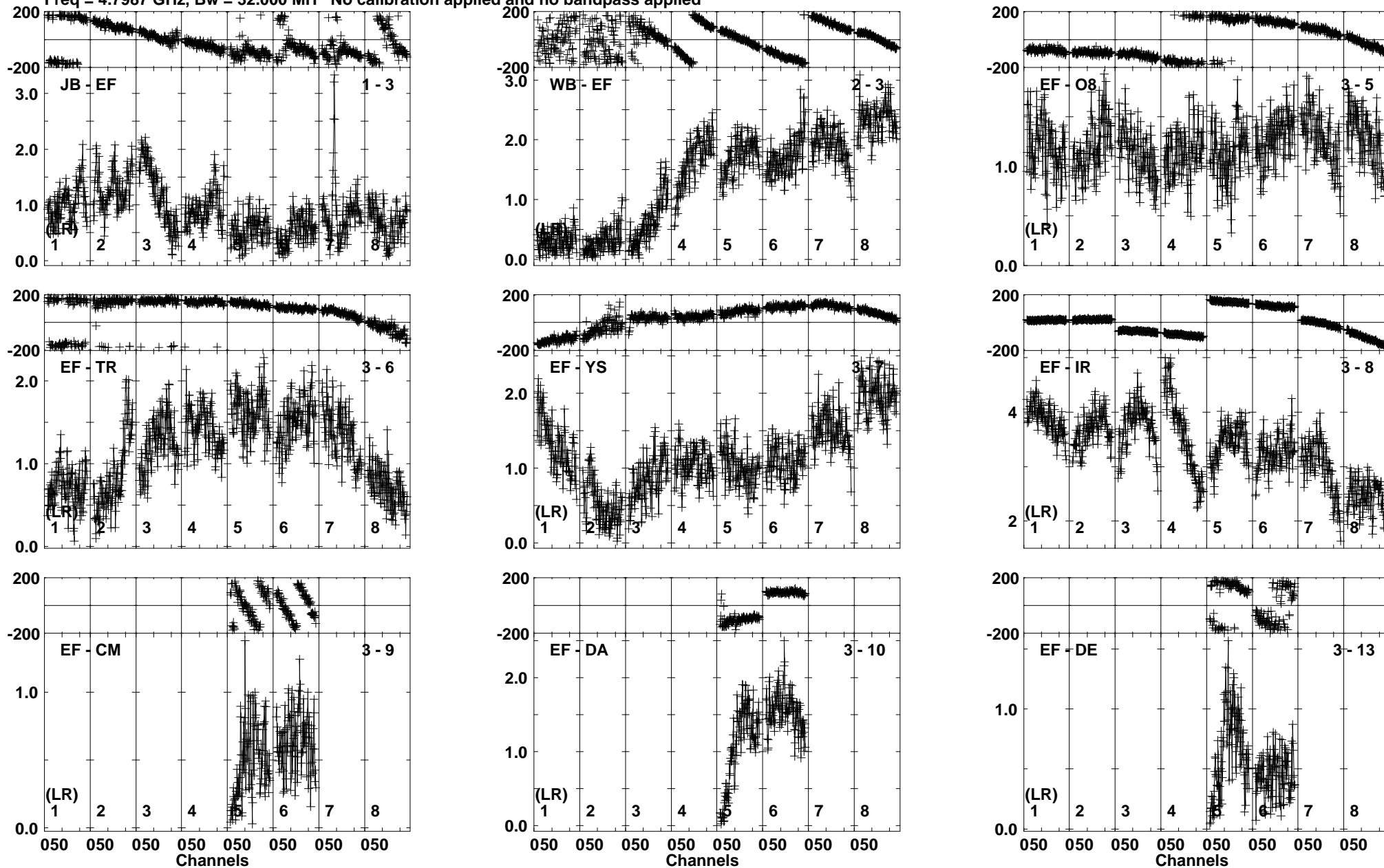
Lower frame: Milli Ampl Jy Top frame: Phas deg Vector averaged cross-power spectrum Baseline: JB (01) - EF (03) Timerange: 01/07:04:50 to 01/07:06:19
