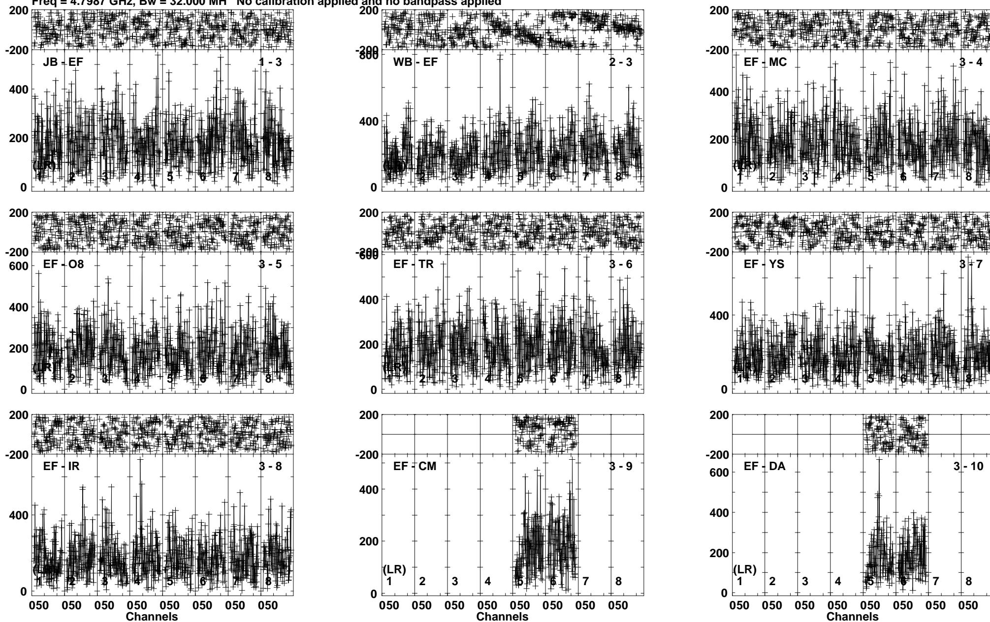
Lower frame: Micro Ampl Jy Top frame: Phas deg Vector averaged cross-power spectrum Baseline: JB (01) - EF (03) Timerange: 01/02:27:01 to 01/02:29:29
