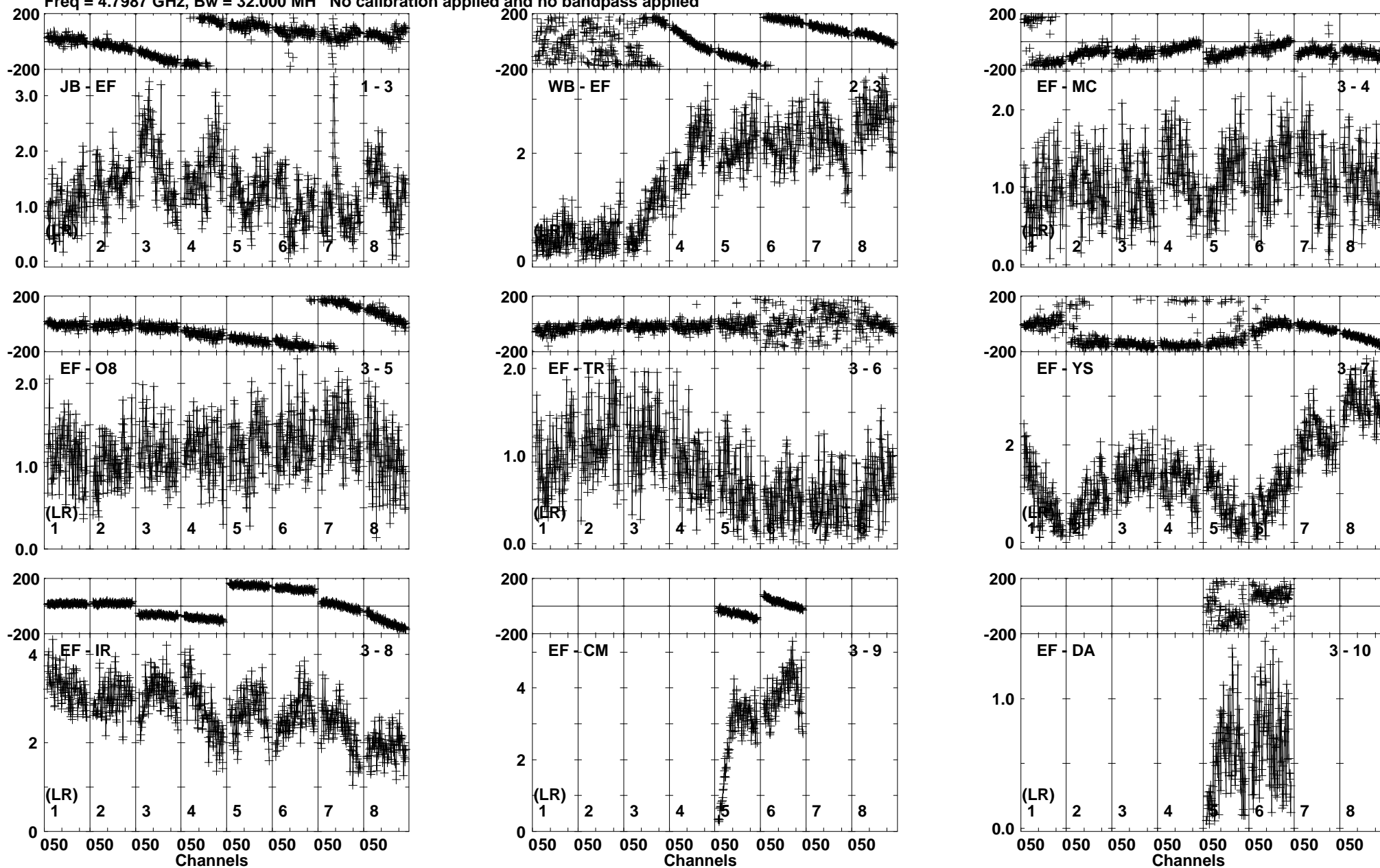
Lower frame: Milli Ampl Jy Top frame: Phas deg Vector averaged cross-power spectrum Baseline: JB (01) - EF (03) Timerange: 01/02:39:40 to 01/02:41:09
