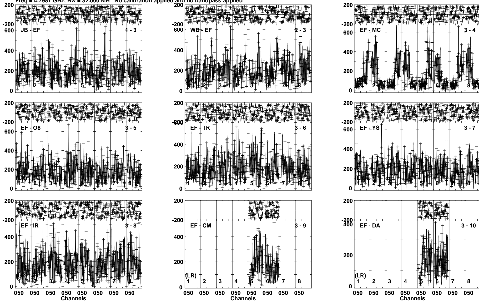
Lower frame: Micro Ampl Jy Top frame: Phas deg Vector averaged cross-power spectrum Baseline: JB (01) - EF (03) Timerange: 01/05:15:00 to 01/05:17:30
