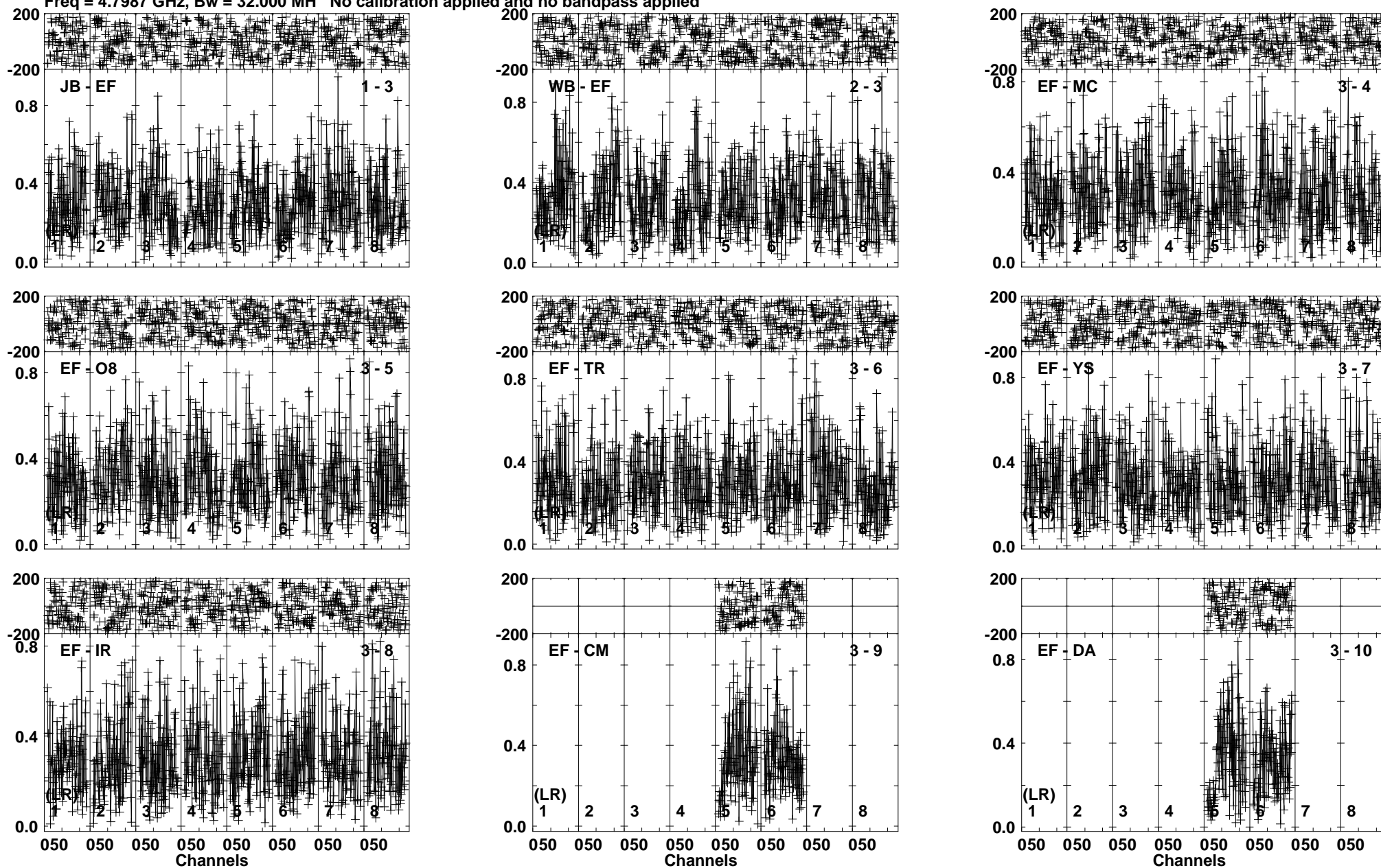
Lower frame: Milli Ampl Jy Top frame: Phas deg Vector averaged cross-power spectrum Baseline: JB (01) - EF (03) Timerange: 01/04:09:30 to 01/04:12:00
