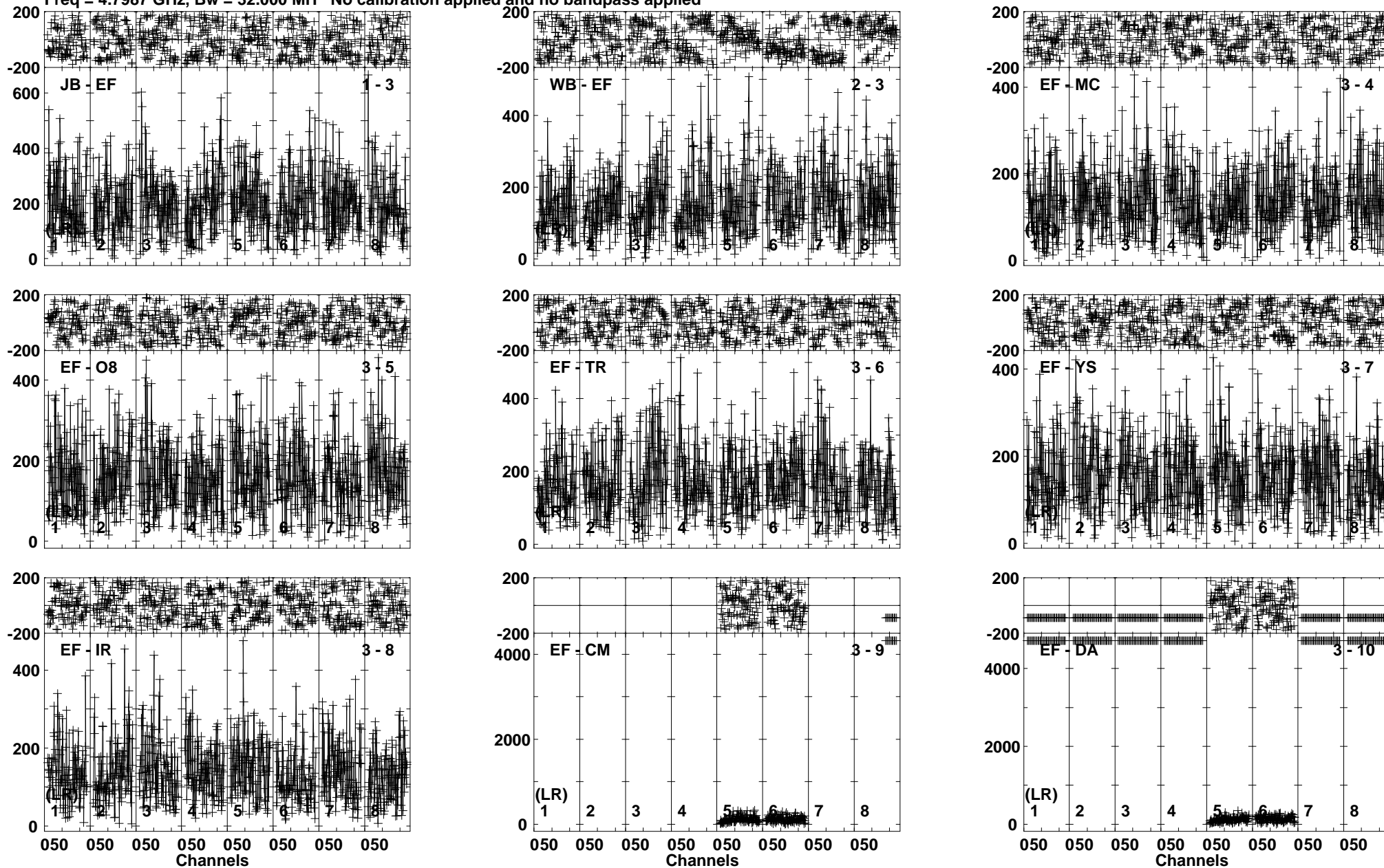
Lower frame: Micro Ampl Jy Top frame: Phas deg Vector averaged cross-power spectrum Baseline: JB (01) - EF (03) Timerange: 01/03:26:40 to 01/03:29:10
