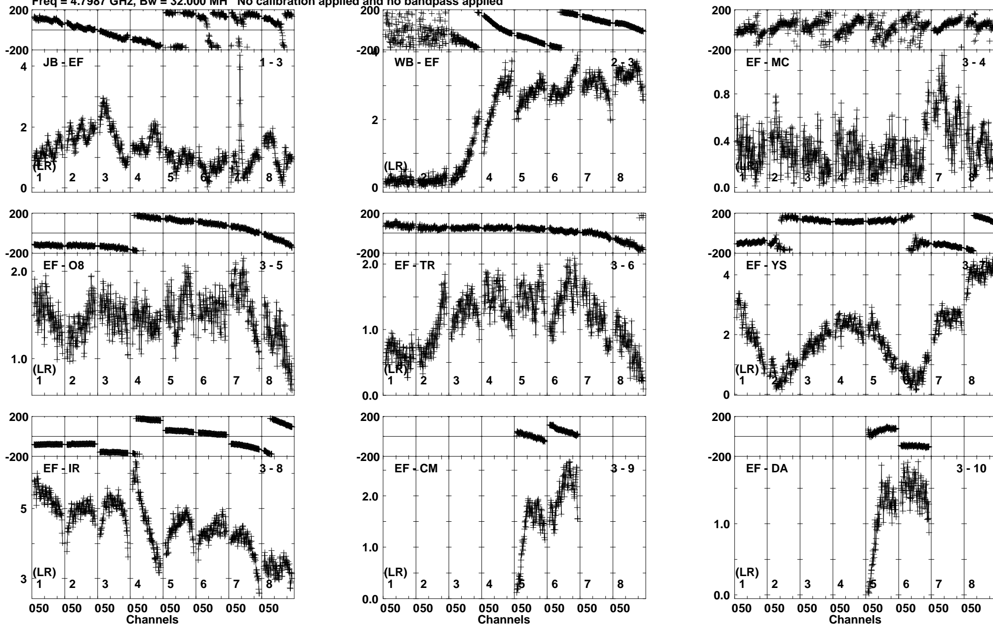
Lower frame: Milli Ampl Jy Top frame: Phas deg Vector averaged cross-power spectrum Baseline: JB (01) - EF (03) Timerange: 01/03:03:31 to 01/03:04:59
