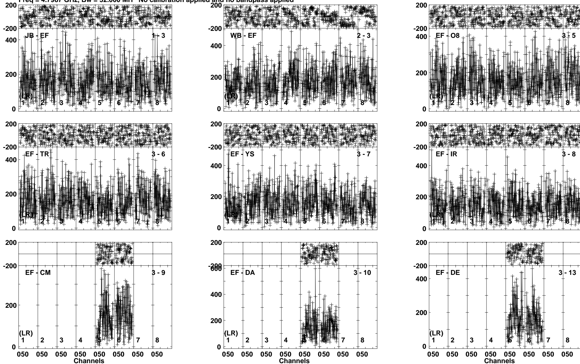
Lower frame: Micro Ampl Jy Top frame: Phas deg Vector averaged cross-power spectrum Baseline: JB (01) - EF (03) Timerange: 01/07:15:10 to 01/07:17:39
