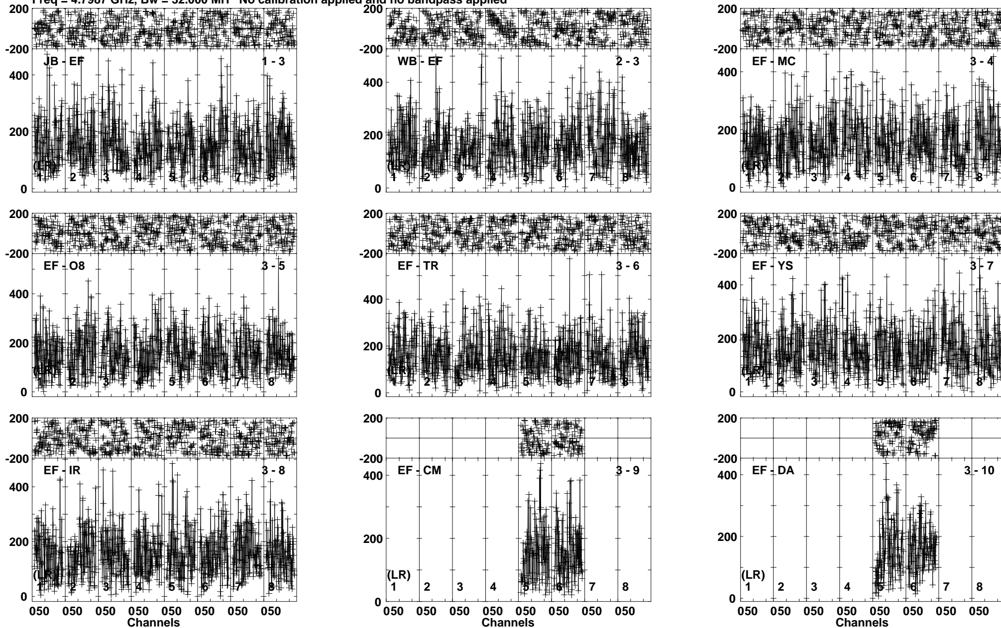
Lower frame: Micro Ampl Jy Top frame: Phas deg Vector averaged cross-power spectrum Baseline: JB (01) - EF (03) Timerange: 01/08:34:40 to 01/08:37:10
