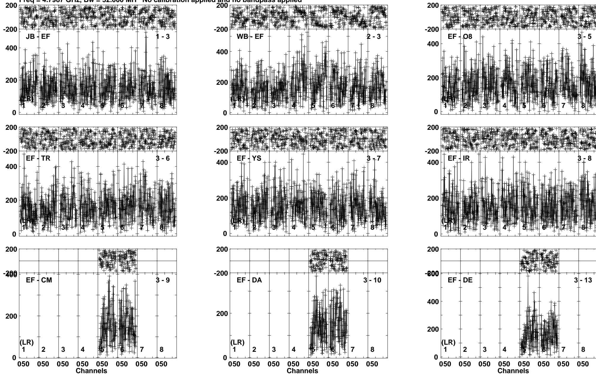
Lower frame: Micro Ampl Jy Top frame: Phas deg Vector averaged cross-power spectrum Baseline: JB (01) - EF (03) Timerange: 01/08:15:40 to 01/08:18:10
