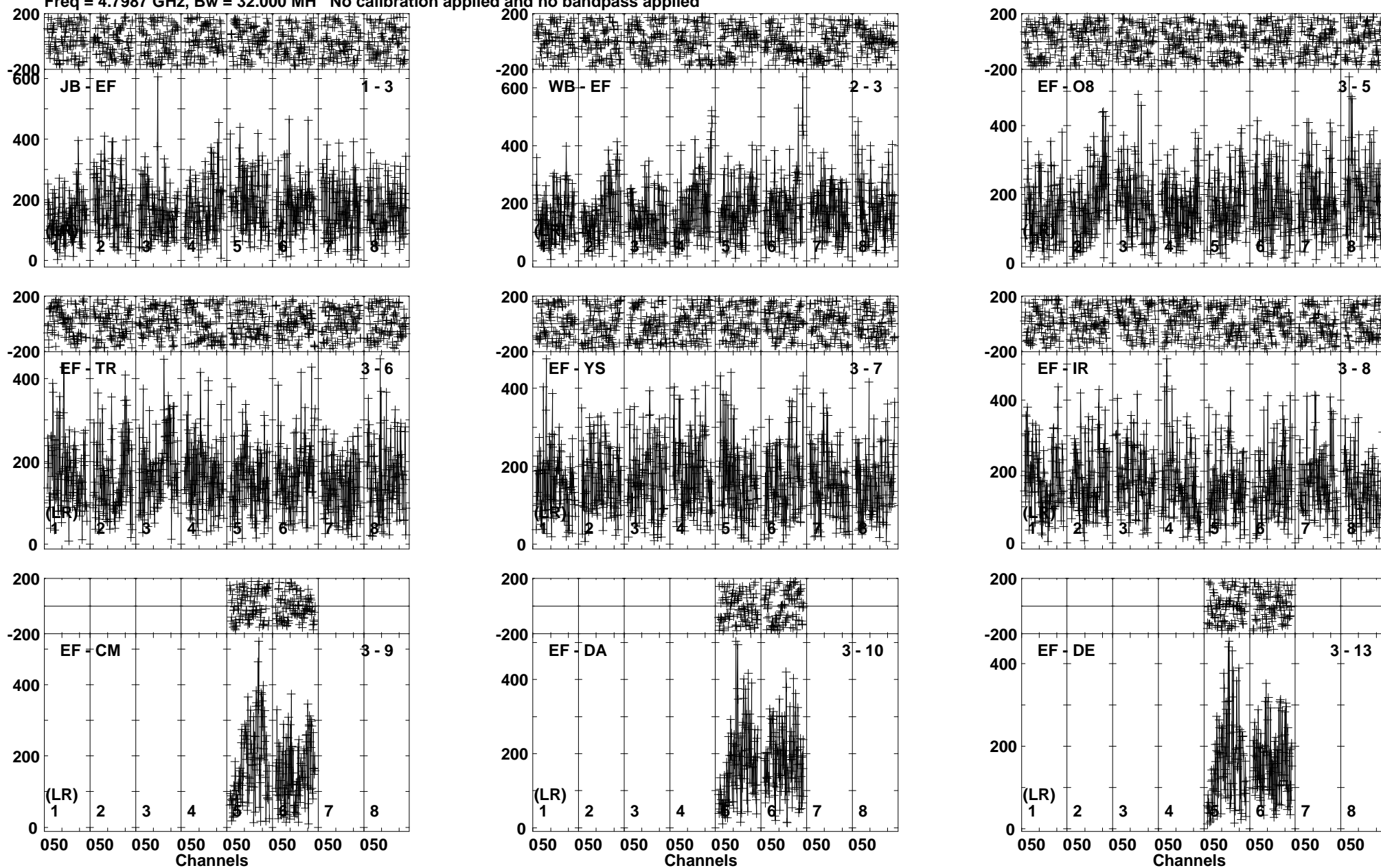
Lower frame: Micro Ampl Jy Top frame: Phas deg Vector averaged cross-power spectrum Baseline: JB (01) - EF (03) Timerange: 01/06:38:30 to 01/06:41:00
