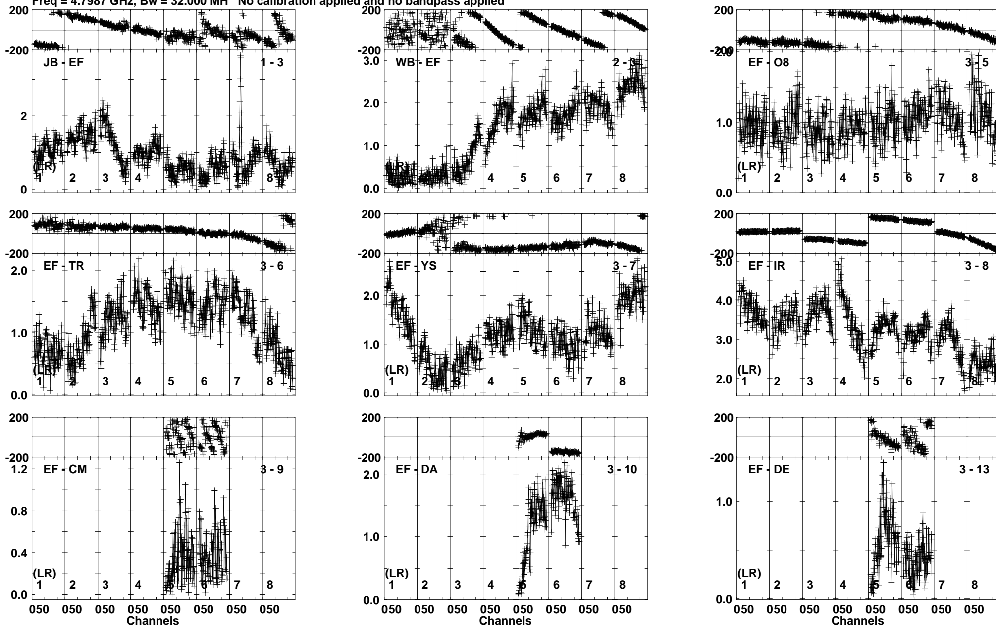
Lower frame: Milli Ampl Jy Top frame: Phas deg Vector averaged cross-power spectrum Baseline: JB (01) - EF (03) Timerange: 01/08:22:11 to 01/08:23:39
