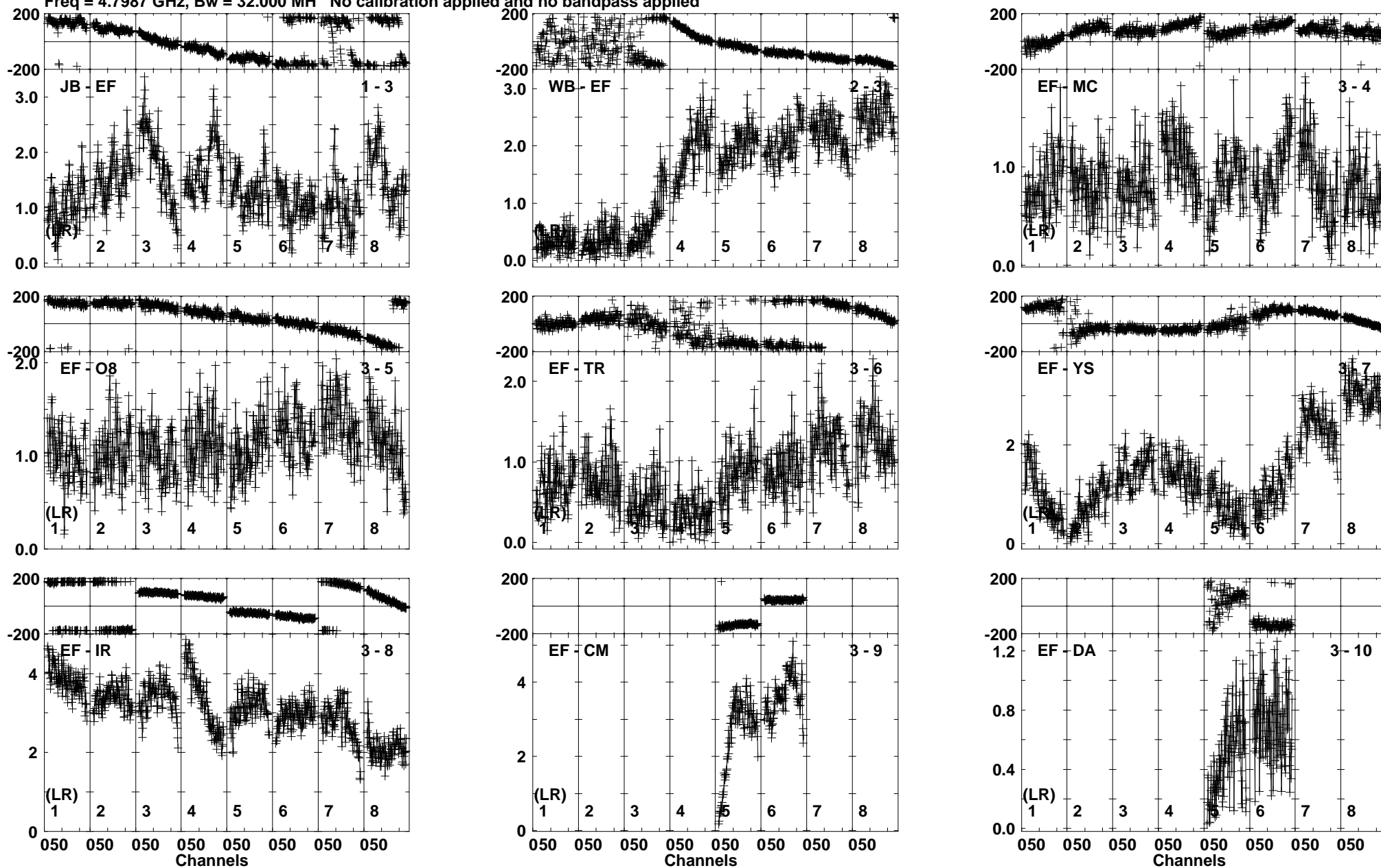
Lower frame: Milli Ampl Jy Top frame: Phas deg Vector averaged cross-power spectrum Baseline: JB (01) - EF (03) Timerange: 01/00:01:31 to 01/00:03:00
