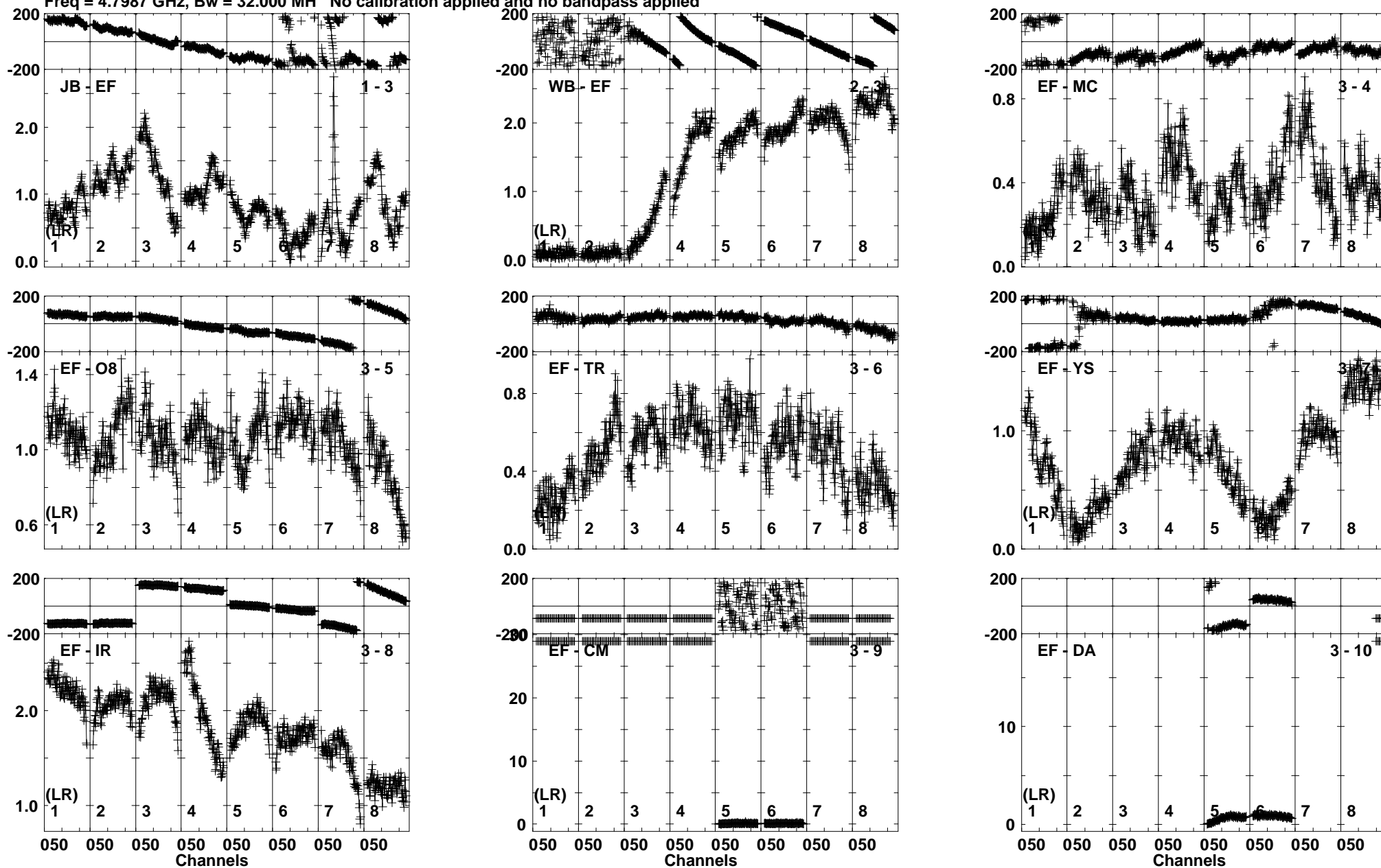
Lower frame: Milli Ampl Jy Top frame: Phas deg Vector averaged cross-power spectrum Baseline: JB (01) - EF (03) Timerange: 01/09:25:31 to 01/09:29:59
