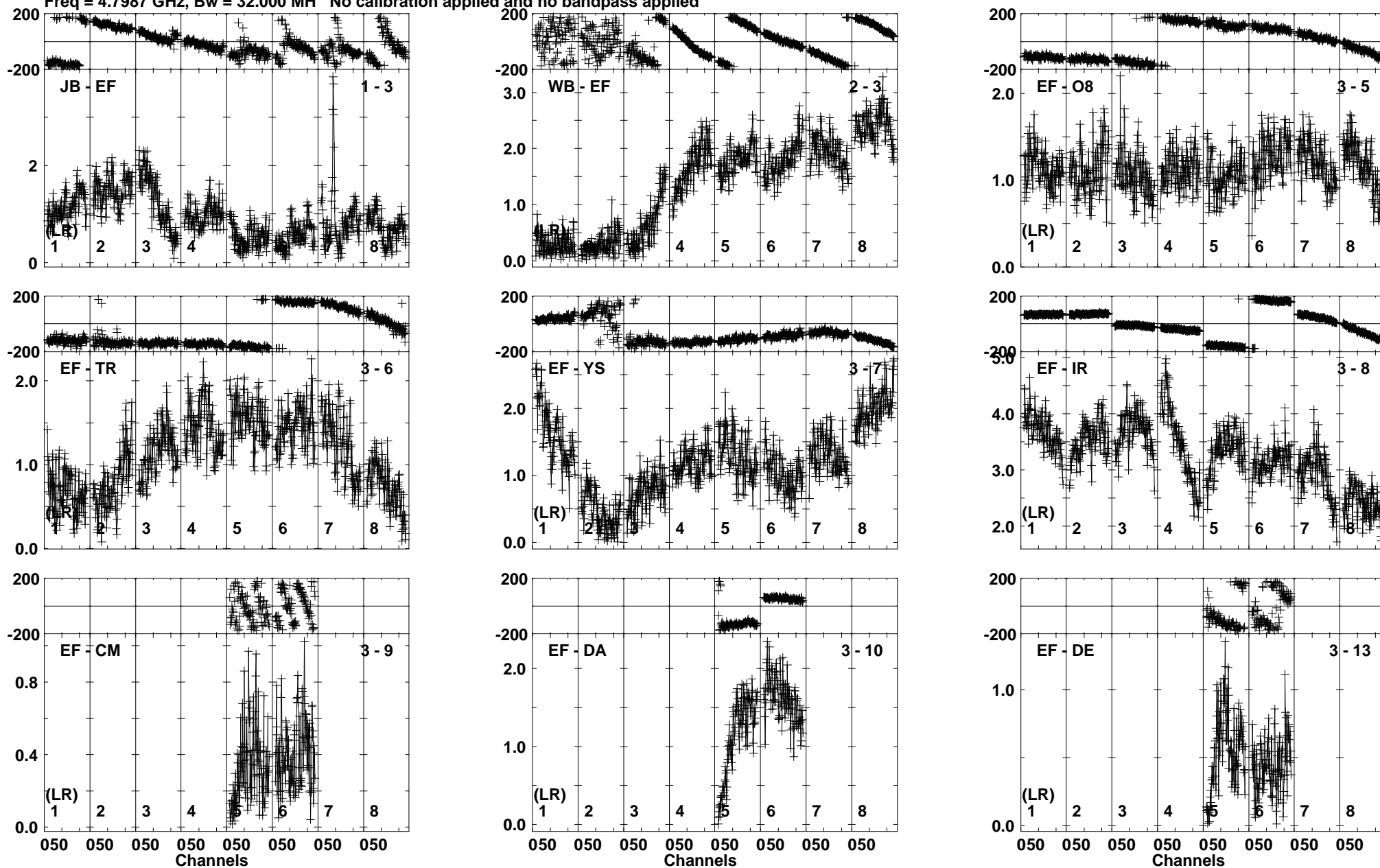
Lower frame: Milli Ampl Jy Top frame: Phas deg Vector averaged cross-power spectrum Baseline: JB (01) - EF (03) Timerange: 01/08:09:21 to 01/08:10:49
