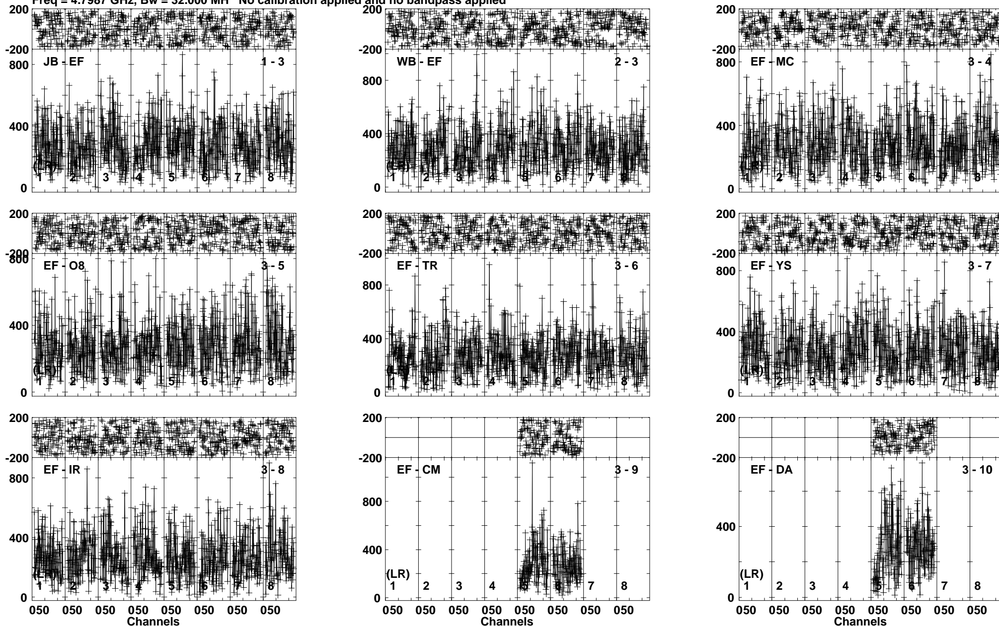
Lower frame: Micro Ampl Jy Top frame: Phas deg Vector averaged cross-power spectrum Baseline: JB (01) - EF (03) Timerange: 01/04:18:20 to 01/04:20:50
