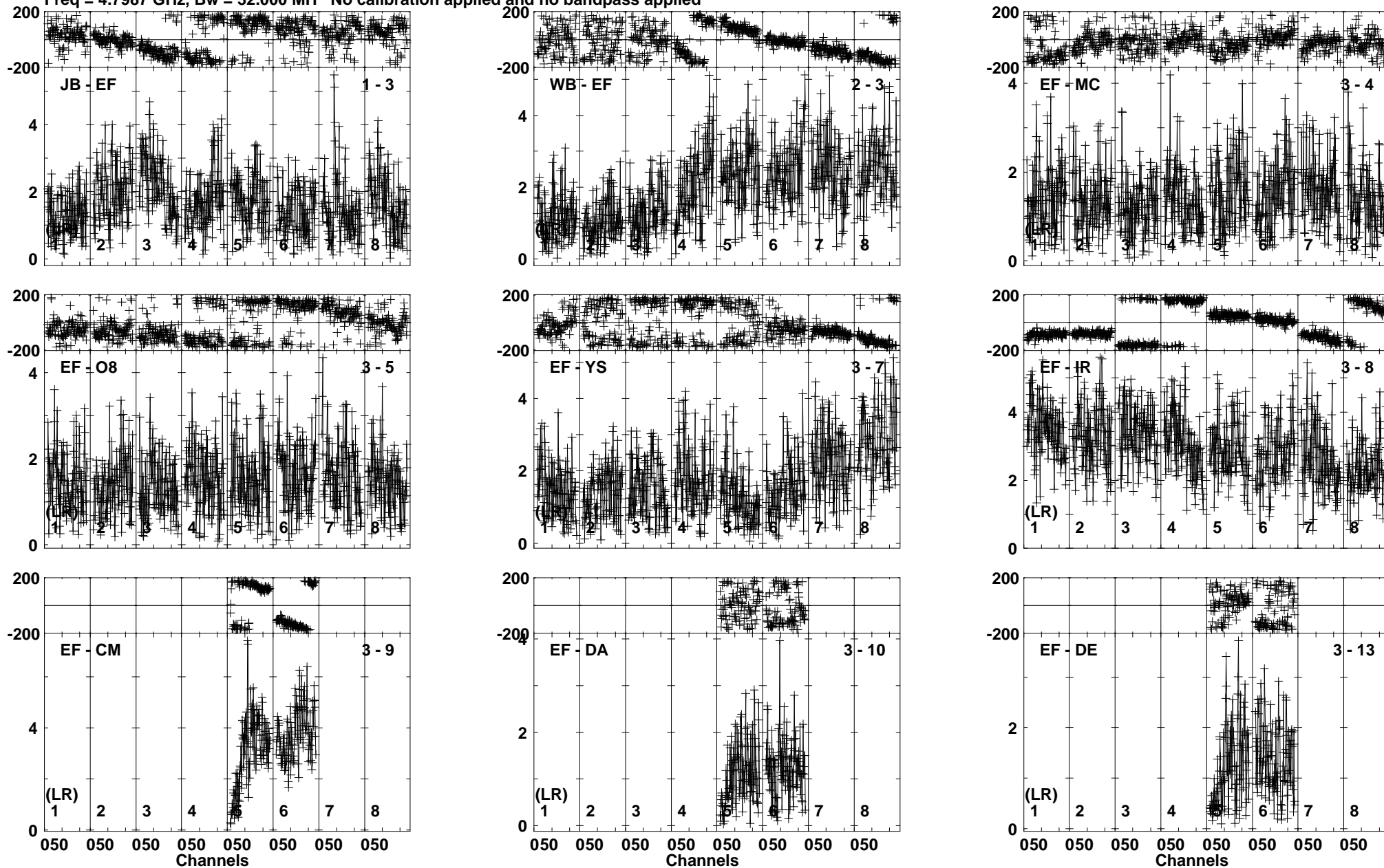
Lower frame: Milli Ampl Jy Top frame: Phas deg Vector averaged cross-power spectrum Baseline: JB (01) - EF (03) Timerange: 01/02:57:20 to 01/02:58:49
