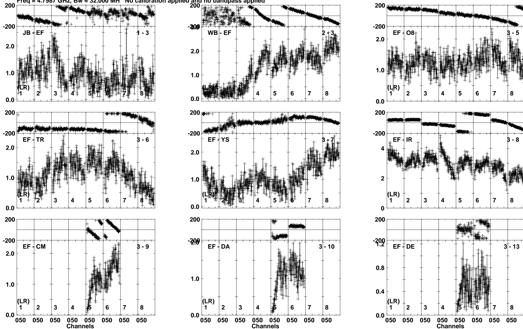
Lower frame: Milli Ampl Jy Top frame: Phas deg Vector averaged cross-power spectrum Baseline: JB (01) - EF (03) Timerange: 01/05:31:10 to 01/05:32:39
