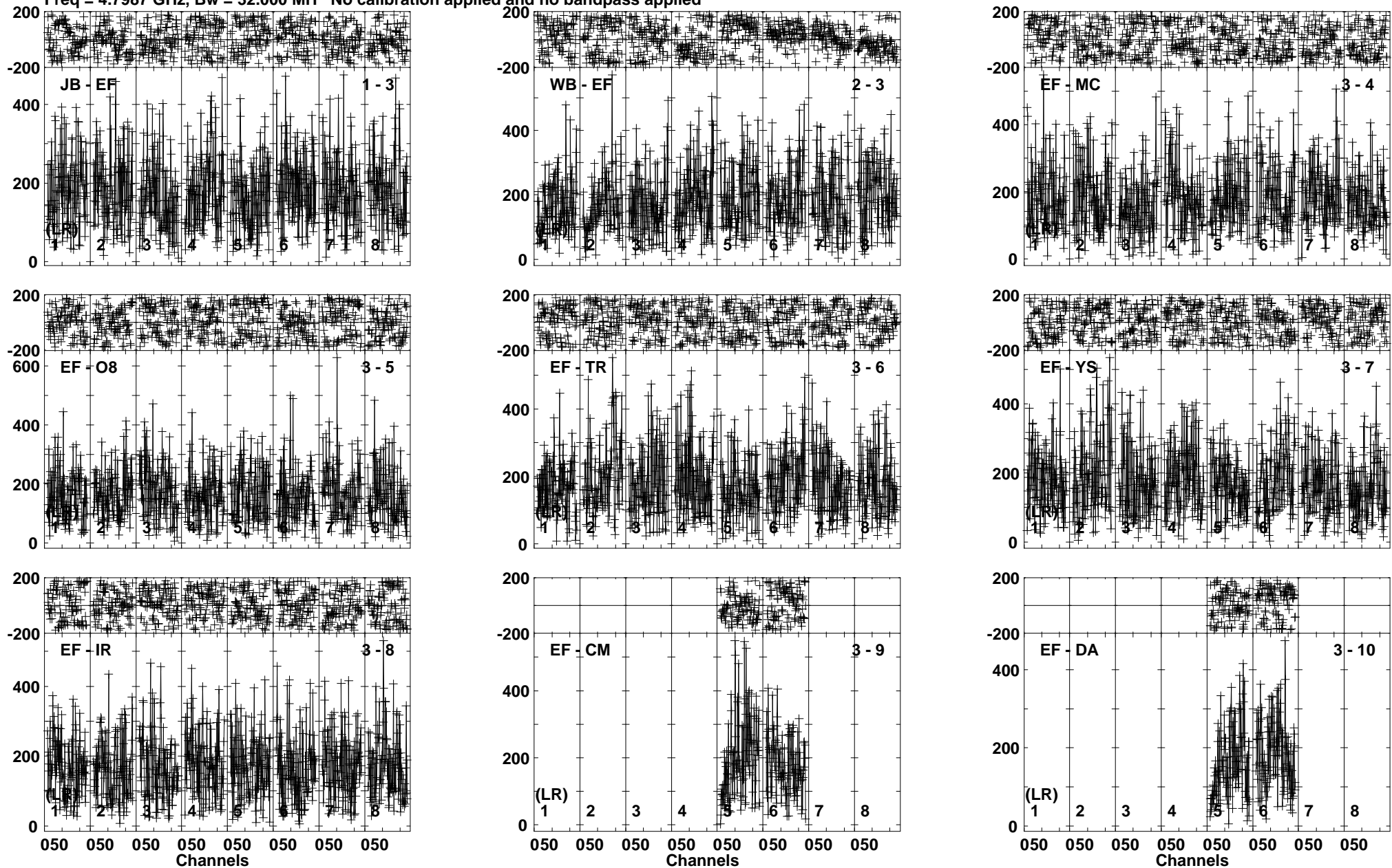
Lower frame: Micro Ampl Jy Top frame: Phas deg Vector averaged cross-power spectrum Baseline: JB (01) - EF (03) Timerange: 01/00:45:50 to 01/00:48:20
