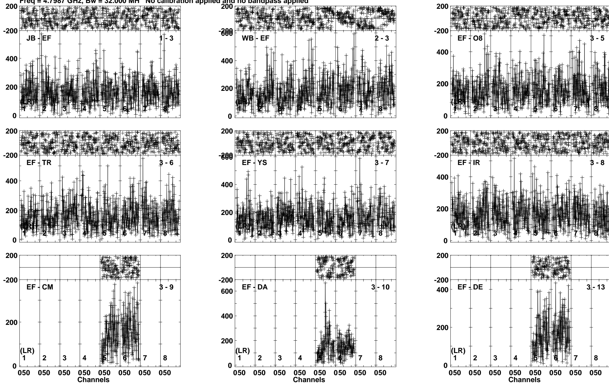
Lower frame: Micro Ampl Jy Top frame: Phas deg Vector averaged cross-power spectrum Baseline: JB (01) - EF (03) Timerange: 01/07:02:20 to 01/07:04:50
