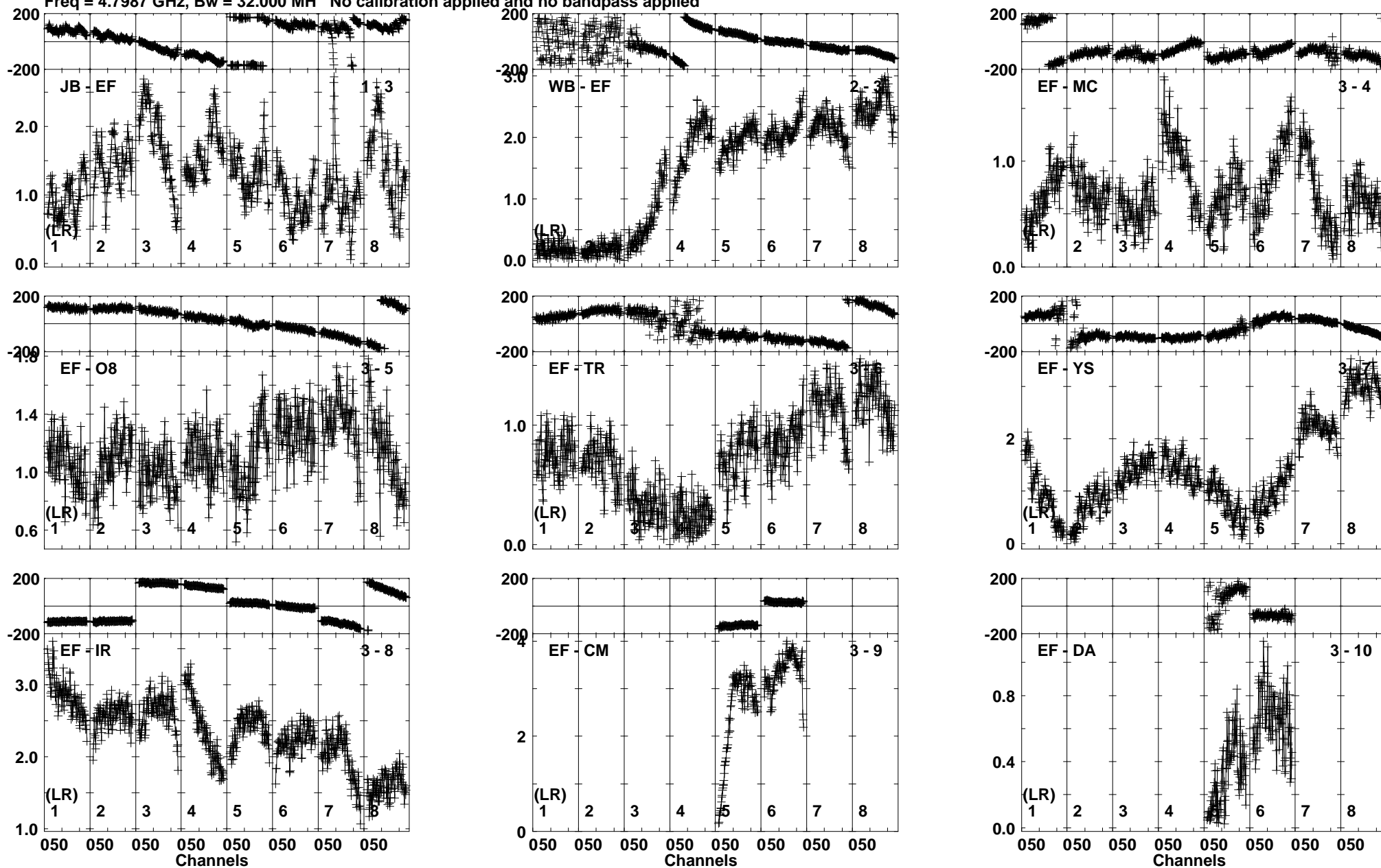
Lower frame: Milli Ampl Jy Top frame: Phas deg Vector averaged cross-power spectrum Baseline: JB (01) - EF (03) Timerange: 01/00:34:11 to 01/00:35:39
