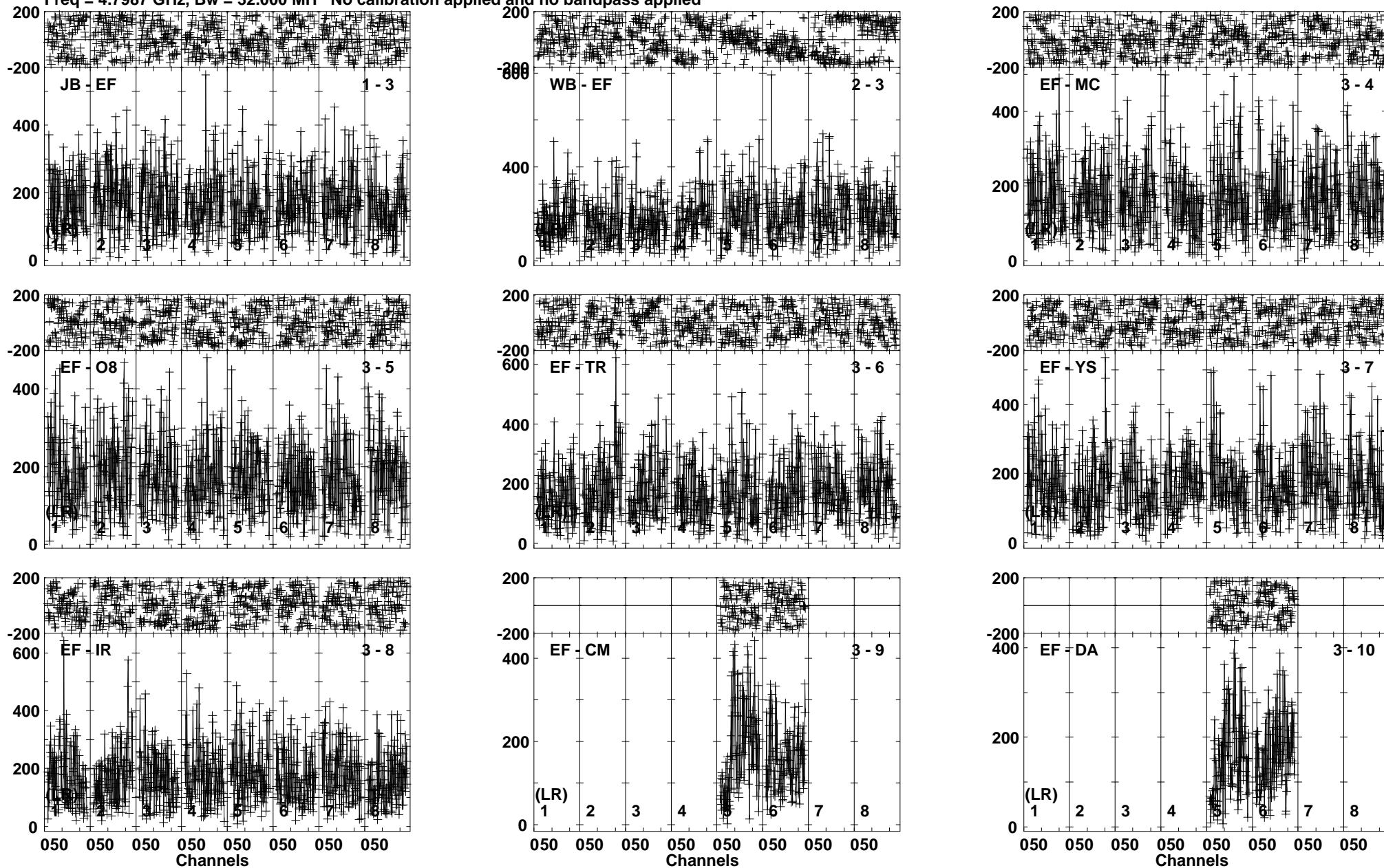
Lower frame: Micro Ampl Jy Top frame: Phas deg Vector averaged cross-power spectrum Baseline: JB (01) - EF (03) Timerange: 01/01:59:11 to 01/02:01:39
