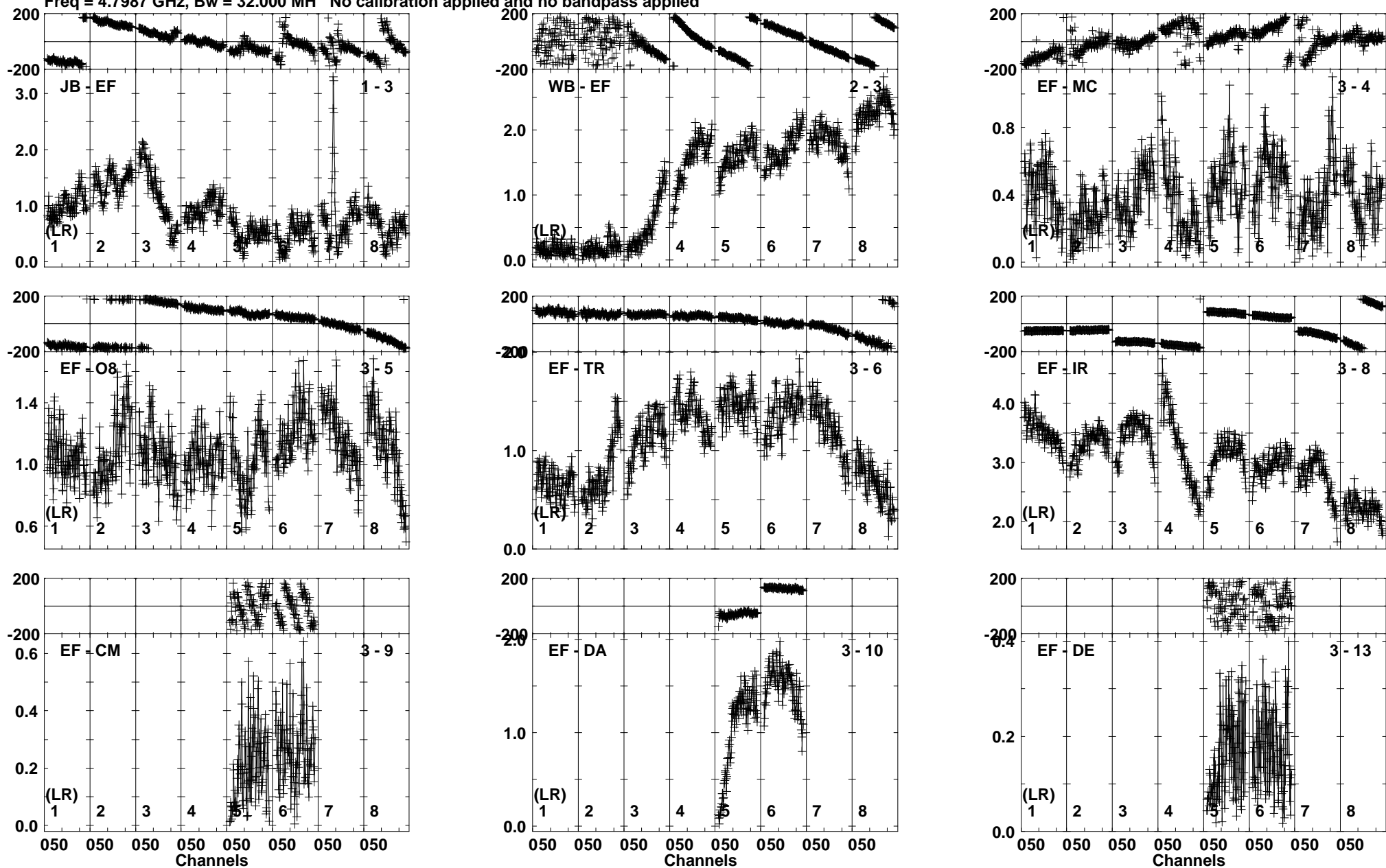
Lower frame: Milli Ampl Jy Top frame: Phas deg Vector averaged cross-power spectrum Baseline: JB (01) - EF (03) Timerange: 01/08:33:11 to 01/08:34:39
