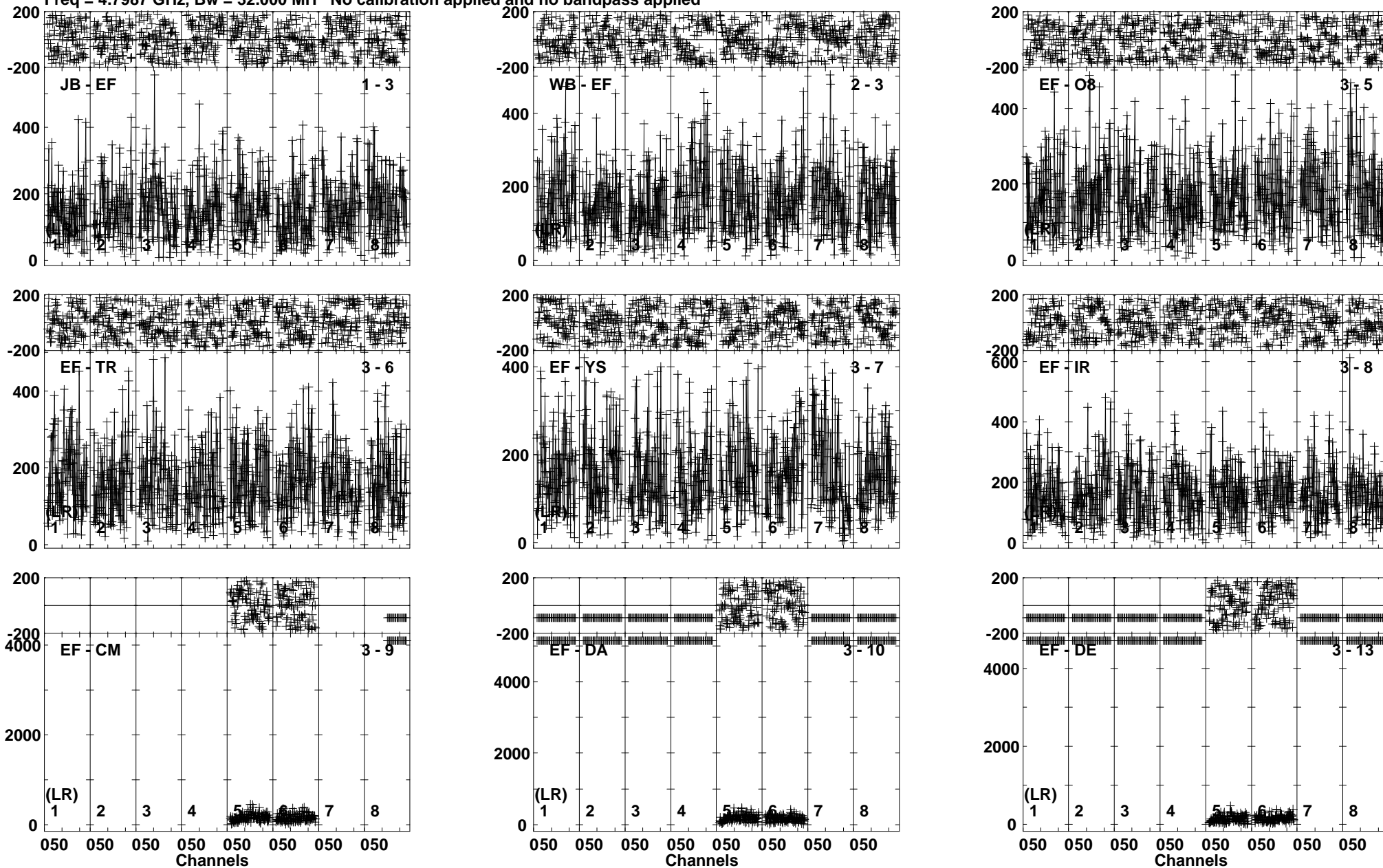
Lower frame: Micro Ampl Jy Top frame: Phas deg Vector averaged cross-power spectrum Baseline: JB (01) - EF (03) Timerange: 01/08:25:50 to 01/08:28:20
