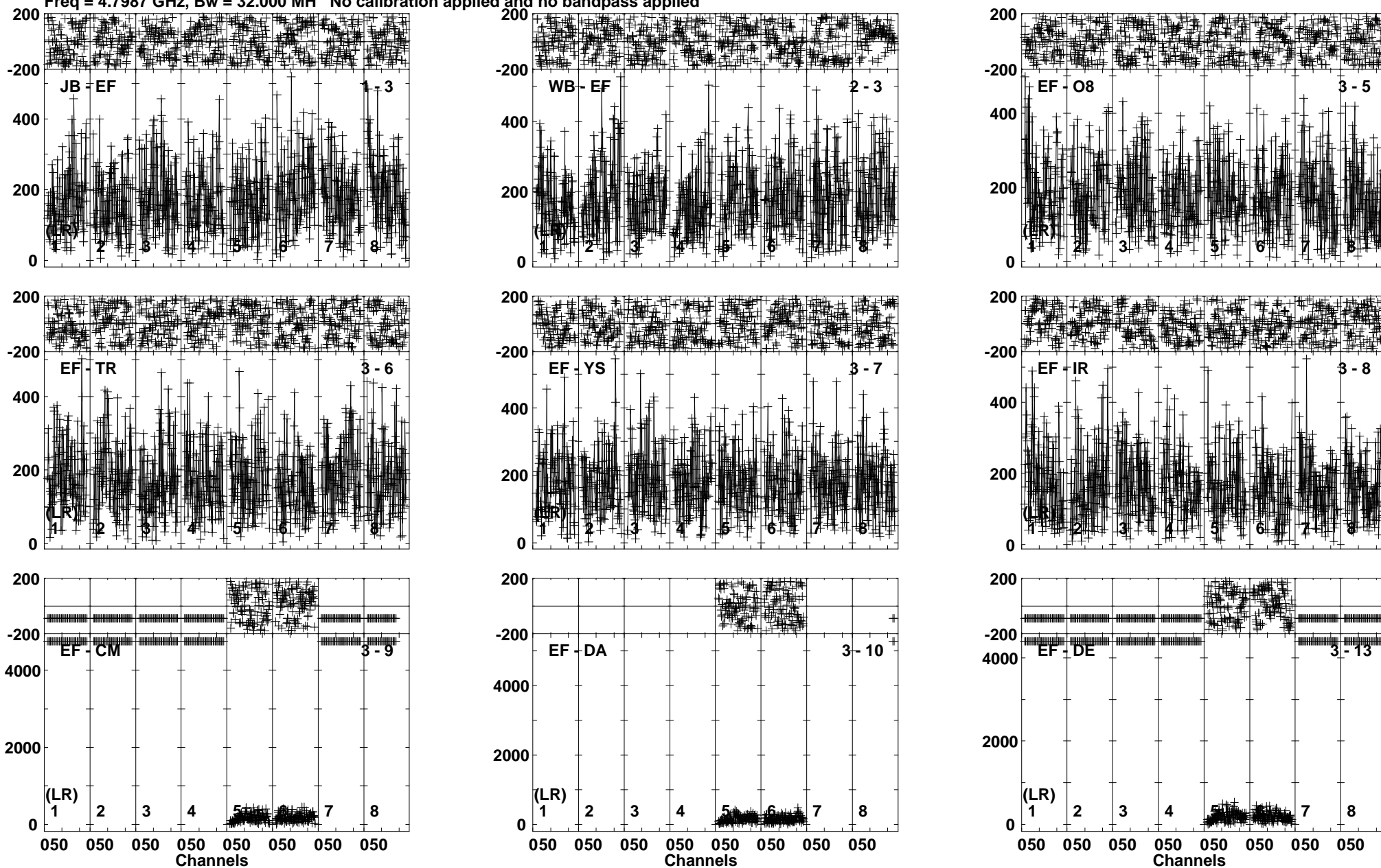
Lower frame: Micro Ampl Jy Top frame: Phas deg Vector averaged cross-power spectrum Baseline: JB (01) - EF (03) Timerange: 01/06:24:20 to 01/06:26:50
