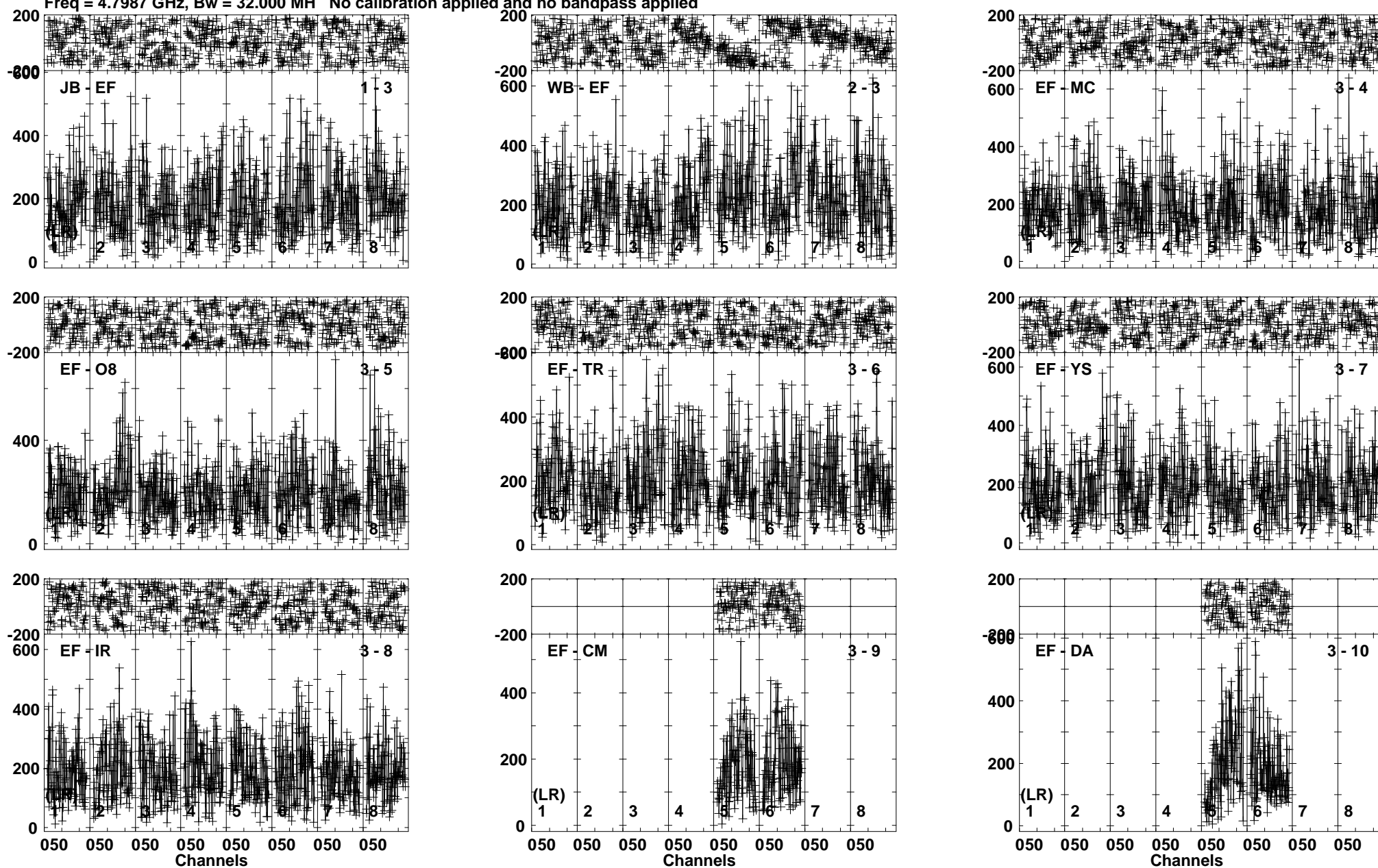
Lower frame: Micro Ampl Jy Top frame: Phas deg Vector averaged cross-power spectrum Baseline: JB (01) - EF (03) Timerange: 01/02:41:10 to 01/02:43:40
