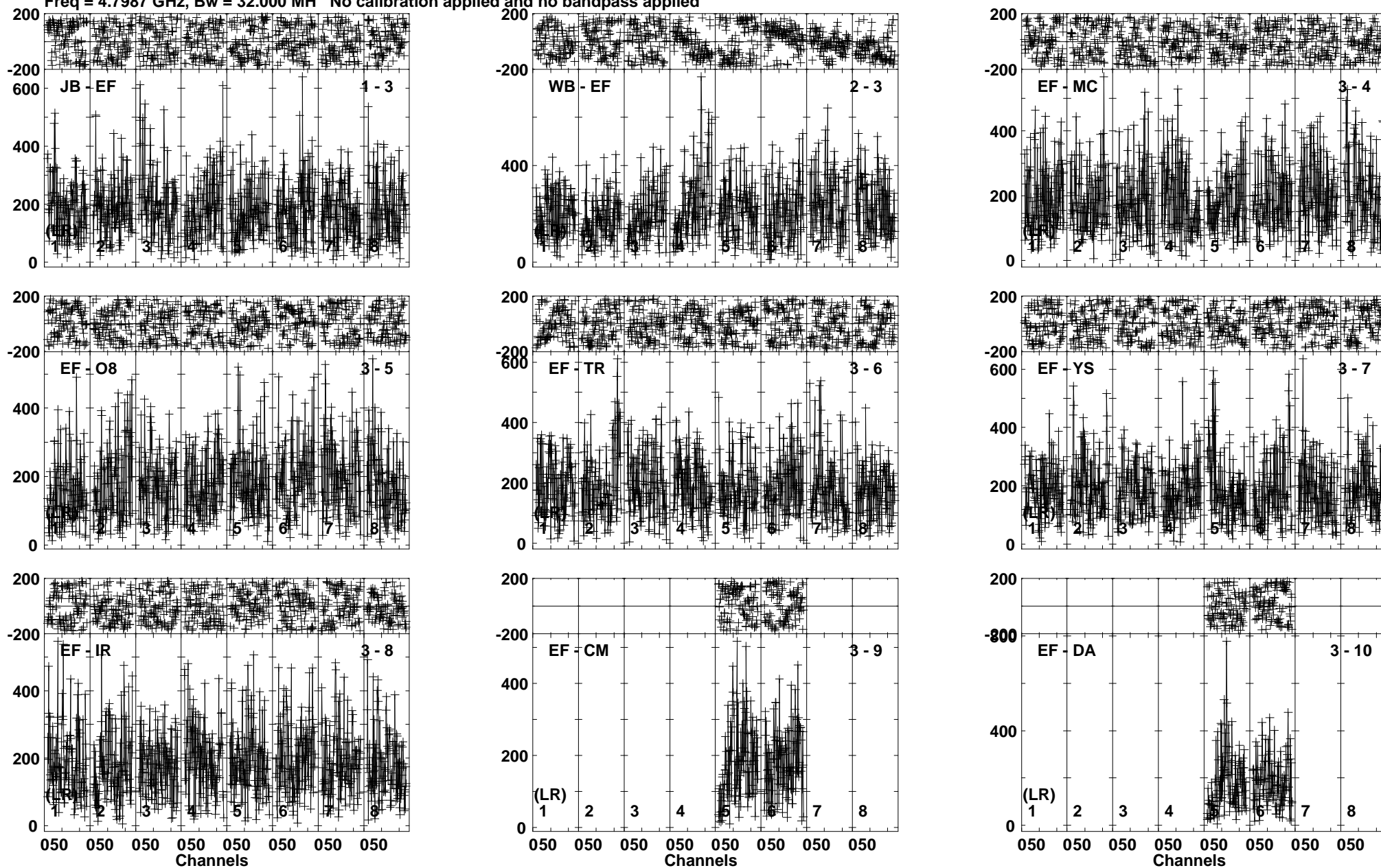
Lower frame: Micro Ampl Jy Top frame: Phas deg Vector averaged cross-power spectrum Baseline: JB (01) - EF (03) Timerange: 01/02:31:00 to 01/02:33:30
