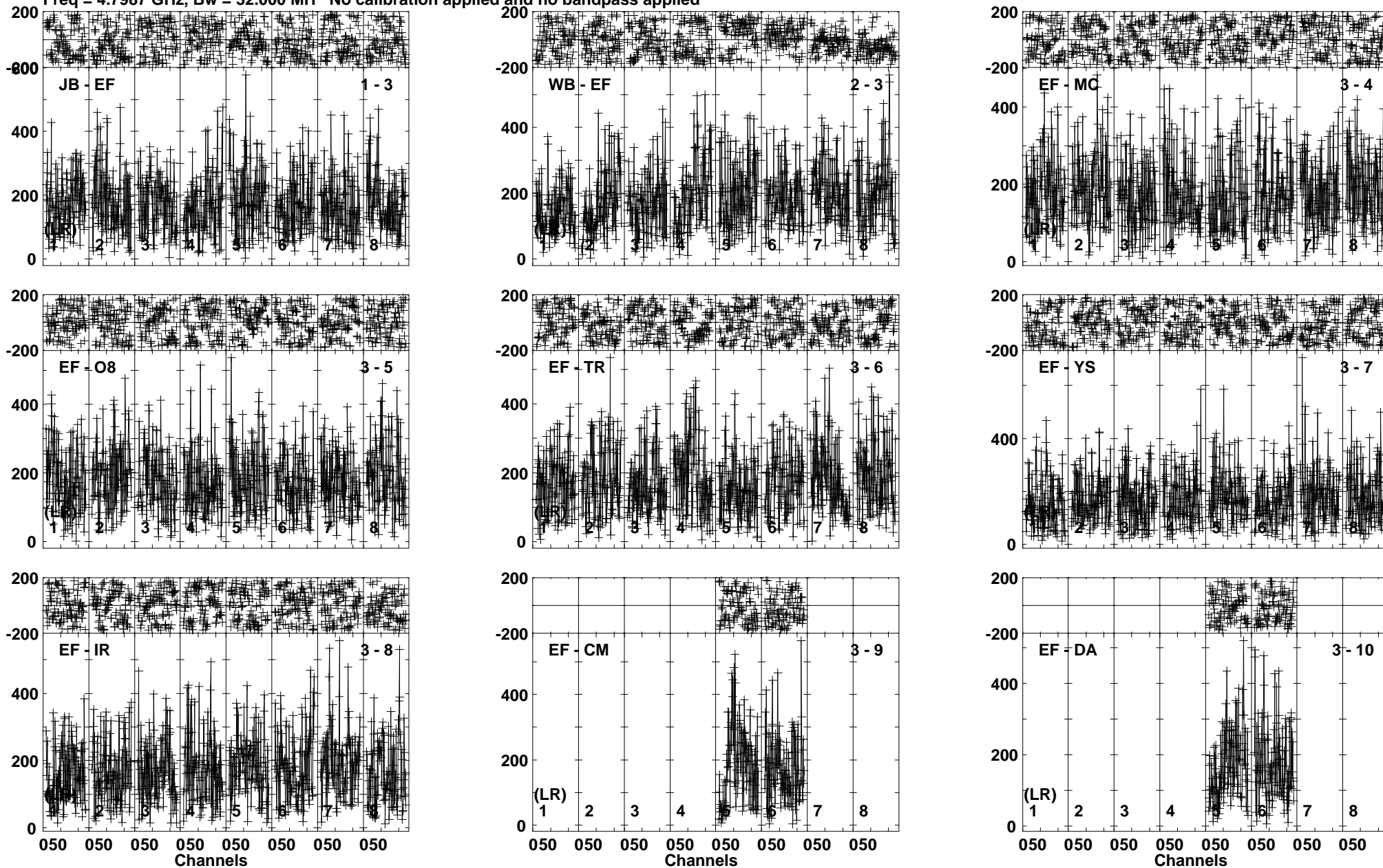
Lower frame: Micro Ampl Jy Top frame: Phas deg Vector averaged cross-power spectrum Baseline: JB (01) - EF (03) Timerange: 01/00:11:51 to 01/00:14:19
