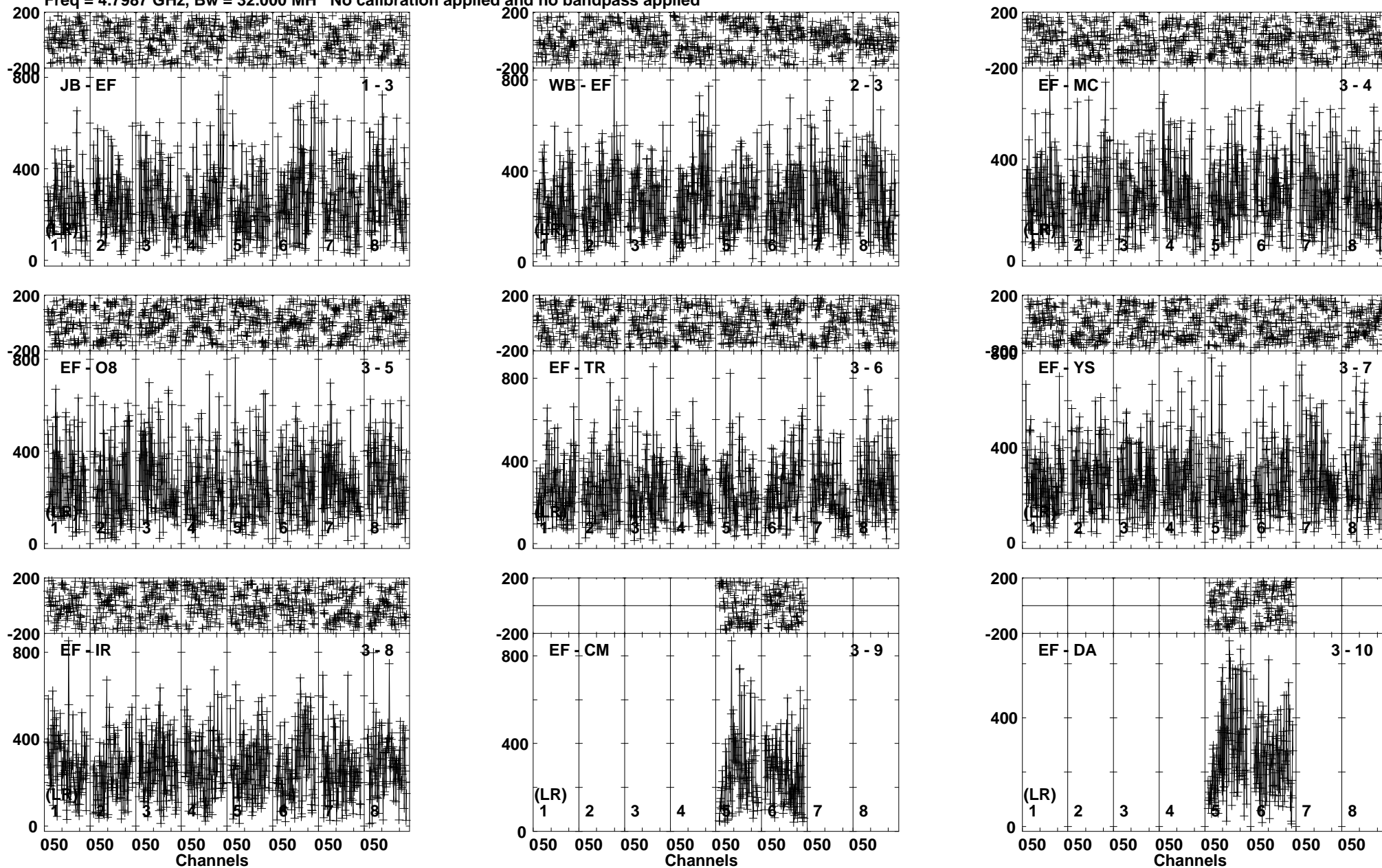
Lower frame: Micro Ampl Jy Top frame: Phas deg Vector averaged cross-power spectrum Baseline: JB (01) - EF (03) Timerange: 01/01:09:16 to 01/01:10:00
