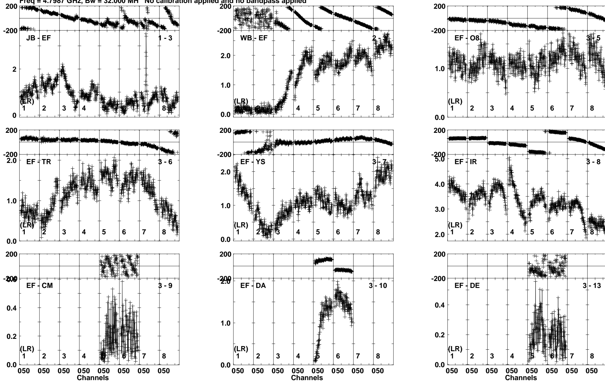
Lower frame: Milli Ampl Jy Top frame: Phas deg Vector averaged cross-power spectrum Baseline: JB (01) - EF (03) Timerange: 01/07:46:21 to 01/07:47:49
