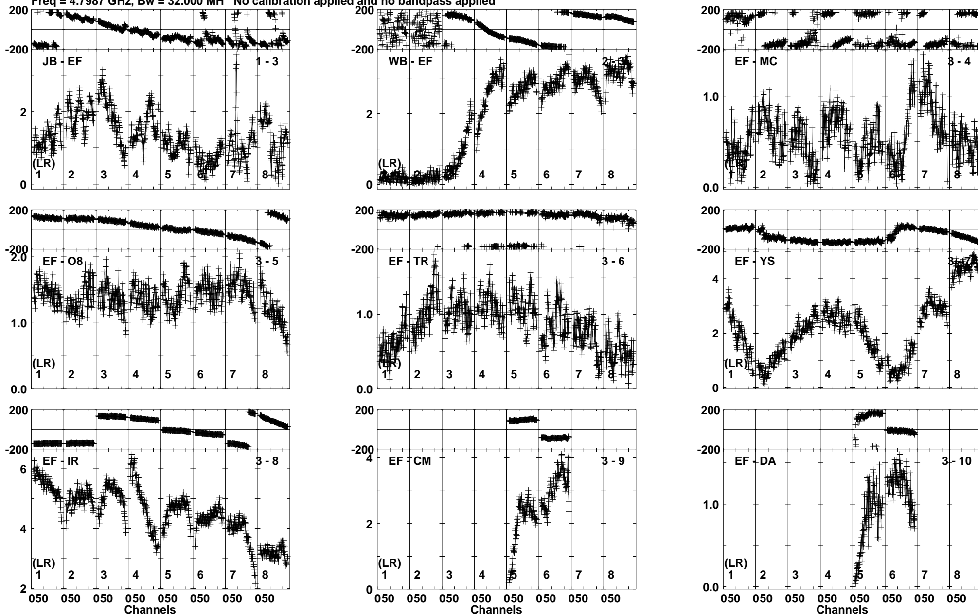
Lower frame: Milli Ampl Jy Top frame: Phas deg Vector averaged cross-power spectrum Baseline: JB (01) - EF (03) Timerange: 01/00:16:30 to 01/00:17:59
