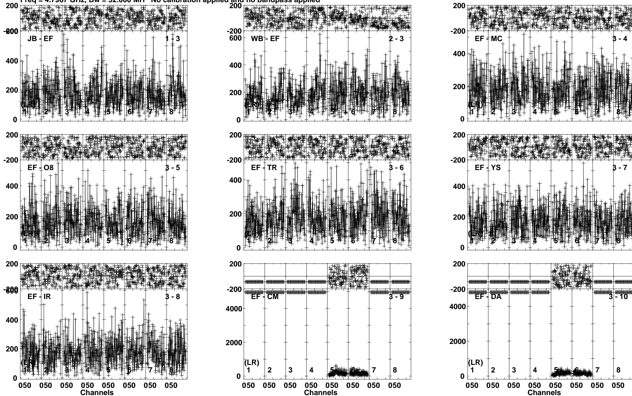
Lower frame: Micro Ampl Jy Top frame: Phas deg Vector averaged cross-power spectrum Baseline: JB (01) - EF (03) Timerange: 01/00:26:50 to 01/00:29:19
