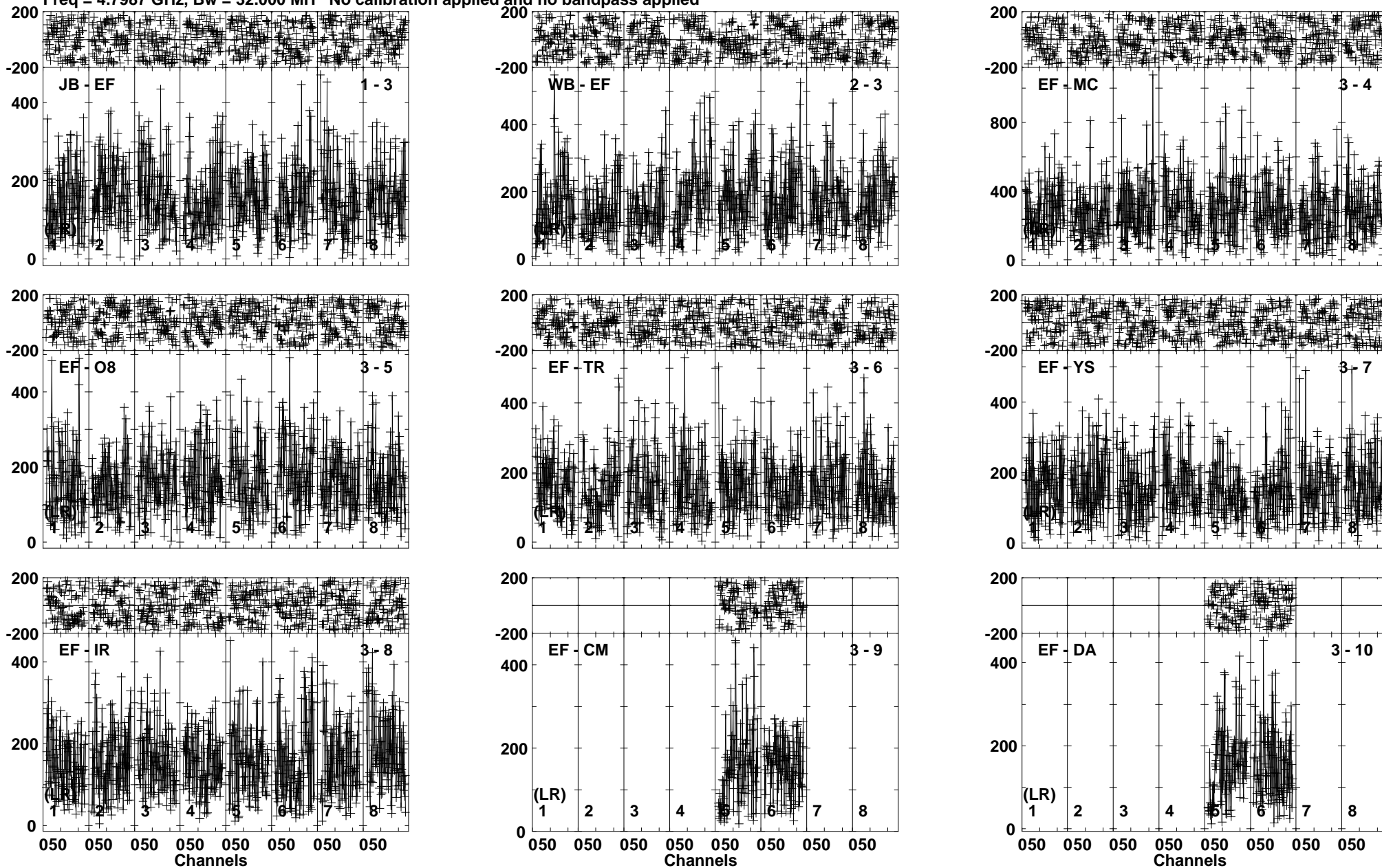
Lower frame: Micro Ampl Jy Top frame: Phas deg Vector averaged cross-power spectrum Baseline: JB (01) - EF (03) Timerange: 01/08:29:50 to 01/08:32:20
