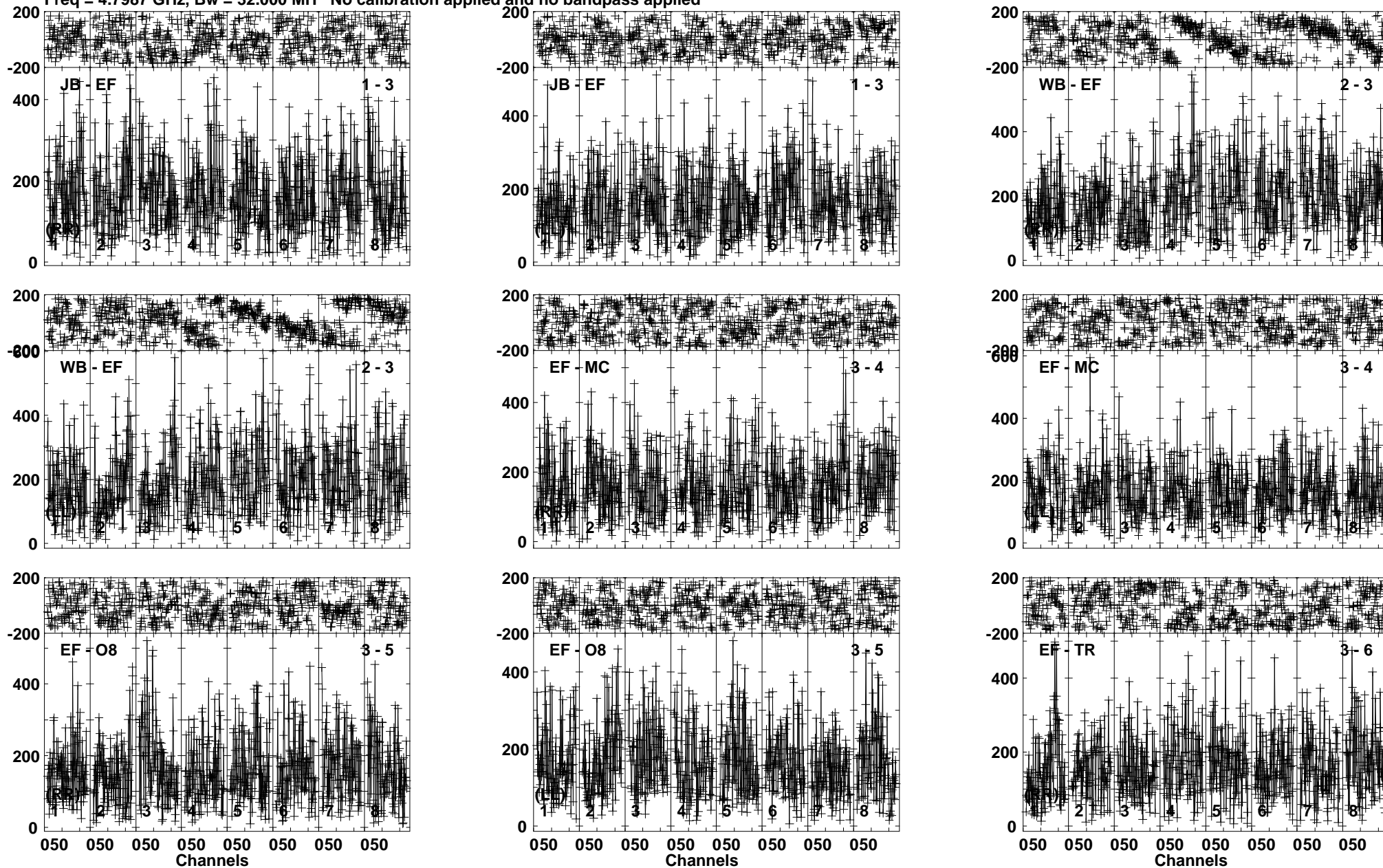
Lower frame: Micro Ampl Jy Top frame: Phas deg Vector averaged cross-power spectrum Baseline: JB (01) - EF (03) Timerange: 01/08:54:33 to 01/08:56:10
