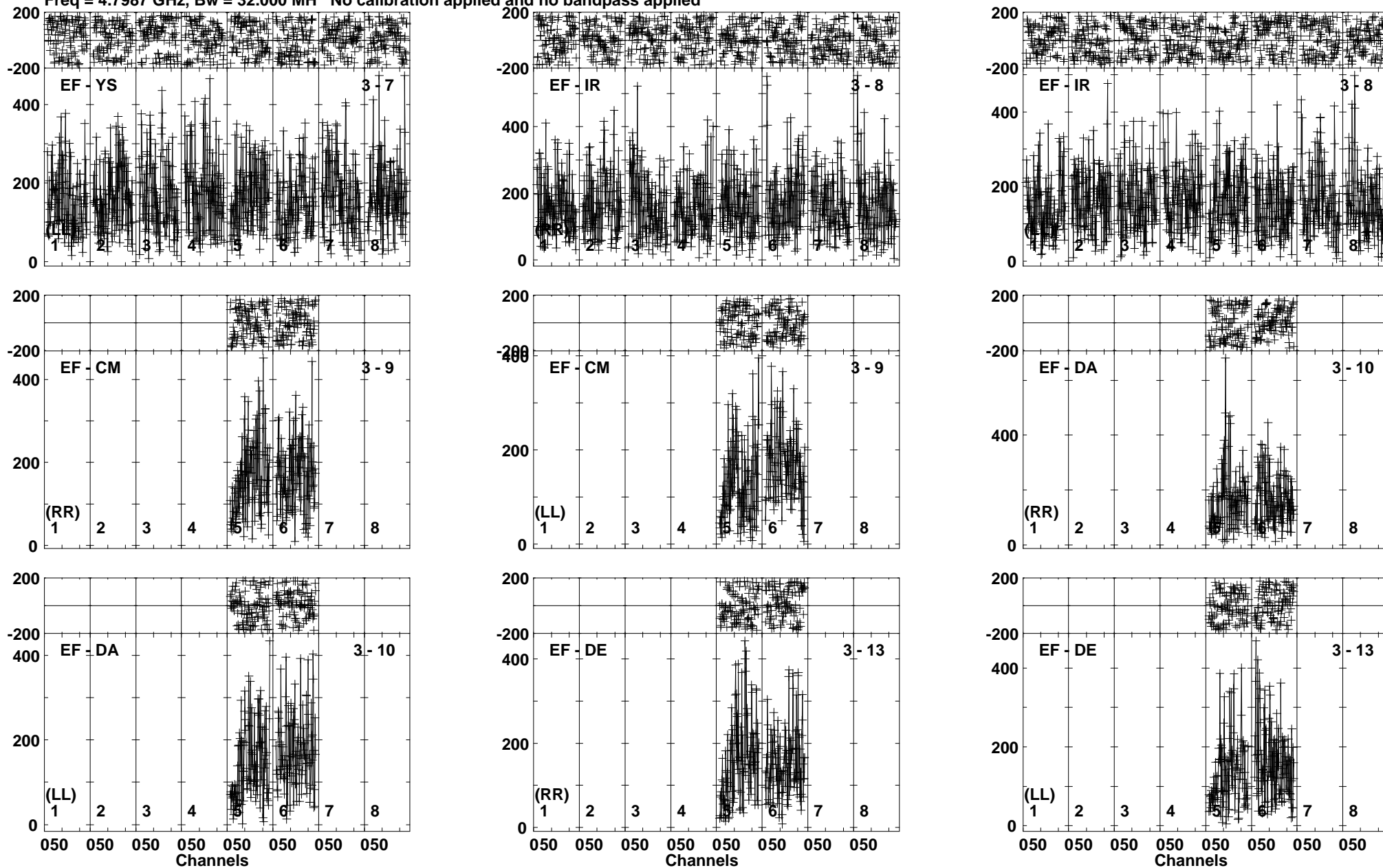
Lower frame: Micro Ampl Jy Top frame: Phas deg Vector averaged cross-power spectrum Baseline: EF (03) - YS (07) Timerange: 01/06:38:30 to 01/06:41:00
