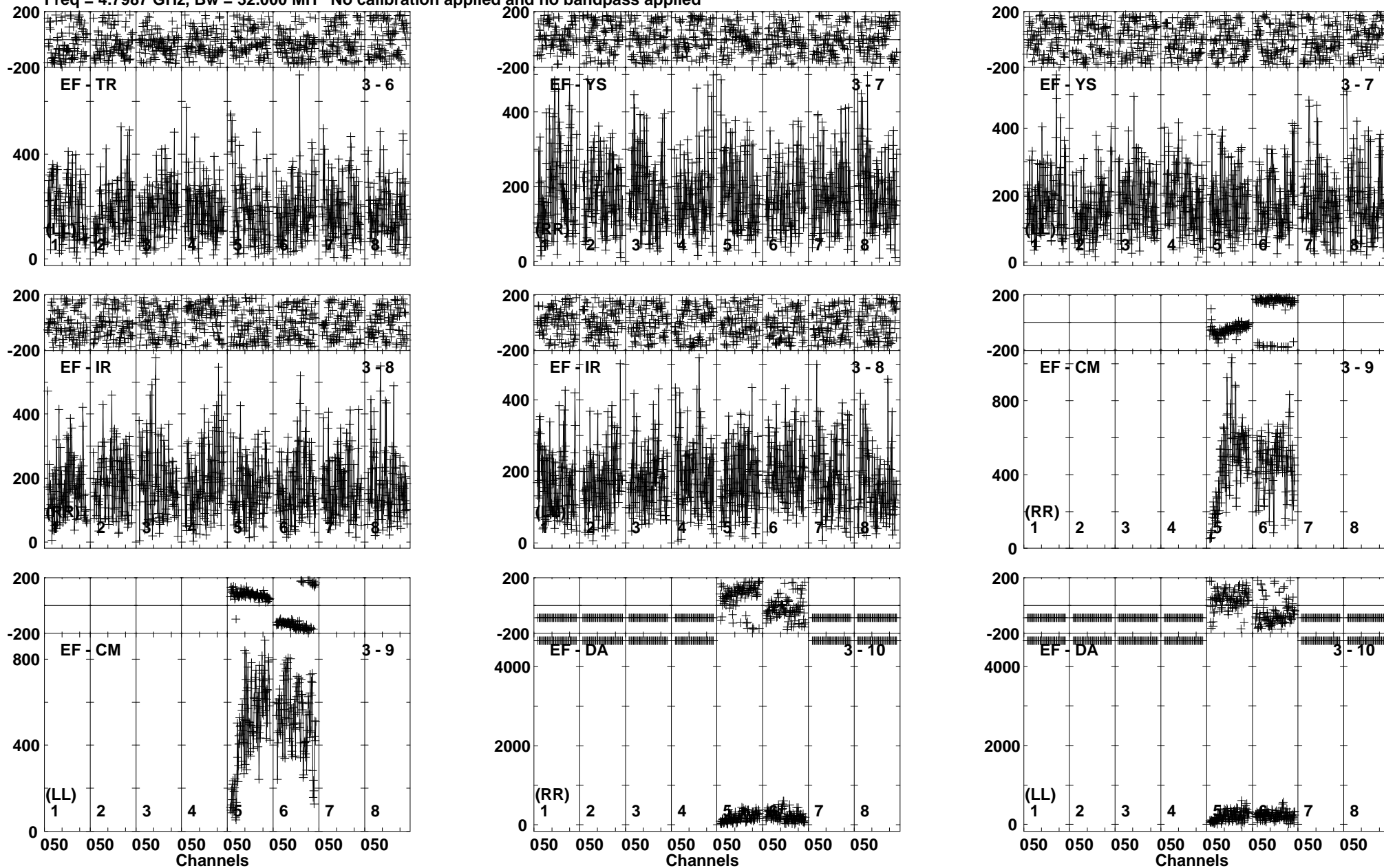
Lower frame: Micro Ampl Jy Top frame: Phas deg Vector averaged cross-power spectrum Baseline: EF (03) - TR (06) Timerange: 01/00:07:50 to 01/00:10:19
