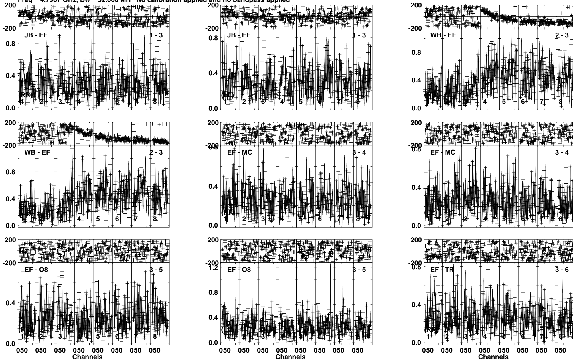
Lower frame: Milli Ampl Jy Top frame: Phas deg Vector averaged cross-power spectrum Baseline: JB (01) - EF (03) Timerange: 01/01:09:16 to 01/01:10:00
