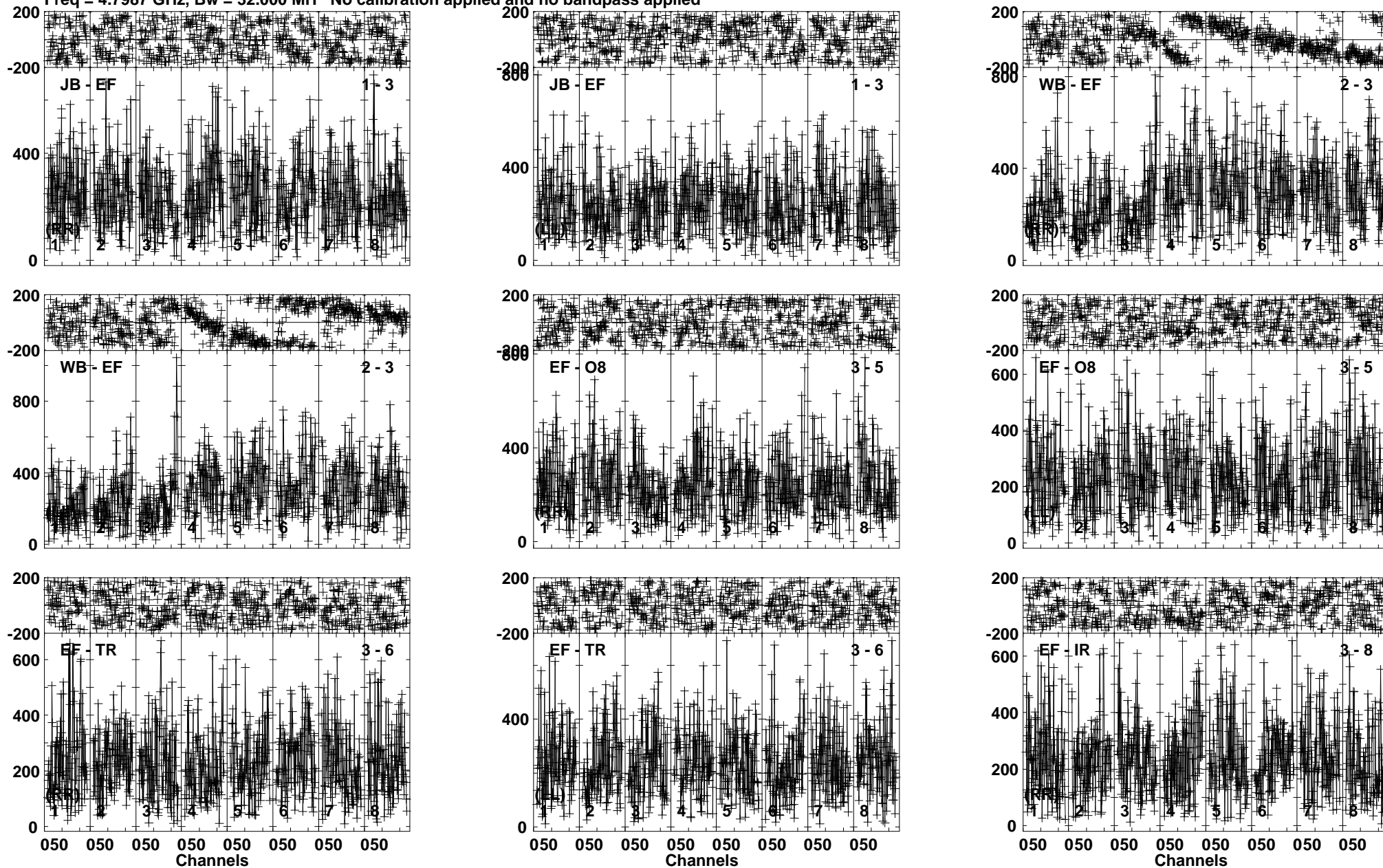
Lower frame: Micro Ampl Jy Top frame: Phas deg Vector averaged cross-power spectrum Baseline: JB (01) - EF (03) Timerange: 01/04:47:11 to 01/04:49:39
