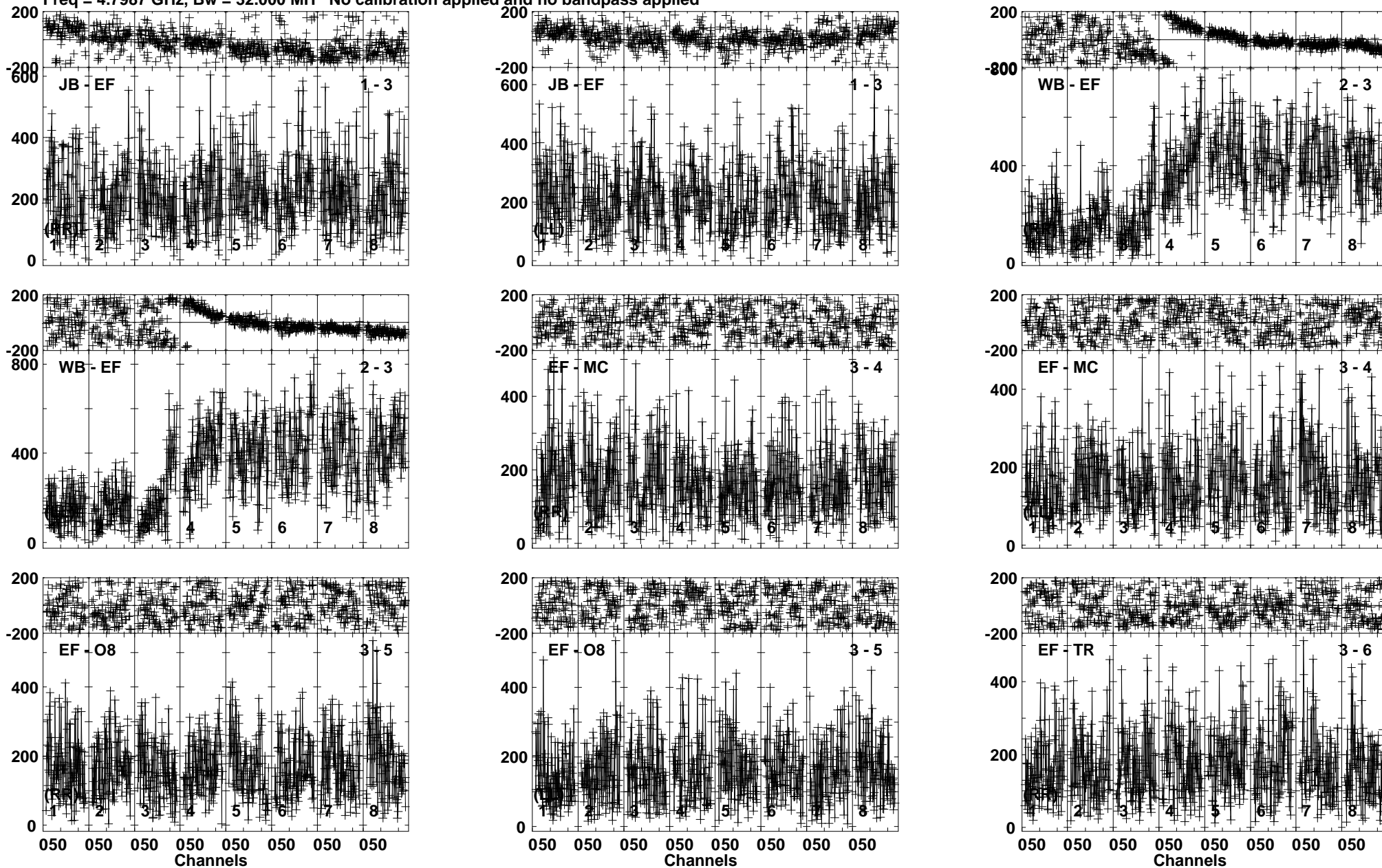
Lower frame: Micro Ampl Jy Top frame: Phas deg Vector averaged cross-power spectrum Baseline: JB (01) - EF (03) Timerange: 01/01:17:41 to 01/01:20:09
