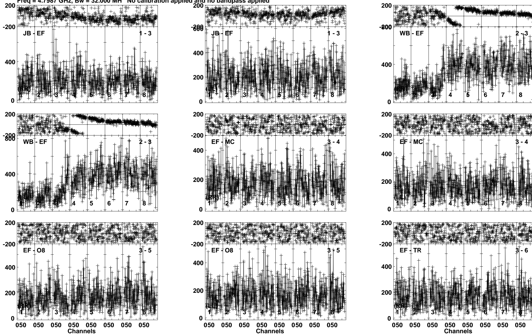
Lower frame: Micro Ampl Jy Top frame: Phas deg Vector averaged cross-power spectrum Baseline: JB (01) - EF (03) Timerange: 01/01:26:31 to 01/01:28:59
