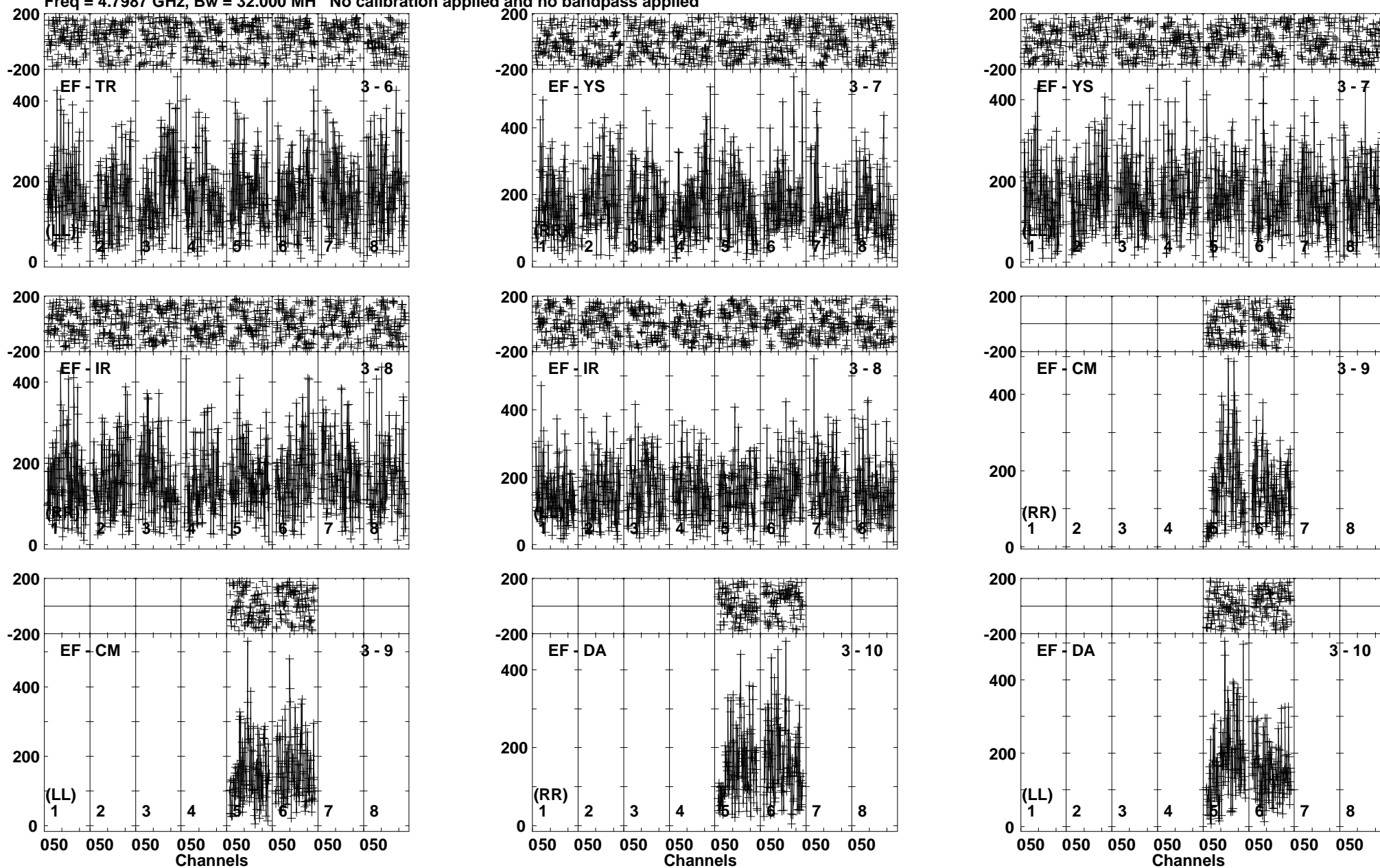
Lower frame: Micro Ampl Jy Top frame: Phas deg Vector averaged cross-power spectrum Baseline: EF (03) - TR (06) Timerange: 01/08:29:50 to 01/08:32:20
