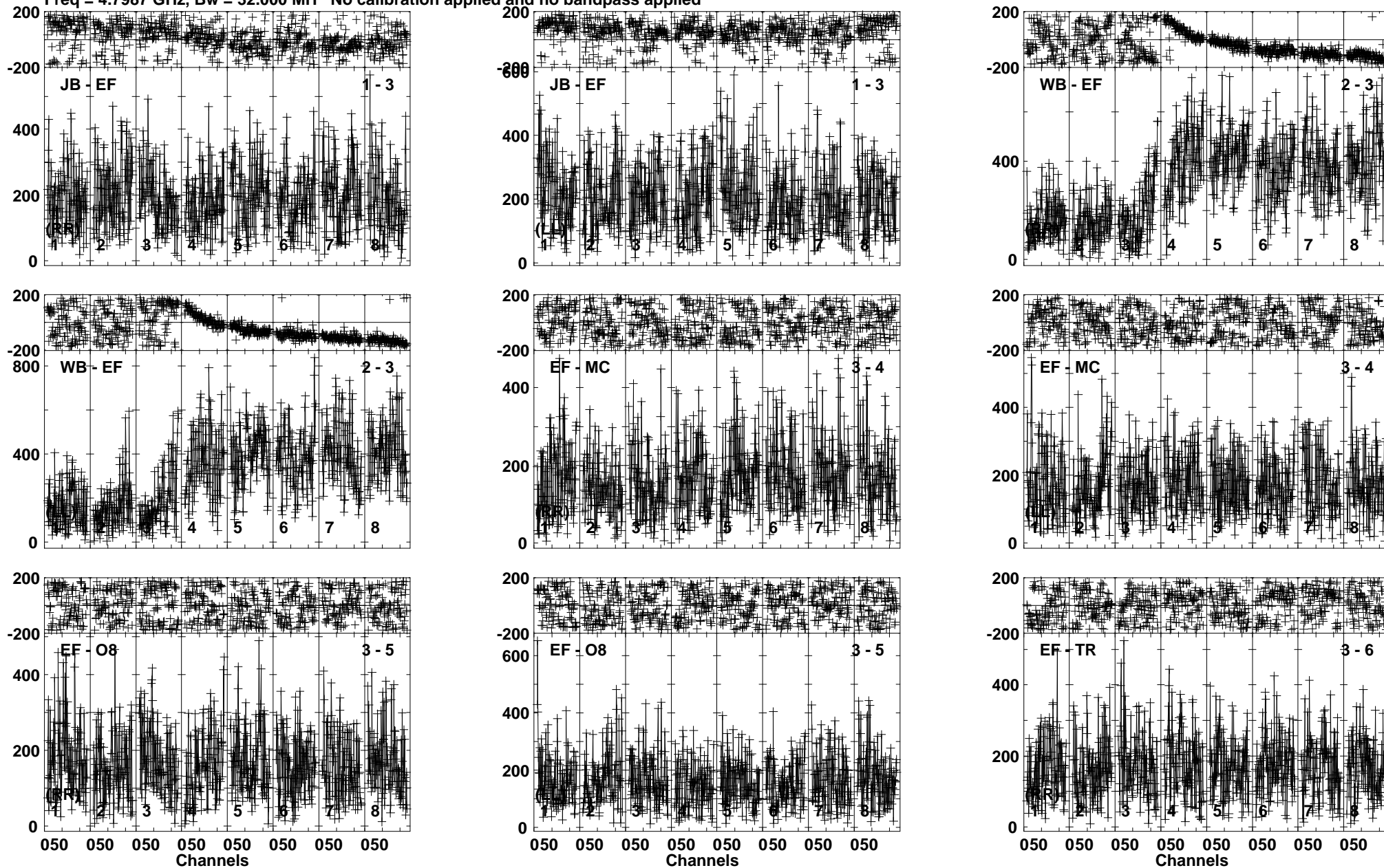
Lower frame: Micro Ampl Jy Top frame: Phas deg Vector averaged cross-power spectrum Baseline: JB (01) - EF (03) Timerange: 01/01:31:21 to 01/01:33:49
