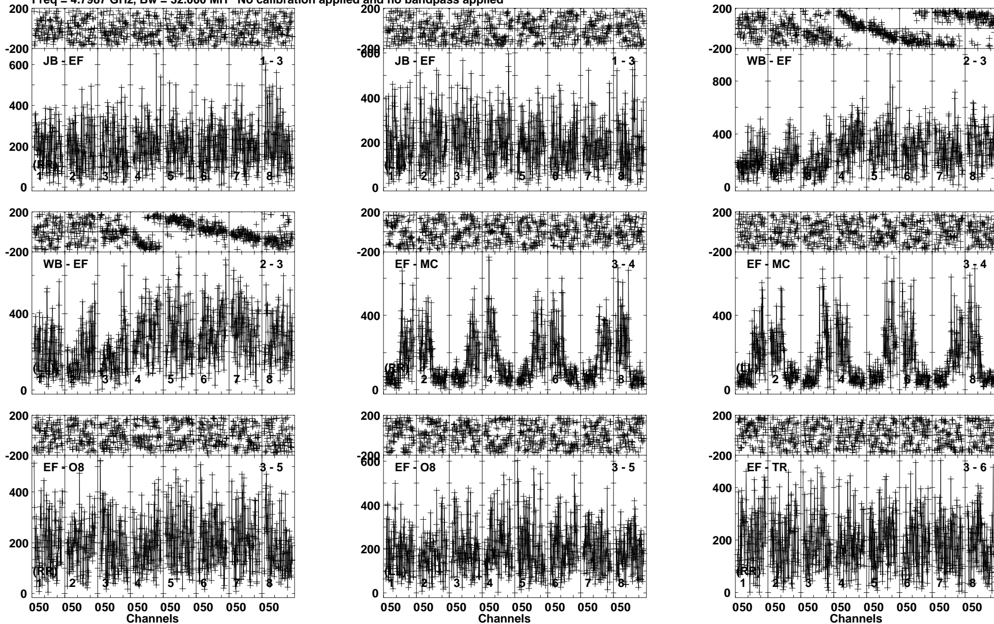
Lower frame: Micro Ampl Jy Top frame: Phas deg Vector averaged cross-power spectrum Baseline: JB (01) - EF (03) Timerange: 01/05:04:50 to 01/05:07:20
