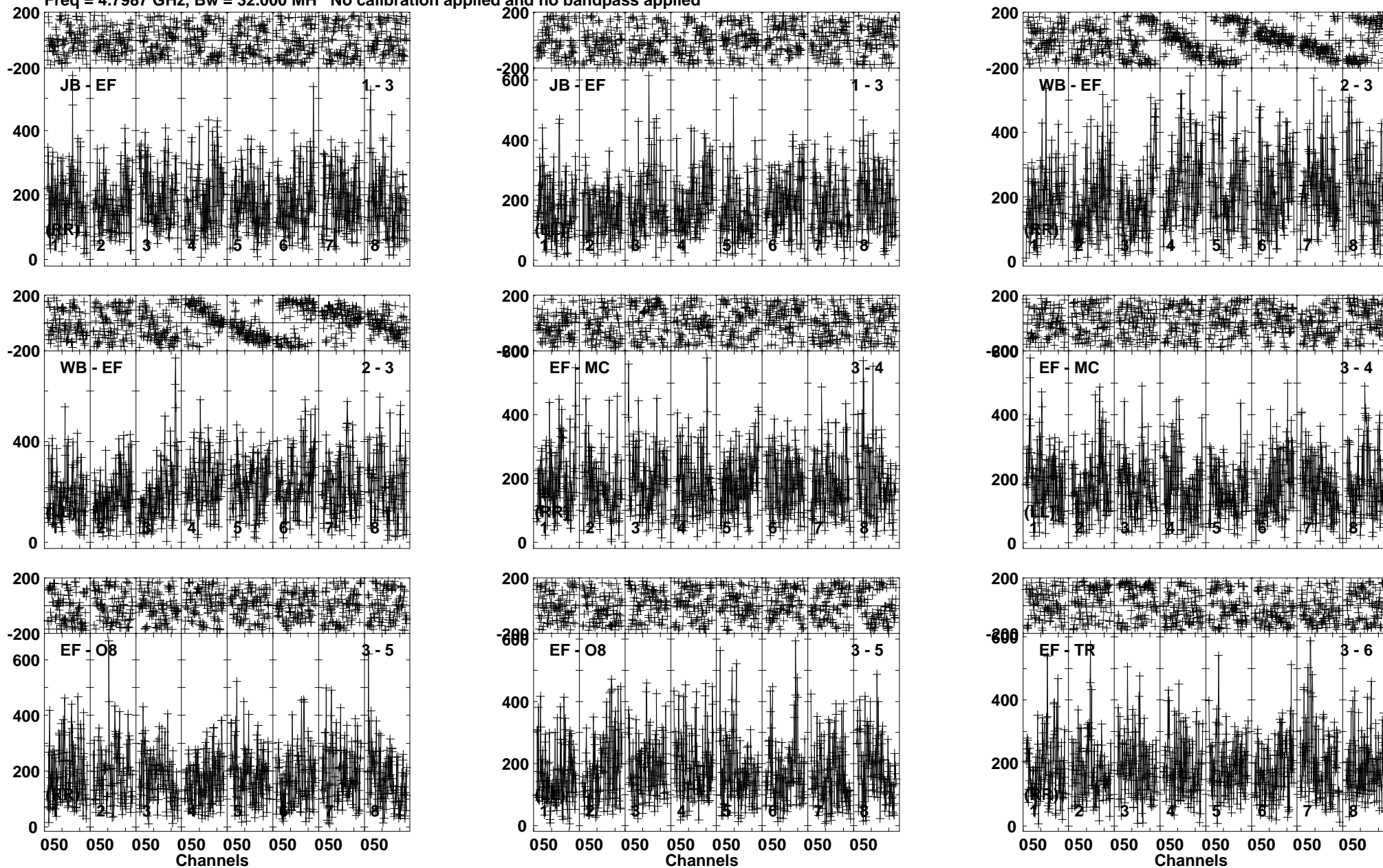
Lower frame: Micro Ampl Jy Top frame: Phas deg Vector averaged cross-power spectrum Baseline: JB (01) - EF (03) Timerange: 01/08:57:41 to 01/09:00:09
