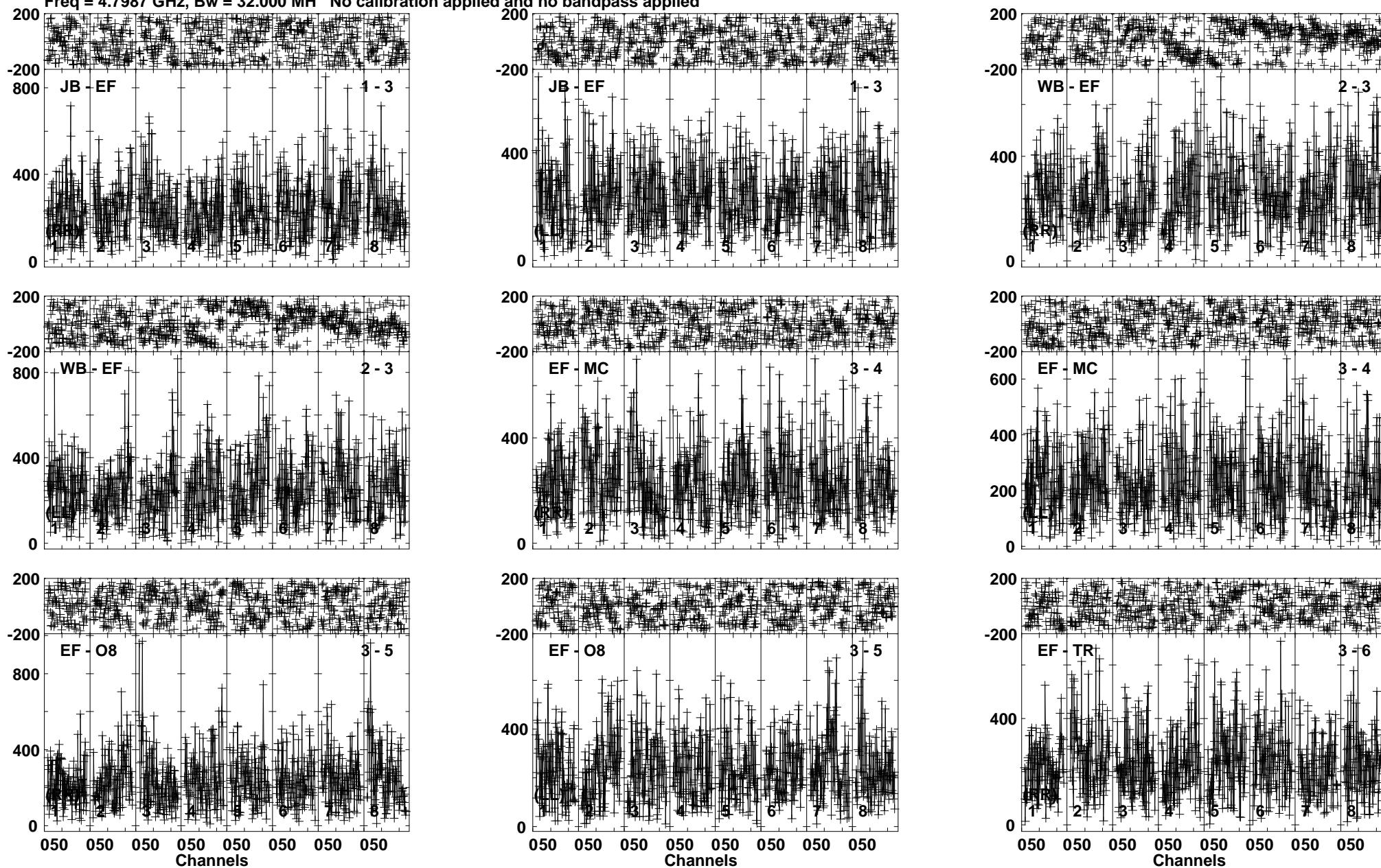
Lower frame: Micro Ampl Jy Top frame: Phas deg Vector averaged cross-power spectrum Baseline: JB (01) - EF (03) Timerange: 01/03:13:51 to 01/03:16:19
