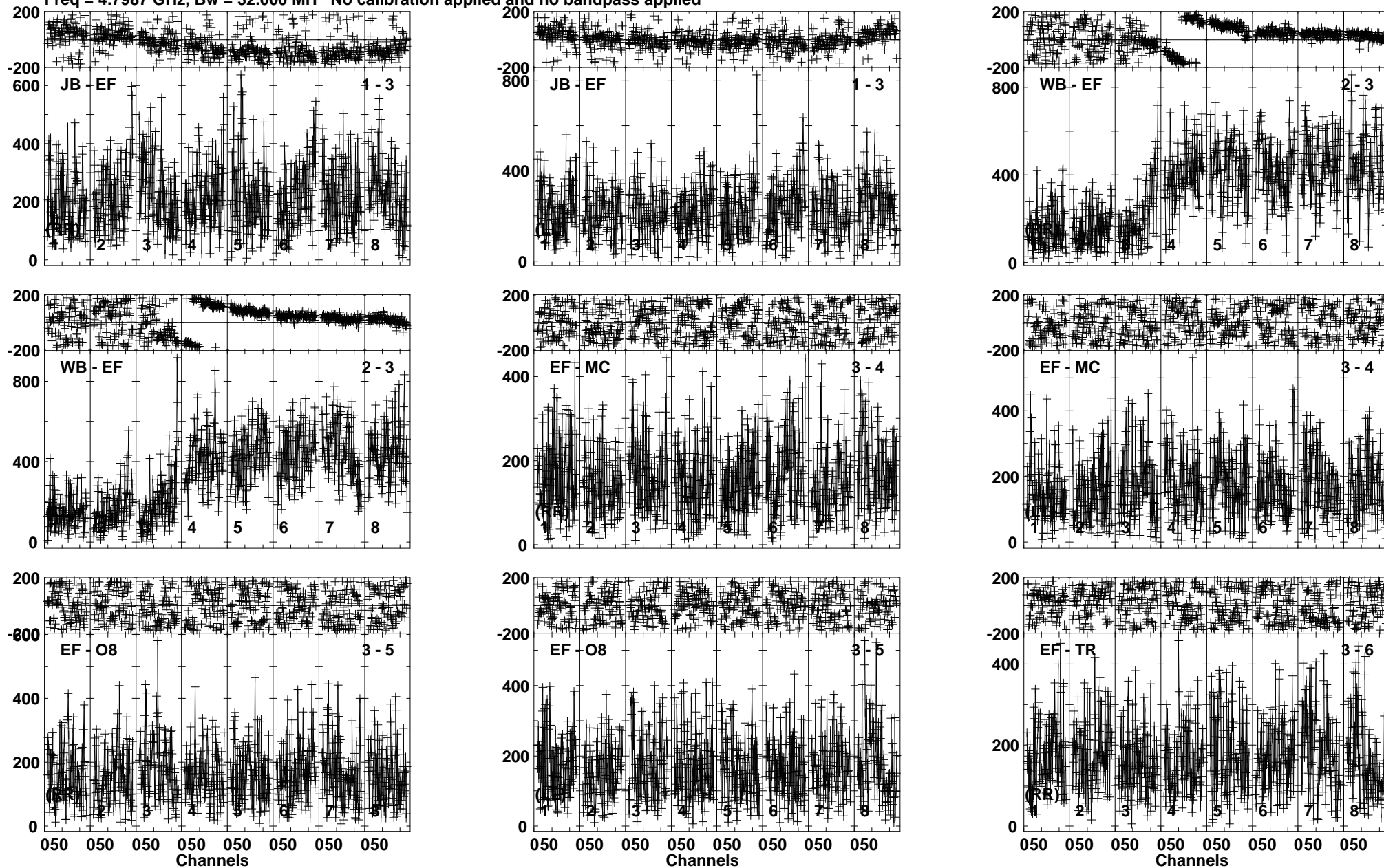
Lower frame: Micro Ampl Jy Top frame: Phas deg Vector averaged cross-power spectrum Baseline: JB (01) - EF (03) Timerange: 01/01:03:31 to 01/01:05:59
