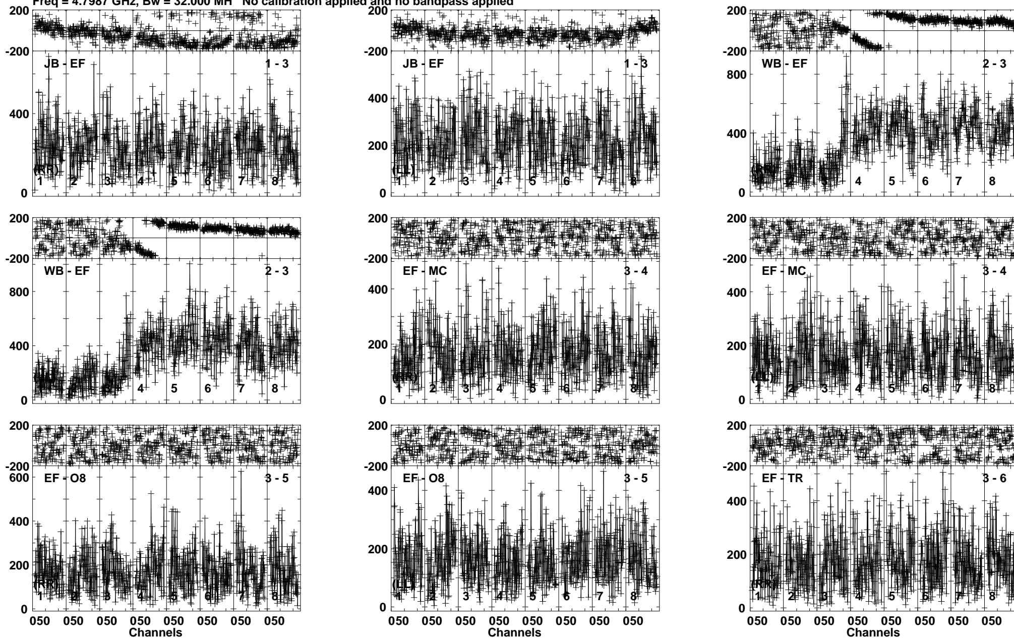
Lower frame: Micro Ampl Jy Top frame: Phas deg Vector averaged cross-power spectrum Baseline: JB (01) - EF (03) Timerange: 01/00:39:41 to 01/00:42:09
