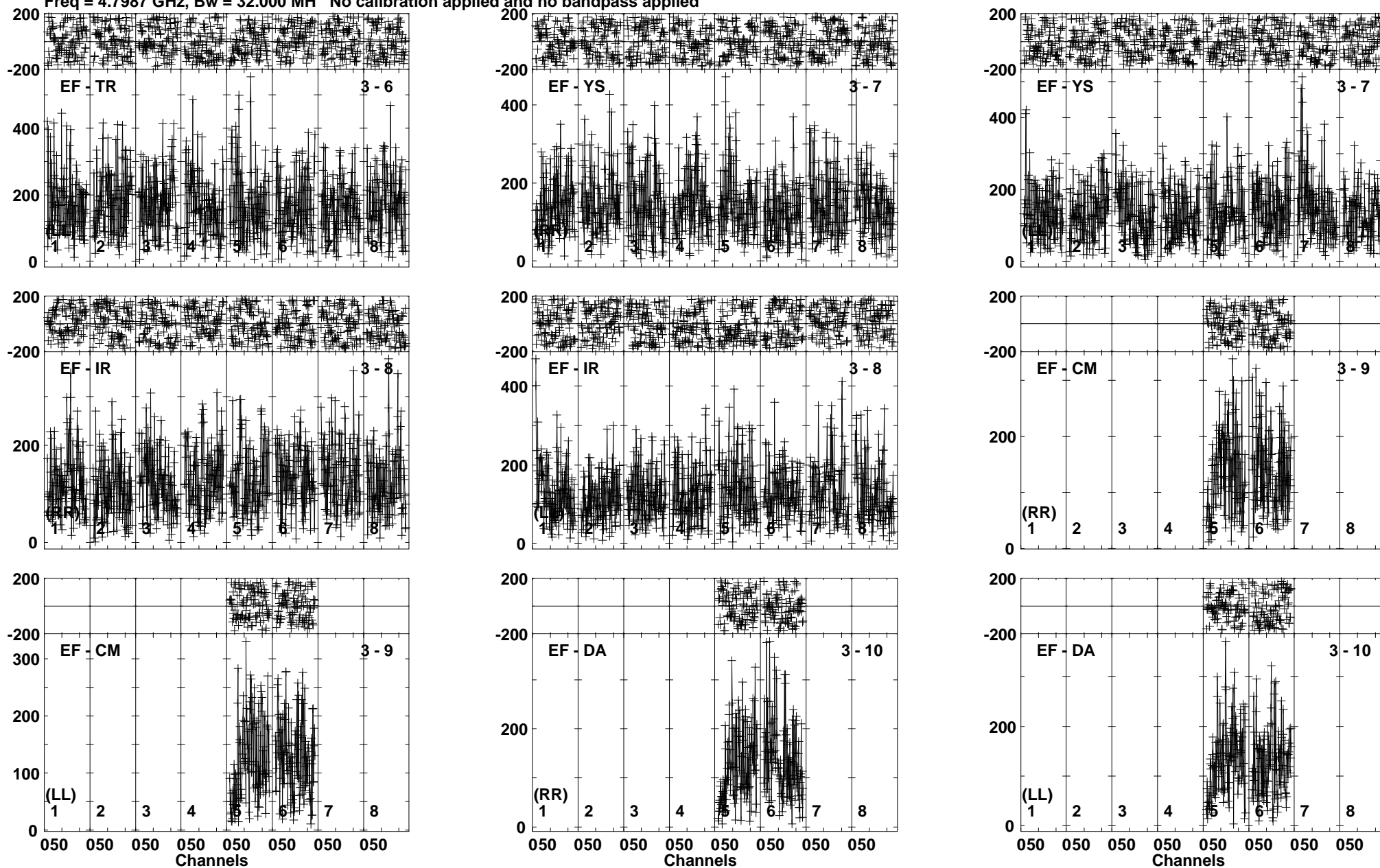
Lower frame: Micro Ampl Jy Top frame: Phas deg Vector averaged cross-power spectrum Baseline: EF (03) - TR (06) Timerange: 01/03:36:50 to 01/03:39:20
