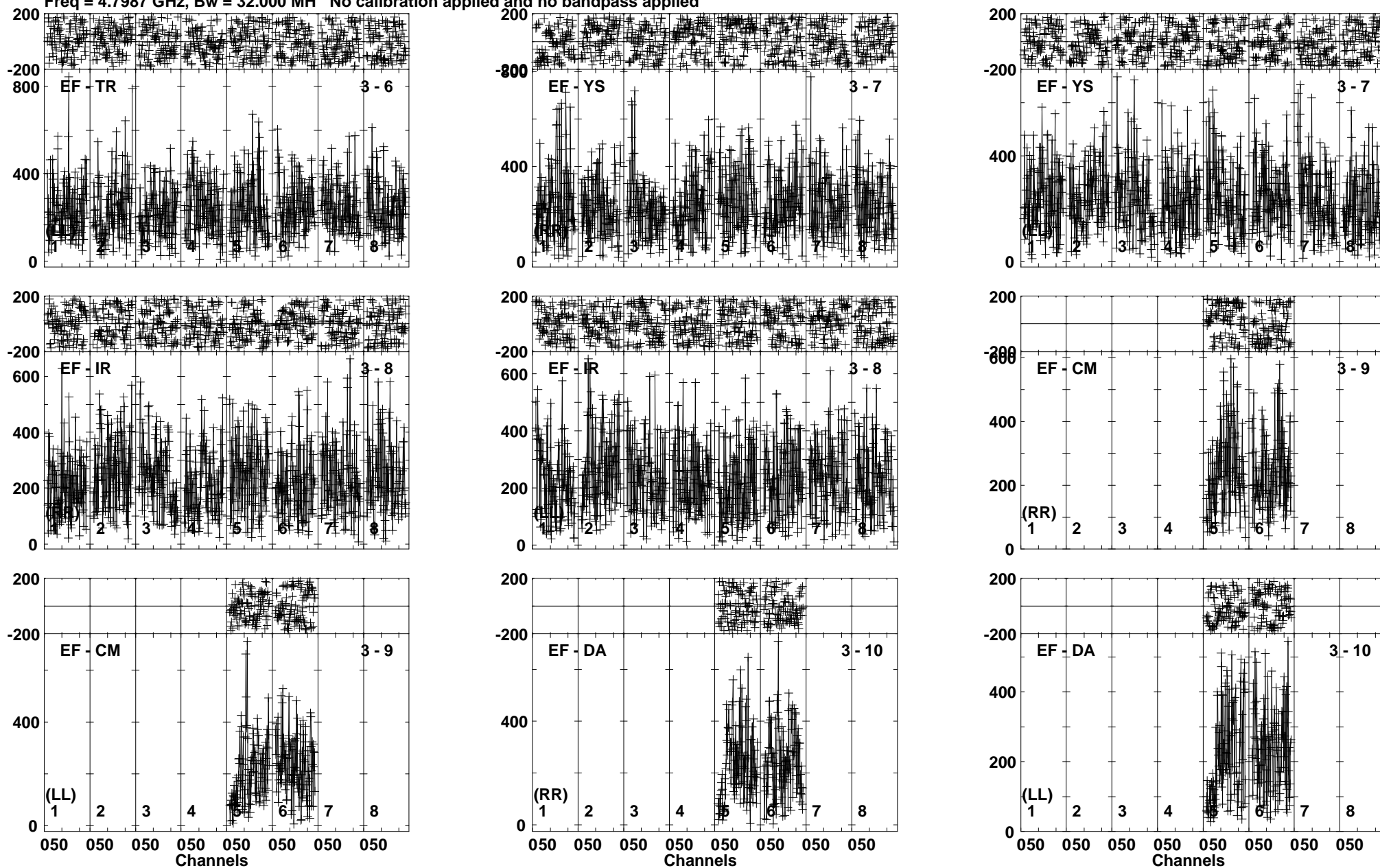
Lower frame: Micro Ampl Jy Top frame: Phas deg Vector averaged cross-power spectrum Baseline: EF (03) - TR (06) Timerange: 01/03:13:51 to 01/03:16:19
