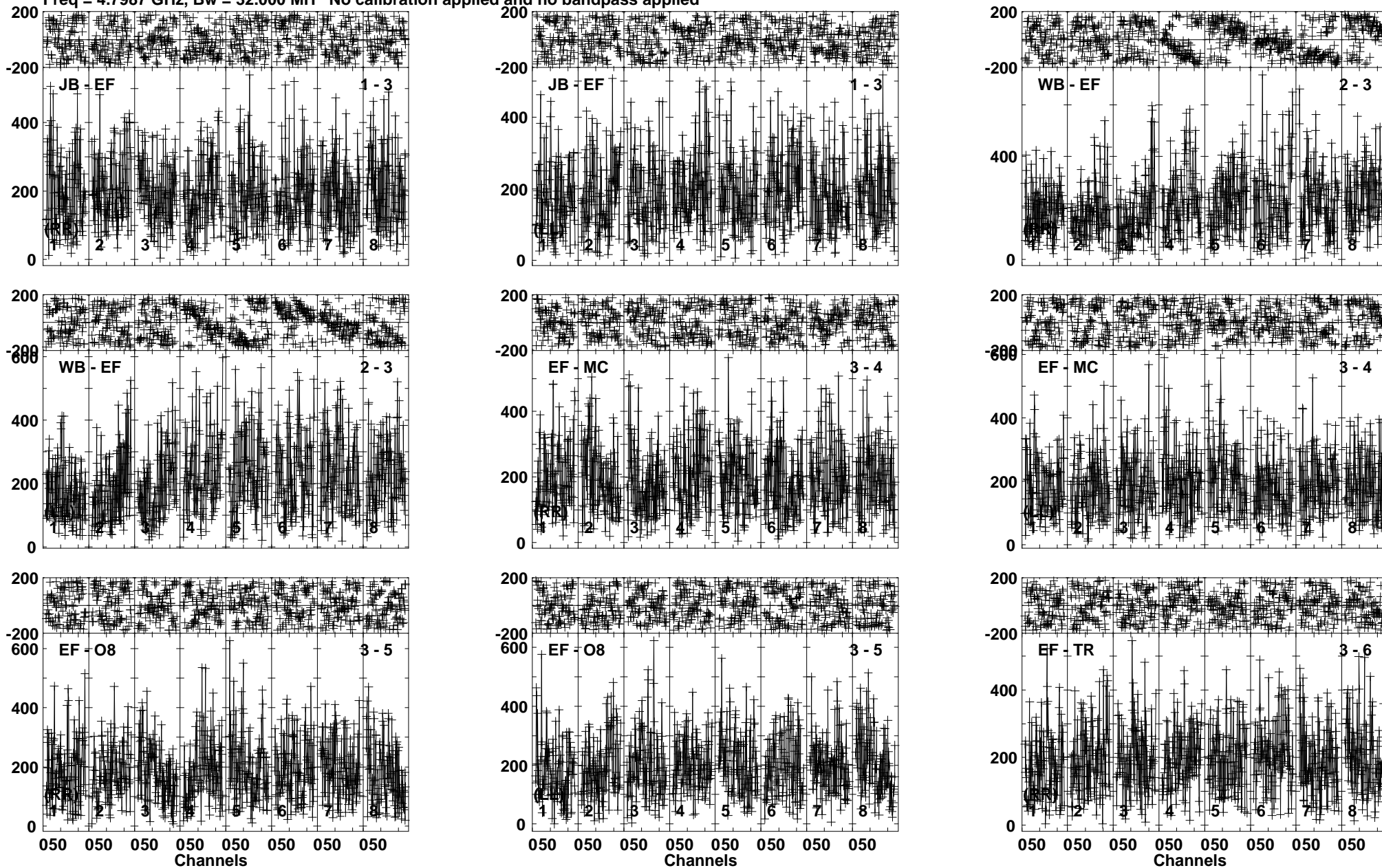
Lower frame: Micro Ampl Jy Top frame: Phas deg Vector averaged cross-power spectrum Baseline: JB (01) - EF (03) Timerange: 01/08:47:31 to 01/08:49:29
