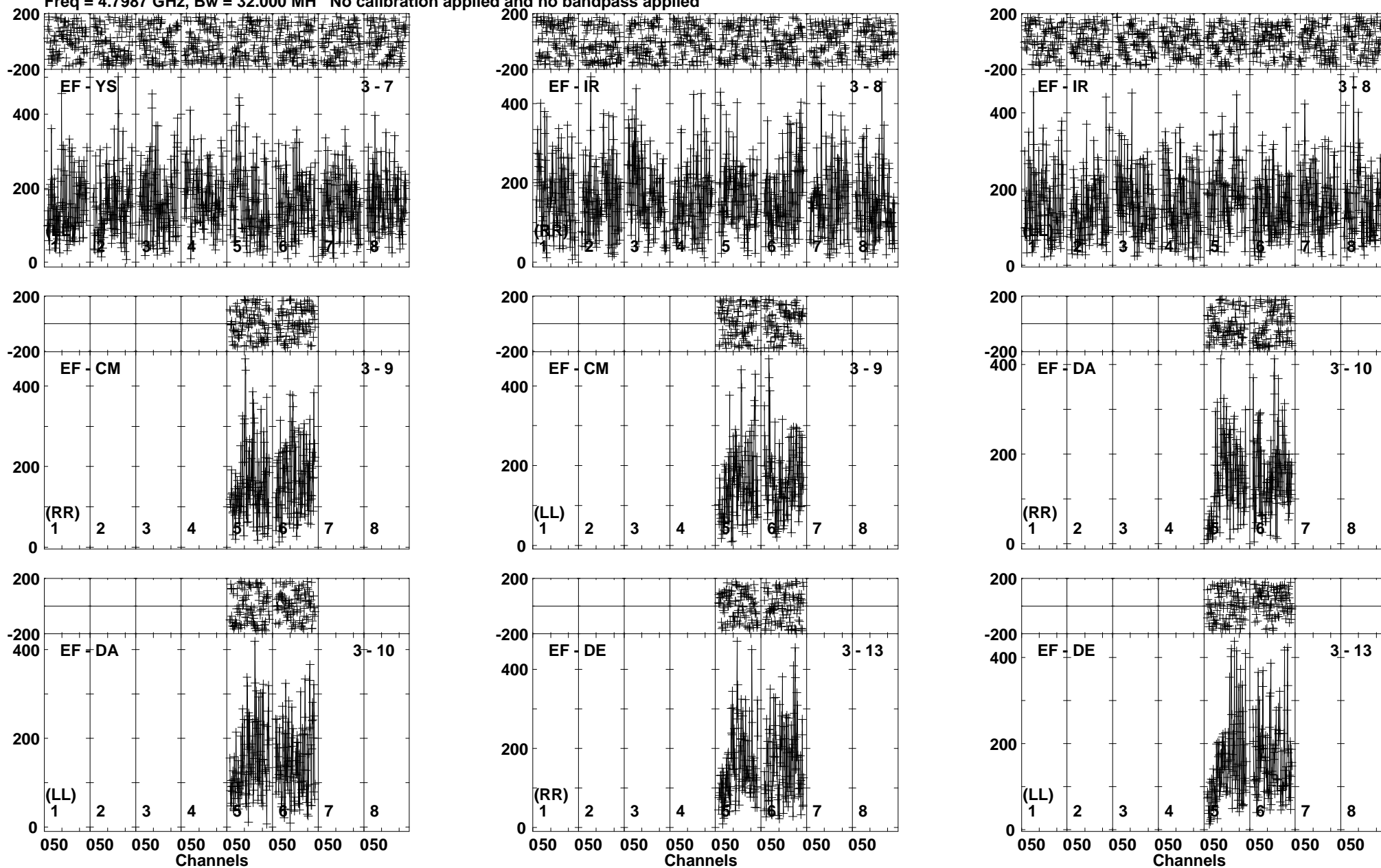
Lower frame: Micro Ampl Jy Top frame: Phas deg Vector averaged cross-power spectrum Baseline: EF (03) - YS (07) Timerange: 01/07:24:00 to 01/07:26:29
