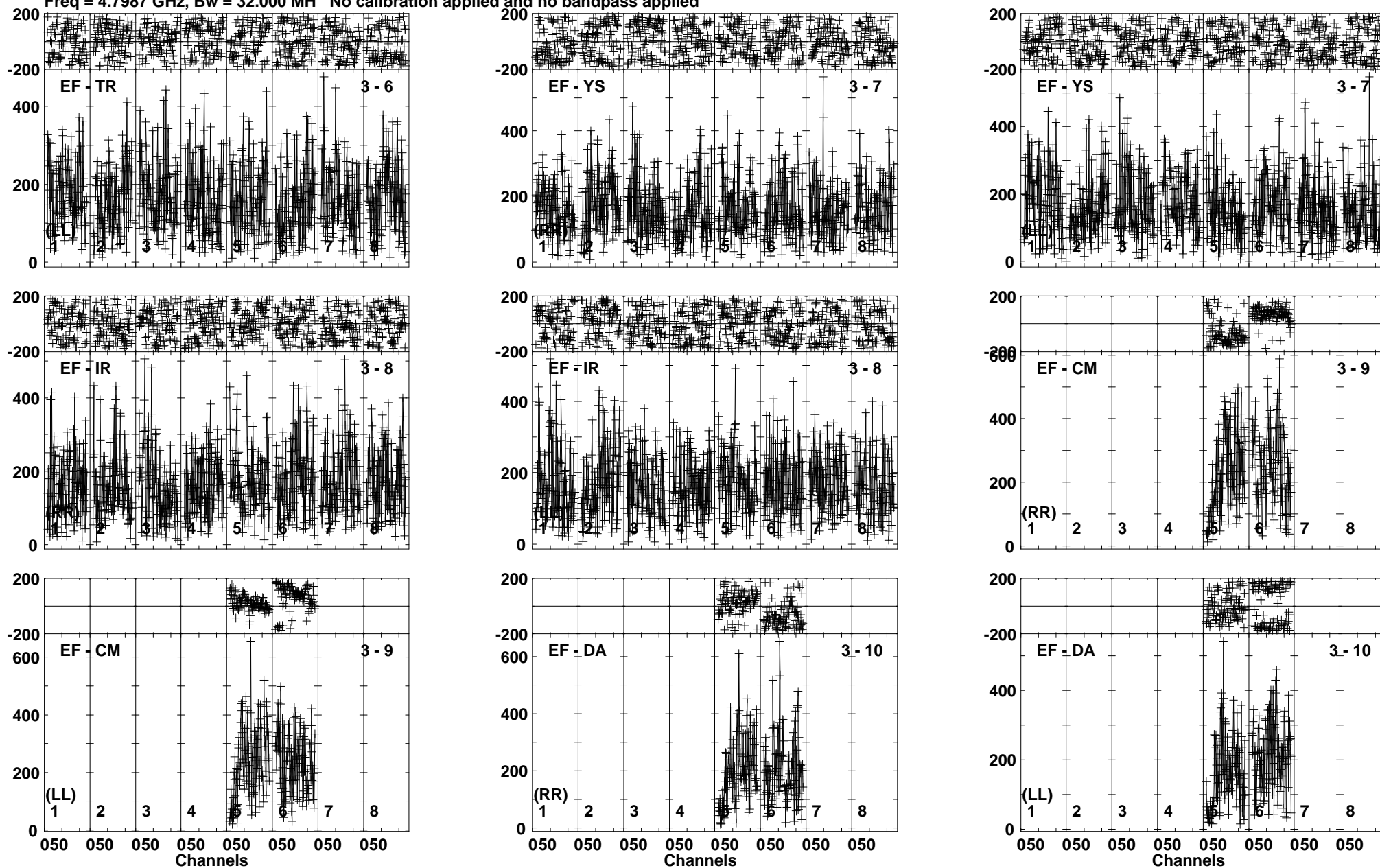
Lower frame: Micro Ampl Jy Top frame: Phas deg Vector averaged cross-power spectrum Baseline: EF (03) - TR (06) Timerange: 01/01:31:21 to 01/01:33:49
