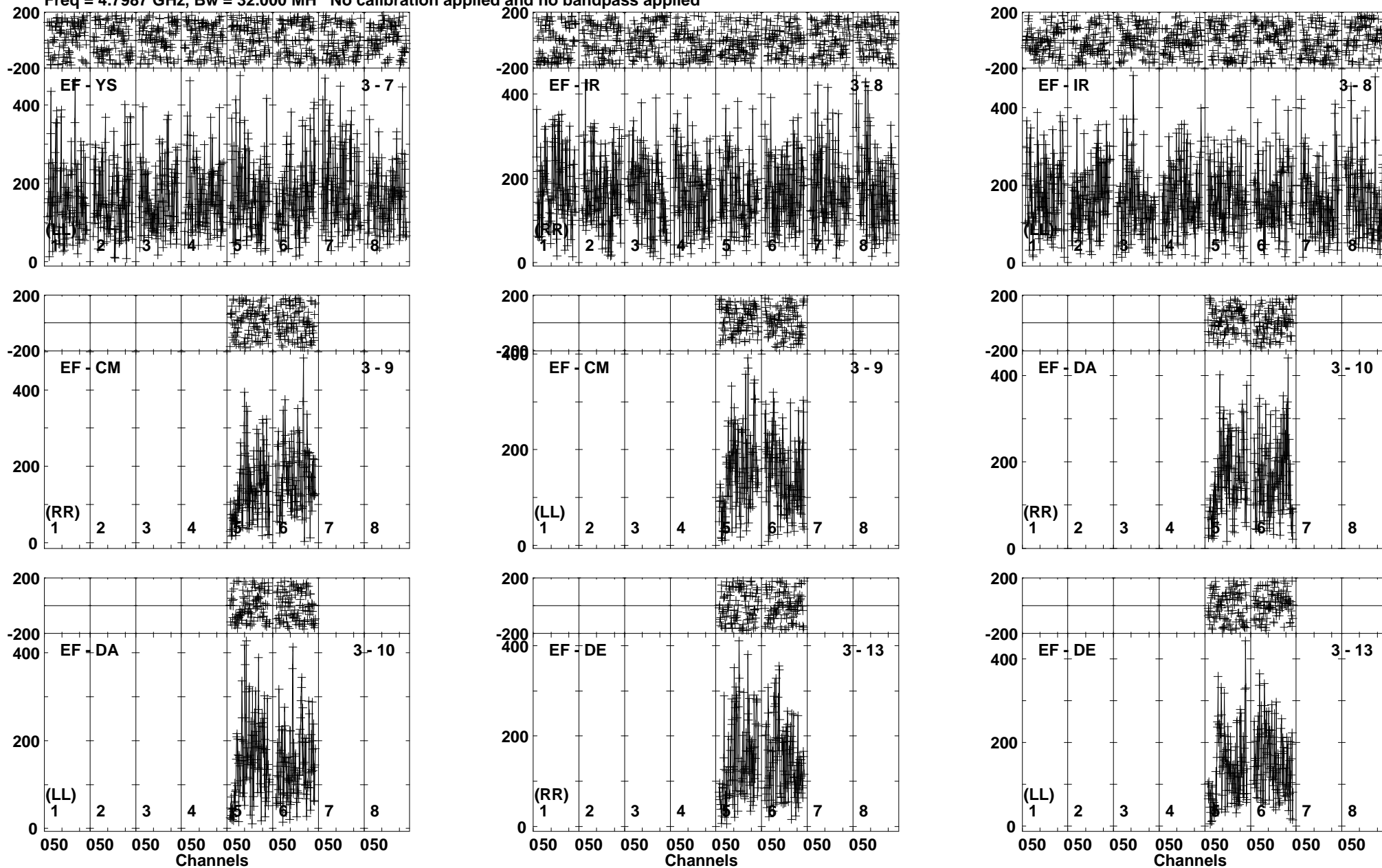
Lower frame: Micro Ampl Jy Top frame: Phas deg Vector averaged cross-power spectrum Baseline: EF (03) - YS (07) Timerange: 01/06:56:10 to 01/06:58:40
