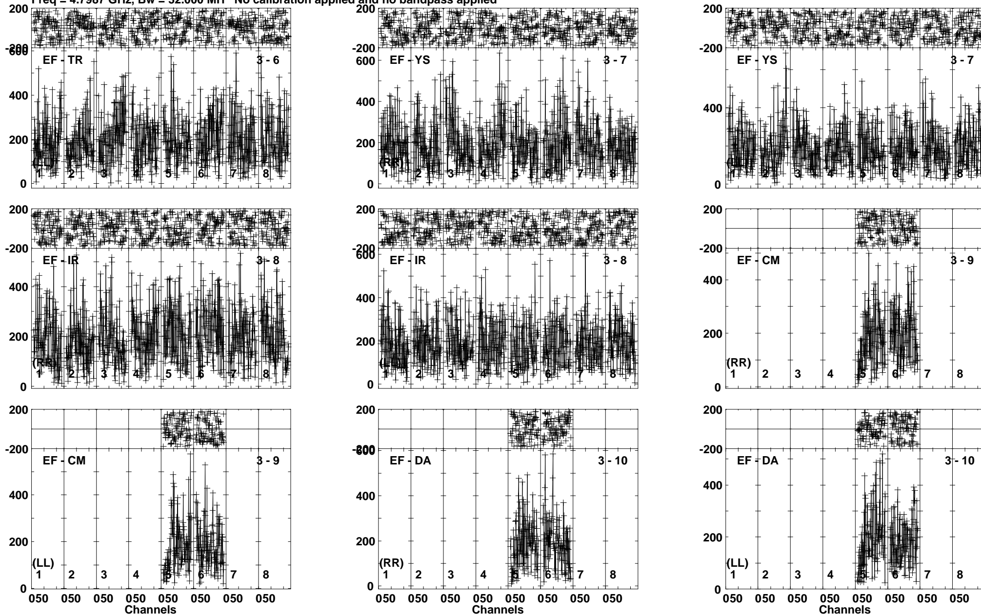
Lower frame: Micro Ampl Jy Top frame: Phas deg Vector averaged cross-power spectrum Baseline: EF (03) - TR (06) Timerange: 01/08:47:31 to 01/08:49:29
