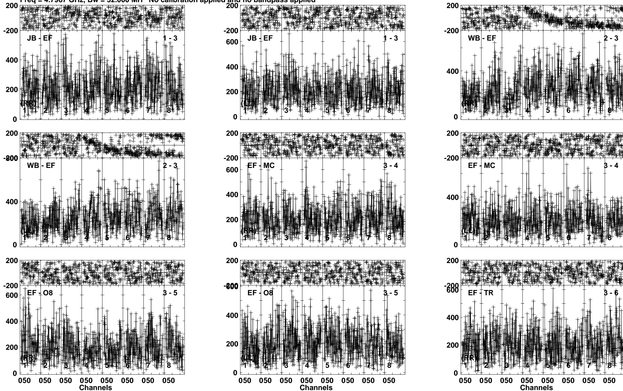
Lower frame: Micro Ampl Jy Top frame: Phas deg Vector averaged cross-power spectrum Baseline: JB (01) - EF (03) Timerange: 01/02:54:50 to 01/02:57:20
