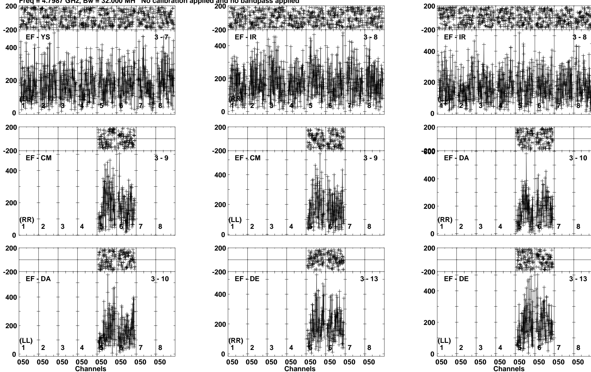
Lower frame: Micro Ampl Jy Top frame: Phas deg Vector averaged cross-power spectrum Baseline: EF (03) - YS (07) Timerange: 01/06:00:30 to 01/06:03:00
