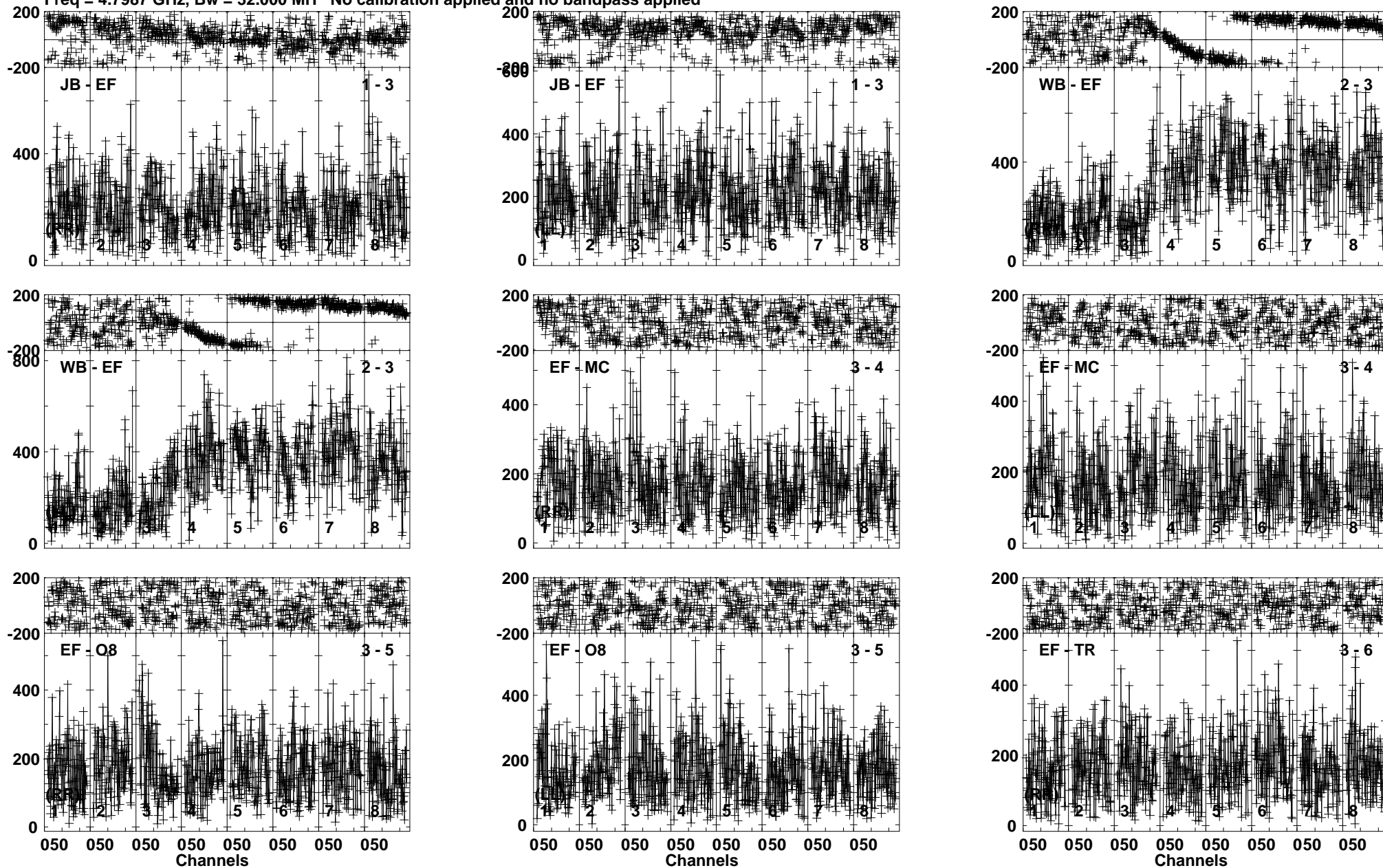
Lower frame: Micro Ampl Jy Top frame: Phas deg Vector averaged cross-power spectrum Baseline: JB (01) - EF (03) Timerange: 01/01:35:20 to 01/01:37:50
