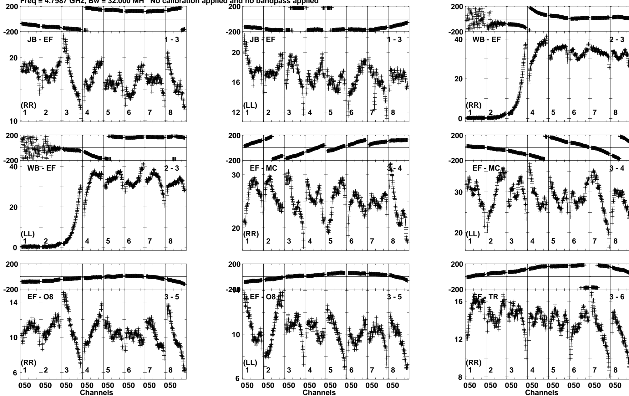
Lower frame: Milli Ampl Jy Top frame: Phas deg Vector averaged cross-power spectrum Baseline: JB (01) - EF (03) Timerange: 00/23:33:37 to 00/23:35:00
