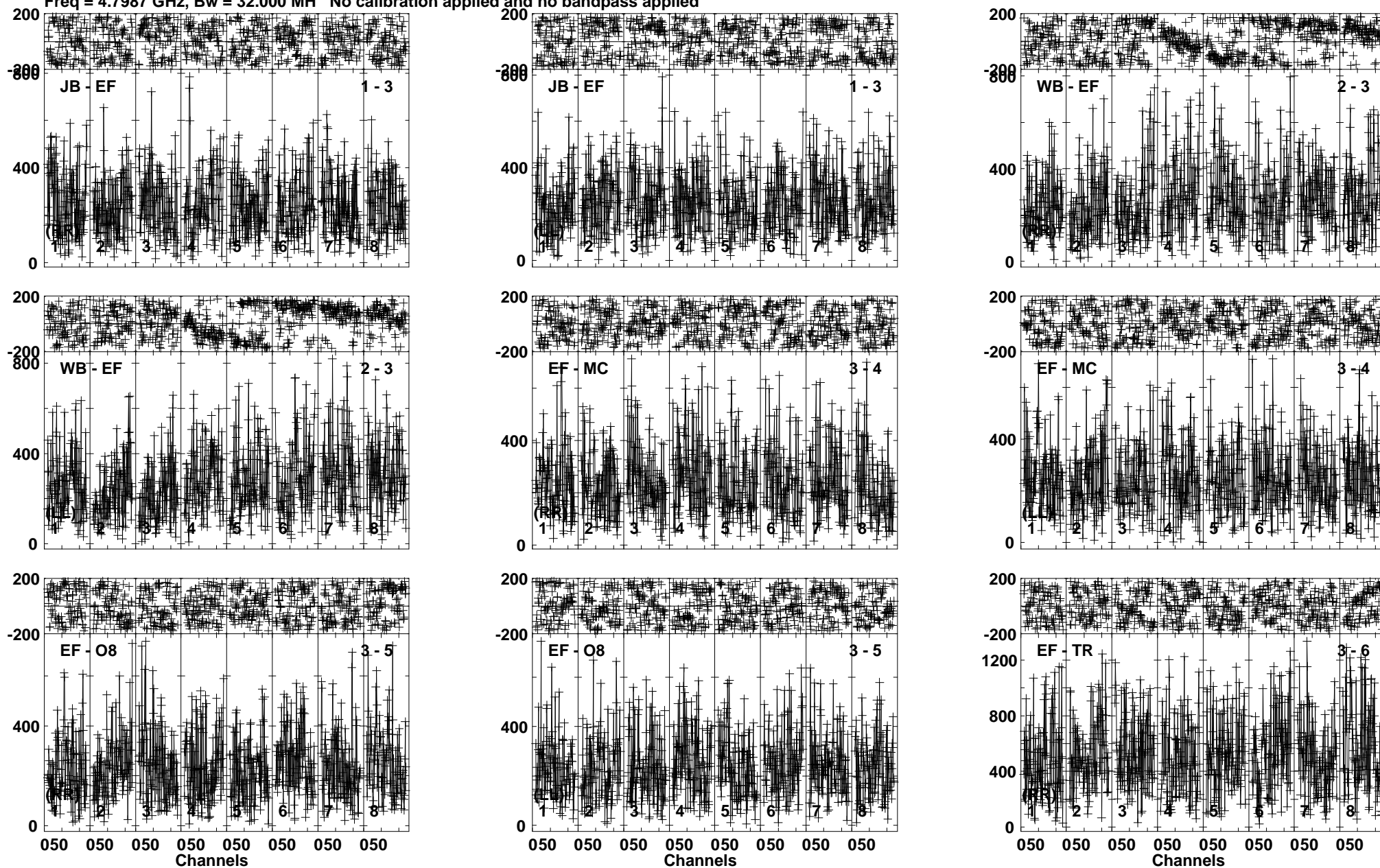
Lower frame: Micro Ampl Jy Top frame: Phas deg Vector averaged cross-power spectrum Baseline: JB (01) - EF (03) Timerange: 01/02:58:50 to 01/03:01:20
