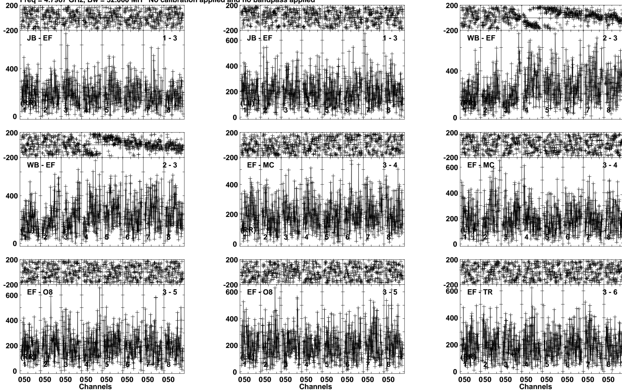
Lower frame: Micro Ampl Jy Top frame: Phas deg Vector averaged cross-power spectrum Baseline: JB (01) - EF (03) Timerange: 01/02:50:00 to 01/02:52:30
