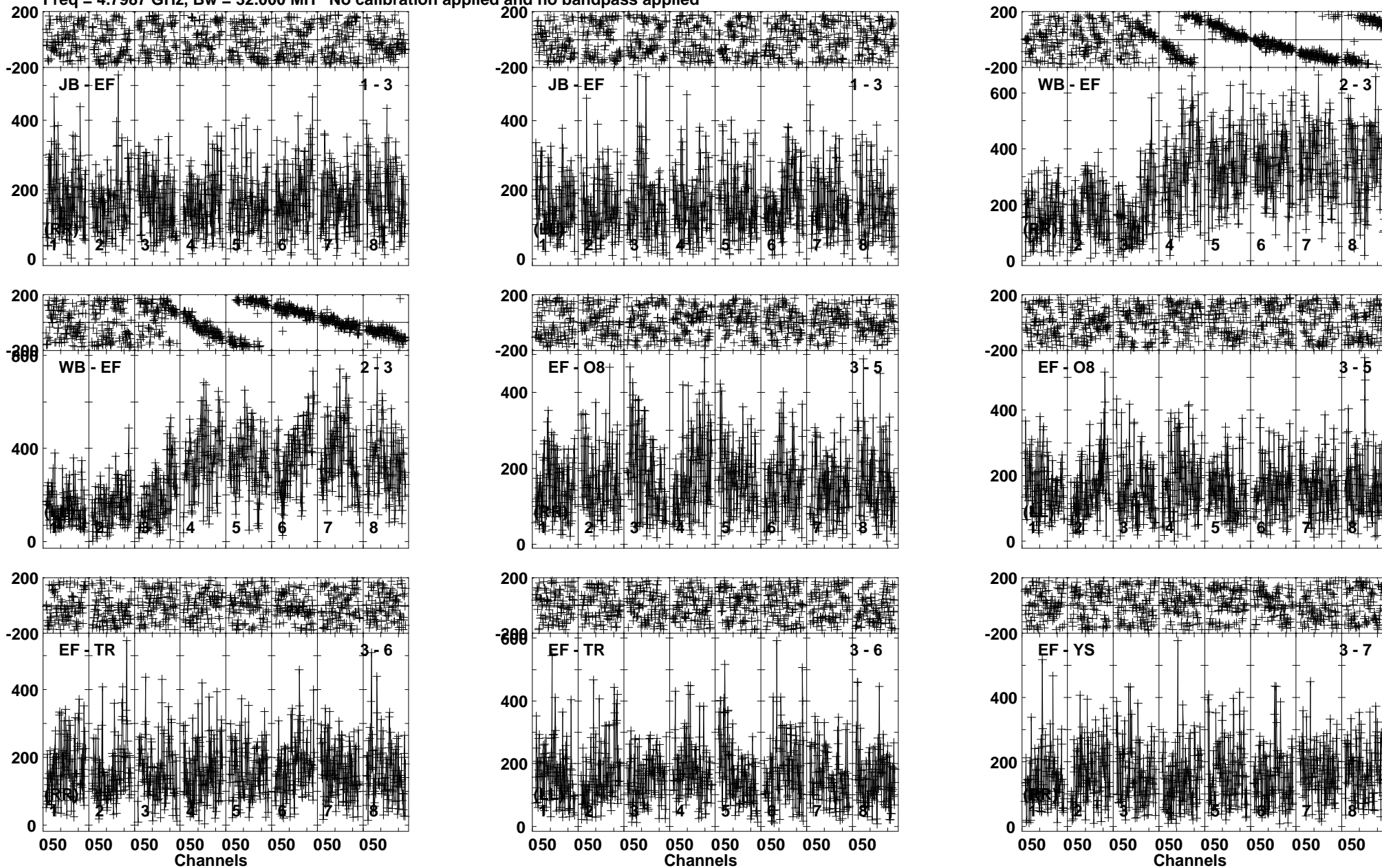
Lower frame: Micro Ampl Jy Top frame: Phas deg Vector averaged cross-power spectrum Baseline: JB (01) - EF (03) Timerange: 01/06:43:21 to 01/06:45:50
