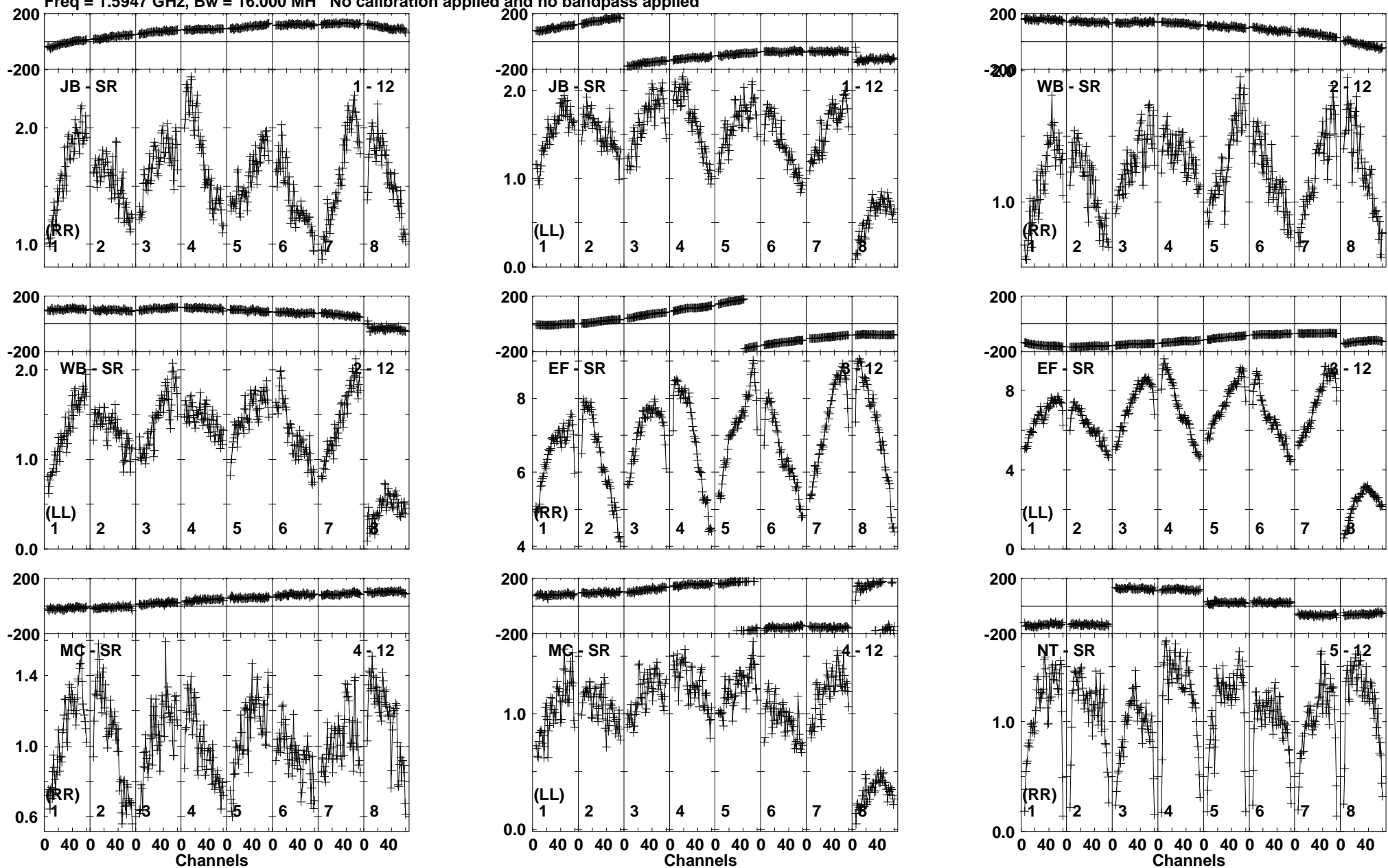
Lower frame: Milli Ampl Jy Top frame: Phas deg Vector averaged cross-power spectrum Baseline: JB (01) - SR (12) Timerange: 00/11:17:00 to 00/11:19:00
