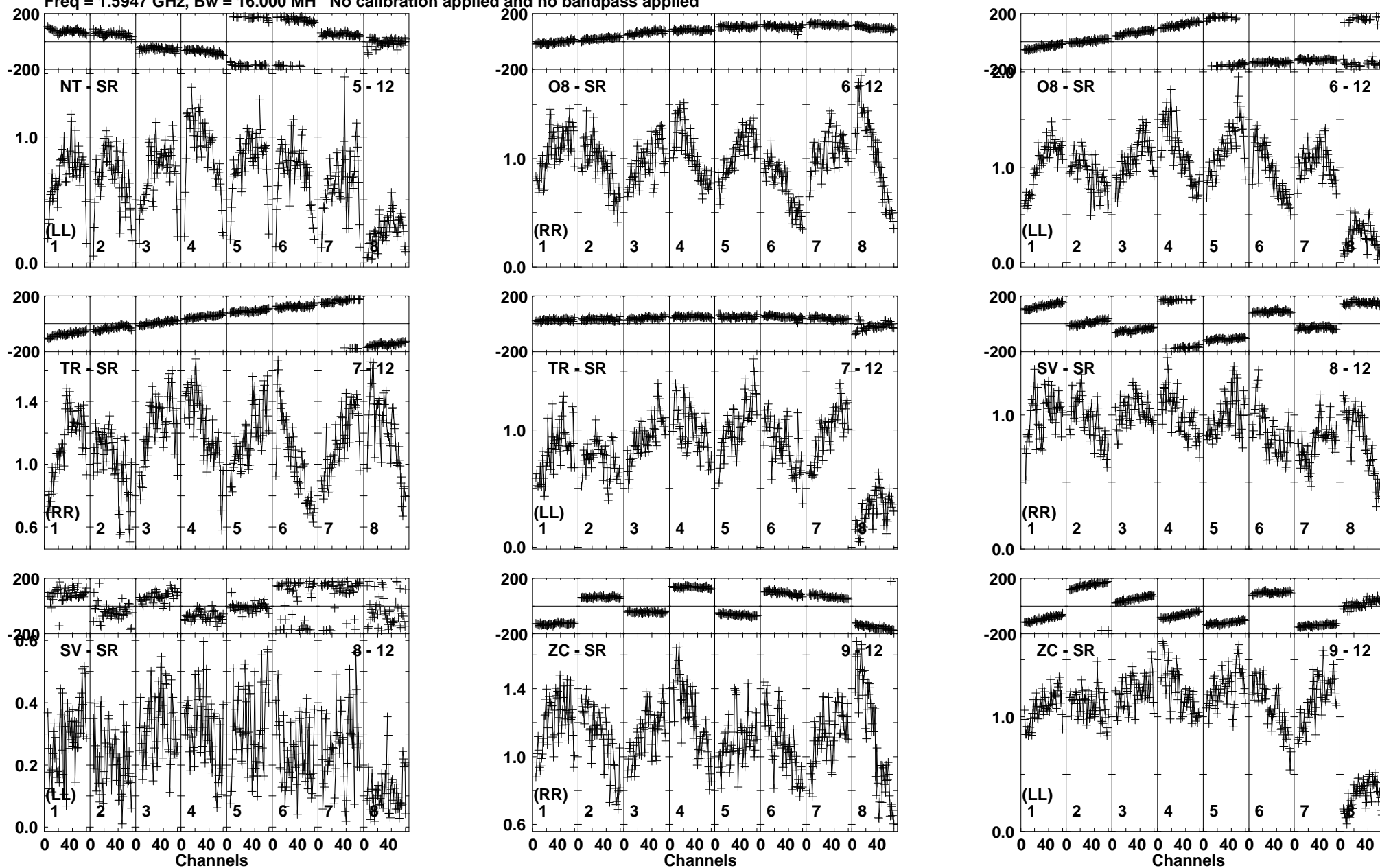
Lower frame: Milli Ampl Jy Top frame: Phas deg Vector averaged cross-power spectrum Baseline: NT (05) - SR (12) Timerange: 00/11:15:31 to 00/11:17:00
