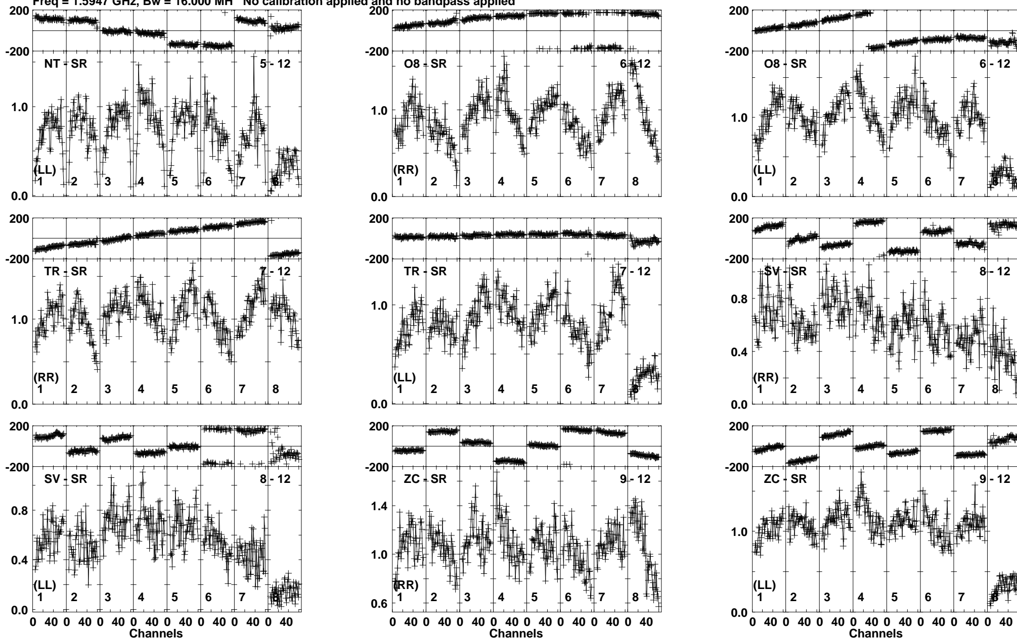
Lower frame: Milli Ampl Jy Top frame: Phas deg Vector averaged cross-power spectrum Baseline: NT (05) - SR (12) Timerange: 00:12:39:30 to 00:12:41:00
