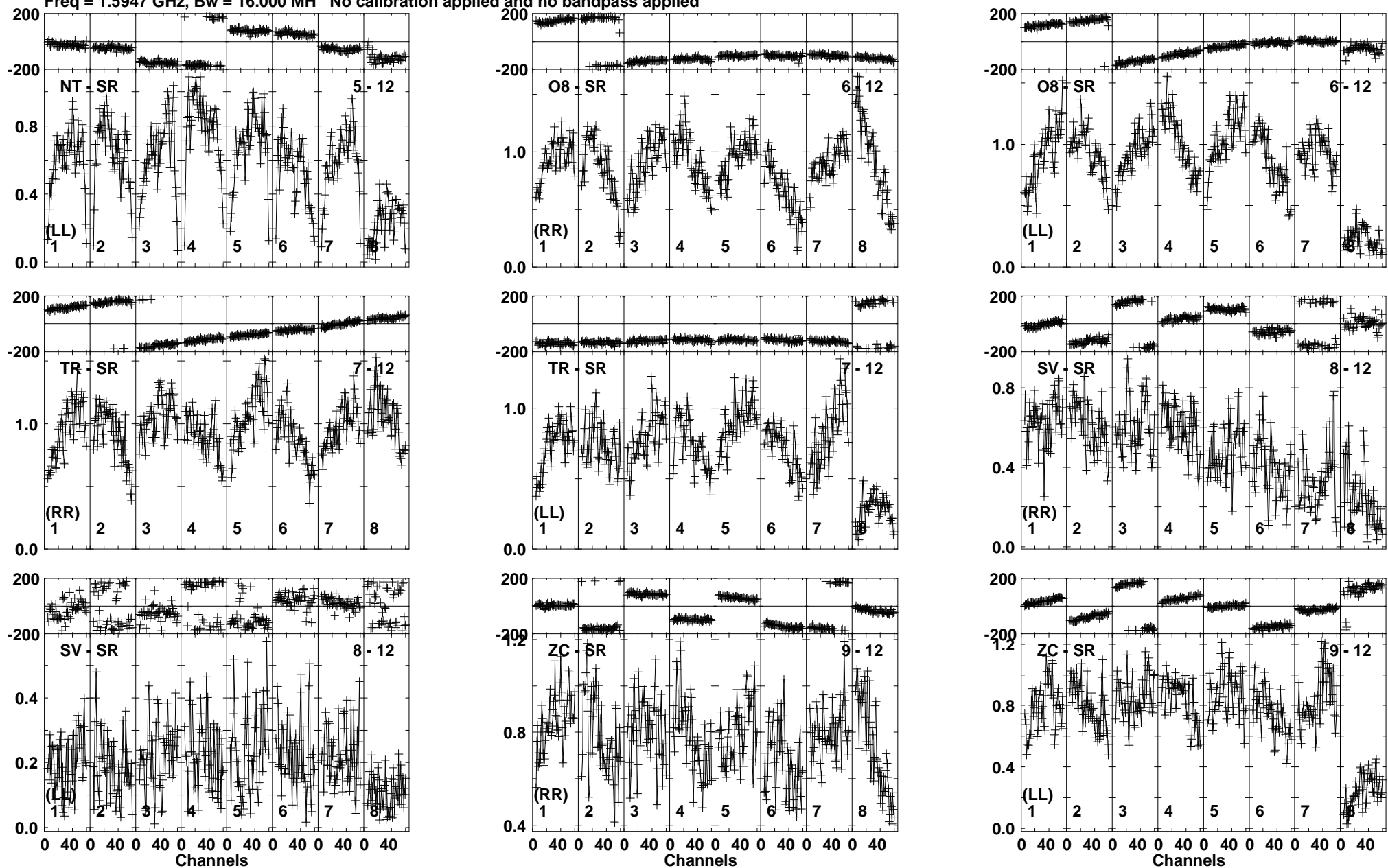
Lower frame: Milli Ampl Jy Top frame: Phas deg Vector averaged cross-power spectrum Baseline: NT (05) - SR (12) Timerange: 00/11:49:01 to 00/11:51:00
