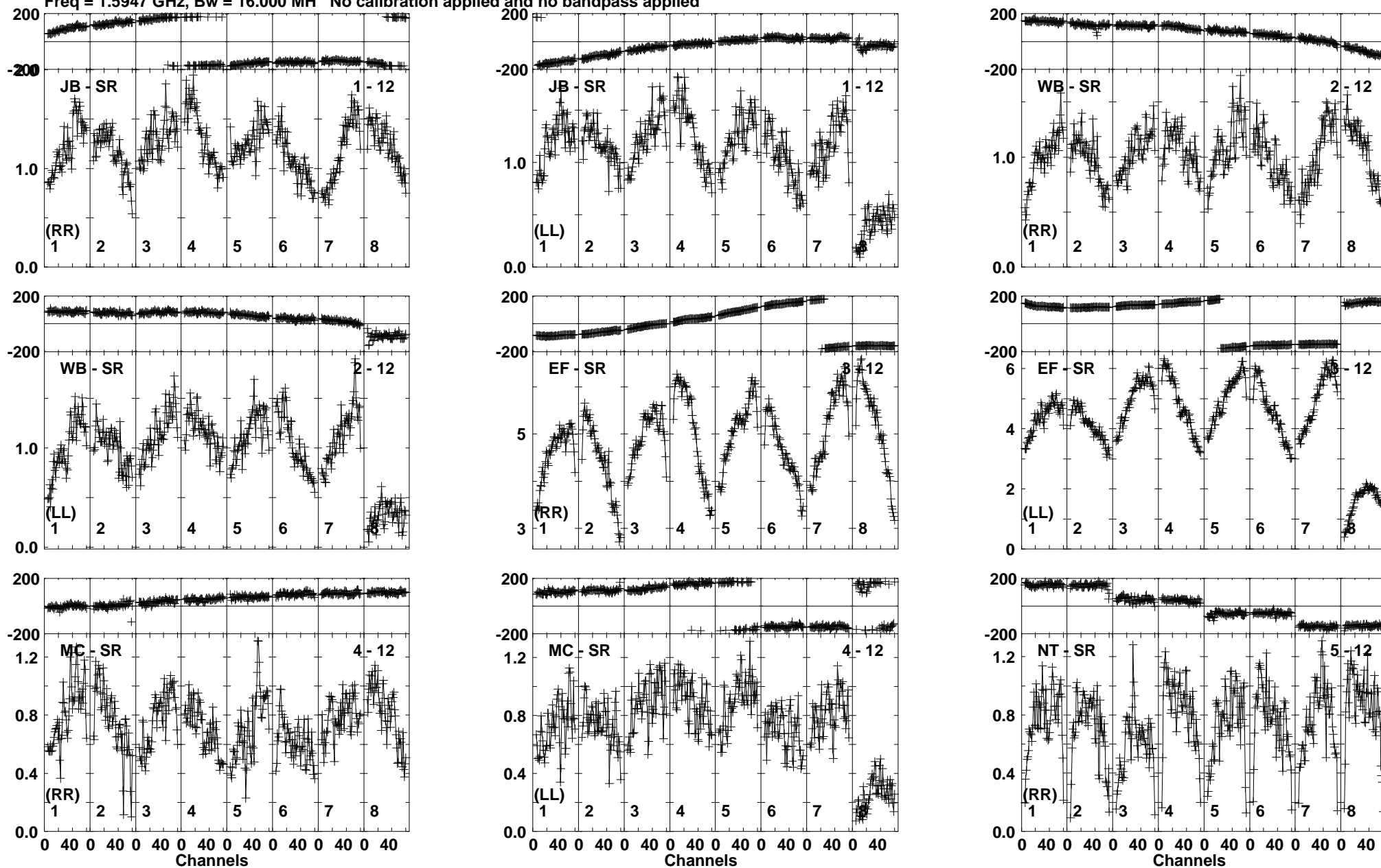
Lower frame: Milli Ampl Jy Top frame: Phas deg Vector averaged cross-power spectrum Baseline: JB (01) - SR (12) Timerange: 00/11:51:31 to 00/11:52:59
