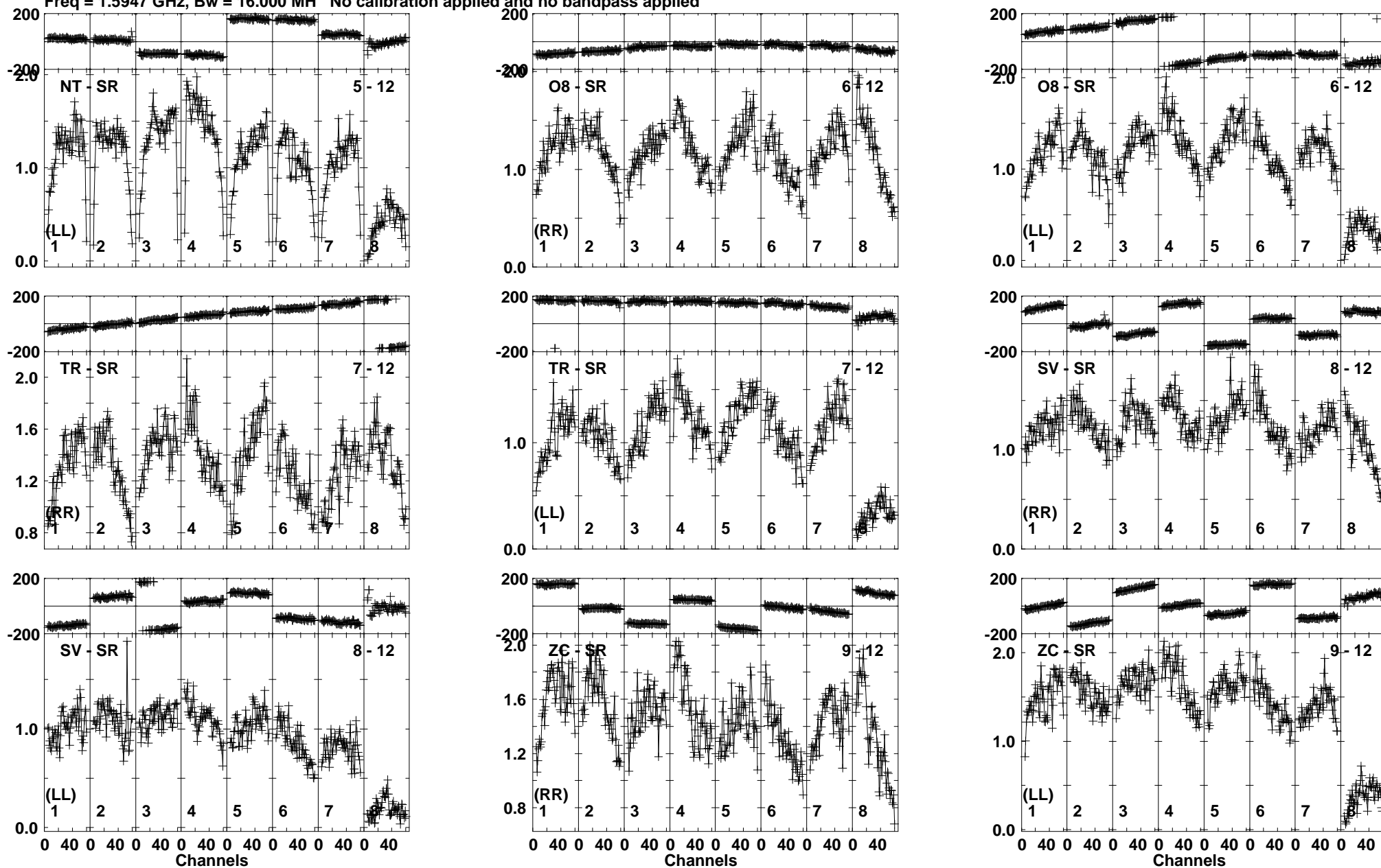
Lower frame: Milli Ampl Jy Top frame: Phas deg Vector averaged cross-power spectrum Baseline: NT (05) - SR (12) Timerange: 00/07:53:00 to 00/07:54:59
