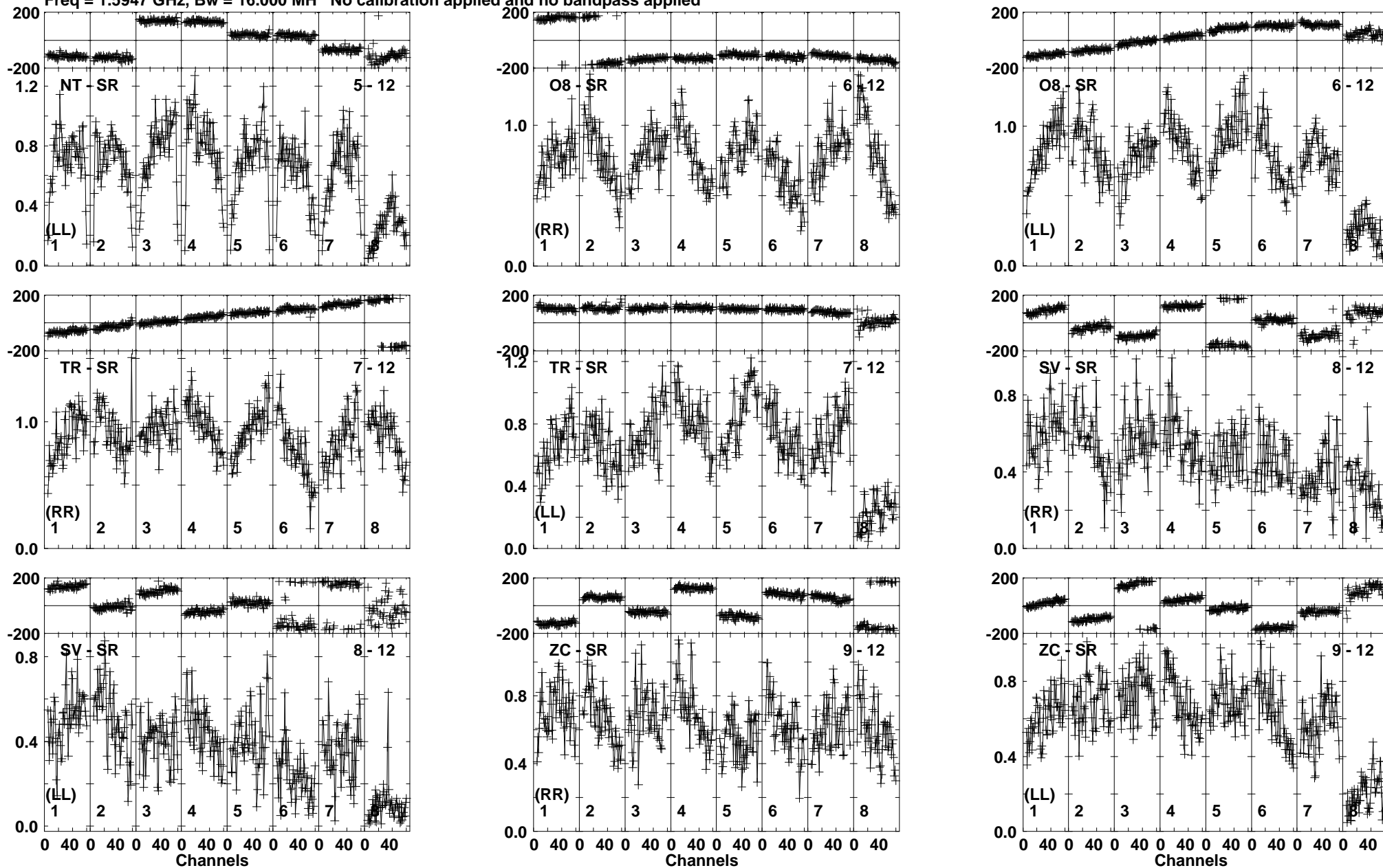
Lower frame: Milli Ampl Jy Top frame: Phas deg Vector averaged cross-power spectrum Baseline: NT (05) - SR (12) Timerange: 00/08:37:00 to 00/08:38:59
