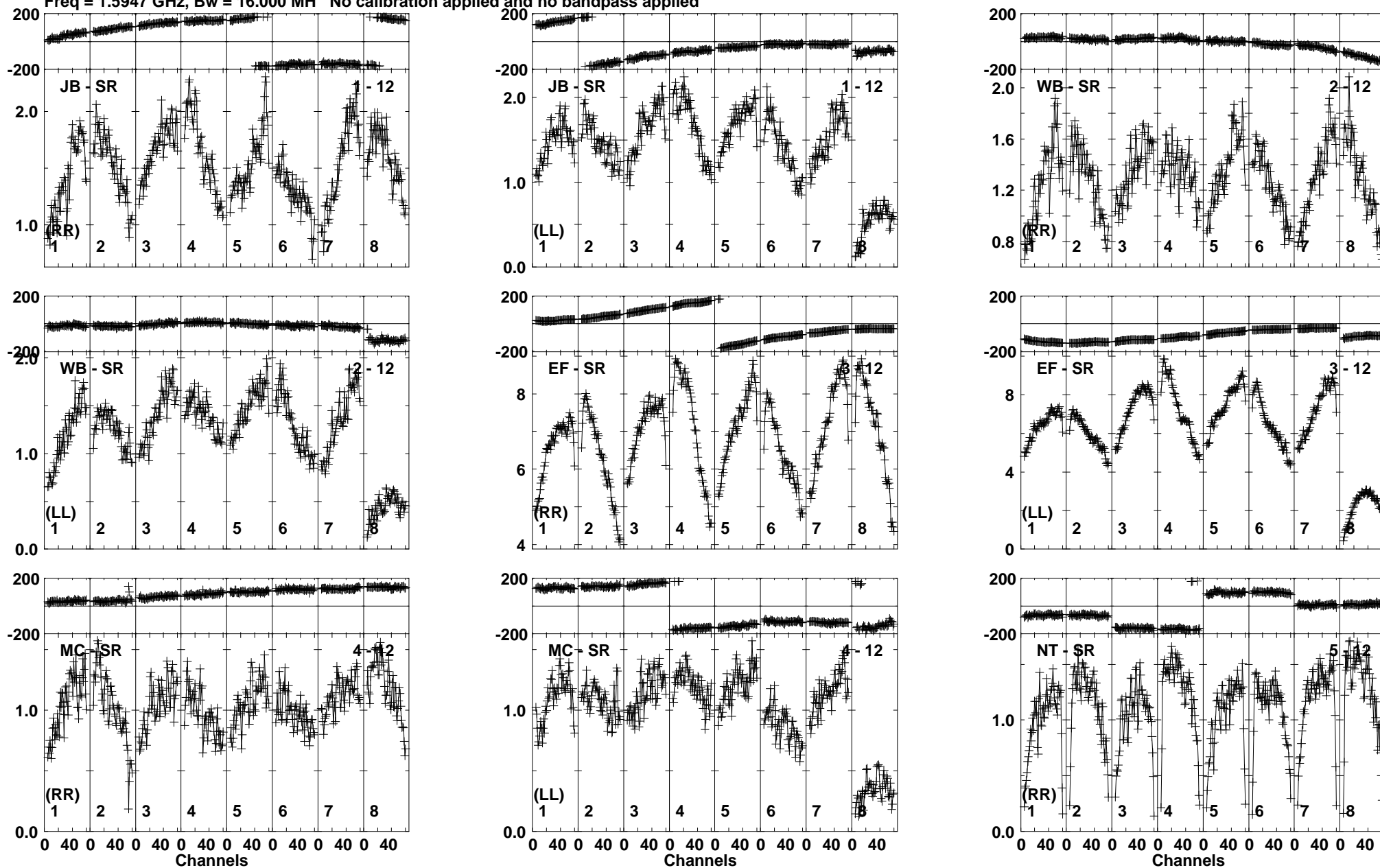
Lower frame: Milli Ampl Jy Top frame: Phas deg Vector averaged cross-power spectrum Baseline: JB (01) - SR (12) Timerange: 00/10/35:00 to 00/10/36:59
