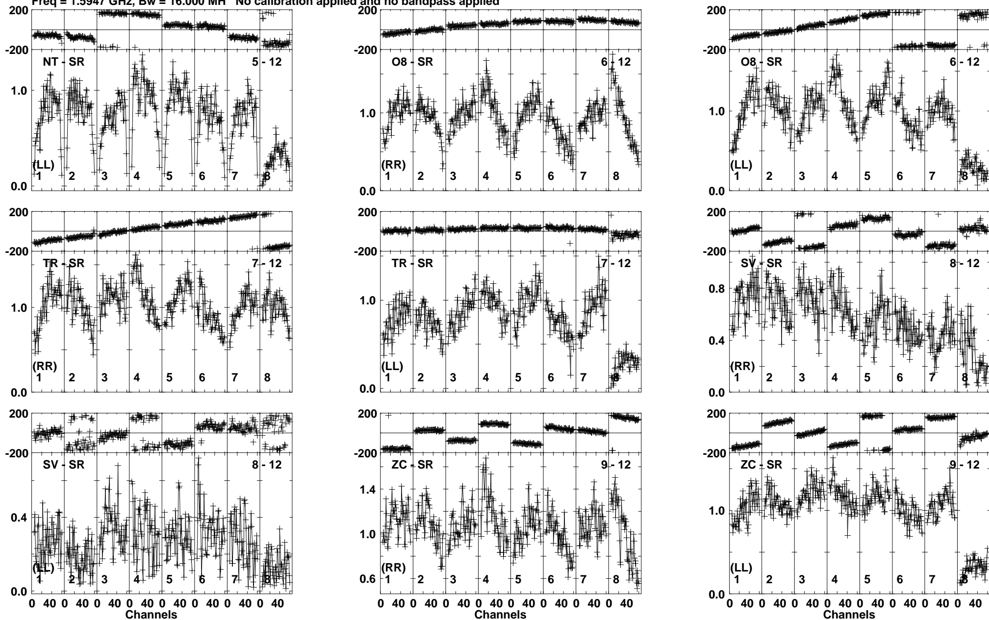
Lower frame: Milli Ampl Jy Top frame: Phas deg Vector averaged cross-power spectrum Baseline: NT (05) - SR (12) Timerange: 00/12:27:30 to 00/12:28:59
