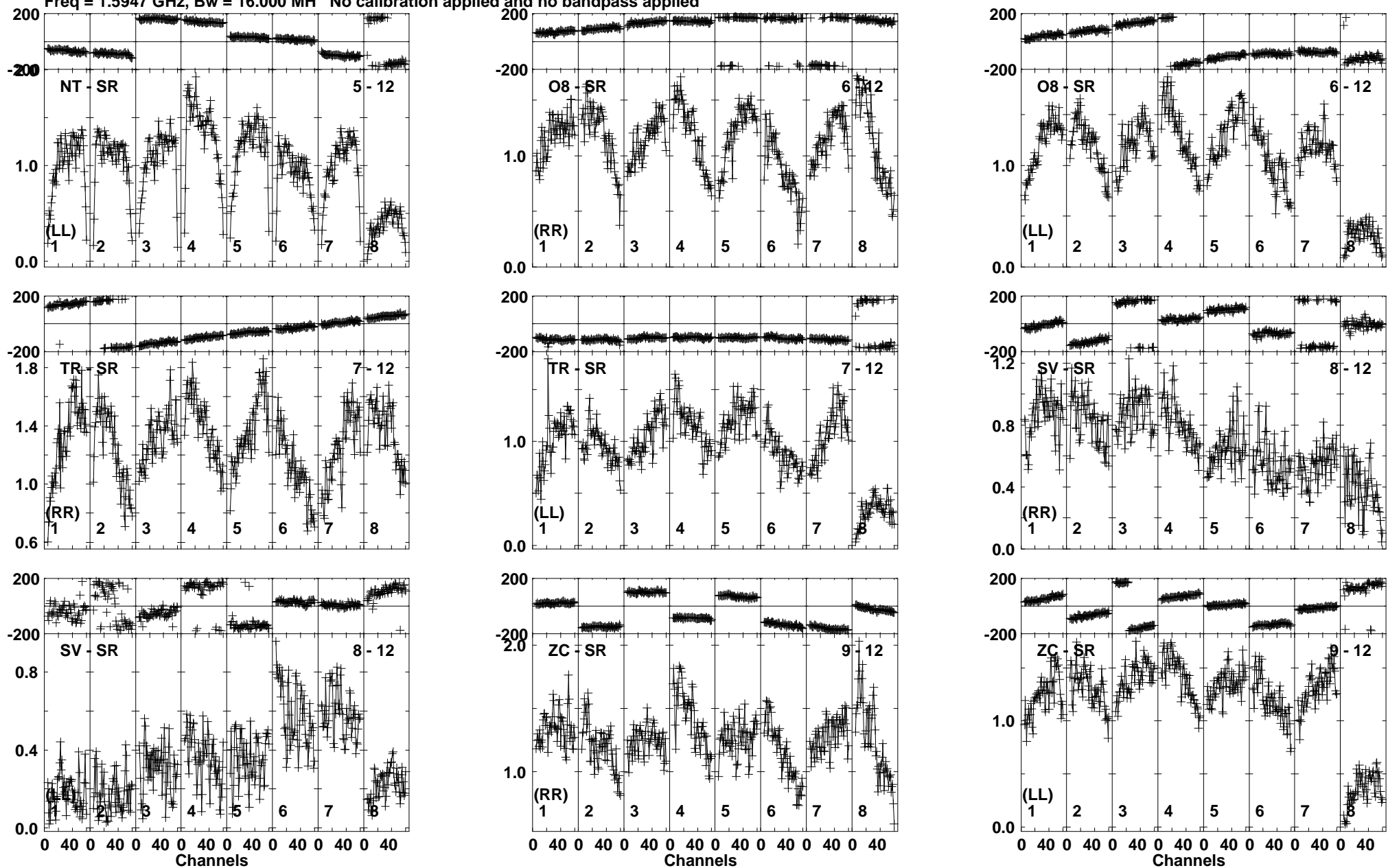
Lower frame: Milli Ampl Jy Top frame: Phas deg Vector averaged cross-power spectrum Baseline: NT (05) - SR (12) Timerange: 00/11:41:00 to 00/11:43:00
