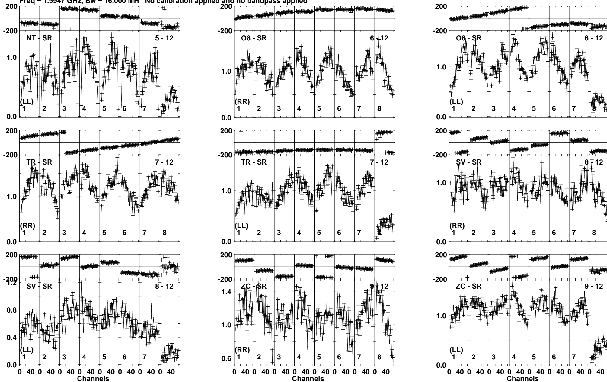
Lower frame: Milli Ampl Jy Top frame: Phas deg Vector averaged cross-power spectrum Baseline: NT (05) - SR (12) Timerange: 00/10:21:31 to 00/10:22:59
