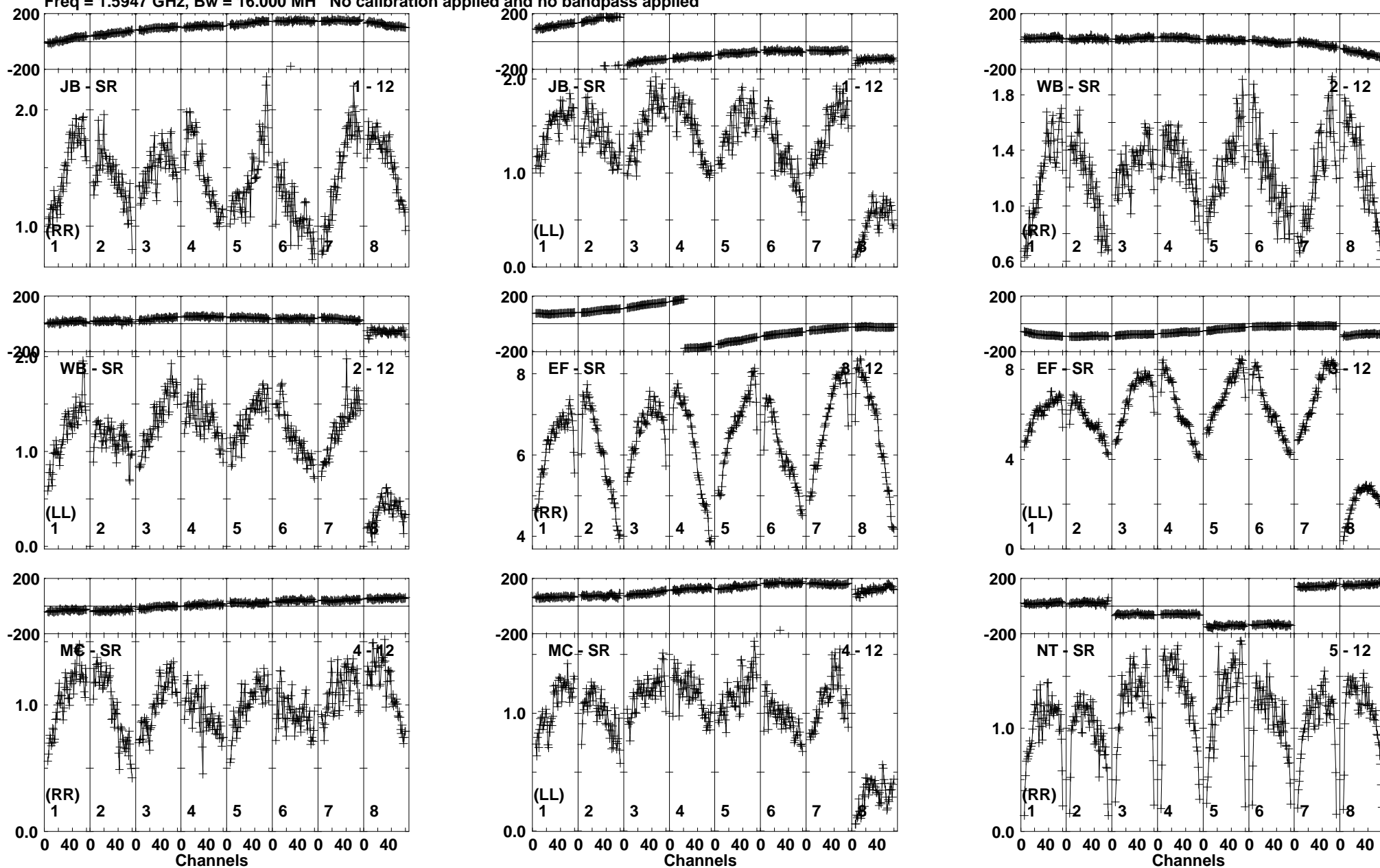
Lower frame: Milli Ampl Jy Top frame: Phas deg Vector averaged cross-power spectrum Baseline: JB (01) - SR (12) Timerange: 00/09:29:00 to 00/09:30:59
