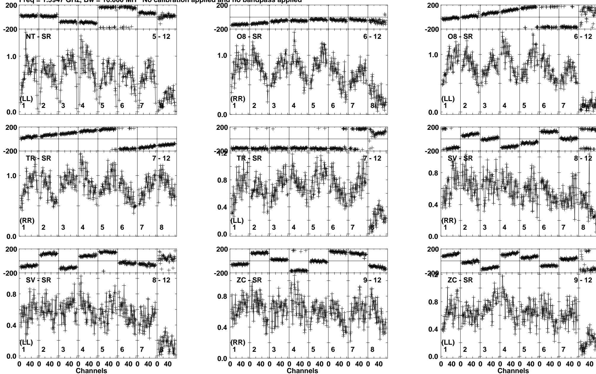
Lower frame: Milli Ampl Jy Top frame: Phas deg Vector averaged cross-power spectrum Baseline: NT (05) - SR (12) Timerange: 00/08:31:00 to 00/08:32:59
