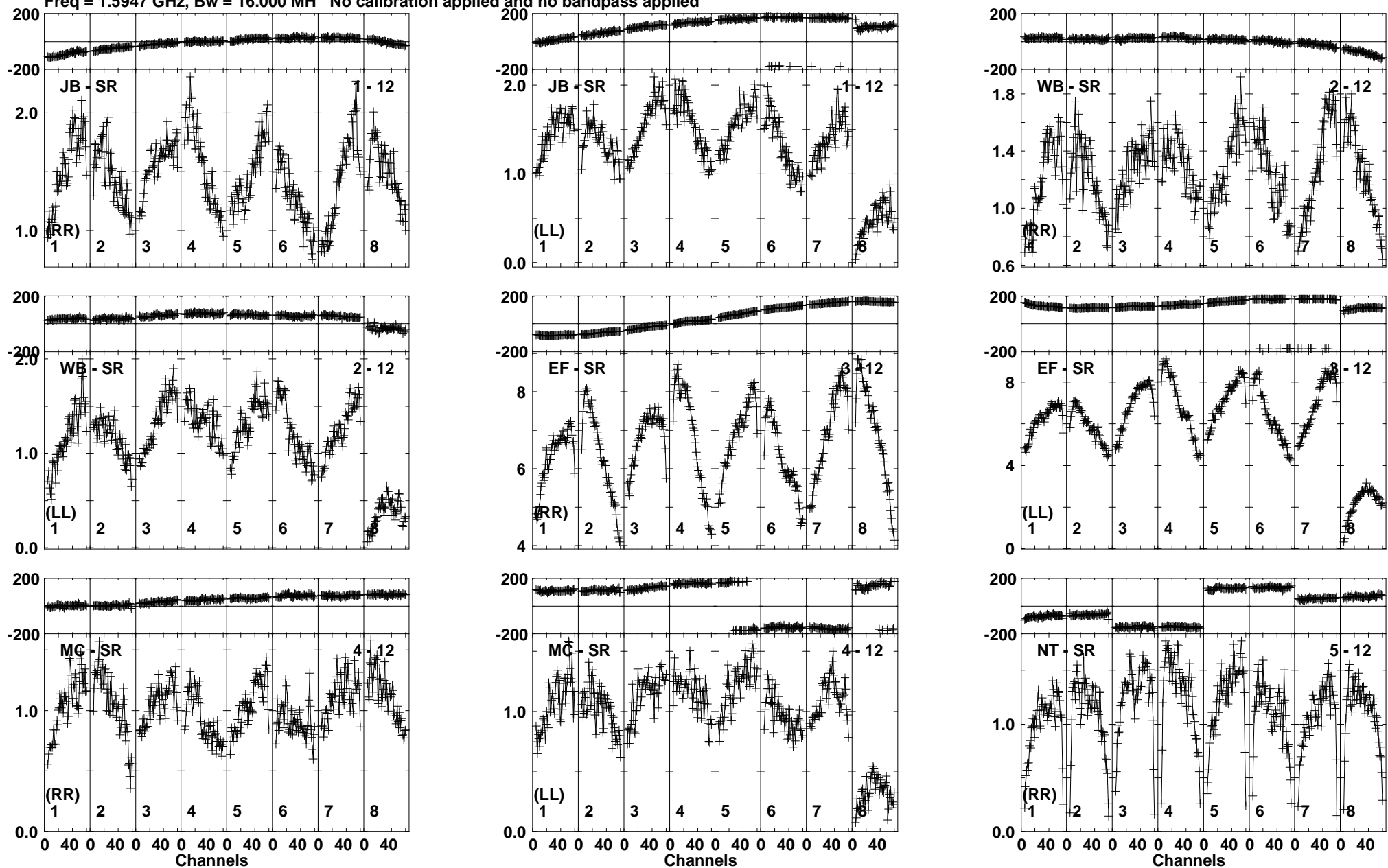
Lower frame: Milli Ampl Jy Top frame: Phas deg Vector averaged cross-power spectrum Baseline: JB (01) - SR (12) Timerange: 00/09:11:00 to 00/09:13:00
