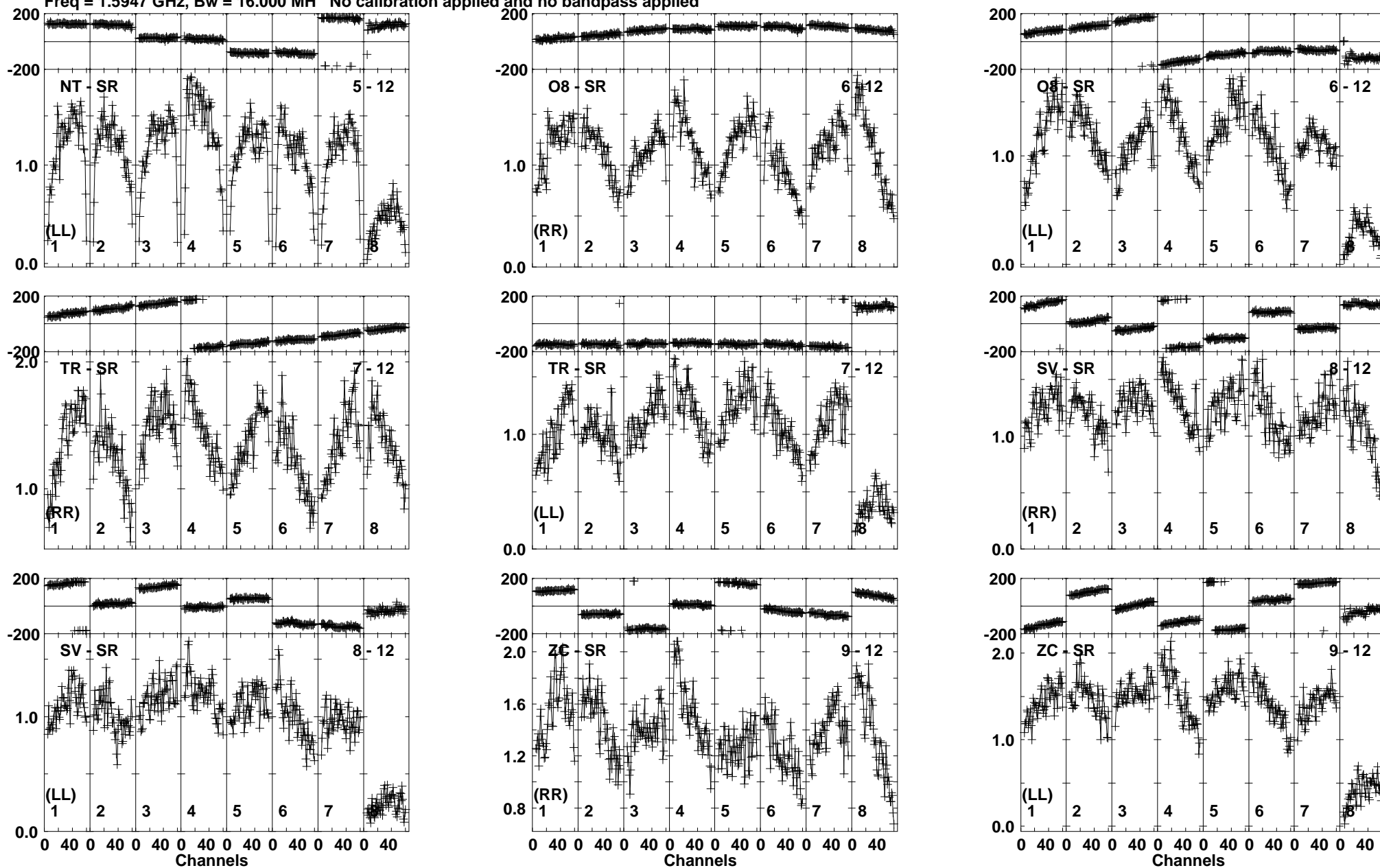
Lower frame: Milli Ampl Jy Top frame: Phas deg Vector averaged cross-power spectrum Baseline: NT (05) - SR (12) Timerange: 00/08:59:00 to 00/09:01:00
