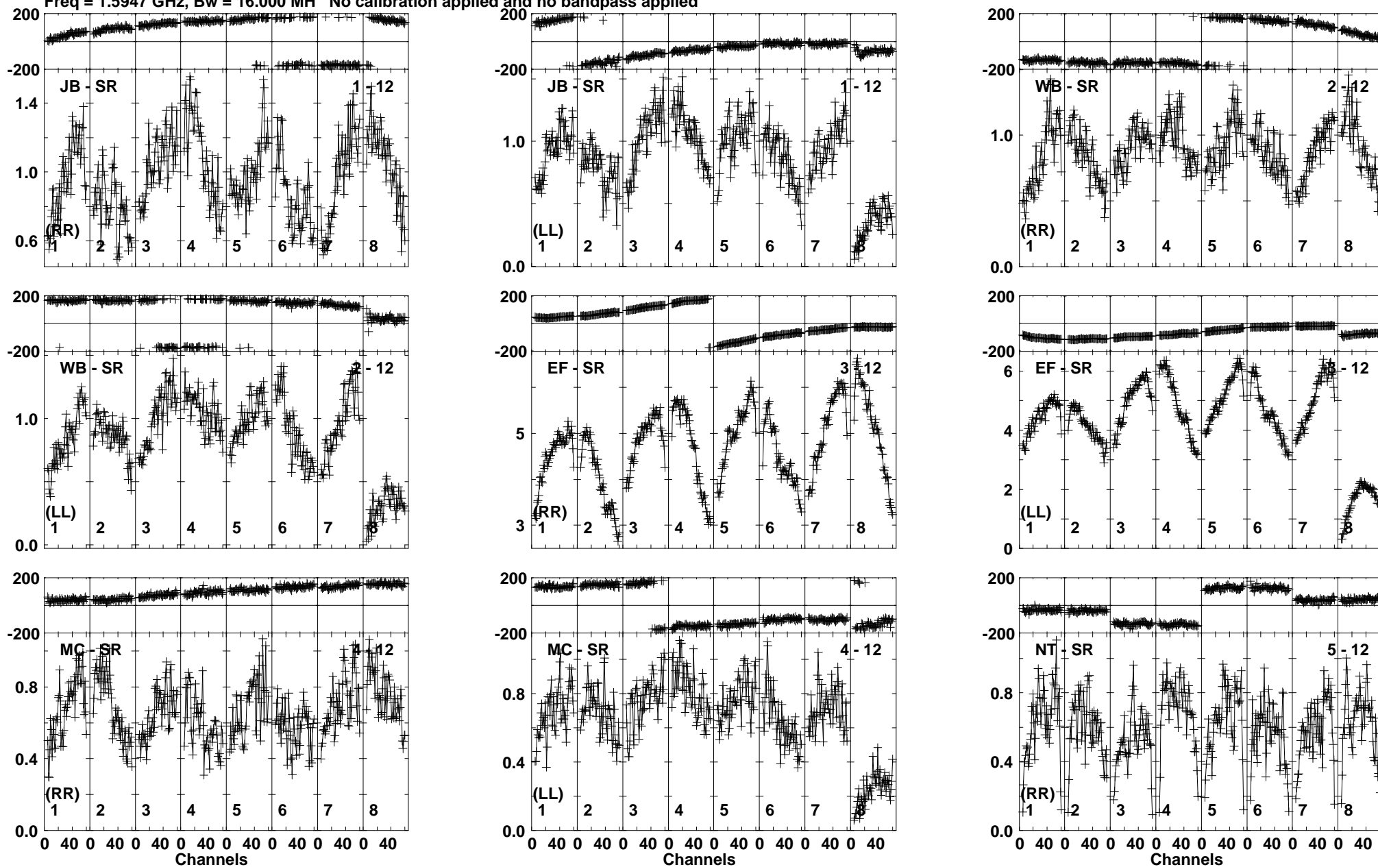
Lower frame: Milli Ampl Jy Top frame: Phas deg Vector averaged cross-power spectrum Baseline: JB (01) - SR (12) Timerange: 00/11:13:00 to 00/11:14:59
