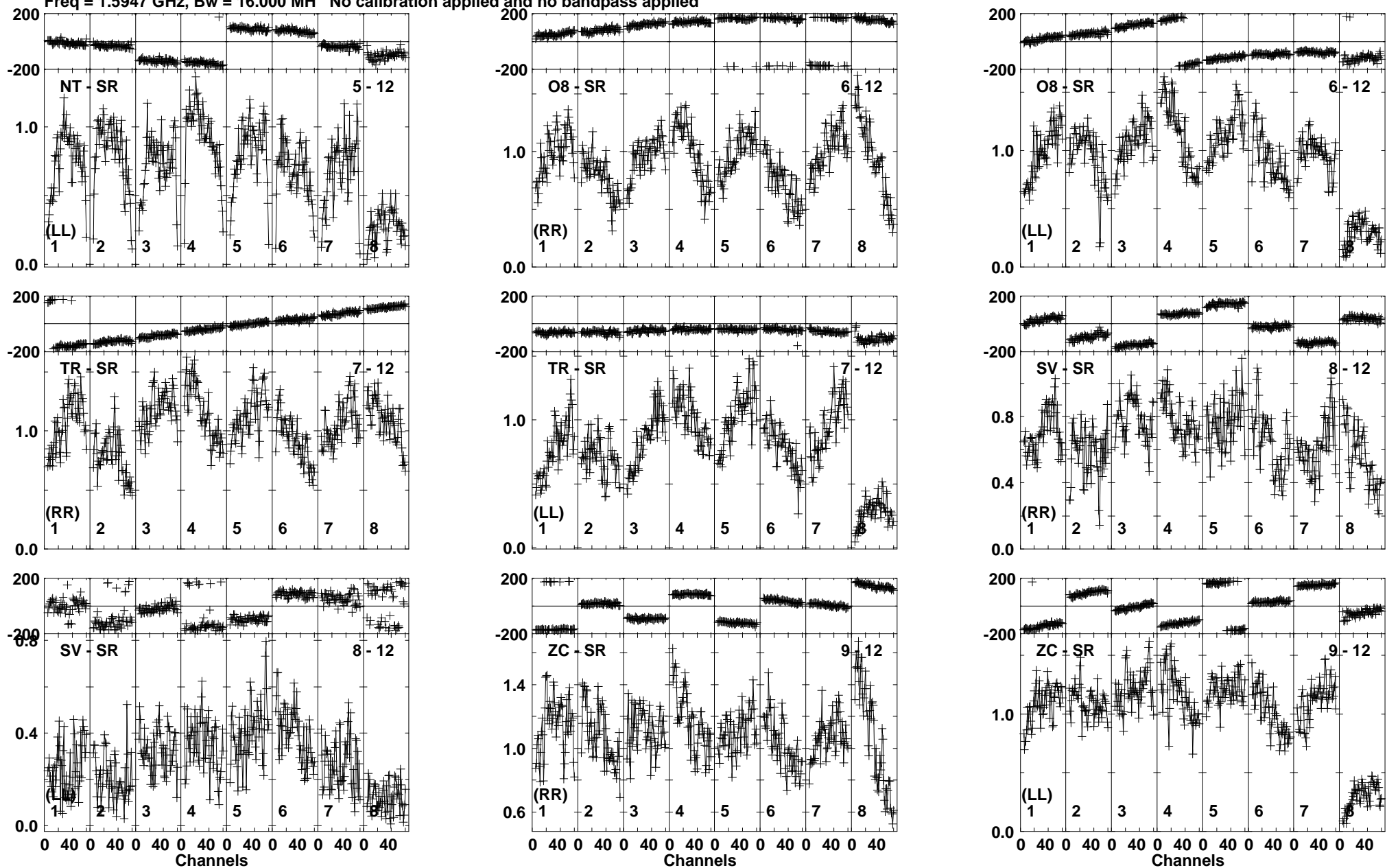
Lower frame: Milli Ampl Jy Top frame: Phas deg Vector averaged cross-power spectrum Baseline: NT (05) - SR (12) Timerange: 00/12:21:30 to 00/12:22:59
