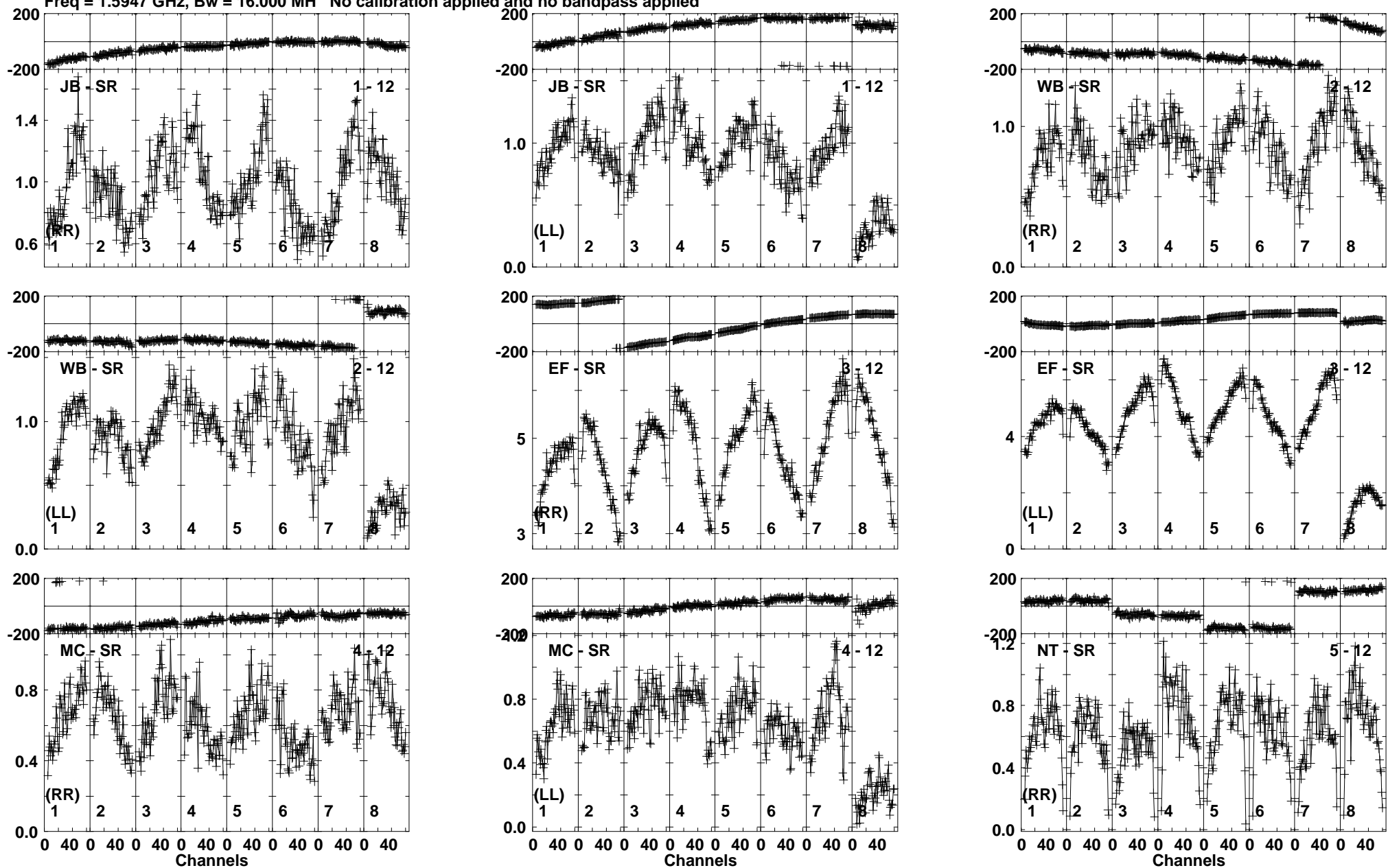
Lower frame: Milli Ampl Jy Top frame: Phas deg Vector averaged cross-power spectrum Baseline: JB (01) - SR (12) Timerange: 00/11:25:00 to 00/11:27:00
