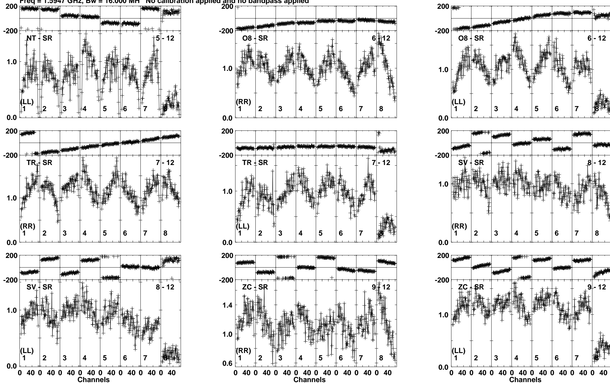
Lower frame: Milli Ampl Jy Top frame: Phas deg Vector averaged cross-power spectrum Baseline: NT (05) - SR (12) Timerange: 00/09:57:31 to 00/09:58:59
