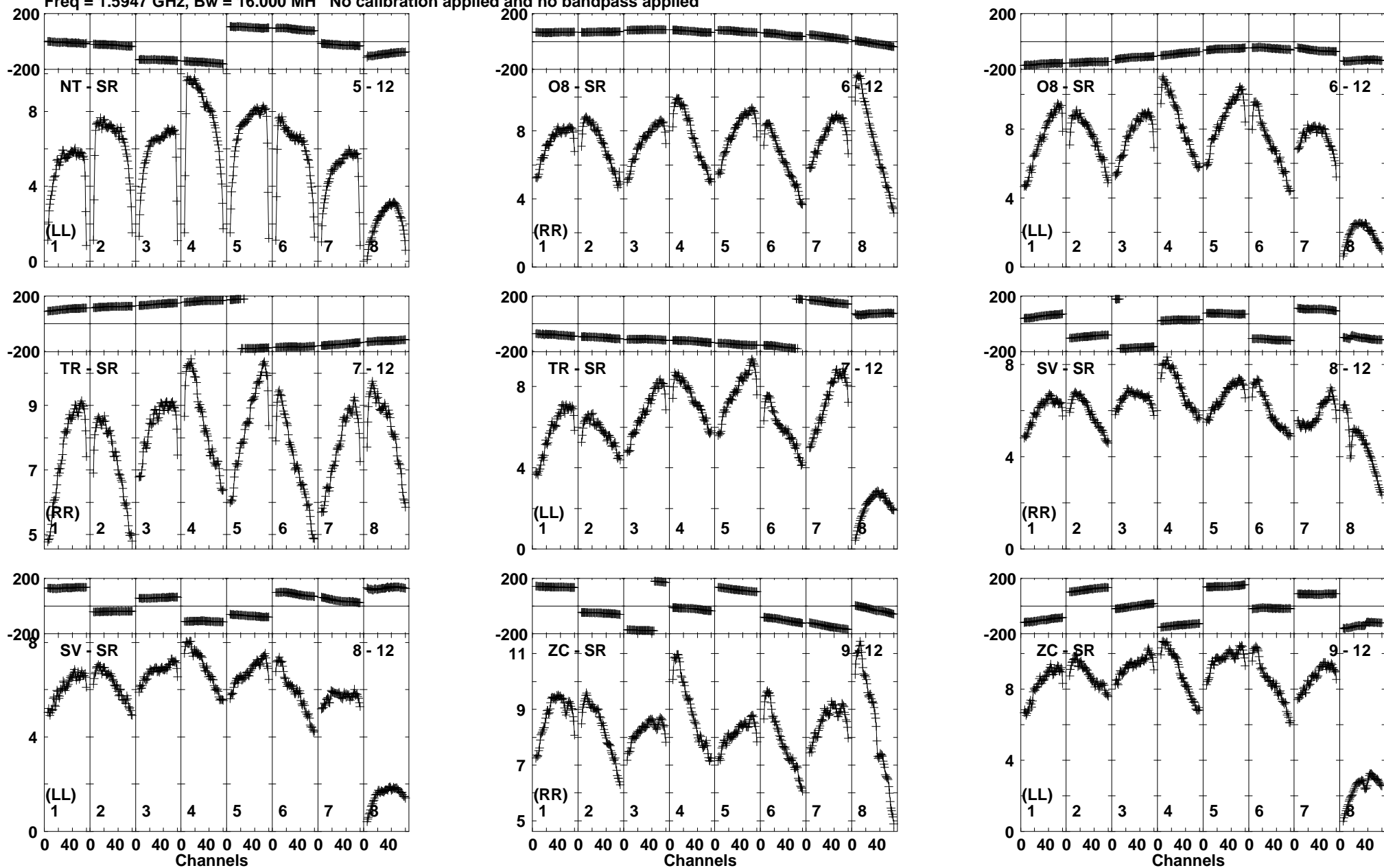
Lower frame: Milli Ampl Jy Top frame: Phas deg Vector averaged cross-power spectrum Baseline: NT (05) - SR (12) Timerange: 00/07:29:32 to 00/07:34:59
