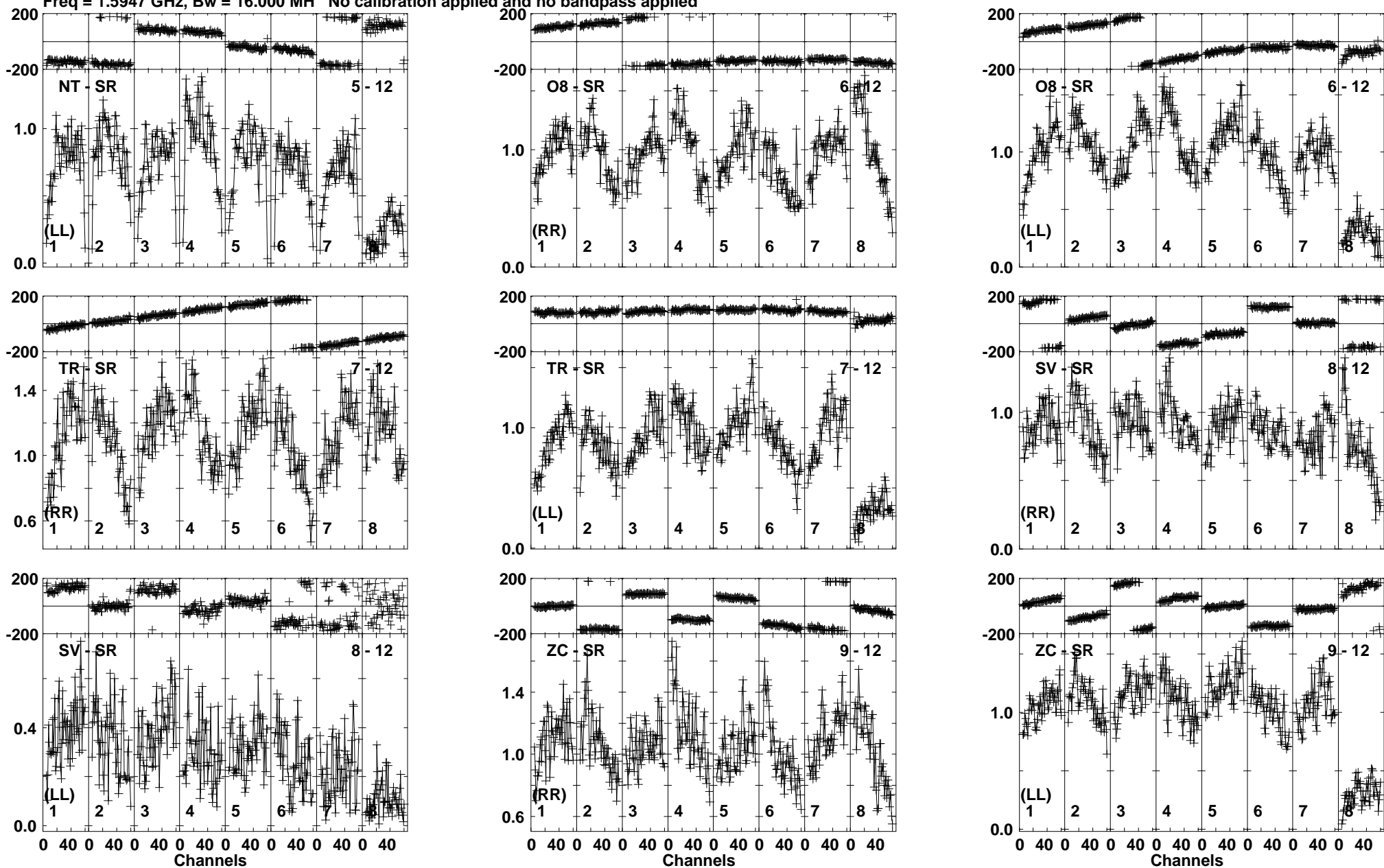
Lower frame: Milli Ampl Jy Top frame: Phas deg Vector averaged cross-power spectrum Baseline: NT (05) - SR (12) Timerange: 00/11:21:30 to 00/11:22:59
