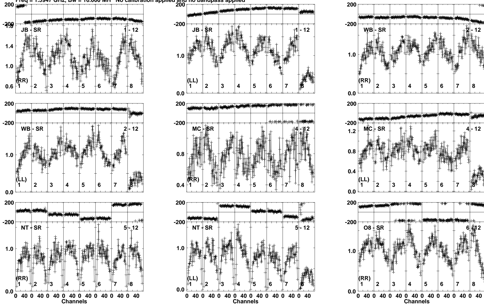
Lower frame: Milli Ampl Jy Top frame: Phas deg Vector averaged cross-power spectrum Baseline: JB (01) - SR (12) Timerange: 00/08:09:30 to 00/08:10:59
