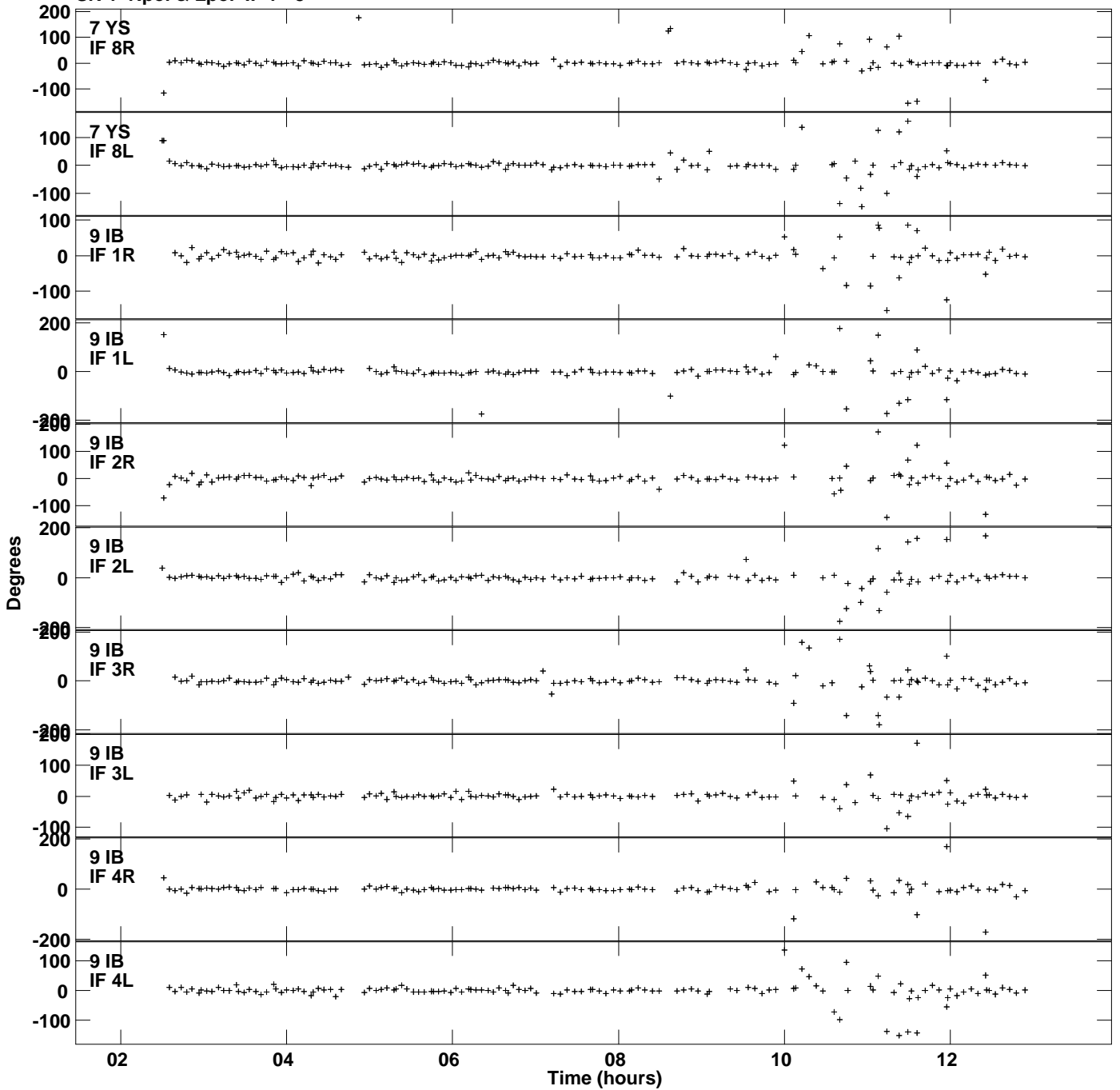
Plot file version 12 created 21-JUN-2018 17:37:49 Gain phs vs UTC time for J0450+4620.MULTI.1 SN 1 Rpol & Lpol IF 1 - 8
