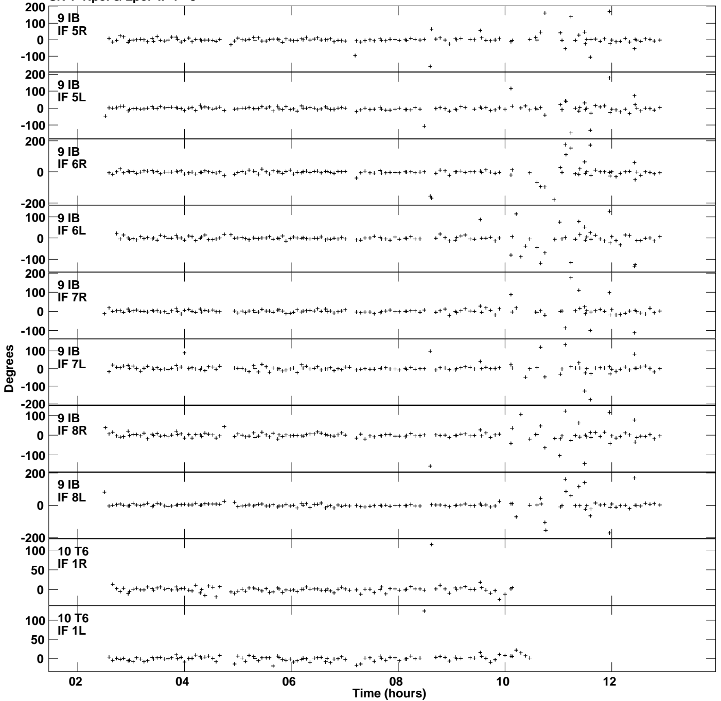
Plot file version 13 created 21-JUN-2018 17:37:49 Gain phs vs UTC time for J0450+4620.MULTI.1 SN 1 Rpol & Lpol IF 1 - 8
