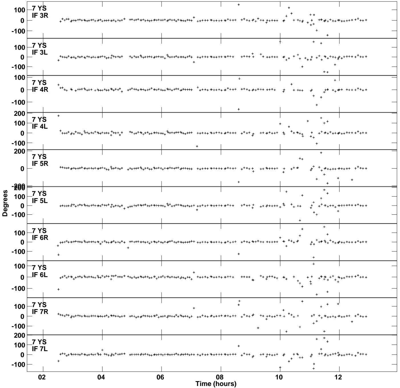
Plot file version 11 created 21-JUN-2018 17:37:49 Gain phs vs UTC time for J0450+4620.MULTI.1 SN 1 Rpol & Lpol IF 1 - 8
