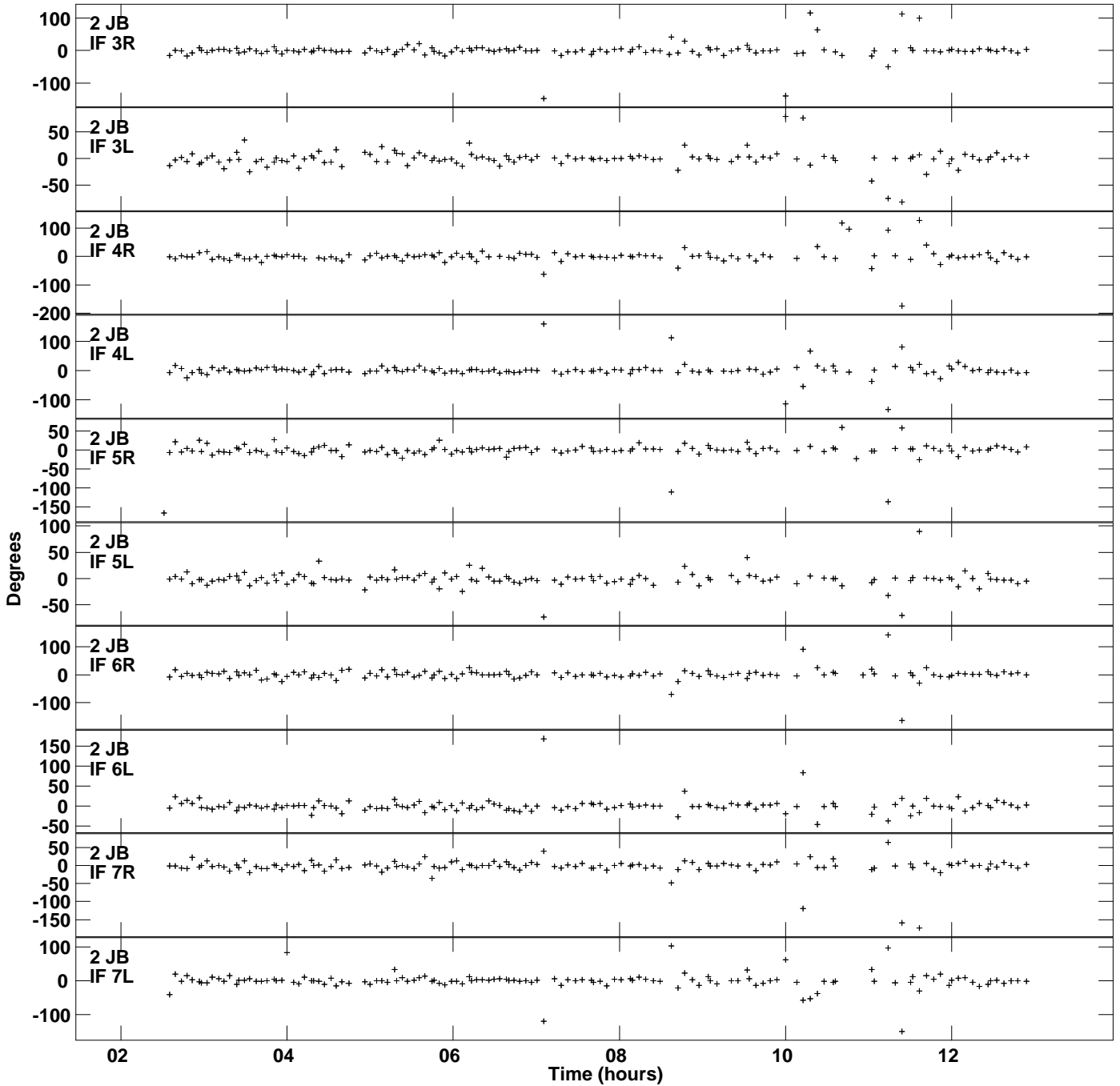
Plot file version 3 created 21-JUN-2018 17:37:49 Gain phs vs UTC time for J0450+4620.MULTI.1 SN 1 Rpol & Lpol IF 1 - 8
