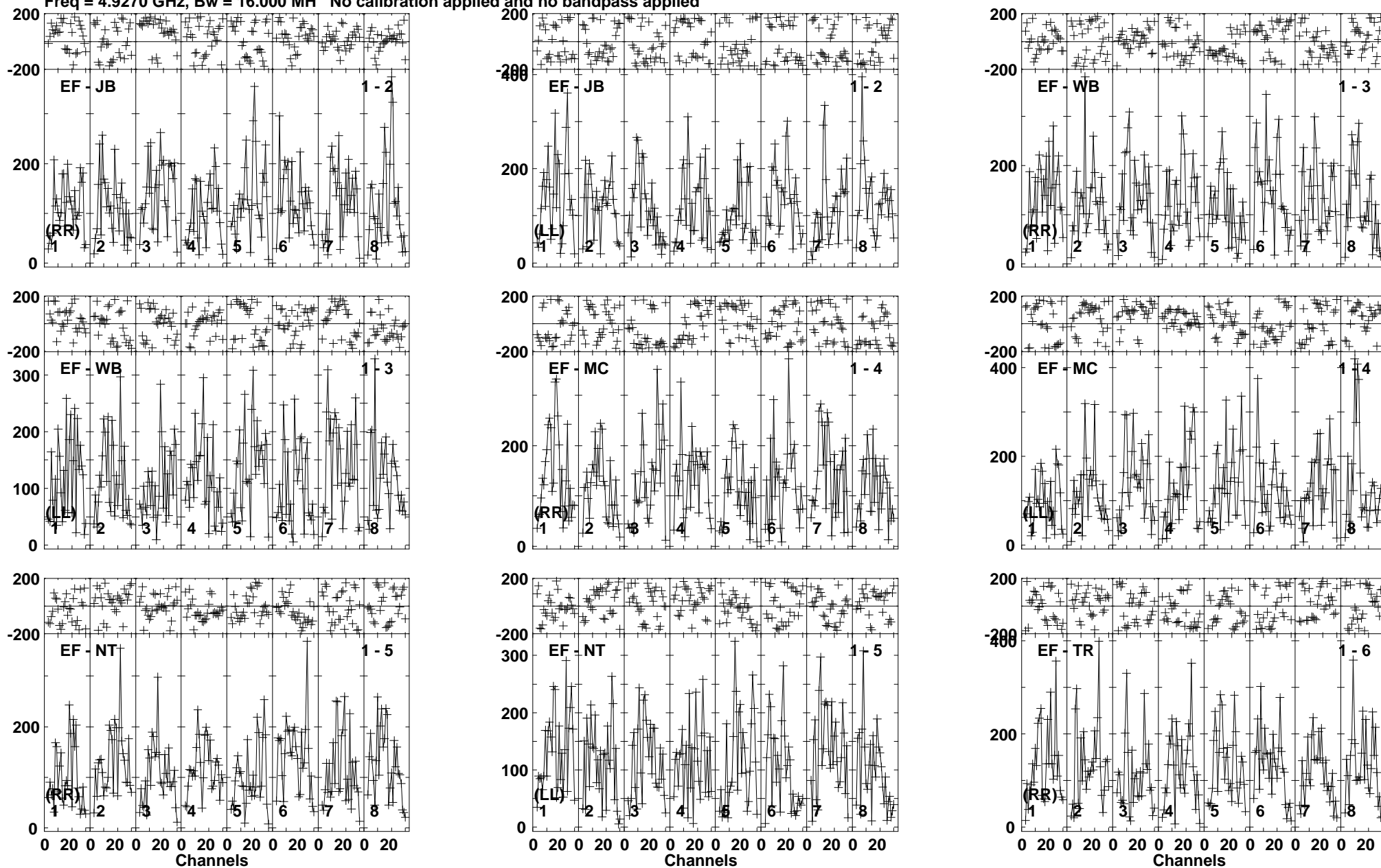
Lower frame: Micro Ampl Jy Top frame: Phas deg Vector averaged cross-power spectrum Baseline: EF (01) - JB (02) Timerange: 00/10:36:30 to 00/10:39:59
