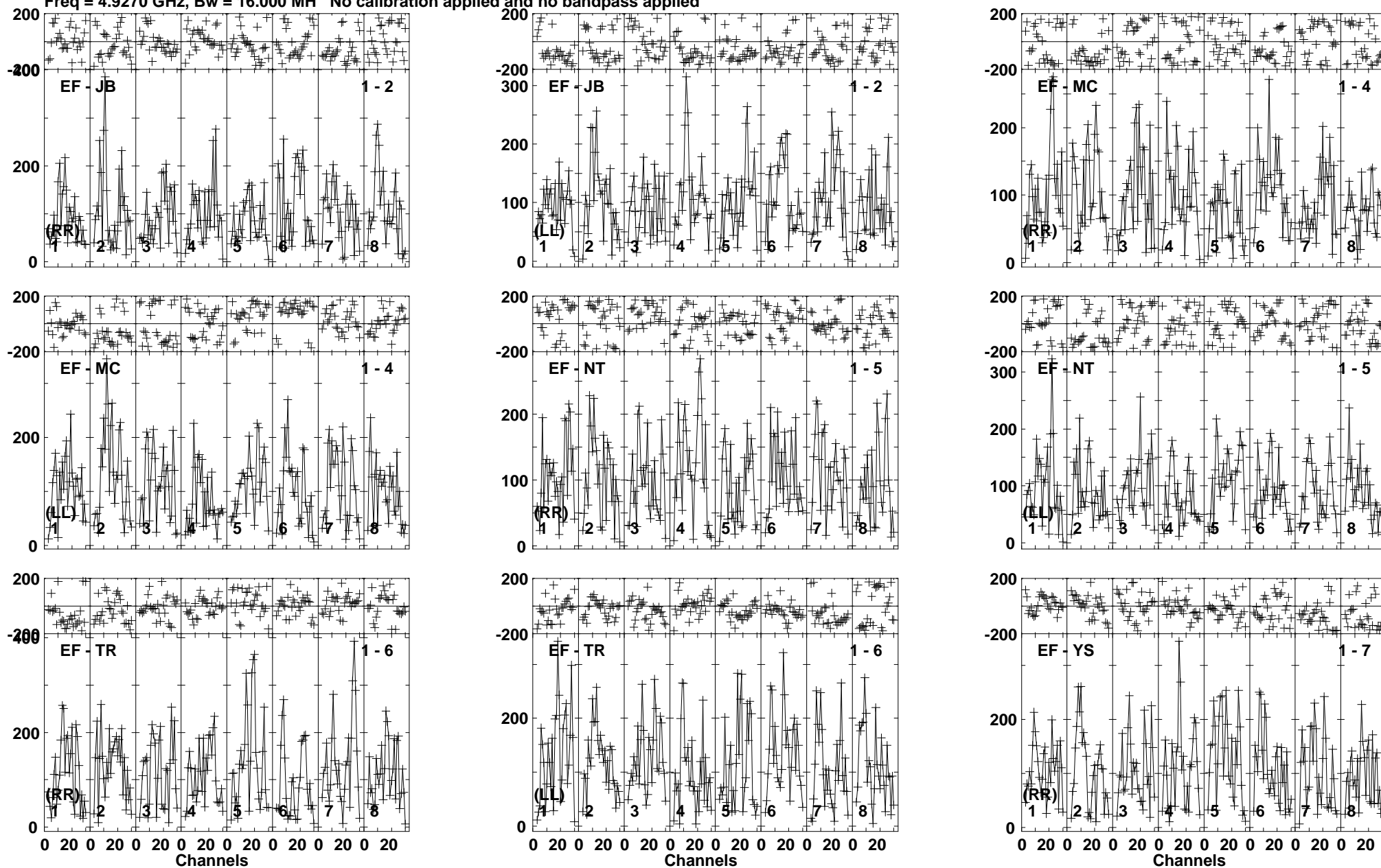
Lower frame: Micro Ampl Jy Top frame: Phas deg Vector averaged cross-power spectrum Baseline: EF (01) - JB (02) Timerange: 00/04:13:01 to 00/04:15:59
