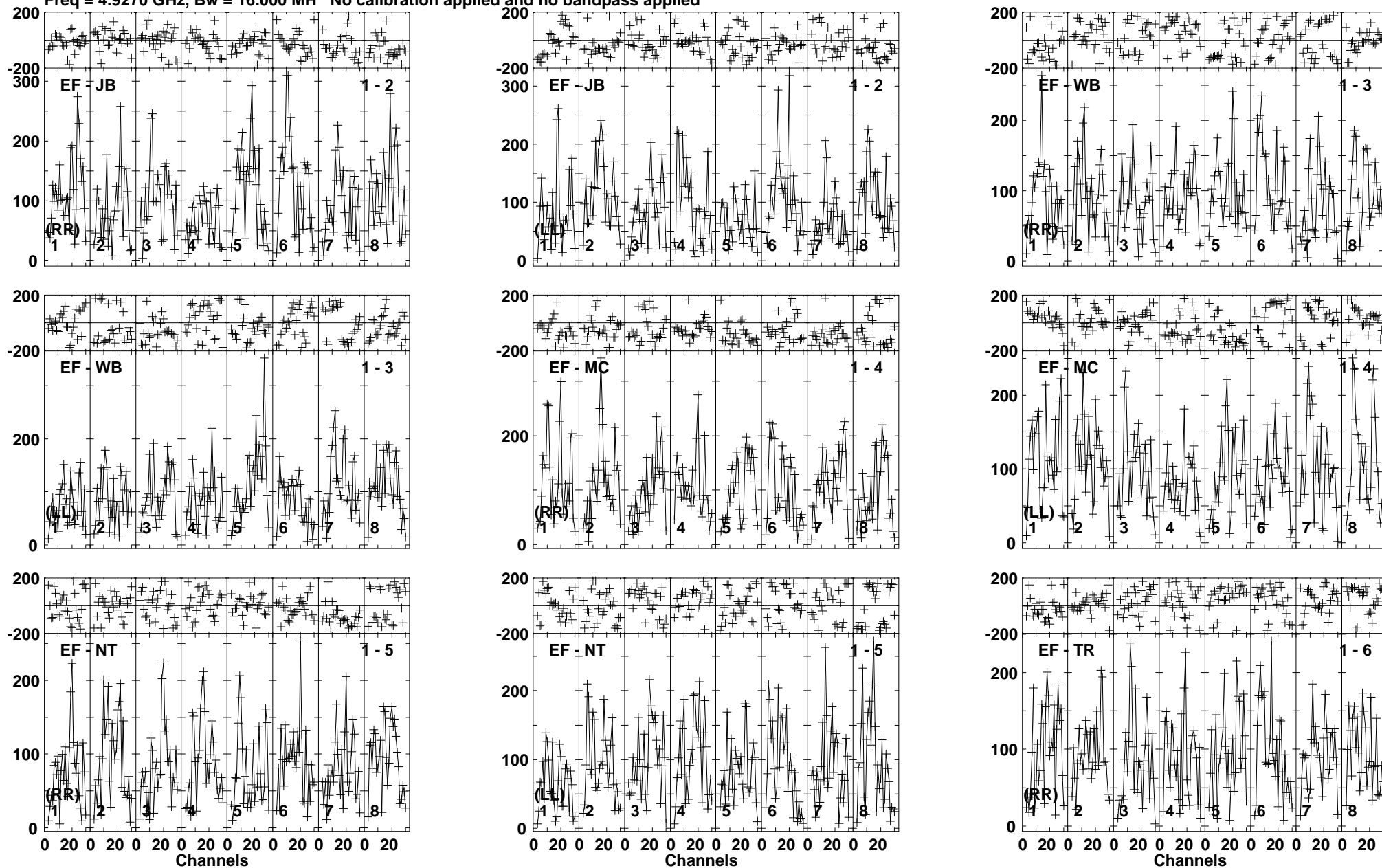
Lower frame: Micro Ampl Jy Top frame: Phas deg Vector averaged cross-power spectrum Baseline: EF (01) - JB (02) Timerange: 00/07:23:30 to 00/07:27:09
