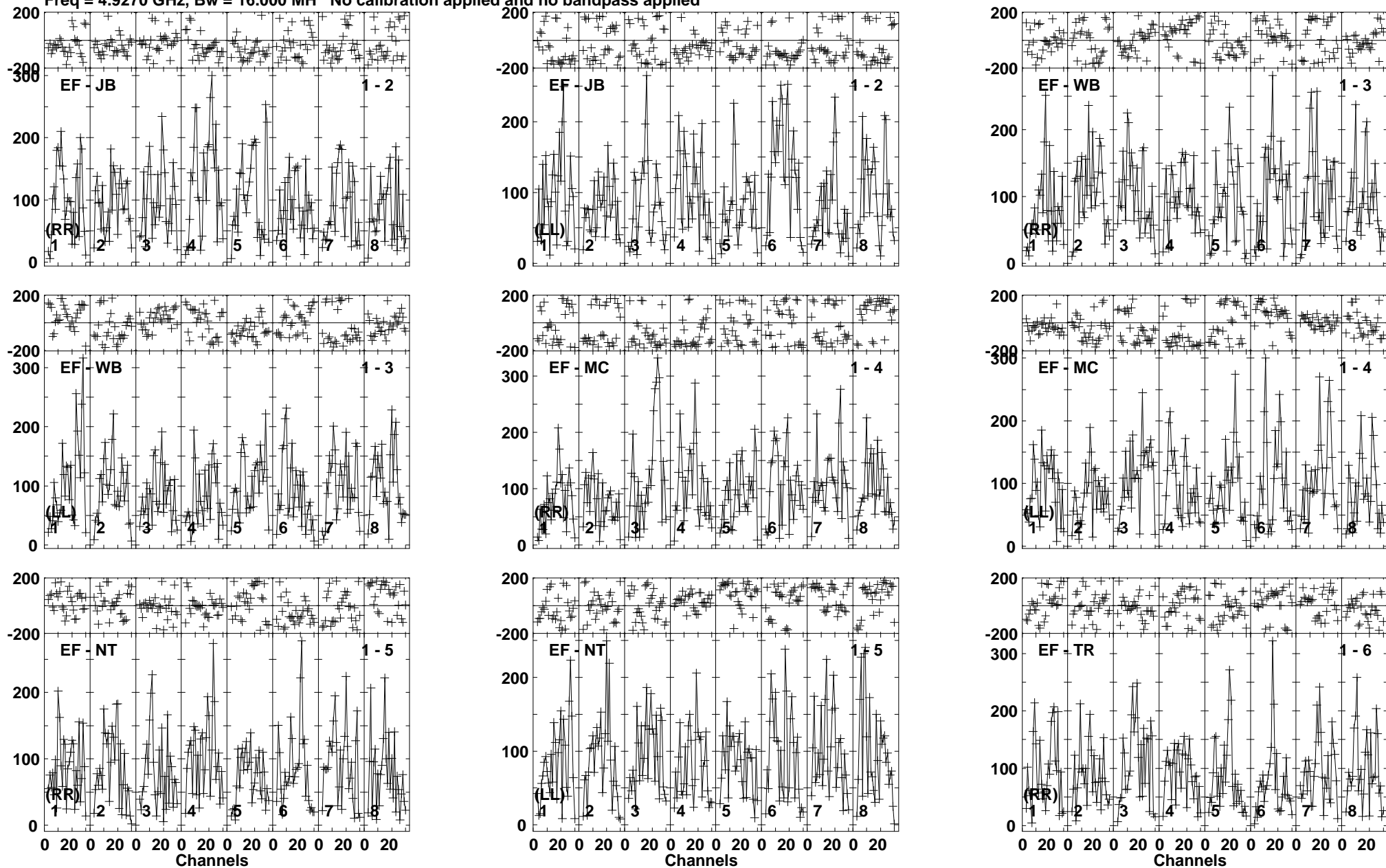
Lower frame: Micro Ampl Jy Top frame: Phas deg Vector averaged cross-power spectrum Baseline: EF (01) - JB (02) Timerange: 00/07:33:41 to 00/07:37:20
