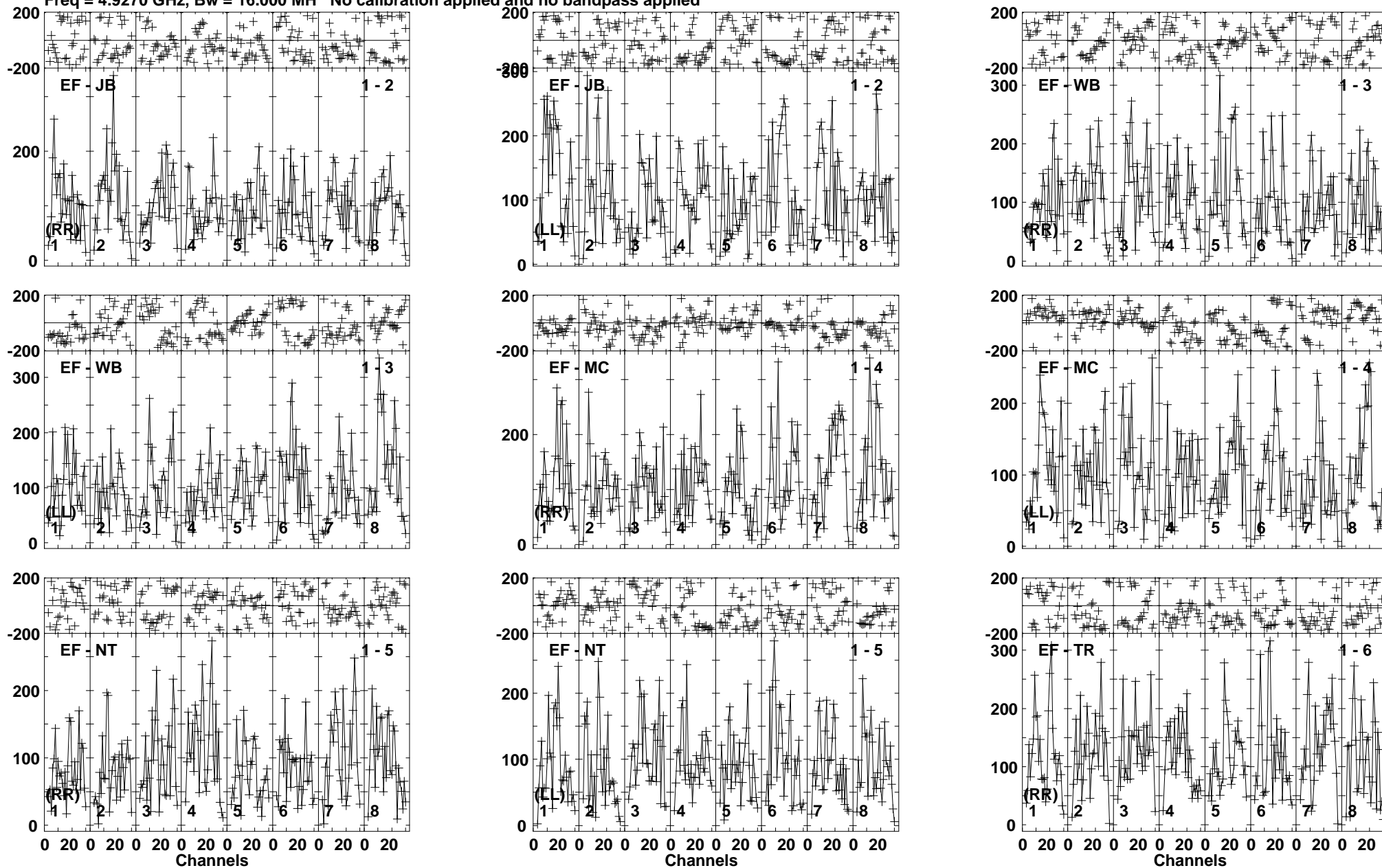
Lower frame: Micro Ampl Jy Top frame: Phas deg Vector averaged cross-power spectrum Baseline: EF (01) - JB (02) Timerange: 00/04:27:31 to 00/04:30:29
