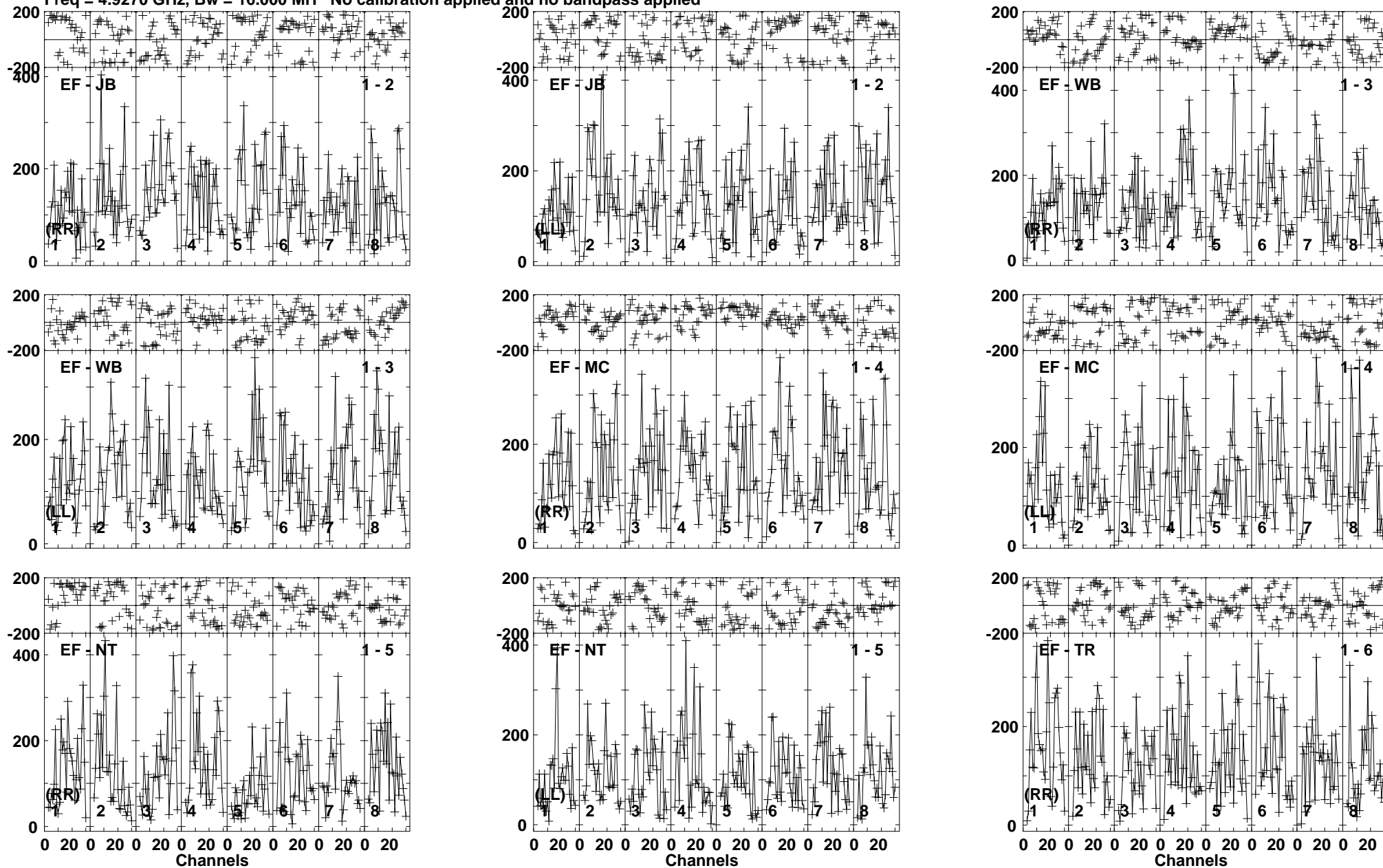
Lower frame: Micro Ampl Jy Top frame: Phas deg Vector averaged cross-power spectrum Baseline: EF (01) - JB (02) Timerange: 00/10:18:30 to 00/10:21:59
