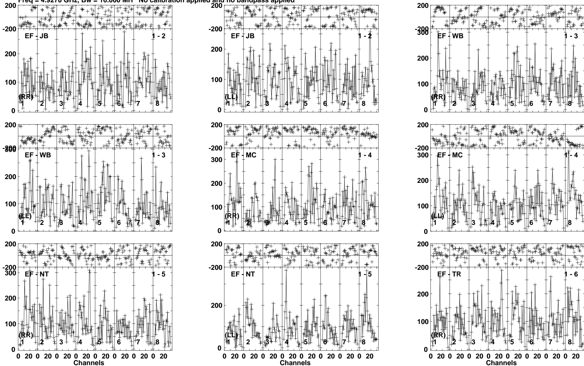
Lower frame: Micro Ampl Jy Top frame: Phas deg Vector averaged cross-power spectrum Baseline: EF (01) - JB (02) Timerange: 00/08:43:00 to 00/08:46:40
