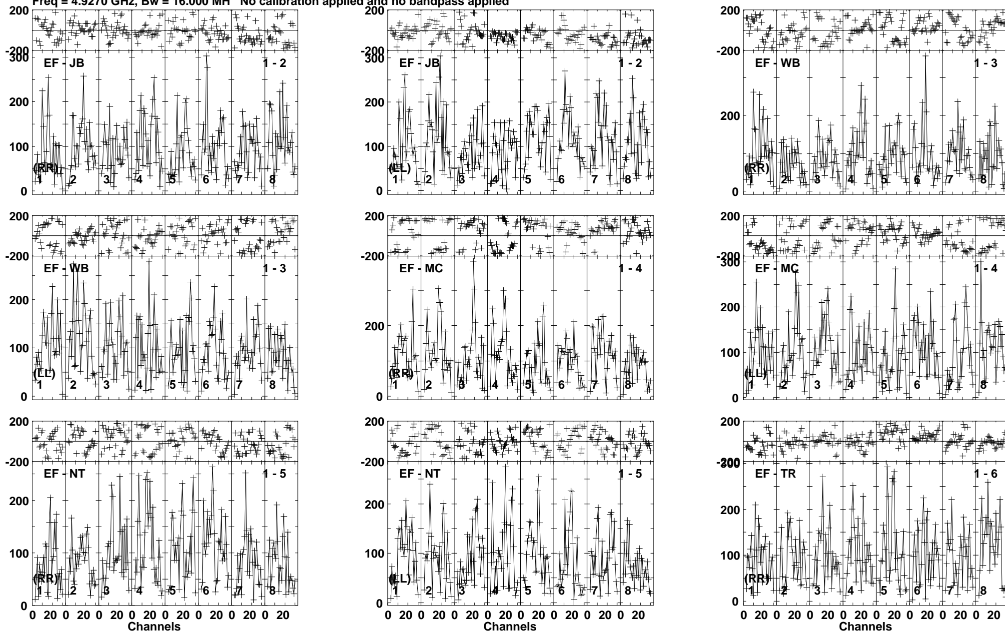
Lower frame: Micro Ampl Jy Top frame: Phas deg Vector averaged cross-power spectrum Baseline: EF (01) - JB (02) Timerange: 00/12:43:40 to 00/12:47:09
