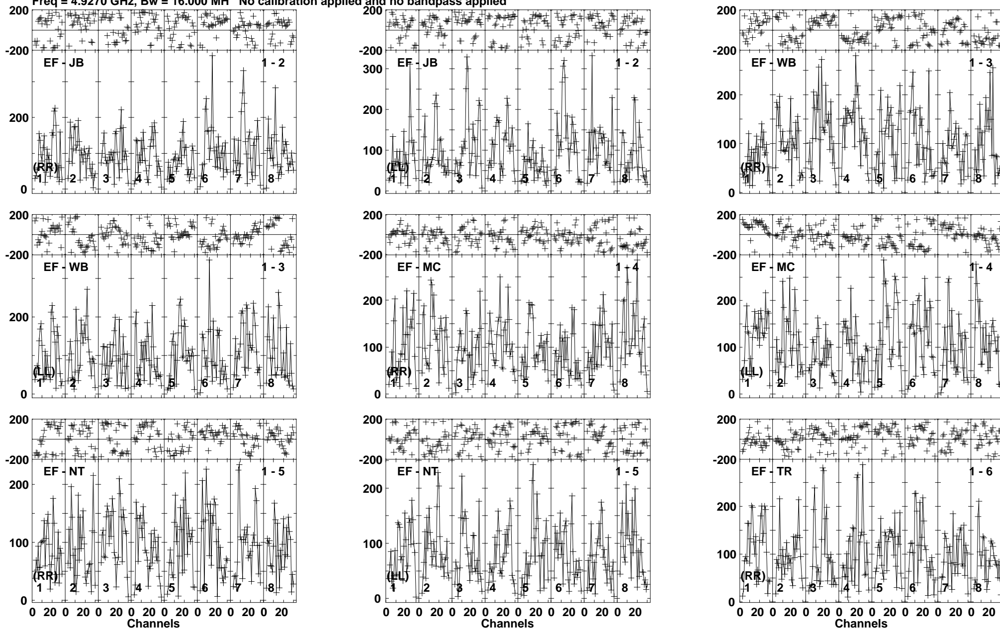
Lower frame: Micro Ampl Jy Top frame: Phas deg Vector averaged cross-power spectrum Baseline: EF (01) - JB (02) Timerange: 00/12:28:30 to 00/12:32:00
