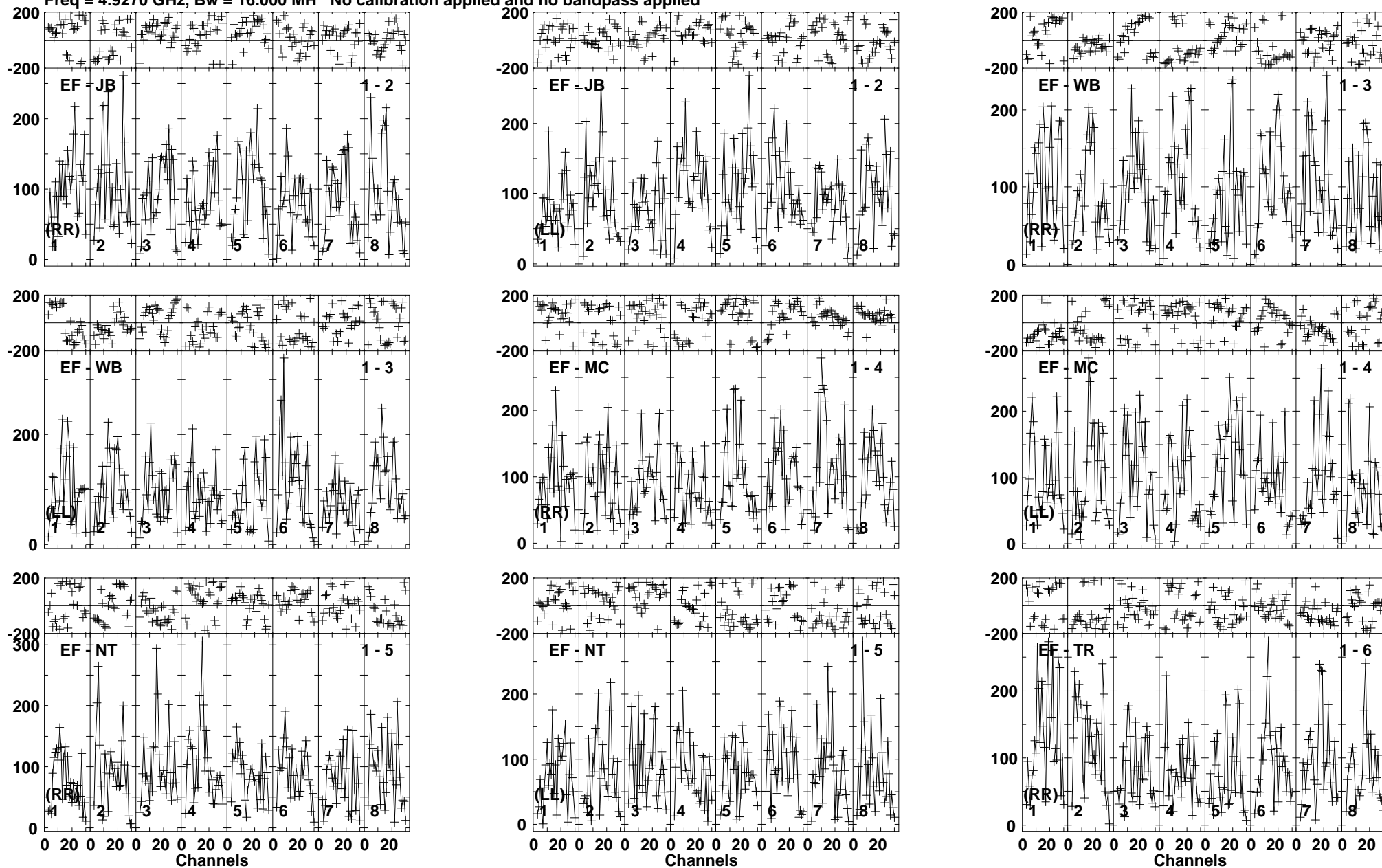
Lower frame: Micro Ampl Jy Top frame: Phas deg Vector averaged cross-power spectrum Baseline: EF (01) - JB (02) Timerange: 00/08:09:51 to 00/08:13:30
