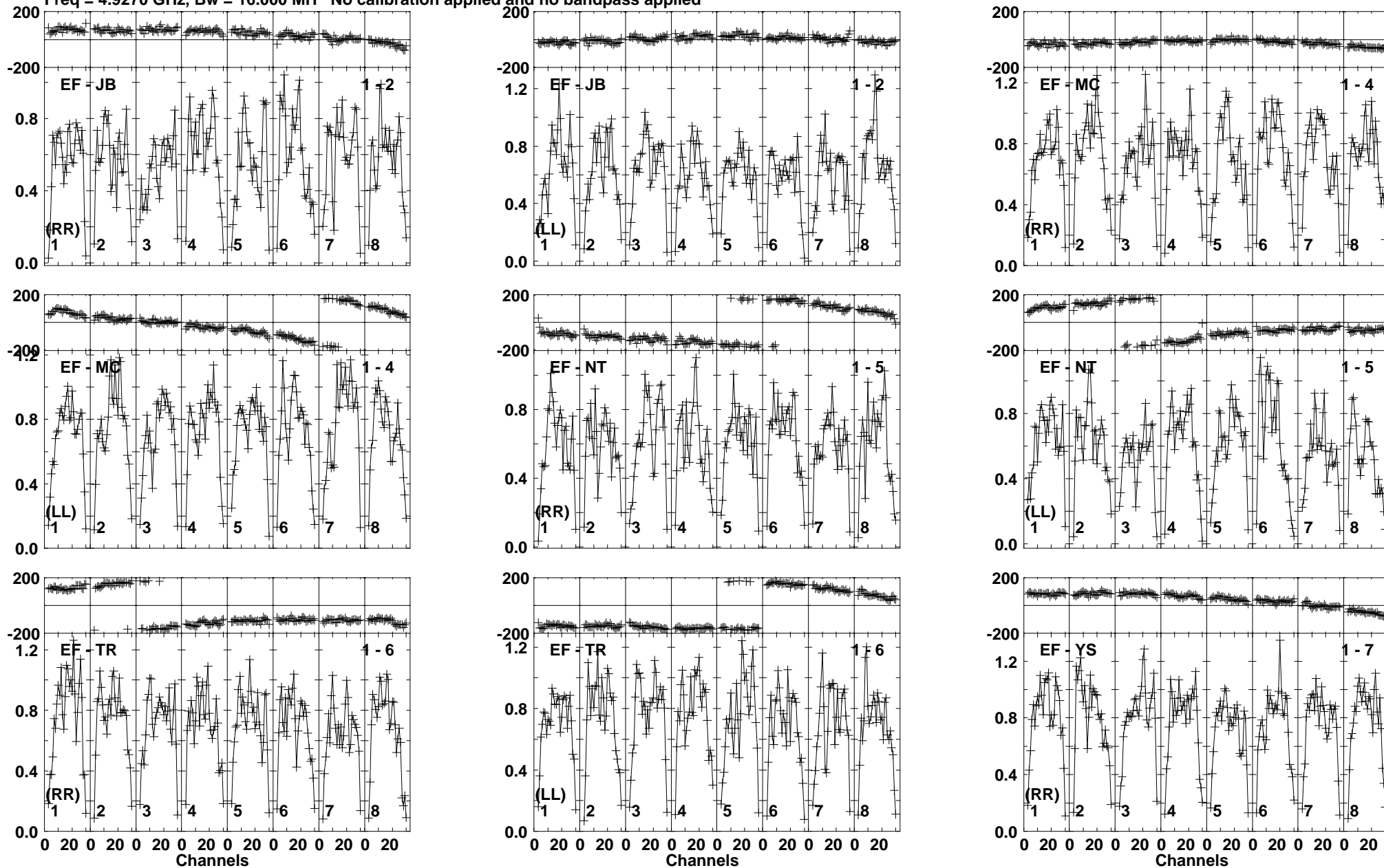
Lower frame: Milli Ampl Jy Top frame: Phas deg Vector averaged cross-power spectrum Baseline: EF (01) - JB (02) Timerange: 00/03:51:41 to 00/03:52:30
