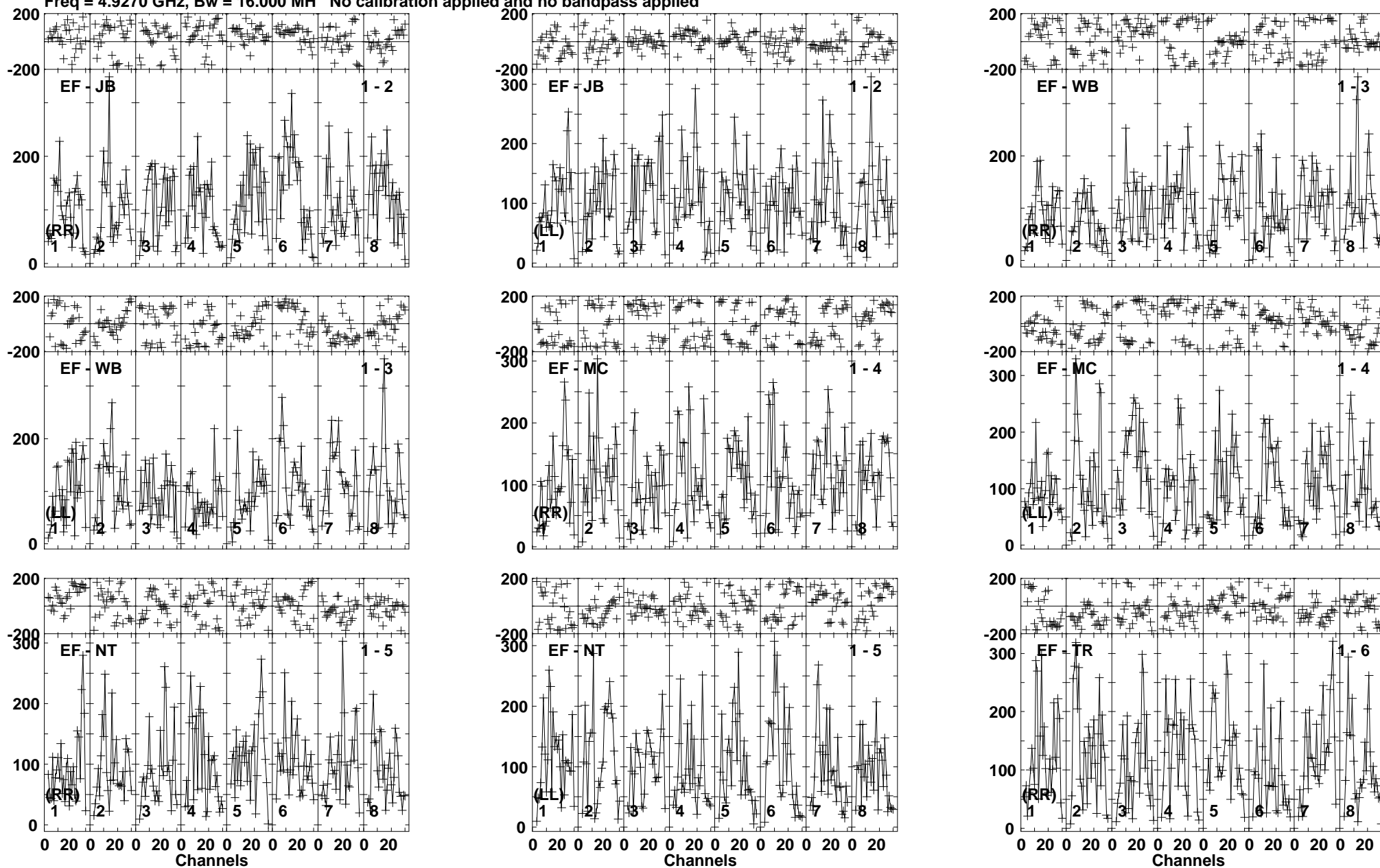
Lower frame: Micro Ampl Jy Top frame: Phas deg Vector averaged cross-power spectrum Baseline: EF (01) - JB (02) Timerange: 00/05:40:01 to 00/05:43:00
