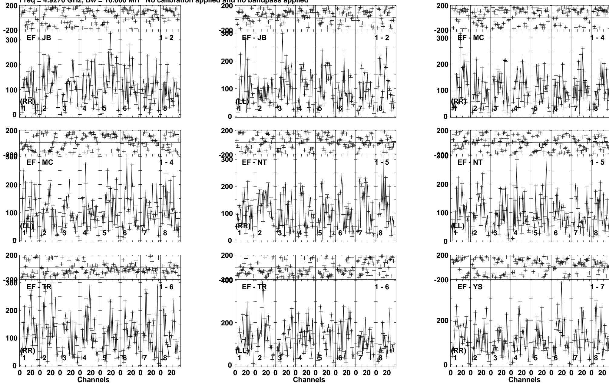
Lower frame: Micro Ampl Jy Top frame: Phas deg Vector averaged cross-power spectrum Baseline: EF (01) - JB (02) Timerange: 00/03:15:01 to 00/03:17:59
