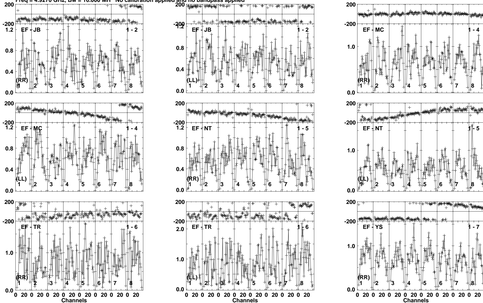
Lower frame: Milli Ampl Jy Top frame: Phas deg Vector averaged cross-power spectrum Baseline: EF (01) - JB (02) Timerange: 00/03:18:00 to 00/03:19:00
