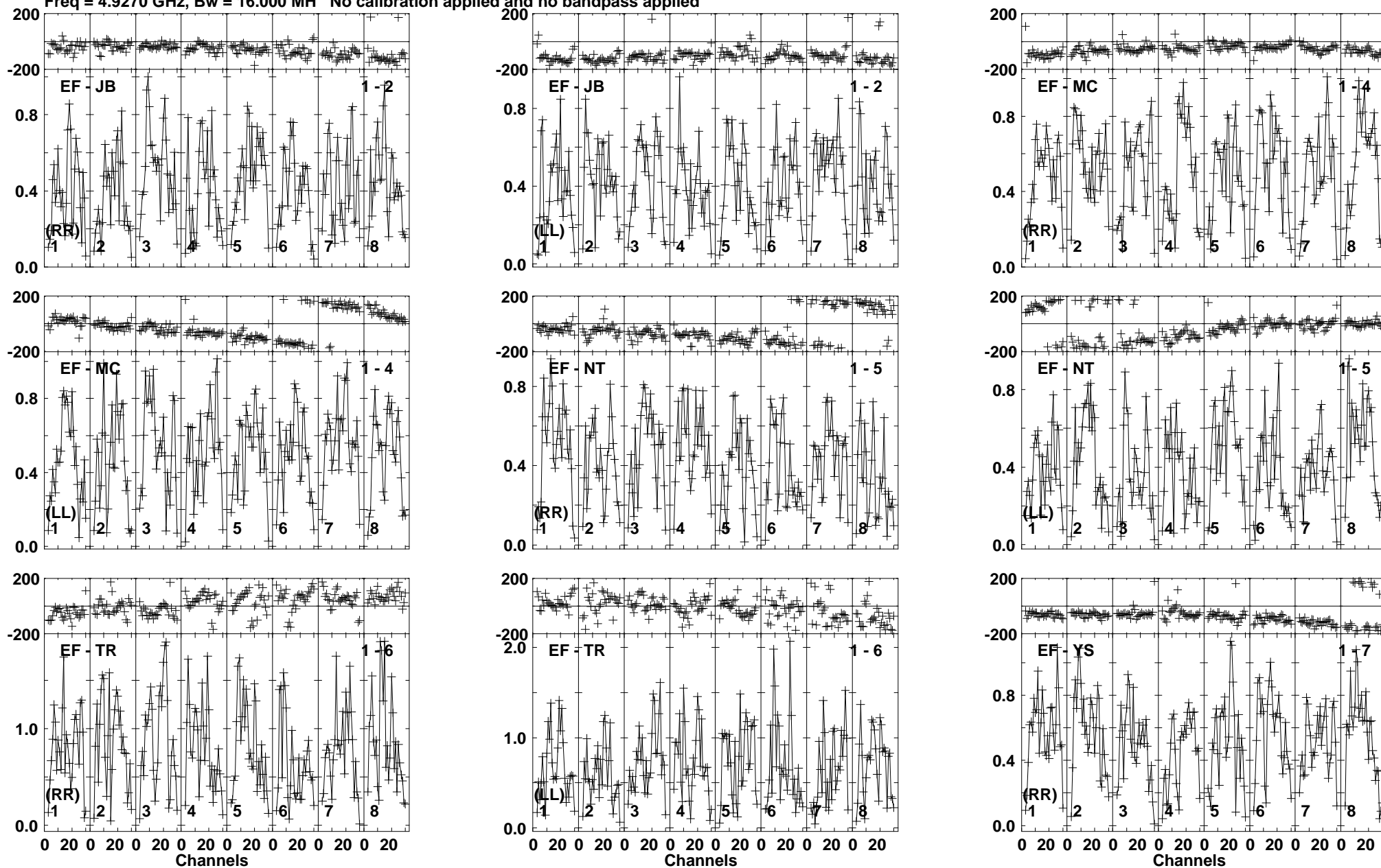
Lower frame: Milli Ampl Jy Top frame: Phas deg Vector averaged cross-power spectrum Baseline: EF (01) - JB (02) Timerange: 00/02:51:01 to 00/02:51:59
