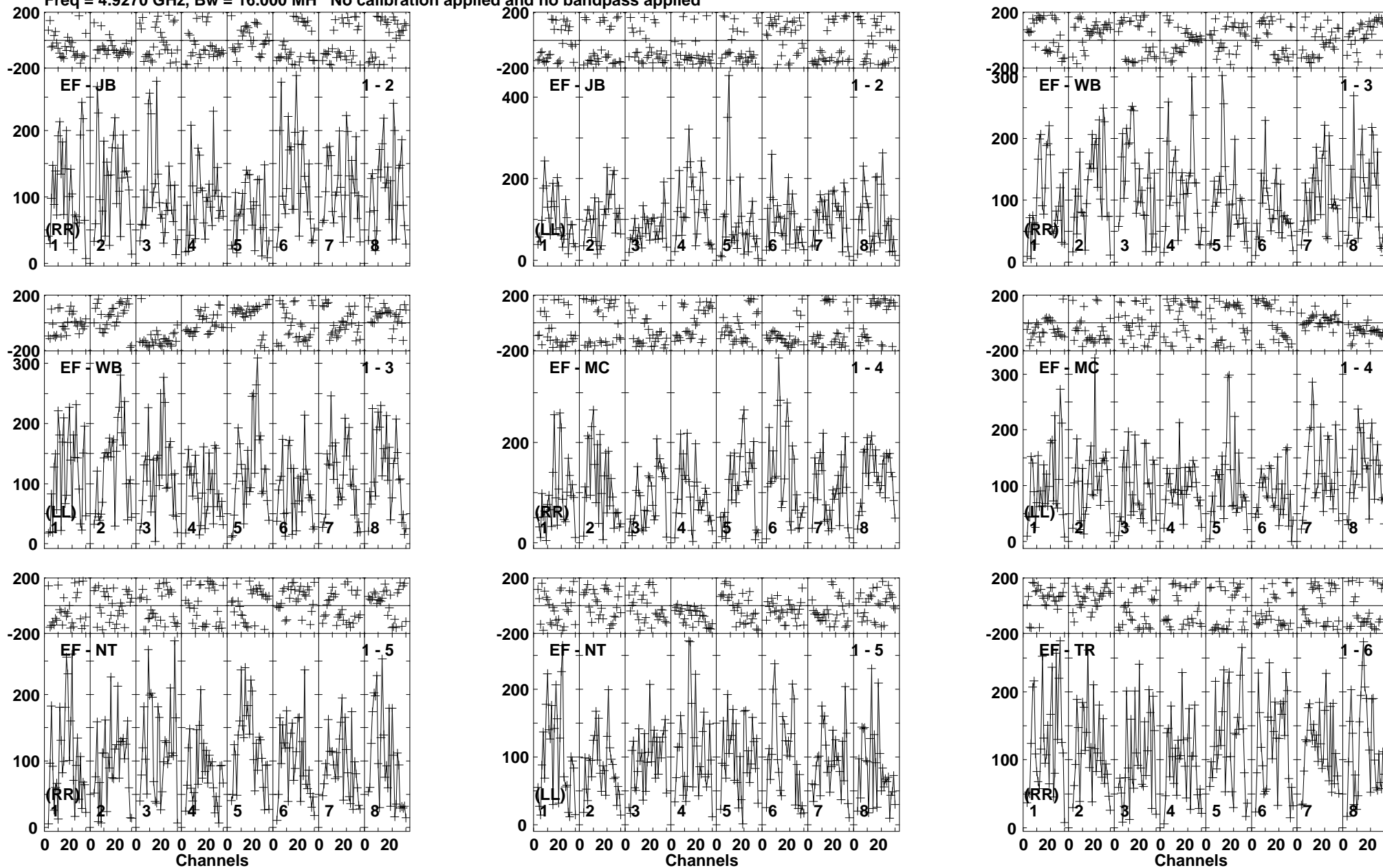
Lower frame: Micro Ampl Jy Top frame: Phas deg Vector averaged cross-power spectrum Baseline: EF (01) - JB (02) Timerange: 00/05:00:30 to 00/05:03:30
