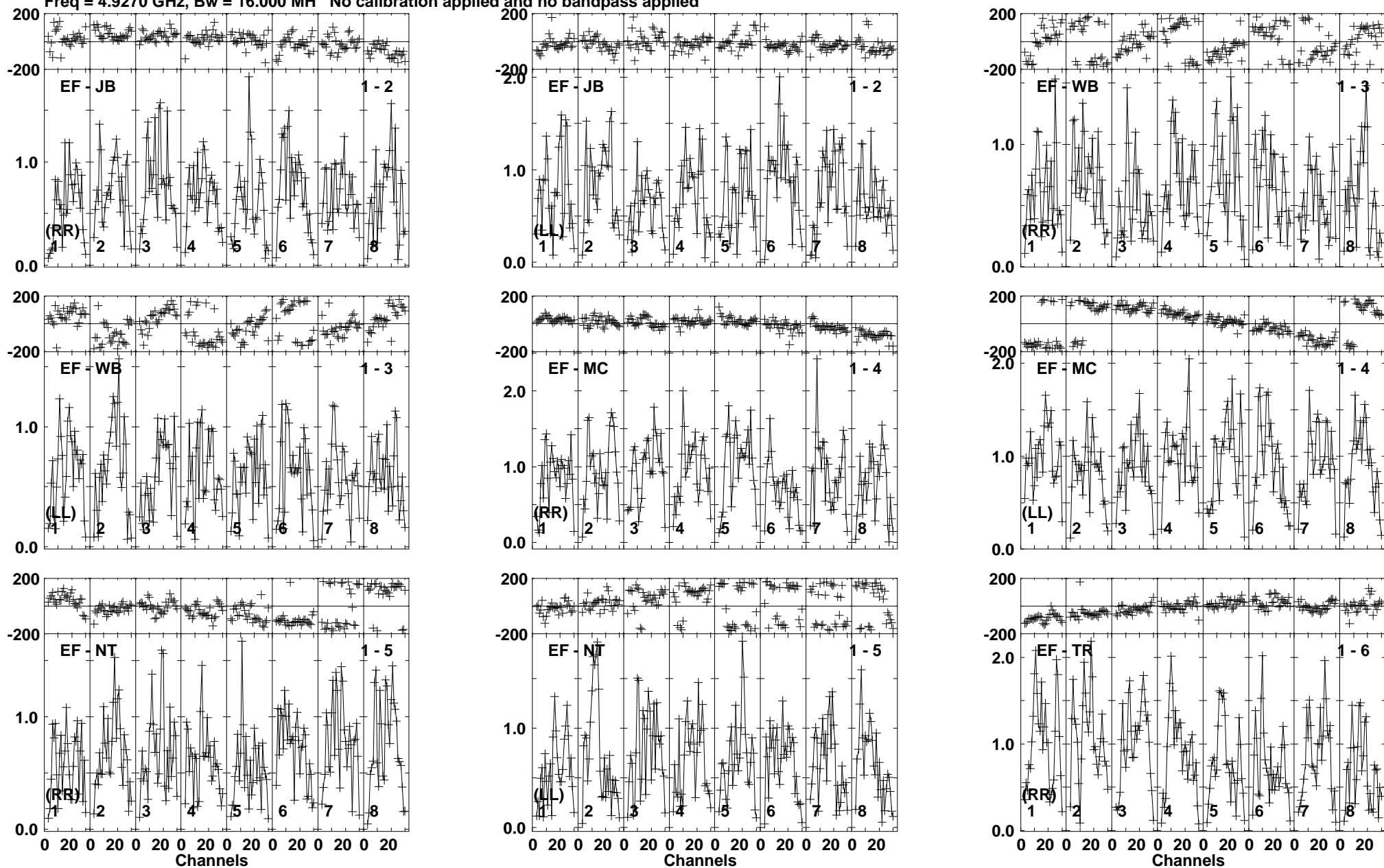
Lower frame: Milli Ampl Jy Top frame: Phas deg Vector averaged cross-power spectrum Baseline: EF (01) - JB (02) Timerange: 00/09:31:21 to 00/09:32:49
