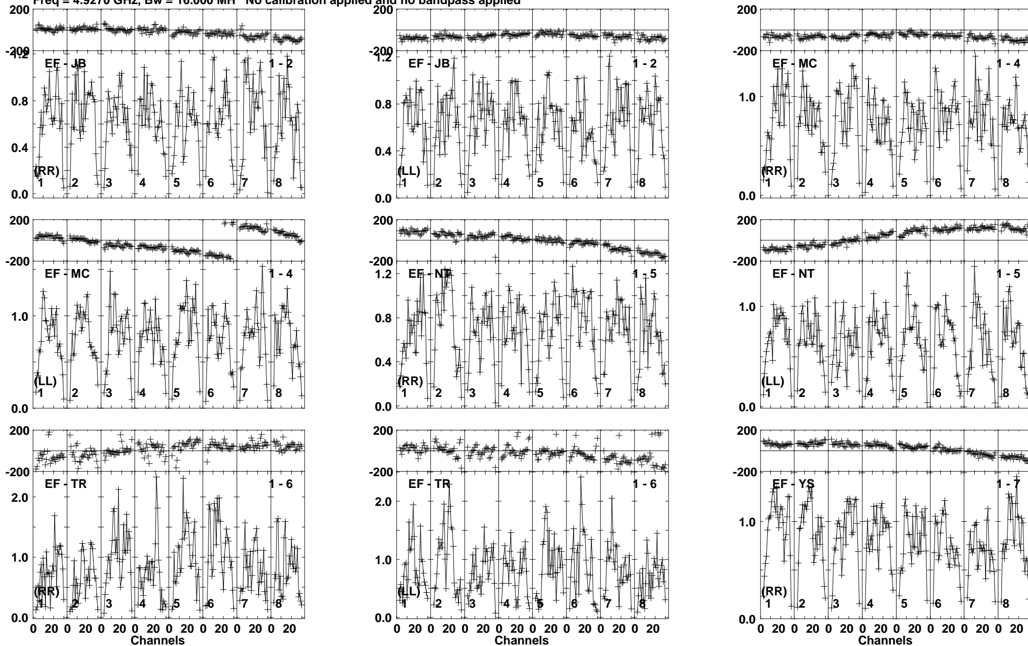
Lower frame: Milli Ampl Jy Top frame: Phas deg Vector averaged cross-power spectrum Baseline: EF (01) - JB (02) Timerange: 00/04:26:31 to 00/04:27:29
