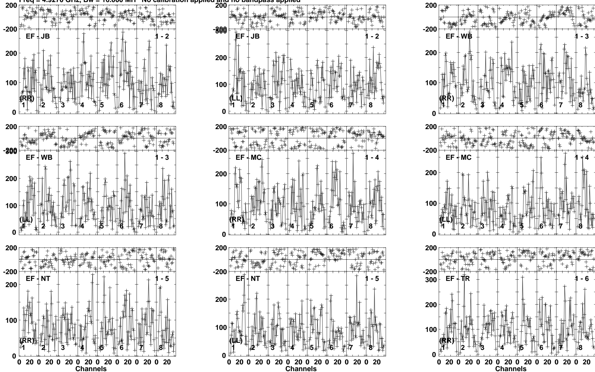
Lower frame: Micro Ampl Jy Top frame: Phas deg Vector averaged cross-power spectrum Baseline: EF (01) - JB (02) Timerange: 00/09:39:20 to 00/09:43:00
