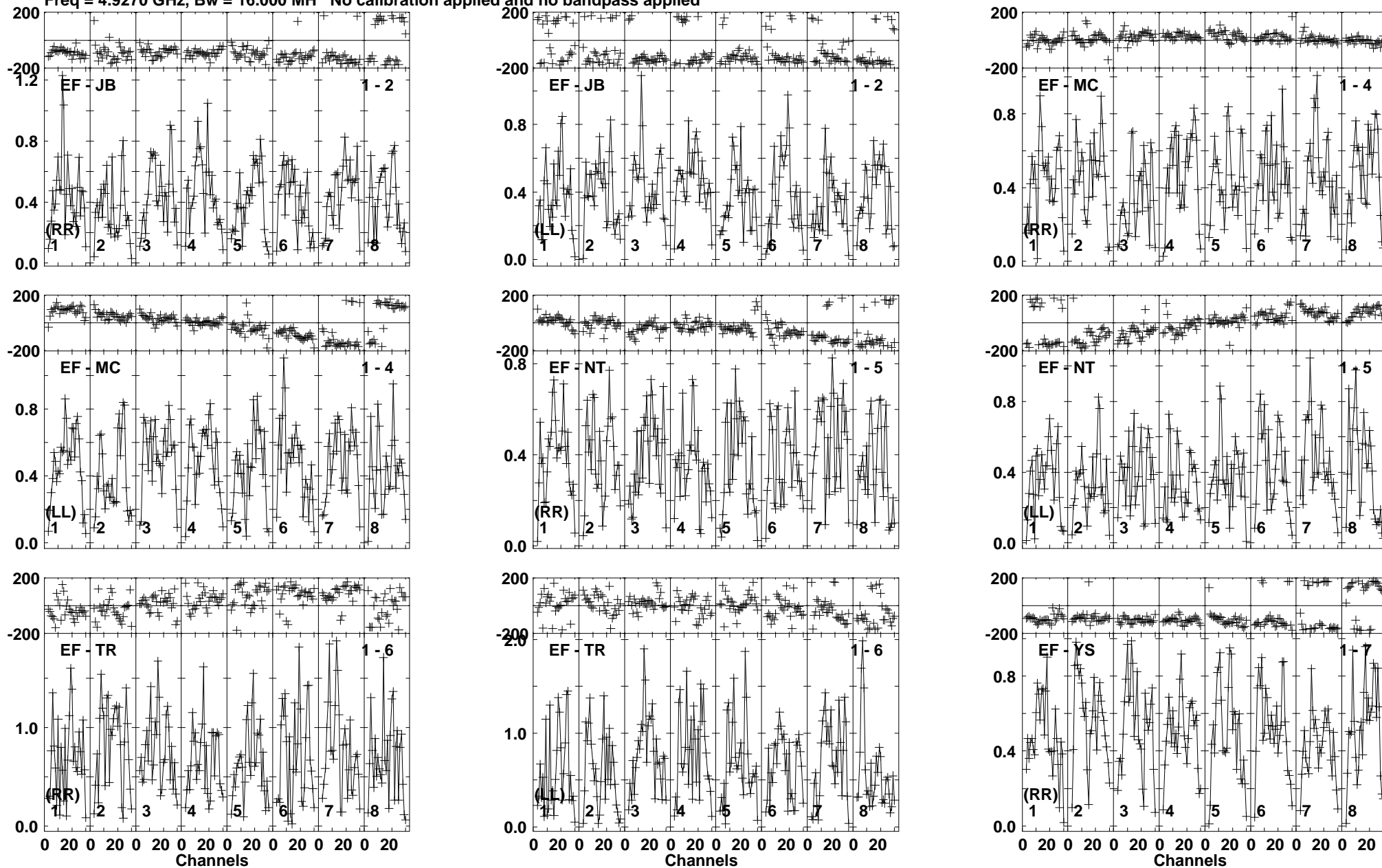
Lower frame: Milli Ampl Jy Top frame: Phas deg Vector averaged cross-power spectrum Baseline: EF (01) - JB (02) Timerange: 00/02:38:30 to 00/02:39:30
