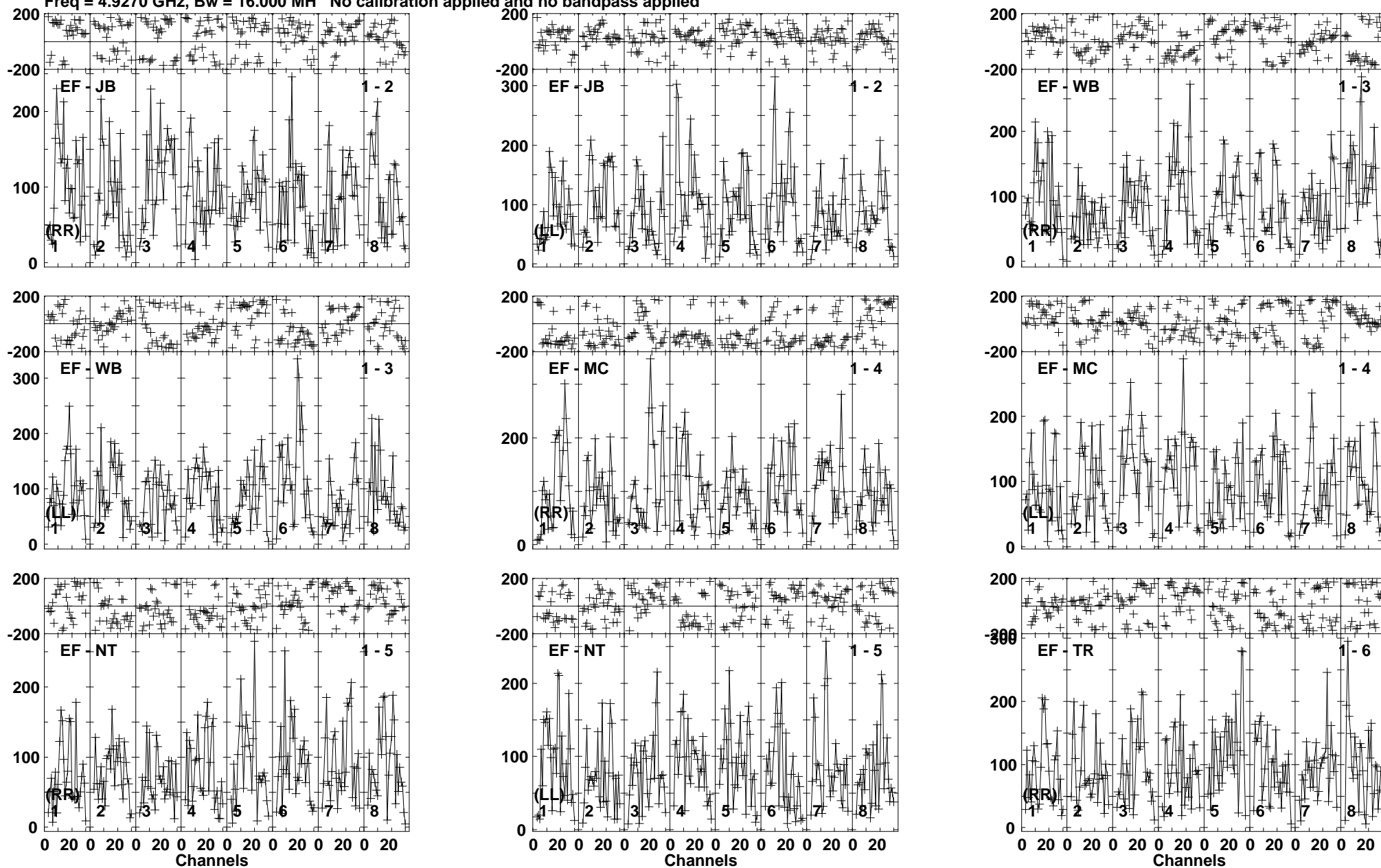
Lower frame: Micro Ampl Jy Top frame: Phas deg Vector averaged cross-power spectrum Baseline: EF (01) - JB (02) Timerange: 00/09:34:20 to 00/09:37:59
