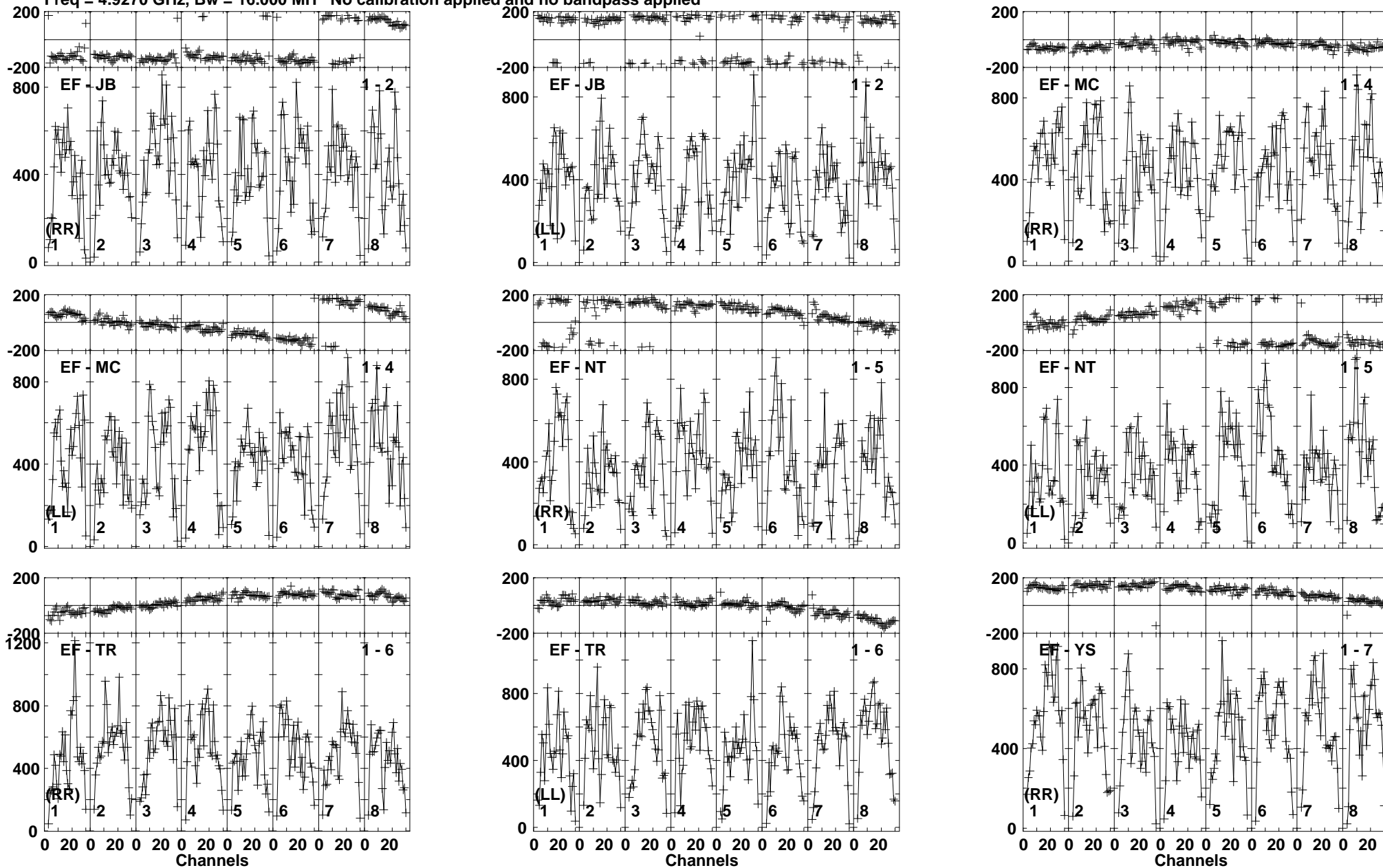
Lower frame: Micro Ampl Jy Top frame: Phas deg Vector averaged cross-power spectrum Baseline: EF (01) - JB (02) Timerange: 00/02:43:10 to 00/02:44:00
