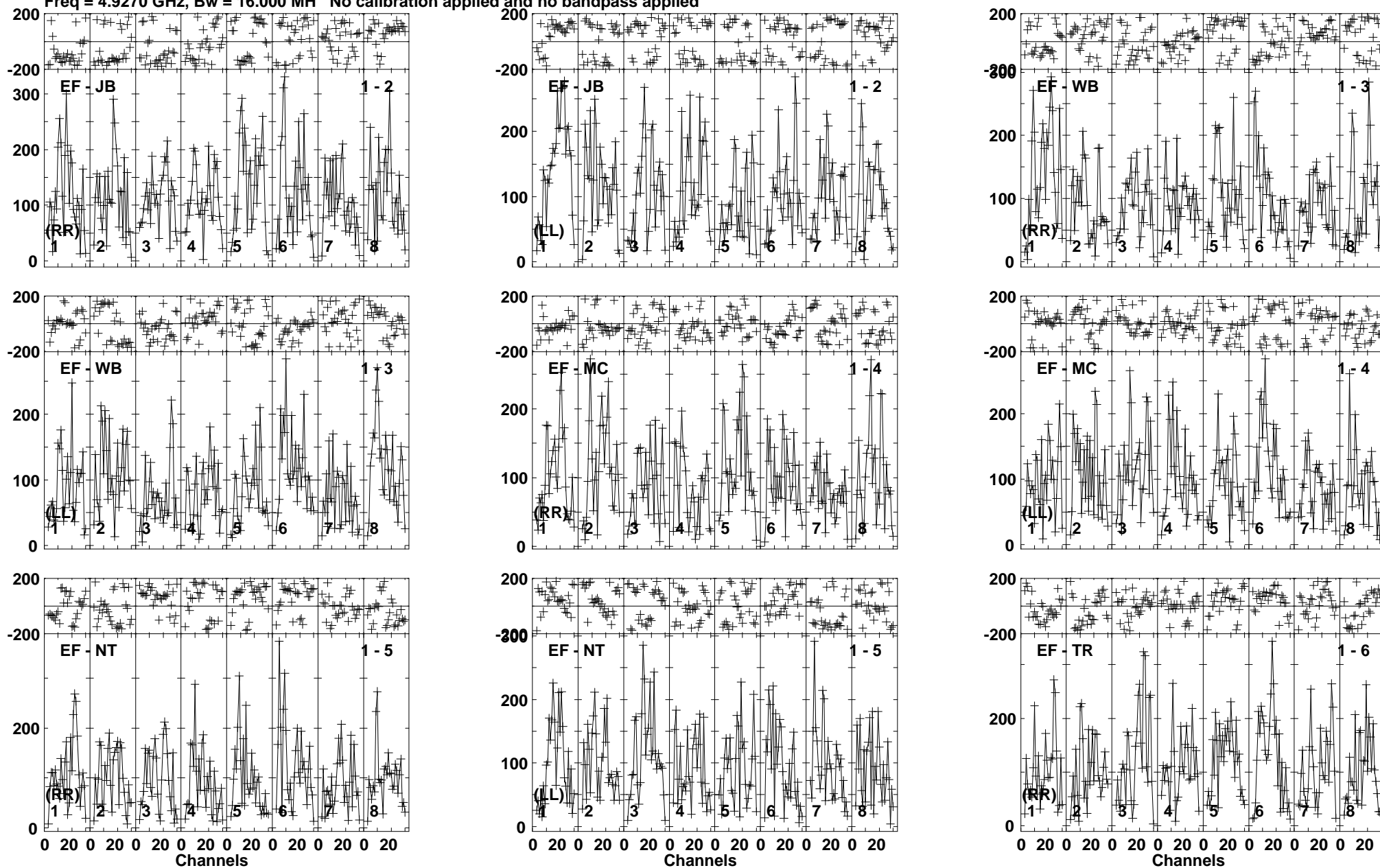
Lower frame: Micro Ampl Jy Top frame: Phas deg Vector averaged cross-power spectrum Baseline: EF (01) - JB (02) Timerange: 00/05:23:31 to 00/05:26:29
