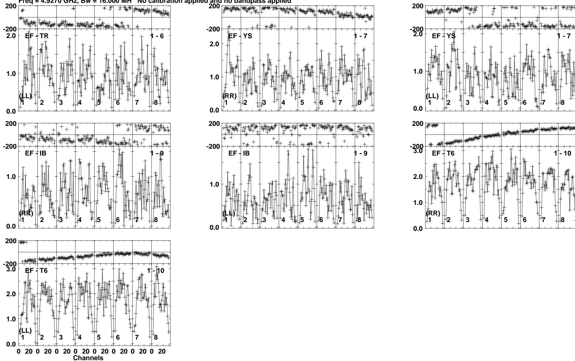
Lower frame: Milli Ampl Jy Top frame: Phas deg Vector averaged cross-power spectrum Baseline: EF (01) - TR (06) Timerange: 00/09:31:21 to 00/09:32:49
