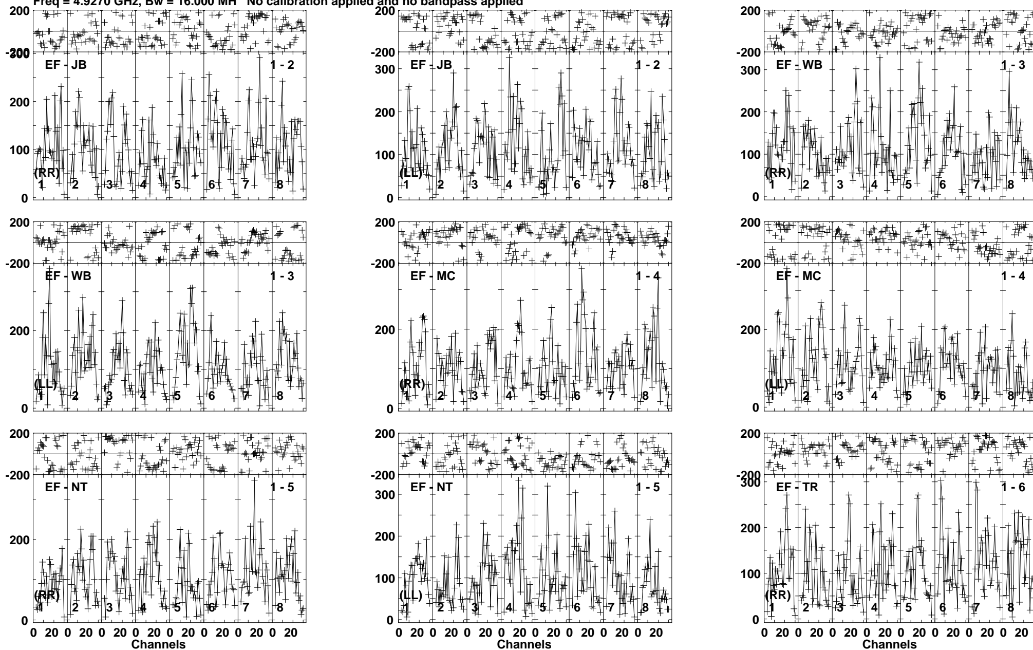
Lower frame: Micro Ampl Jy Top frame: Phas deg Vector averaged cross-power spectrum Baseline: EF (01) - JB (02) Timerange: 00/05:13:00 to 00/05:15:59
