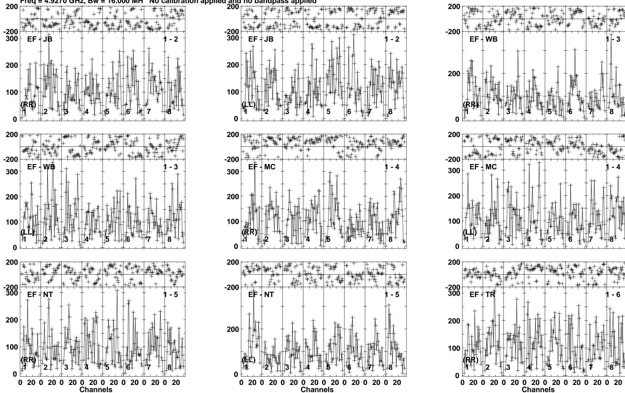
Lower frame: Micro Ampl Jy Top frame: Phas deg Vector averaged cross-power spectrum Baseline: EF (01) - JB (02) Timerange: 00/05:09:00 to 00/05:12:00
