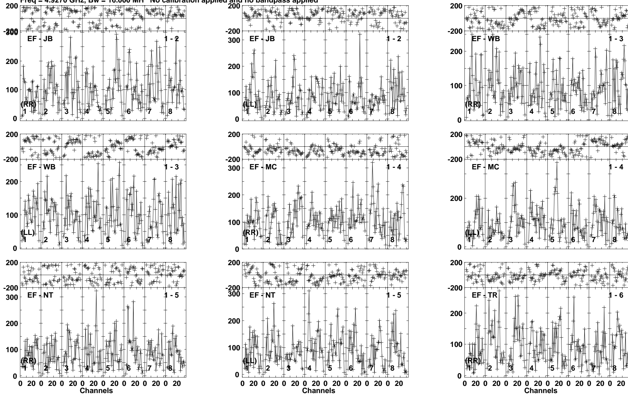
Lower frame: Micro Ampl Jy Top frame: Phas deg Vector averaged cross-power spectrum Baseline: EF (01) - JB (02) Timerange: 00/07:56:50 to 00/08:00:30
