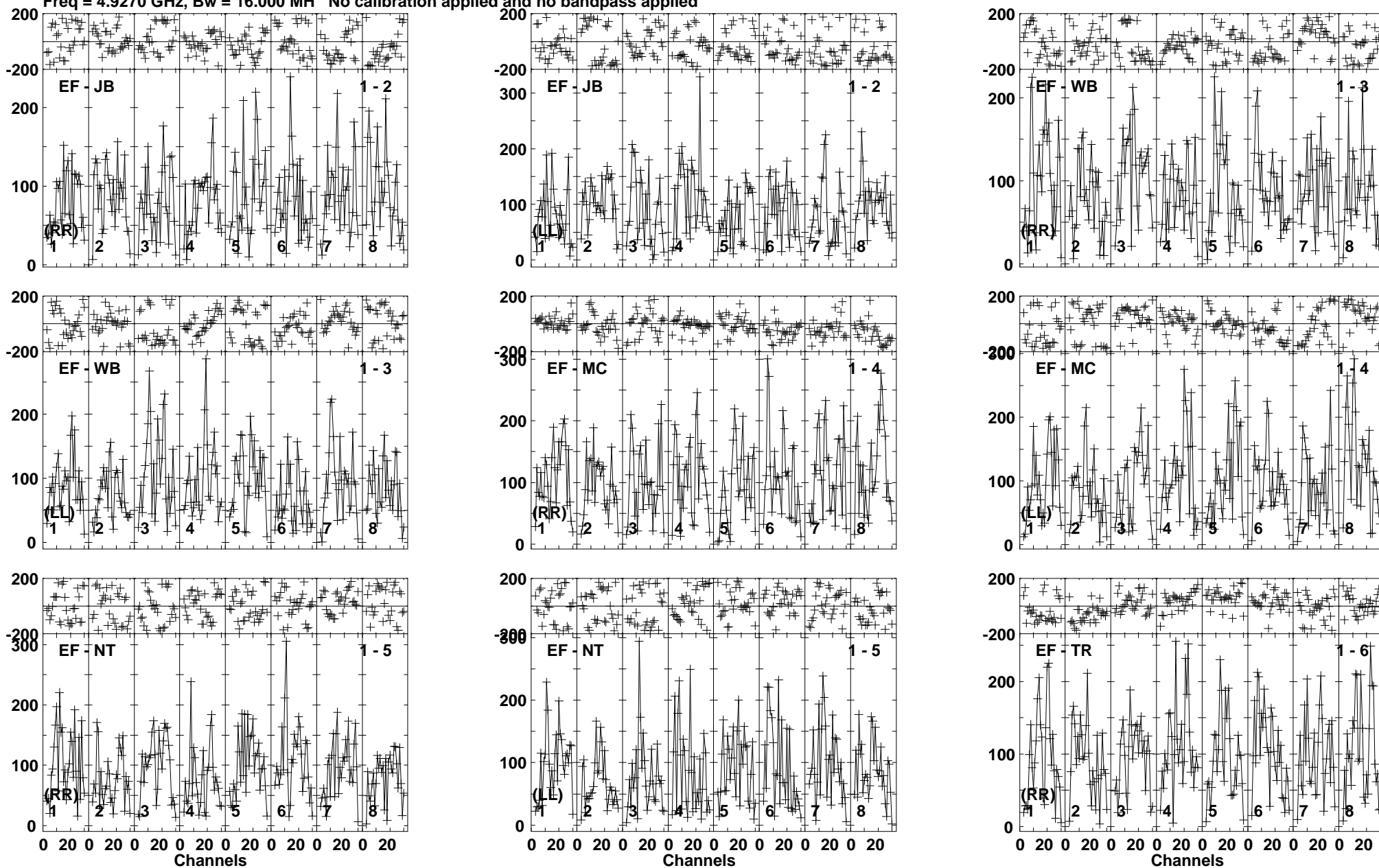
Lower frame: Micro Ampl Jy Top frame: Phas deg Vector averaged cross-power spectrum Baseline: EF (01) - JB (02) Timerange: 00/09:16:10 to 00/09:19:50
