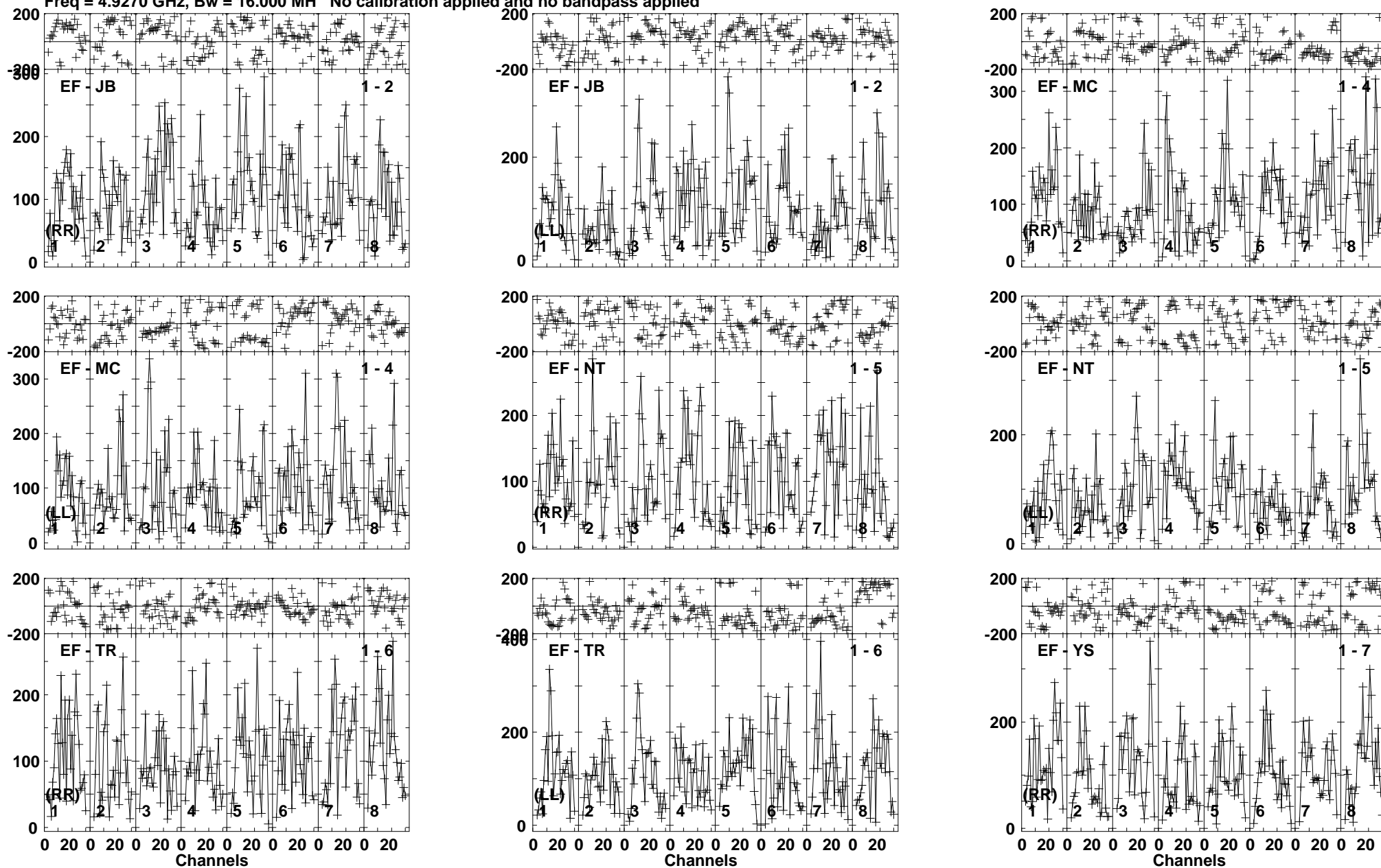
Lower frame: Micro Ampl Jy Top frame: Phas deg Vector averaged cross-power spectrum Baseline: EF (01) - JB (02) Timerange: 00/03:02:31 to 00/03:05:29
