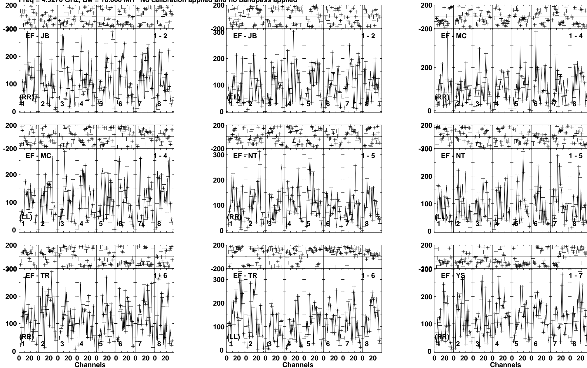
Lower frame: Micro Ampl Jy Top frame: Phas deg Vector averaged cross-power spectrum Baseline: EF (01) - JB (02) Timerange: 00/03:33:31 to 00/03:36:29
