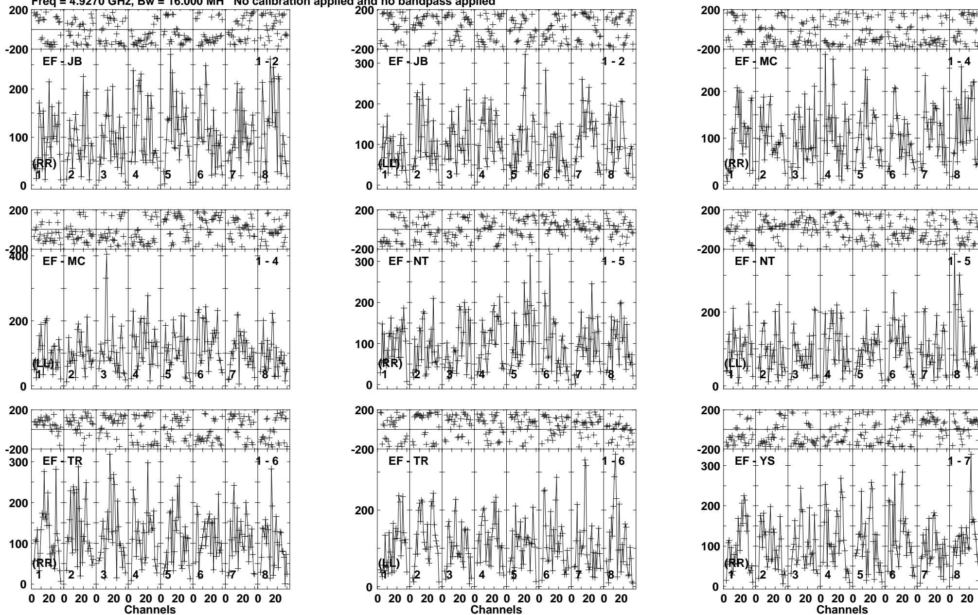
Lower frame: Micro Ampl Jy Top frame: Phas deg Vector averaged cross-power spectrum Baseline: EF (01) - JB (02) Timerange: 00/03:38:01 to 00/03:40:59
