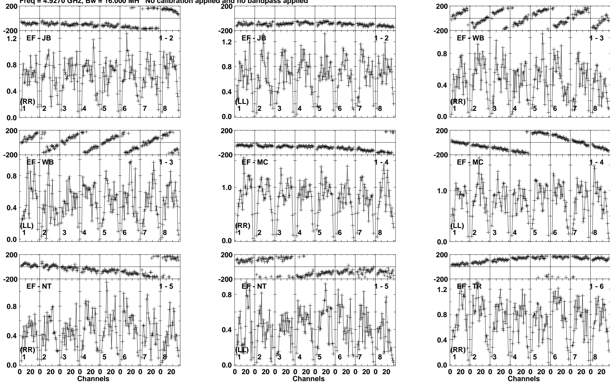
Lower frame: Milli Ampl Jy Top frame: Phas deg Vector averaged cross-power spectrum Baseline: EF (01) - JB (02) Timerange: 00/11:36:01 to 00/11:37:29
