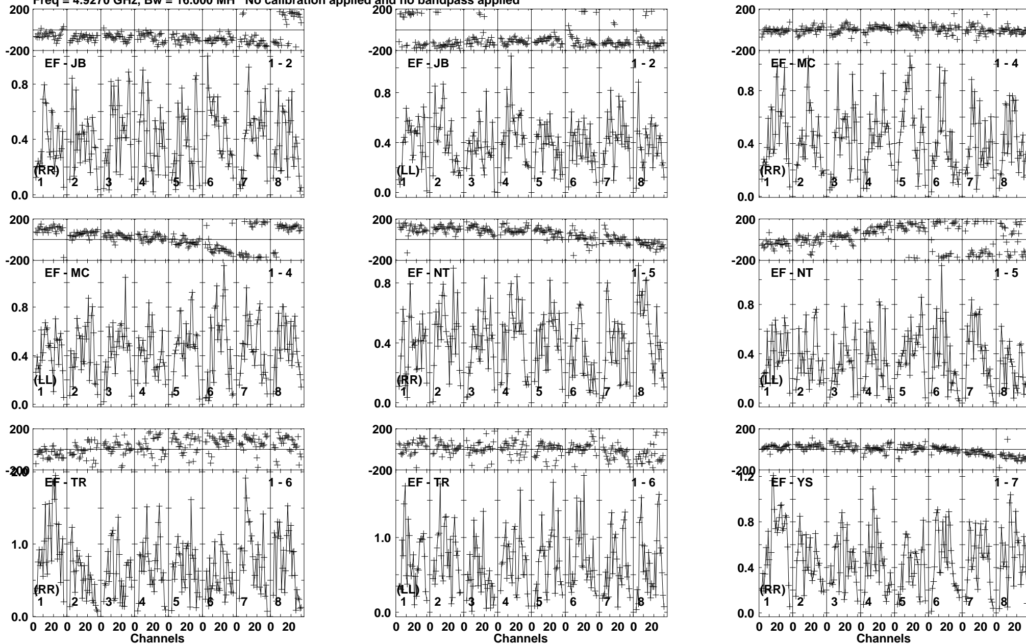
Lower frame: Milli Ampl Jy Top frame: Phas deg Vector averaged cross-power spectrum Baseline: EF (01) - JB (02) Timerange: 00/02:34:30 to 00/02:35:30
