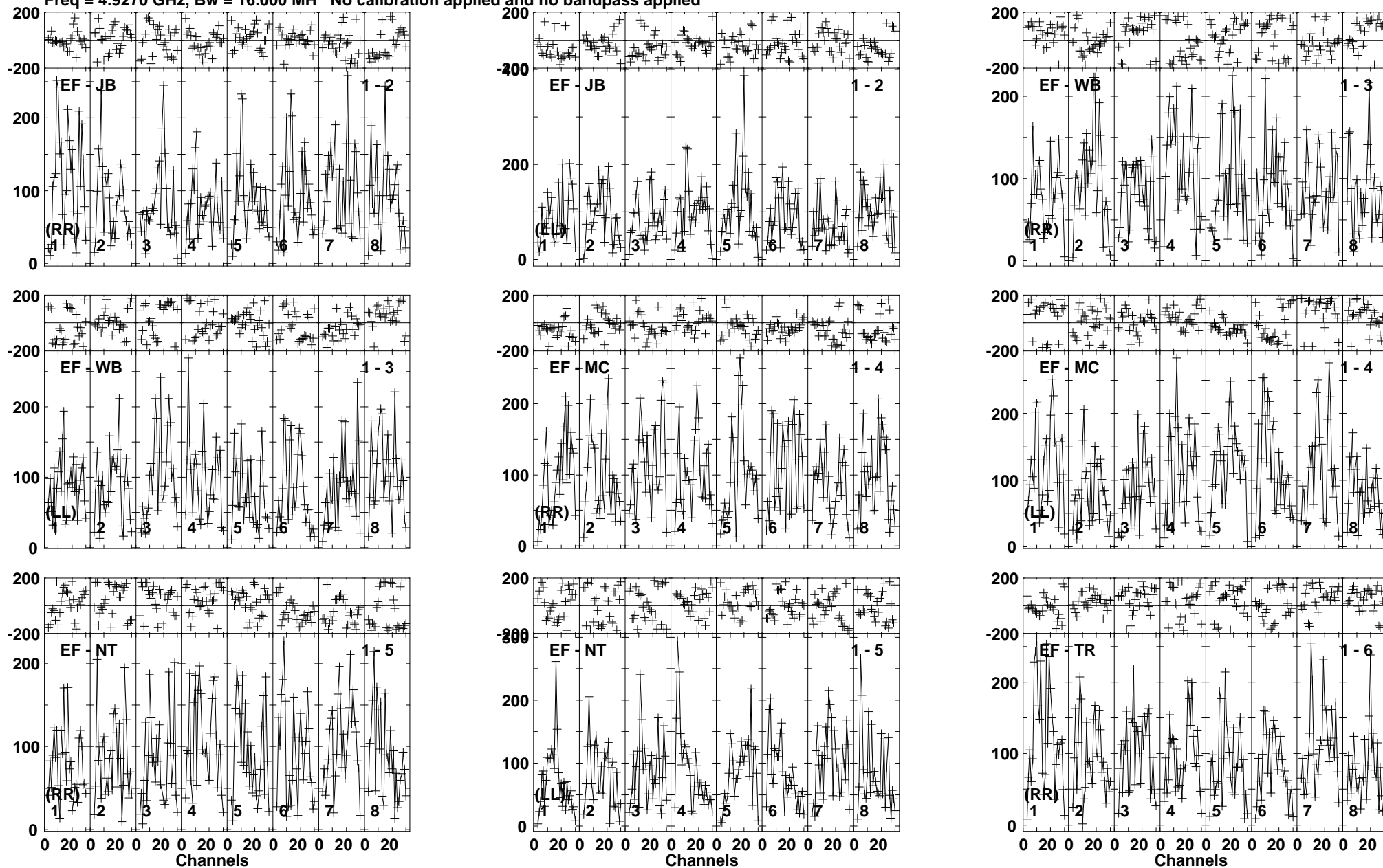
Lower frame: Micro Ampl Jy Top frame: Phas deg Vector averaged cross-power spectrum Baseline: EF (01) - JB (02) Timerange: 00/07:18:30 to 00/07:22:10
