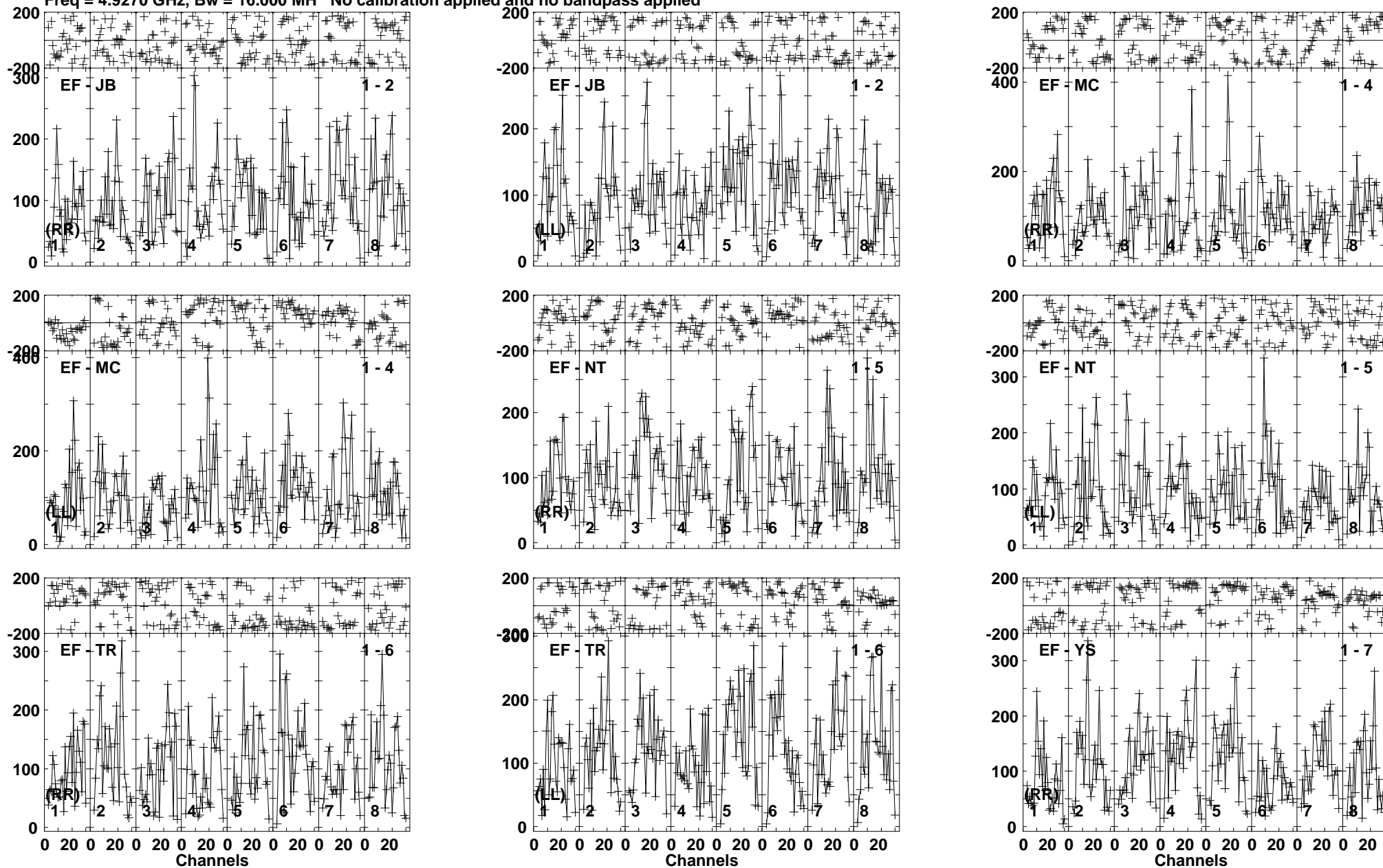
Lower frame: Micro Ampl Jy Top frame: Phas deg Vector averaged cross-power spectrum Baseline: EF (01) - JB (02) Timerange: 00/03:42:00 to 00/03:45:00
