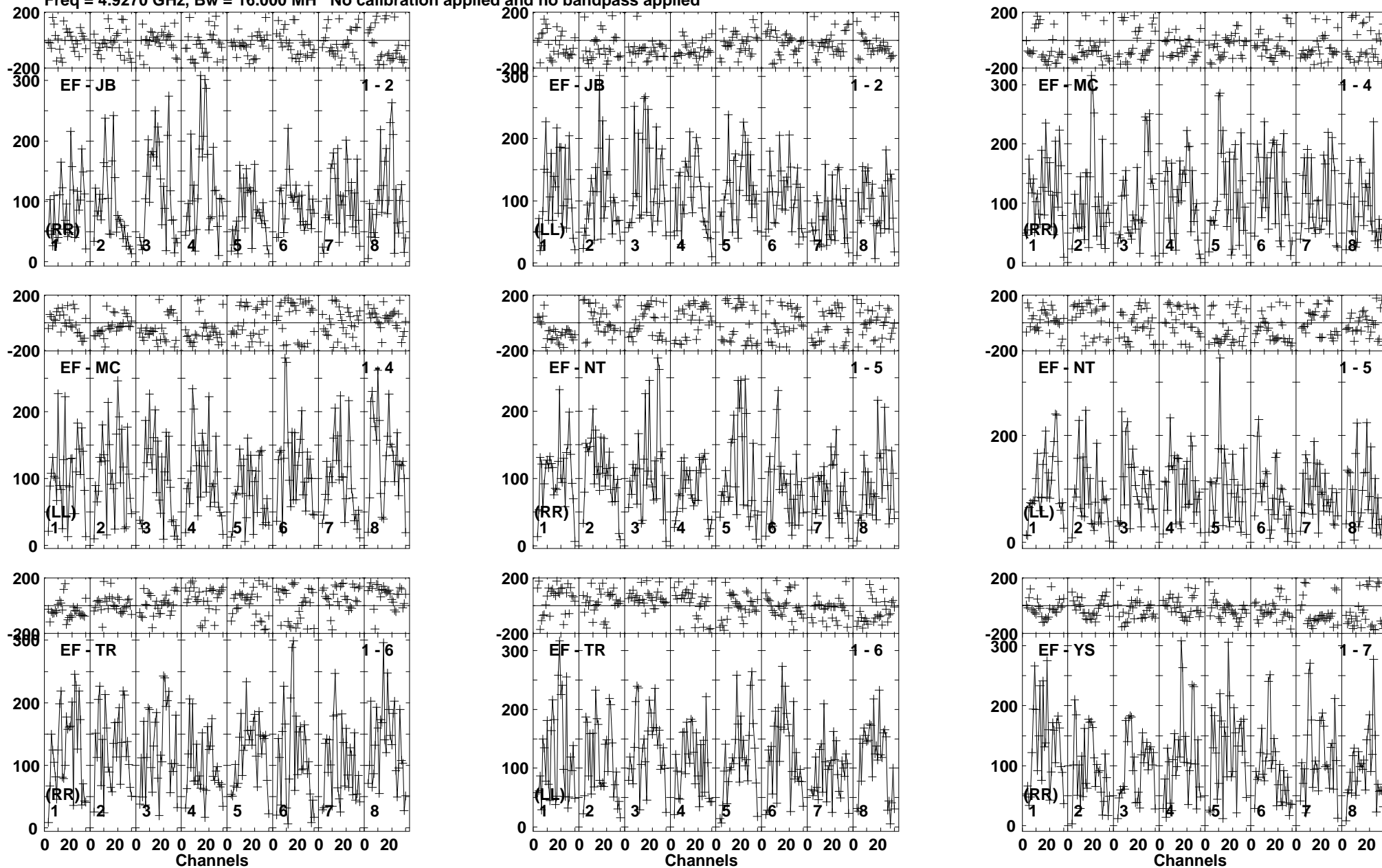
Lower frame: Micro Ampl Jy Top frame: Phas deg Vector averaged cross-power spectrum Baseline: EF (01) - JB (02) Timerange: 00/04:09:00 to 00/04:11:59
