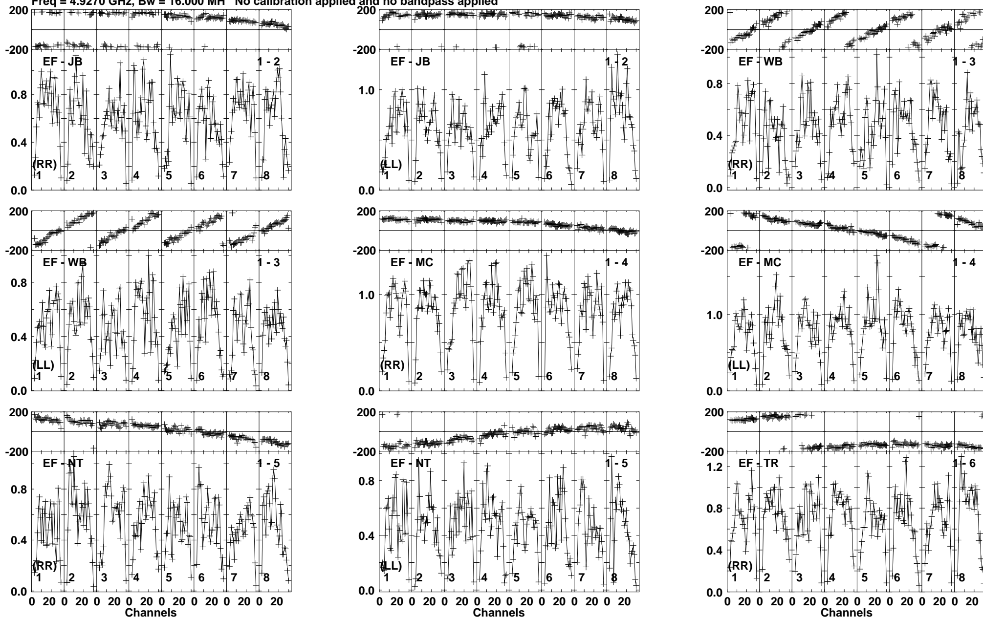
Lower frame: Milli Ampl Jy Top frame: Phas deg Vector averaged cross-power spectrum Baseline: EF (01) - JB (02) Timerange: 00:12:04:00 to 00:12:05:30
