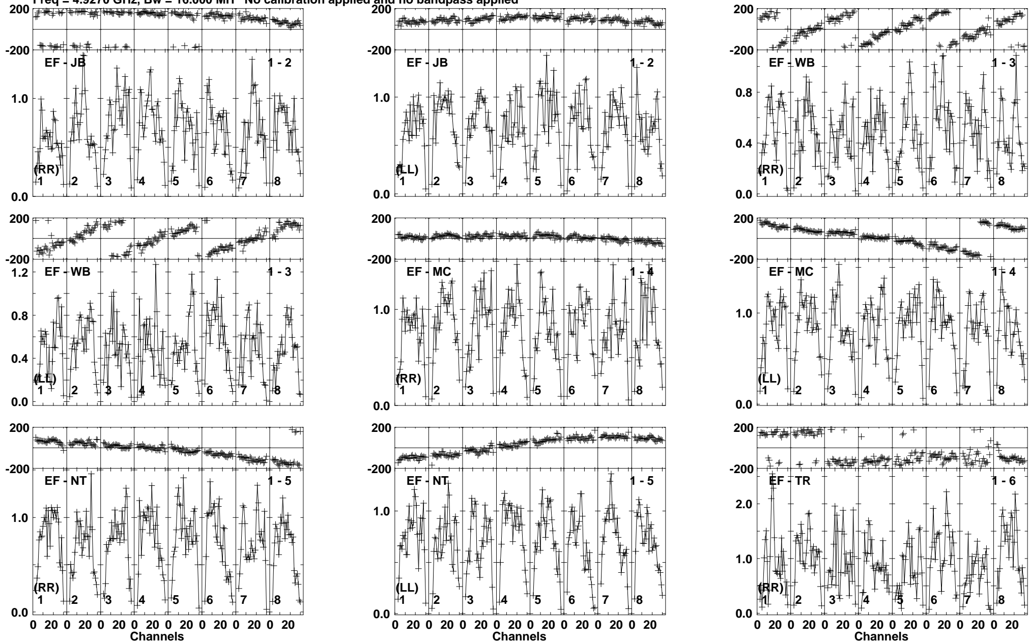
Lower frame: Milli Ampl Jy Top frame: Phas deg Vector averaged cross-power spectrum Baseline: EF (01) - JB (02) Timerange: 00/06:16:30 to 00/06:17:29
