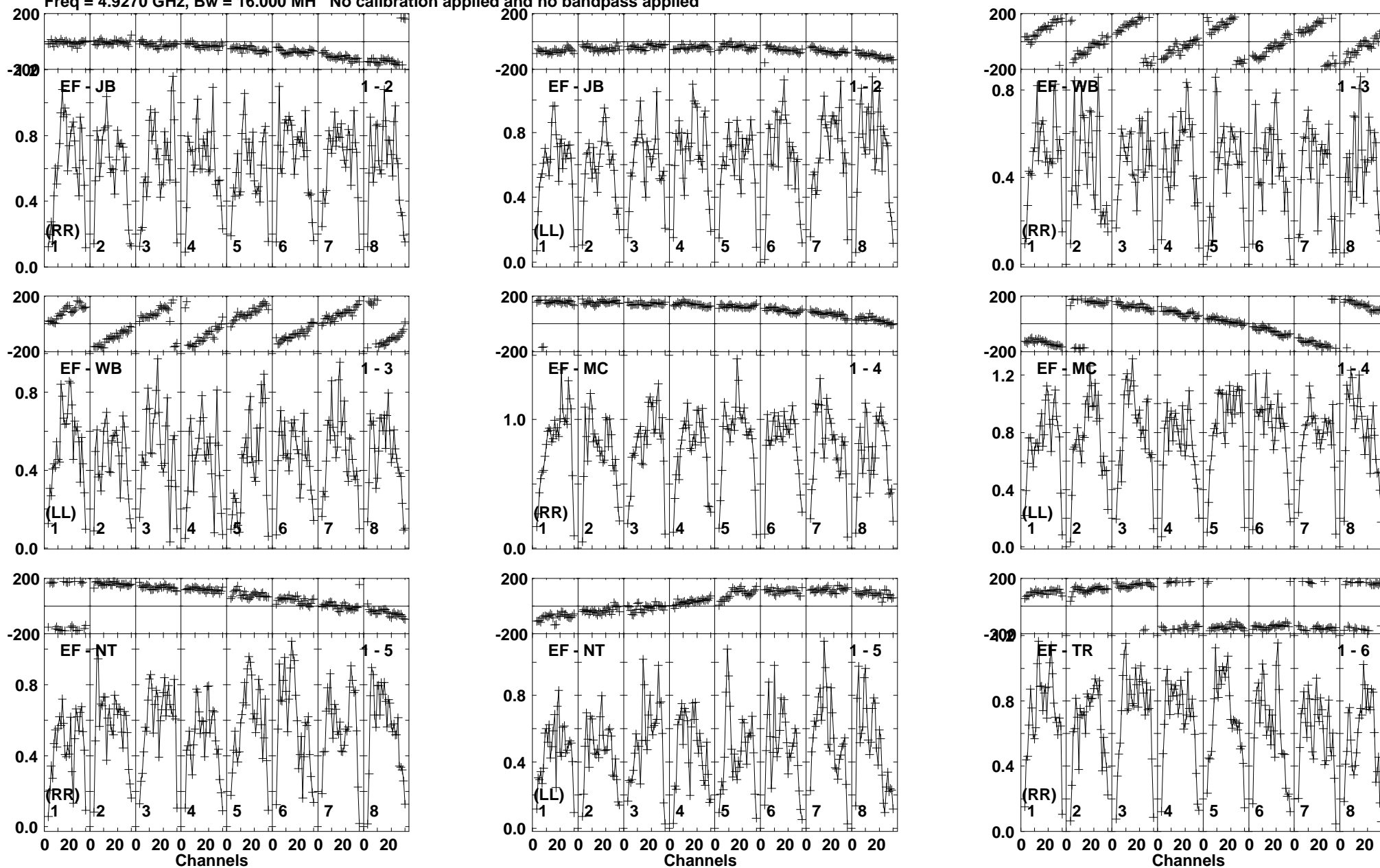
Lower frame: Milli Ampl Jy Top frame: Phas deg Vector averaged cross-power spectrum Baseline: EF (01) - JB (02) Timerange: 00:12:32:00 to 00:12:33:29
