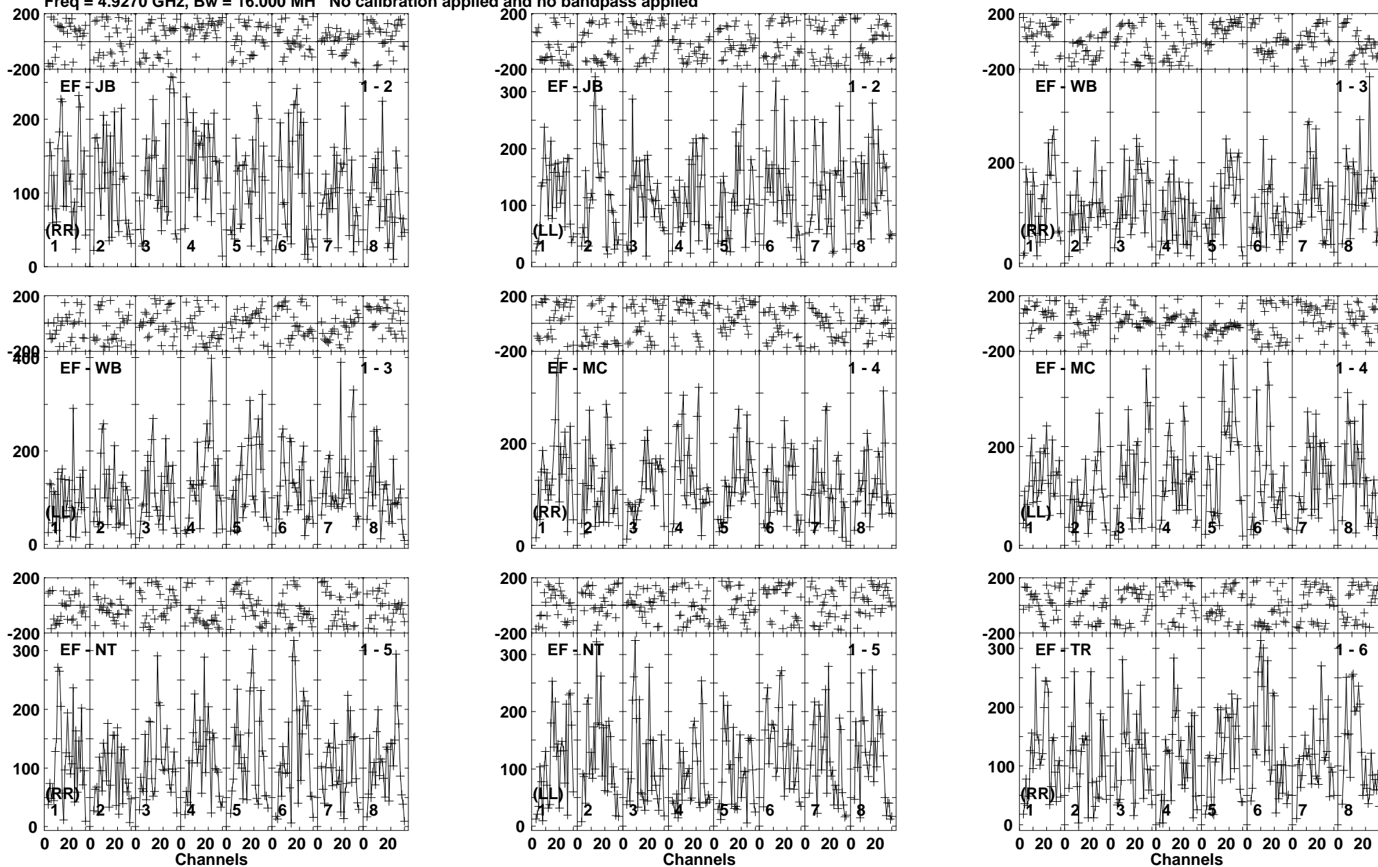
Lower frame: Micro Ampl Jy Top frame: Phas deg Vector averaged cross-power spectrum Baseline: EF (01) - JB (02) Timerange: 00/10:41:31 to 00/10:45:00
