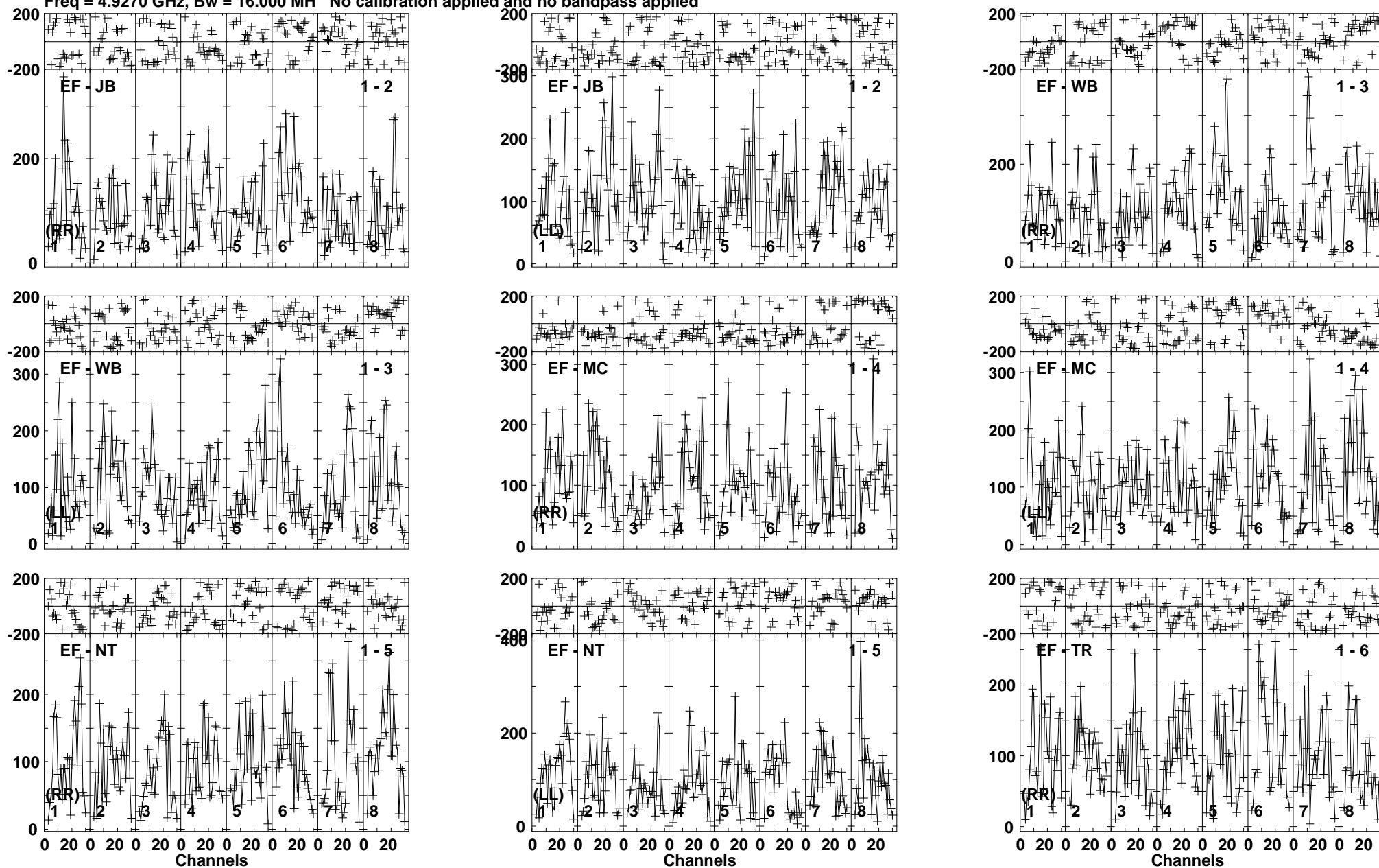
Lower frame: Micro Ampl Jy Top frame: Phas deg Vector averaged cross-power spectrum Baseline: EF (01) - JB (02) Timerange: 00/11:19:40 to 00/11:23:09
