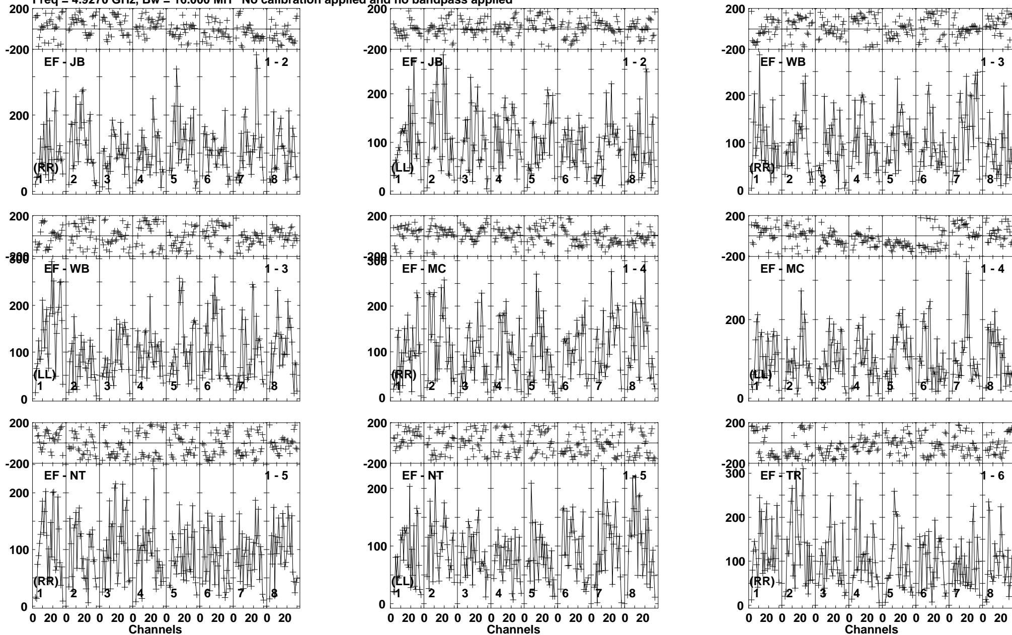
Lower frame: Micro Ampl Jy Top frame: Phas deg Vector averaged cross-power spectrum Baseline: EF (01) - JB (02) Timerange: 00/11:42:30 to 00/11:45:59
