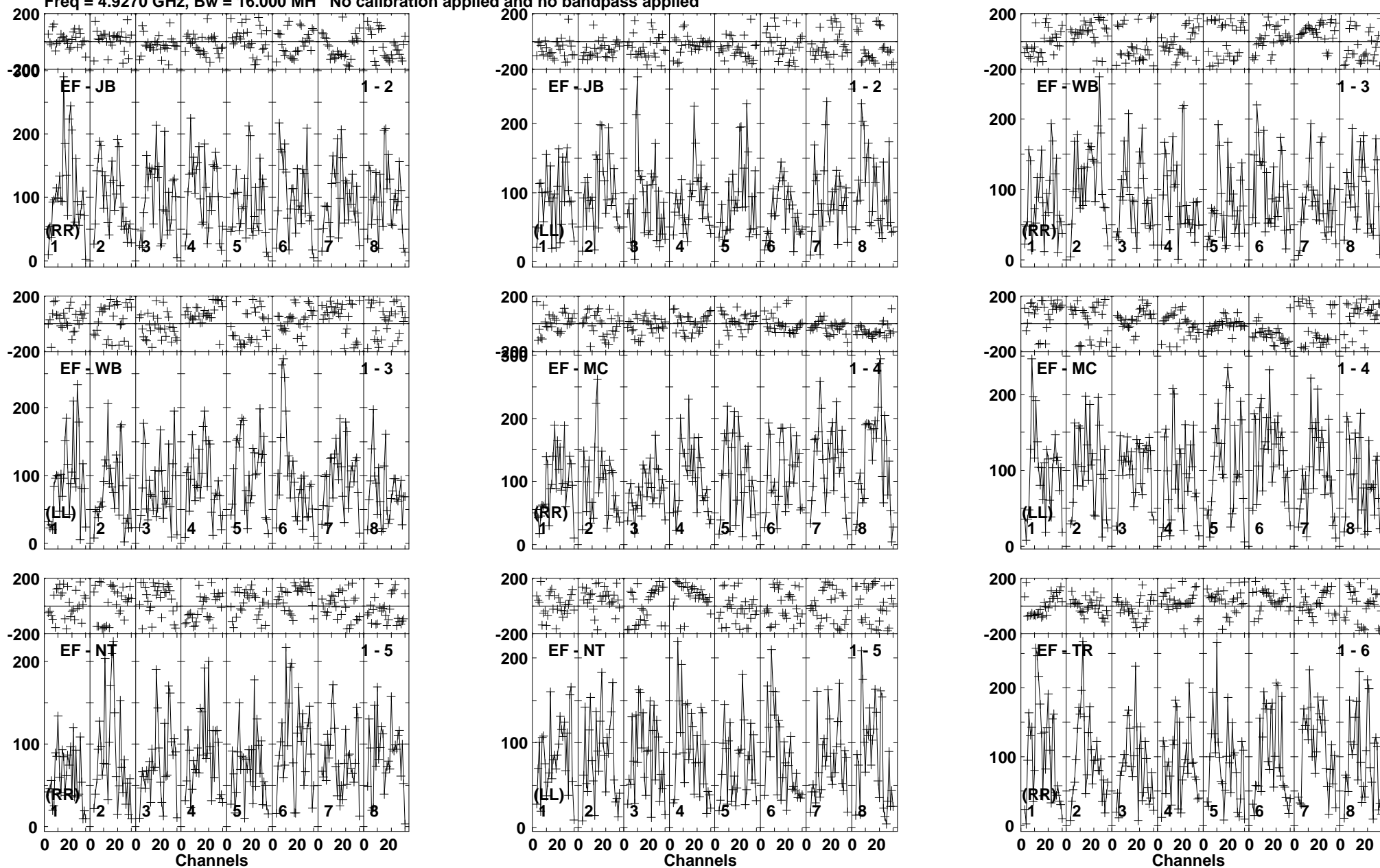
Lower frame: Micro Ampl Jy Top frame: Phas deg Vector averaged cross-power spectrum Baseline: EF (01) - JB (02) Timerange: 00/07:13:30 to 00/07:17:10
