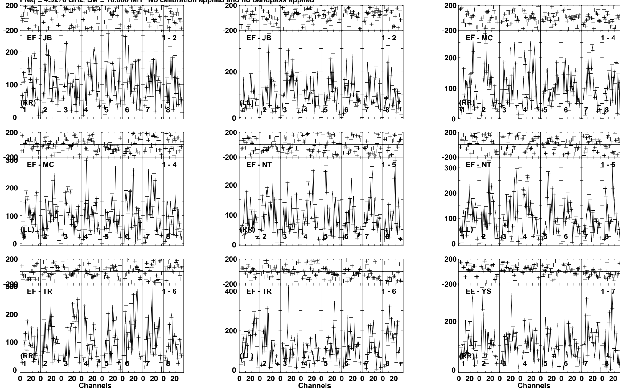
Lower frame: Micro Ampl Jy Top frame: Phas deg Vector averaged cross-power spectrum Baseline: EF (01) - JB (02) Timerange: 00/02:52:00 to 00/02:54:59
