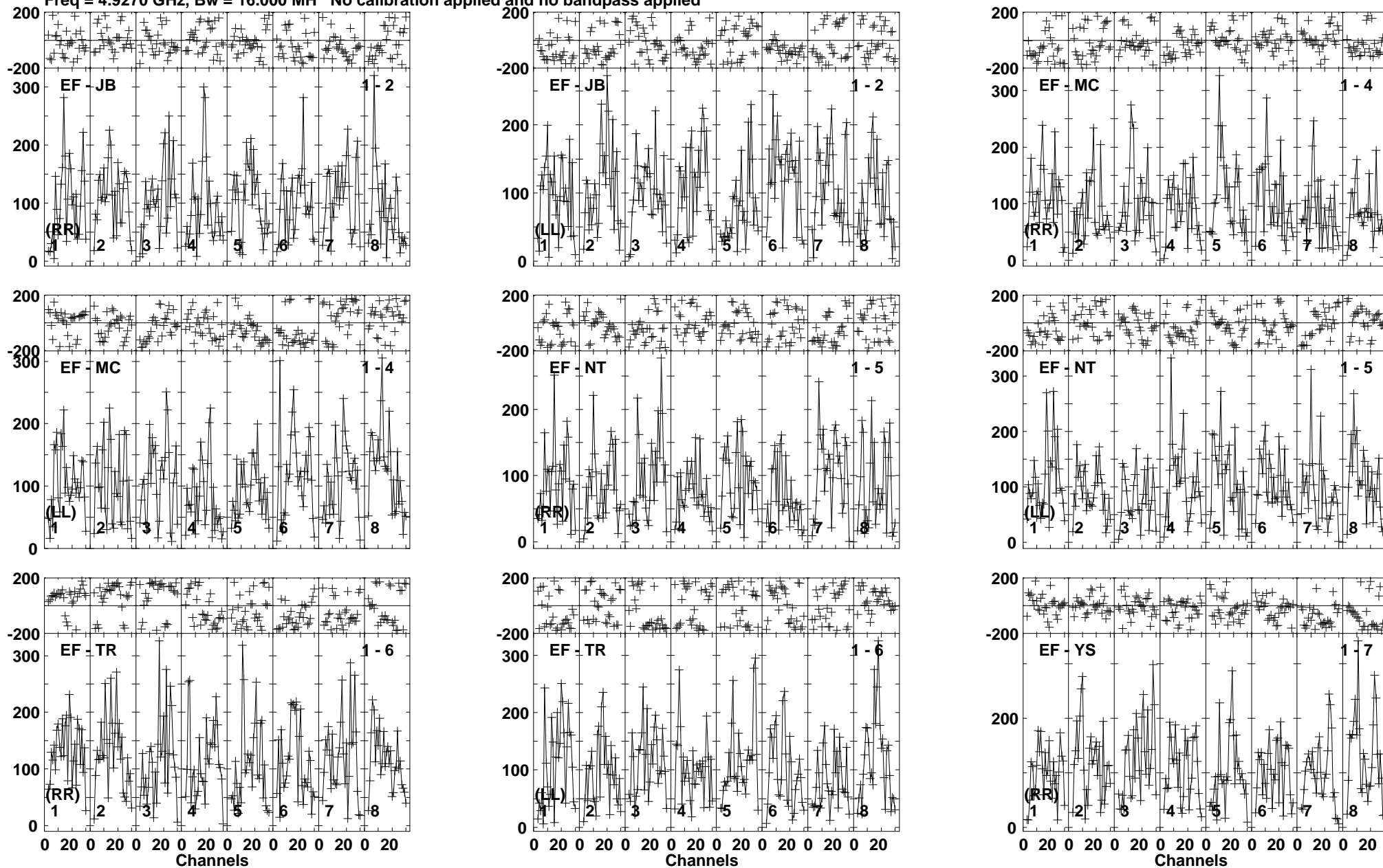
Lower frame: Micro Ampl Jy Top frame: Phas deg Vector averaged cross-power spectrum Baseline: EF (01) - JB (02) Timerange: 00/03:25:30 to 00/03:28:30
