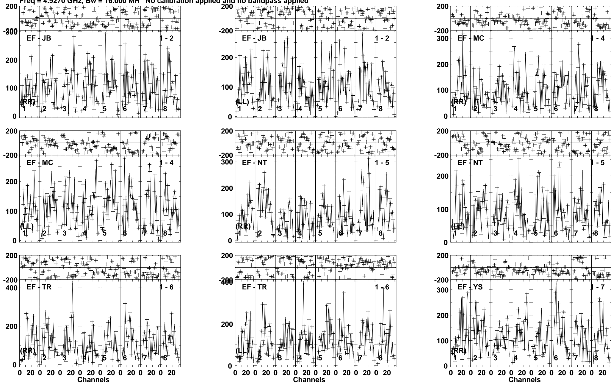
Lower frame: Micro Ampl Jy Top frame: Phas deg Vector averaged cross-power spectrum Baseline: EF (01) - JB (02) Timerange: 00/03:29:30 to 00/03:32:29
