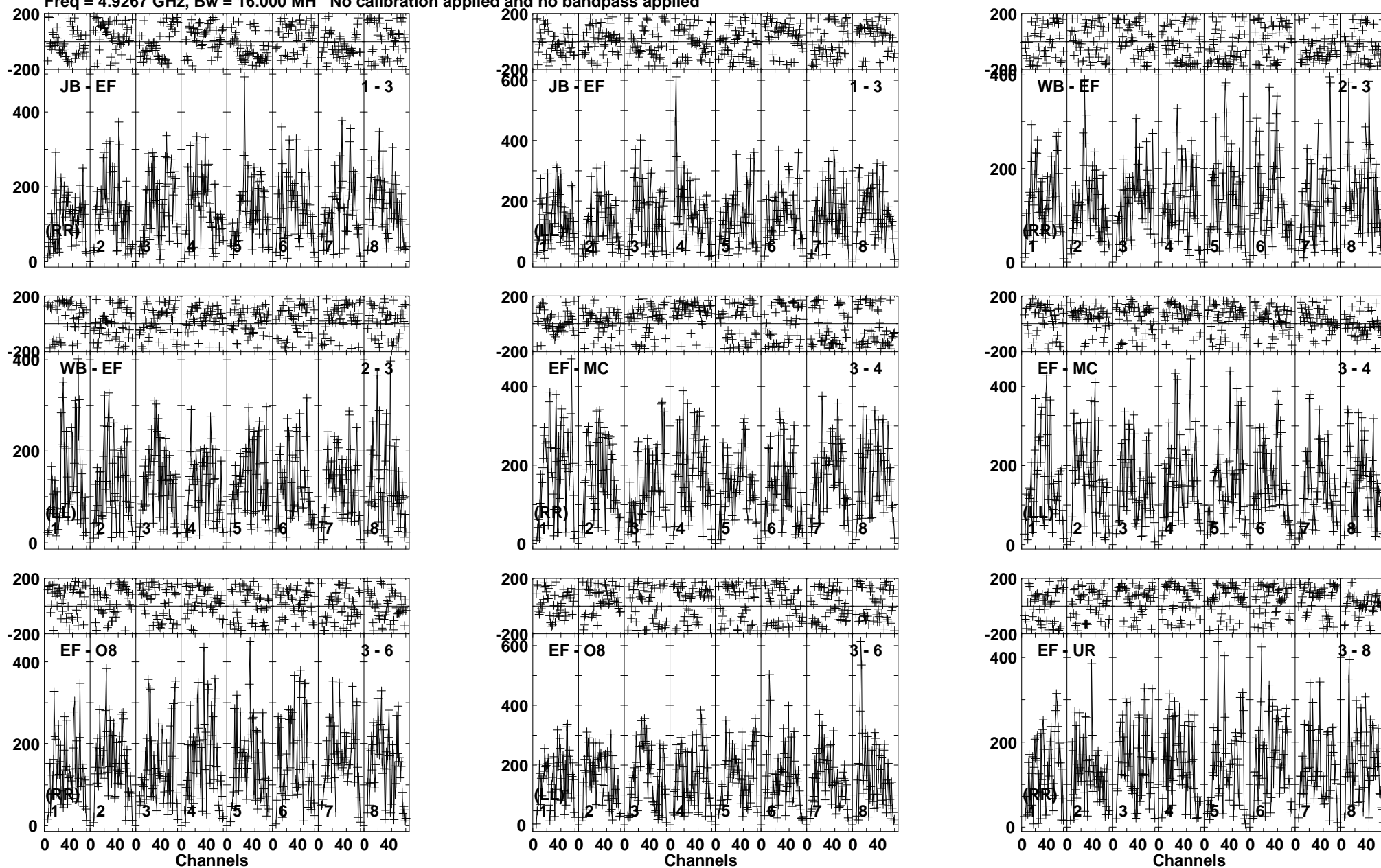
Lower frame: Micro Ampl Jy Top frame: Phas deg Vector averaged cross-power spectrum Baseline: JB (01) - EF (03) Timerange: 00/10:38:01 to 00/10:40:59
