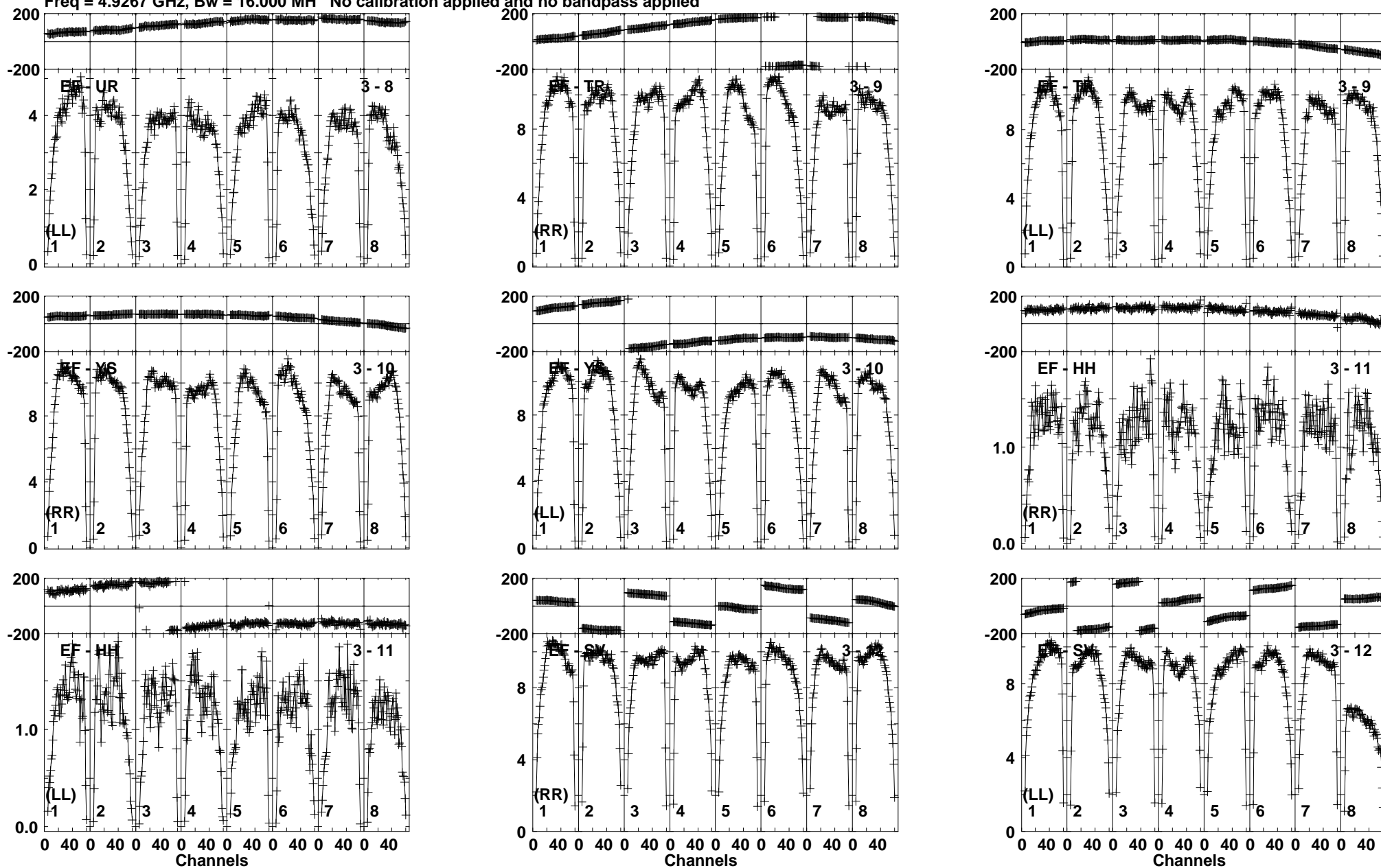
Lower frame: Milli Ampl Jy Top frame: Phas deg Vector averaged cross-power spectrum Baseline: EF (03) - UR (08) Timerange: 00/08:45:31 to 00/08:46:29
