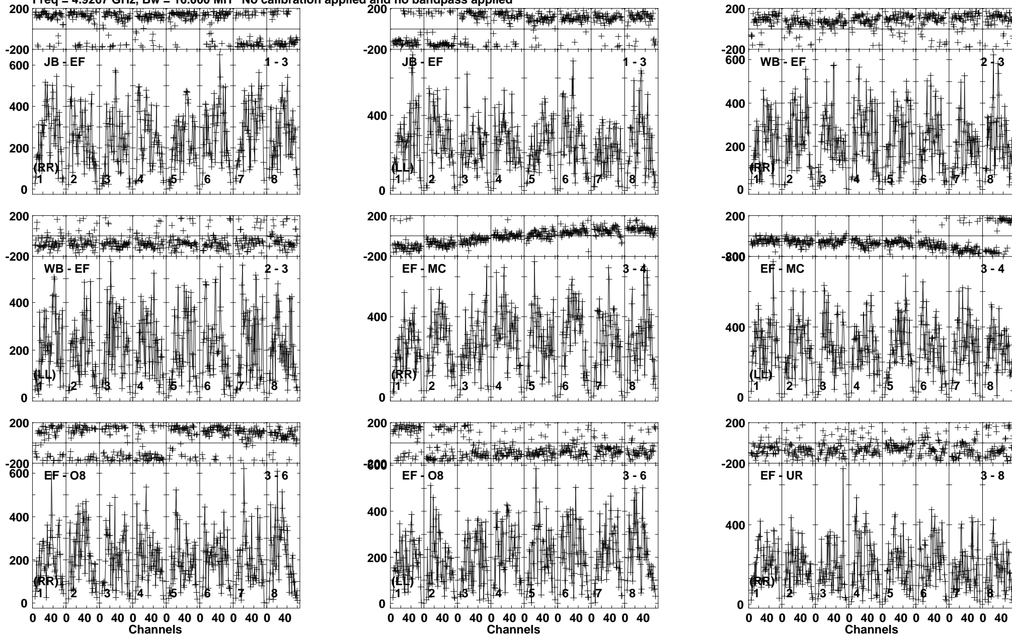
Lower frame: Micro Ampl Jy Top frame: Phas deg Vector averaged cross-power spectrum Baseline: JB (01) - EF (03) Timerange: 00/13:43:01 to 00/13:44:59
