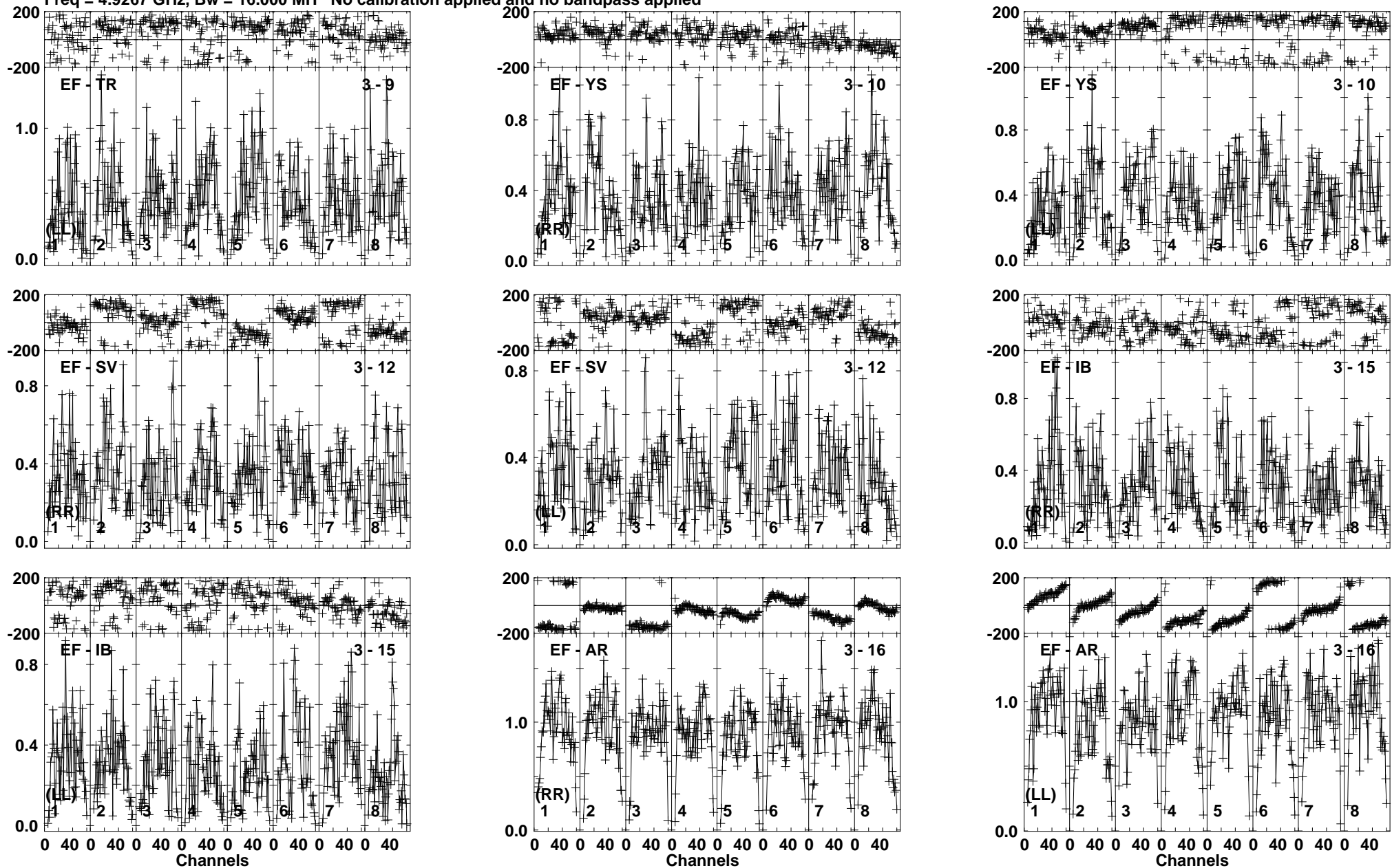
Lower frame: Milli Ampl Jy Top frame: Phas deg Vector averaged cross-power spectrum Baseline: EF (03) - TR (09) Timerange: 00/18:52:01 to 00/18:52:59
