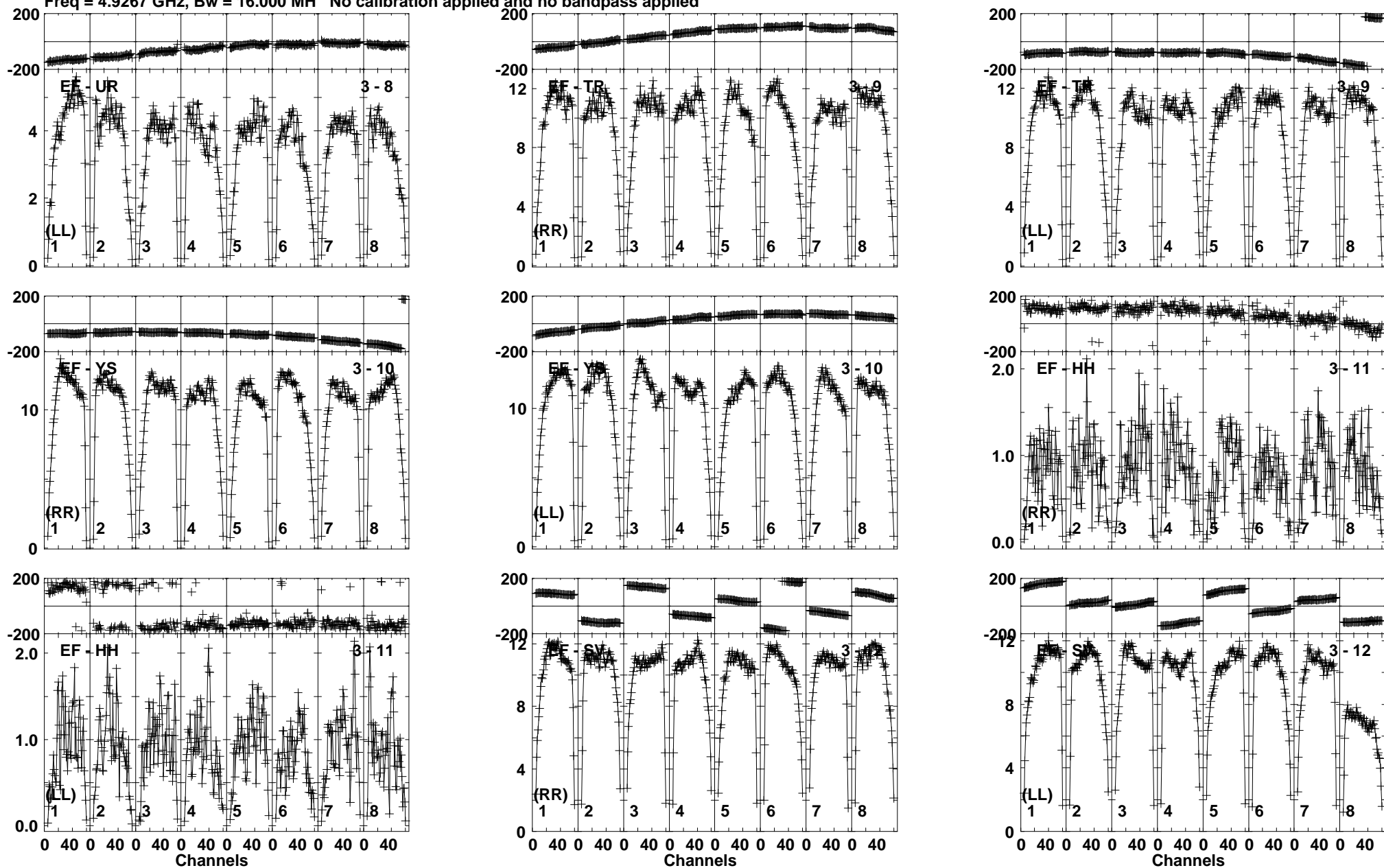
Lower frame: Milli Ampl Jy Top frame: Phas deg Vector averaged cross-power spectrum Baseline: EF (03) - UR (08) Timerange: 00/11:49:31 to 00/11:50:29
