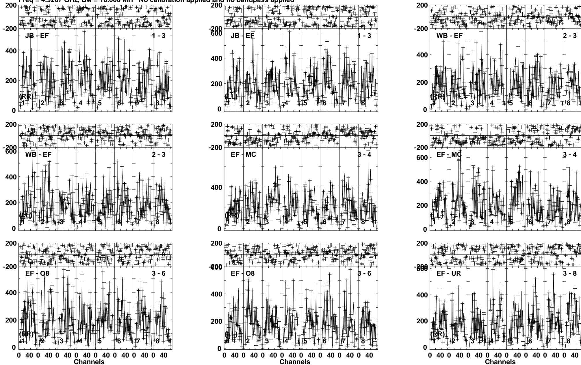
Lower frame: Micro Ampl Jy Top frame: Phas deg Vector averaged cross-power spectrum Baseline: JB (01) - EF (03) Timerange: 00/14:50:01 to 00/14:51:59
