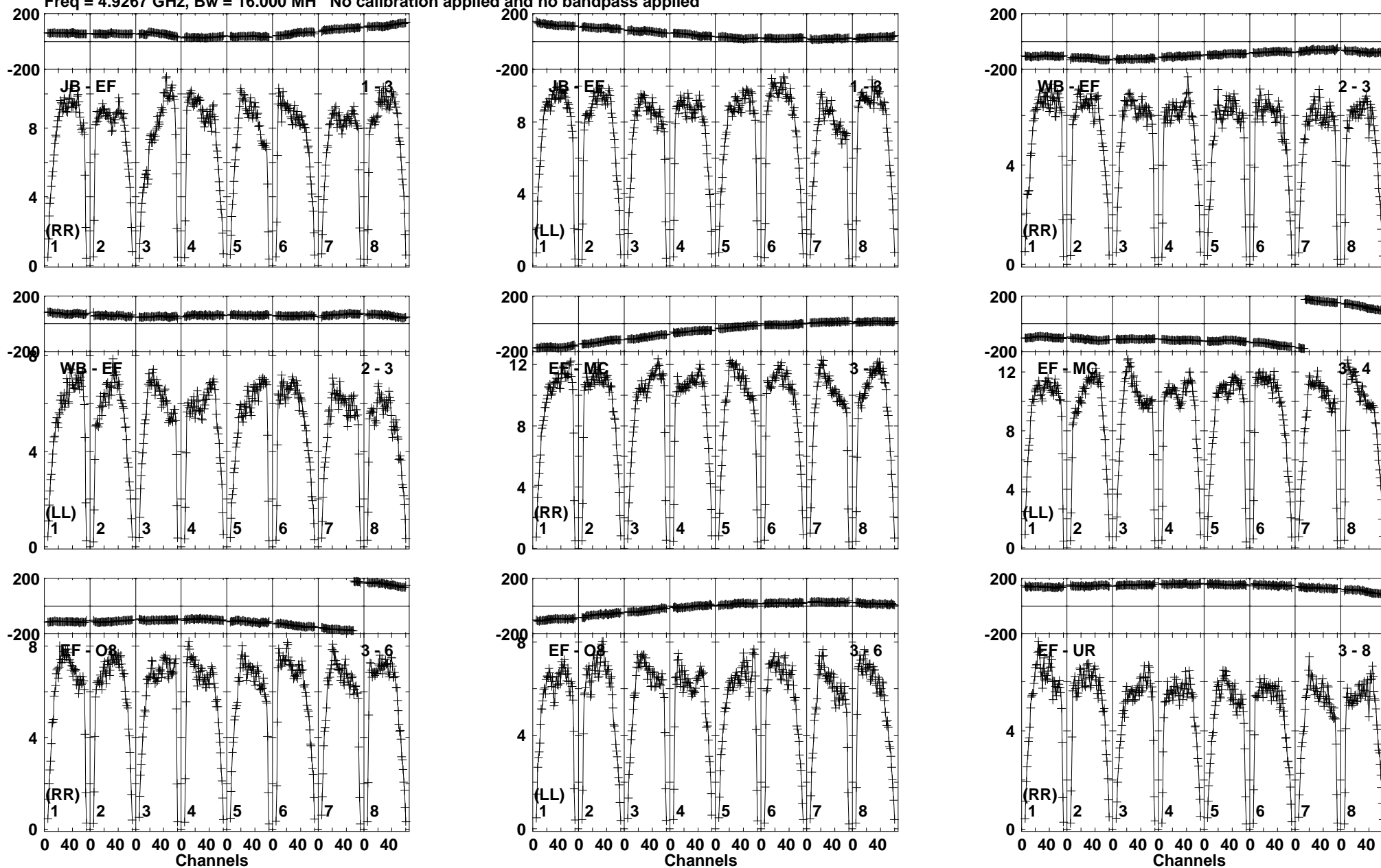
Lower frame: Milli Ampl Jy Top frame: Phas deg Vector averaged cross-power spectrum Baseline: JB (01) - EF (03) Timerange: 00/14:17:31 to 00/14:18:29
