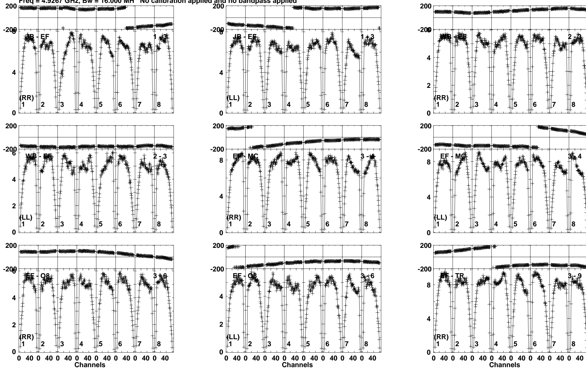
Lower frame: Milli Ampl Jy Top frame: Phas deg Vector averaged cross-power spectrum Baseline: JB (01) - EF (03) Timerange: 00/19:33:31 to 00/19:34:29
