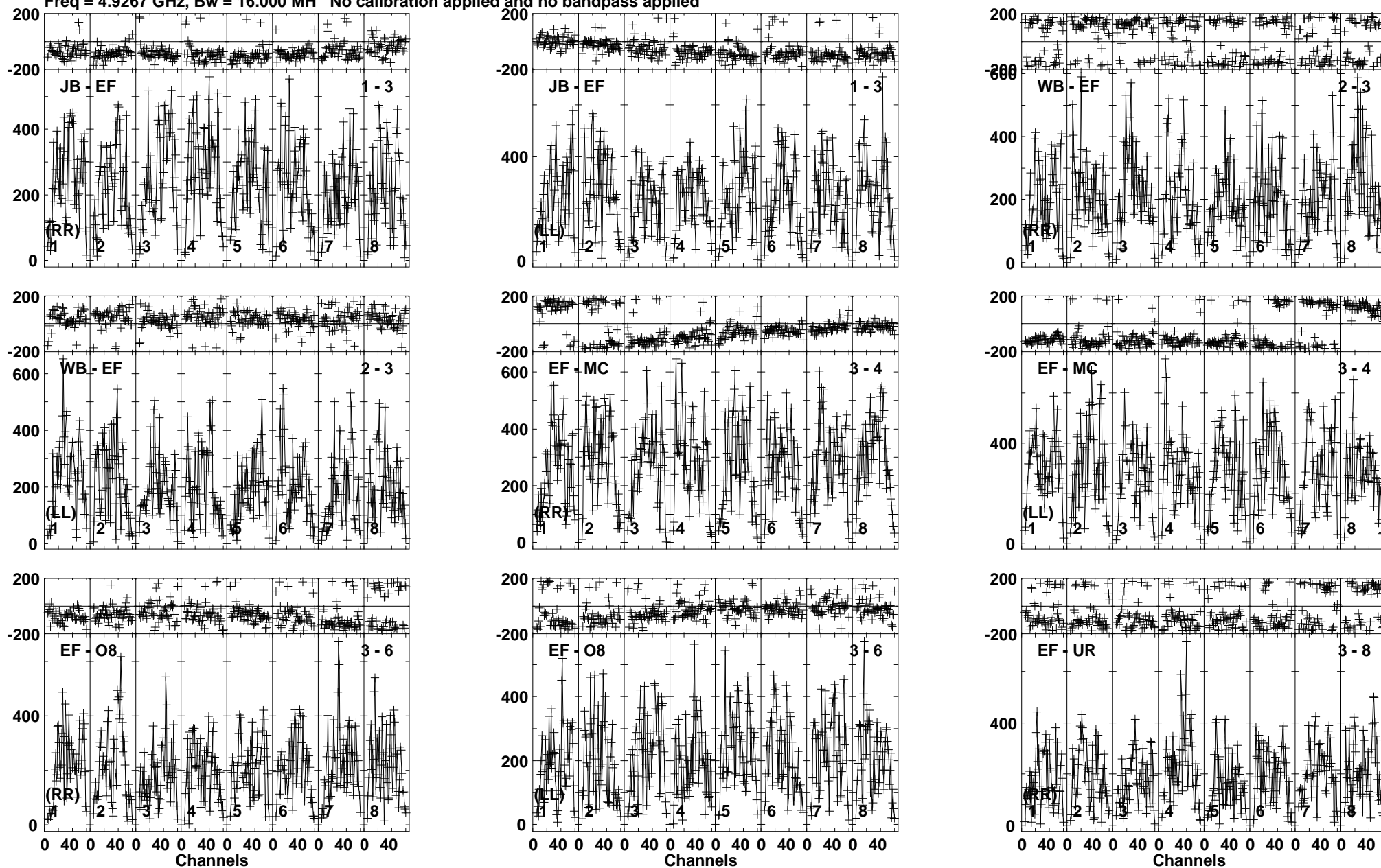
Lower frame: Micro Ampl Jy Top frame: Phas deg Vector averaged cross-power spectrum Baseline: JB (01) - EF (03) Timerange: 00/11:35:01 to 00/11:36:59
