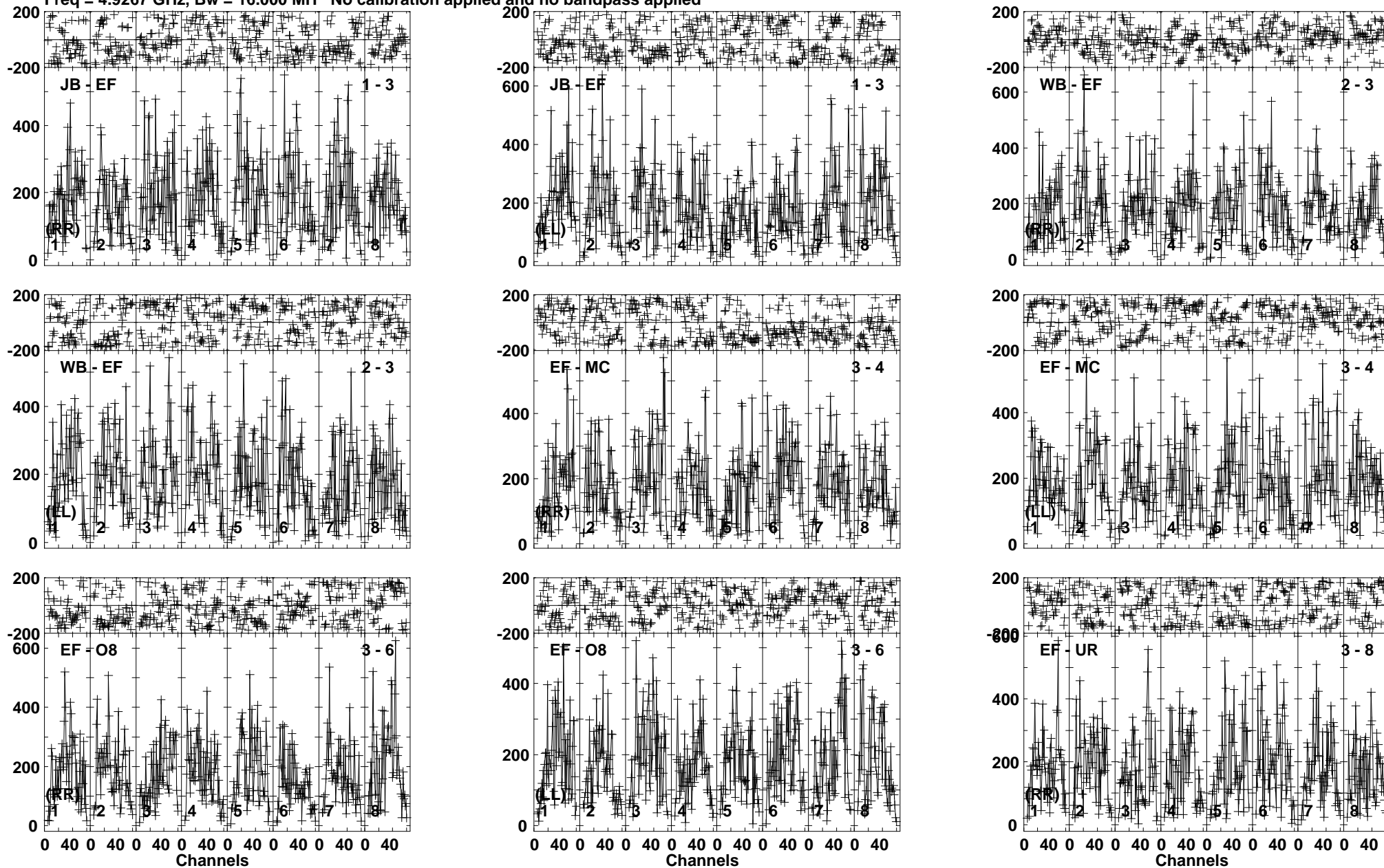
Lower frame: Micro Ampl Jy Top frame: Phas deg Vector averaged cross-power spectrum Baseline: JB (01) - EF (03) Timerange: 00/15:10:01 to 00/15:11:59
