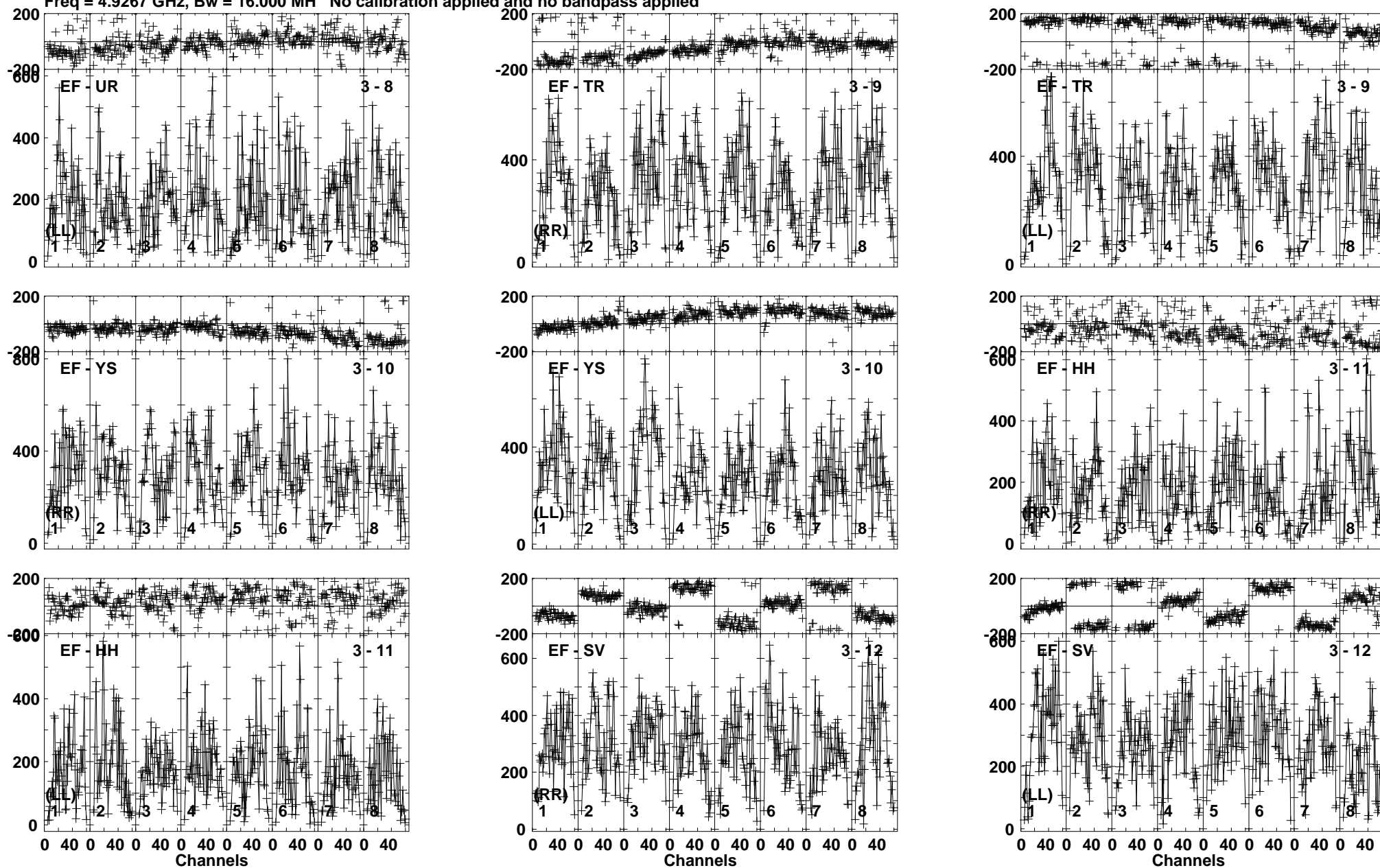
Lower frame: Micro Ampl Jy Top frame: Phas deg Vector averaged cross-power spectrum Baseline: EF (03) - UR (08) Timerange: 00/11:55:01 to 00/11:56:59
