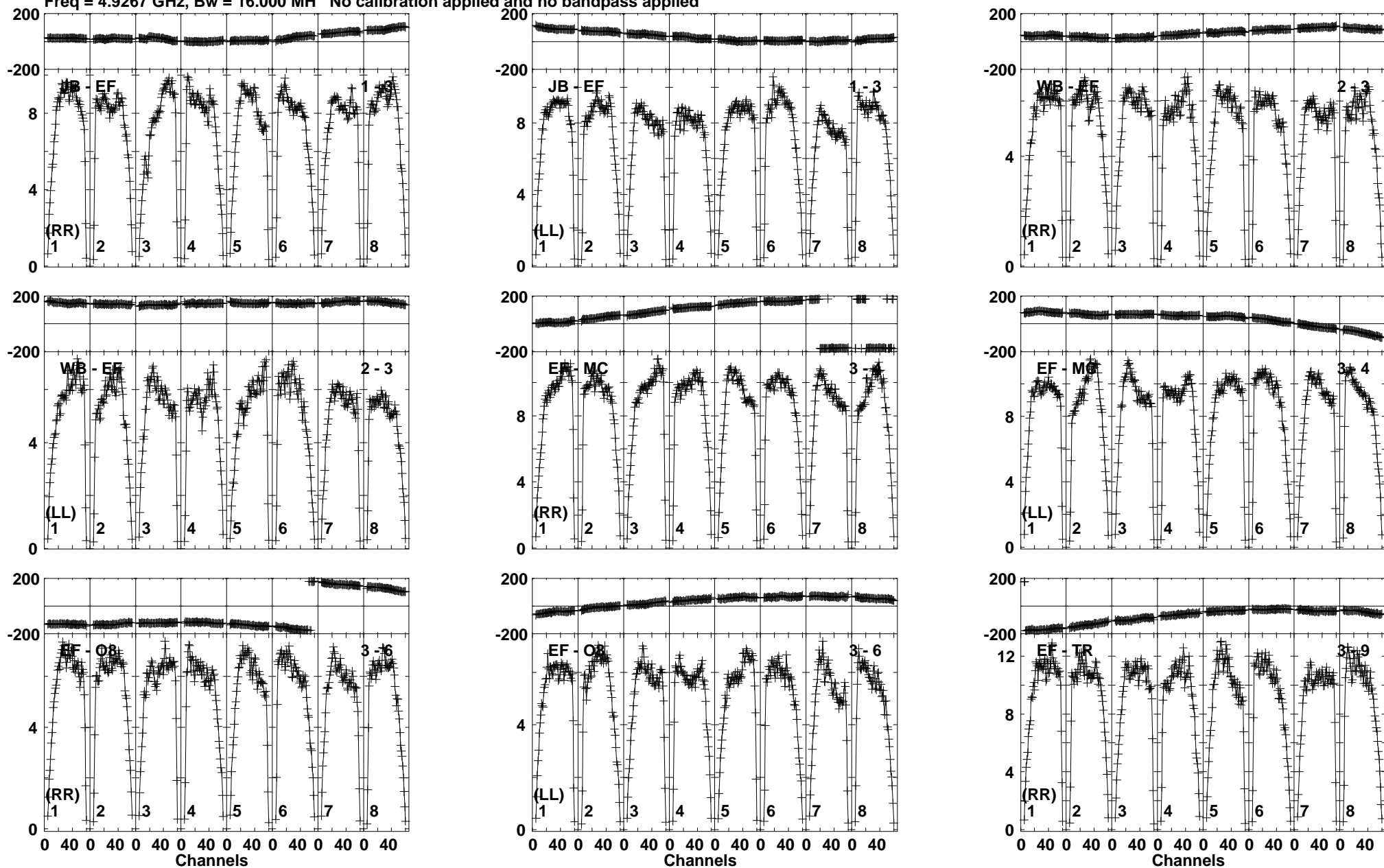
Lower frame: Milli Ampl Jy Top frame: Phas deg Vector averaged cross-power spectrum Baseline: JB (01) - EF (03) Timerange: 00:17:41:31 to 00:17:42:29
