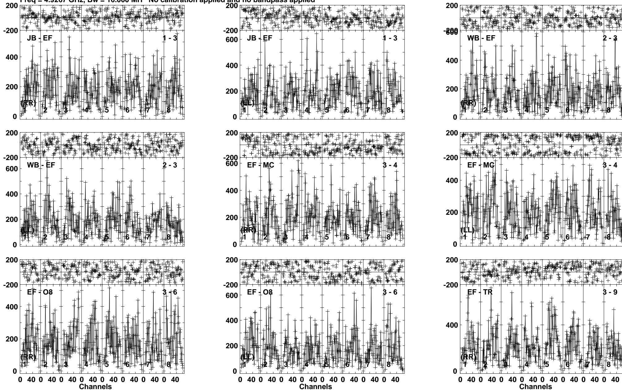
Lower frame: Micro Ampl Jy Top frame: Phas deg Vector averaged cross-power spectrum Baseline: JB (01) - EF (03) Timerange: 00/16:30:01 to 00/16:31:59
