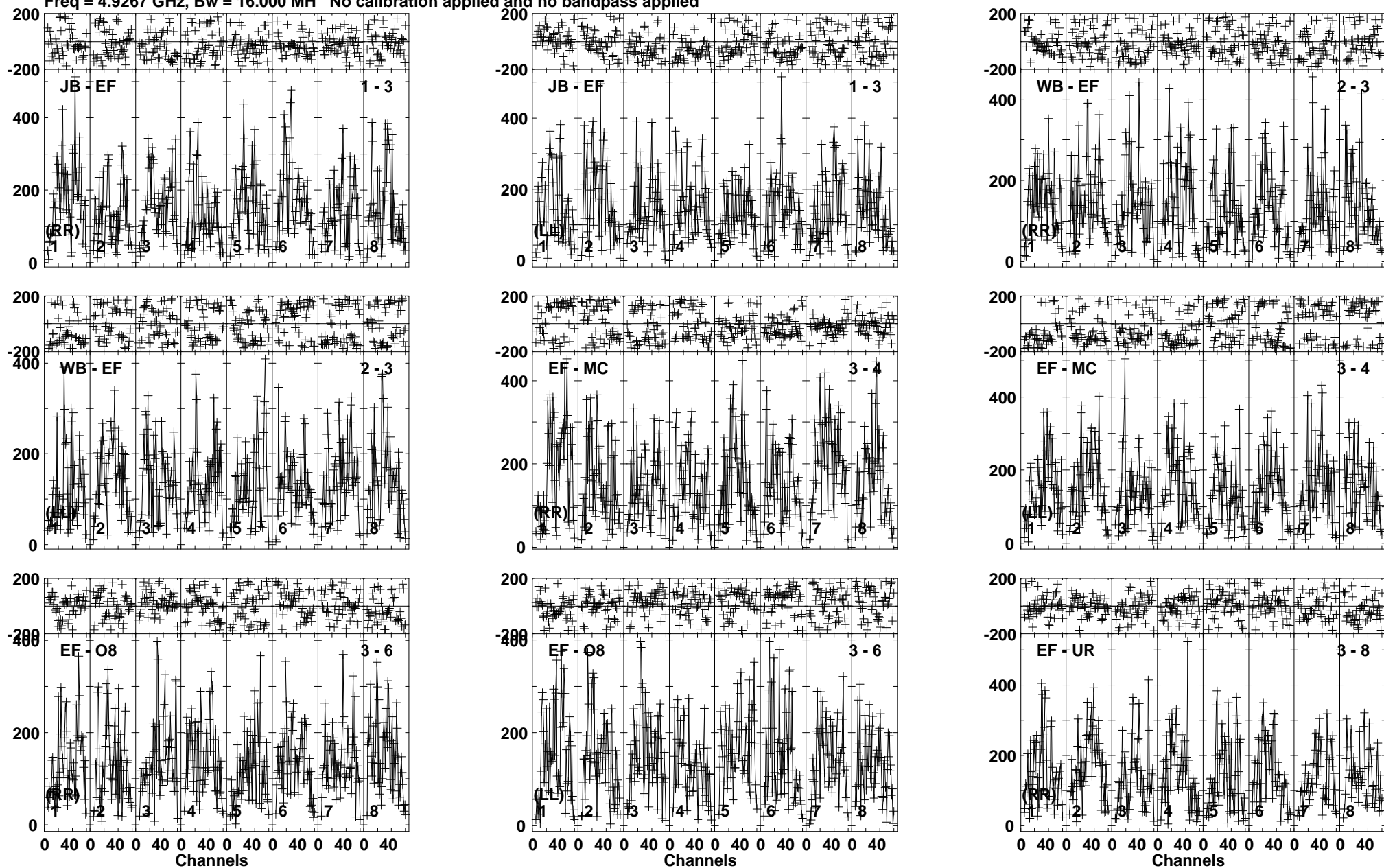
Lower frame: Micro Ampl Jy Top frame: Phas deg Vector averaged cross-power spectrum Baseline: JB (01) - EF (03) Timerange: 00/12:18:01 to 00/12:20:59
