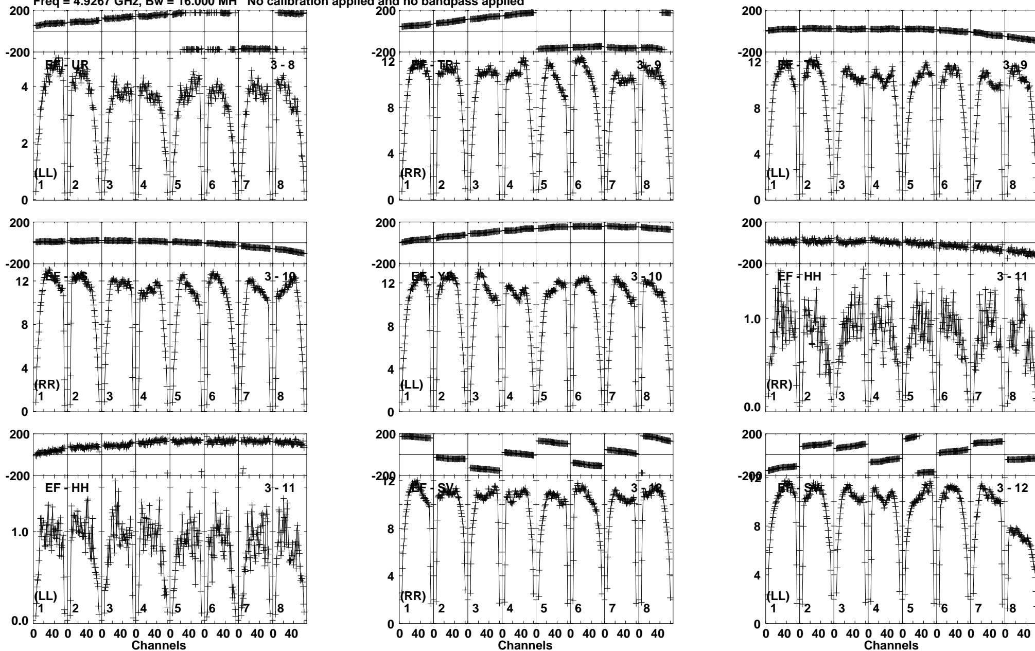
Lower frame: Milli Ampl Jy Top frame: Phas deg Vector averaged cross-power spectrum Baseline: EF (03) - UR (08) Timerange: 00/11:25:31 to 00/11:26:29
