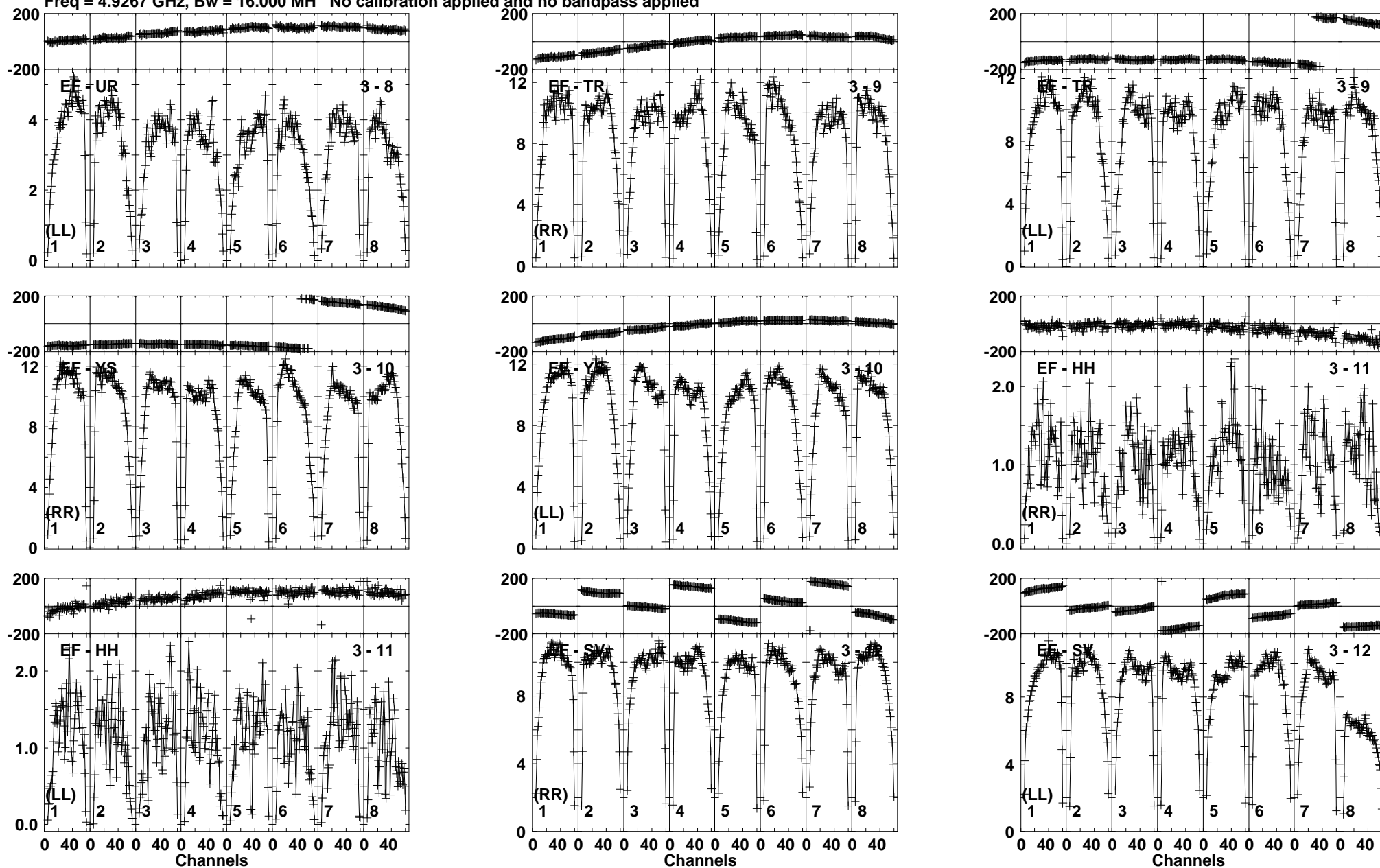
Lower frame: Milli Ampl Jy Top frame: Phas deg Vector averaged cross-power spectrum Baseline: EF (03) - UR (08) Timerange: 00/09:29:31 to 00/09:30:29
