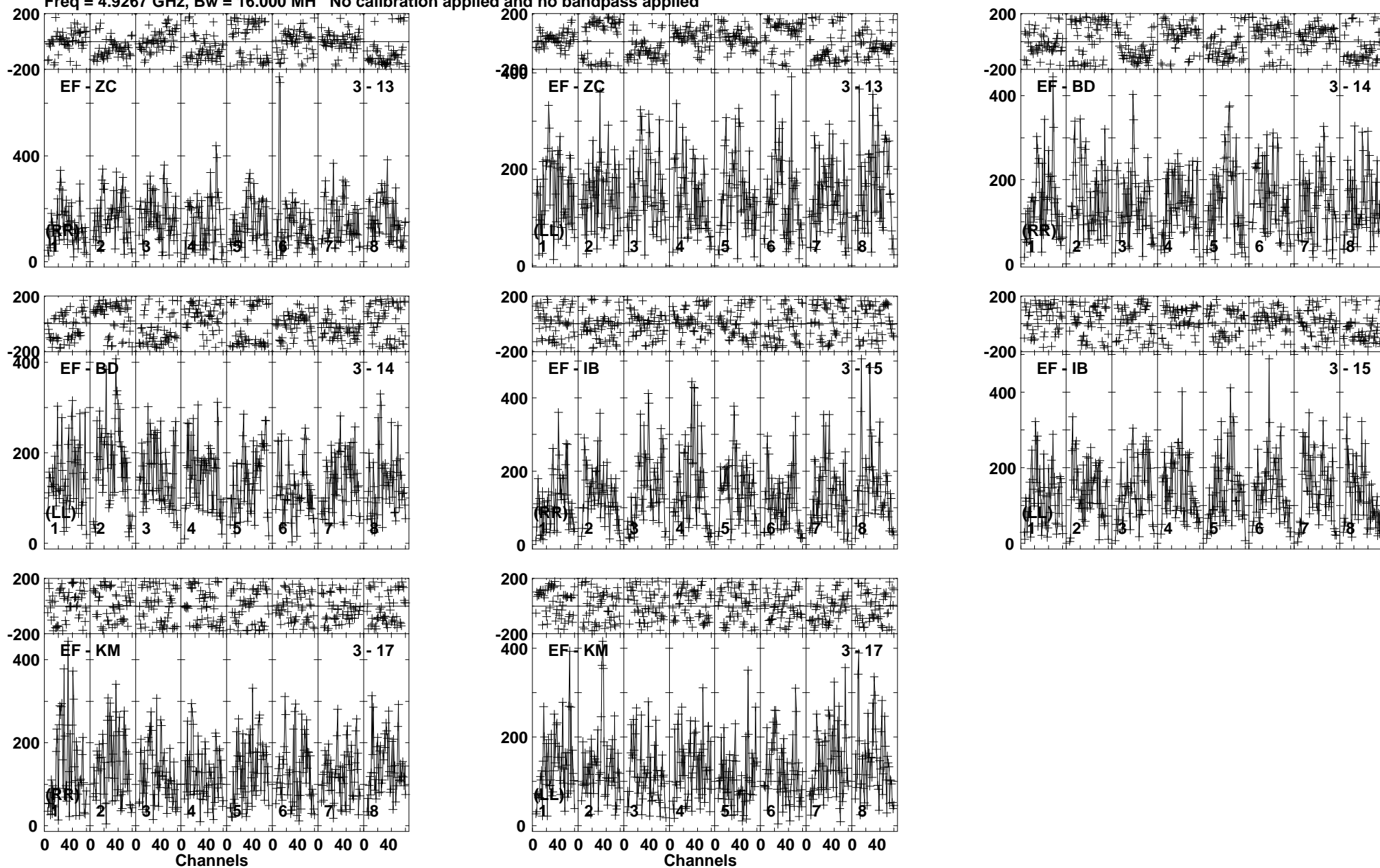
Lower frame: Micro Ampl Jy Top frame: Phas deg Vector averaged cross-power spectrum Baseline: EF (03) - ZC (13) Timerange: 00/11:26:31 to 00/11:29:29
