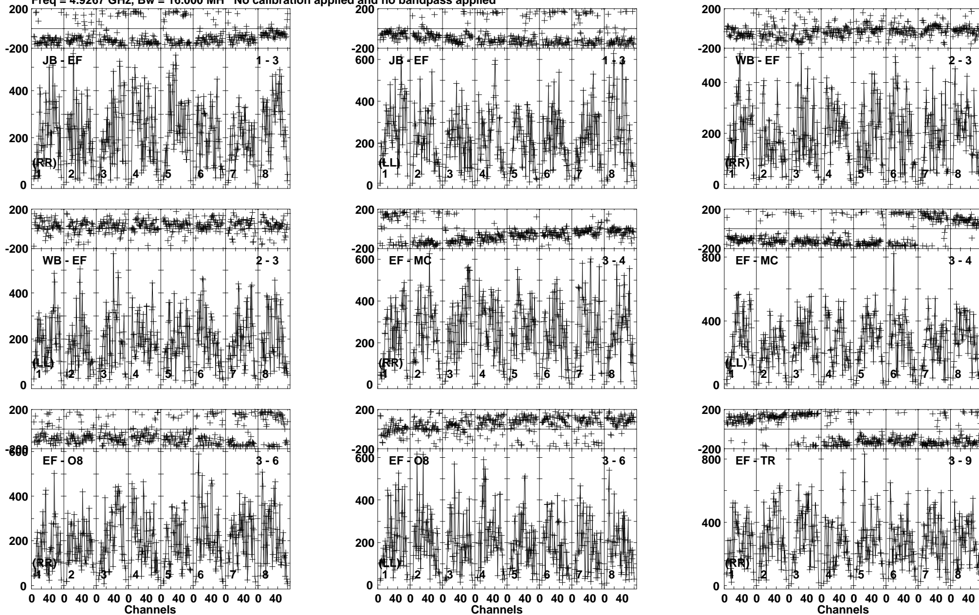
Lower frame: Micro Ampl Jy Top frame: Phas deg Vector averaged cross-power spectrum Baseline: JB (01) - EF (03) Timerange: 00/18:23:01 to 00/18:24:59
