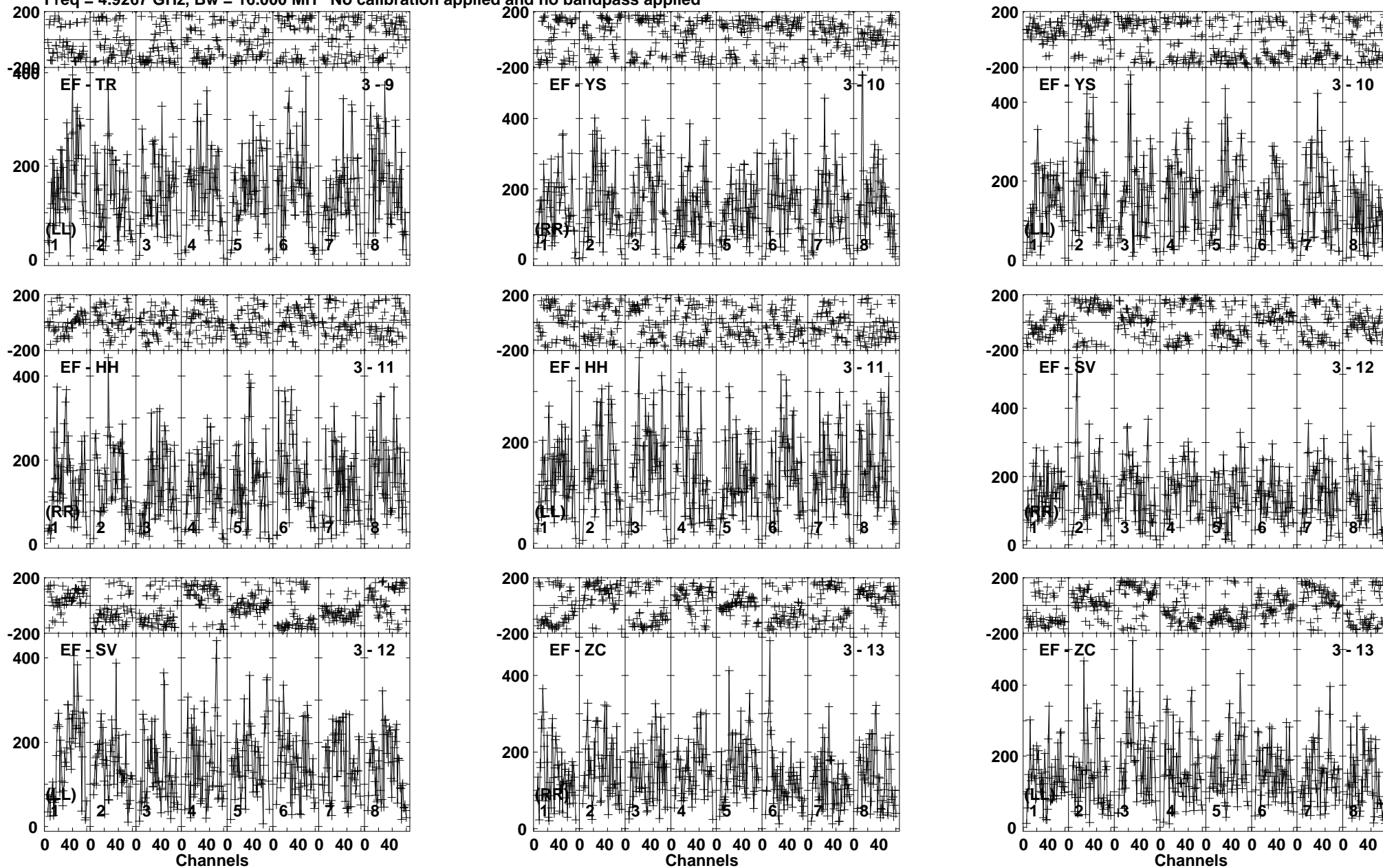
Lower frame: Micro Ampl Jy Top frame: Phas deg Vector averaged cross-power spectrum Baseline: EF (03) - TR (09) Timerange: 00/15:58:31 to 00/16:01:29
