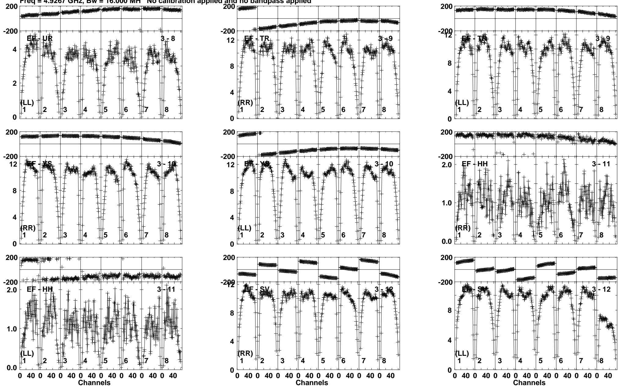
Lower frame: Milli Ampl Jy Top frame: Phas deg Vector averaged cross-power spectrum Baseline: EF (03) - UR (08) Timerange: 00/10:17:01 to 00/10:17:59
