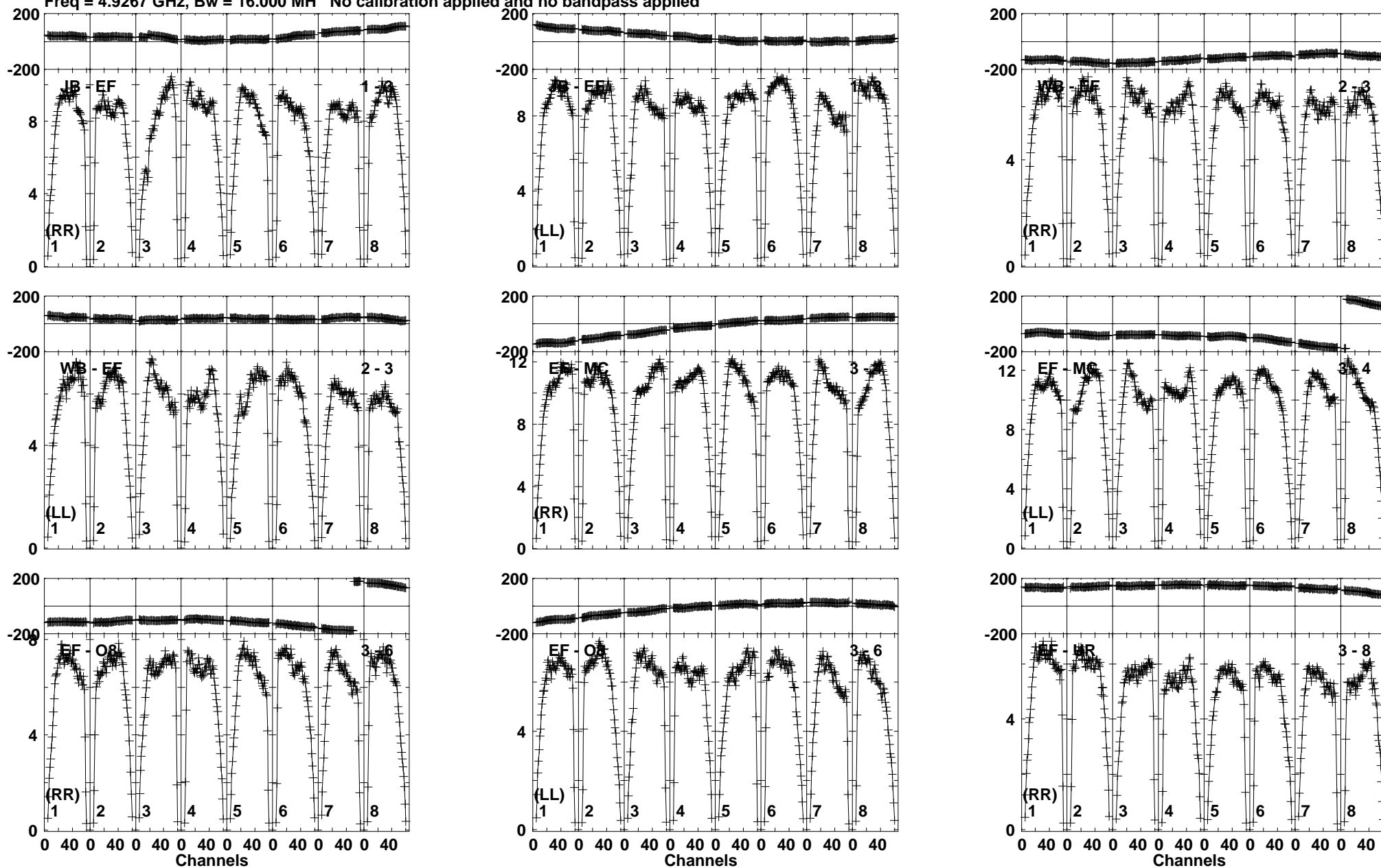
Lower frame: Milli Ampl Jy Top frame: Phas deg Vector averaged cross-power spectrum Baseline: JB (01) - EF (03) Timerange: 00/14:13:31 to 00/14:14:29
