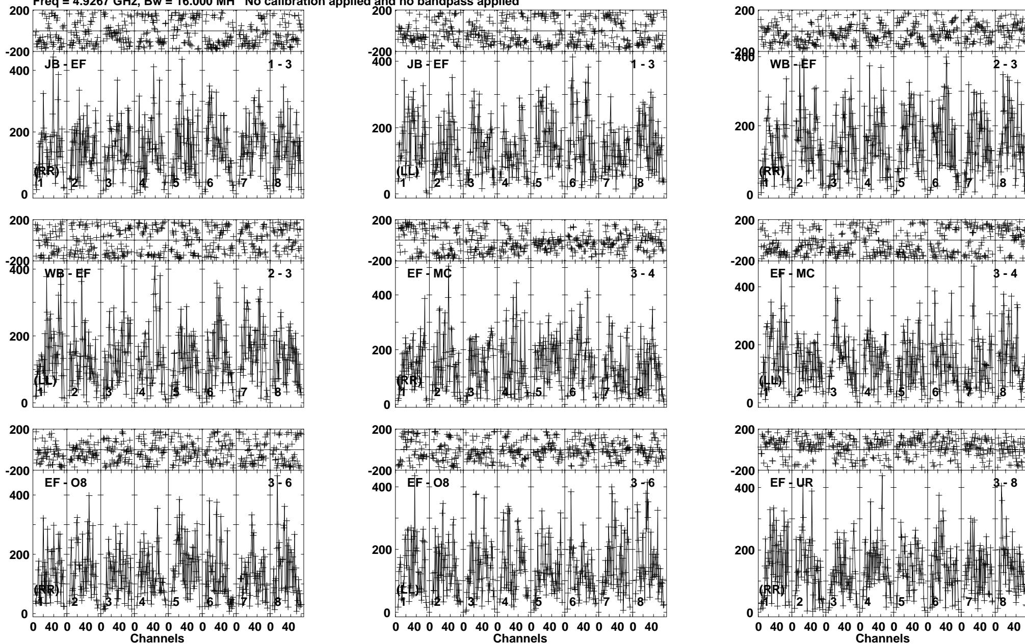
Lower frame: Micro Ampl Jy Top frame: Phas deg Vector averaged cross-power spectrum Baseline: JB (01) - EF (03) Timerange: 00/11:06:31 to 00/11:09:29
