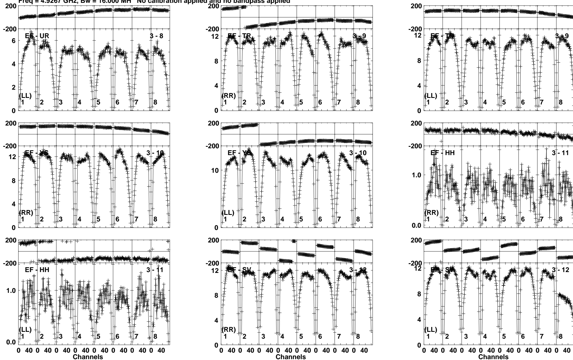
Lower frame: Milli Ampl Jy Top frame: Phas deg Vector averaged cross-power spectrum Baseline: EF (03) - UR (08) Timerange: 00:13:33:31 to 00:13:34:29
