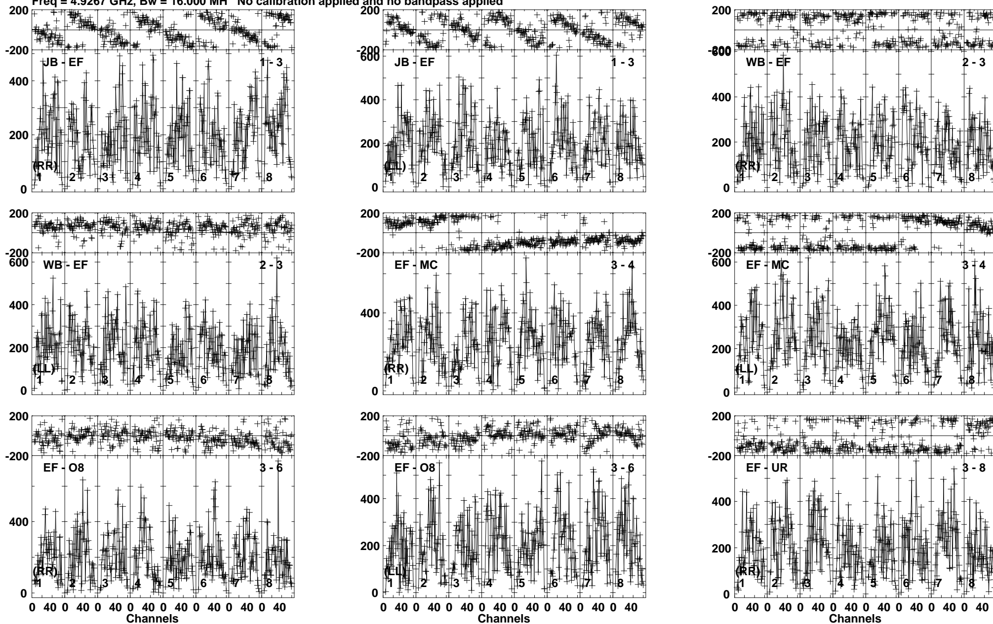
Lower frame: Micro Ampl Jy Top frame: Phas deg Vector averaged cross-power spectrum Baseline: JB (01) - EF (03) Timerange: 00/08:55:01 to 00/08:56:59
