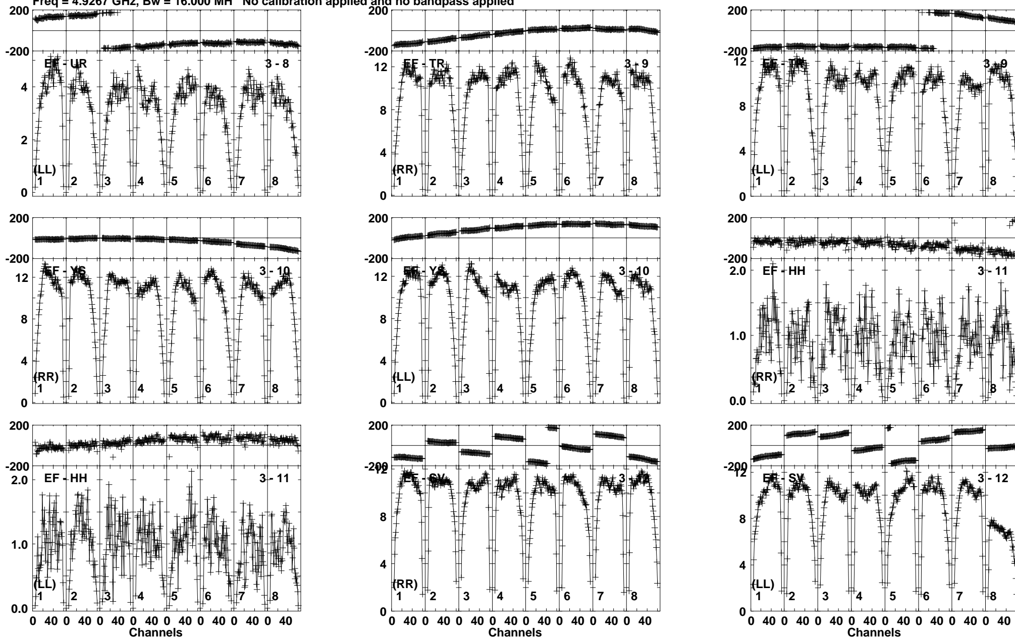
Lower frame: Milli Ampl Jy Top frame: Phas deg Vector averaged cross-power spectrum Baseline: EF (03) - UR (08) Timerange: 00/11:01:01 to 00/11:01:59
