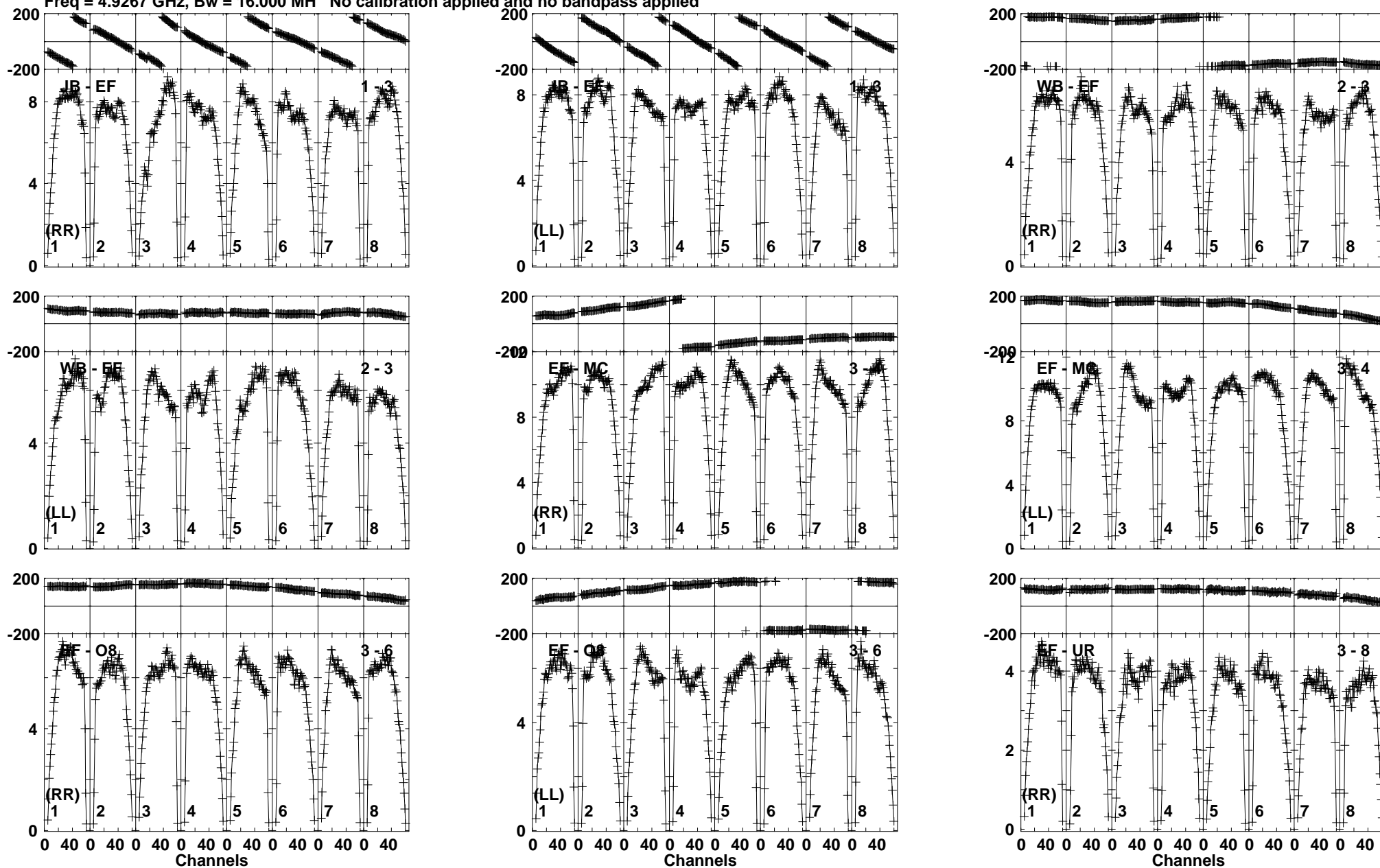
Lower frame: Milli Ampl Jy Top frame: Phas deg Vector averaged cross-power spectrum Baseline: JB (01) - EF (03) Timerange: 00/10:05:31 to 00/10:06:29
