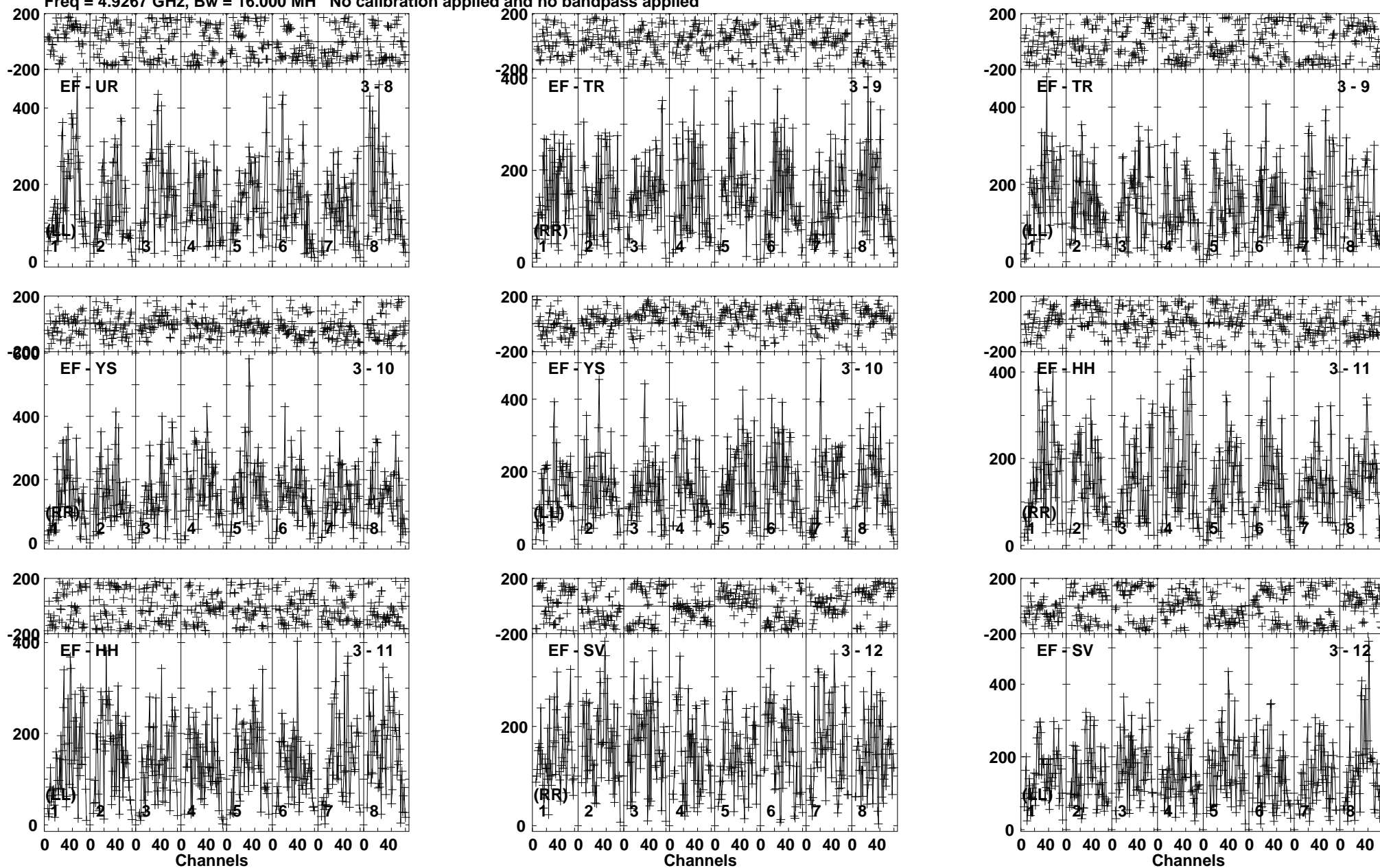
Lower frame: Micro Ampl Jy Top frame: Phas deg Vector averaged cross-power spectrum Baseline: EF (03) - UR (08) Timerange: 00/13:58:31 to 00/14:01:29
