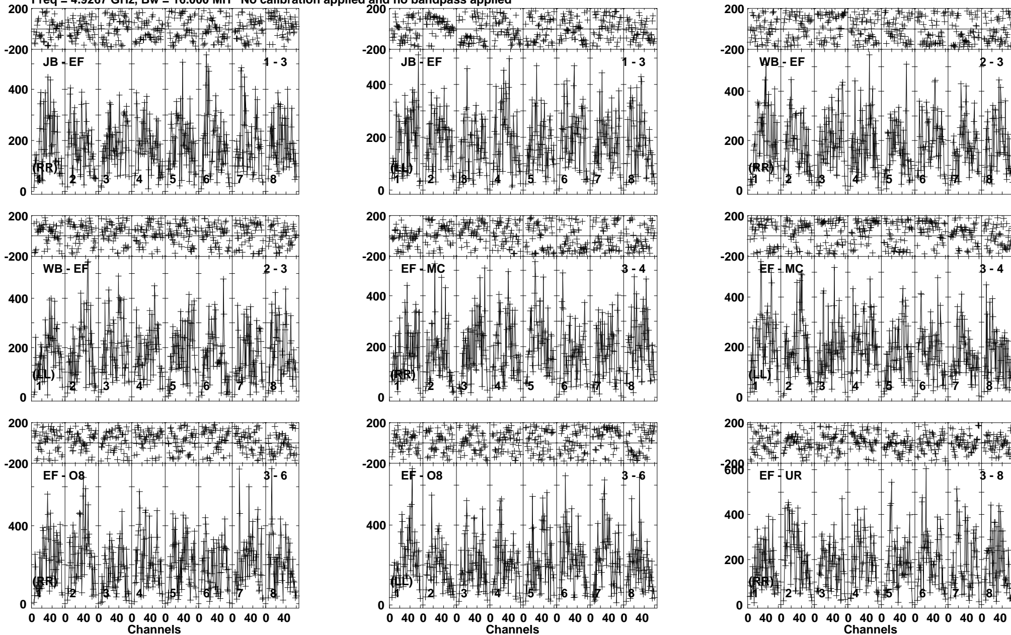
Lower frame: Micro Ampl Jy Top frame: Phas deg Vector averaged cross-power spectrum Baseline: JB (01) - EF (03) Timerange: 00/10:22:01 to 00/10:23:59
