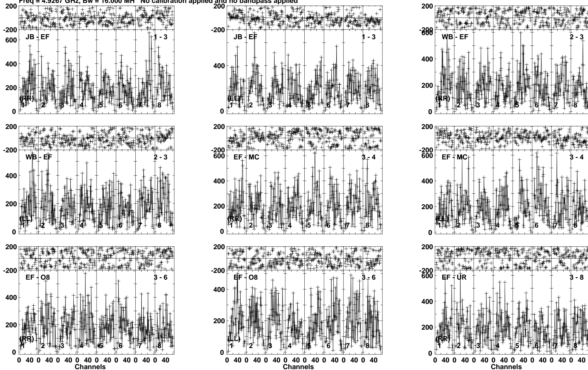
Lower frame: Micro Ampl Jy Top frame: Phas deg Vector averaged cross-power spectrum Baseline: JB (01) - EF (03) Timerange: 00/13:50:01 to 00/13:51:59
