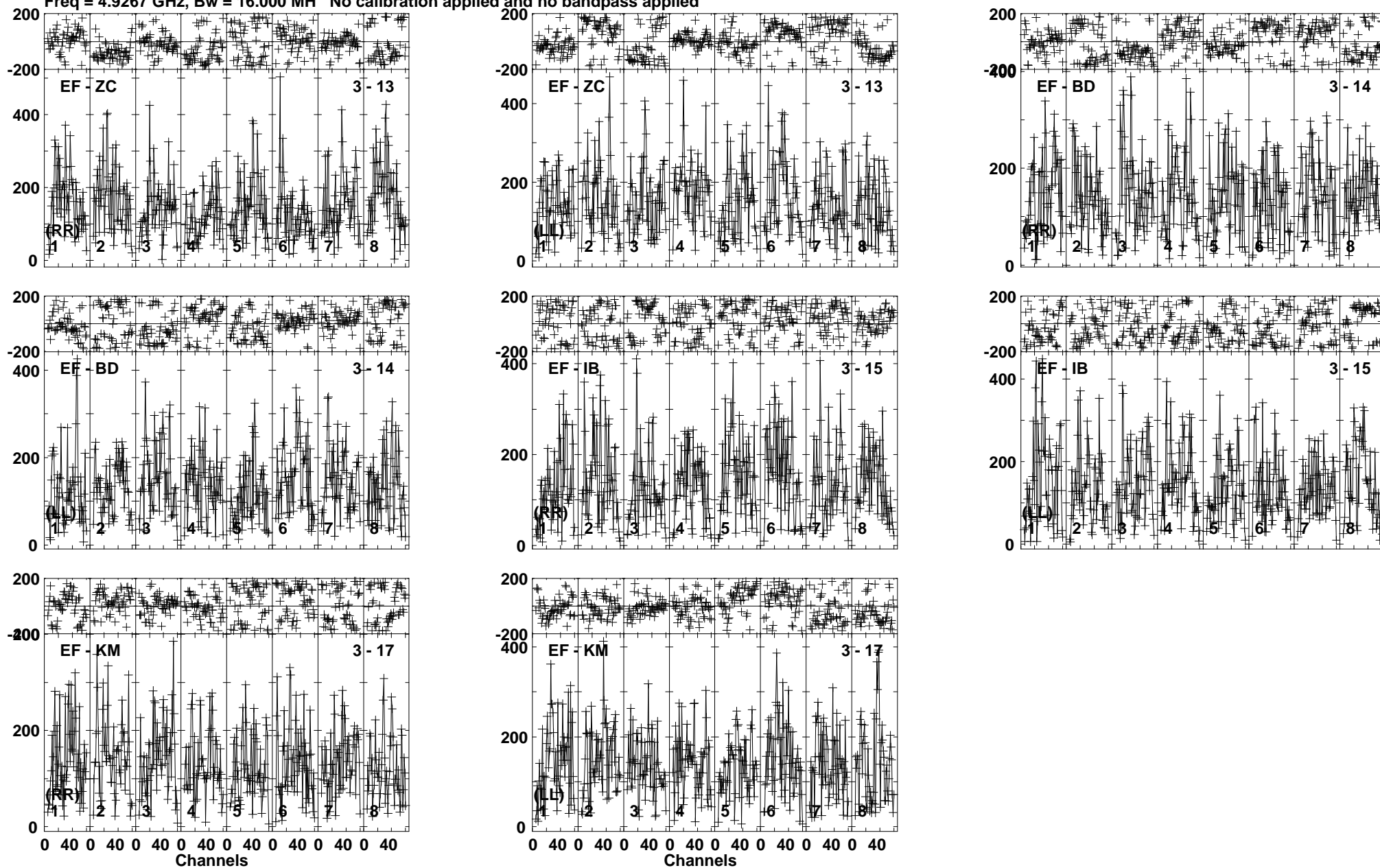
Lower frame: Micro Ampl Jy Top frame: Phas deg Vector averaged cross-power spectrum Baseline: EF (03) - ZC (13) Timerange: 00:12:10:31 to 00:12:13:29
