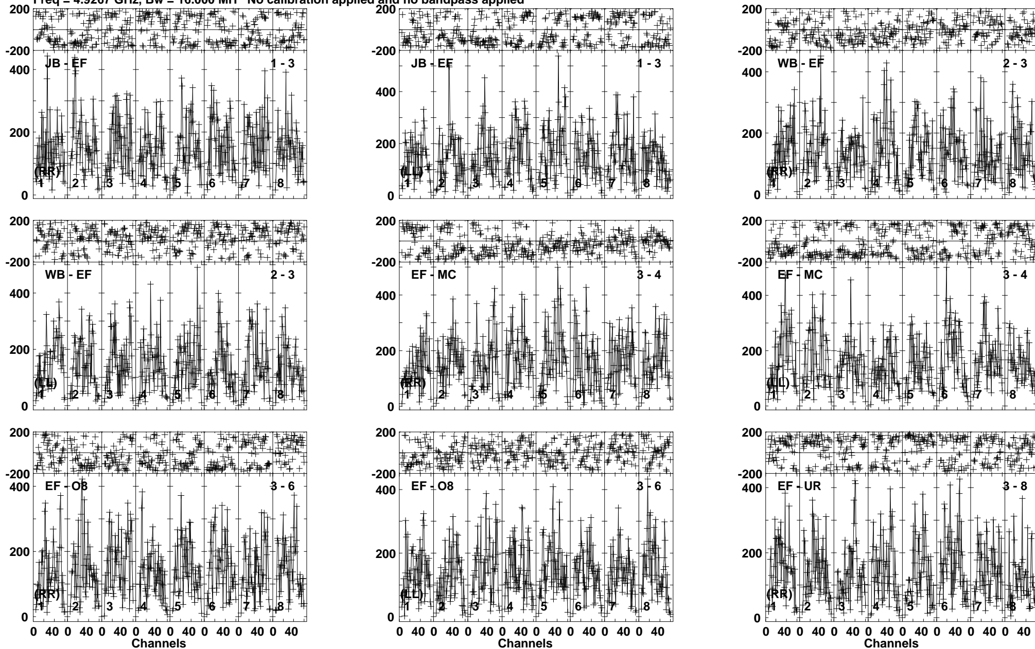
Lower frame: Micro Ampl Jy Top frame: Phas deg Vector averaged cross-power spectrum Baseline: JB (01) - EF (03) Timerange: 00/14:58:31 to 00/15:01:29
