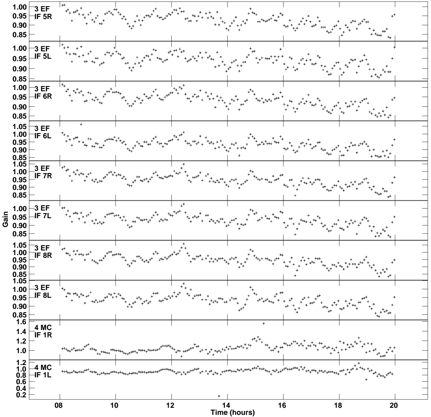
Plot file version 5 created 19-DEC-2018 18:27:39 Gain amp vs UTC time for J1619+2247.MULTI.1 SN 2 Rpol & Lpol IF 1 - 8
