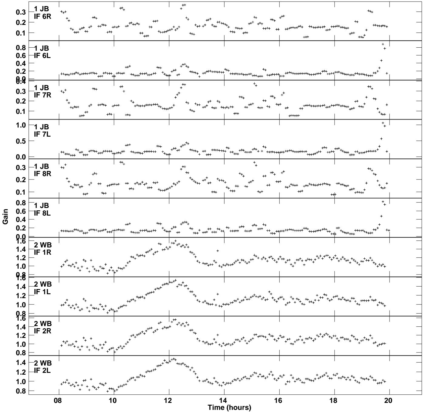
Plot file version 2 created 19-DEC-2018 18:27:39 Gain amp vs UTC time for J1619+2247.MULTI.1 SN 2 Rpol & Lpol IF 1 - 8
