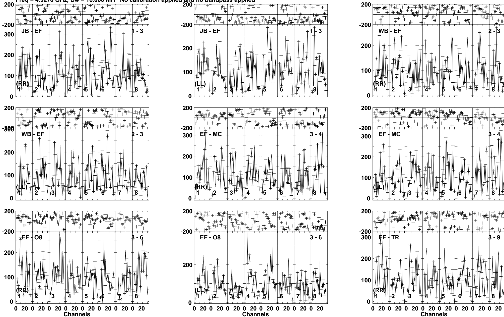
Lower frame: Micro Ampl Jy Top frame: Phas deg Vector averaged cross-power spectrum Baseline: JB (01) - EF (03) Timerange: 00/18:46:01 to 00/18:48:59
