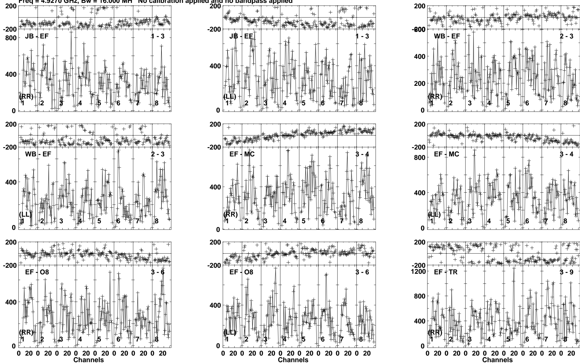
Lower frame: Micro Ampl Jy Top frame: Phas deg Vector averaged cross-power spectrum Baseline: JB (01) - EF (03) Timerange: 00/10/04:01 to 00/10/04:59
