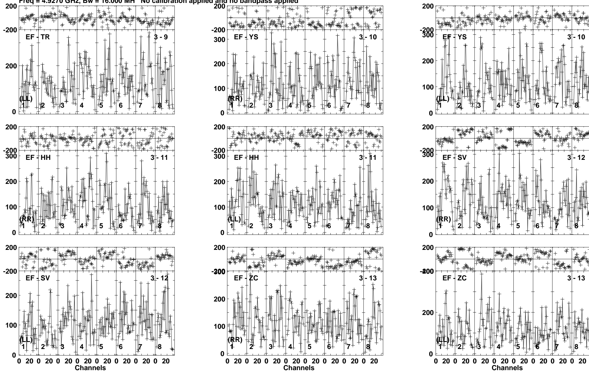
Lower frame: Micro Ampl Jy Top frame: Phas deg Vector averaged cross-power spectrum Baseline: EF (03) - TR (09) Timerange: 00/11:38:01 to 00/11:40:59
