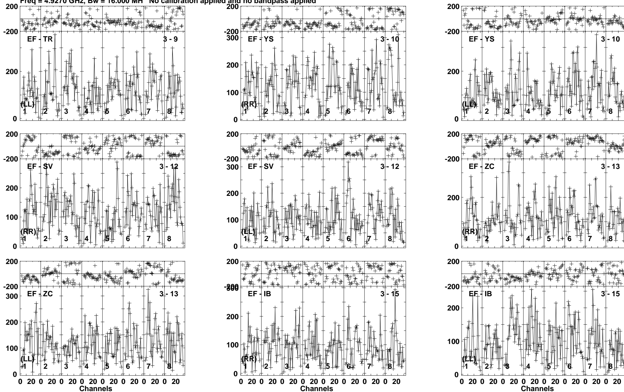
Lower frame: Micro Ampl Jy Top frame: Phas deg Vector averaged cross-power spectrum Baseline: EF (03) - TR (09) Timerange: 00/17:26:01 to 00/17:28:59
