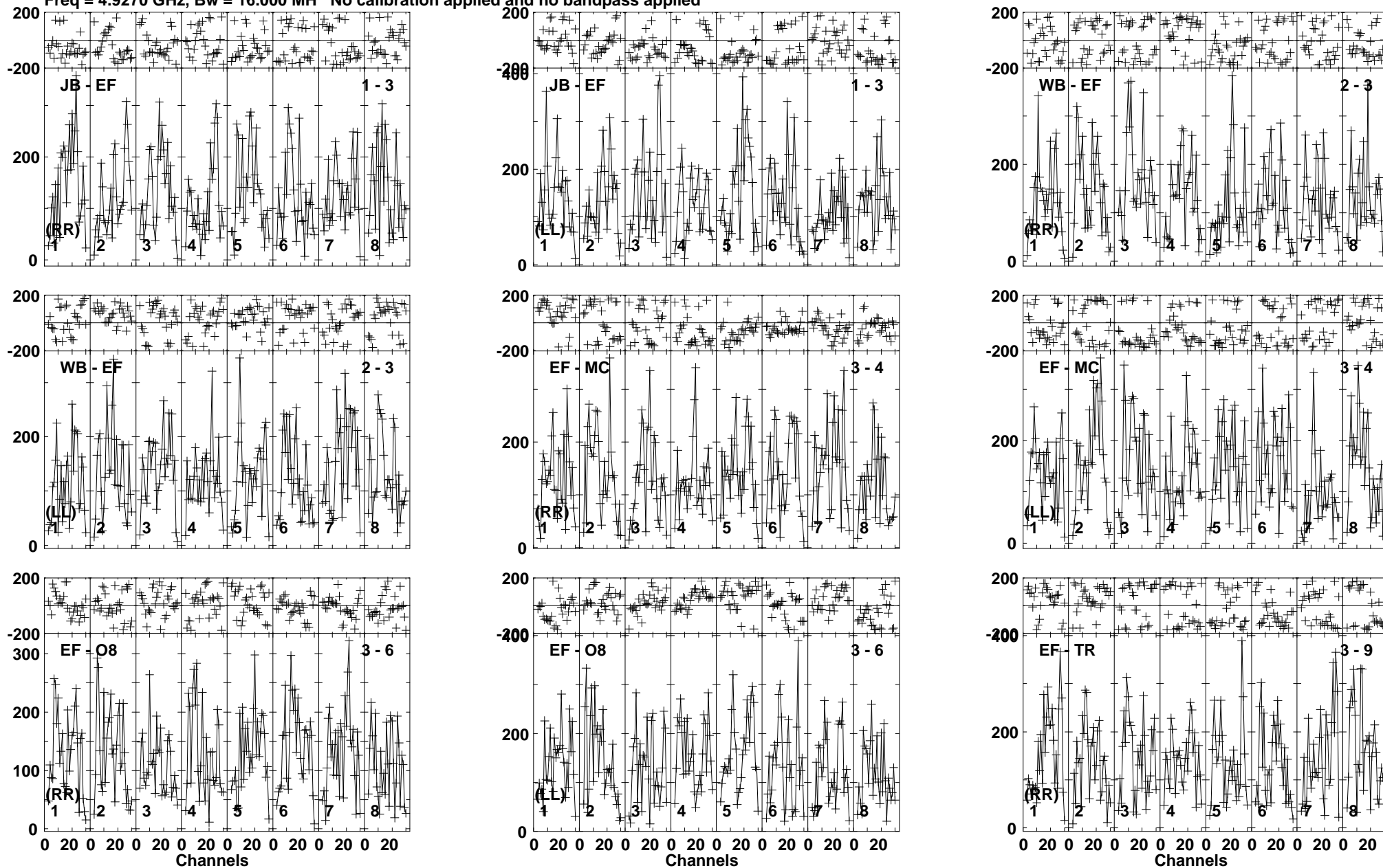
Lower frame: Micro Ampl Jy Top frame: Phas deg Vector averaged cross-power spectrum Baseline: JB (01) - EF (03) Timerange: 00/10:42:01 to 00/10:43:59
