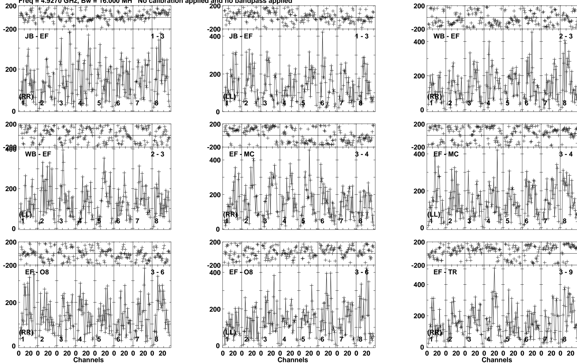
Lower frame: Micro Ampl Jy Top frame: Phas deg Vector averaged cross-power spectrum Baseline: JB (01) - EF (03) Timerange: 00/11:22:01 to 00/11:23:59
