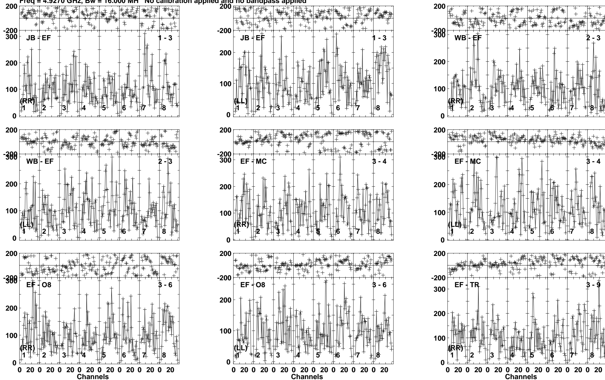
Lower frame: Micro Ampl Jy Top frame: Phas deg Vector averaged cross-power spectrum Baseline: JB (01) - EF (03) Timerange: 00/19:06:01 to 00/19:08:59
