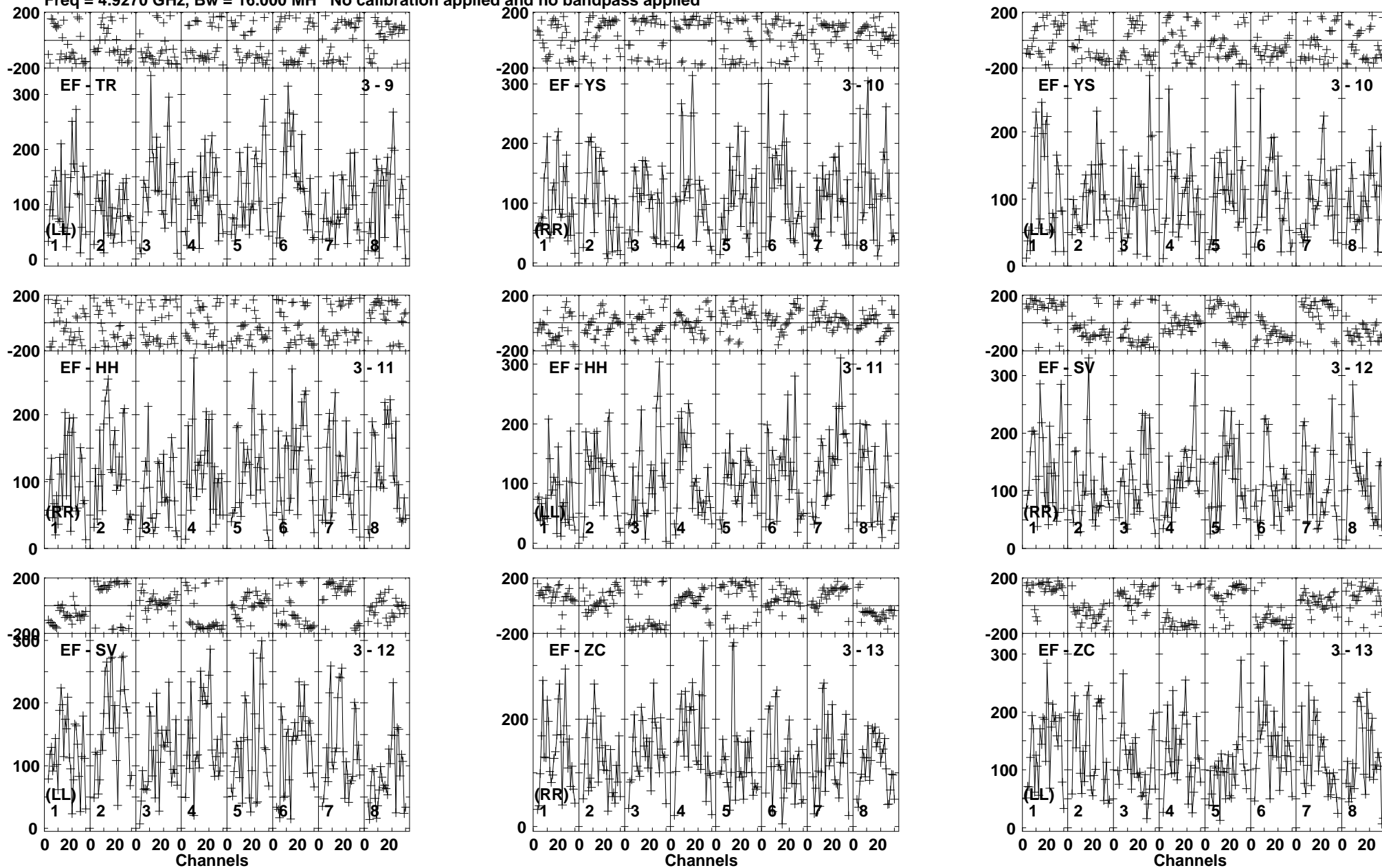
Lower frame: Micro Ampl Jy Top frame: Phas deg Vector averaged cross-power spectrum Baseline: EF (03) - TR (09) Timerange: 00/13:14:31 to 00/13:17:29
