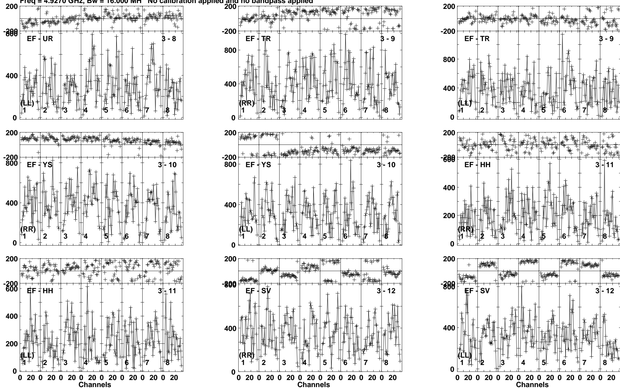
Lower frame: Micro Ampl Jy Top frame: Phas deg Vector averaged cross-power spectrum Baseline: EF (03) - UR (08) Timerange: 00/09:24:01 to 00/09:24:59
