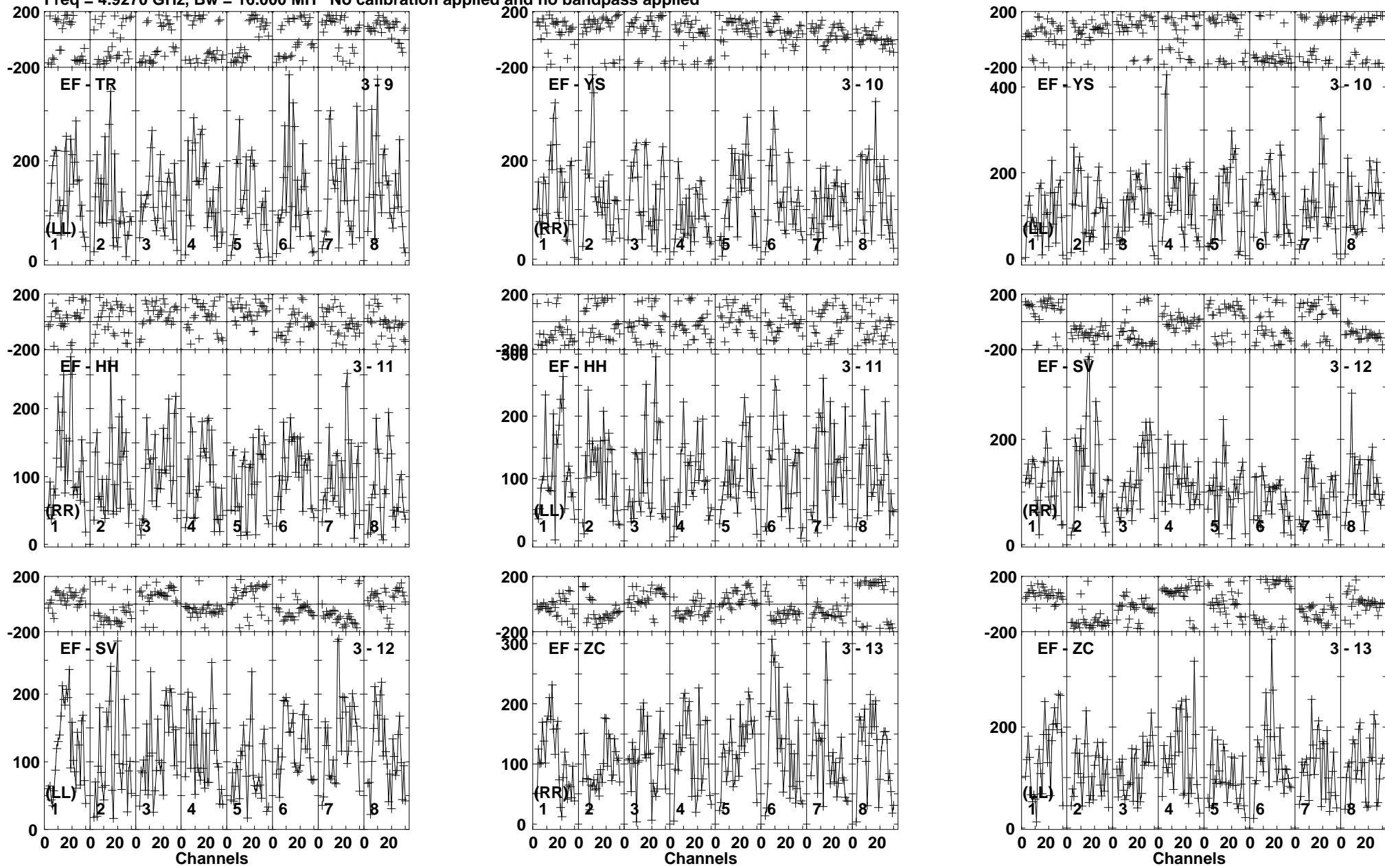
Lower frame: Micro Ampl Jy Top frame: Phas deg Vector averaged cross-power spectrum Baseline: EF (03) - TR (09) Timerange: 00/14:34:31 to 00/14:37:29
