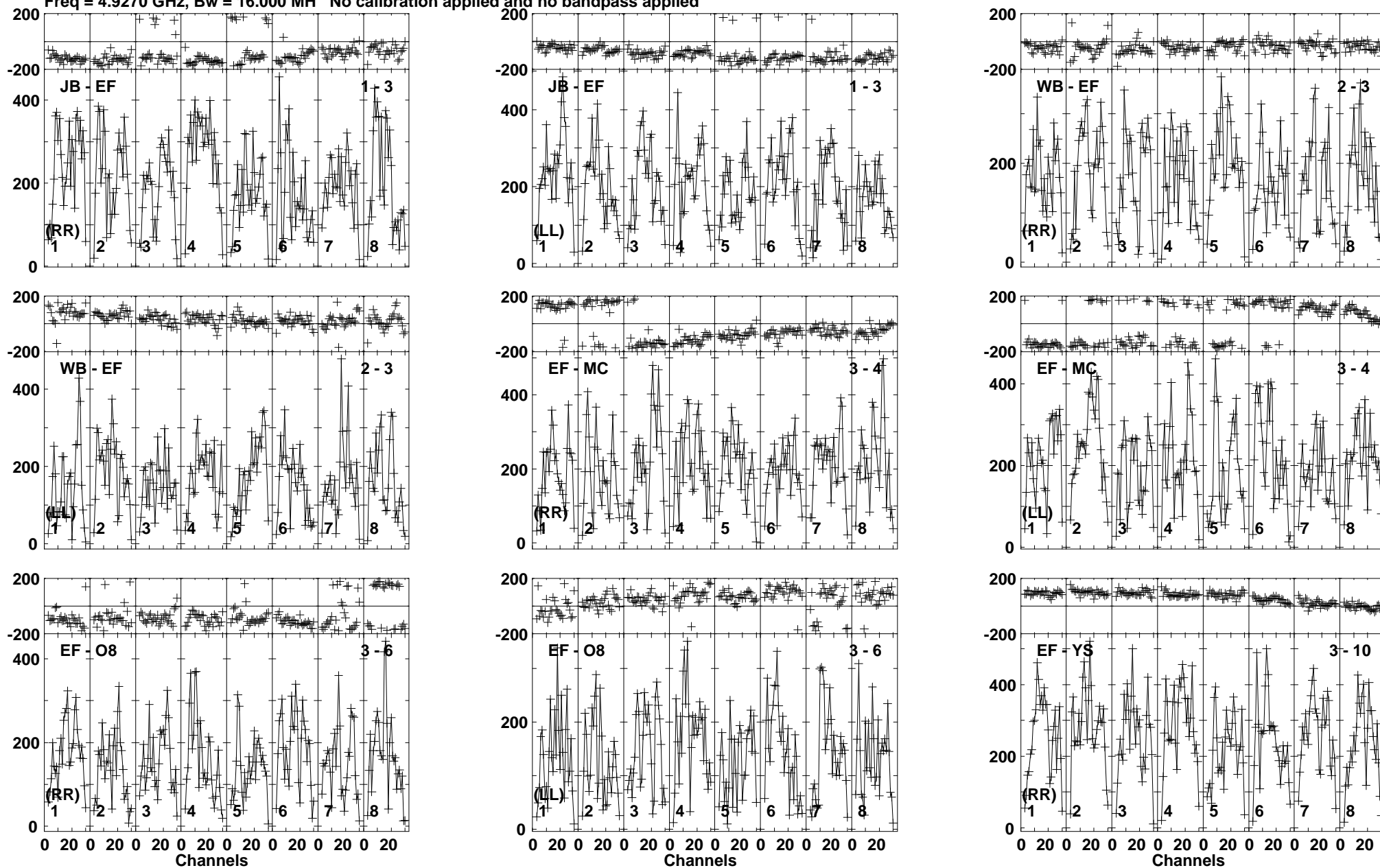
Lower frame: Micro Ampl Jy Top frame: Phas deg Vector averaged cross-power spectrum Baseline: JB (01) - EF (03) Timerange: 00/17:43:01 to 00/17:44:59
