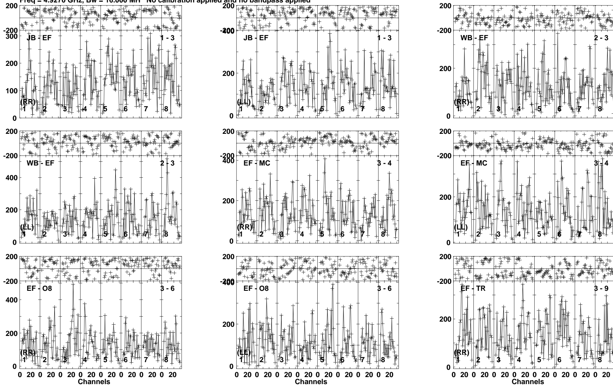
Lower frame: Micro Ampl Jy Top frame: Phas deg Vector averaged cross-power spectrum Baseline: JB (01) - EF (03) Timerange: 00/17:50:01 to 00/17:51:59
