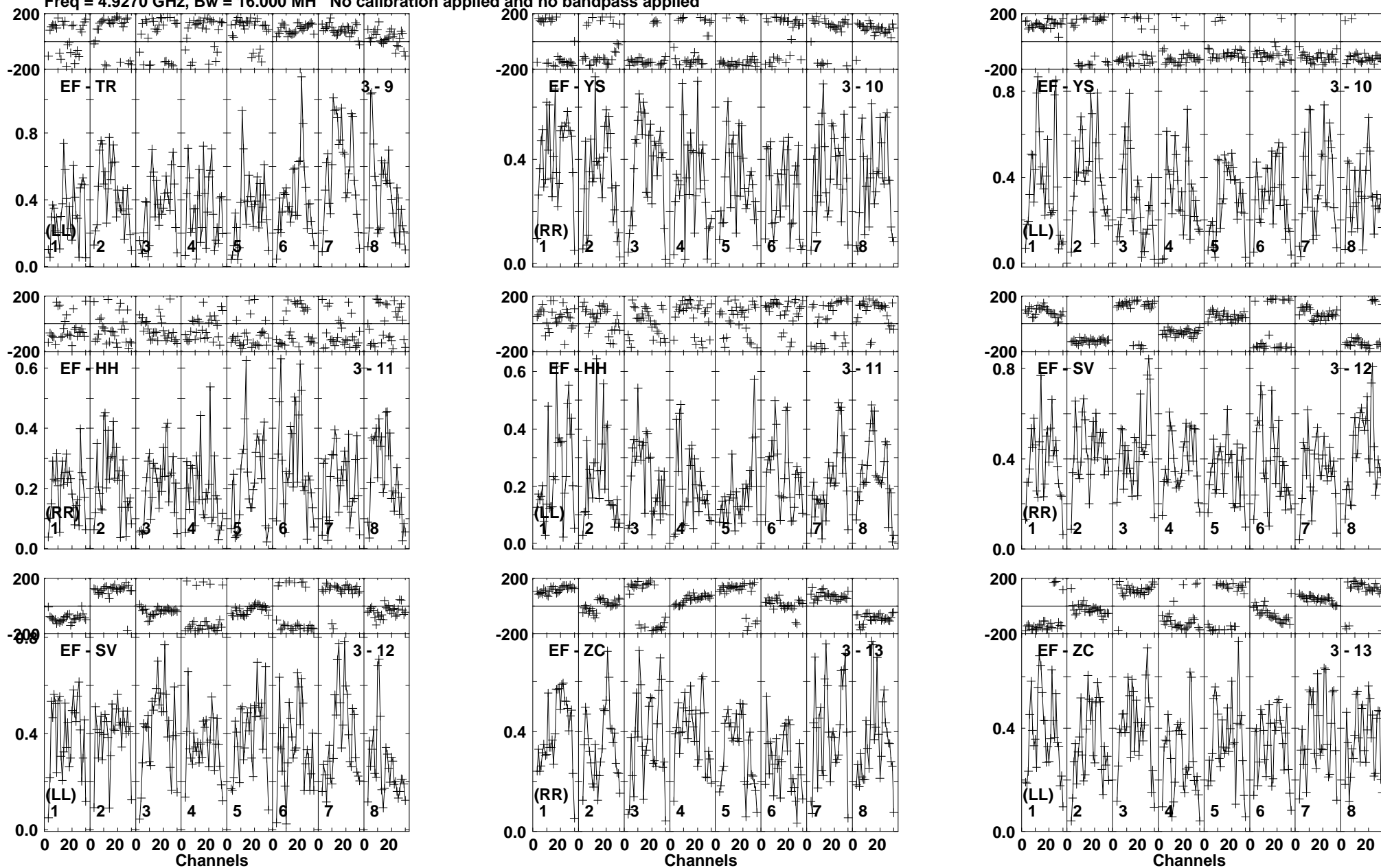
Lower frame: Milli Ampl Jy Top frame: Phas deg Vector averaged cross-power spectrum Baseline: EF (03) - TR (09) Timerange: 00/15:12:01 to 00/15:12:59
