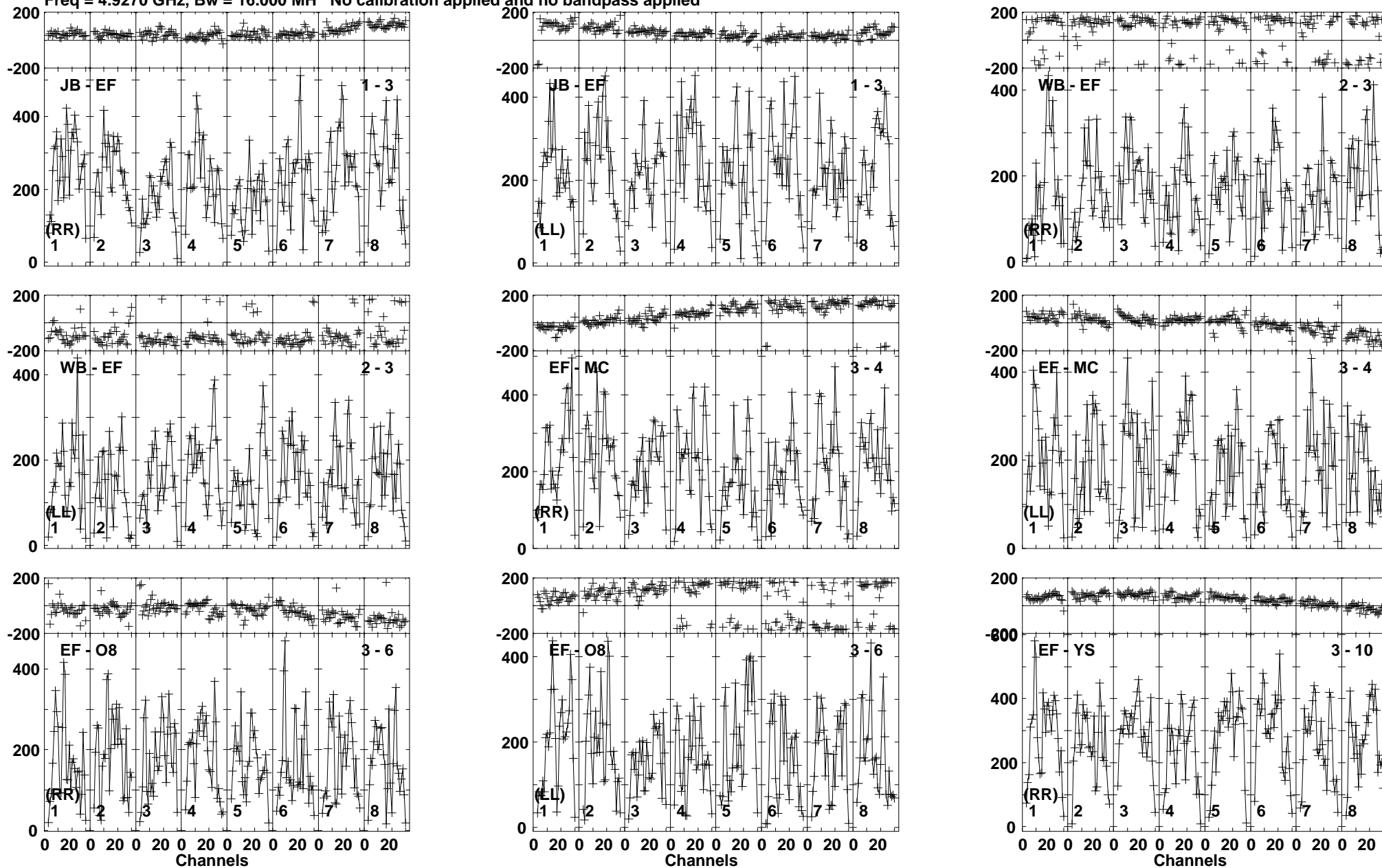
Lower frame: Micro Ampl Jy Top frame: Phas deg Vector averaged cross-power spectrum Baseline: JB (01) - EF (03) Timerange: 00/16:43:01 to 00/16:44:59
