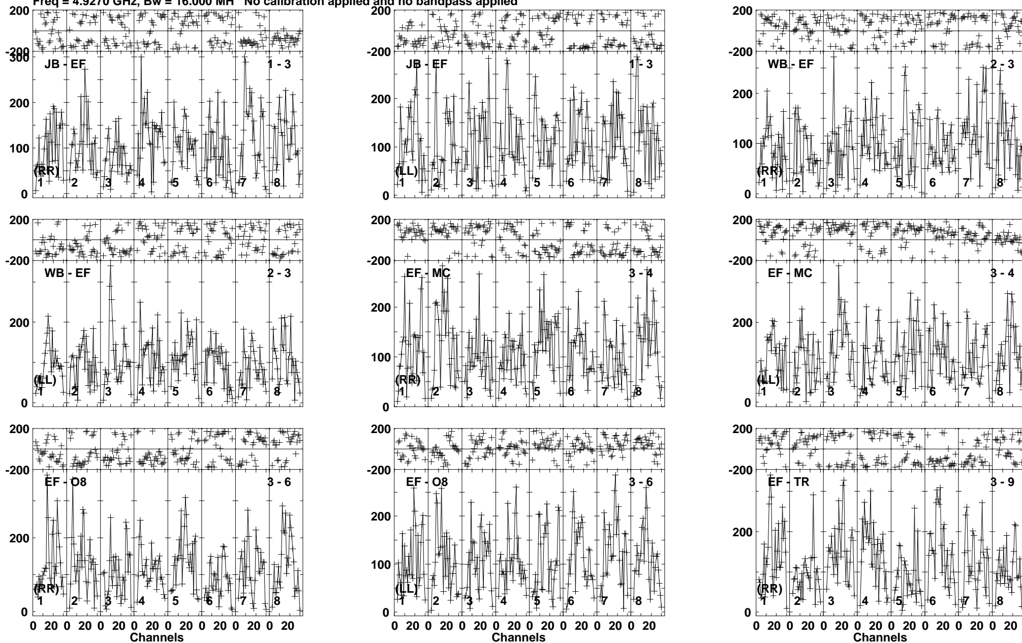
Lower frame: Micro Ampl Jy Top frame: Phas deg Vector averaged cross-power spectrum Baseline: JB (01) - EF (03) Timerange: 00/16:14:31 to 00/16:17:29
