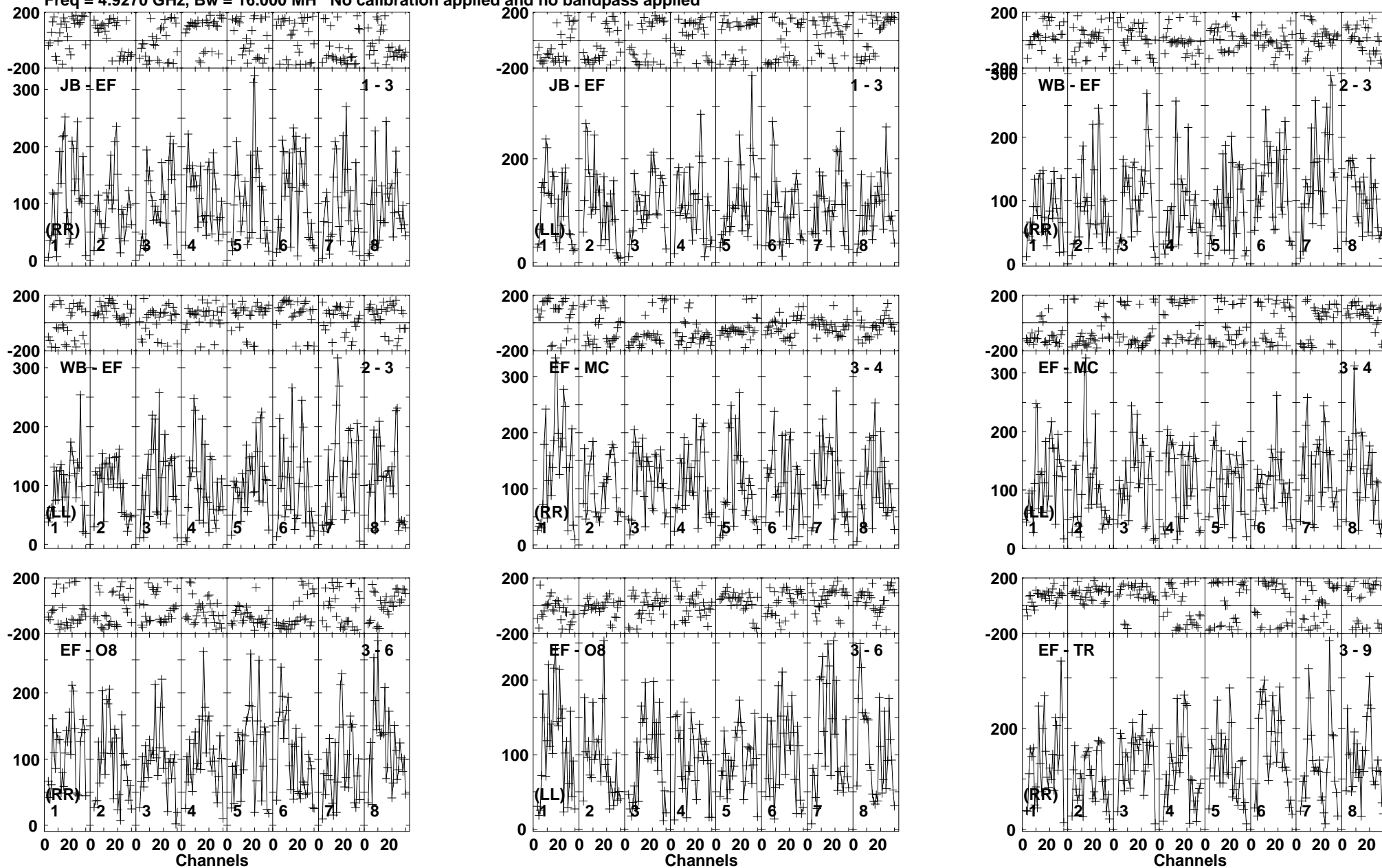
Lower frame: Micro Ampl Jy Top frame: Phas deg Vector averaged cross-power spectrum Baseline: JB (01) - EF (03) Timerange: 00/16:26:01 to 00/16:28:59
