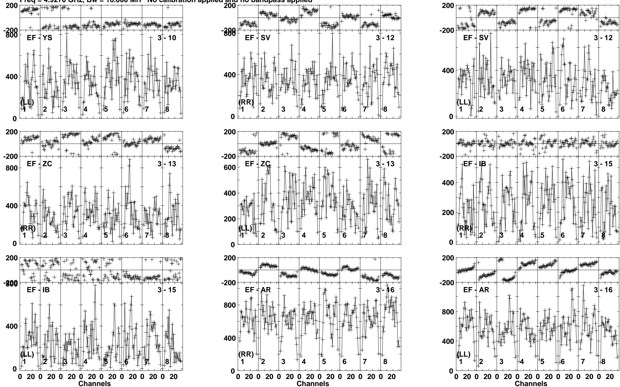
Lower frame: Micro Ampl Jy Top frame: Phas deg Vector averaged cross-power spectrum Baseline: EF (03) - YS (10) Timerange: 00/17:52:01 to 00/17:52:59
