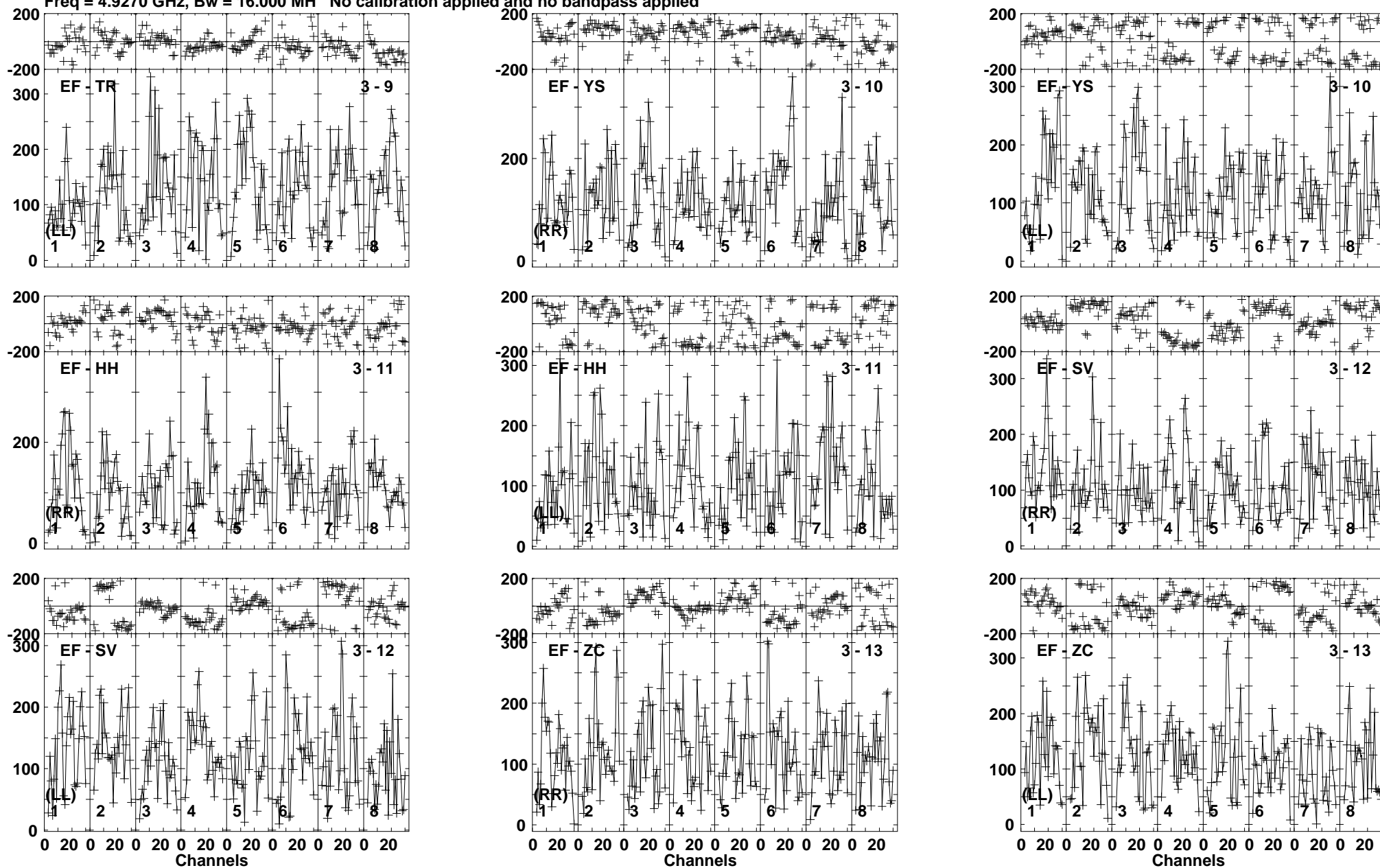
Lower frame: Micro Ampl Jy Top frame: Phas deg Vector averaged cross-power spectrum Baseline: EF (03) - TR (09) Timerange: 00/13:26:01 to 00/13:28:59
