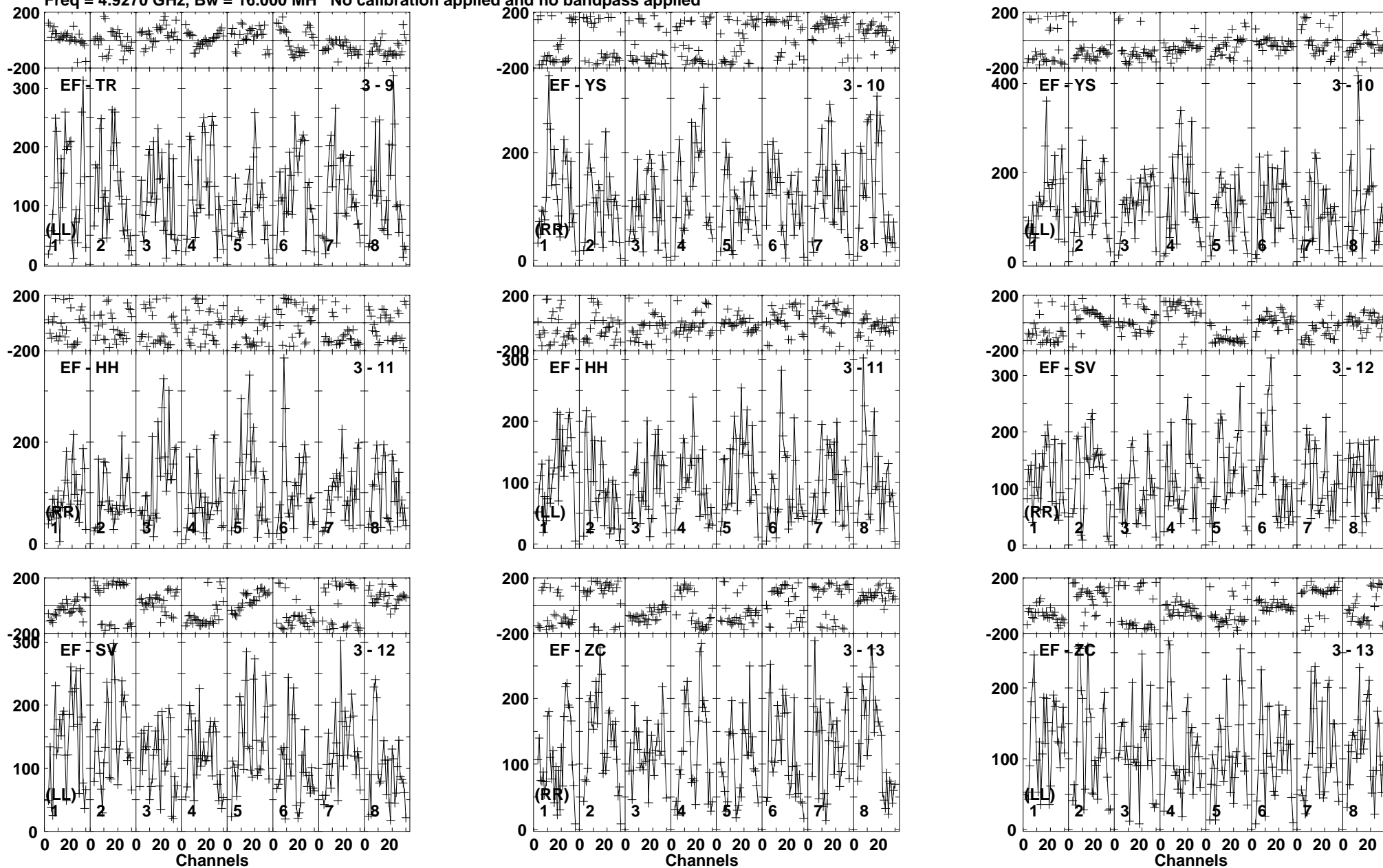
Lower frame: Micro Ampl Jy Top frame: Phas deg Vector averaged cross-power spectrum Baseline: EF (03) - TR (09) Timerange: 00/11:50:31 to 00/11:53:29
