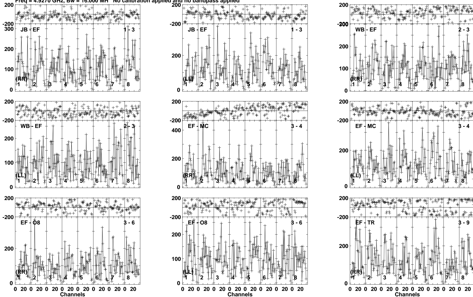
Lower frame: Micro Ampl Jy Top frame: Phas deg Vector averaged cross-power spectrum Baseline: JB (01) - EF (03) Timerange: 00/11:58:01 to 00/12:00:59
