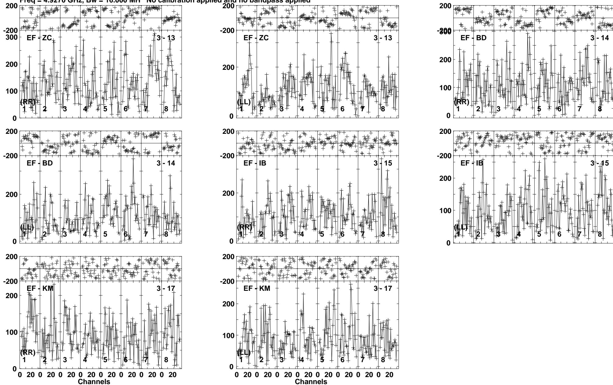
Lower frame: Micro Ampl Jy Top frame: Phas deg Vector averaged cross-power spectrum Baseline: EF (03) - ZC (13) Timerange: 00/08:50:31 to 00/08:53:29
