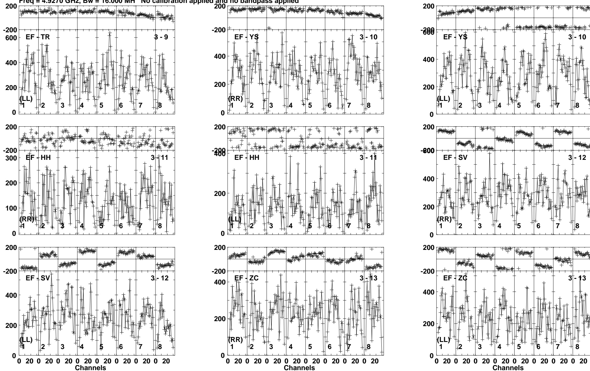
Lower frame: Micro Ampl Jy Top frame: Phas deg Vector averaged cross-power spectrum Baseline: EF (03) - TR (09) Timerange: 00/15:03:01 to 00/15:04:59
