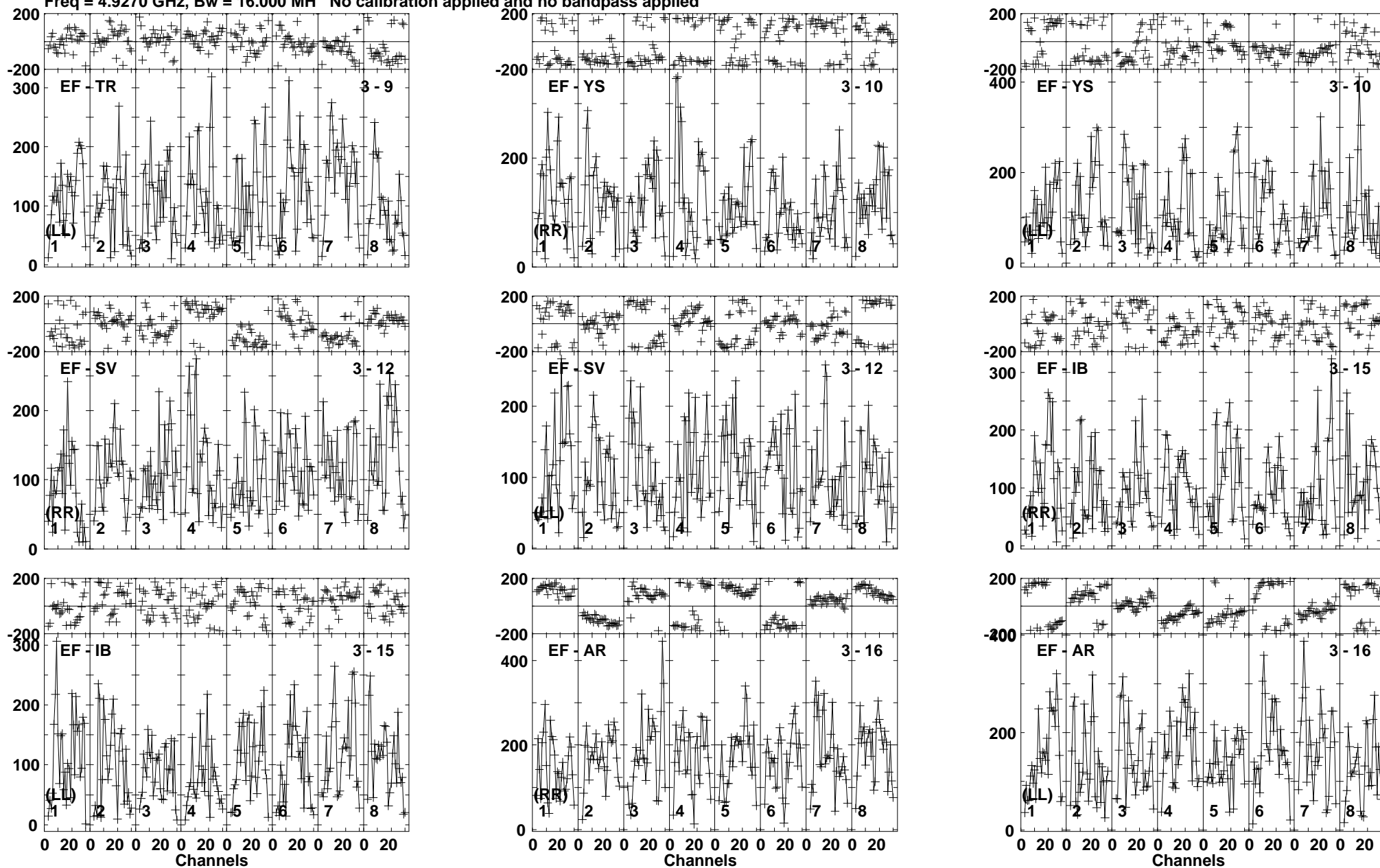
Lower frame: Micro Ampl Jy Top frame: Phas deg Vector averaged cross-power spectrum Baseline: EF (03) - TR (09) Timerange: 00/18:06:01 to 00/18:08:59
