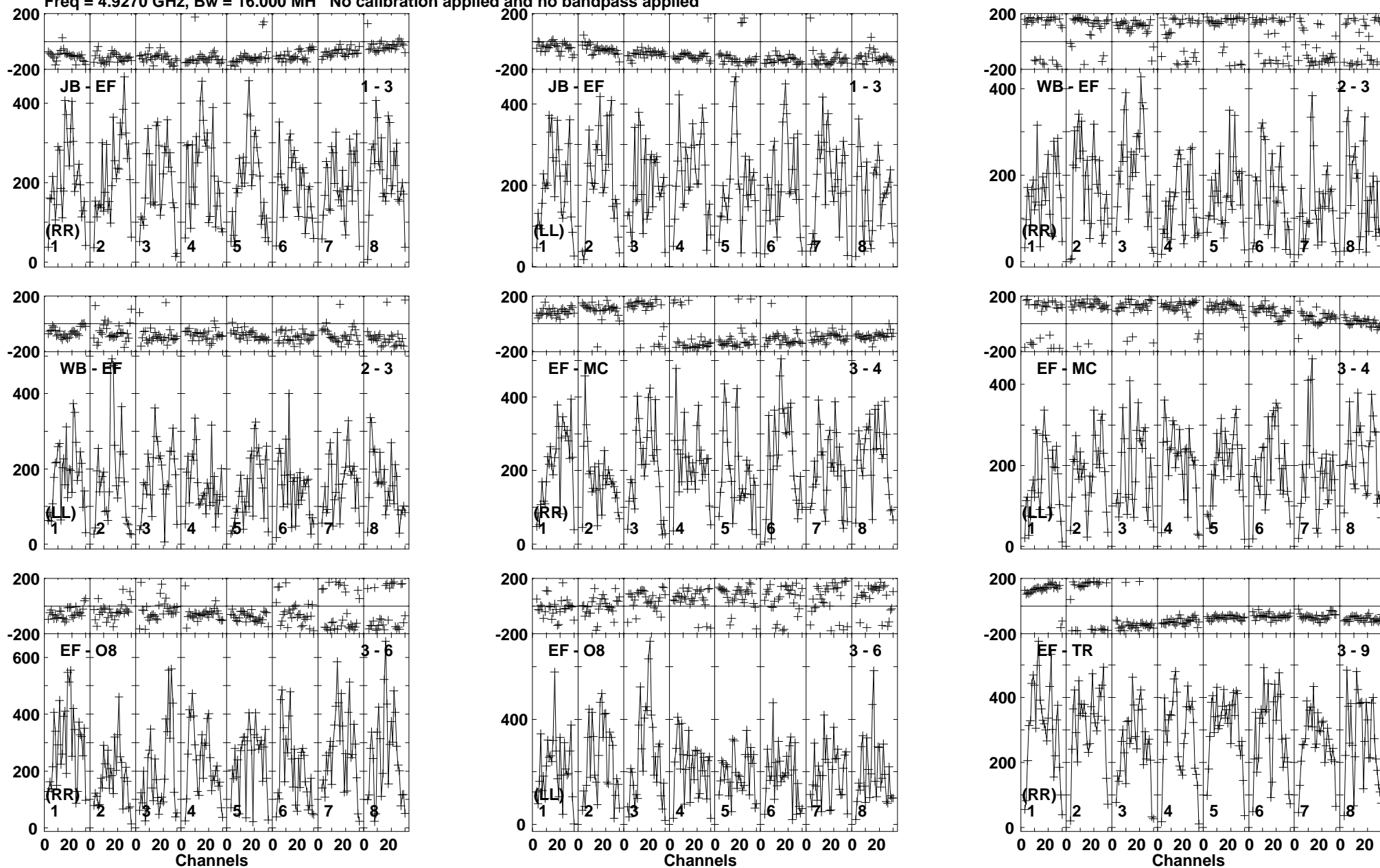
Lower frame: Micro Ampl Jy Top frame: Phas deg Vector averaged cross-power spectrum Baseline: JB (01) - EF (03) Timerange: 00/15:23:01 to 00/15:24:59
