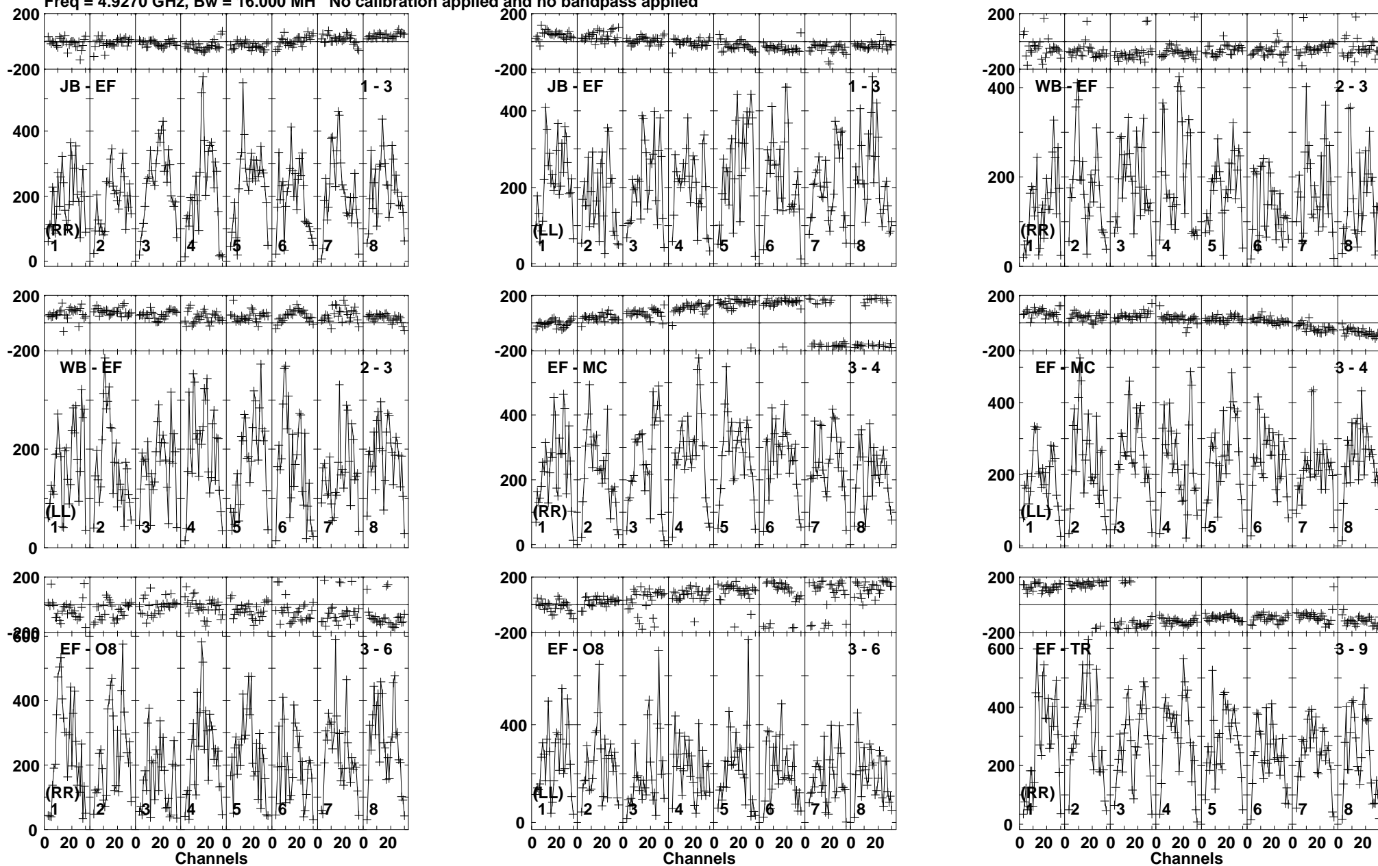
Lower frame: Micro Ampl Jy Top frame: Phas deg Vector averaged cross-power spectrum Baseline: JB (01) - EF (03) Timerange: 00/14:43:01 to 00/14:44:59
