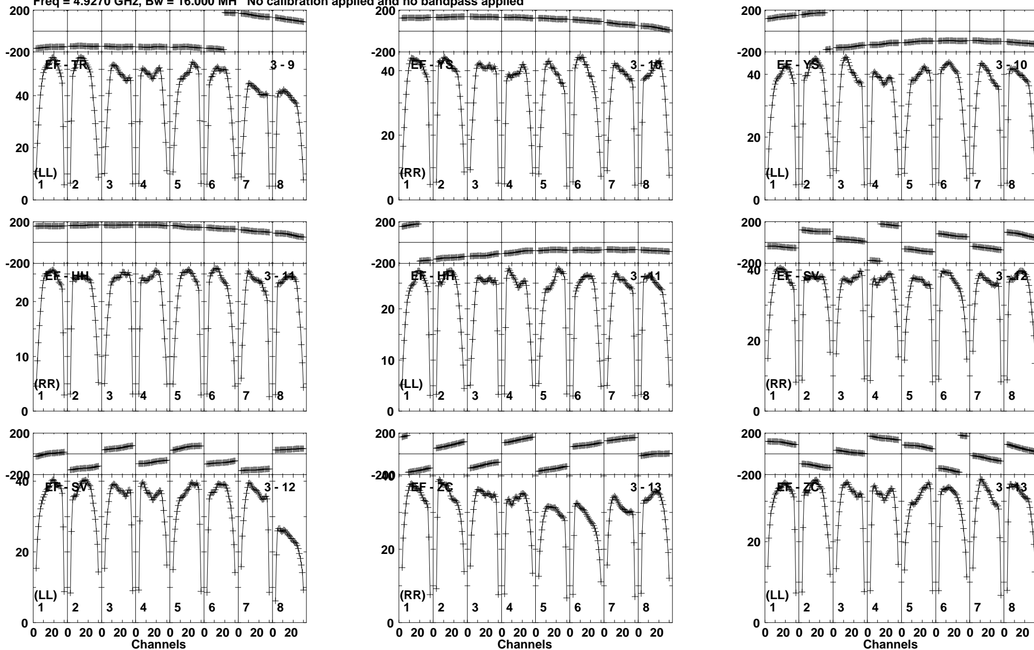
Lower frame: Milli Amply Jy Top frame: Phas deg Vector averaged cross-power spectrum Baseline: EF (03) - TR (09) Timerange: 00/13:08:31 to 00/13:11:29
