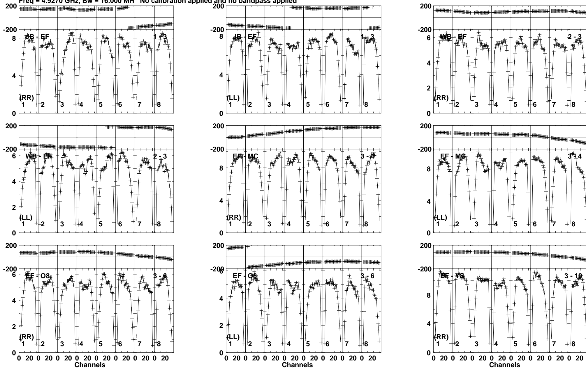
Lower frame: Milli Ampl Jy Top frame: Phas deg Vector averaged cross-power spectrum Baseline: JB (01) - EF (03) Timerange: 00:18:45:01 to 00:18:45:59
