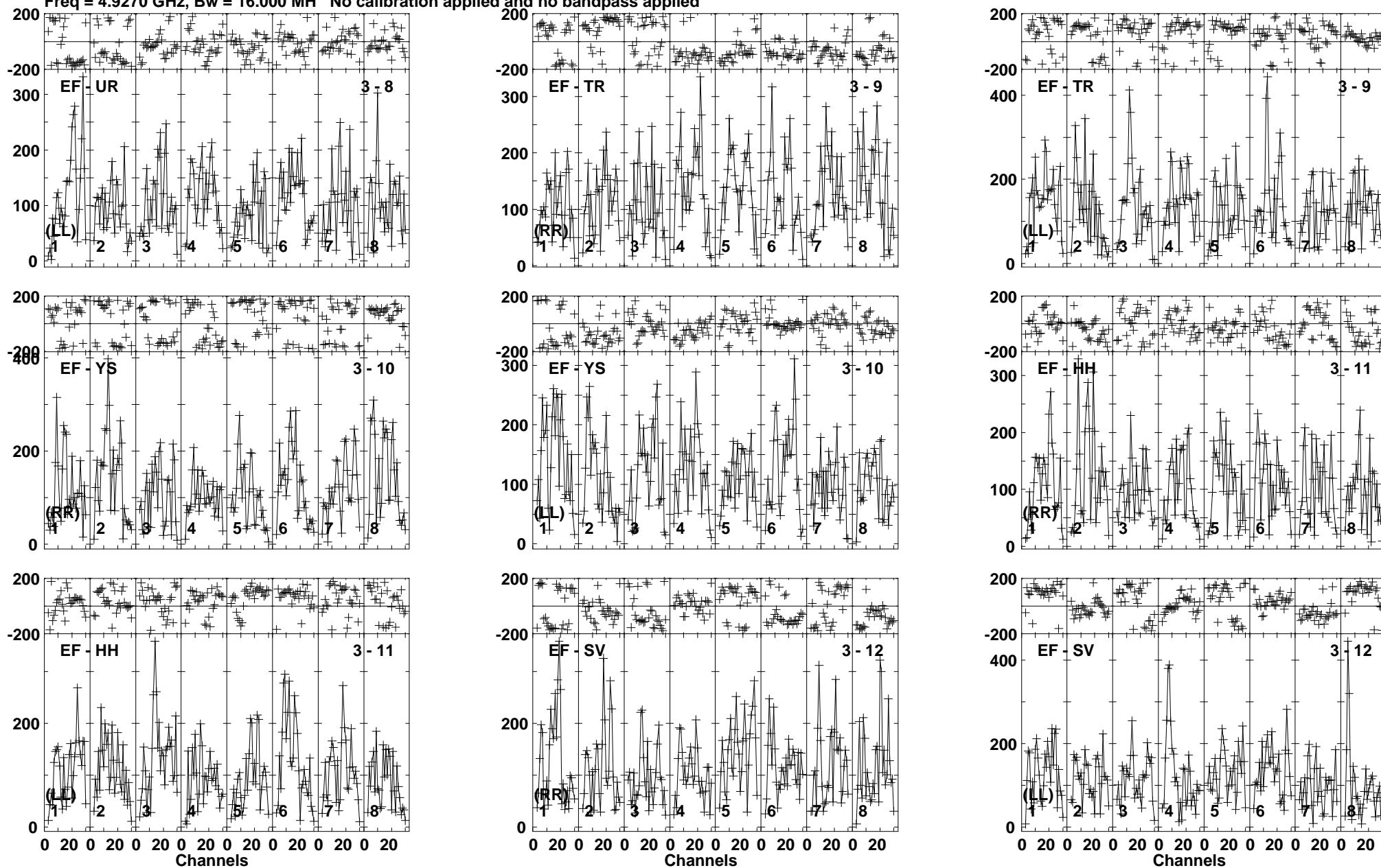
Lower frame: Micro Ampl Jy Top frame: Phas deg Vector averaged cross-power spectrum Baseline: EF (03) - UR (08) Timerange: 00/09:30:31 to 00/09:33:29
