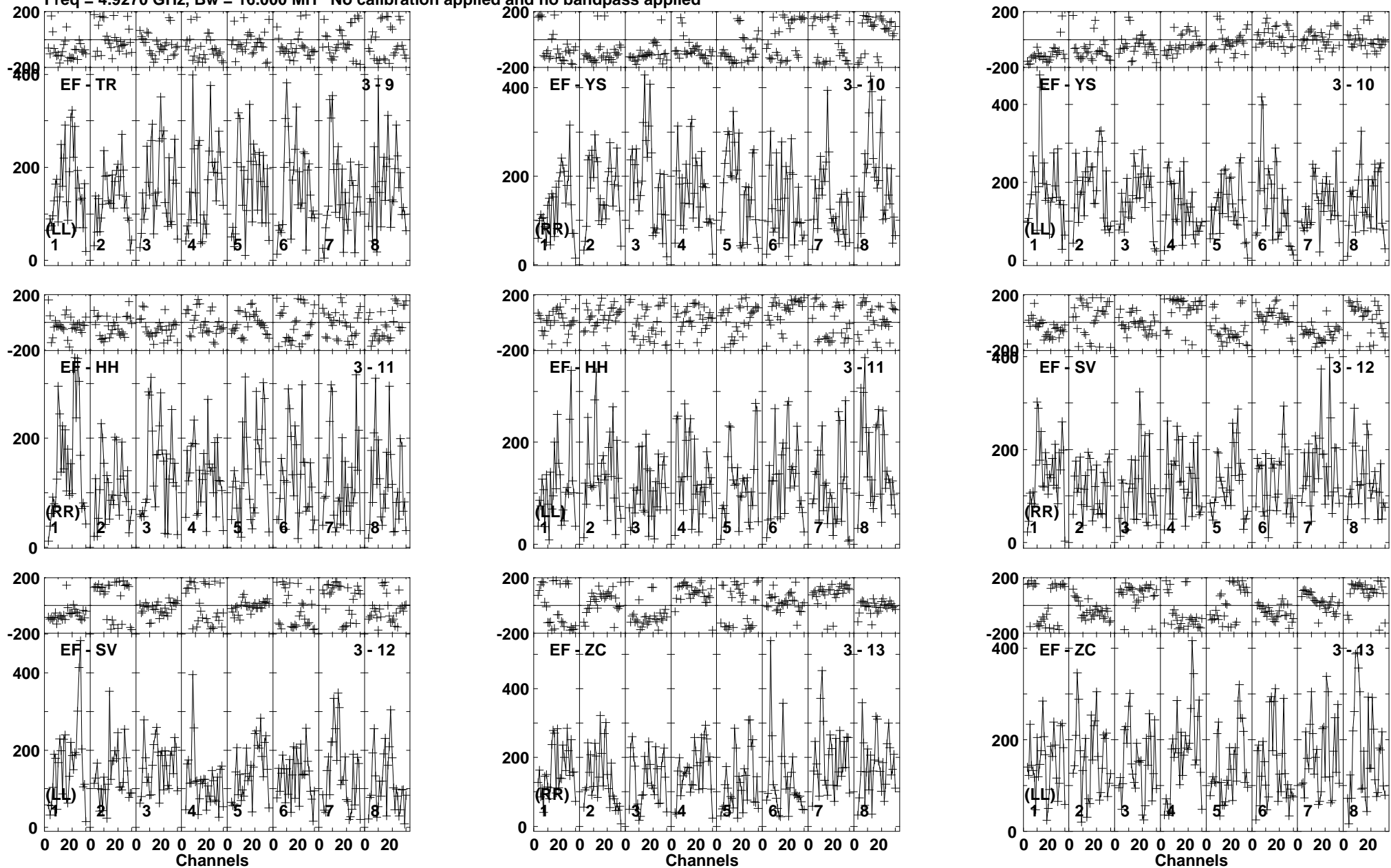
Lower frame: Micro Ampl Jy Top frame: Phas deg Vector averaged cross-power spectrum Baseline: EF (03) - TR (09) Timerange: 00/13:02:01 to 00/13:03:59
