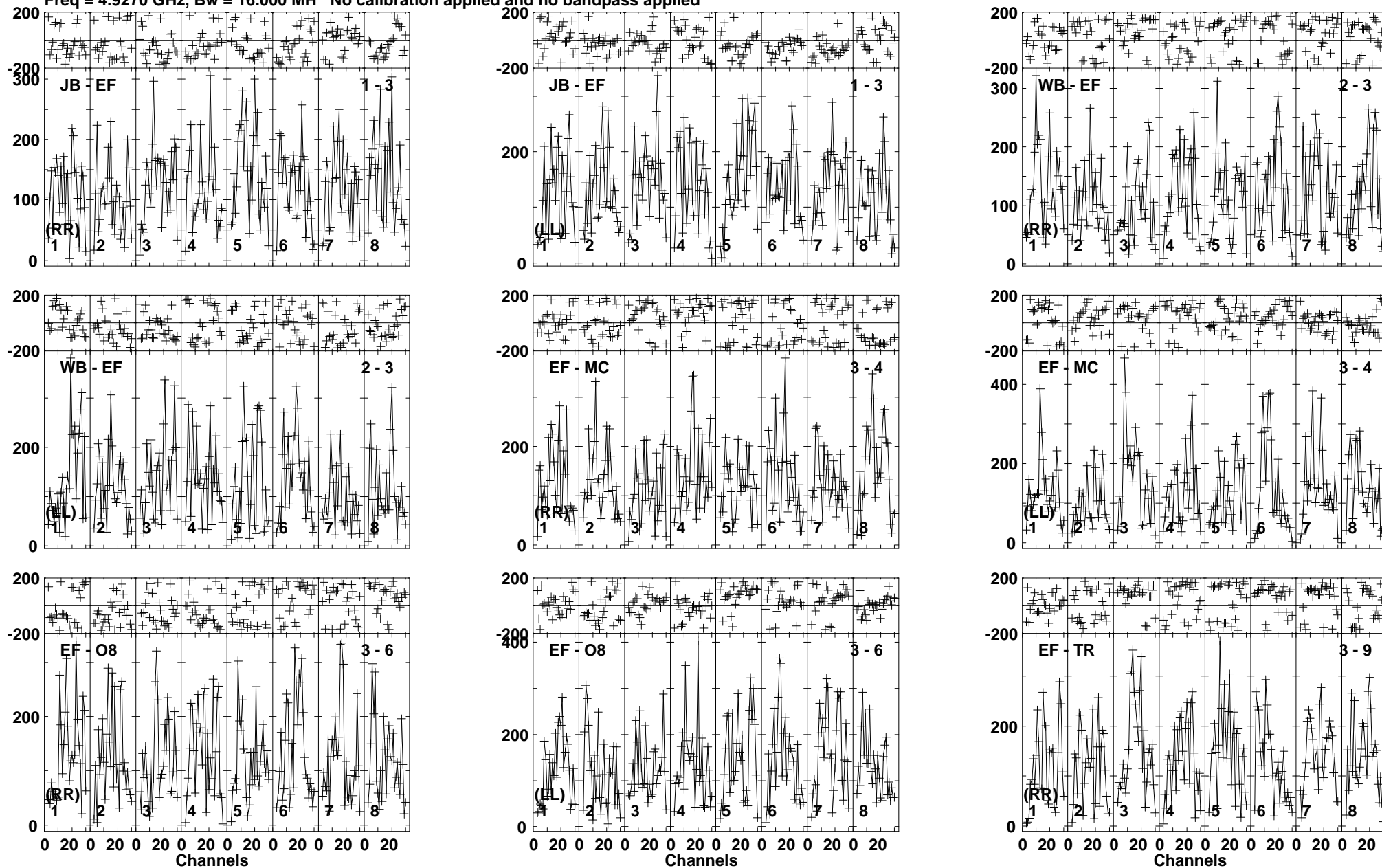
Lower frame: Micro Ampl Jy Top frame: Phas deg Vector averaged cross-power spectrum Baseline: JB (01) - EF (03) Timerange: 00:18:10:01 to 00:18:11:59
