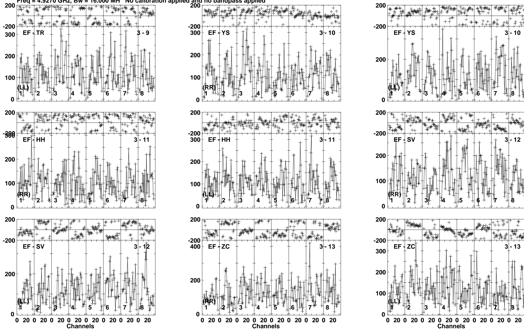
Lower frame: Micro Ampl Jy Top frame: Phas deg Vector averaged cross-power spectrum Baseline: EF (03) - TR (09) Timerange: 00/14:26:01 to 00/14:28:59
