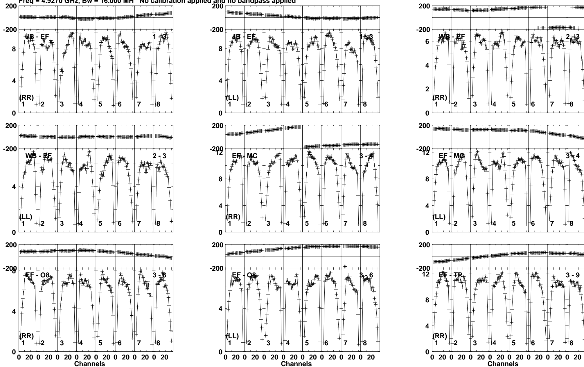
Lower frame: Milli Ampl Jy Top frame: Phas deg Vector averaged cross-power spectrum Baseline: JB (01) - EF (03) Timerange: 00:12:57:01 to 00:12:57:59
