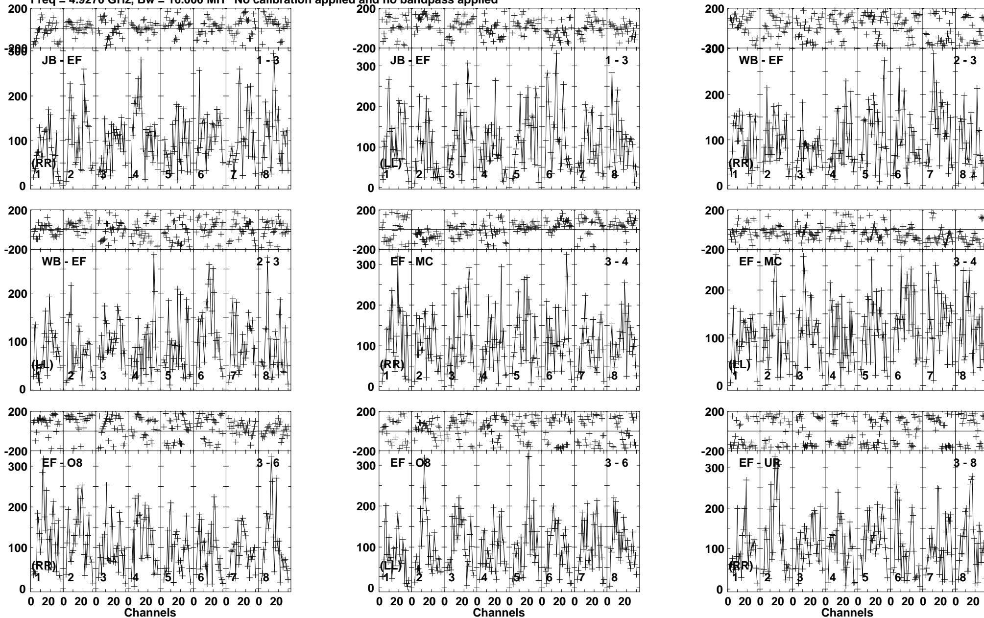
Lower frame: Micro Ampl Jy Top frame: Phas deg Vector averaged cross-power spectrum Baseline: JB (01) - EF (03) Timerange: 00/08:58:01 to 00/09:00:59
