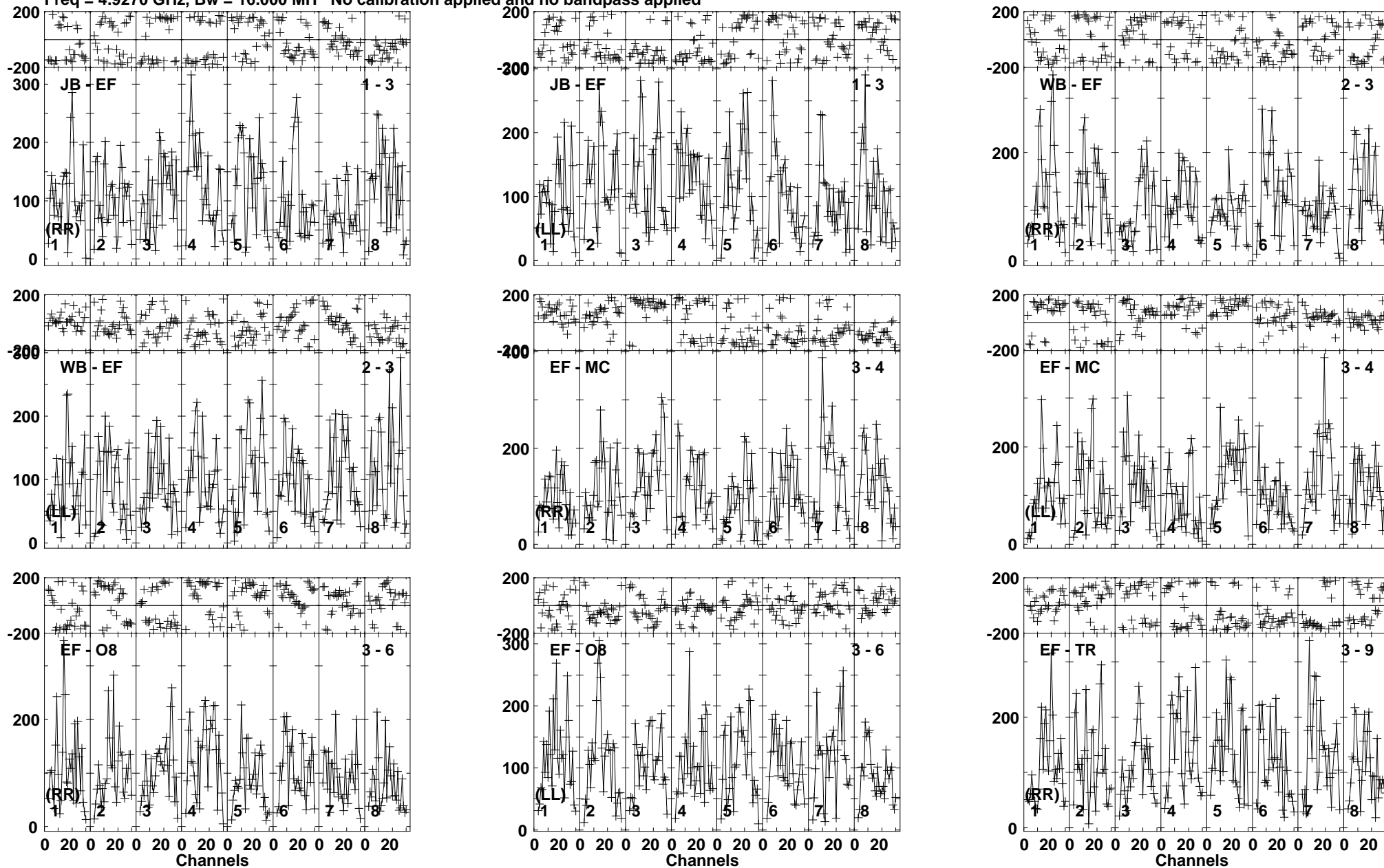
Lower frame: Micro Ampl Jy Top frame: Phas deg Vector averaged cross-power spectrum Baseline: JB (01) - EF (03) Timerange: 00/16:06:01 to 00/16:08:59
