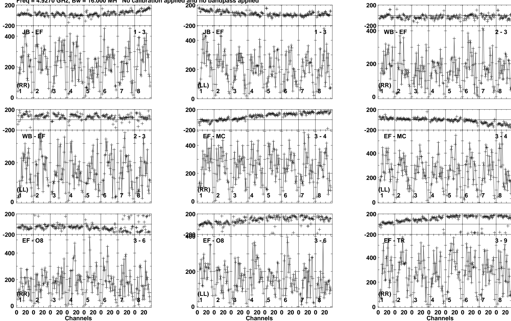
Lower frame: Micro Ampl Jy Top frame: Phas deg Vector averaged cross-power spectrum Baseline: JB (01) - EF (03) Timerange: 00/16:23:01 to 00/16:24:59
