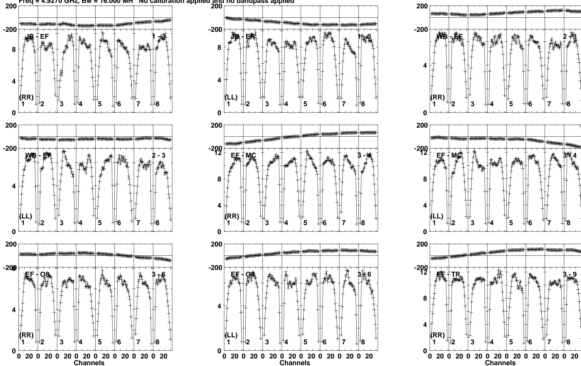
Lower frame: Milli Ampl Jy Top frame: Phas deg Vector averaged cross-power spectrum Baseline: JB (01) - EF (03) Timerange: 00/11:57:01 to 00/11:57:59
