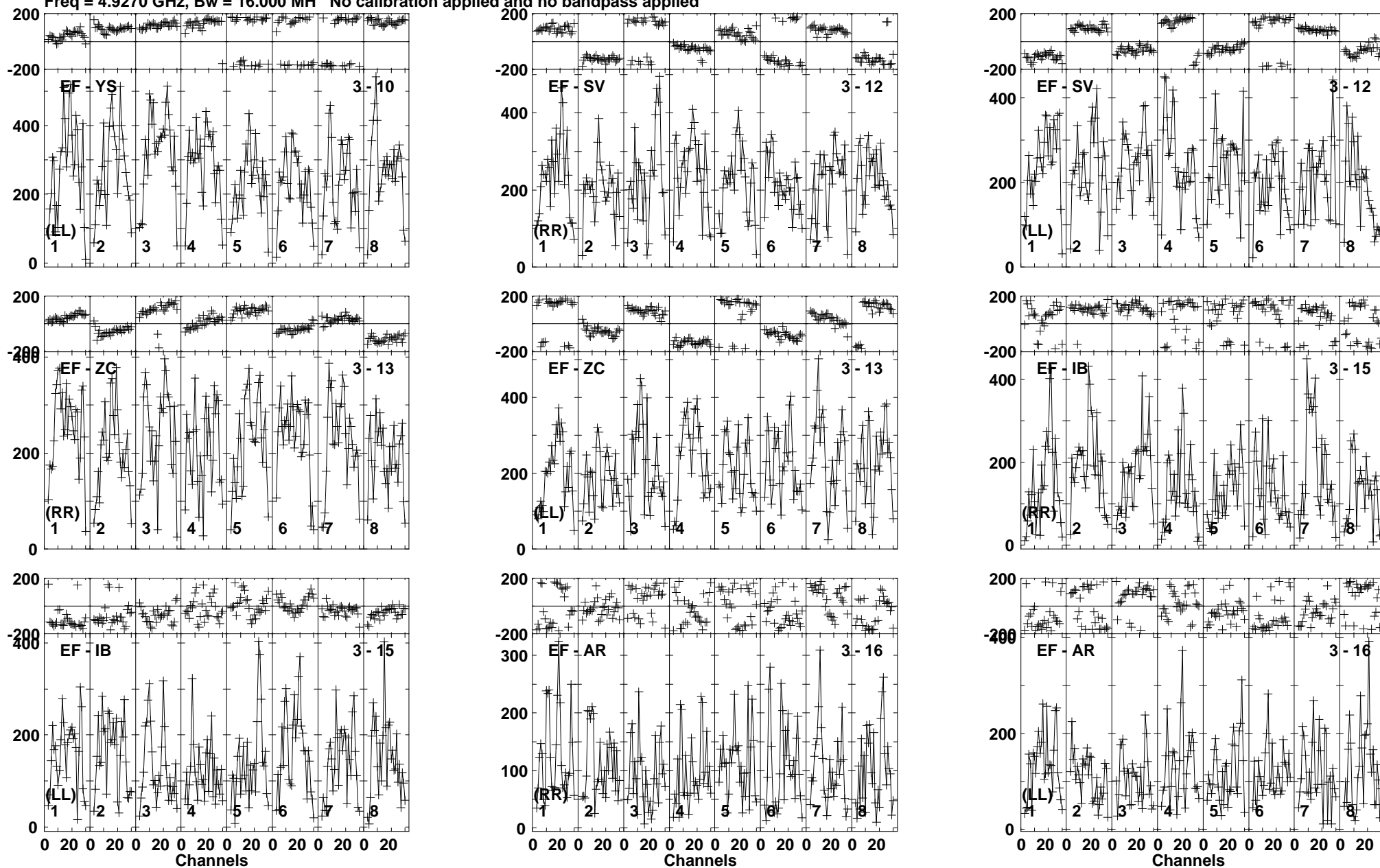
Lower frame: Micro Ampl Jy Top frame: Phas deg Vector averaged cross-power spectrum Baseline: EF (03) - YS (10) Timerange: 00:17:43:01 to 00:17:44:59
