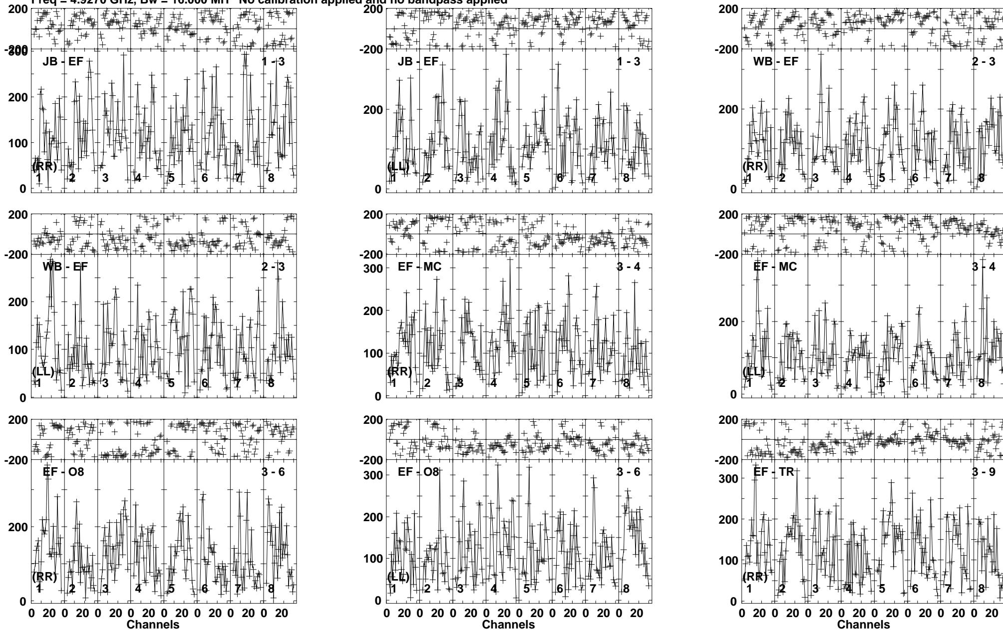
Lower frame: Micro Ampl Jy Top frame: Phas deg Vector averaged cross-power spectrum Baseline: JB (01) - EF (03) Timerange: 00/14:26:01 to 00/14:28:59
