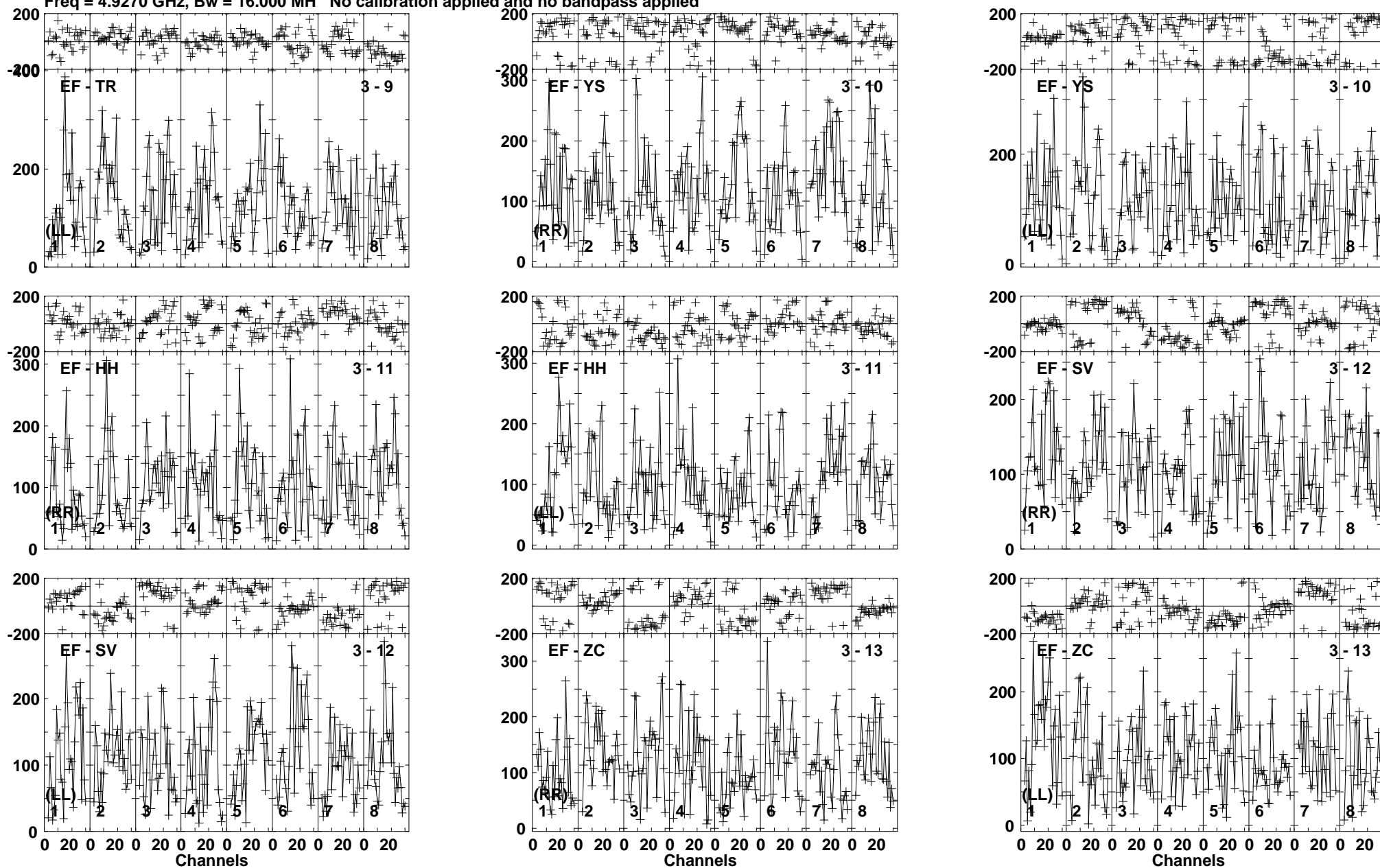
Lower frame: Micro Ampl Jy Top frame: Phas deg Vector averaged cross-power spectrum Baseline: EF (03) - TR (09) Timerange: 00/16:38:31 to 00/16:41:29
