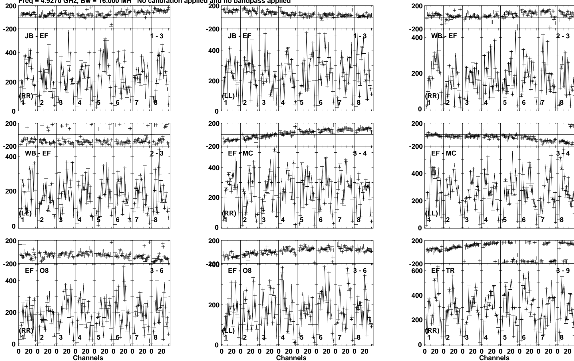
Lower frame: Micro Ampl Jy Top frame: Phas deg Vector averaged cross-power spectrum Baseline: JB (01) - EF (03) Timerange: 00/13:23:01 to 00/13:24:59
