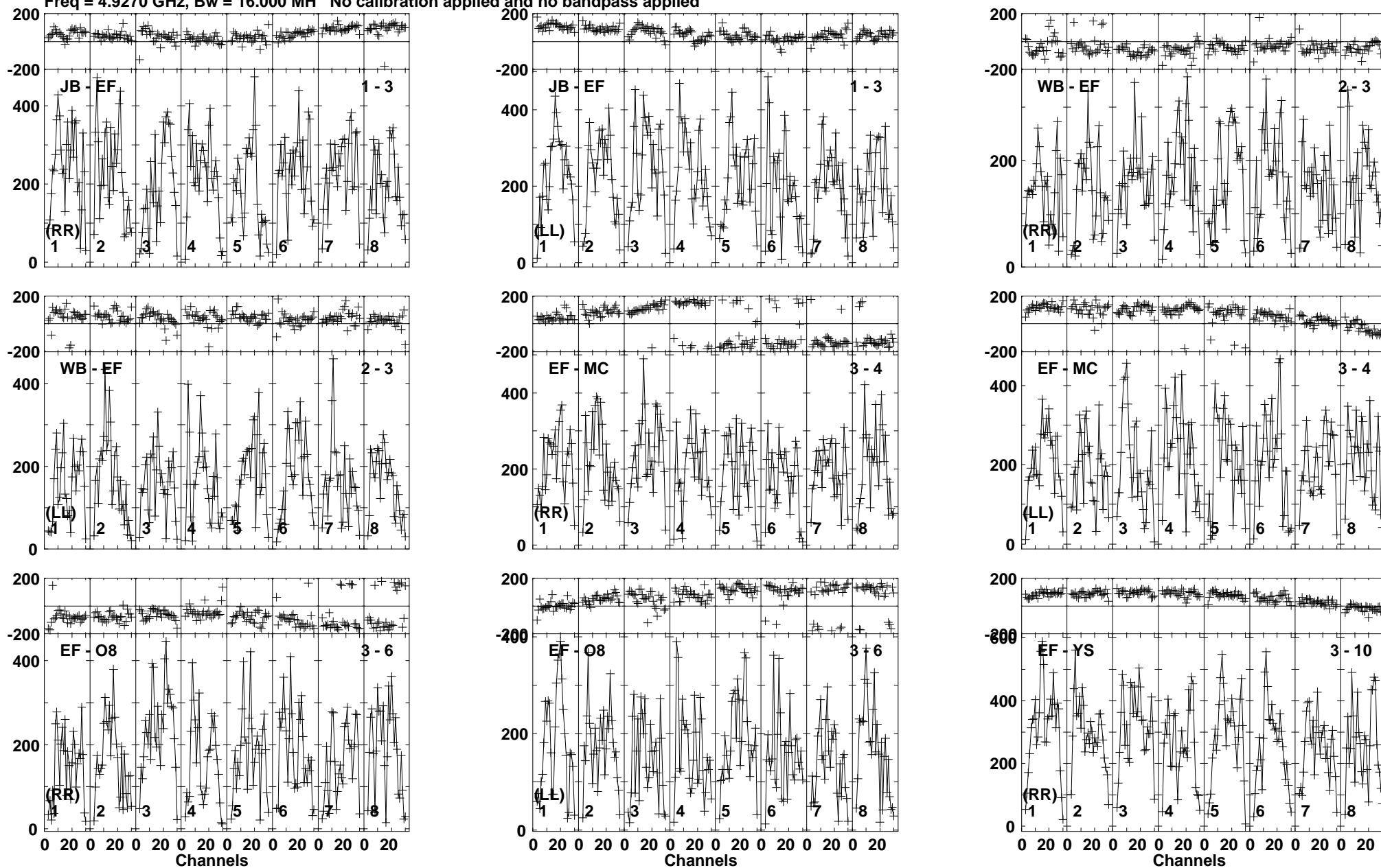
Lower frame: Micro Ampl Jy Top frame: Phas deg Vector averaged cross-power spectrum Baseline: JB (01) - EF (03) Timerange: 00/17:03:01 to 00/17:04:59
