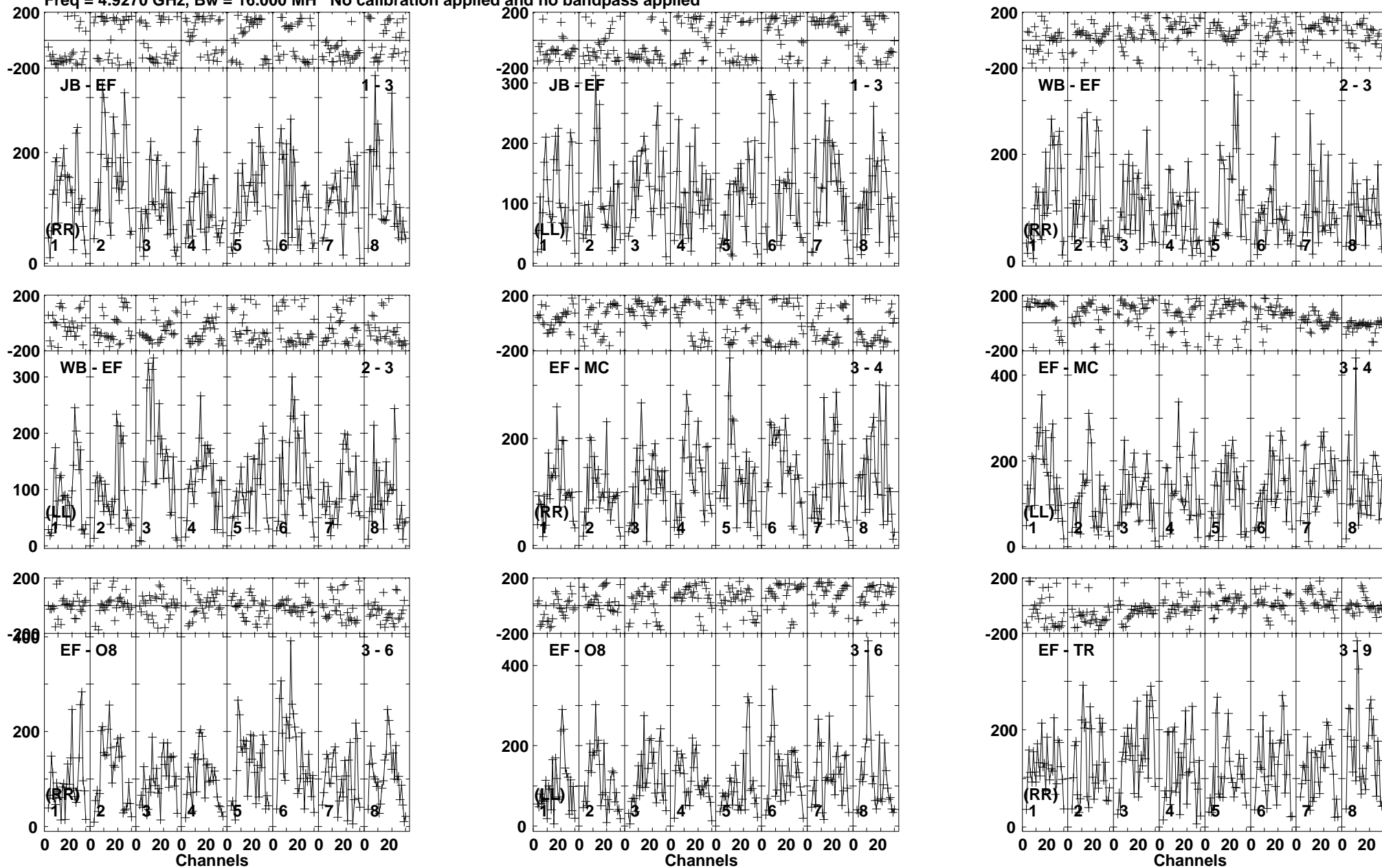
Lower frame: Micro Ampl Jy Top frame: Phas deg Vector averaged cross-power spectrum Baseline: JB (01) - EF (03) Timerange: 00/13:18:31 to 00/13:21:29
