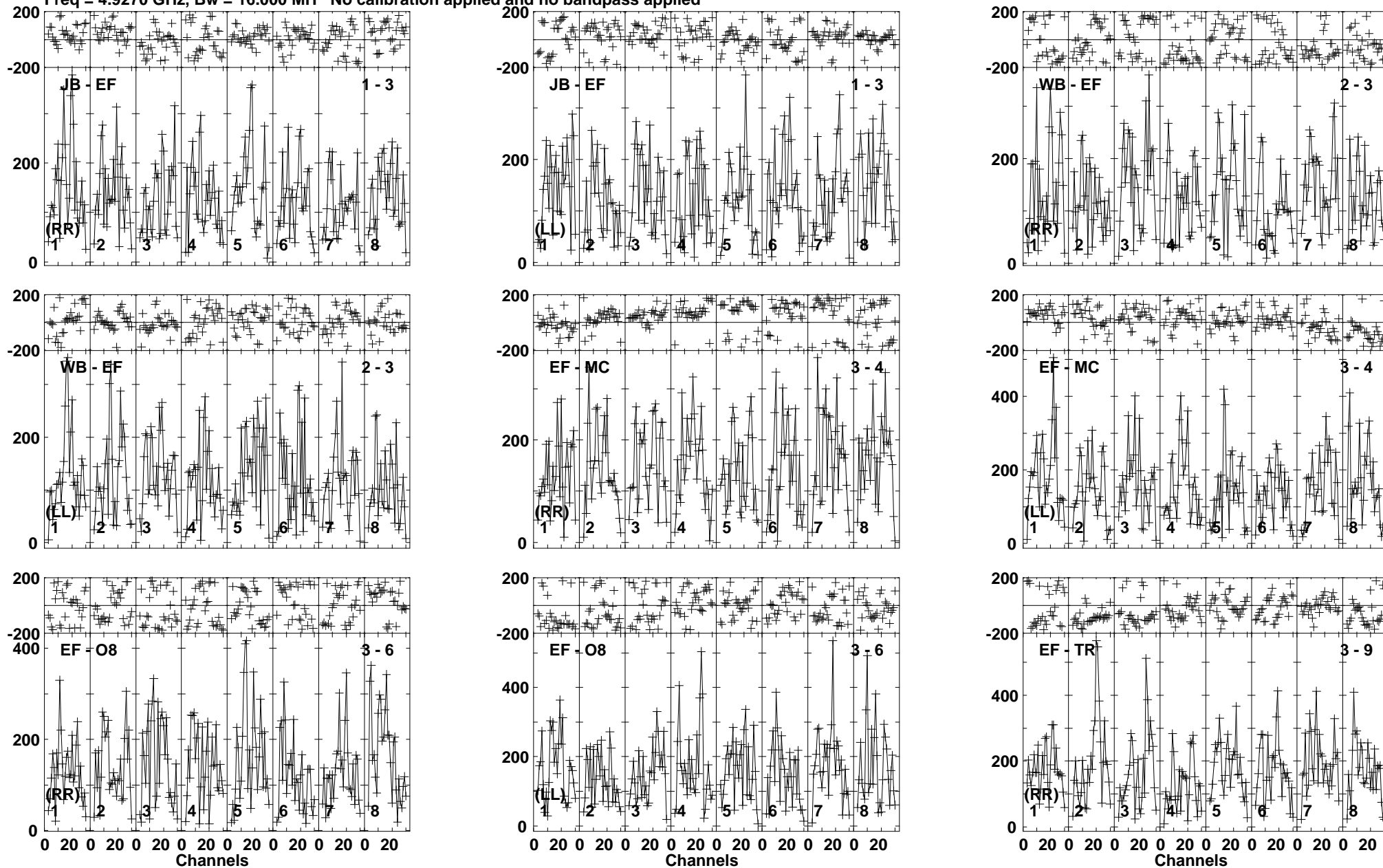
Lower frame: Micro Ampl Jy Top frame: Phas deg Vector averaged cross-power spectrum Baseline: JB (01) - EF (03) Timerange: 00/14:10:01 to 00/14:11:59
